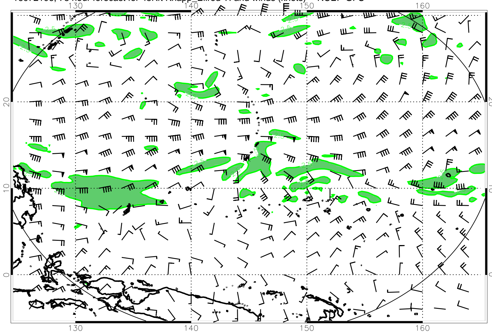
16072106, 78 hour forecast for 45Kft Knapp_Ellrod TI and winds (knots) -- NCEP GFS
