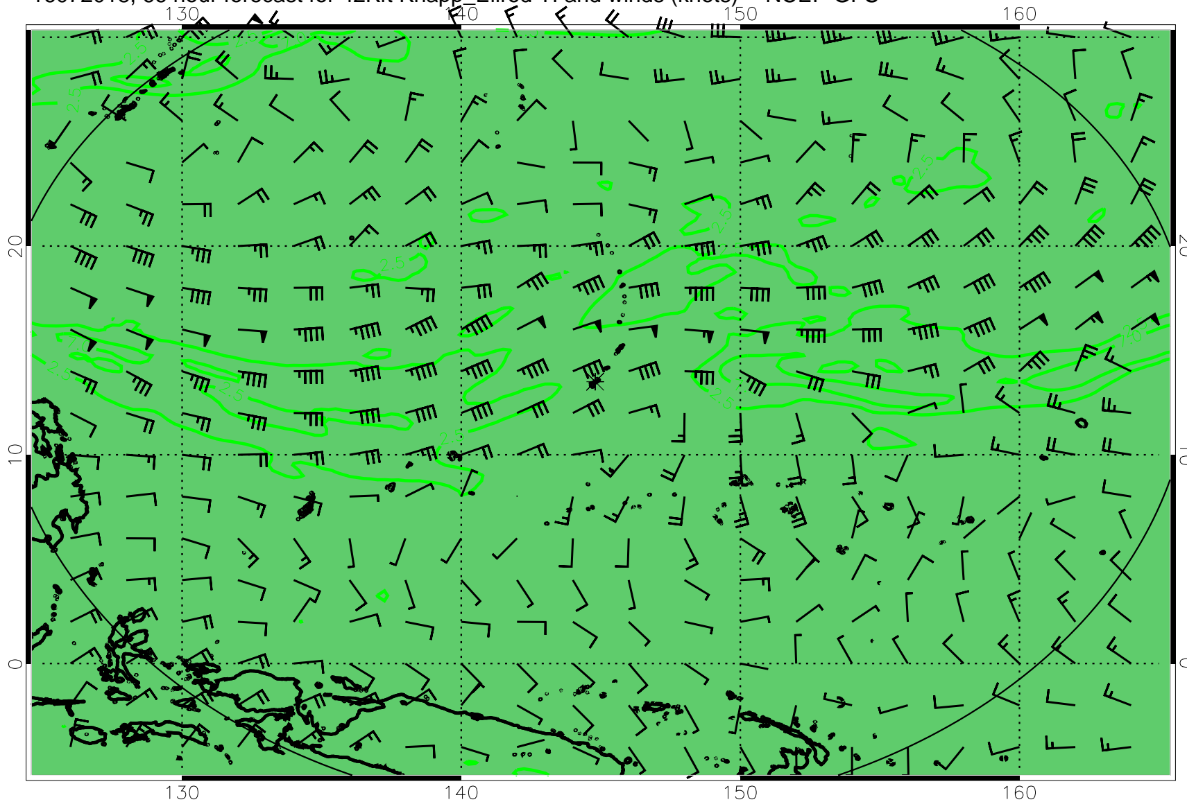
16072018, 66 hour forecast for 42Kft Knapp_Ellrod TI and winds (knots) -- NCEP GFS
