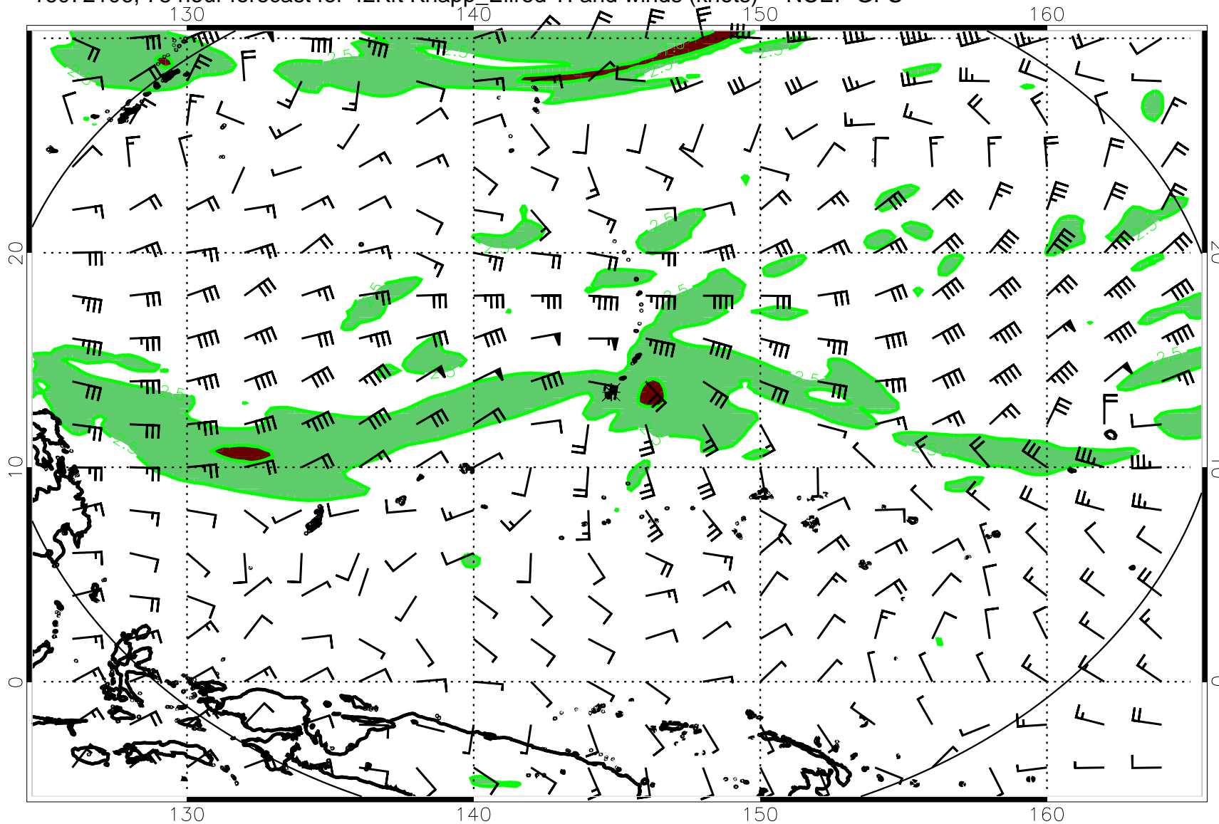
16072106, 78 hour forecast for 42Kft Knapp_Ellrod TI and winds (knots) -- NCEP GFS
