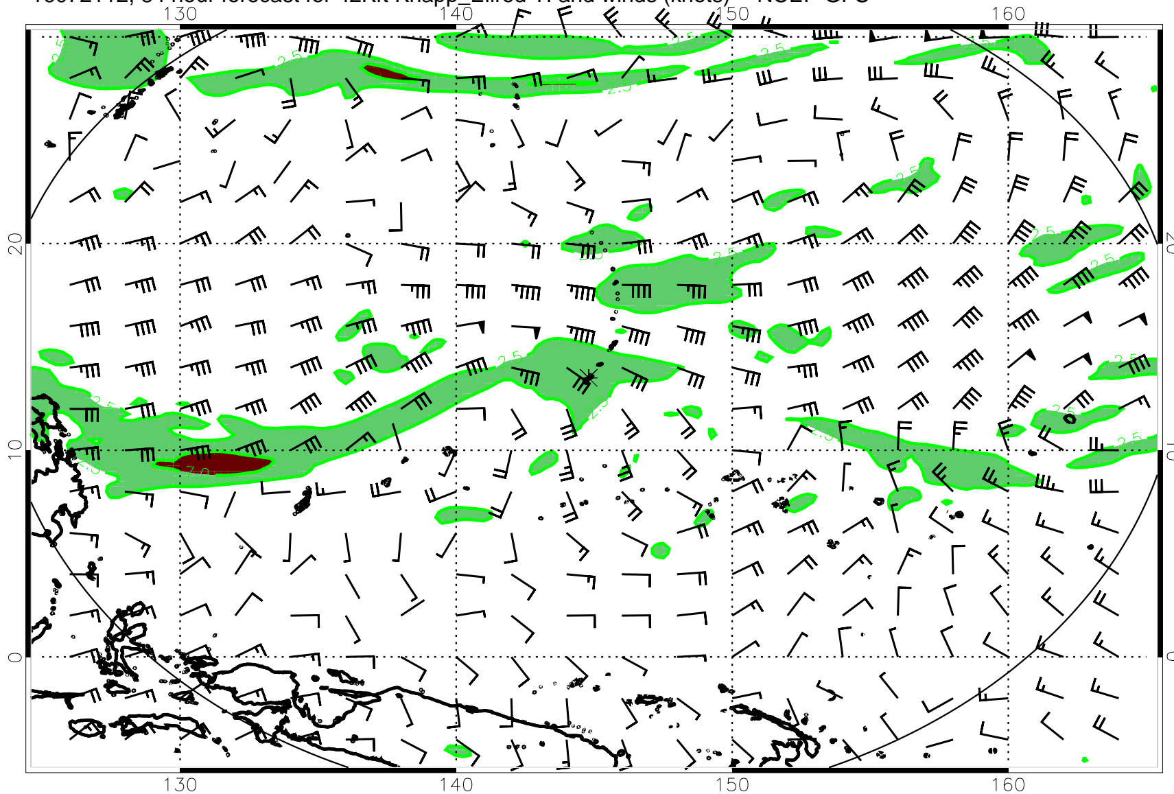
16072112, 84 hour forecast for 42Kft Knapp_Ellrod TI and winds (knots) -- NCEP GFS
