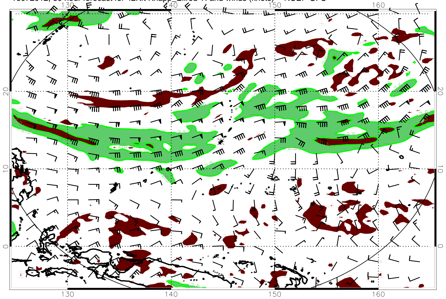
16072012, 60 hour forecast for 42Kft Knapp_Ellrod TI and winds (knots) -- NCEP GFS
