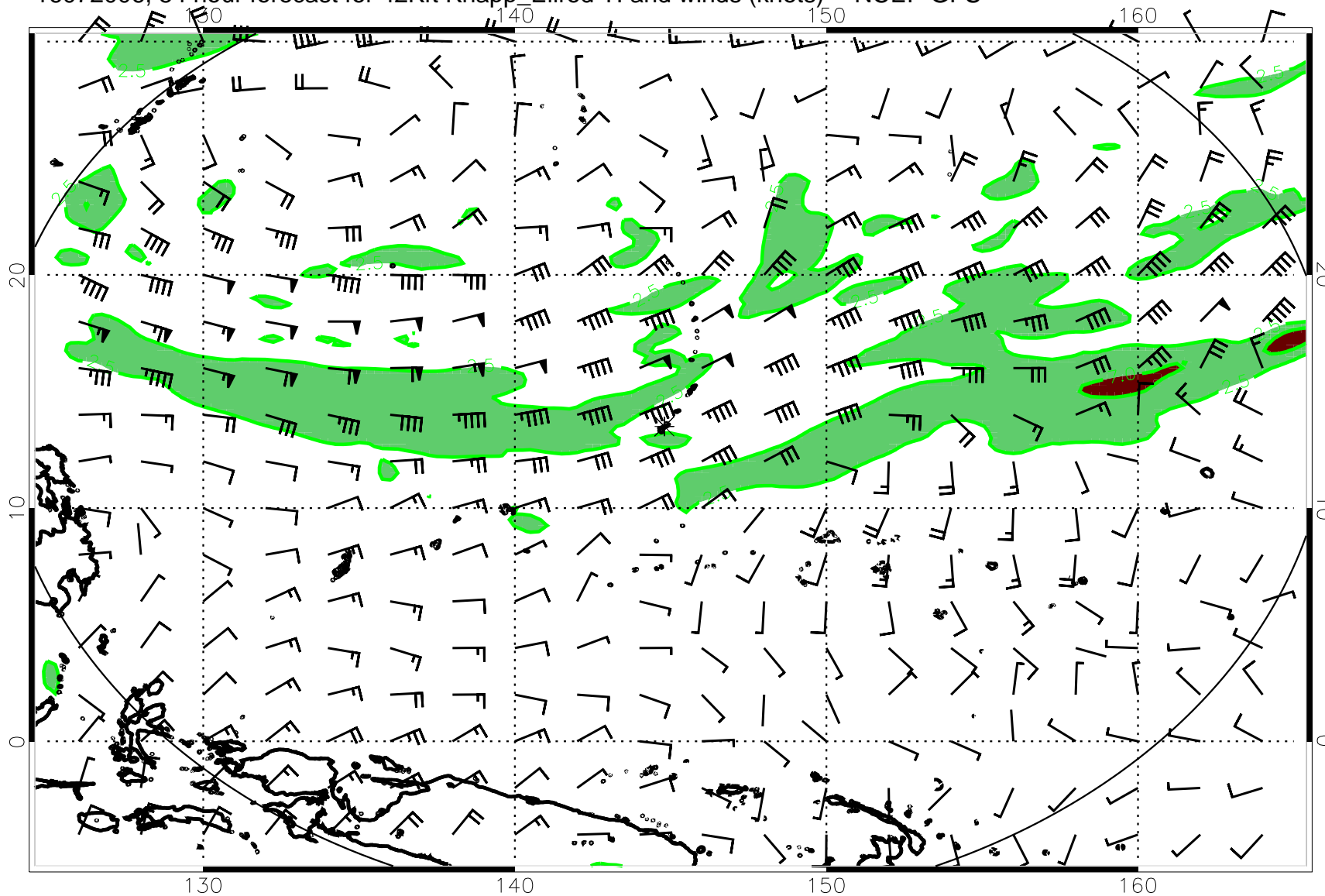
16072006, 54 hour forecast for 42Kft Knapp_Ellrod TI and winds (knots) -- NCEP GFS
