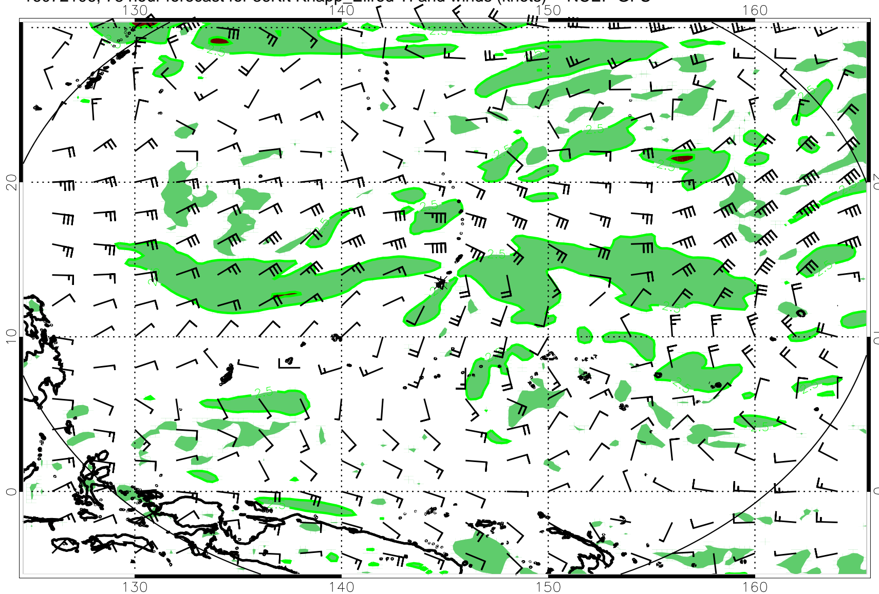
16072106, 78 hour forecast for 36Kft Knapp_Ellrod TI and winds (knots) -- NCEP GFS
