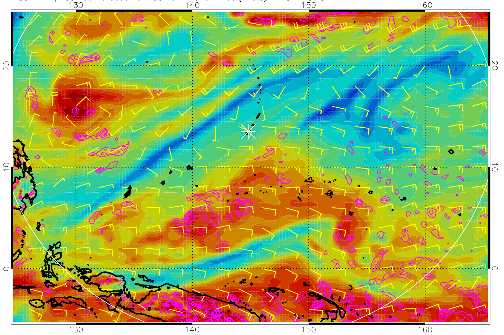
16072212, 108 hour forecast for 700mb RH and winds (knots) -- NCEP GFS
