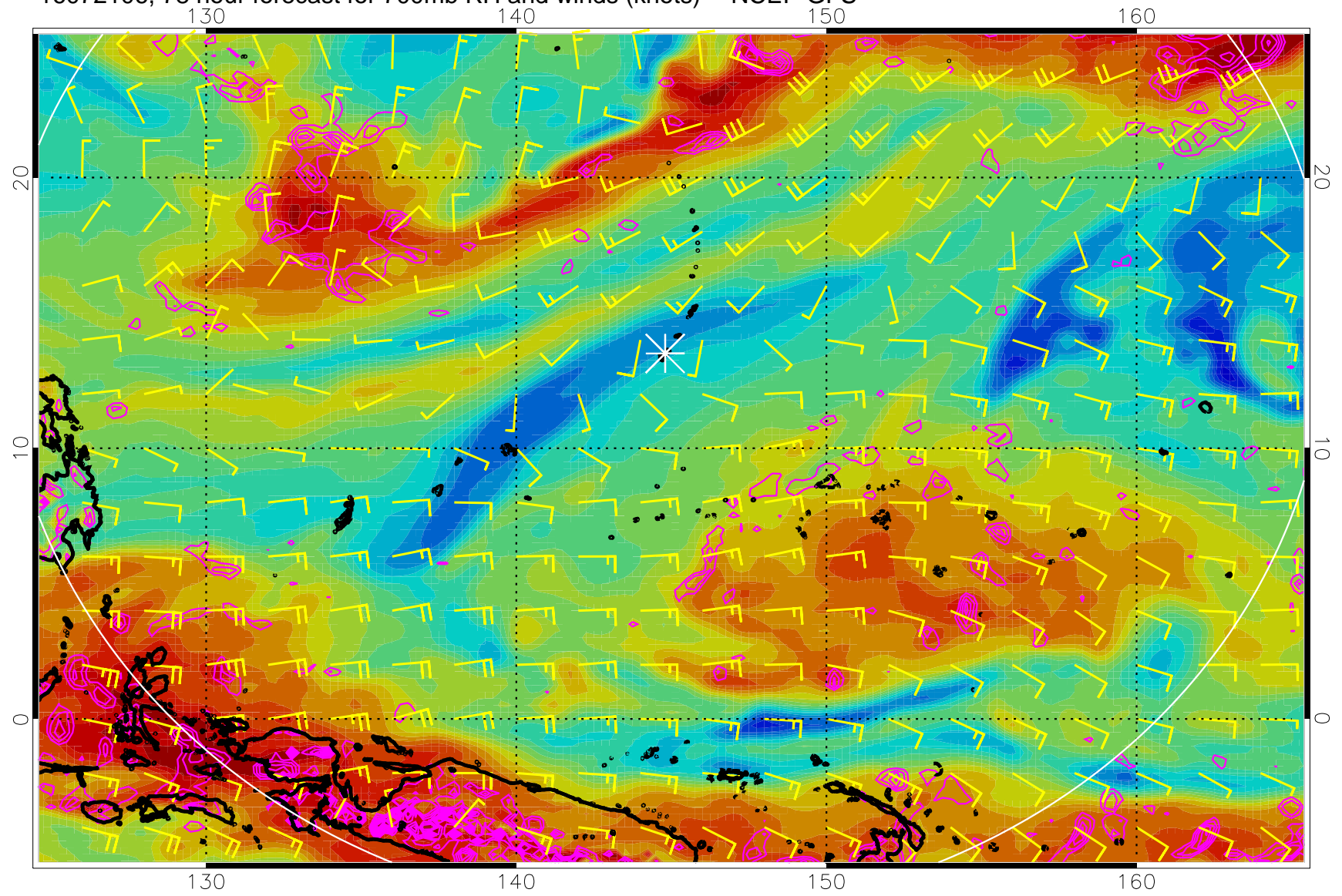
16072106, 78 hour forecast for 700mb RH and winds (knots) -- NCEP GFS
