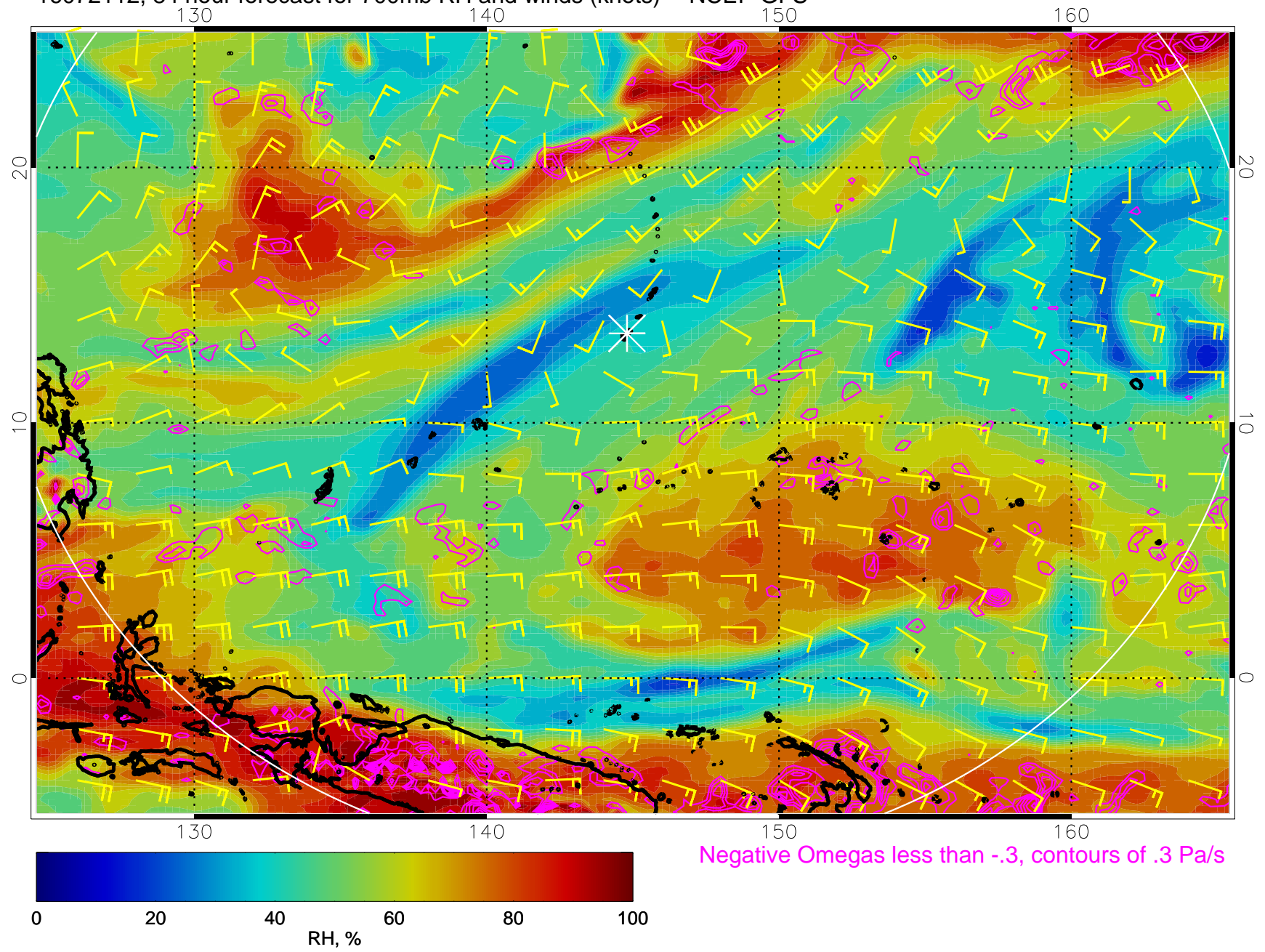
16072112, 84 hour forecast for 700mb RH and winds (knots) -- NCEP GFS
