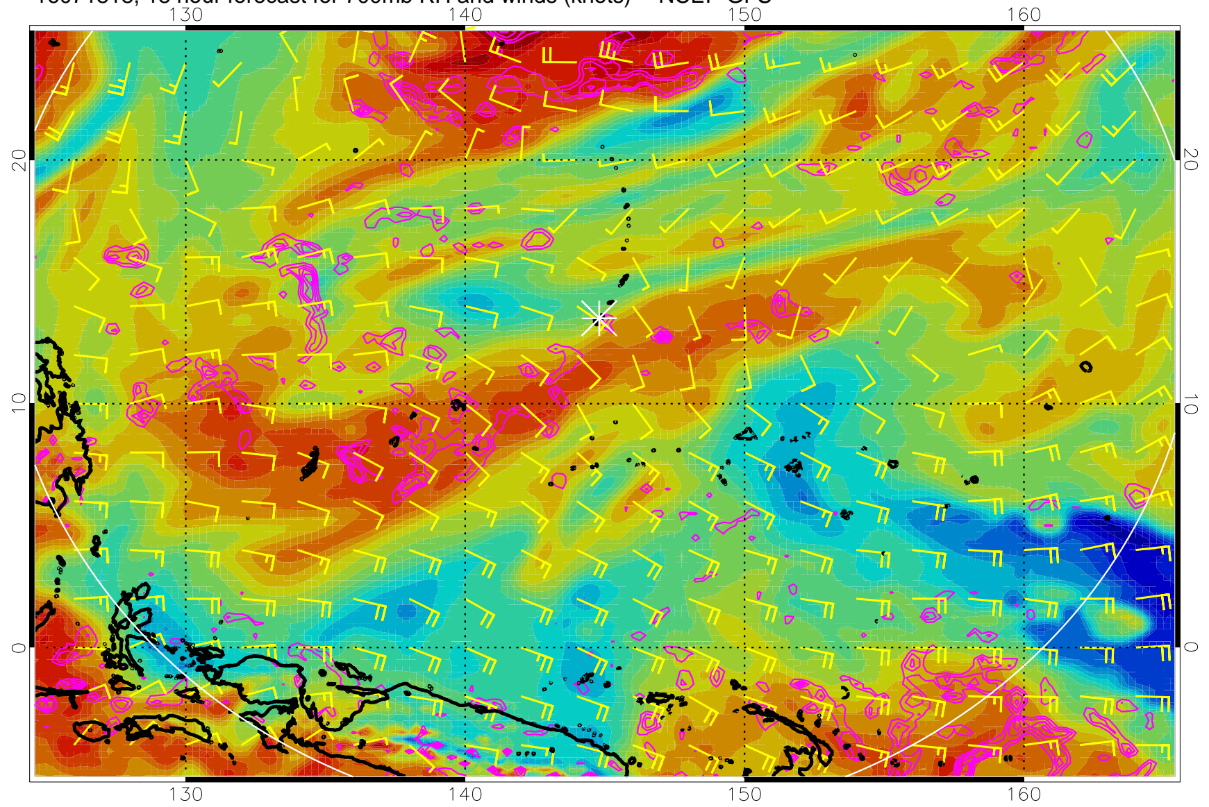
16071818, 18 hour forecast for 700mb RH and winds (knots) -- NCEP GFS
