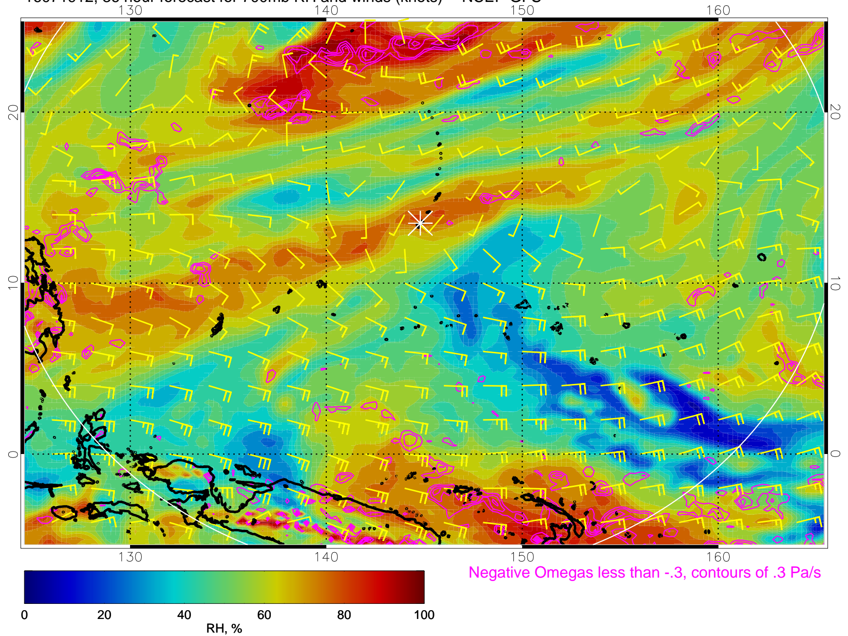
16071912, 36 hour forecast for 700mb RH and winds (knots) -- NCEP GFS
