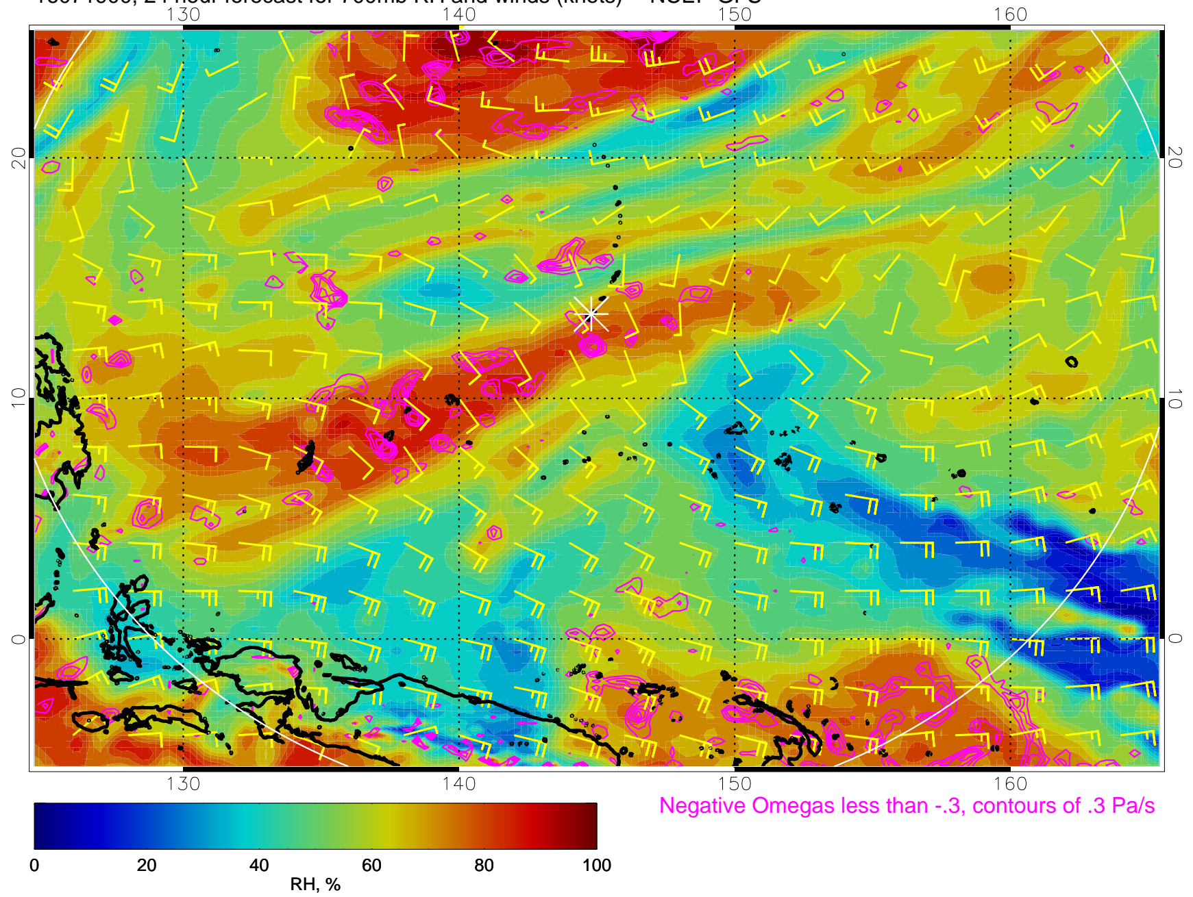
16071900, 24 hour forecast for 700mb RH and winds (knots) -- NCEP GFS
