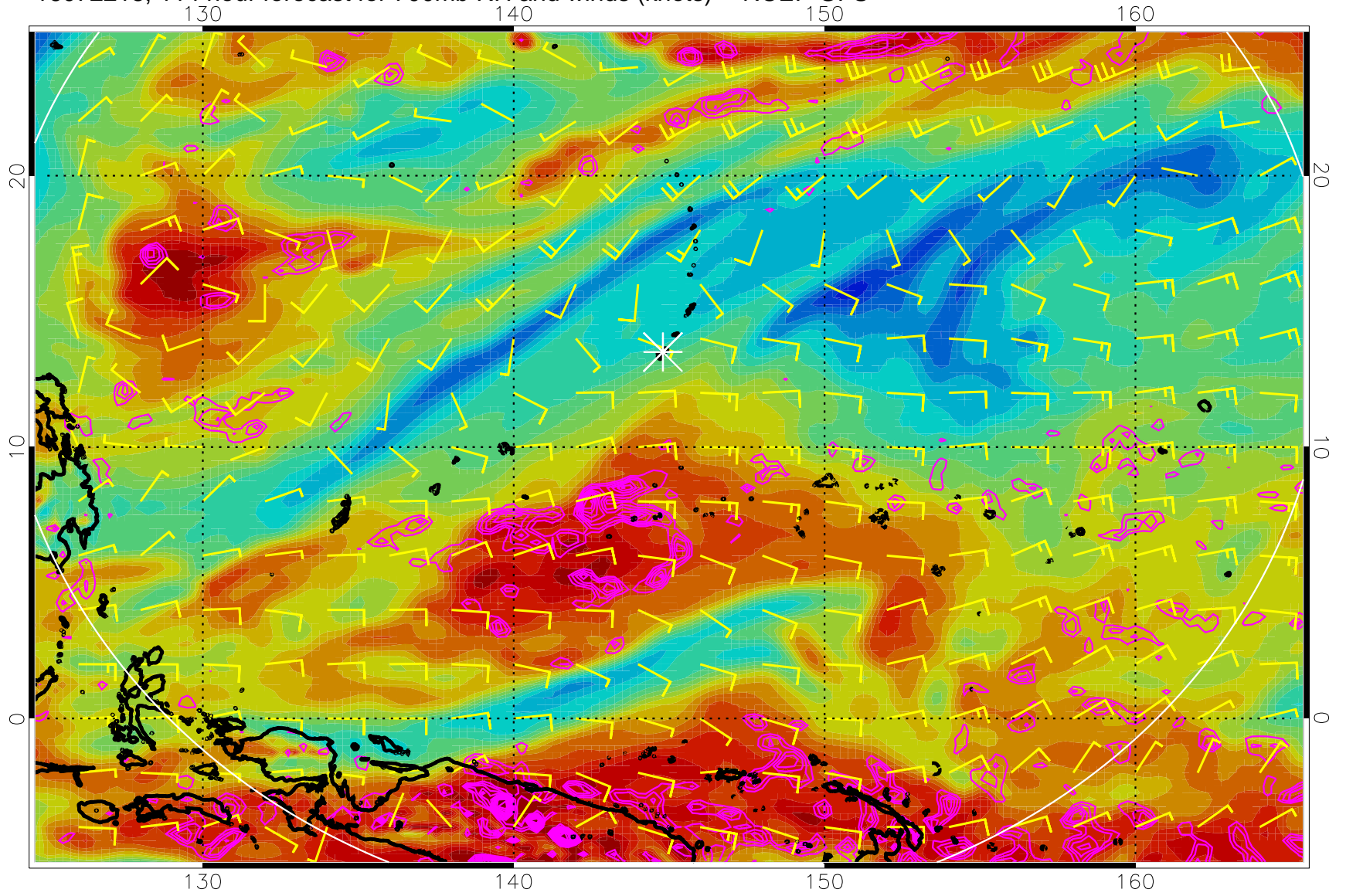
16072218, 114 hour forecast for 700mb RH and winds (knots) -- NCEP GFS
