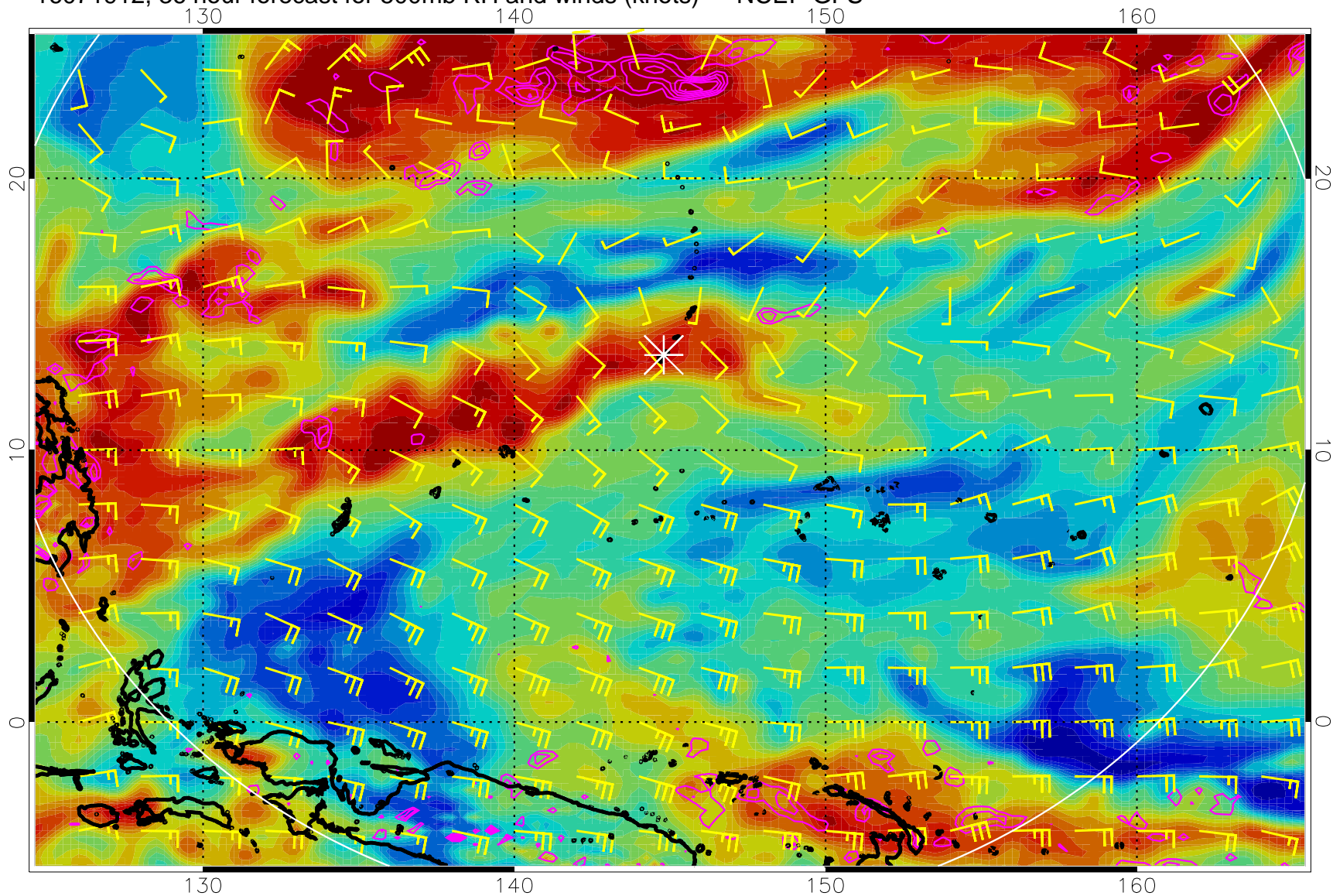
16071912, 36 hour forecast for 500mb RH and winds (knots) -- NCEP GFS
