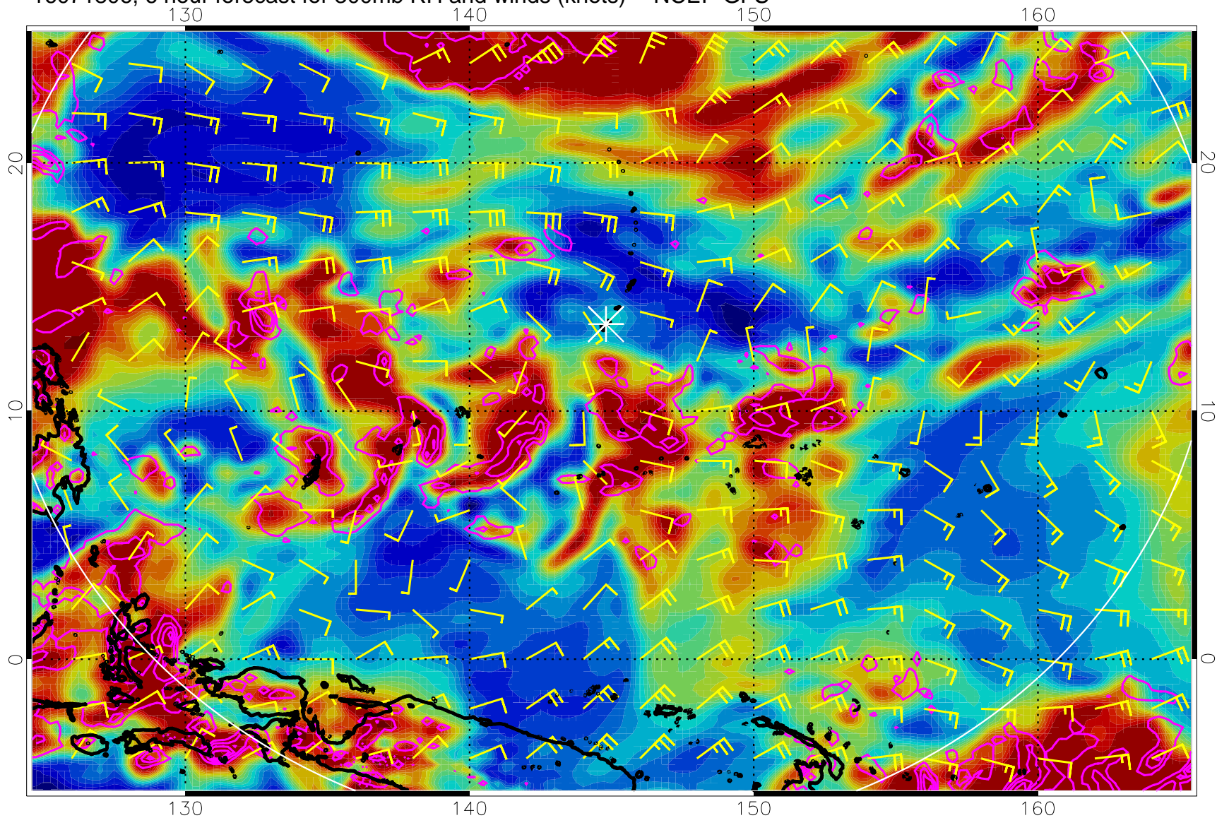
16071806, 6 hour forecast for 300mb RH and winds (knots) -- NCEP GFS
