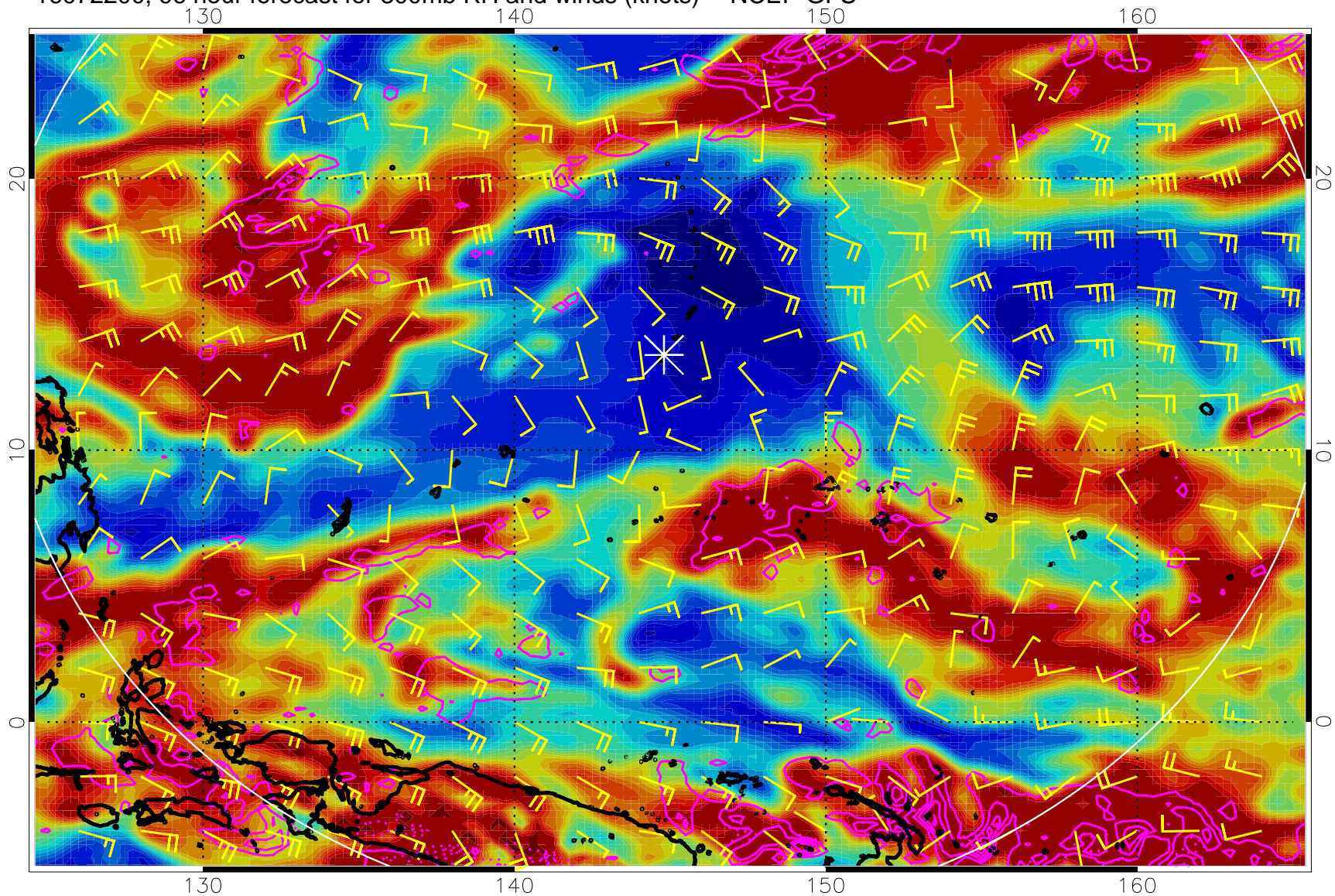
16072200, 96 hour forecast for 300mb RH and winds (knots) -- NCEP GFS
