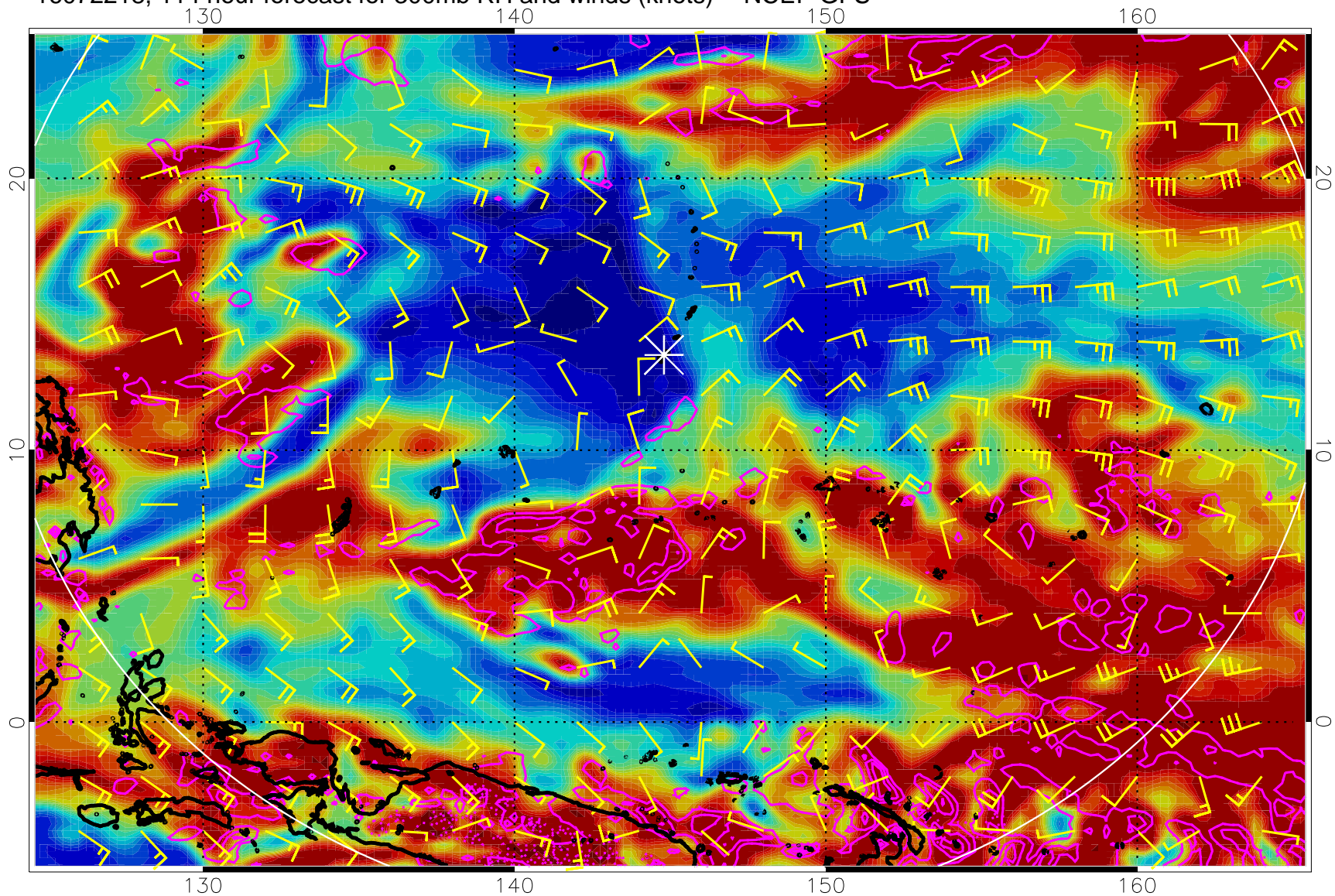
16072218, 114 hour forecast for 300mb RH and winds (knots) -- NCEP GFS
