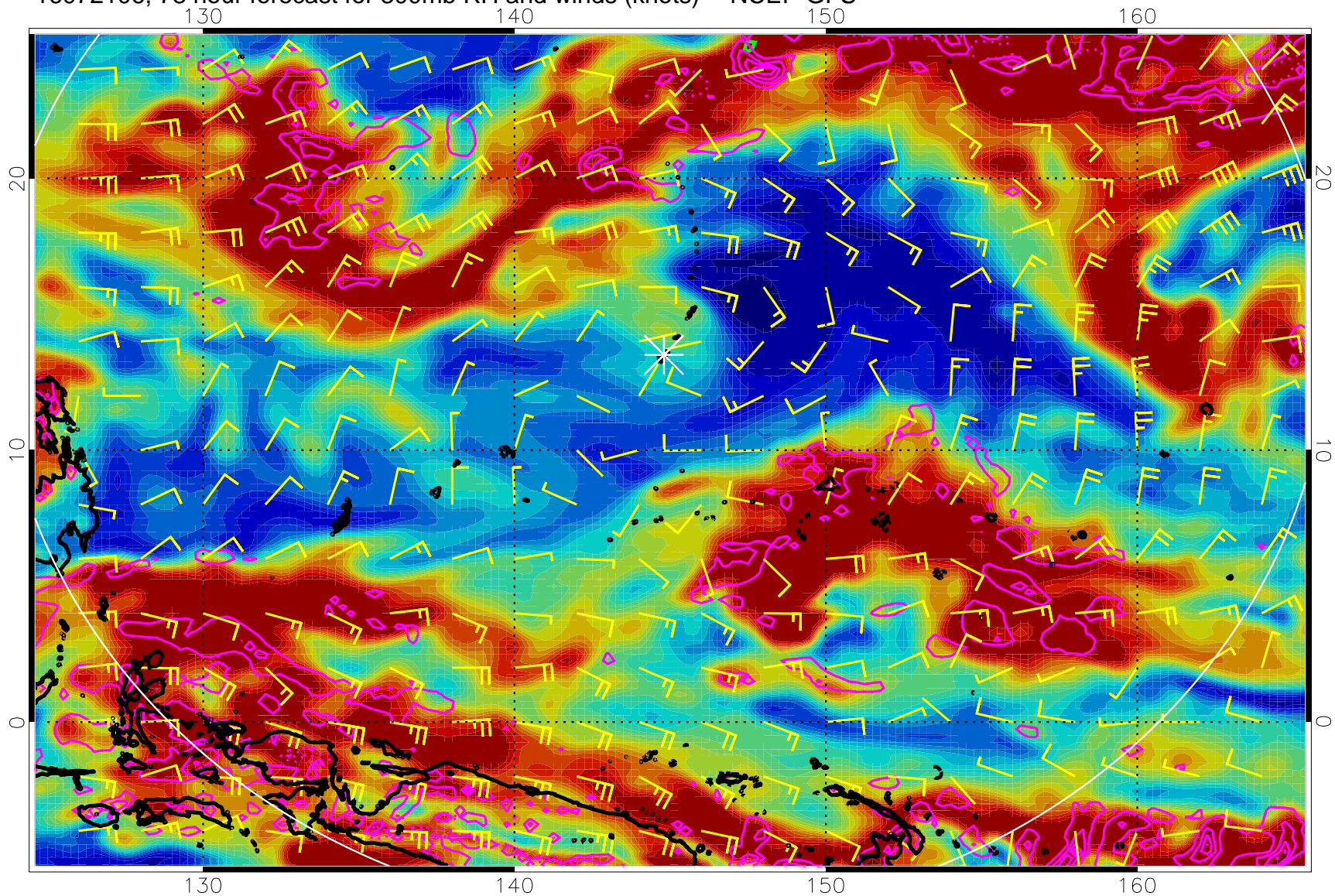
16072106, 78 hour forecast for 300mb RH and winds (knots) -- NCEP GFS
