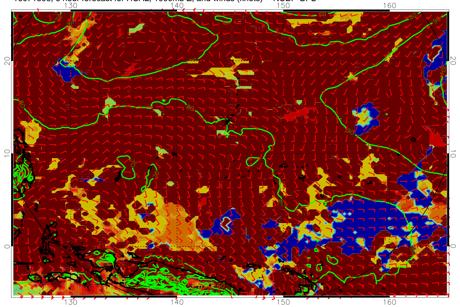
16071806, 6 hour forecast for HCAL, 1000mb Z, and winds (knots) -- NCEP GFS
