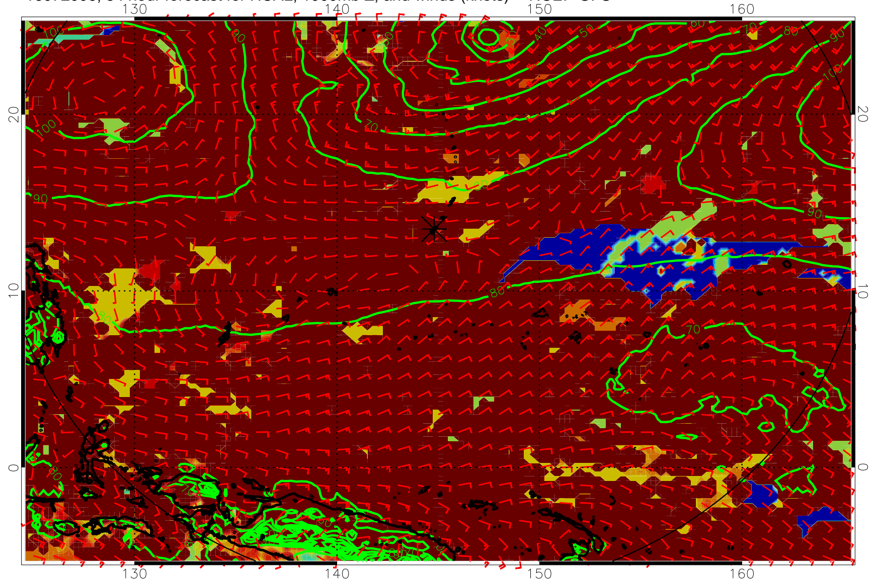
16072006, 54 hour forecast for HCAL, 1000mb Z, and winds (knots) -- NCEP GFS
