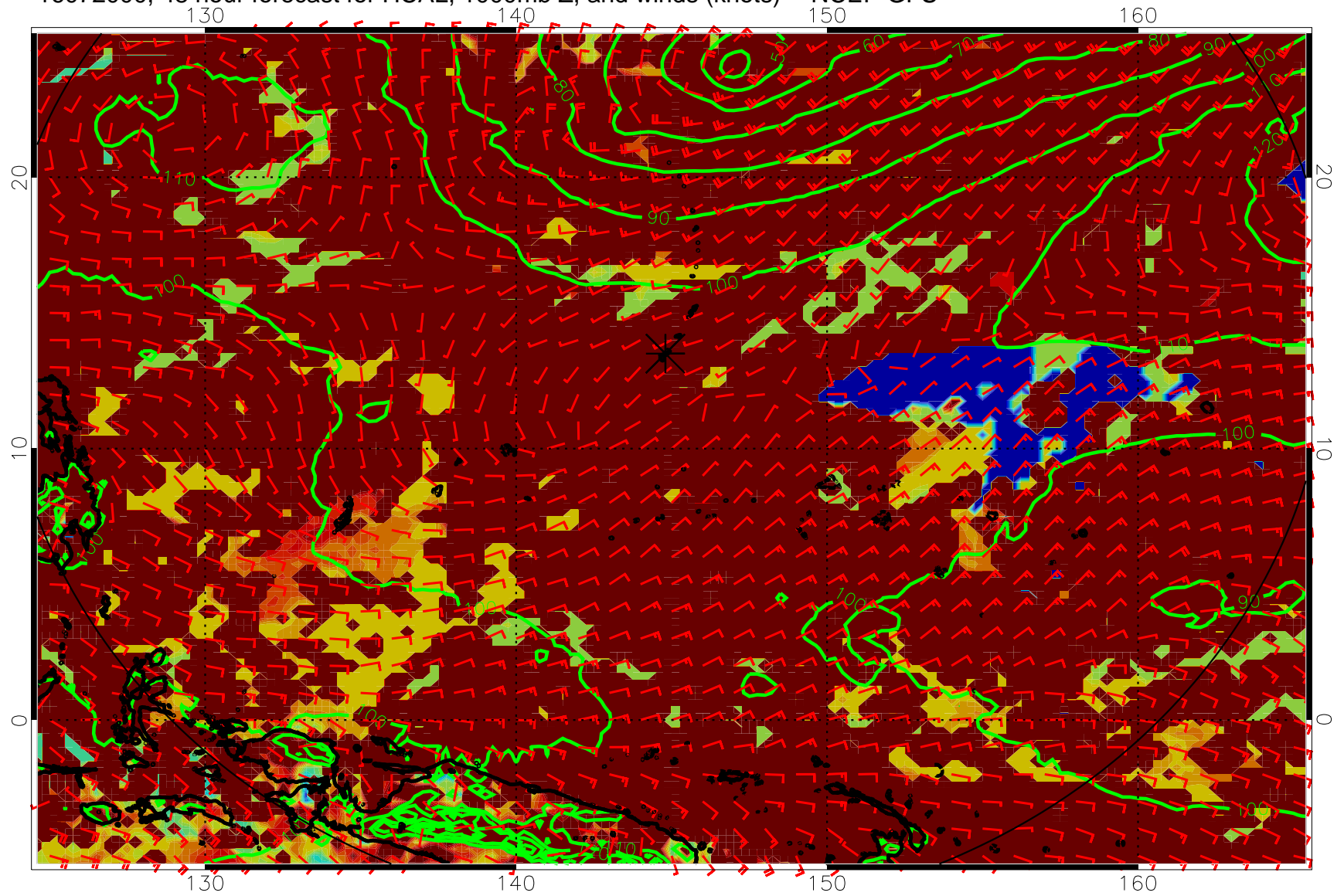
16072000, 48 hour forecast for HCAL, 1000mb Z, and winds (knots) -- NCEP GFS
