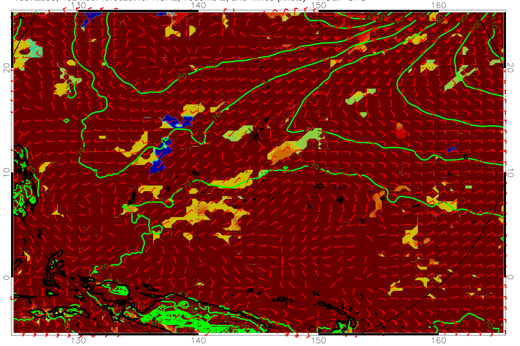
16072206, 102 hour forecast for HCAL, 1000mb Z, and winds (knots) -- NCEP GFS
