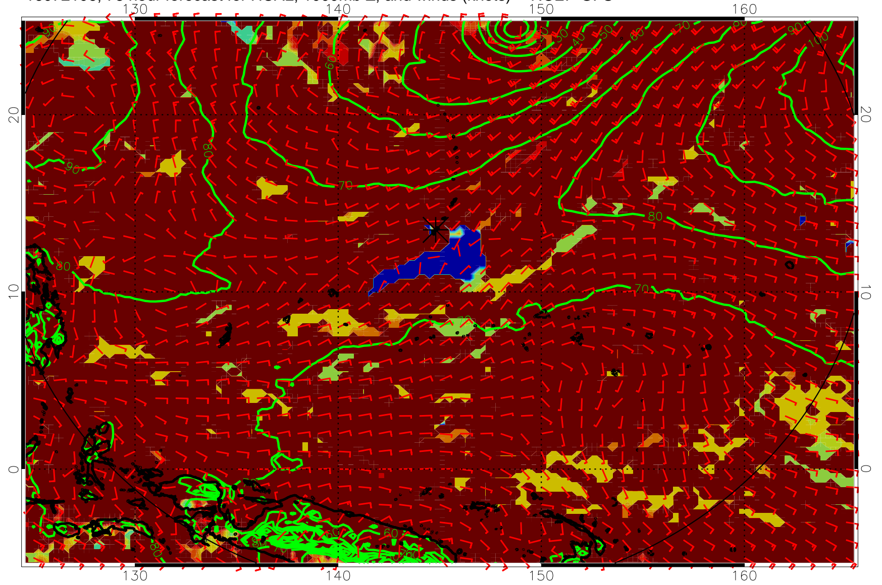
16072106, 78 hour forecast for HCAL, 1000mb Z, and winds (knots) -- NCEP GFS
