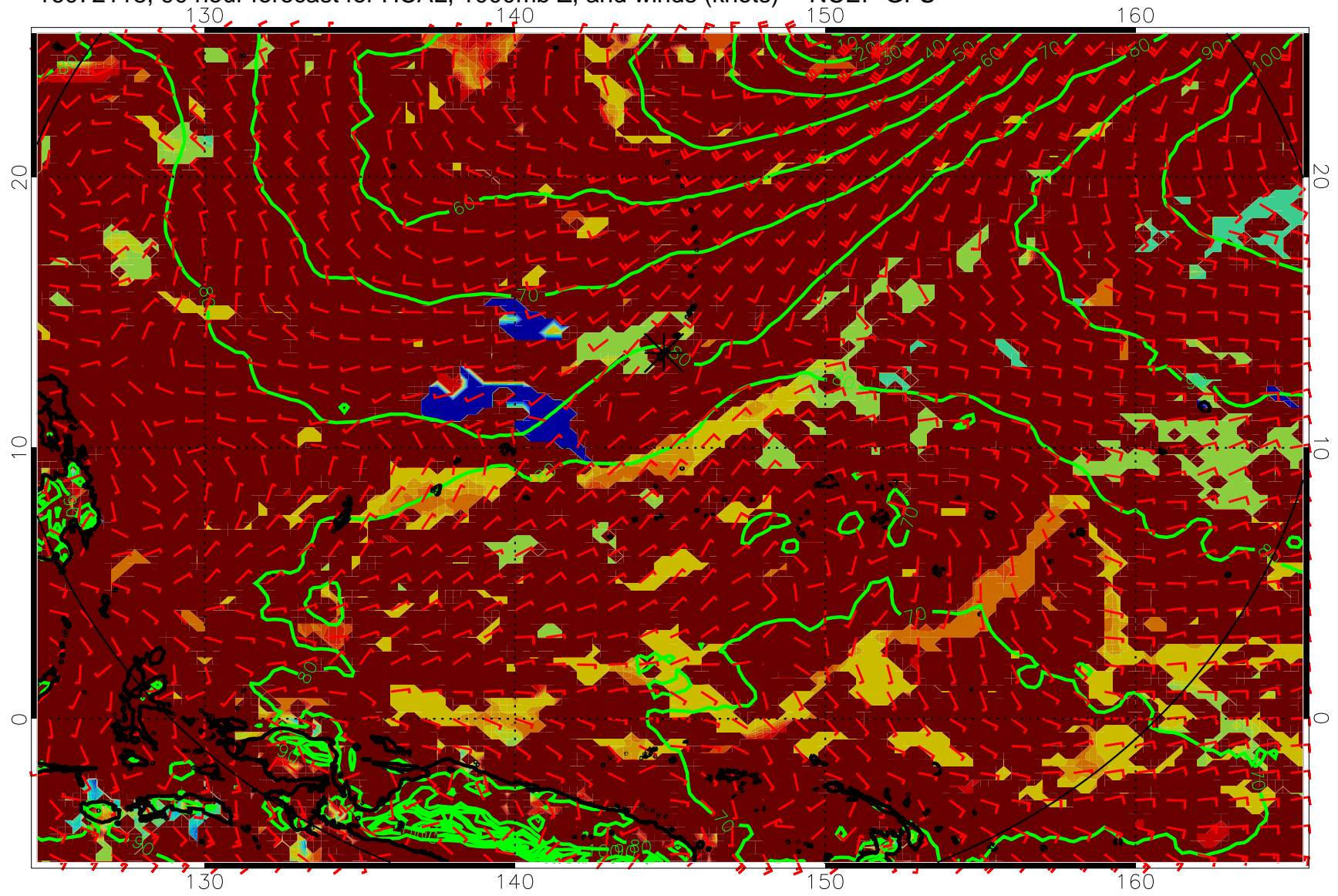
16072118, 90 hour forecast for HCAL, 1000mb Z, and winds (knots) -- NCEP GFS
