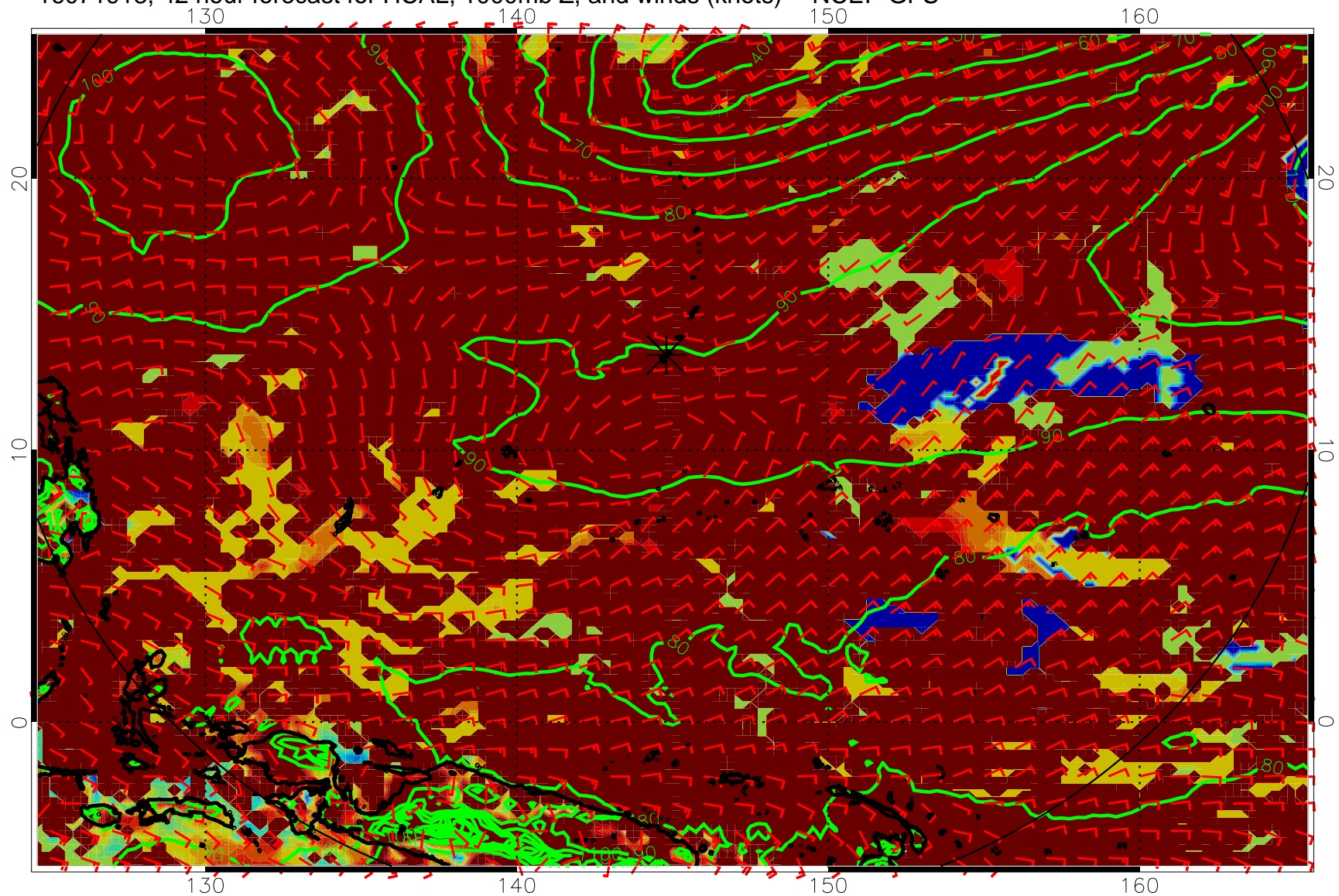
16071918, 42 hour forecast for HCAL, 1000mb Z, and winds (knots) -- NCEP GFS
