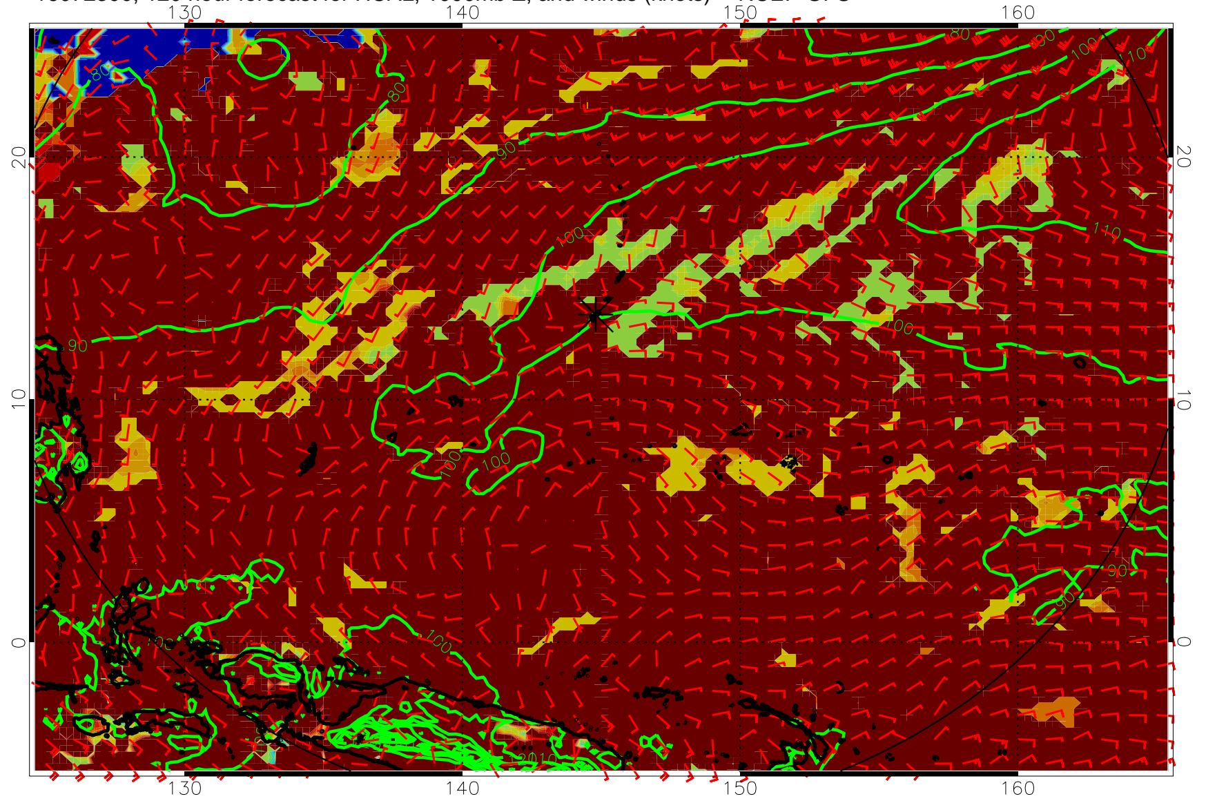
16072300, 120 hour forecast for HCAL, 1000mb Z, and winds (knots) -- NCEP GFS
