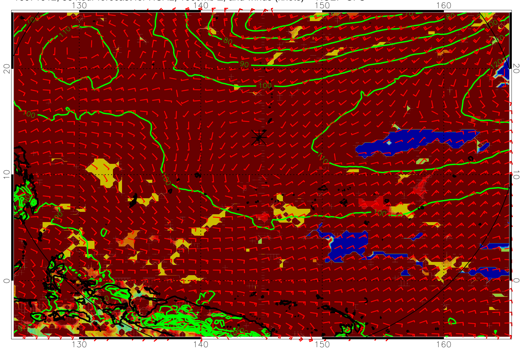
16071912, 36 hour forecast for HCAL, 1000mb Z, and winds (knots) -- NCEP GFS
