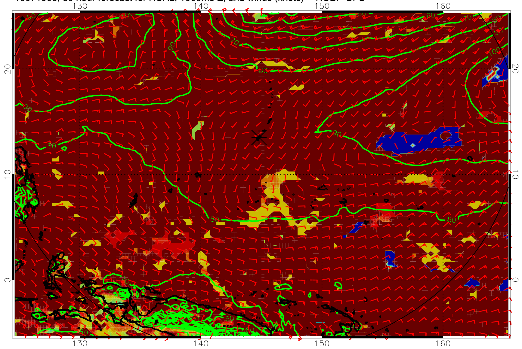
16071906, 30 hour forecast for HCAL, 1000mb Z, and winds (knots) -- NCEP GFS
