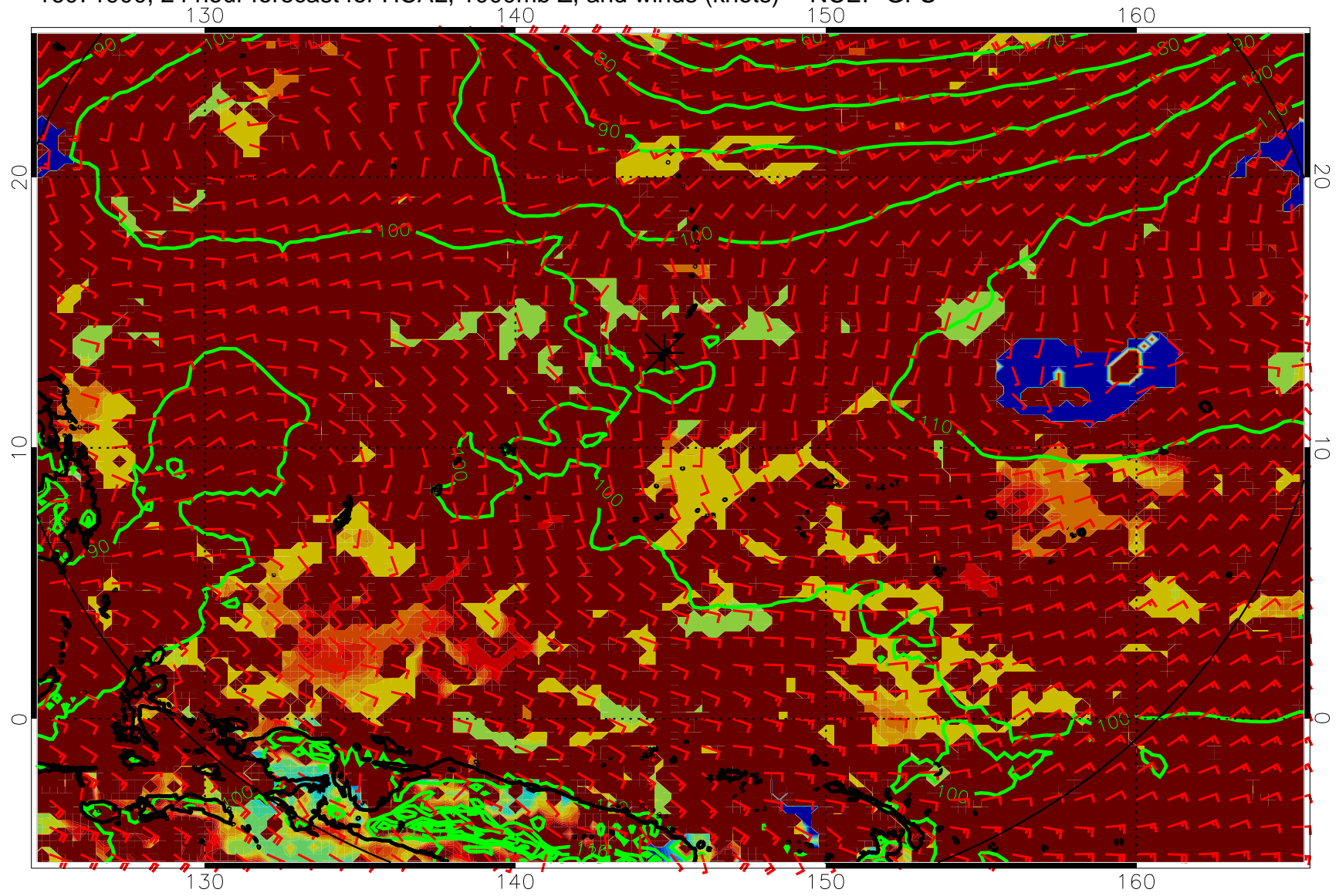
16071900, 24 hour forecast for HCAL, 1000mb Z, and winds (knots) -- NCEP GFS
