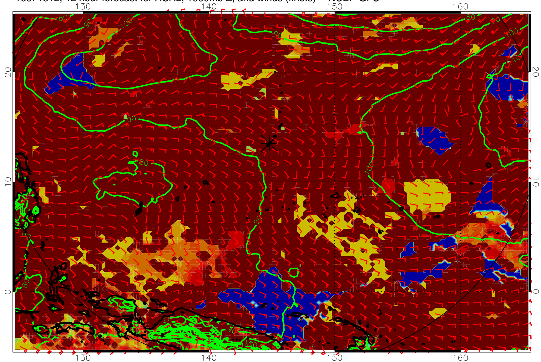
16071812, 12 hour forecast for HCAL, 1000mb Z, and winds (knots) -- NCEP GFS
