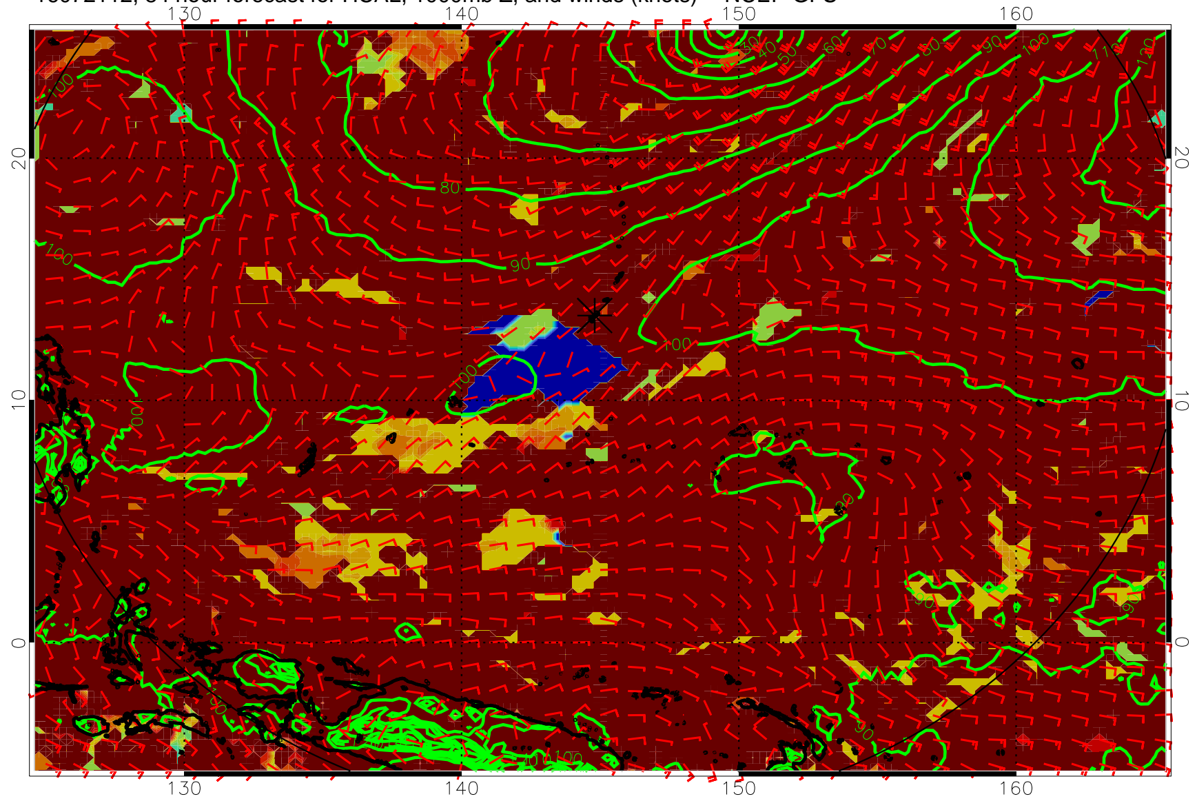
16072112, 84 hour forecast for HCAL, 1000mb Z, and winds (knots) -- NCEP GFS
