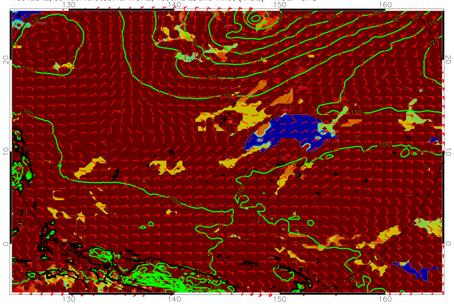
16072012, 60 hour forecast for HCAL, 1000mb Z, and winds (knots) -- NCEP GFS
