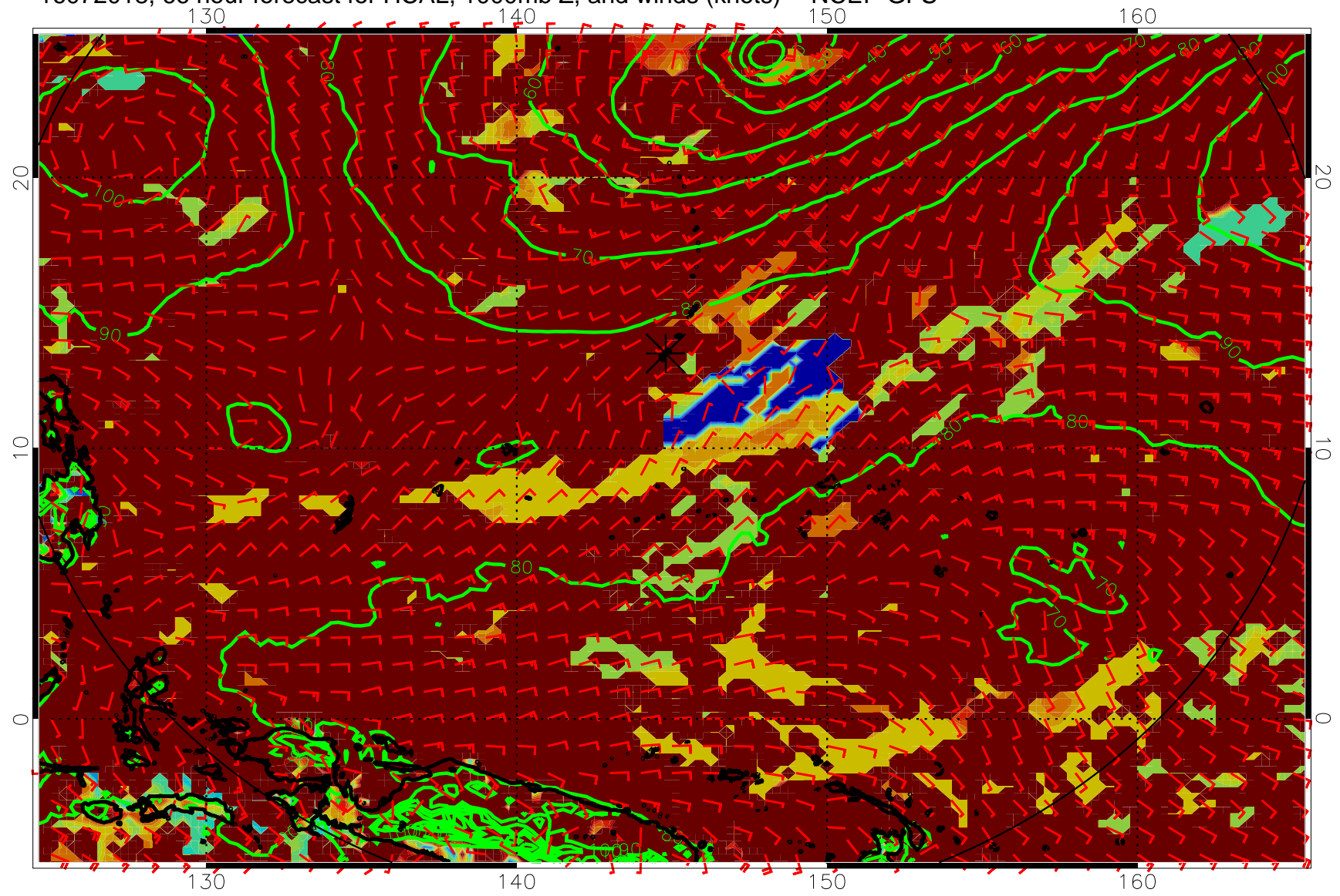
16072018, 66 hour forecast for HCAL, 1000mb Z, and winds (knots) -- NCEP GFS
