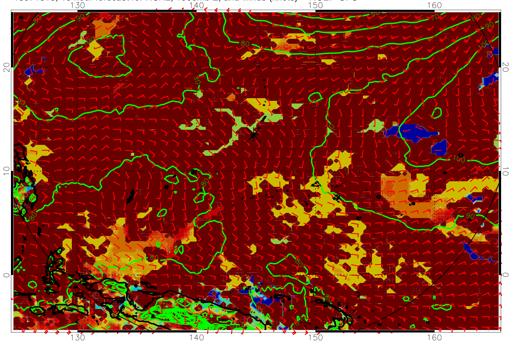
16071818, 18 hour forecast for HCAL, 1000mb Z, and winds (knots) -- NCEP GFS
