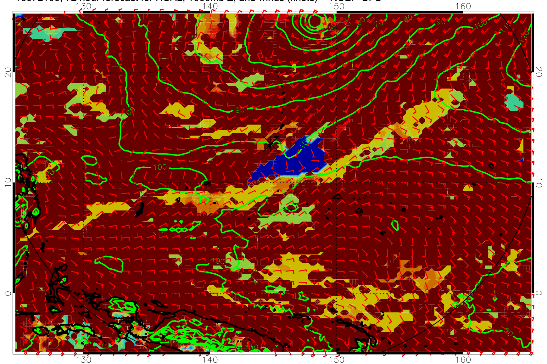
16072100, 72 hour forecast for HCAL, 1000mb Z, and winds (knots) -- NCEP GFS
