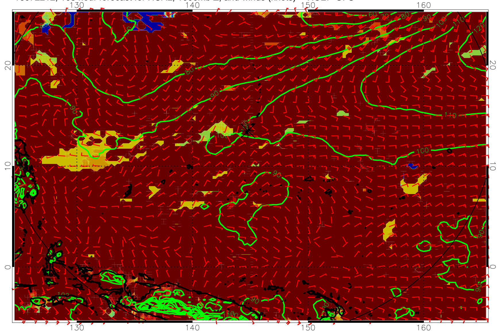
16072212, 108 hour forecast for HCAL, 1000mb Z, and winds (knots) -- NCEP GFS
