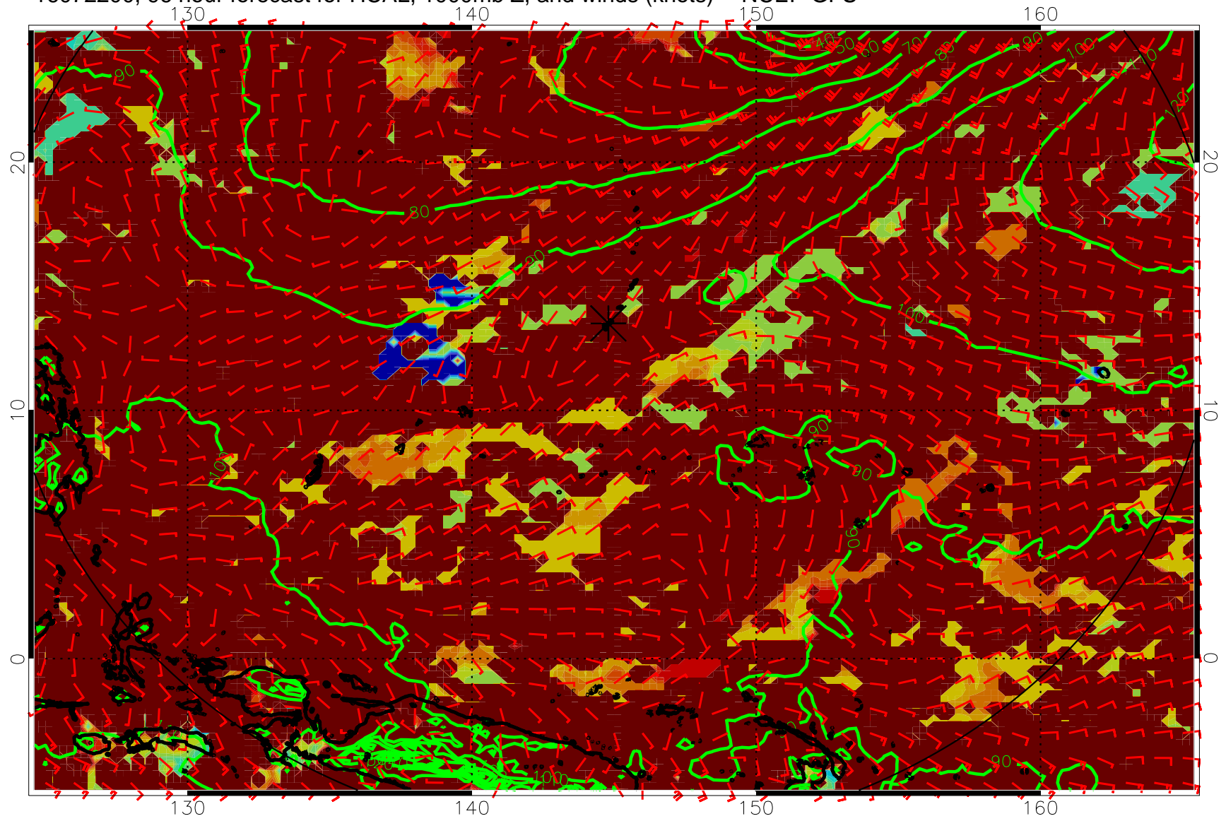
16072200, 96 hour forecast for HCAL, 1000mb Z, and winds (knots) -- NCEP GFS
