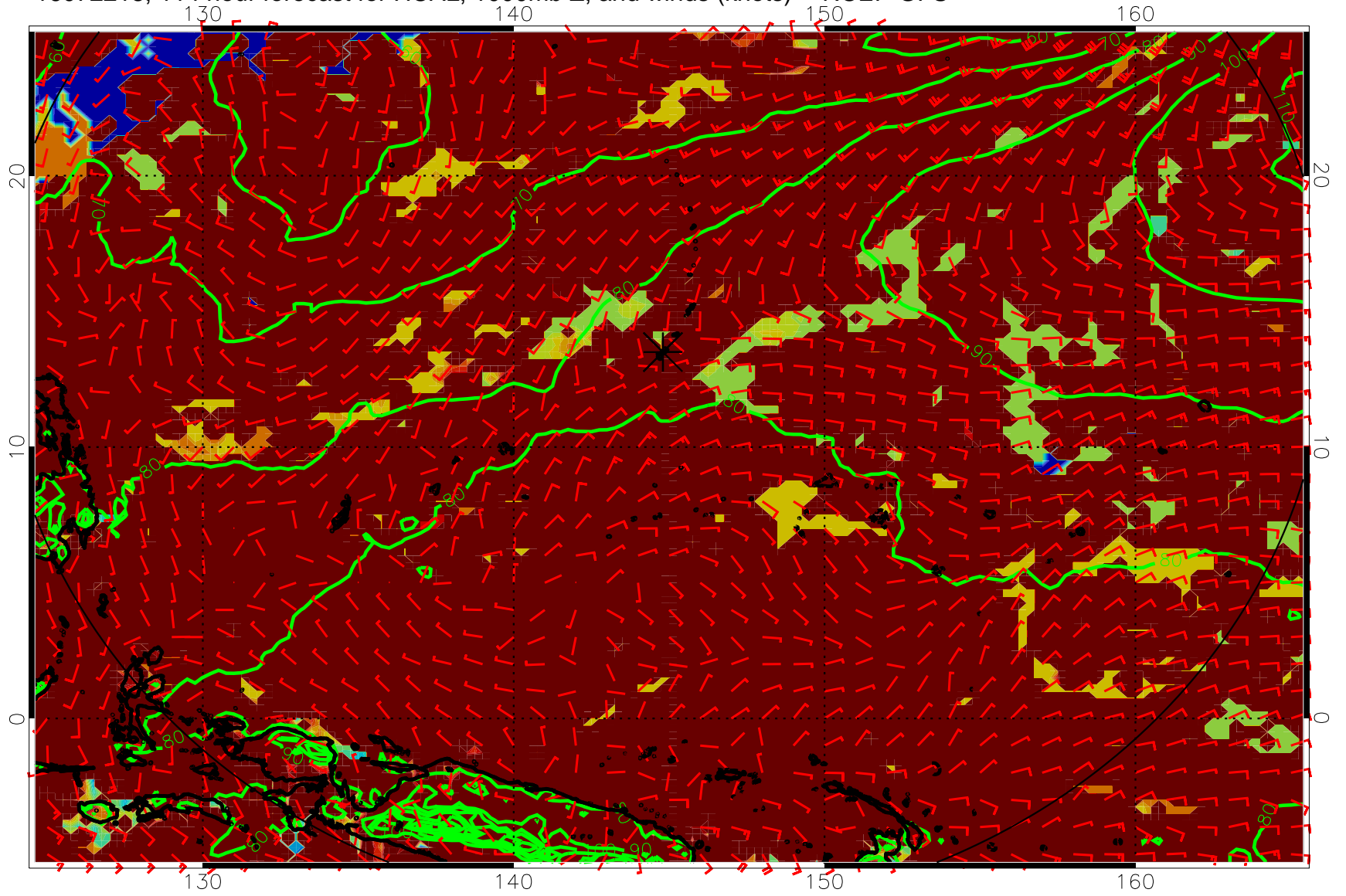
16072218, 114 hour forecast for HCAL, 1000mb Z, and winds (knots) -- NCEP GFS
