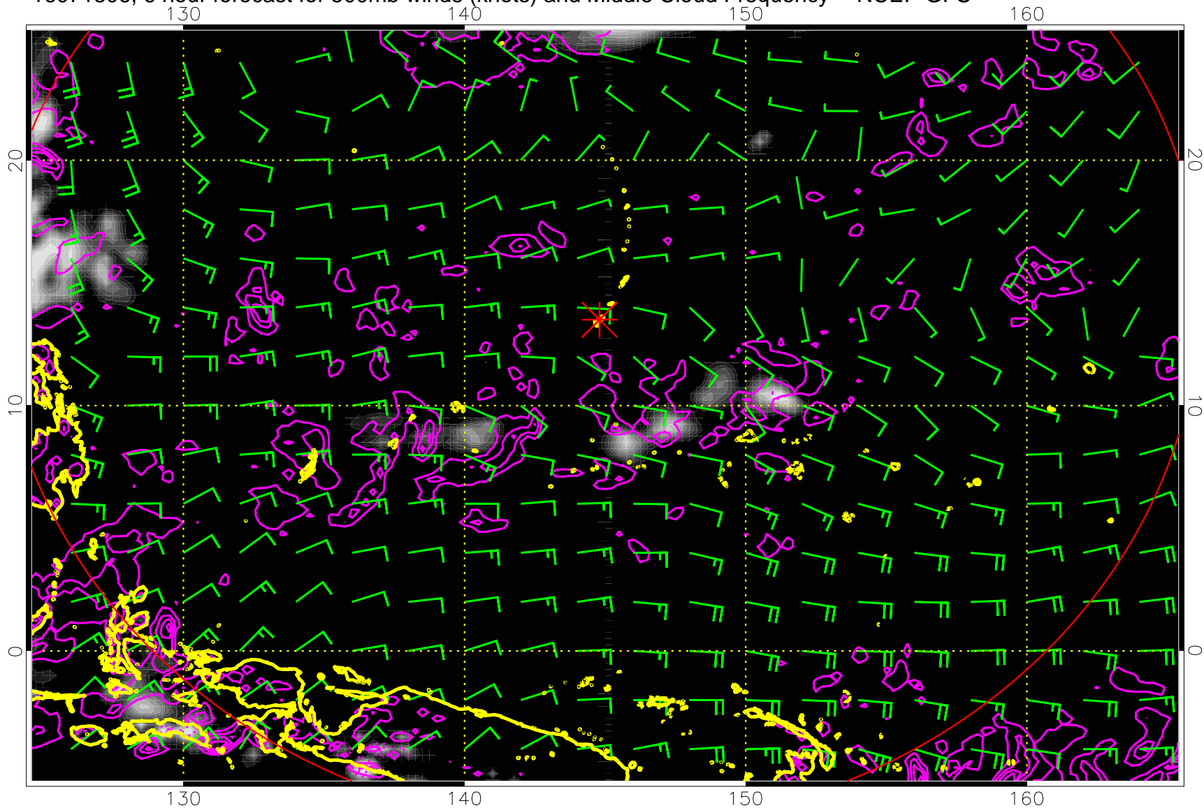
16071806, 6 hour forecast for 500mb winds (knots) and Middle Cloud Frequency -- NCEP GFS
