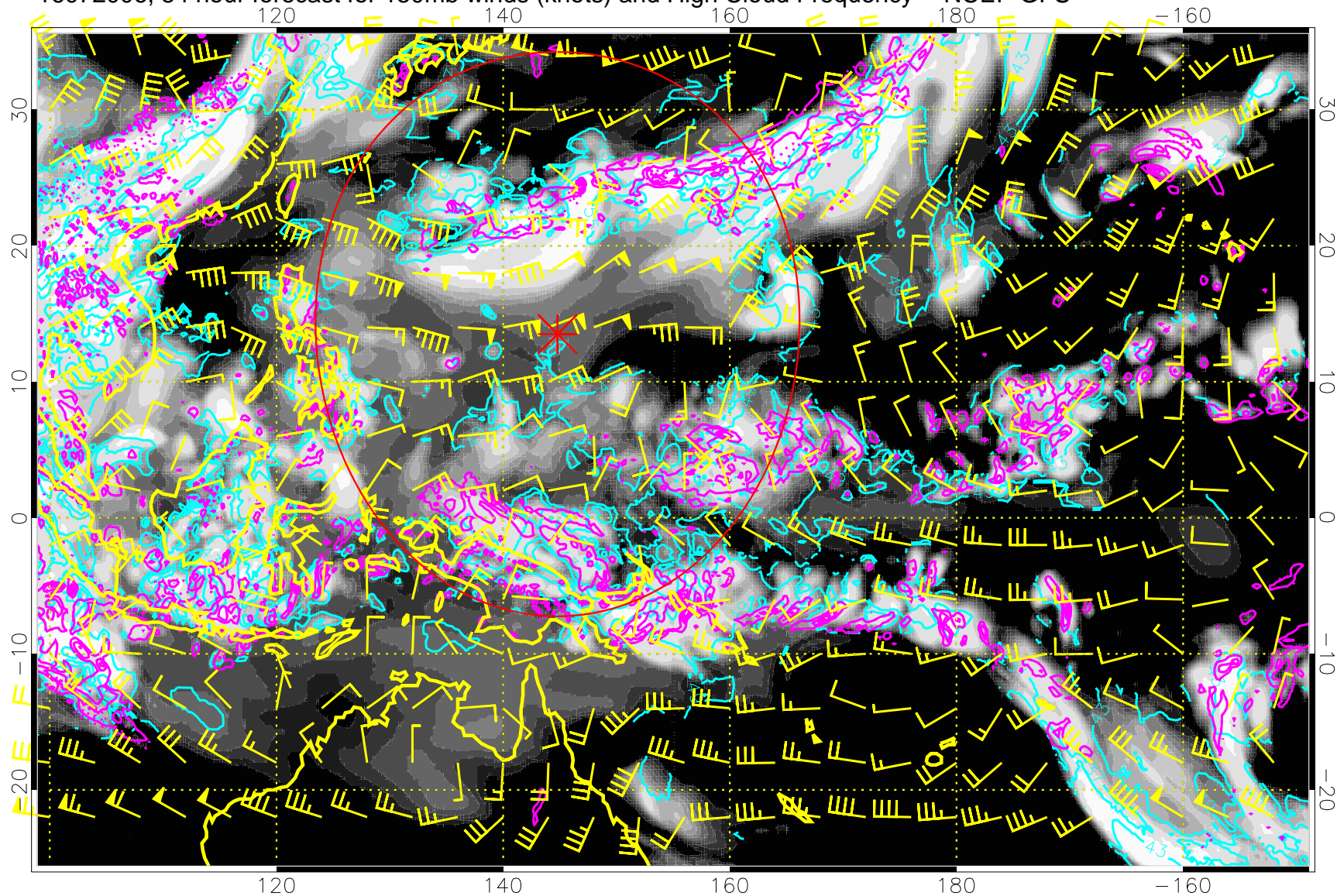
16072006, 54 hour forecast for 150mb winds (knots) and High Cloud Frequency -- NCEP GFS
