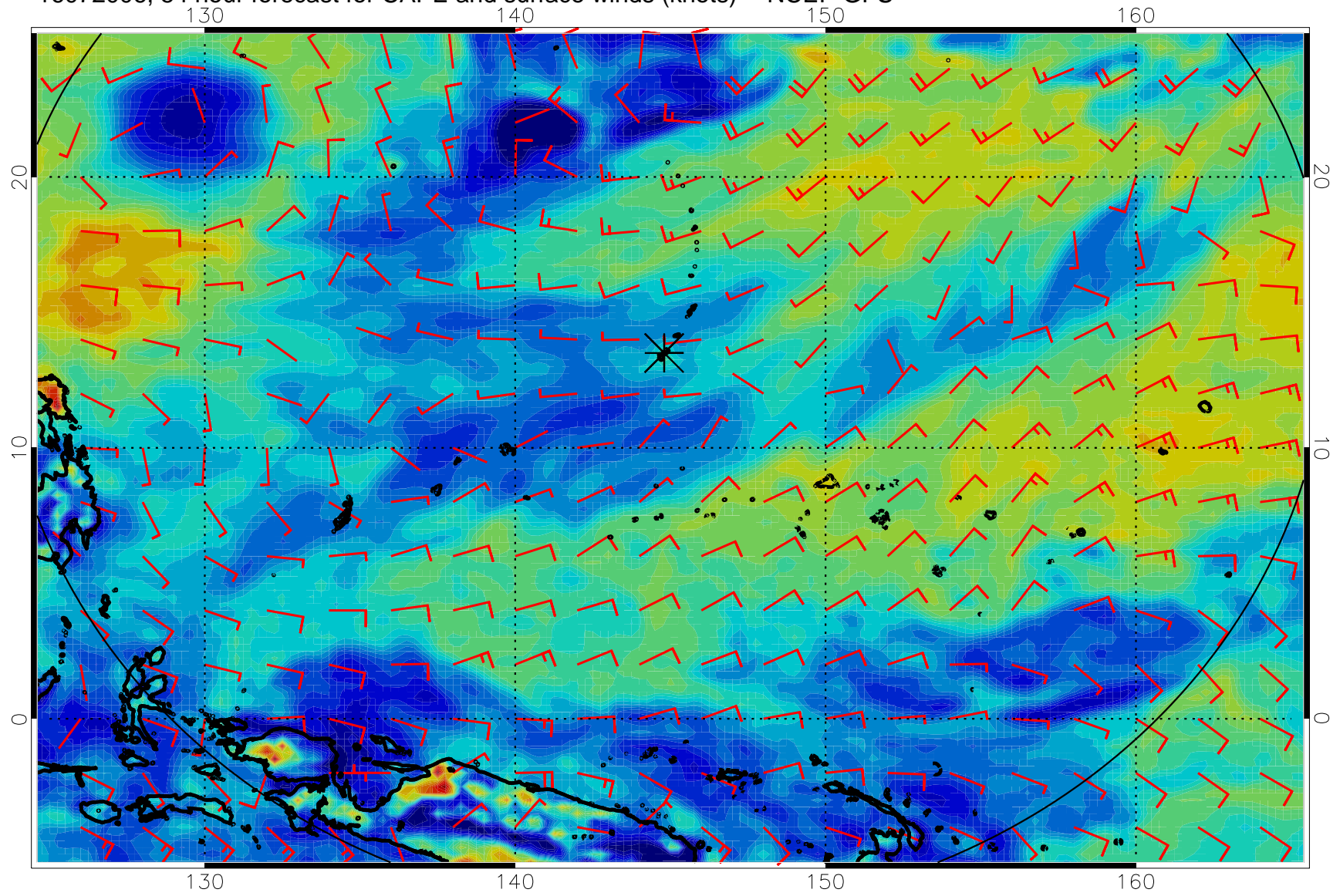
16072006, 54 hour forecast for CAPE and surface winds (knots) -- NCEP GFS
