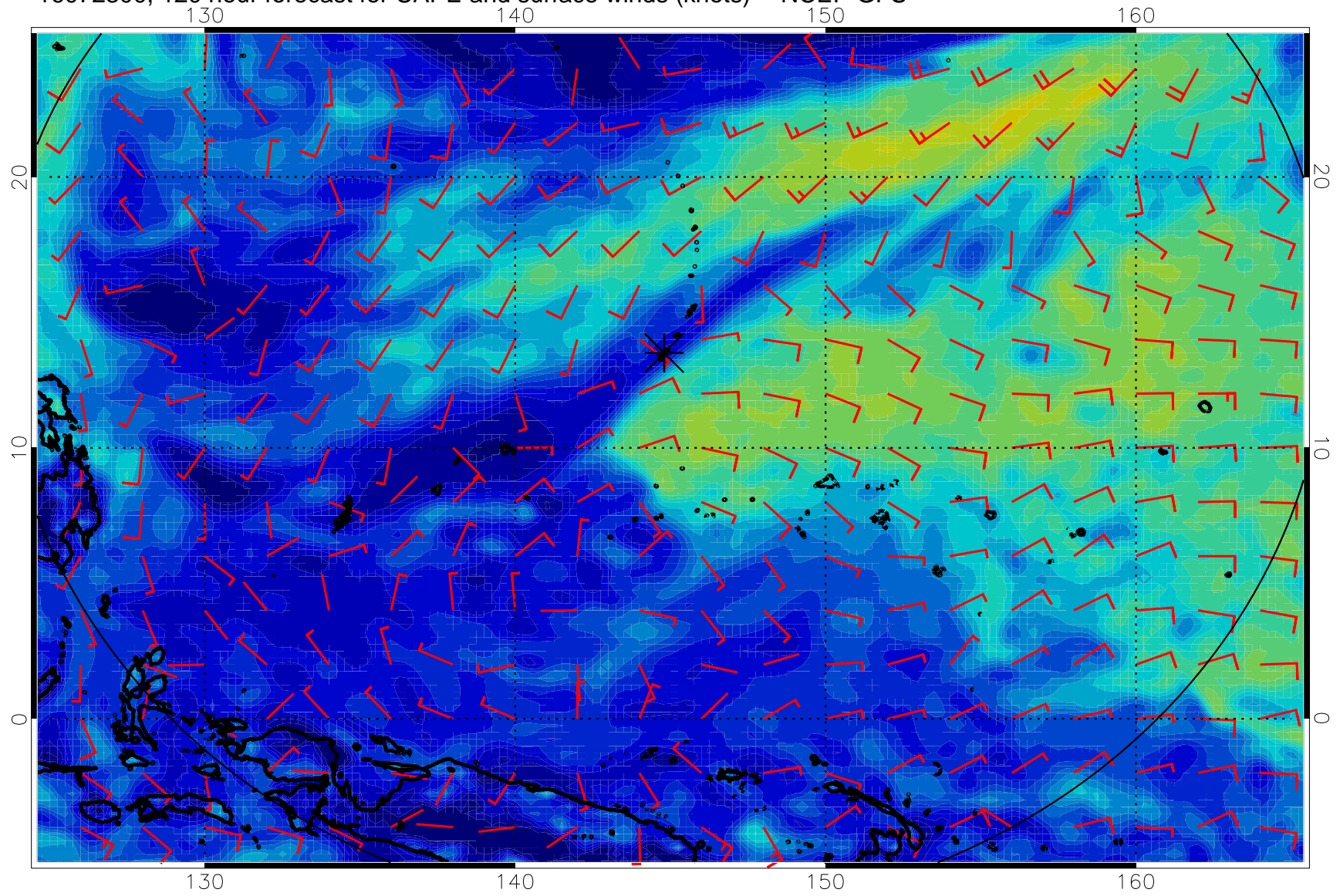
16072300, 120 hour forecast for CAPE and surface winds (knots) -- NCEP GFS
