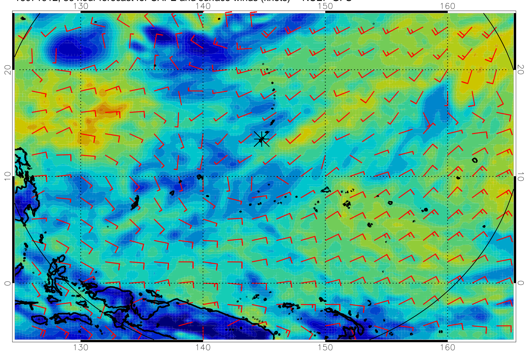
16071912, 36 hour forecast for CAPE and surface winds (knots) -- NCEP GFS
