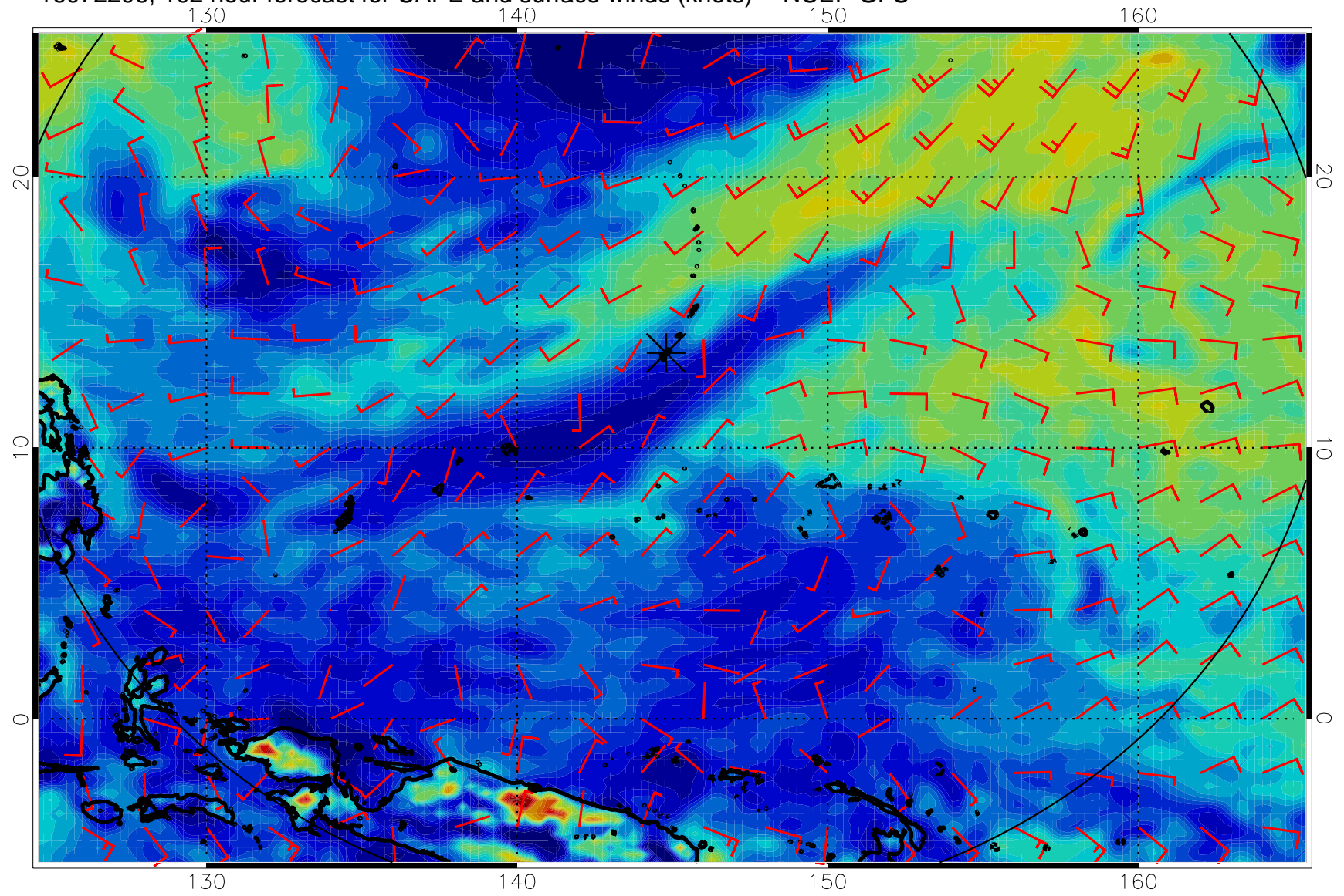
16072206, 102 hour forecast for CAPE and surface winds (knots) -- NCEP GFS
