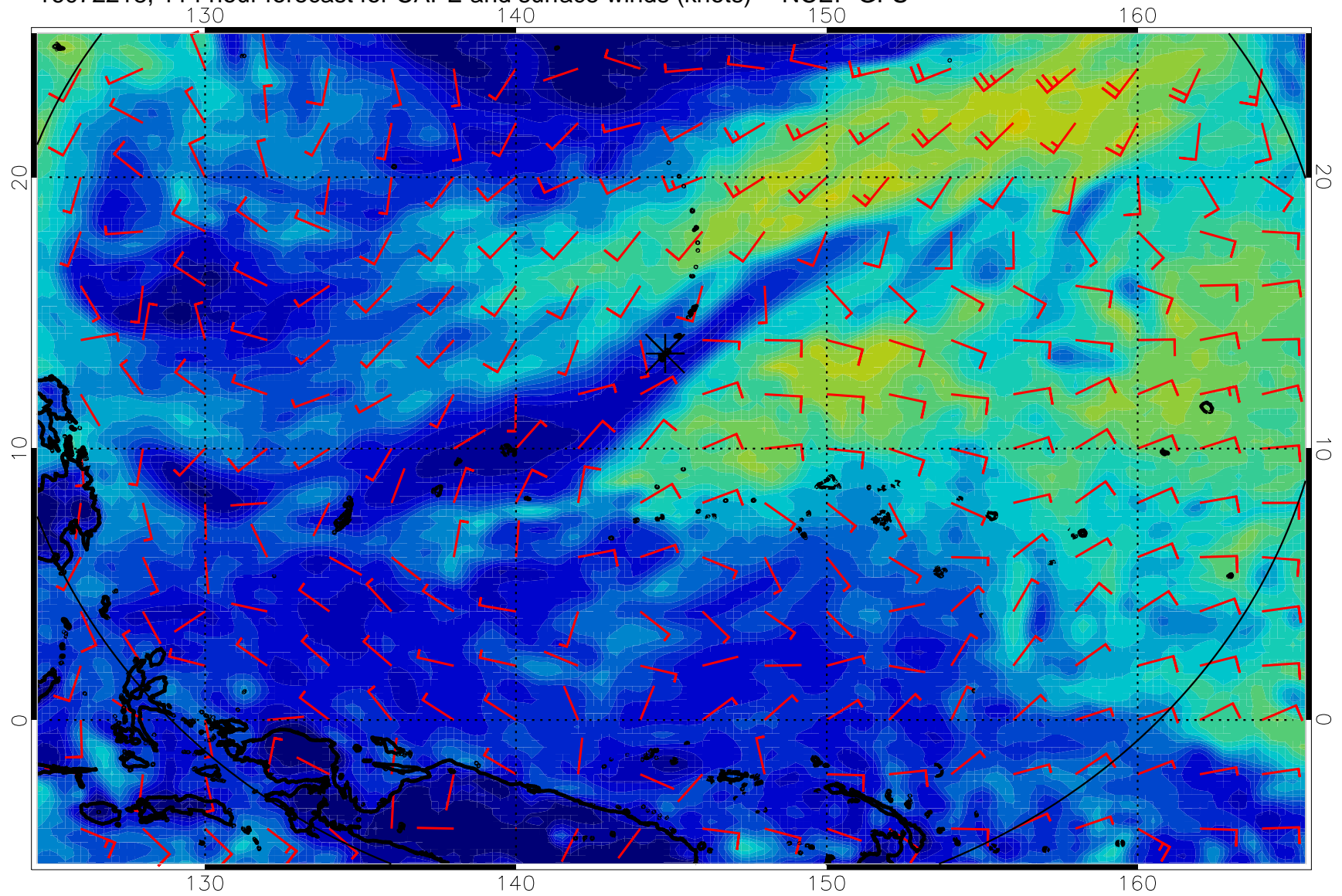
16072218, 114 hour forecast for CAPE and surface winds (knots) -- NCEP GFS
