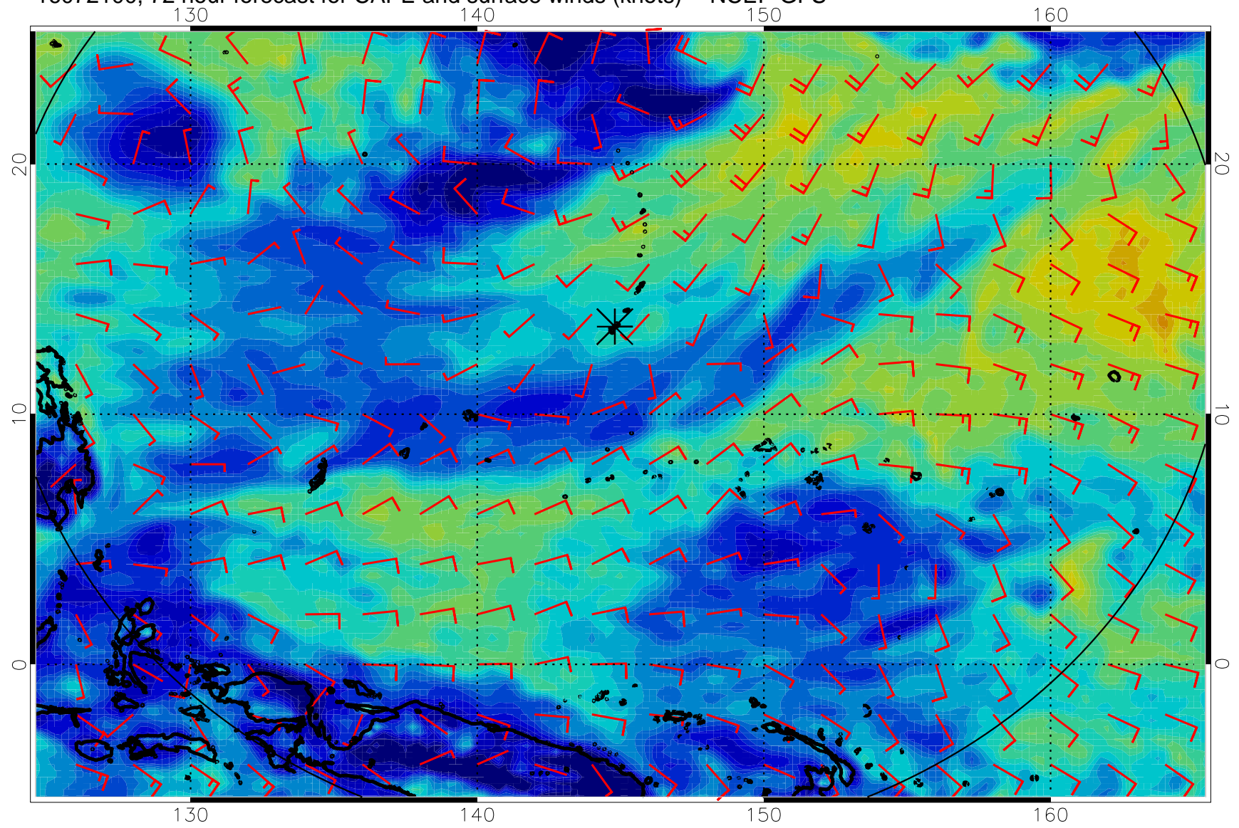
16072100, 72 hour forecast for CAPE and surface winds (knots) -- NCEP GFS
