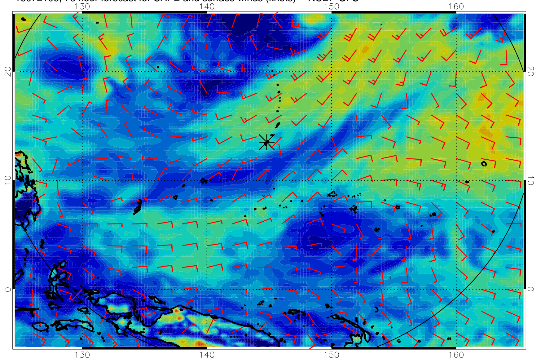
16072106, 78 hour forecast for CAPE and surface winds (knots) -- NCEP GFS
