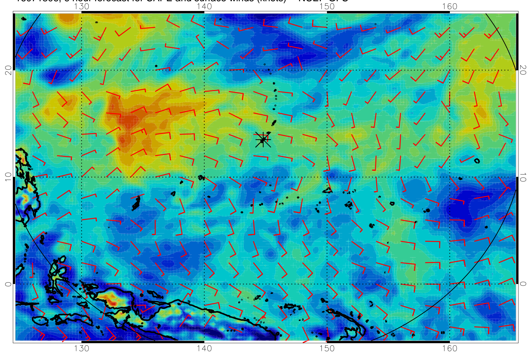
16071806, 6 hour forecast for CAPE and surface winds (knots) -- NCEP GFS
