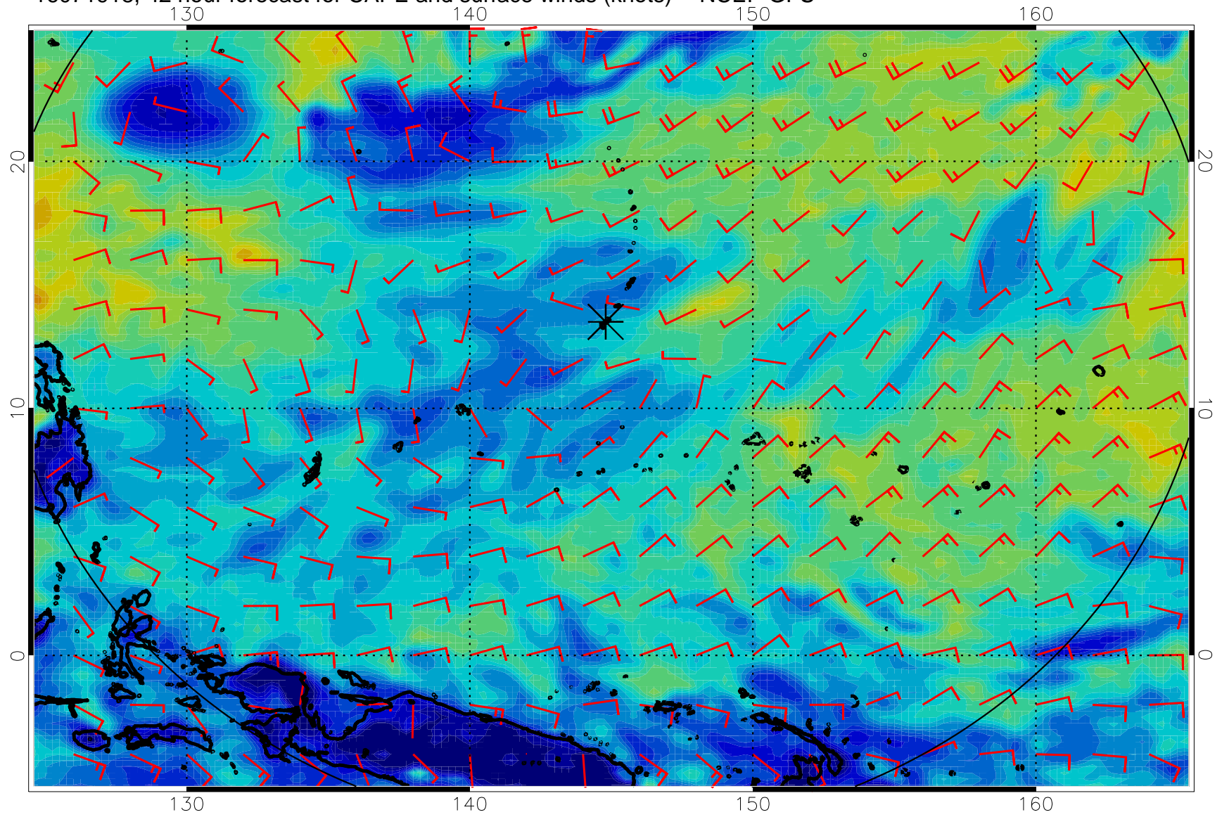
16071918, 42 hour forecast for CAPE and surface winds (knots) -- NCEP GFS
