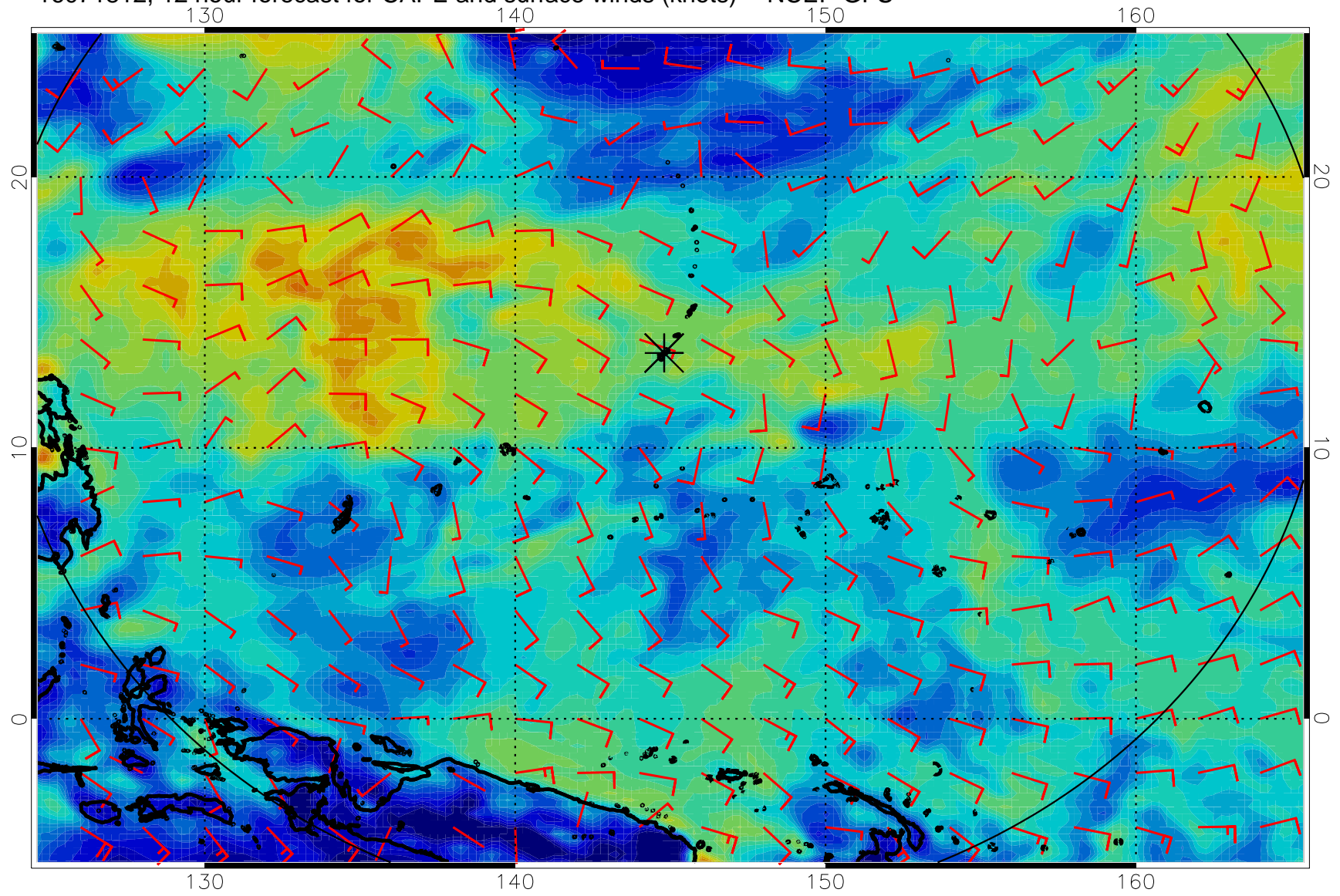
16071812, 12 hour forecast for CAPE and surface winds (knots) -- NCEP GFS
