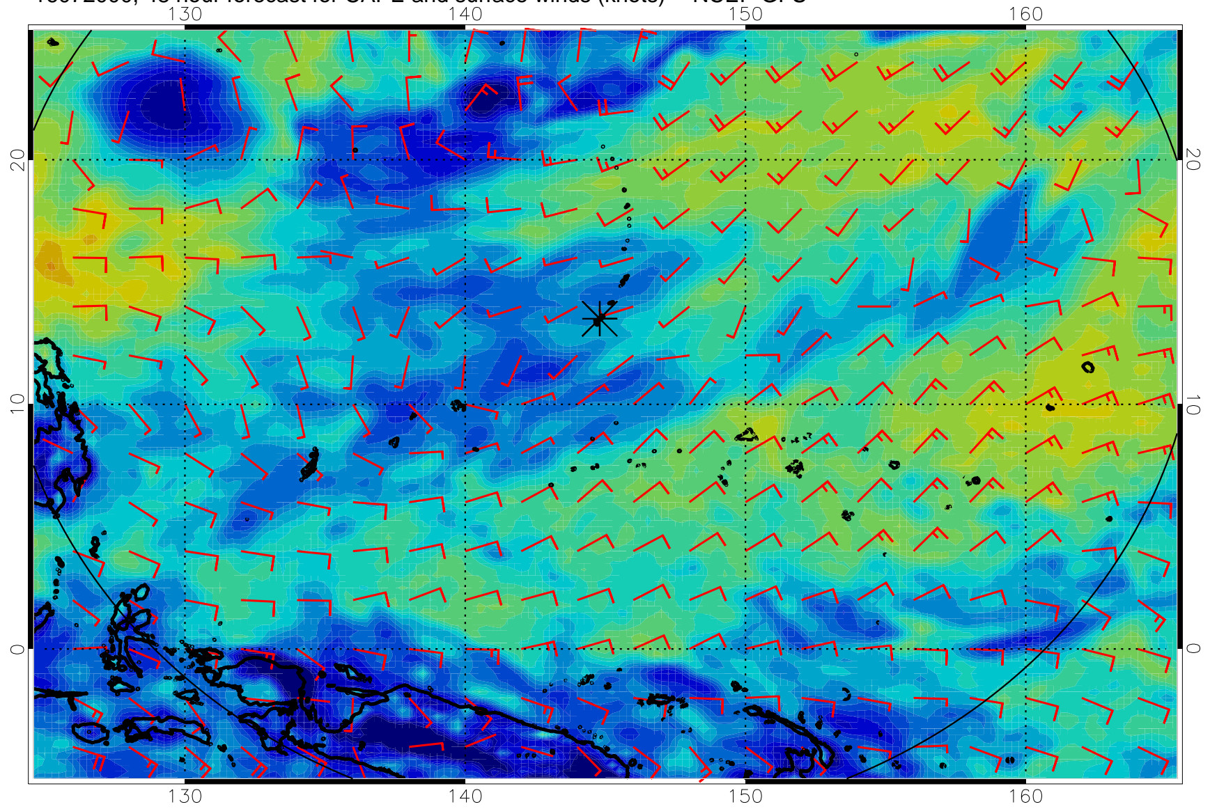
16072000, 48 hour forecast for CAPE and surface winds (knots) -- NCEP GFS
