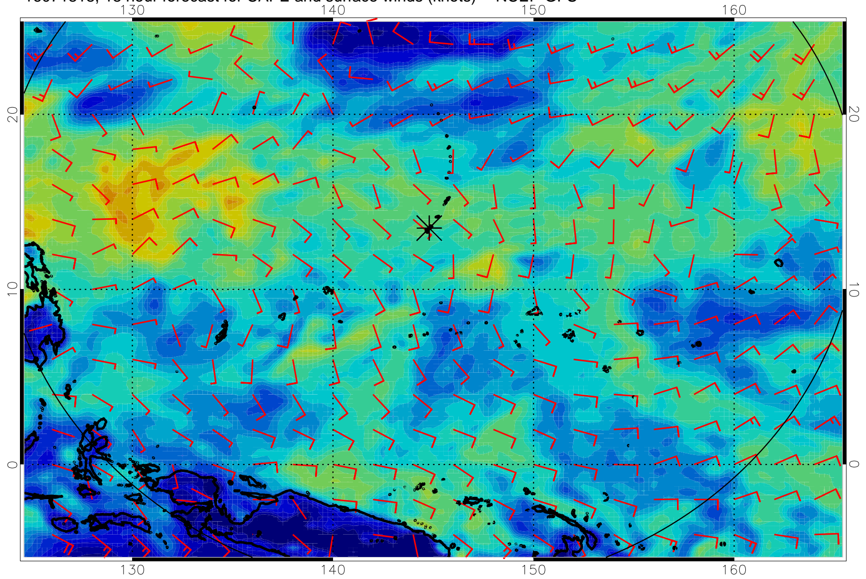
16071818, 18 hour forecast for CAPE and surface winds (knots) -- NCEP GFS
