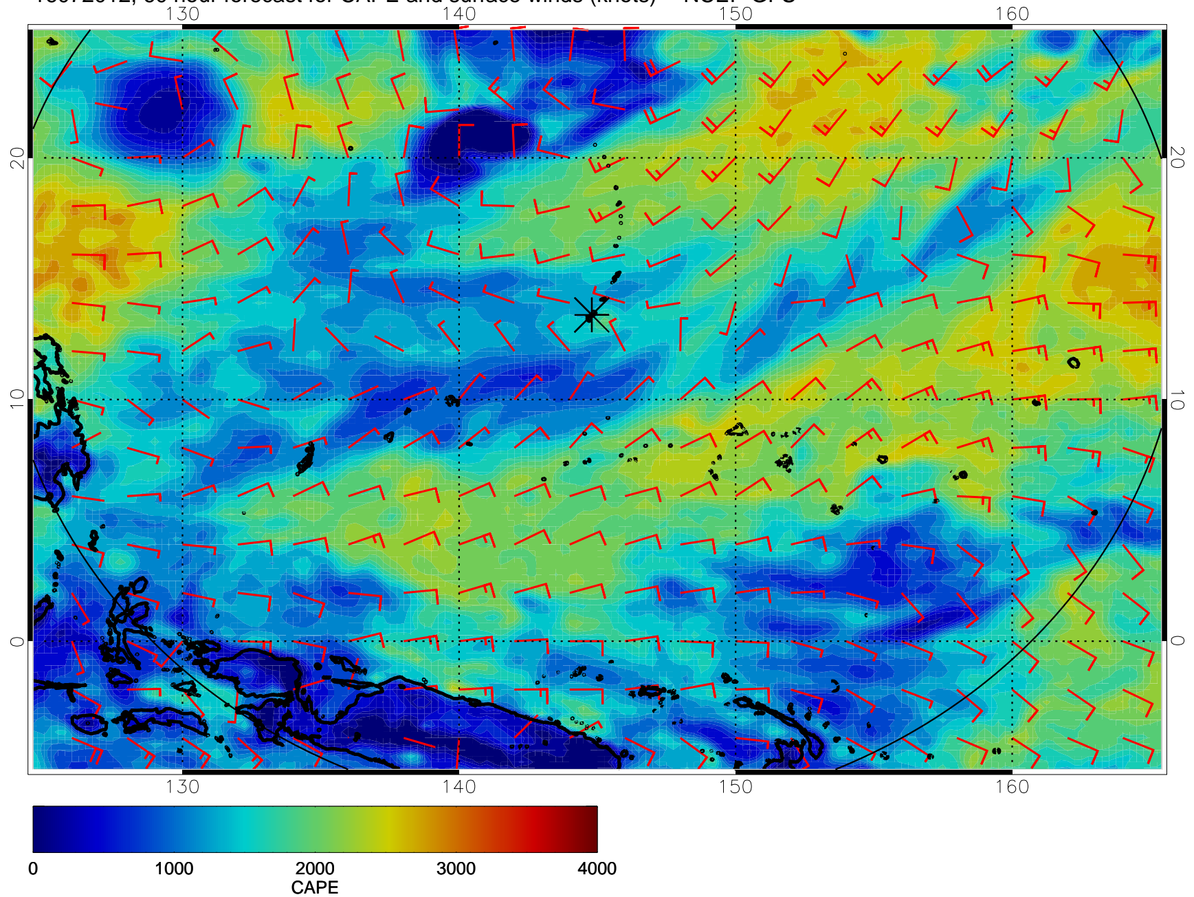
16072012, 60 hour forecast for CAPE and surface winds (knots) -- NCEP GFS
