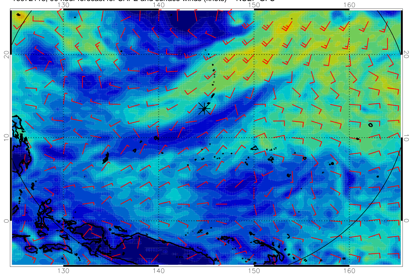
16072118, 90 hour forecast for CAPE and surface winds (knots) -- NCEP GFS
