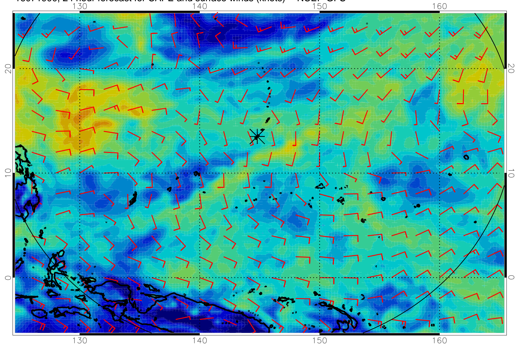
16071900, 24 hour forecast for CAPE and surface winds (knots) -- NCEP GFS
