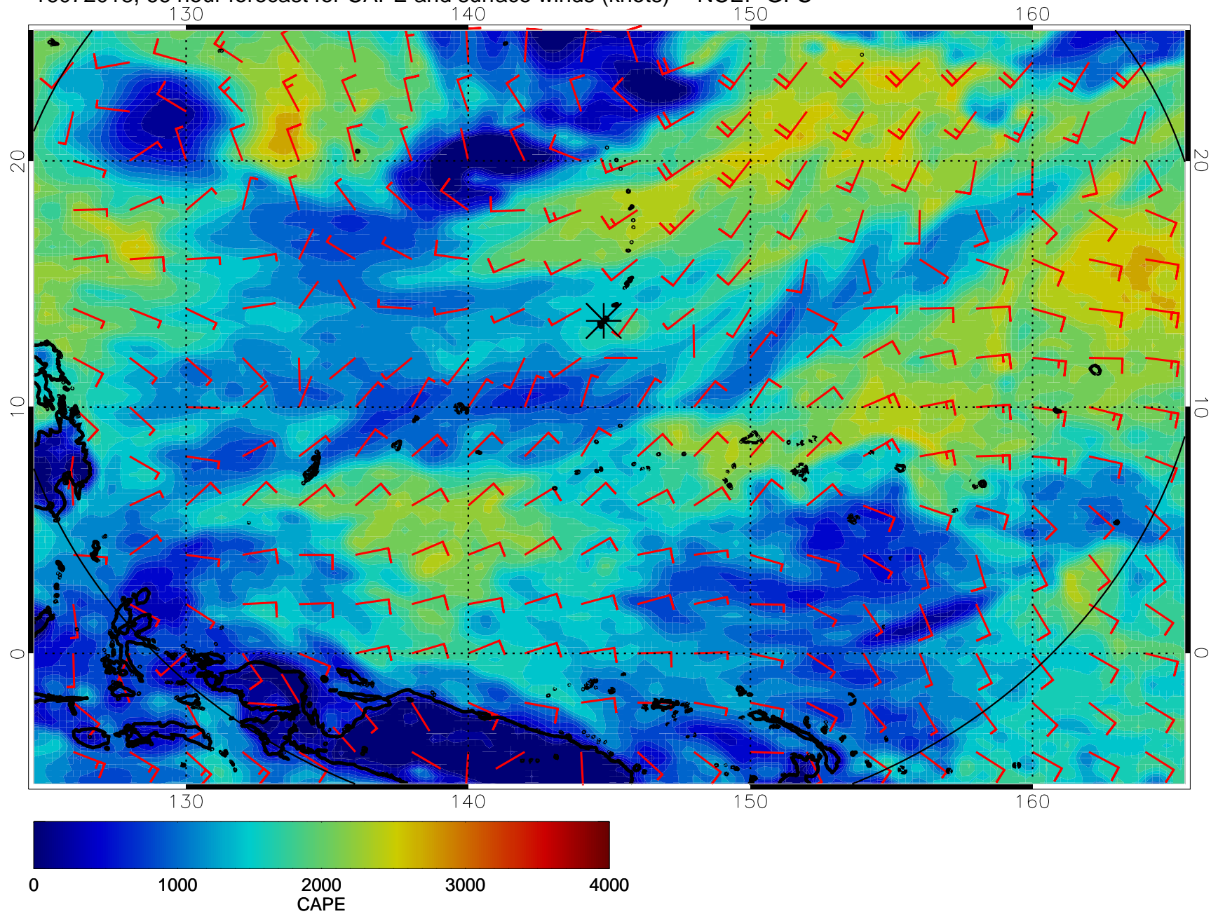
16072018, 66 hour forecast for CAPE and surface winds (knots) -- NCEP GFS
