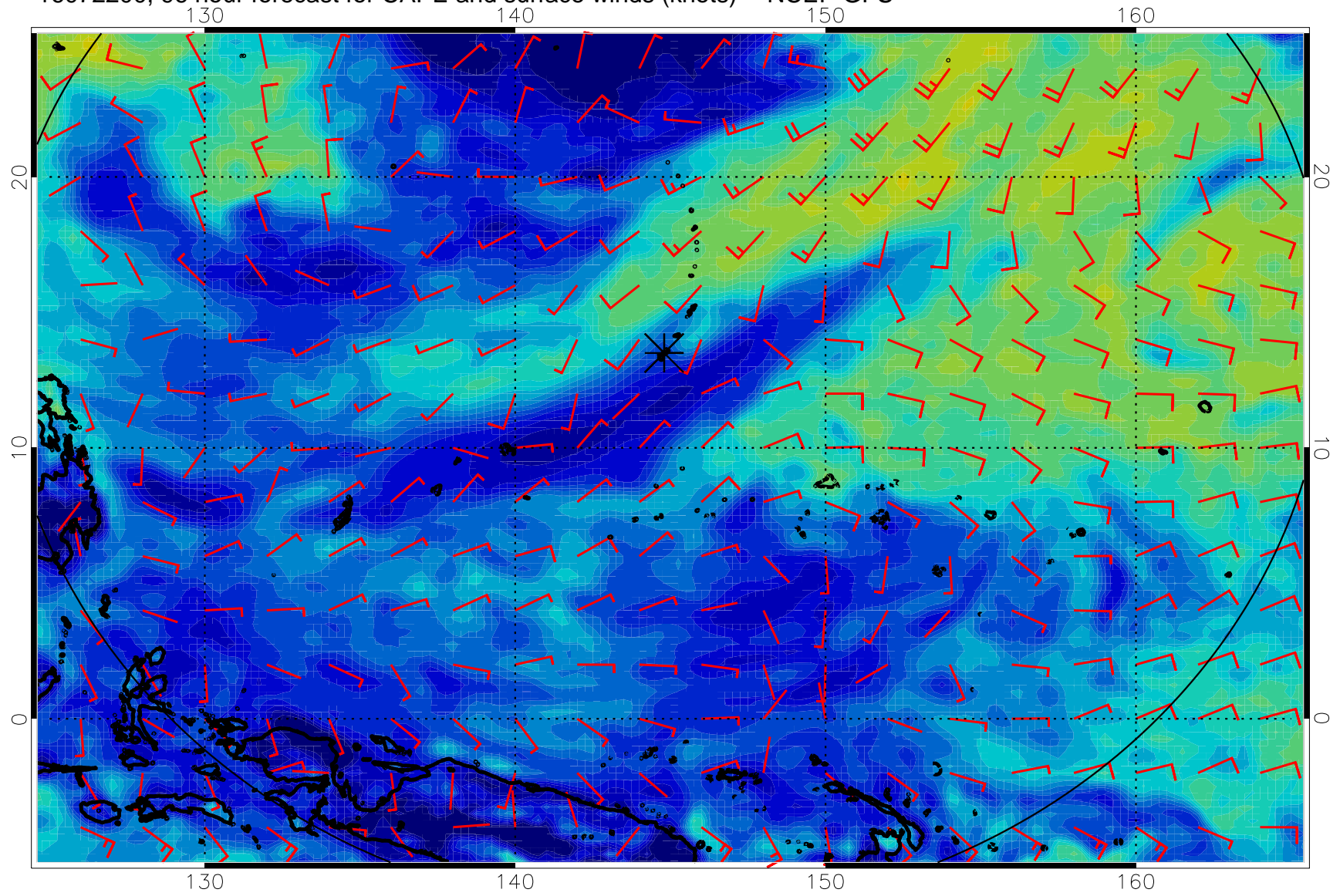
16072200, 96 hour forecast for CAPE and surface winds (knots) -- NCEP GFS
