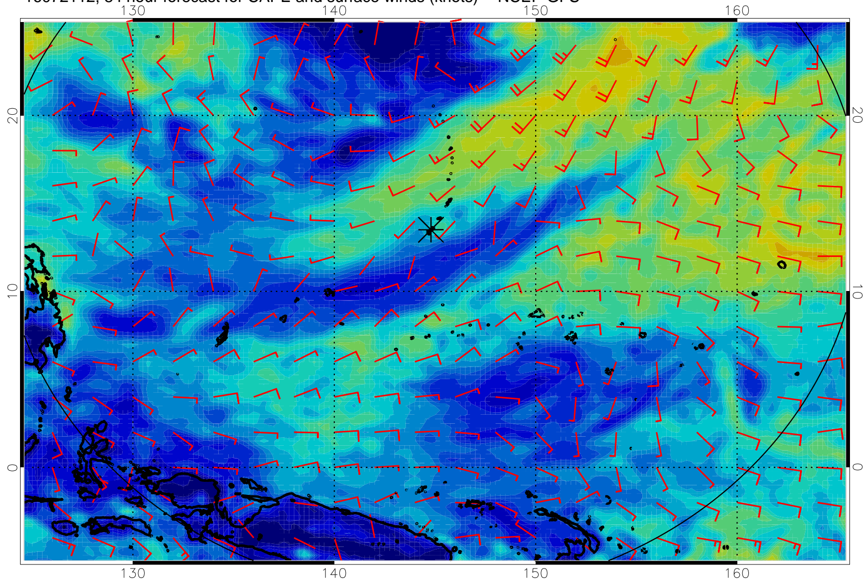
16072112, 84 hour forecast for CAPE and surface winds (knots) -- NCEP GFS
