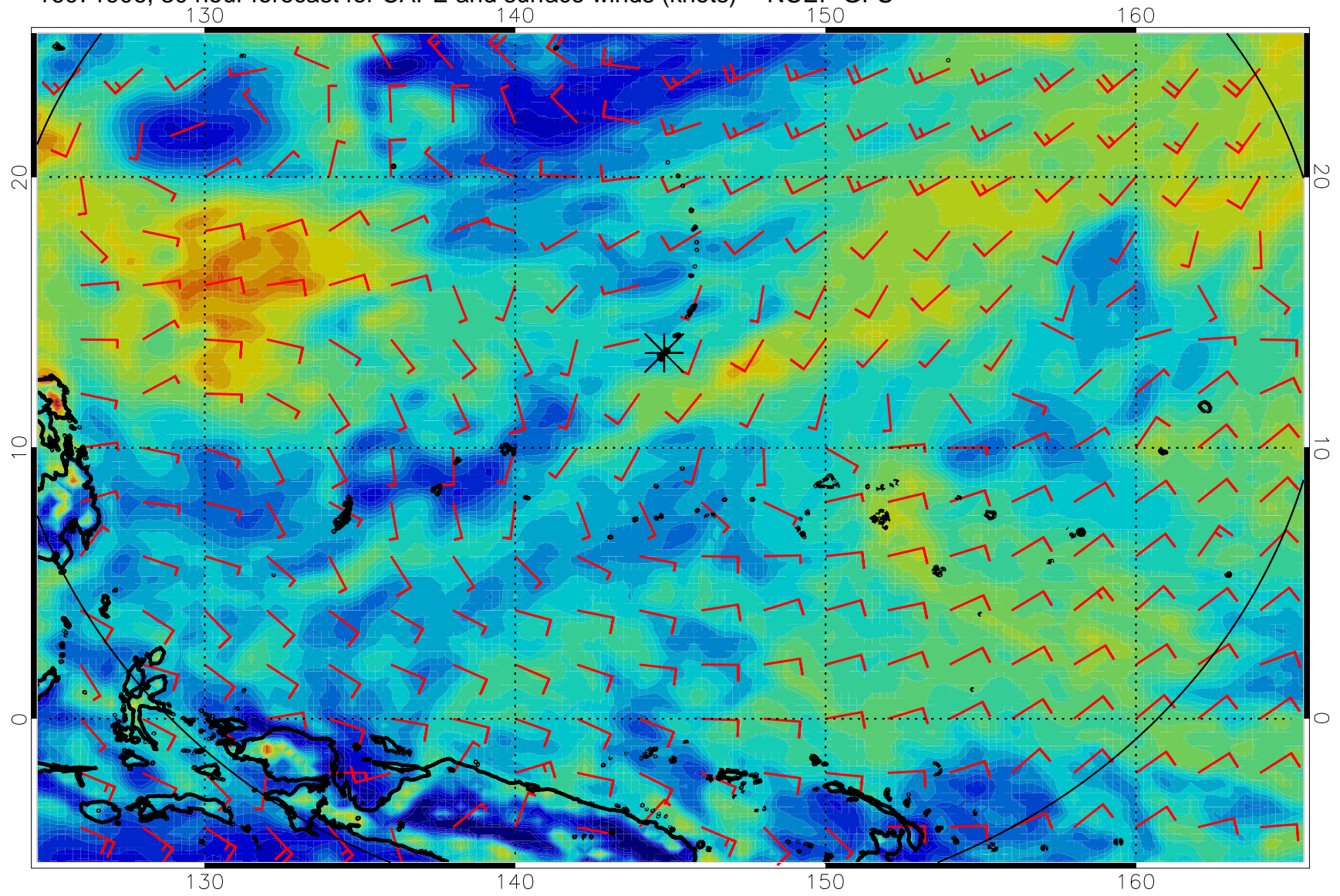
16071906, 30 hour forecast for CAPE and surface winds (knots) -- NCEP GFS
