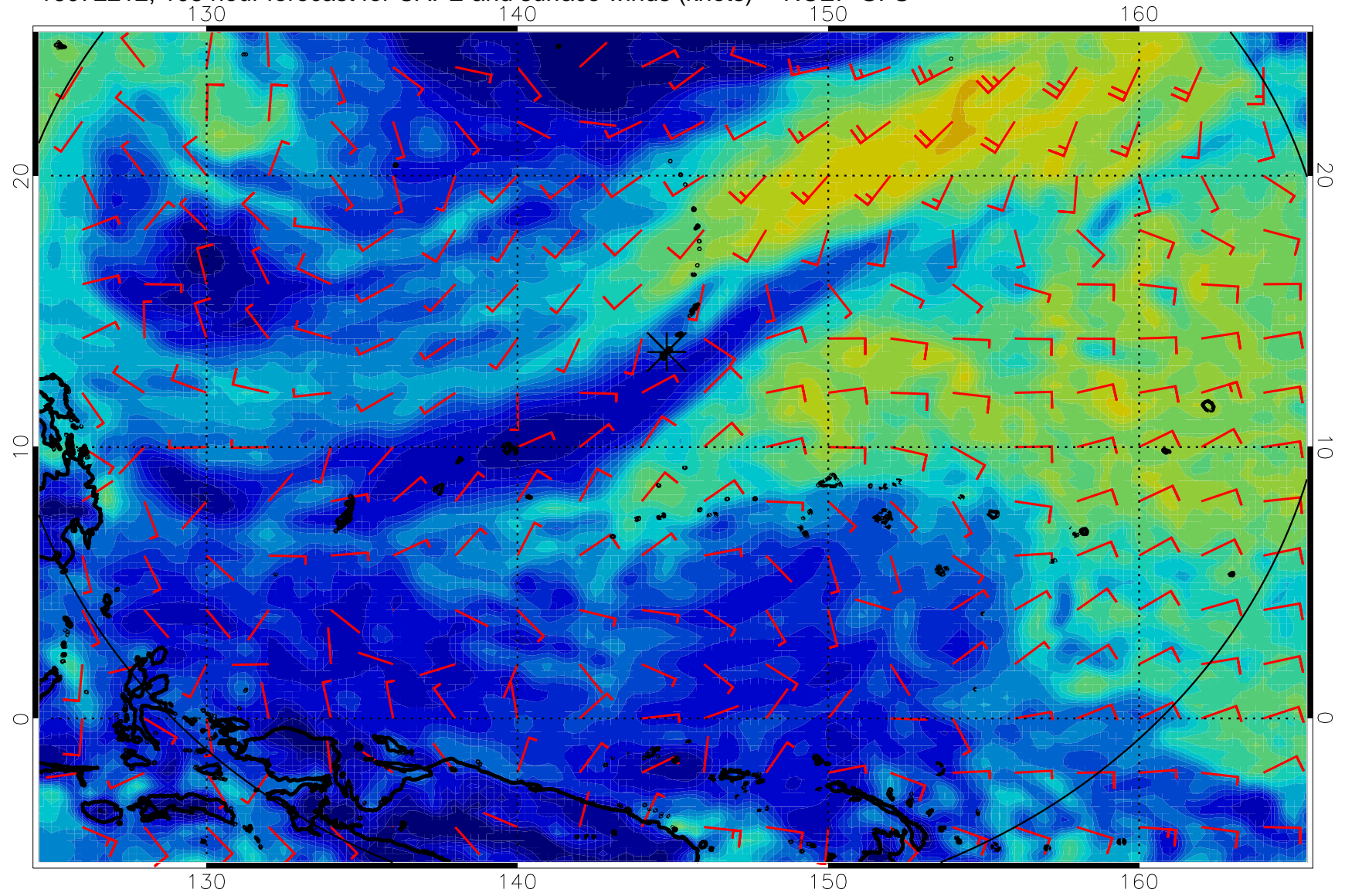
16072212, 108 hour forecast for CAPE and surface winds (knots) -- NCEP GFS
