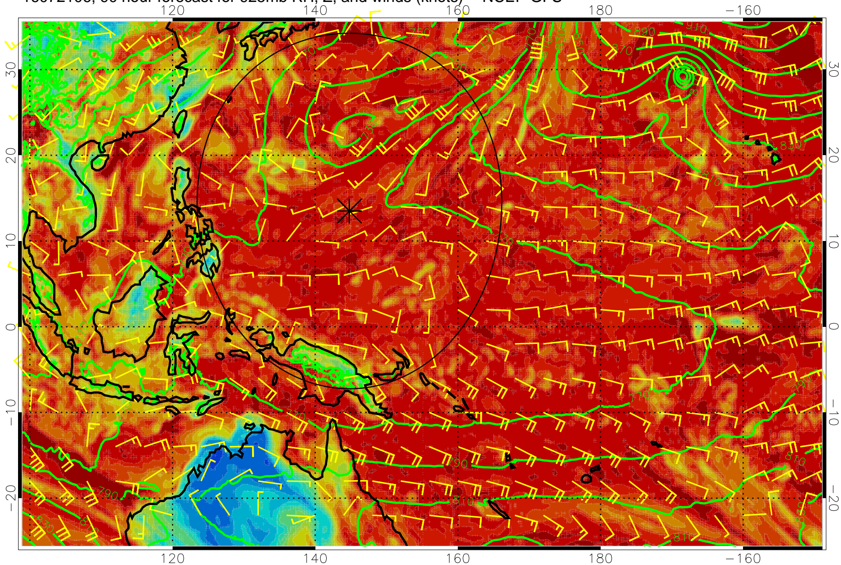
16072106, 90 hour forecast for 925mb RH, Z, and winds (knots) -- NCEP GFS
