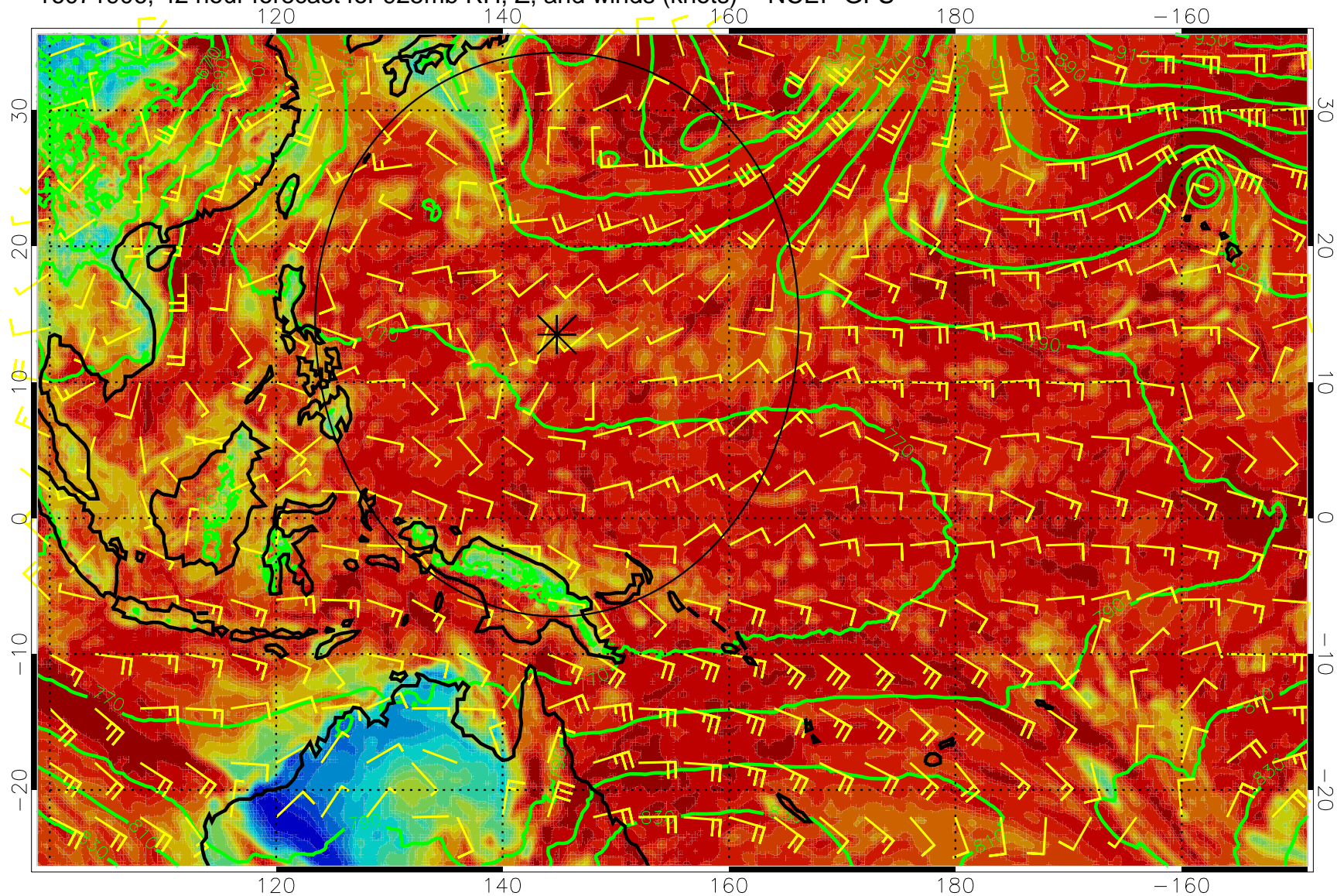
16071906, 42 hour forecast for 925mb RH, Z, and winds (knots) -- NCEP GFS
