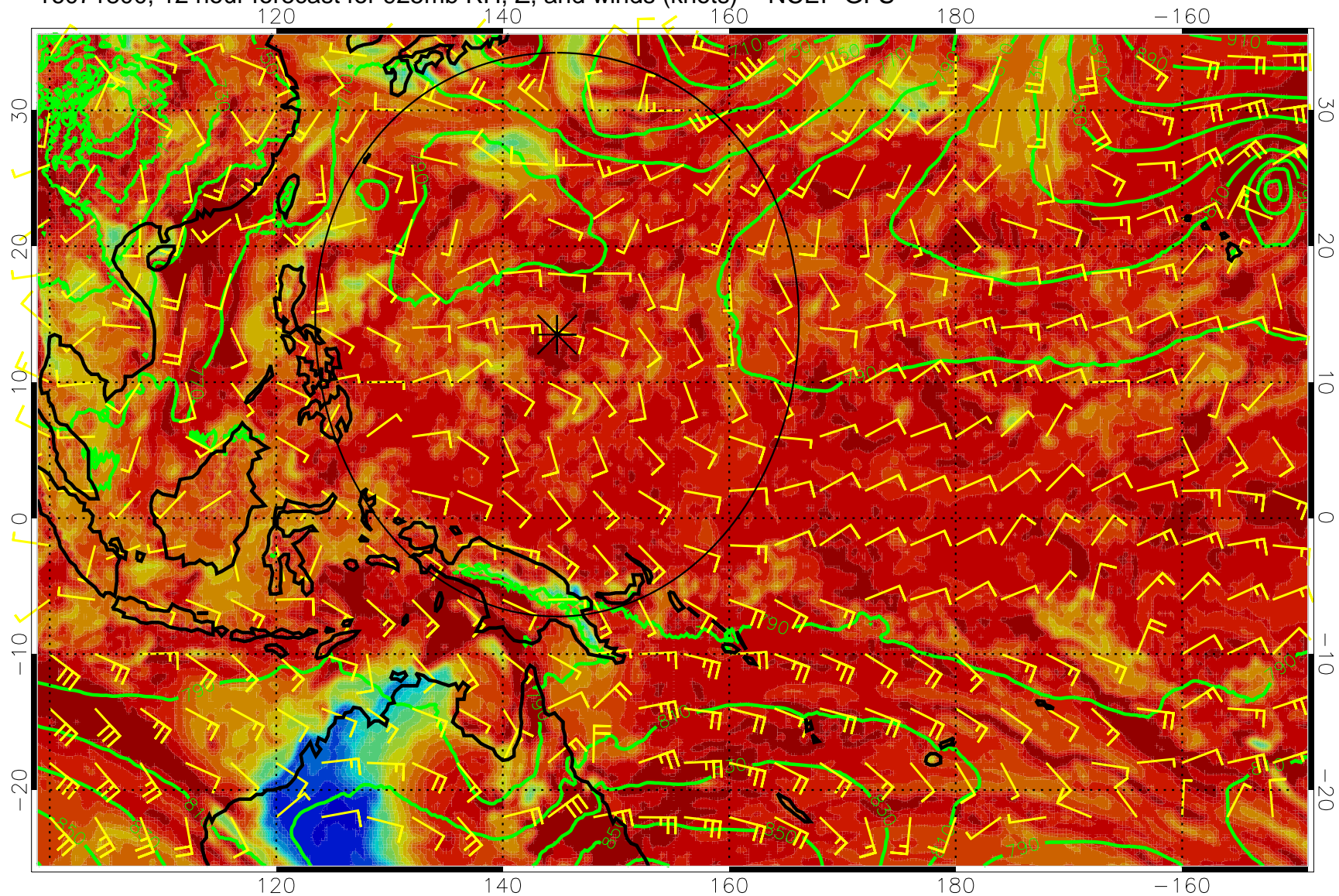
16071800, 12 hour forecast for 925mb RH, Z, and winds (knots) -- NCEP GFS
