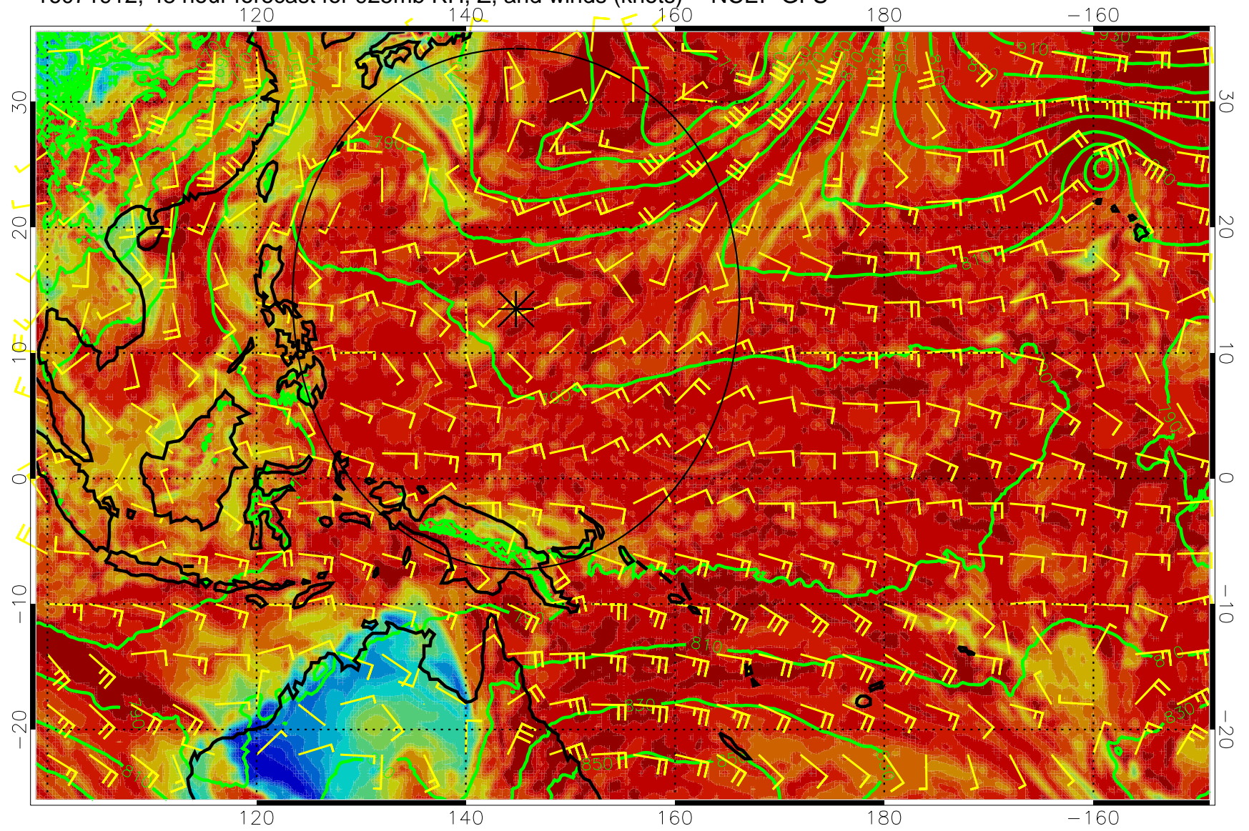
16071912, 48 hour forecast for 925mb RH, Z, and winds (knots) -- NCEP GFS
