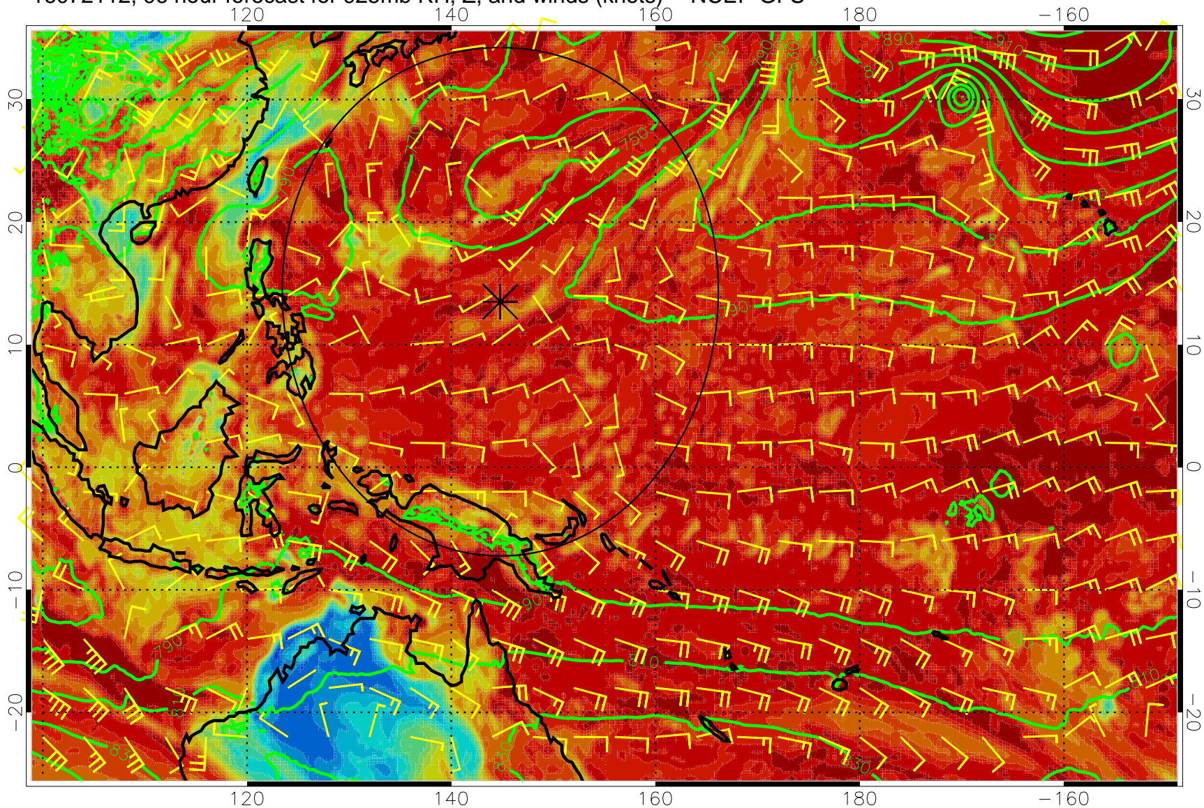
16072112, 96 hour forecast for 925mb RH, Z, and winds (knots) -- NCEP GFS
