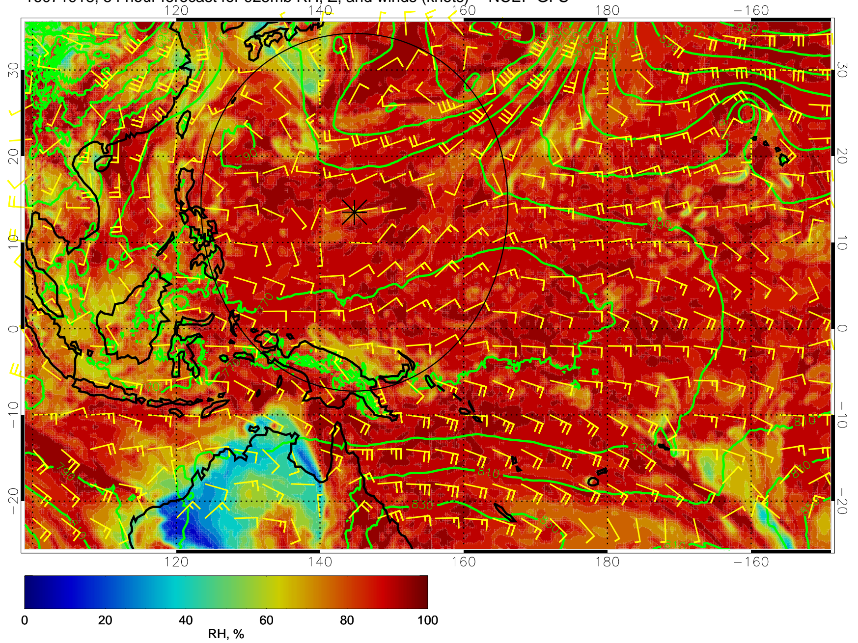
16071918, 54 hour forecast for 925mb RH, Z, and winds (knots) -- NCEP GFS
