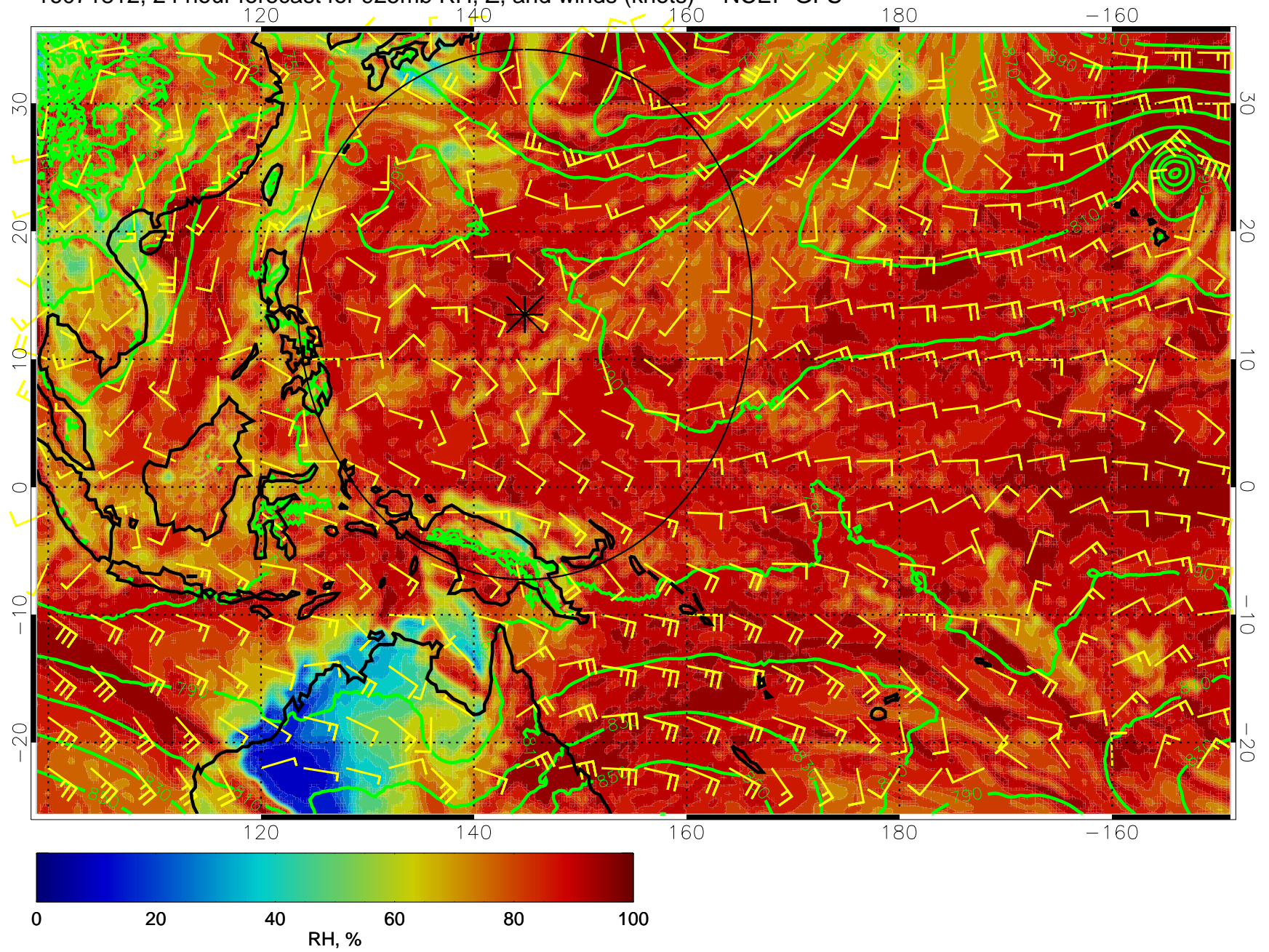
16071812, 24 hour forecast for 925mb RH, Z, and winds (knots) -- NCEP GFS
