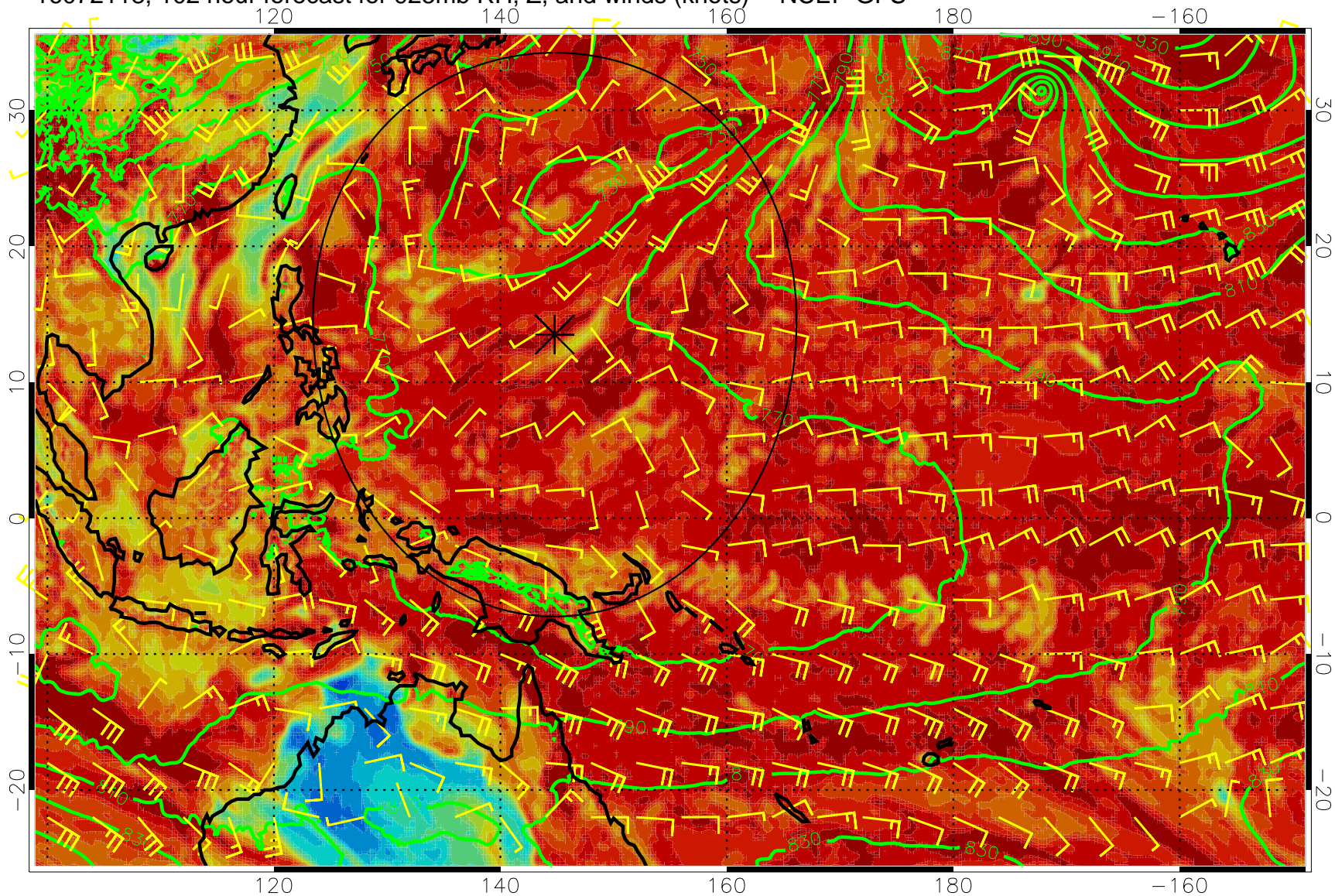
16072118, 102 hour forecast for 925mb RH, Z, and winds (knots) -- NCEP GFS
