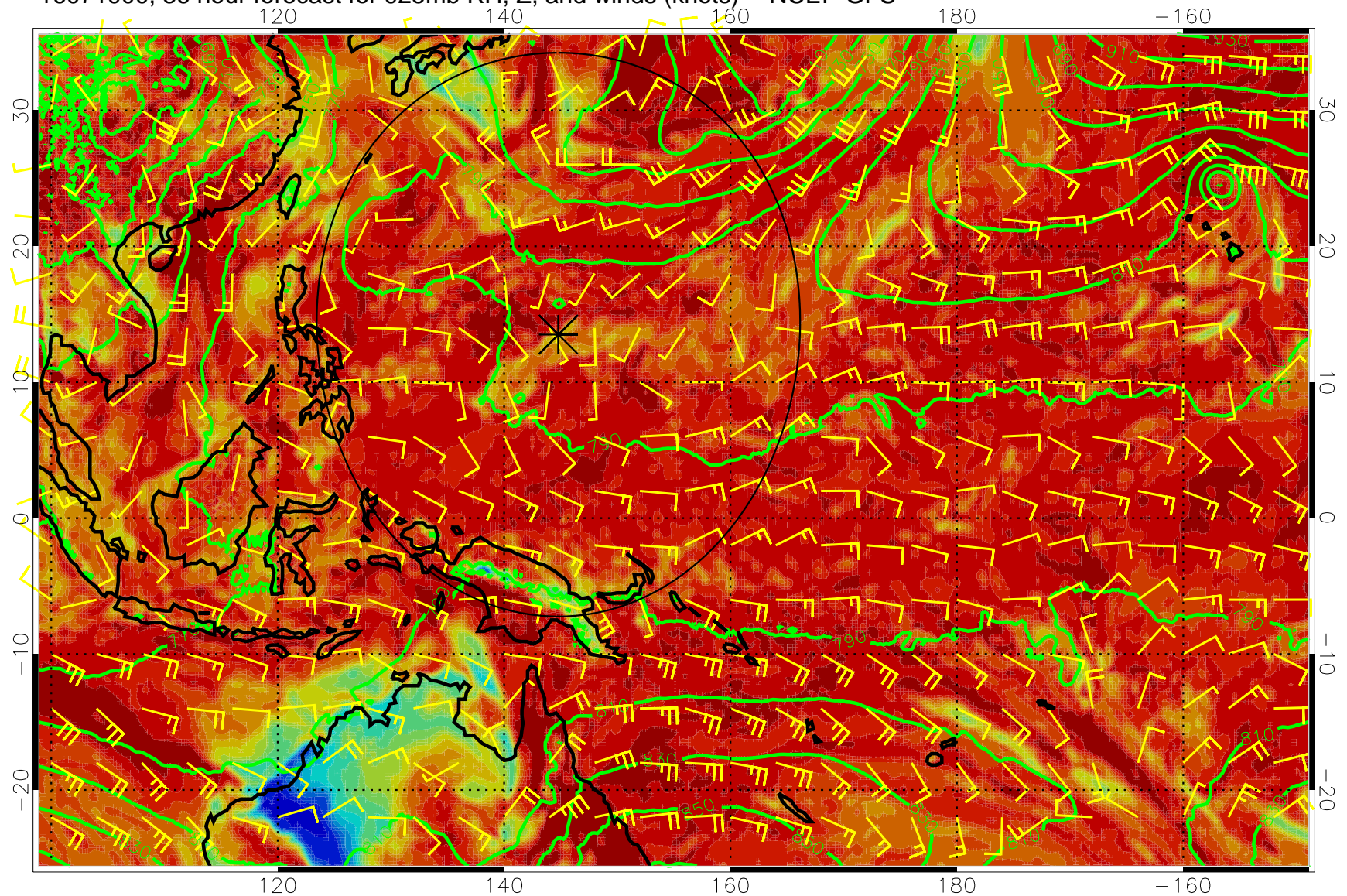
16071900, 36 hour forecast for 925mb RH, Z, and winds (knots) -- NCEP GFS
