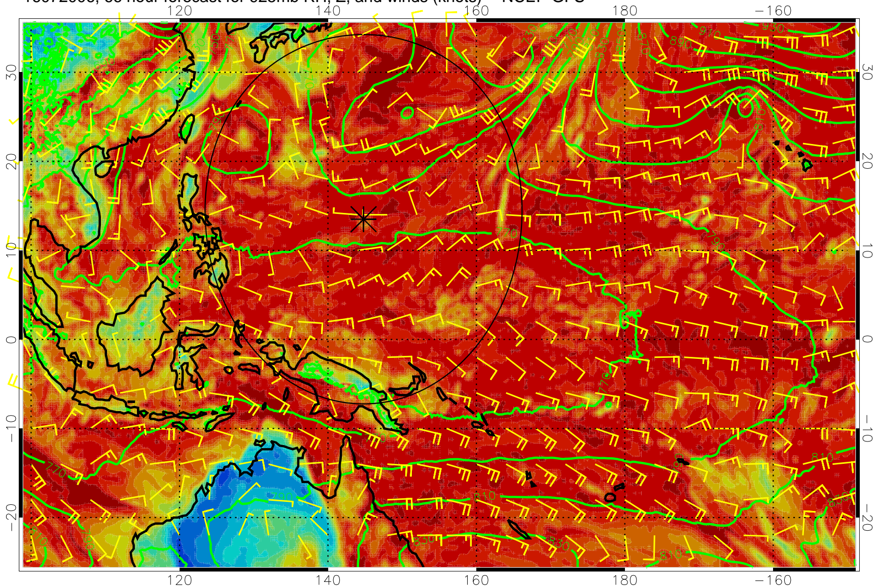
16072006, 66 hour forecast for 925mb RH, Z, and winds (knots) -- NCEP GFS
