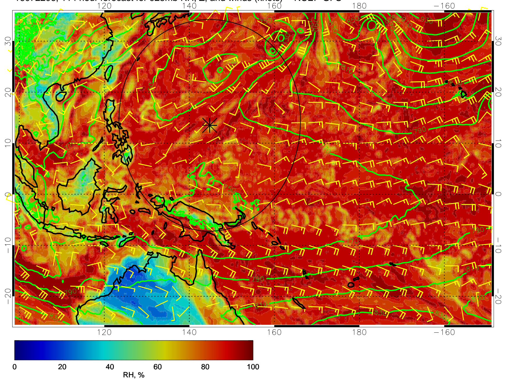
16072206, 114 hour forecast for 925mb RH, Z, and winds (knots) -- NCEP GFS
