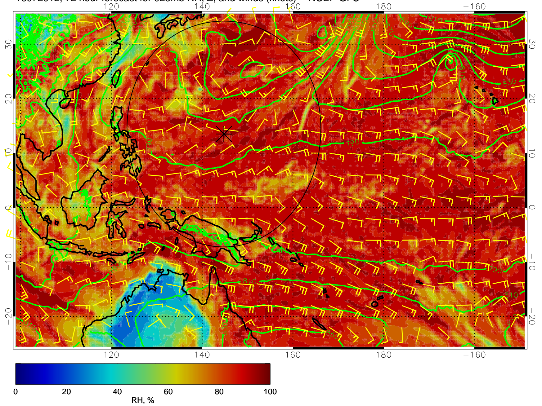
16072012, 72 hour forecast for 925mb RH, Z, and winds (knots) -- NCEP GFS
