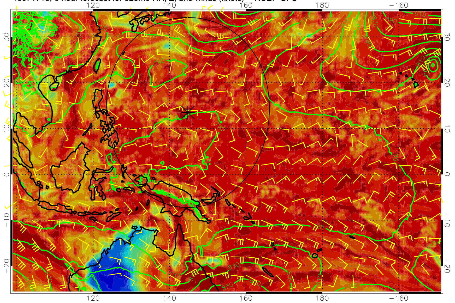
16071718, 6 hour forecast for 925mb RH, Z, and winds (knots) -- NCEP GFS
