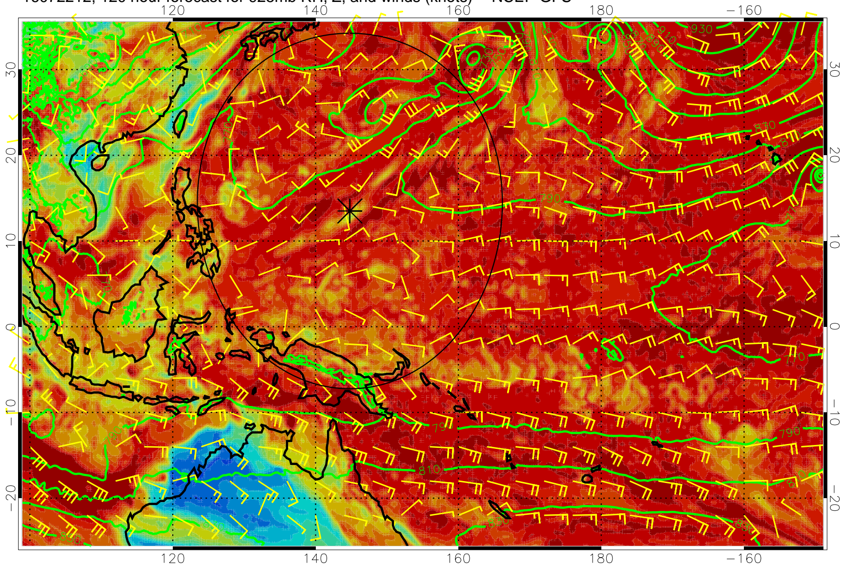
16072212, 120 hour forecast for 925mb RH, Z, and winds (knots) -- NCEP GFS
