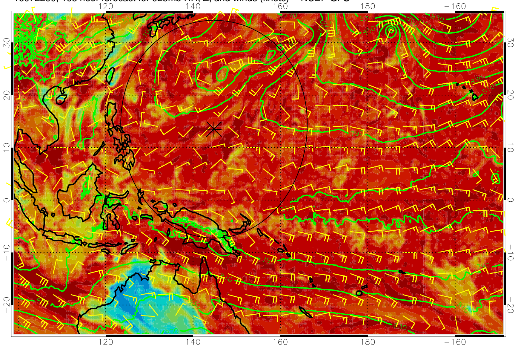
16072200, 108 hour forecast for 925mb RH, Z, and winds (knots) -- NCEP GFS
