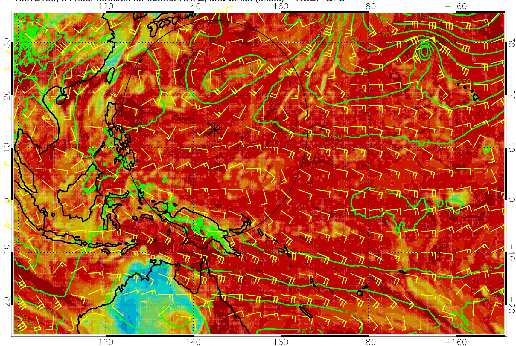
16072100, 84 hour forecast for 925mb RH, Z, and winds (knots) -- NCEP GFS
