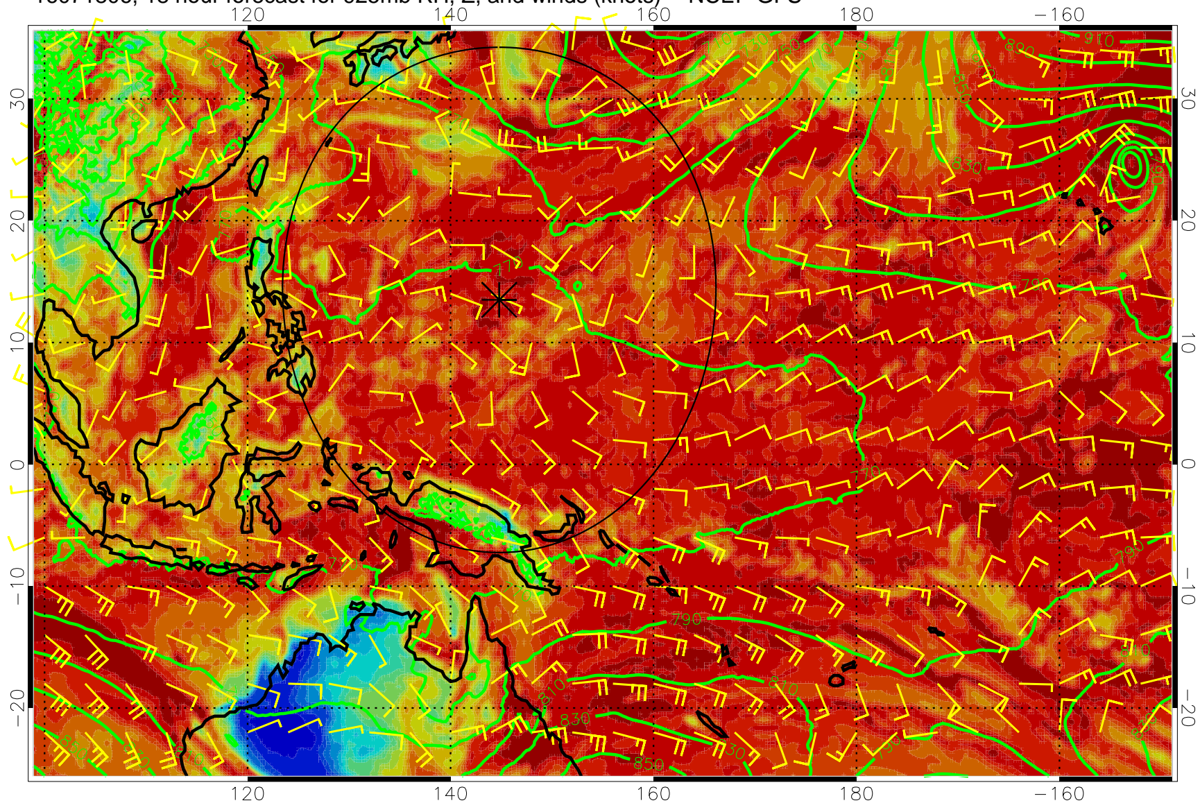
16071806, 18 hour forecast for 925mb RH, Z, and winds (knots) -- NCEP GFS
