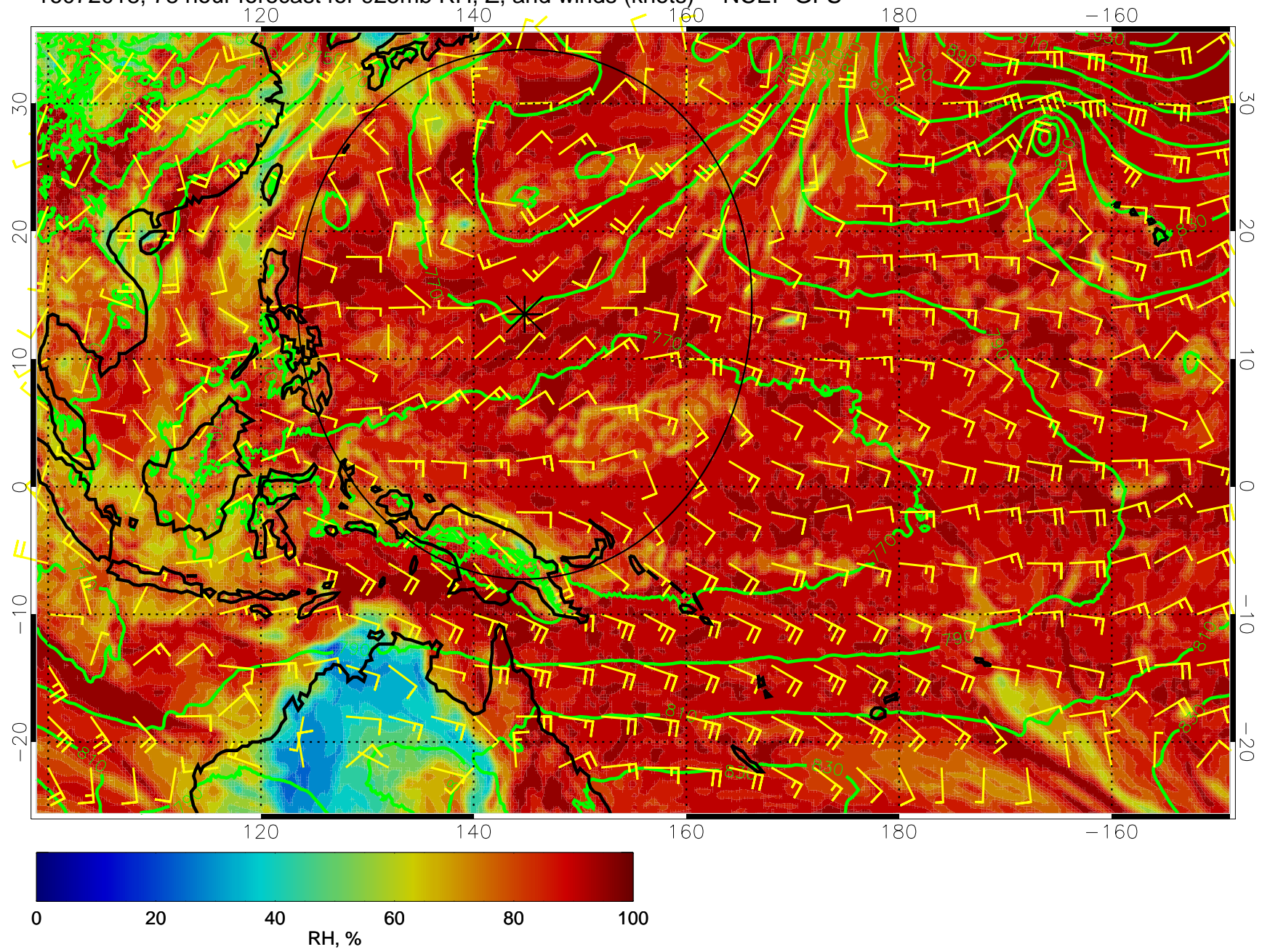
16072018, 78 hour forecast for 925mb RH, Z, and winds (knots) -- NCEP GFS
