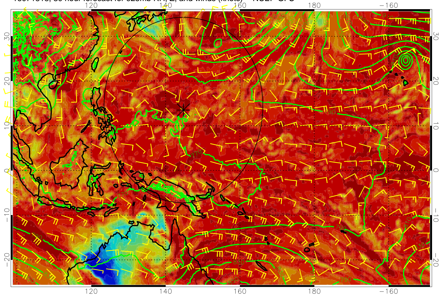
16071818, 30 hour forecast for 925mb RH, Z, and winds (knots) -- NCEP GFS
