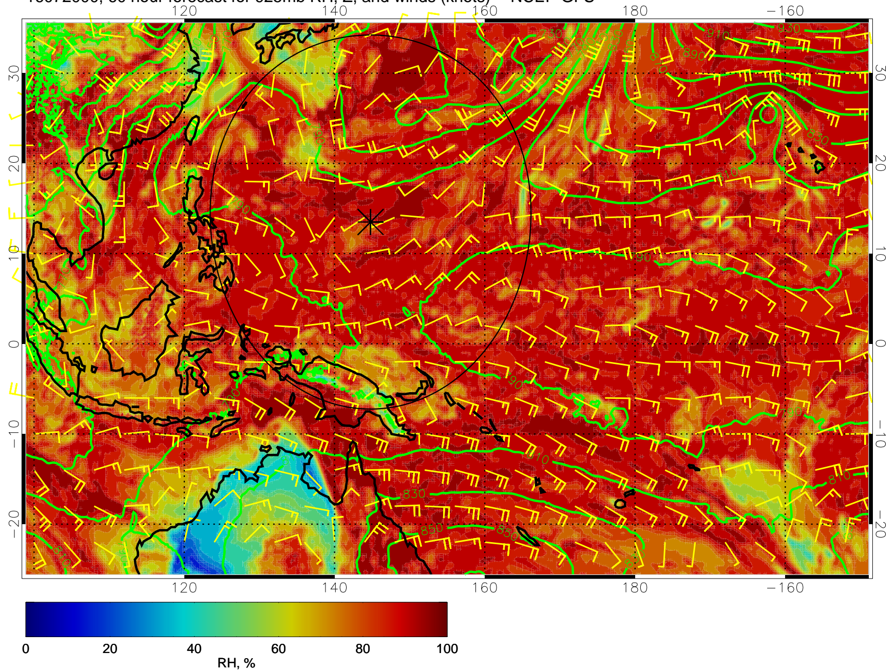
16072000, 60 hour forecast for 925mb RH, Z, and winds (knots) -- NCEP GFS
