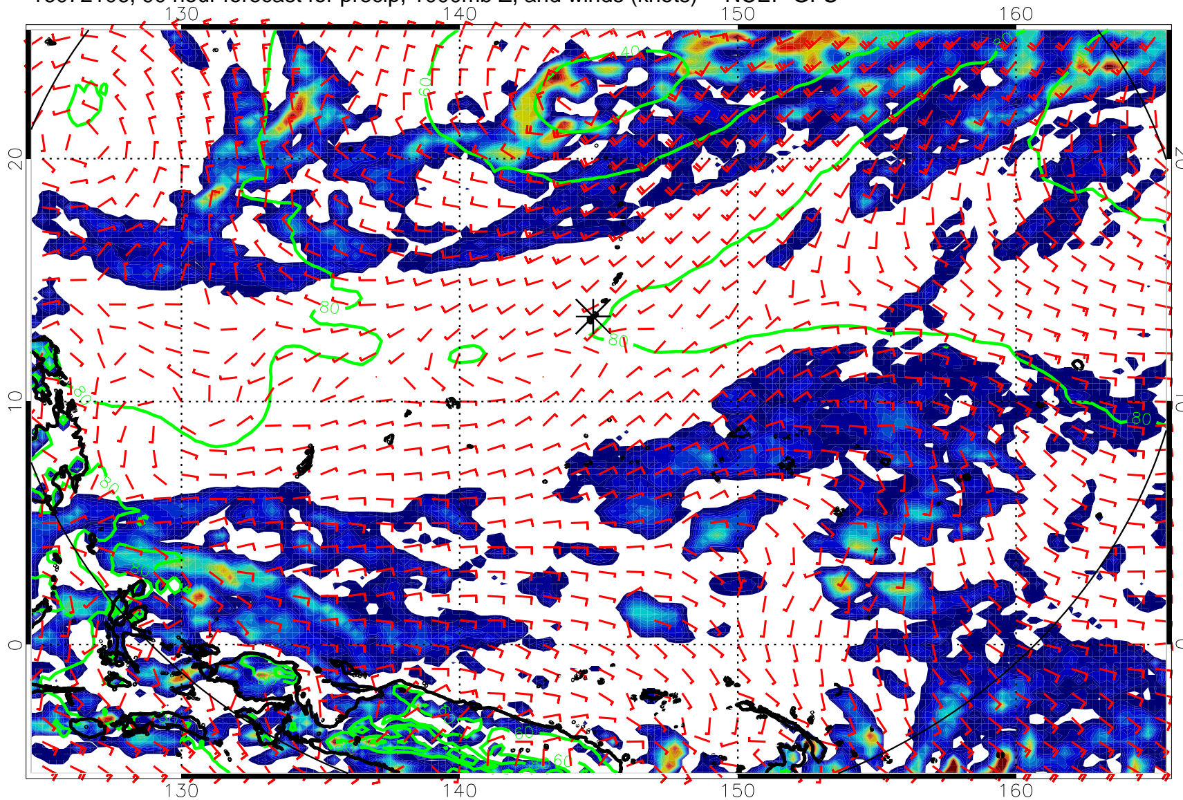
16072106, 90 hour forecast for precip, 1000mb Z, and winds (knots) -- NCEP GFS
