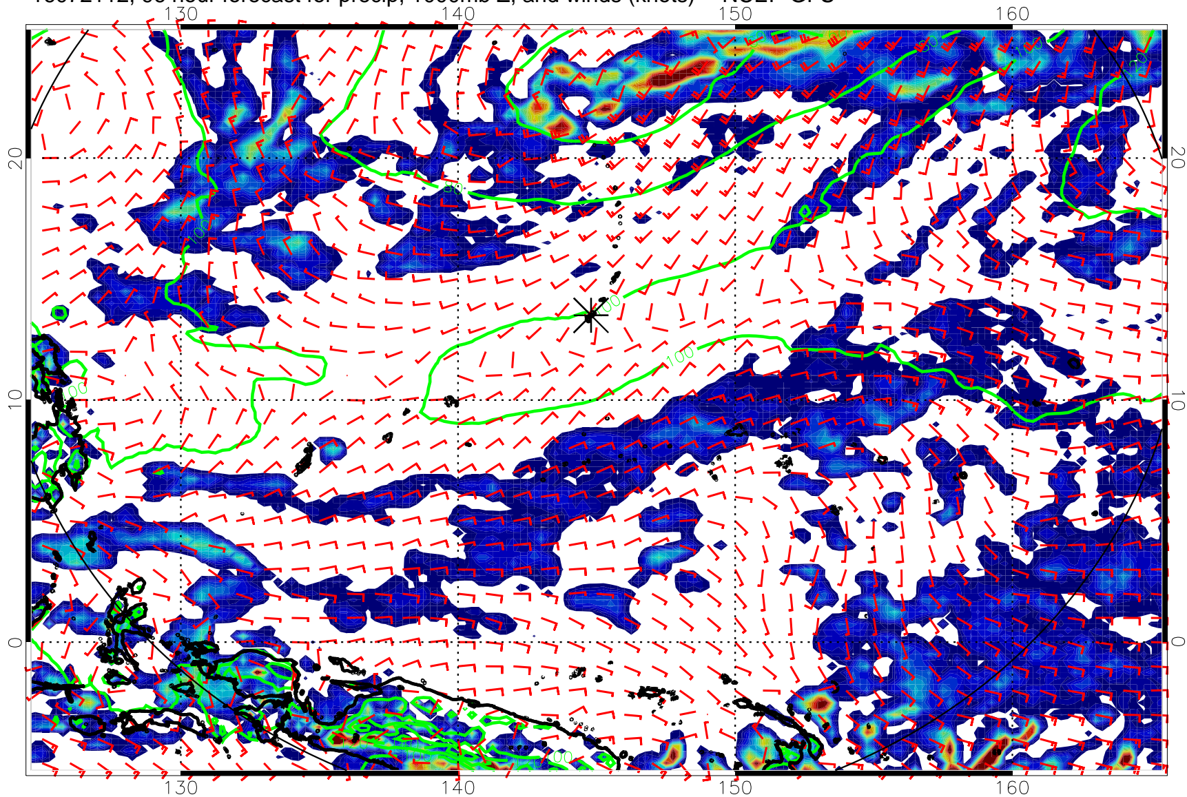
16072112, 96 hour forecast for precip, 1000mb Z, and winds (knots) -- NCEP GFS
