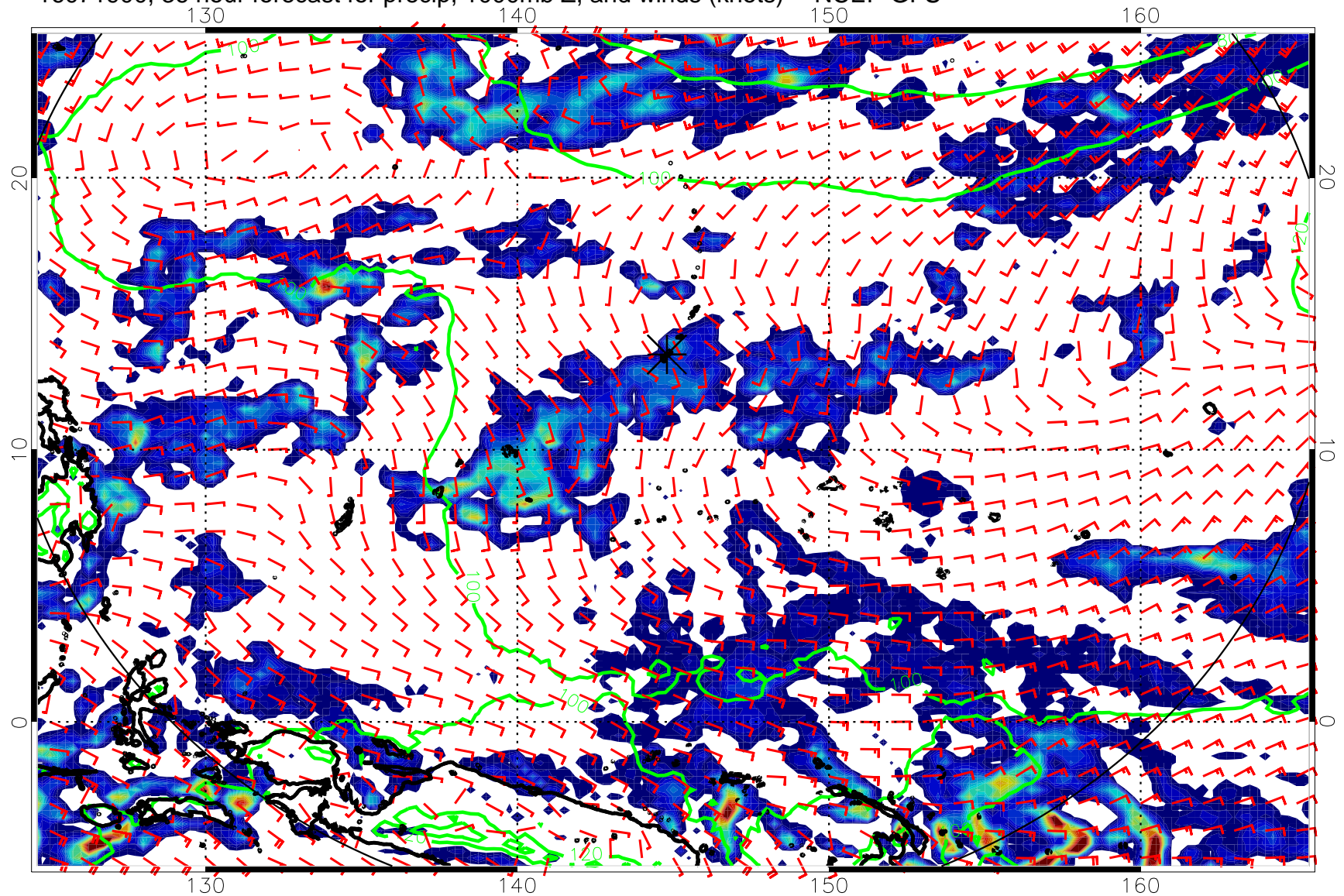
16071900, 36 hour forecast for precip, 1000mb Z, and winds (knots) -- NCEP GFS
