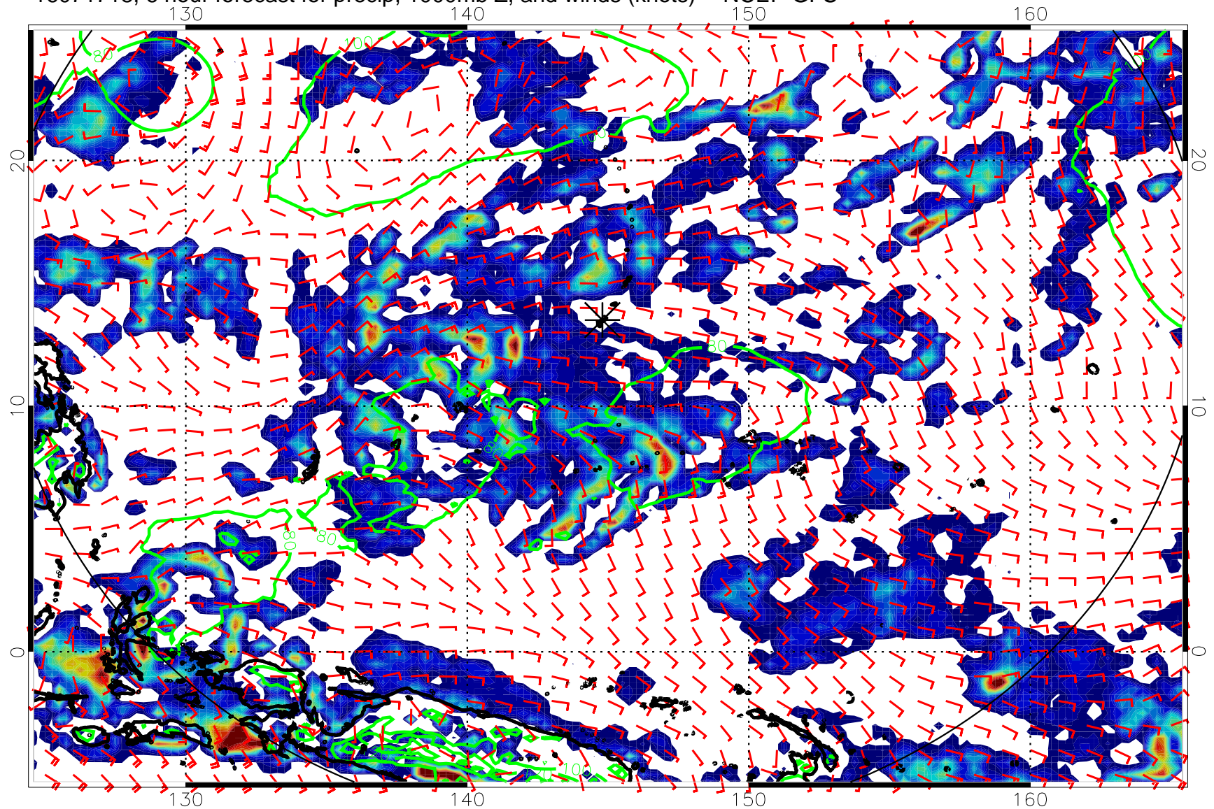
16071718, 6 hour forecast for precip, 1000mb Z, and winds (knots) -- NCEP GFS
