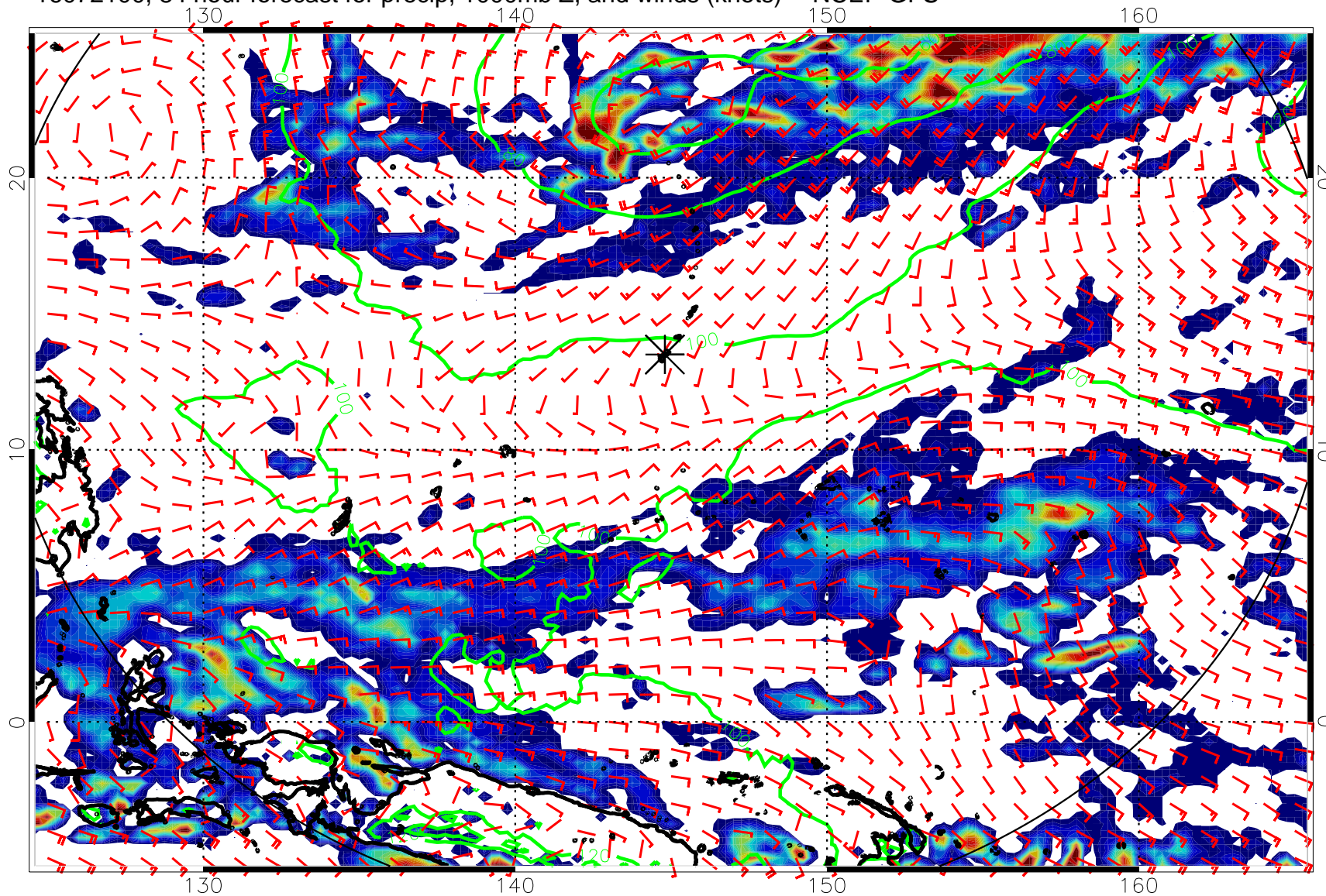
16072100, 84 hour forecast for precip, 1000mb Z, and winds (knots) -- NCEP GFS
