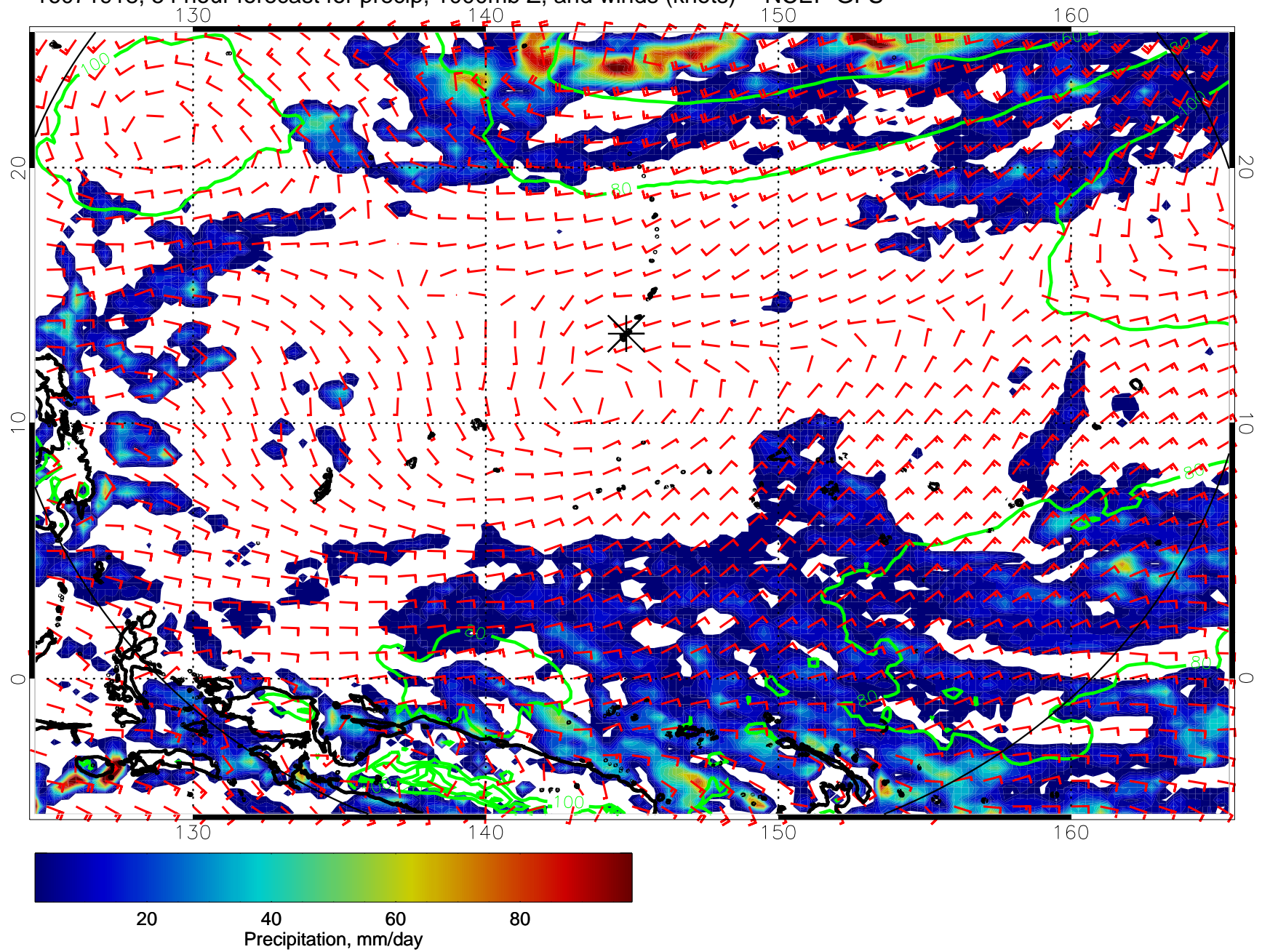
16071918, 54 hour forecast for precip, 1000mb Z, and winds (knots) -- NCEP GFS
