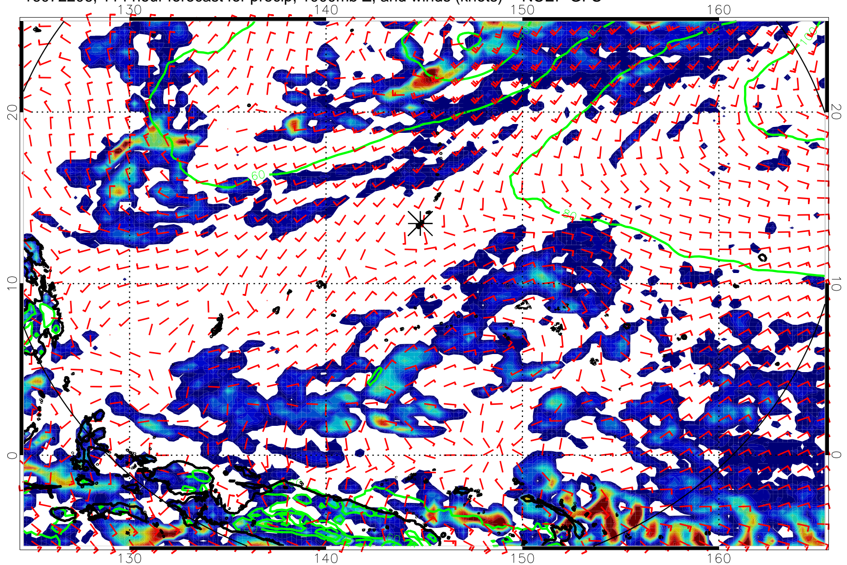
16072206, 114 hour forecast for precip, 1000mb Z, and winds (knots) -- NCEP GFS
