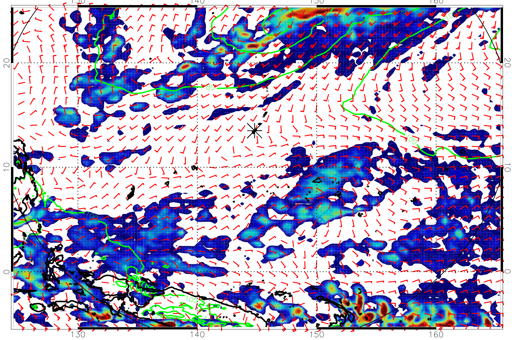
16072200, 108 hour forecast for precip, 1000mb Z, and winds (knots) -- NCEP GFS
