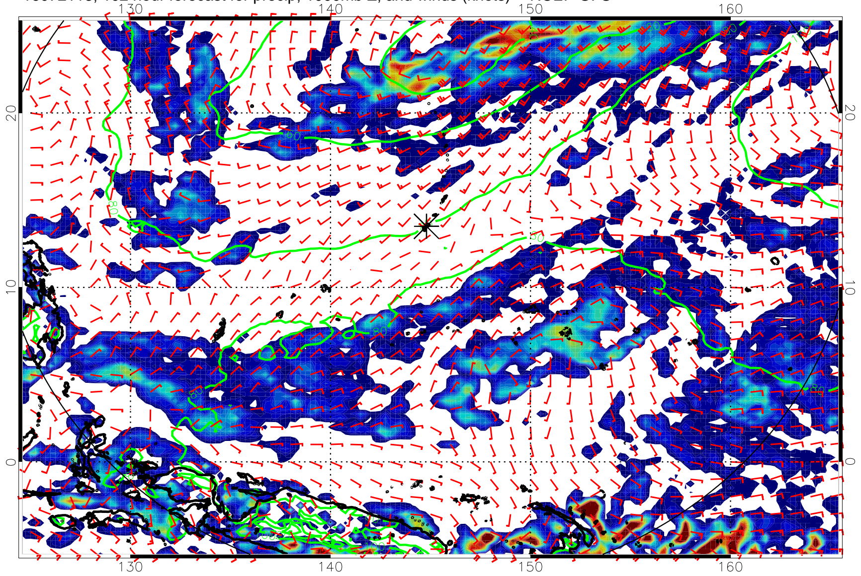
16072118, 102 hour forecast for precip, 1000mb Z, and winds (knots) -- NCEP GFS
