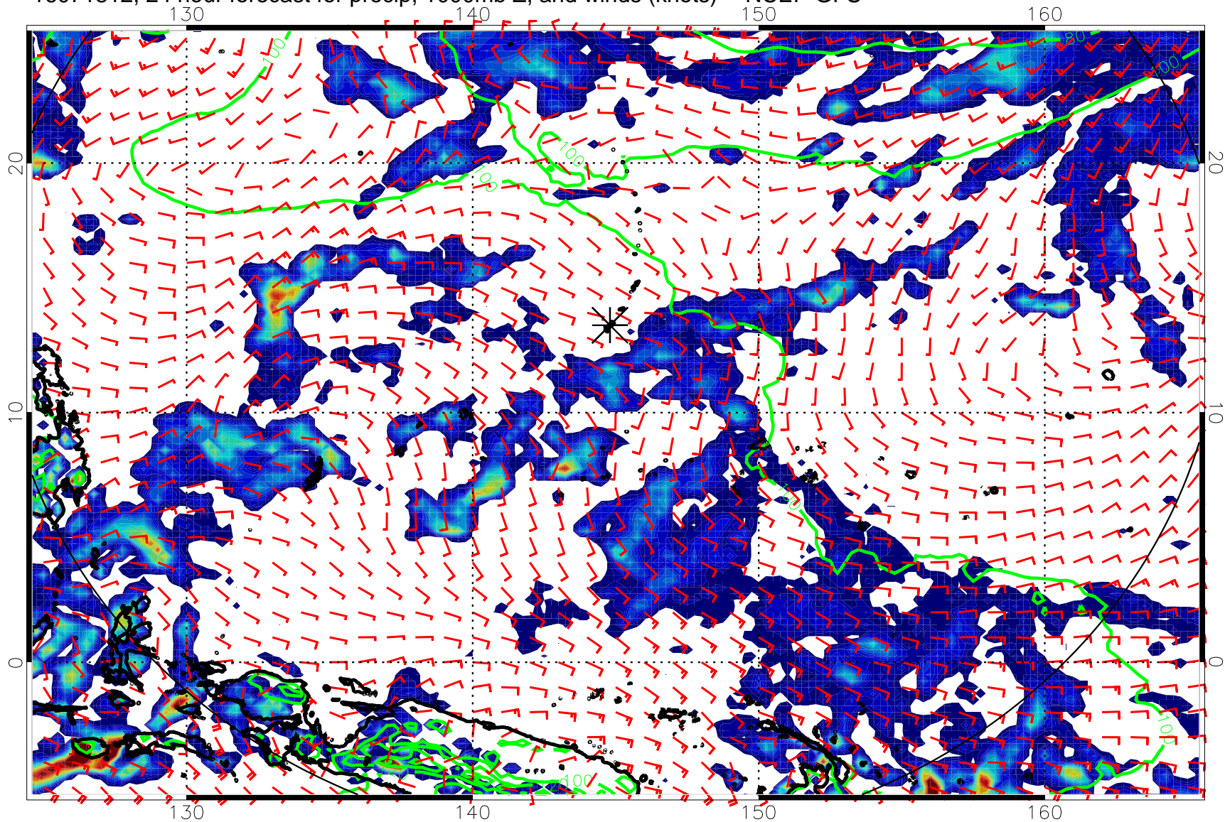
16071812, 24 hour forecast for precip, 1000mb Z, and winds (knots) -- NCEP GFS
