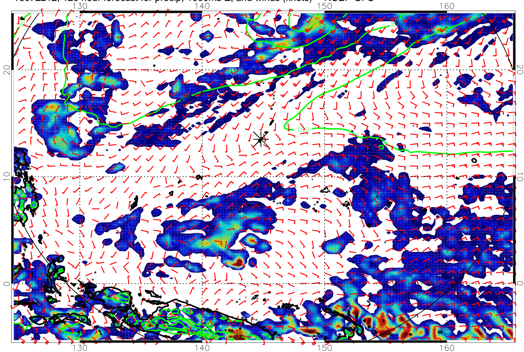
16072212, 120 hour forecast for precip, 1000mb Z, and winds (knots) -- NCEP GFS
