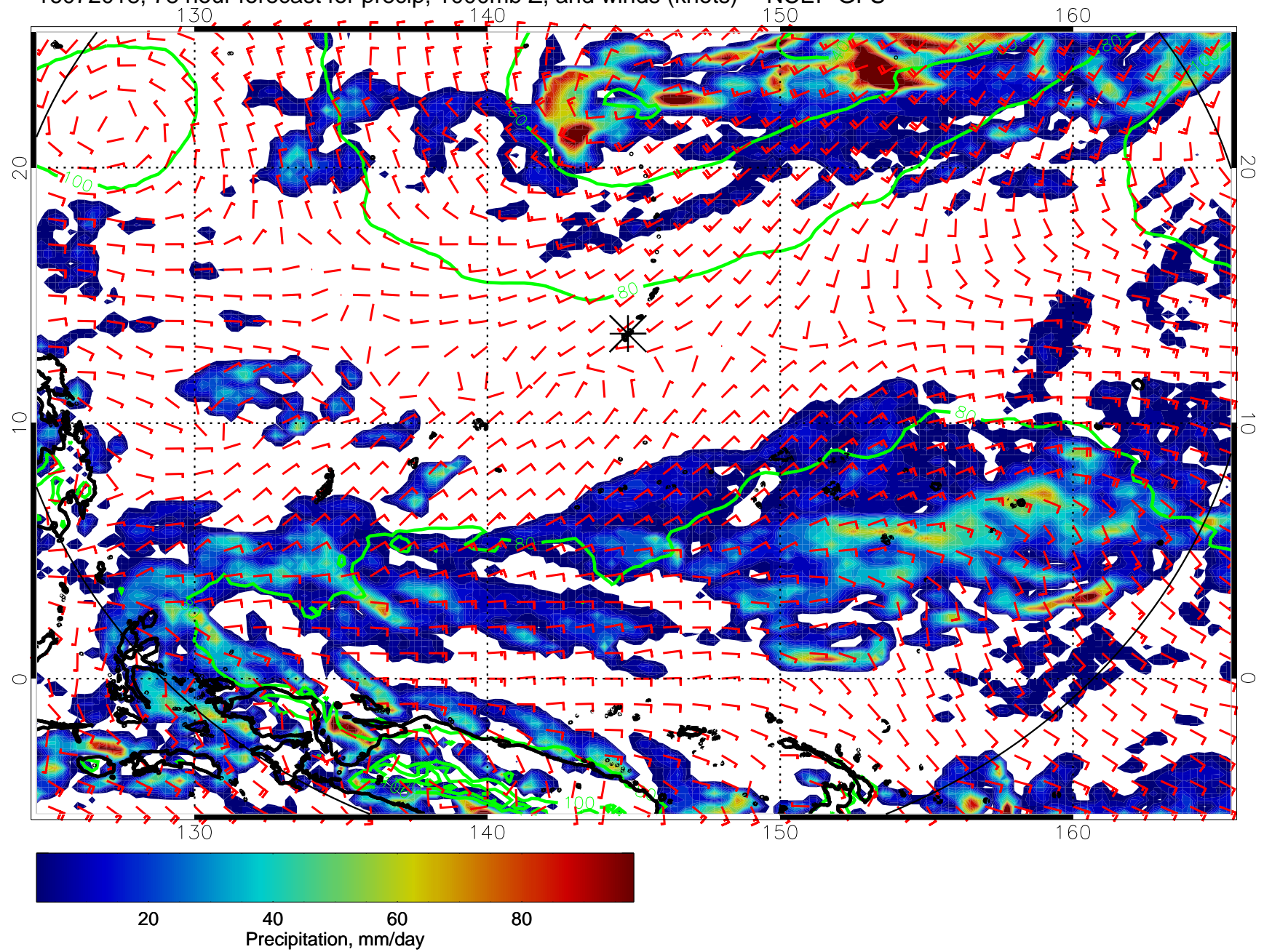
16072018, 78 hour forecast for precip, 1000mb Z, and winds (knots) -- NCEP GFS
