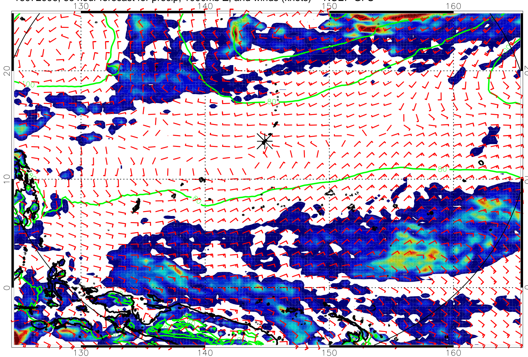
16072006, 66 hour forecast for precip, 1000mb Z, and winds (knots) -- NCEP GFS
