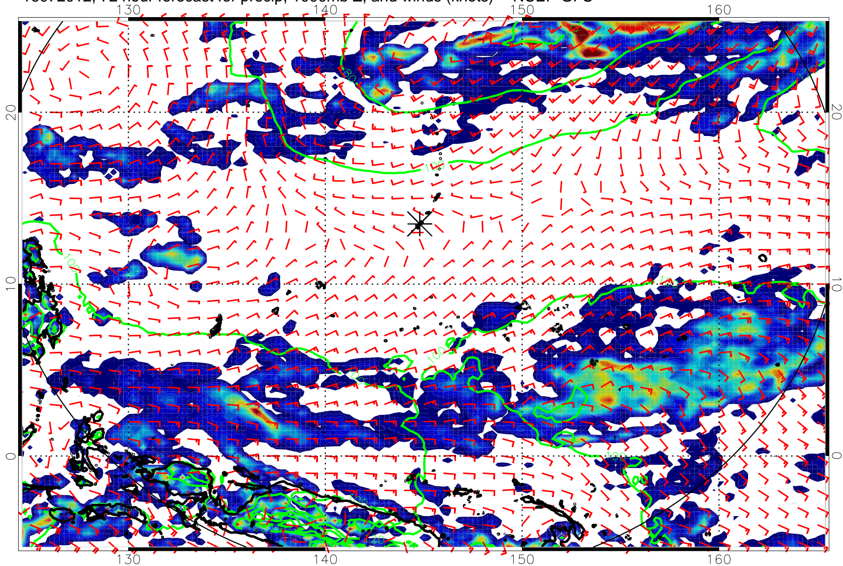
16072012, 72 hour forecast for precip, 1000mb Z, and winds (knots) -- NCEP GFS
