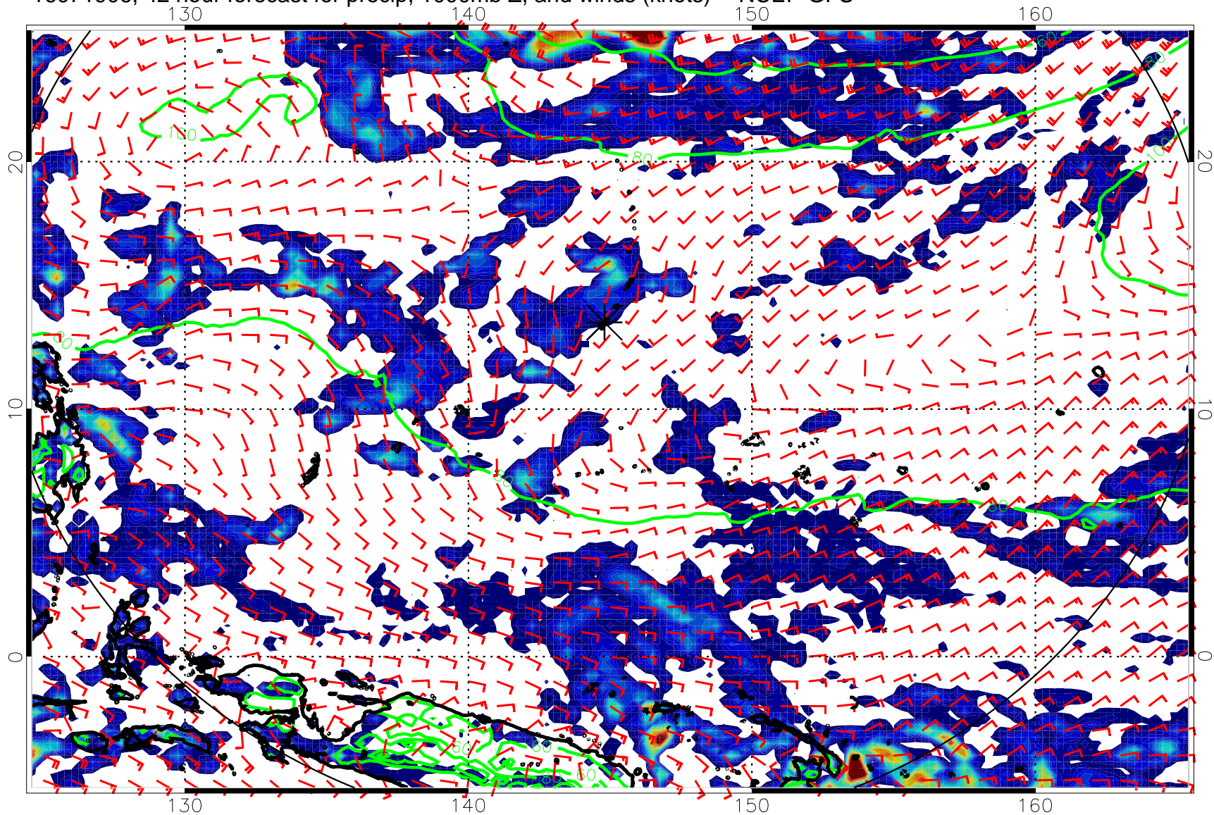
16071906, 42 hour forecast for precip, 1000mb Z, and winds (knots) -- NCEP GFS
