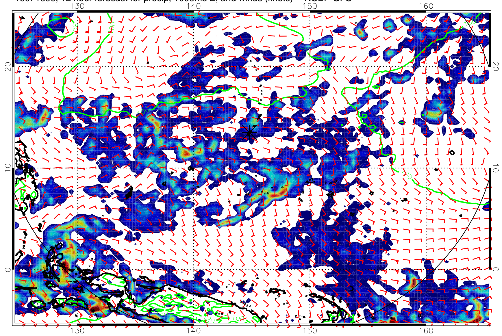
16071800, 12 hour forecast for precip, 1000mb Z, and winds (knots) -- NCEP GFS
