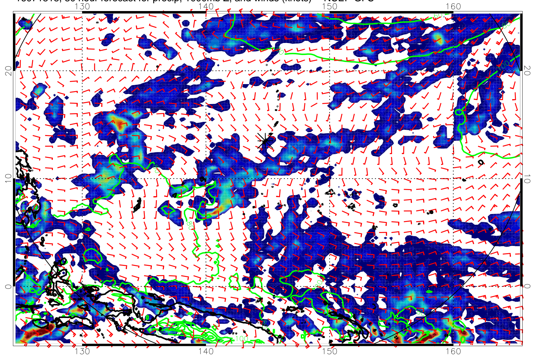
16071818, 30 hour forecast for precip, 1000mb Z, and winds (knots) -- NCEP GFS
