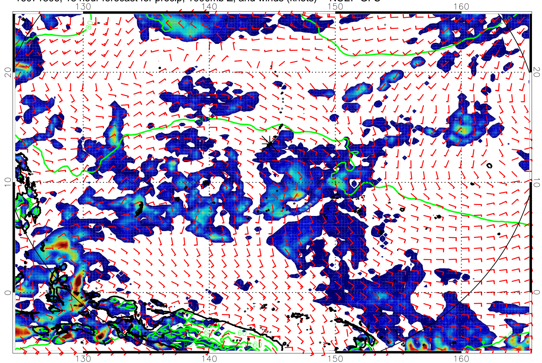
16071806, 18 hour forecast for precip, 1000mb Z, and winds (knots) -- NCEP GFS
