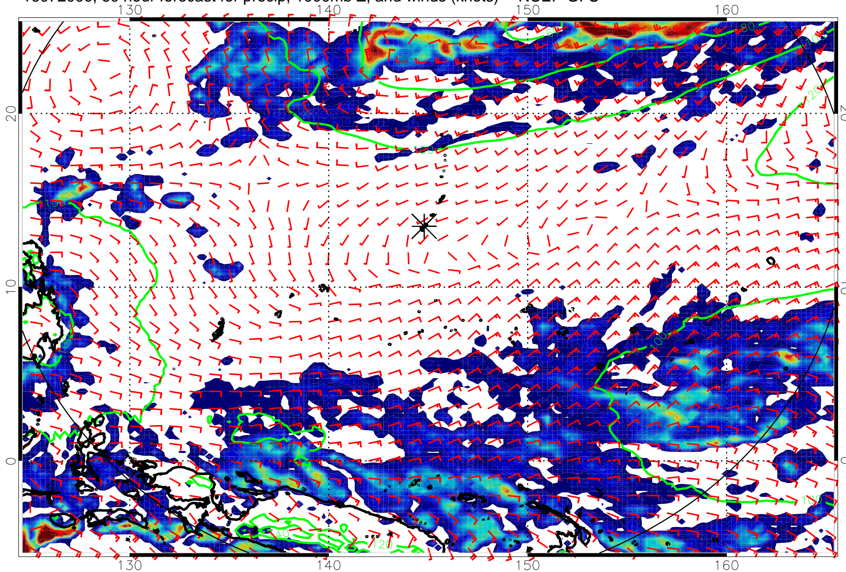
16072000, 60 hour forecast for precip, 1000mb Z, and winds (knots) -- NCEP GFS
