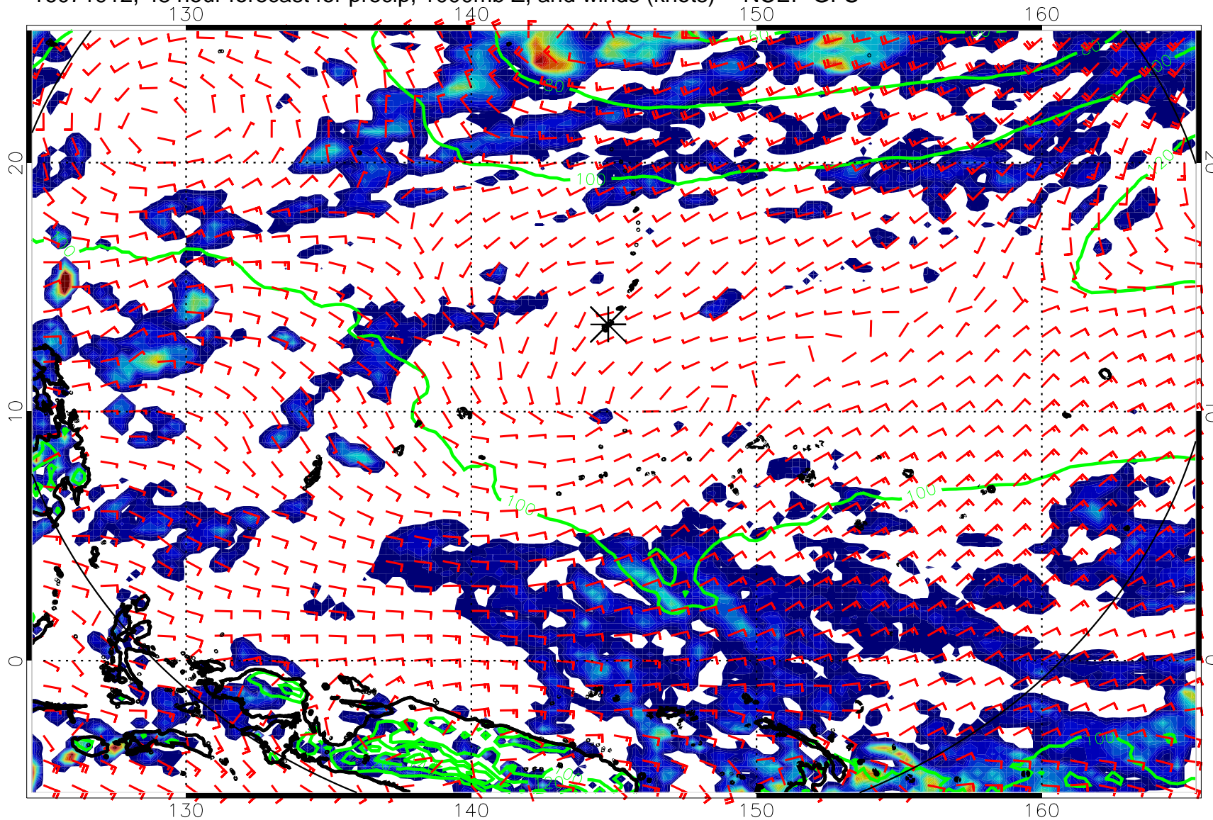
16071912, 48 hour forecast for precip, 1000mb Z, and winds (knots) -- NCEP GFS
