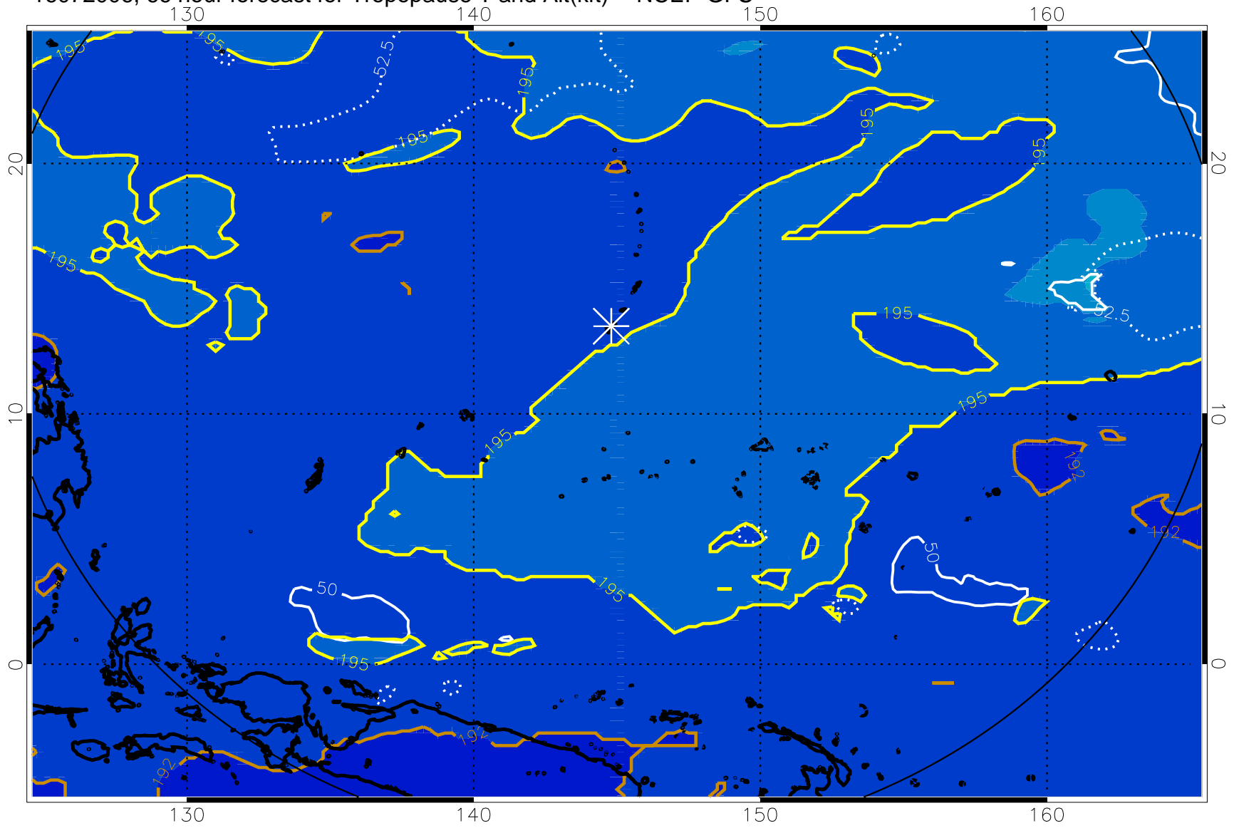
16072006, 66 hour forecast for Tropopause T and Alt(kft) -- NCEP GFS
