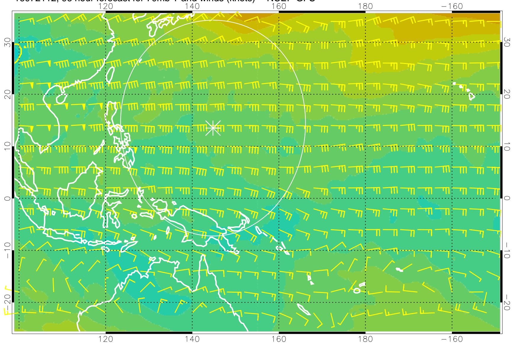
16072112, 96 hour forecast for 70mb T and winds (knots) -- NCEP GFS
