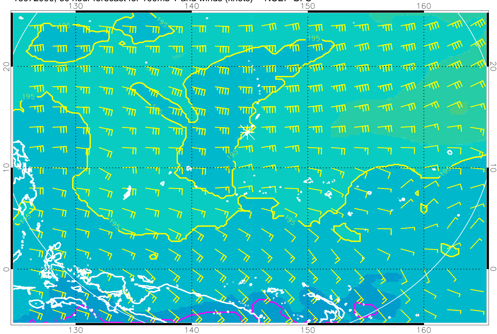
16072000, 60 hour forecast for 100mb T and winds (knots) -- NCEP GFS
