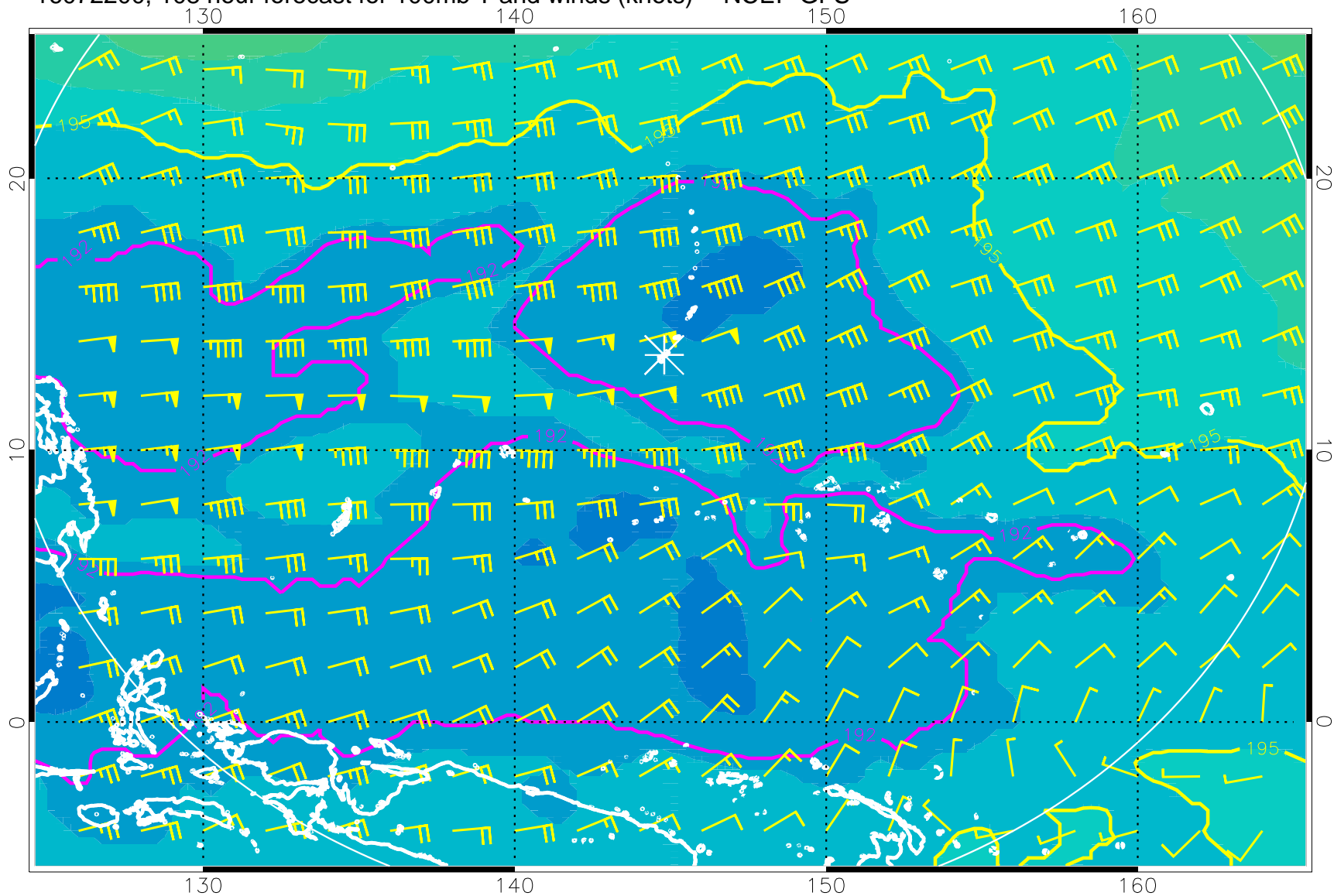
16072200, 108 hour forecast for 100mb T and winds (knots) -- NCEP GFS
