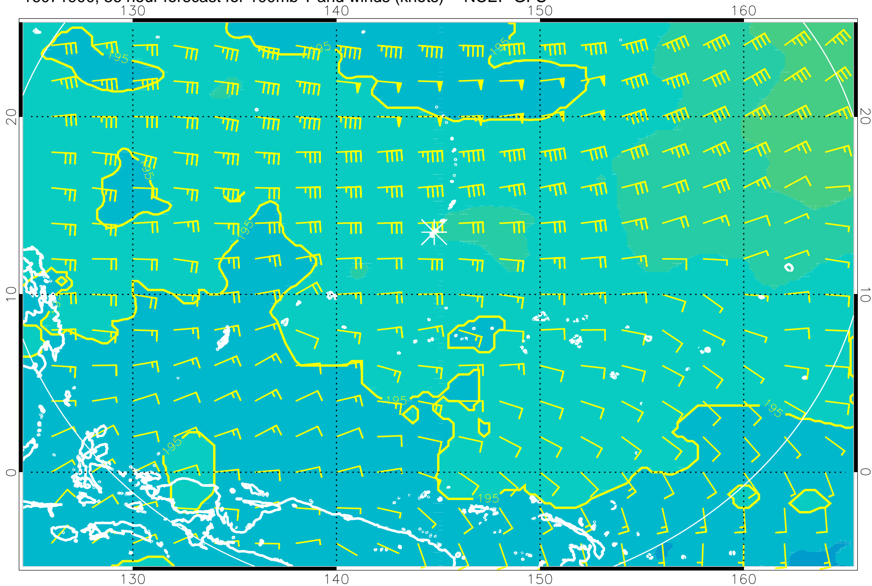
16071900, 36 hour forecast for 100mb T and winds (knots) -- NCEP GFS
