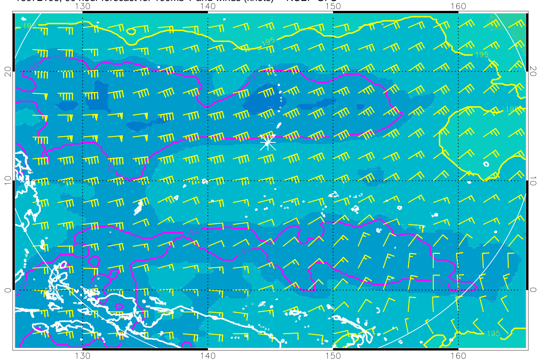
16072106, 90 hour forecast for 100mb T and winds (knots) -- NCEP GFS
