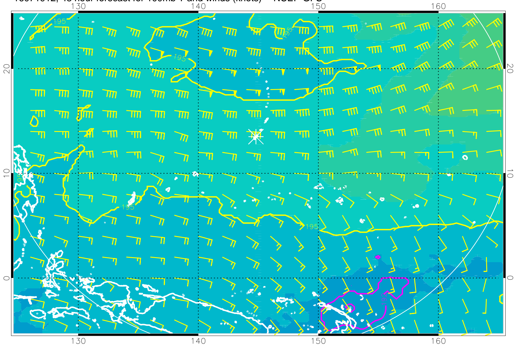
16071912, 48 hour forecast for 100mb T and winds (knots) -- NCEP GFS
