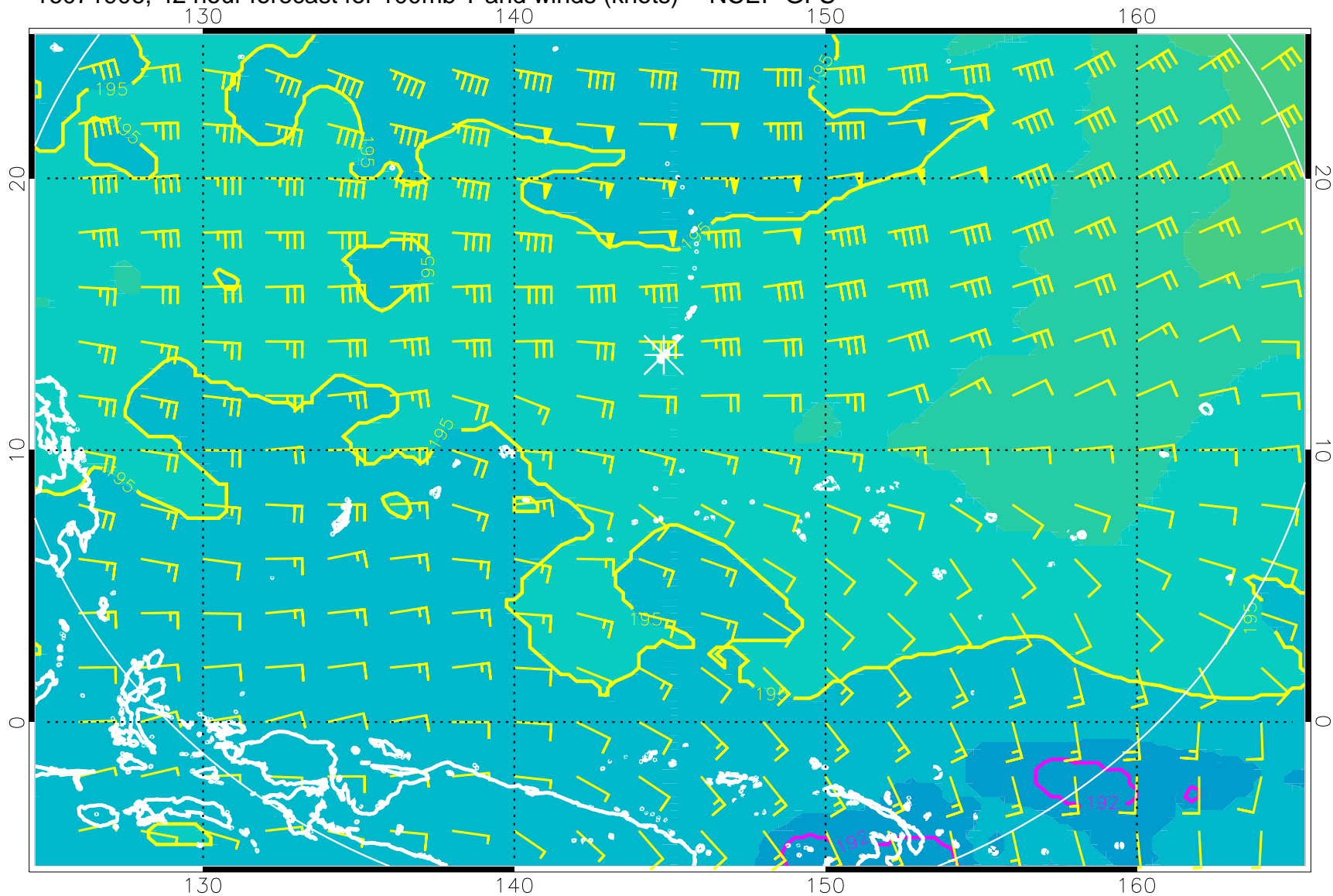
16071906, 42 hour forecast for 100mb T and winds (knots) -- NCEP GFS
