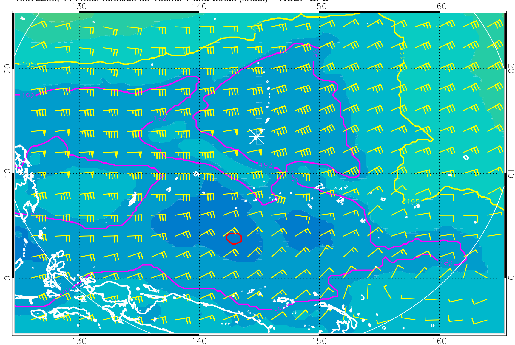
16072206, 114 hour forecast for 100mb T and winds (knots) -- NCEP GFS
