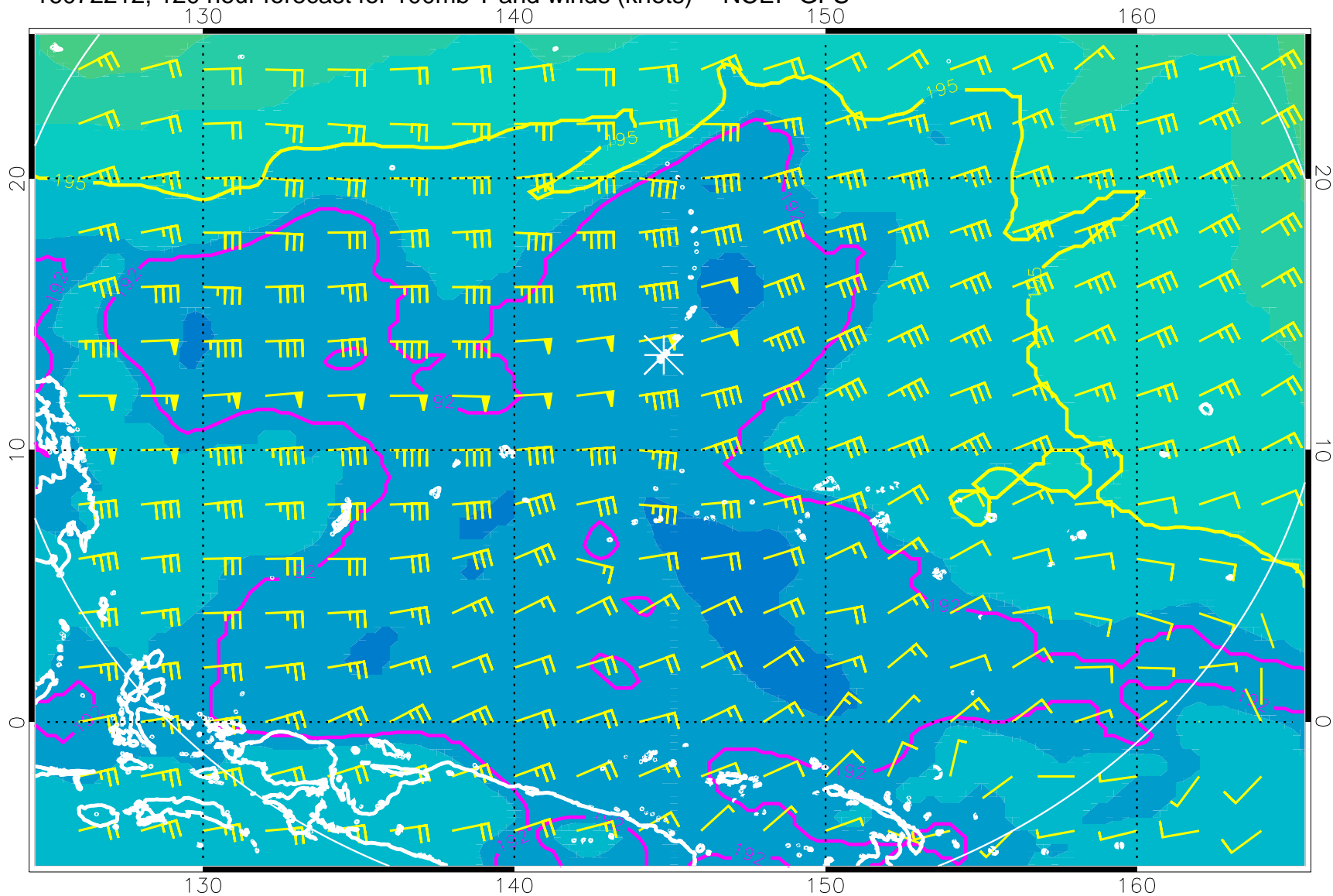
16072212, 120 hour forecast for 100mb T and winds (knots) -- NCEP GFS
