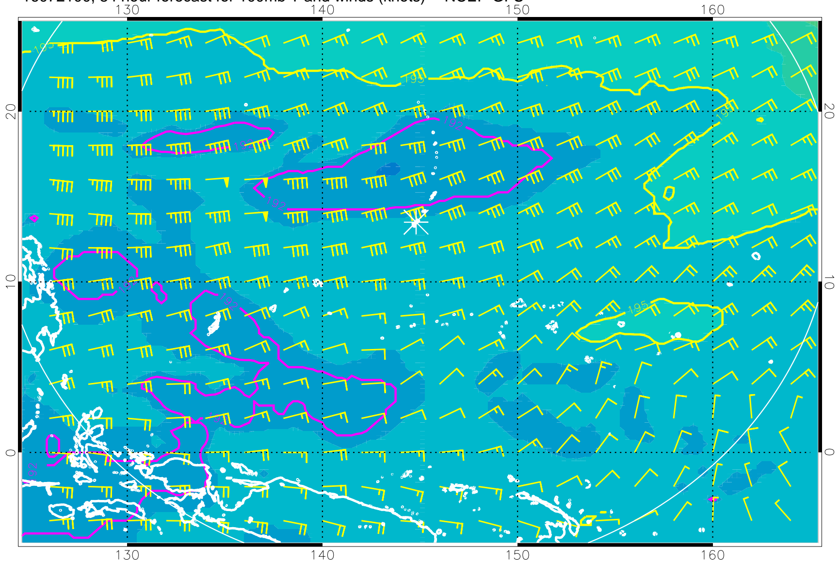
16072100, 84 hour forecast for 100mb T and winds (knots) -- NCEP GFS
