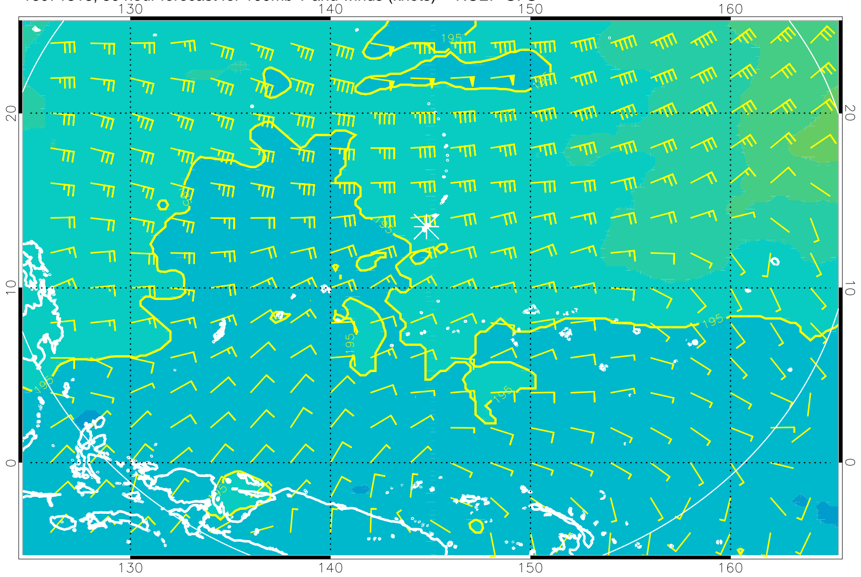
16071818, 30 hour forecast for 100mb T and winds (knots) -- NCEP GFS
