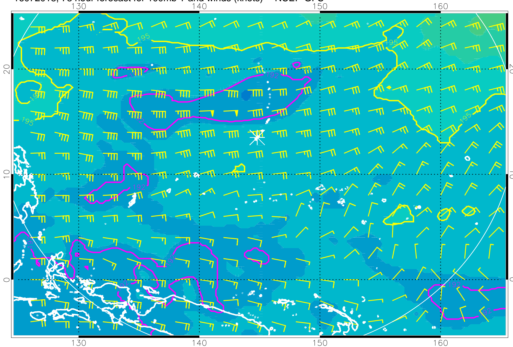
16072018, 78 hour forecast for 100mb T and winds (knots) -- NCEP GFS
