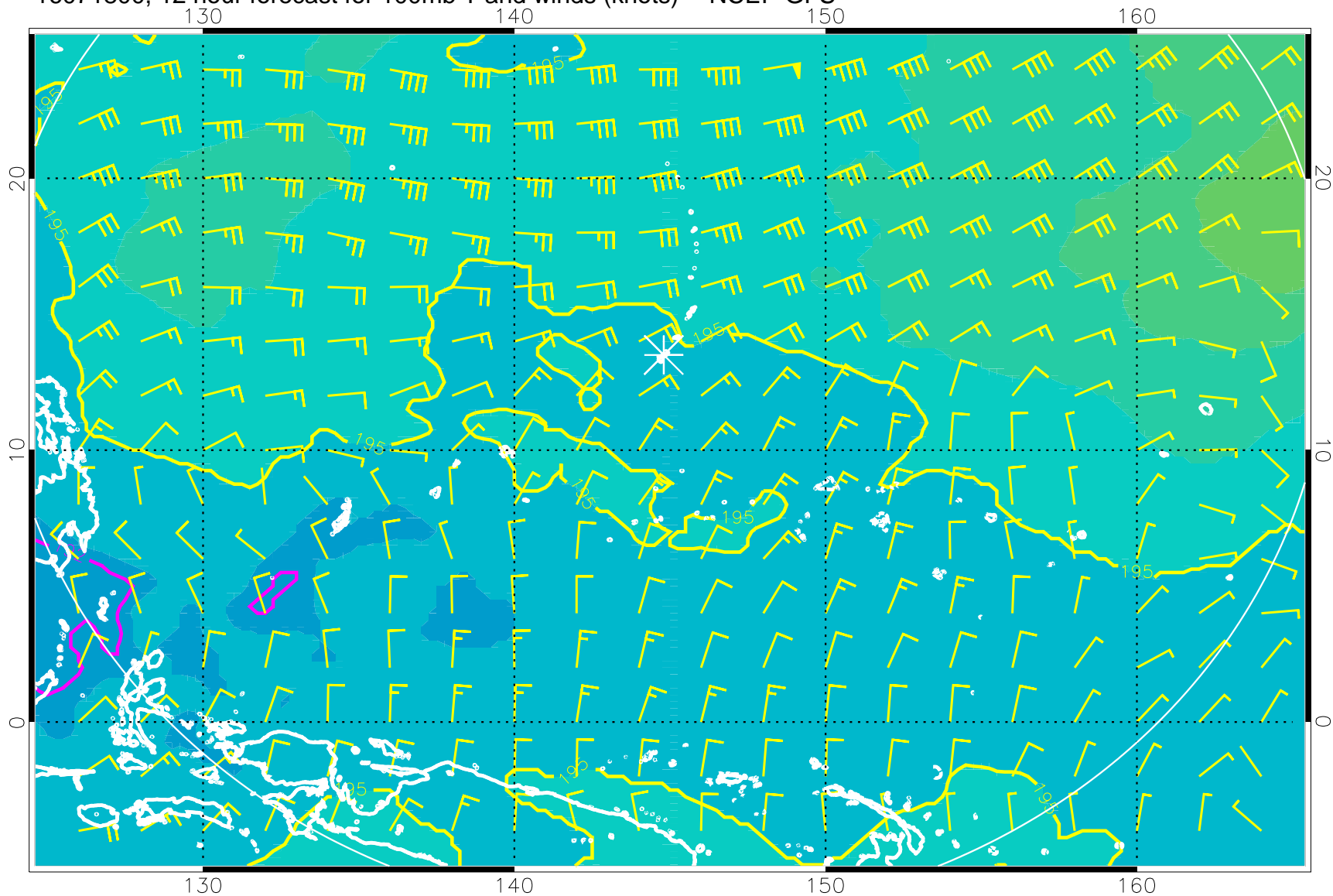
16071800, 12 hour forecast for 100mb T and winds (knots) -- NCEP GFS
