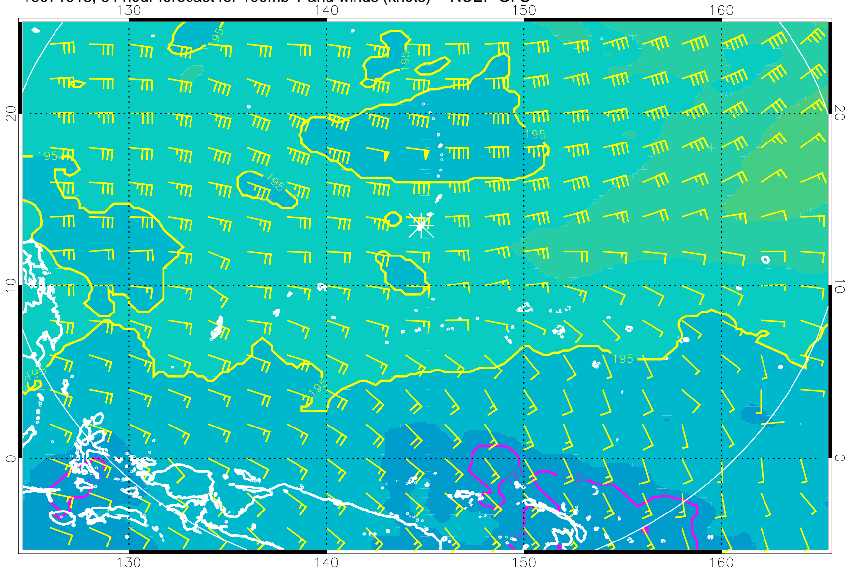
16071918, 54 hour forecast for 100mb T and winds (knots) -- NCEP GFS
