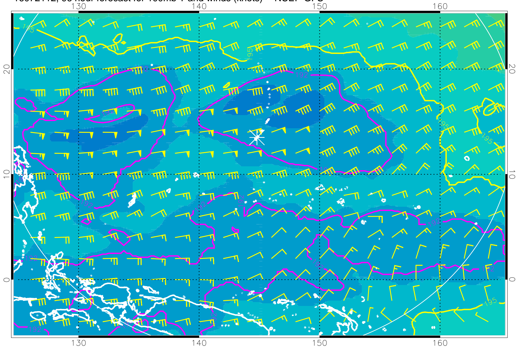
16072112, 96 hour forecast for 100mb T and winds (knots) -- NCEP GFS
