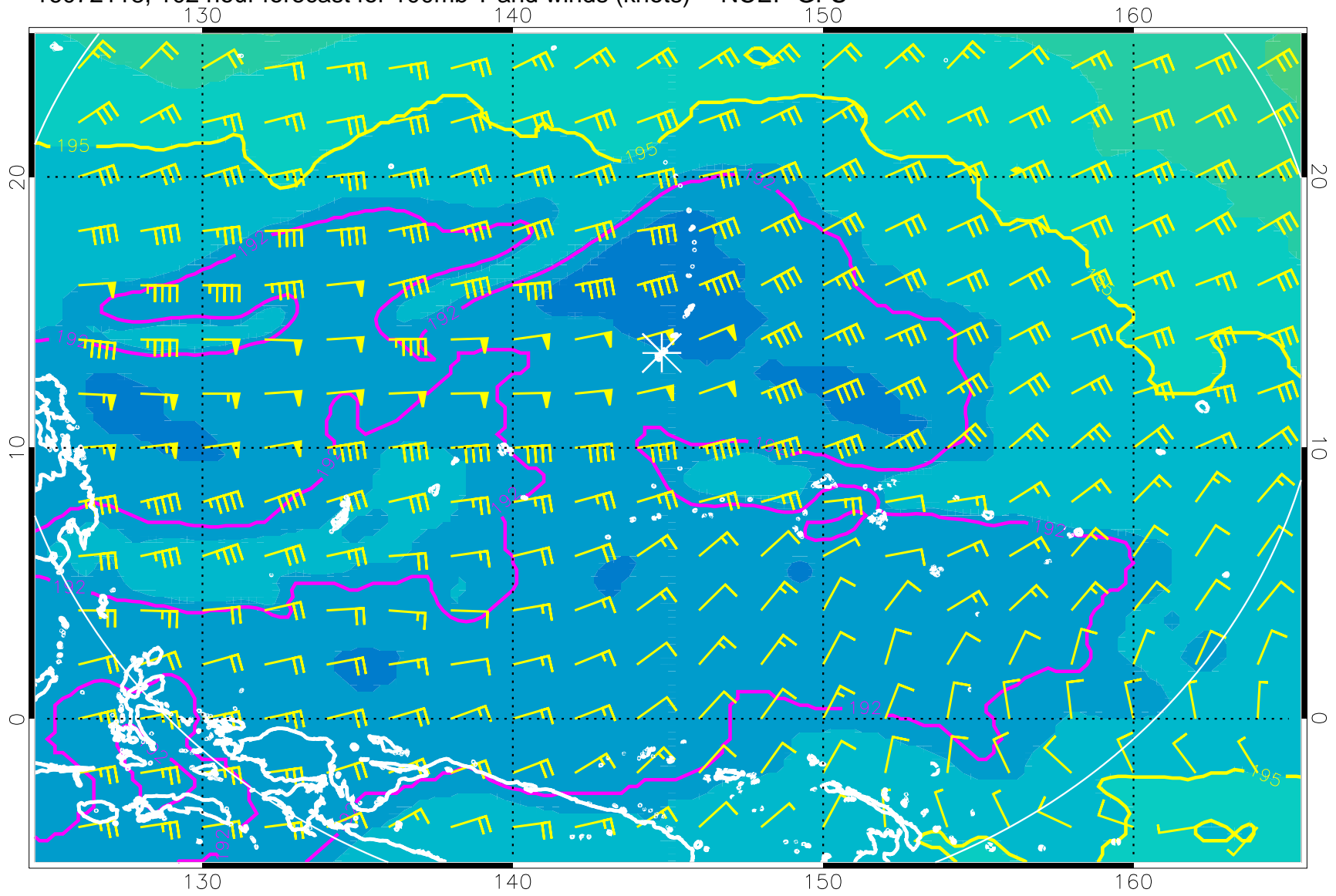
16072118, 102 hour forecast for 100mb T and winds (knots) -- NCEP GFS
