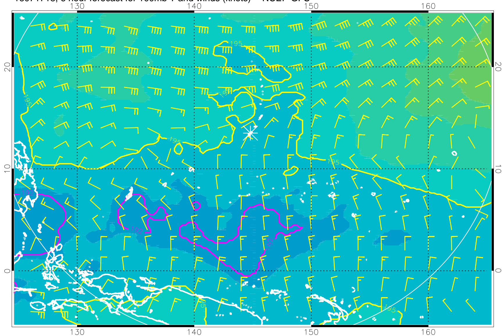
16071718, 6 hour forecast for 100mb T and winds (knots) -- NCEP GFS
