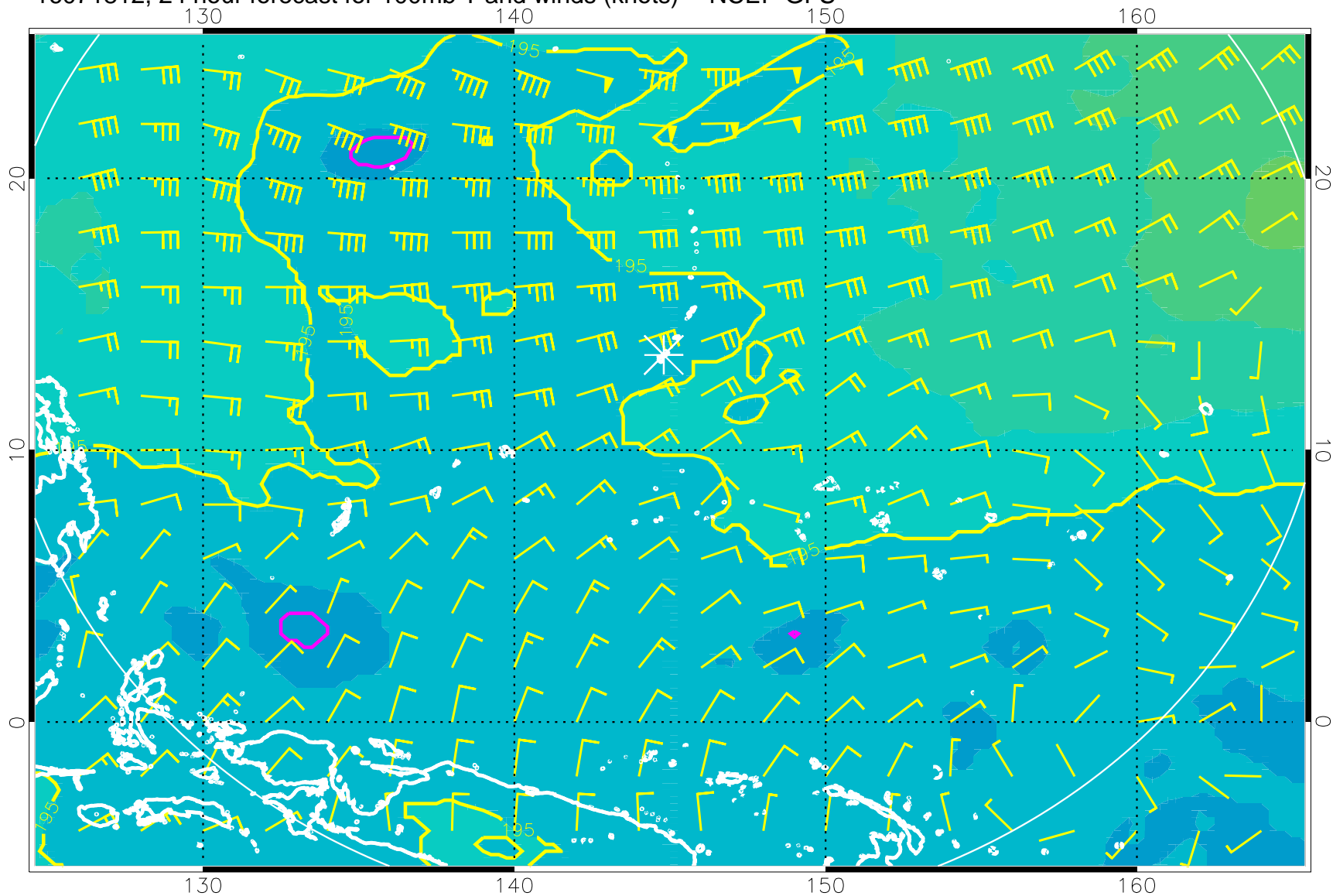
16071812, 24 hour forecast for 100mb T and winds (knots) -- NCEP GFS
