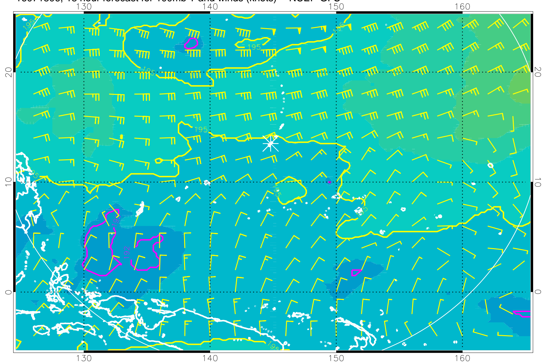
16071806, 18 hour forecast for 100mb T and winds (knots) -- NCEP GFS
