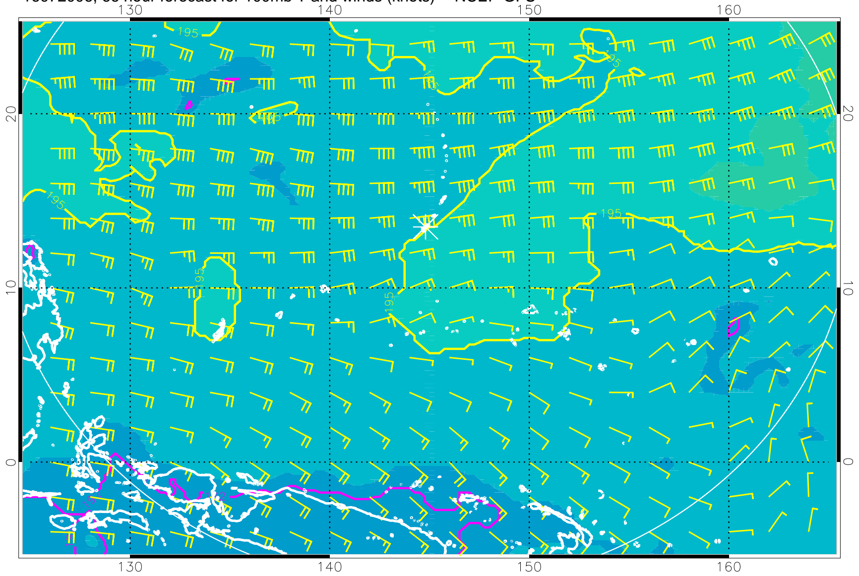
16072006, 66 hour forecast for 100mb T and winds (knots) -- NCEP GFS
