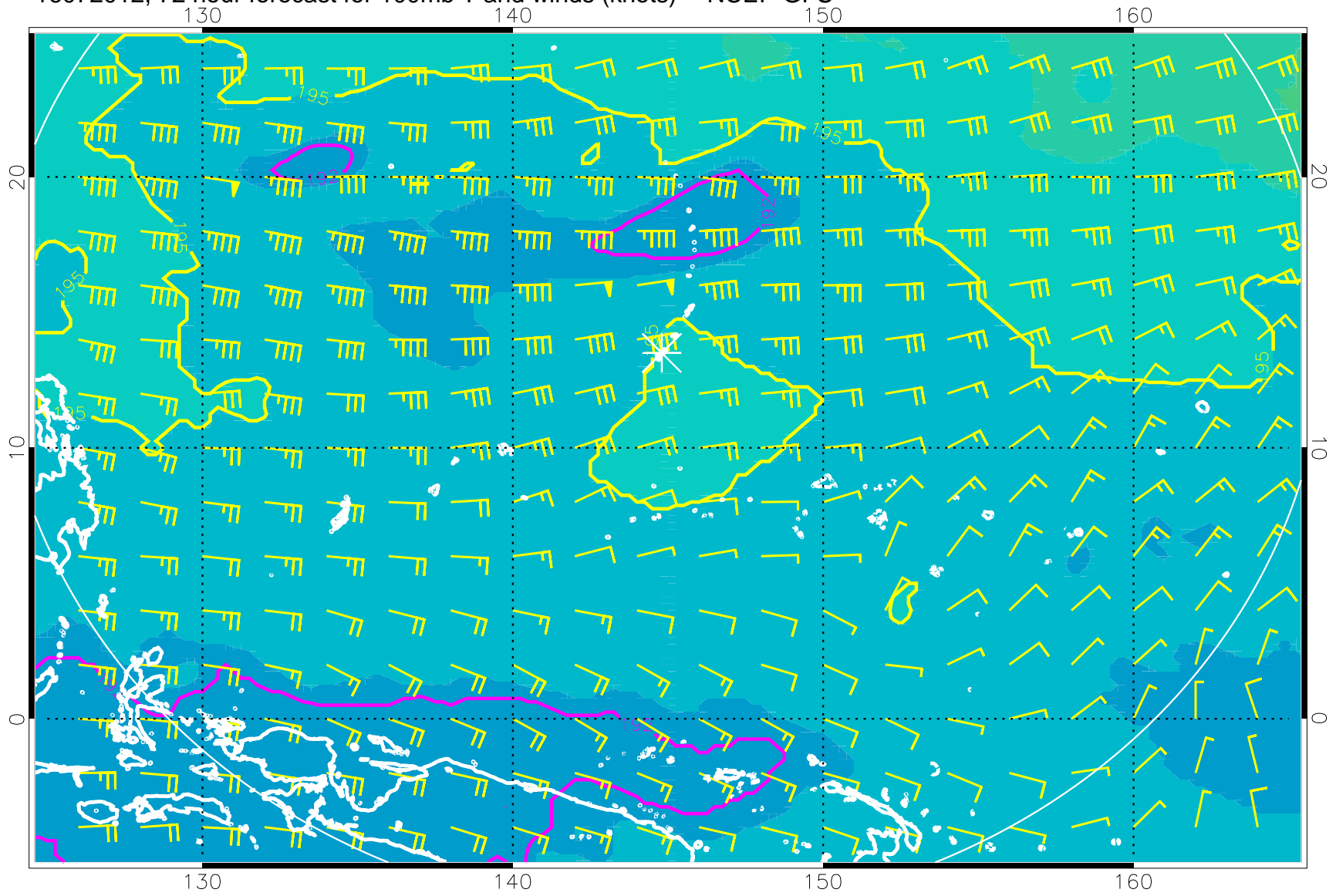
16072012, 72 hour forecast for 100mb T and winds (knots) -- NCEP GFS
