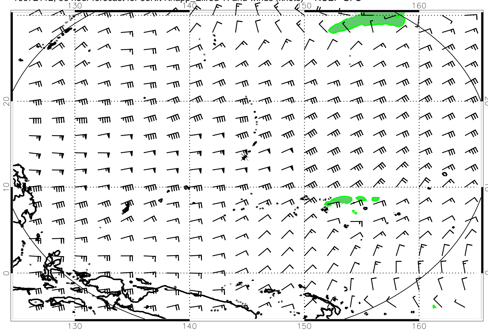
16072112, 96 hour forecast for 53Kft Knapp_Ellrod TI and winds (knots) -- NCEP GFS
