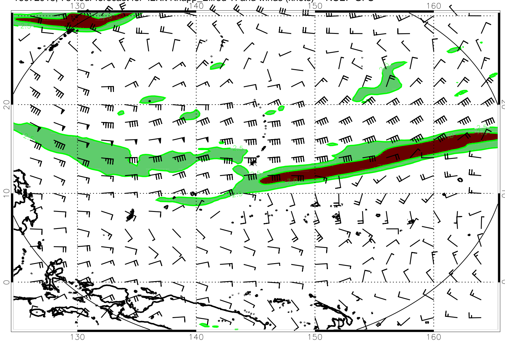
16072018, 78 hour forecast for 42Kft Knapp_Ellrod TI and winds (knots) -- NCEP GFS
