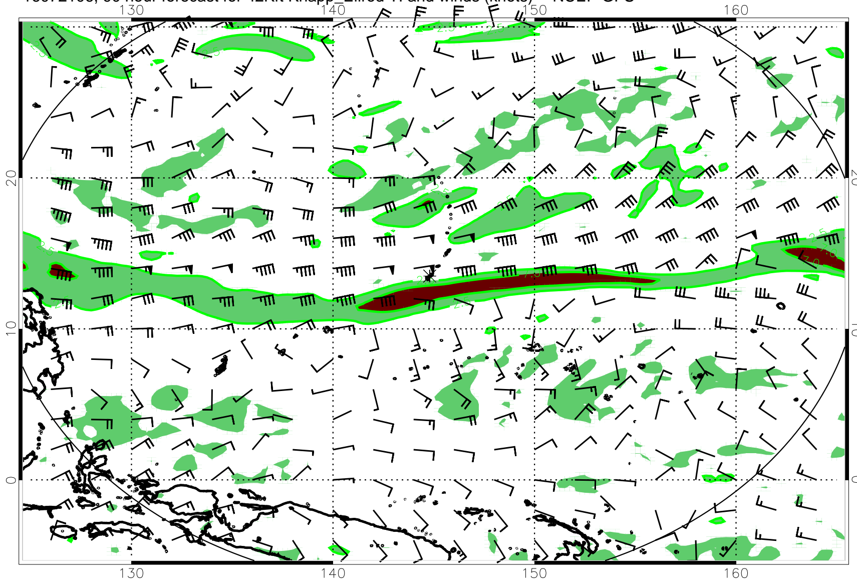
16072106, 90 hour forecast for 42Kft Knapp_Ellrod TI and winds (knots) -- NCEP GFS
