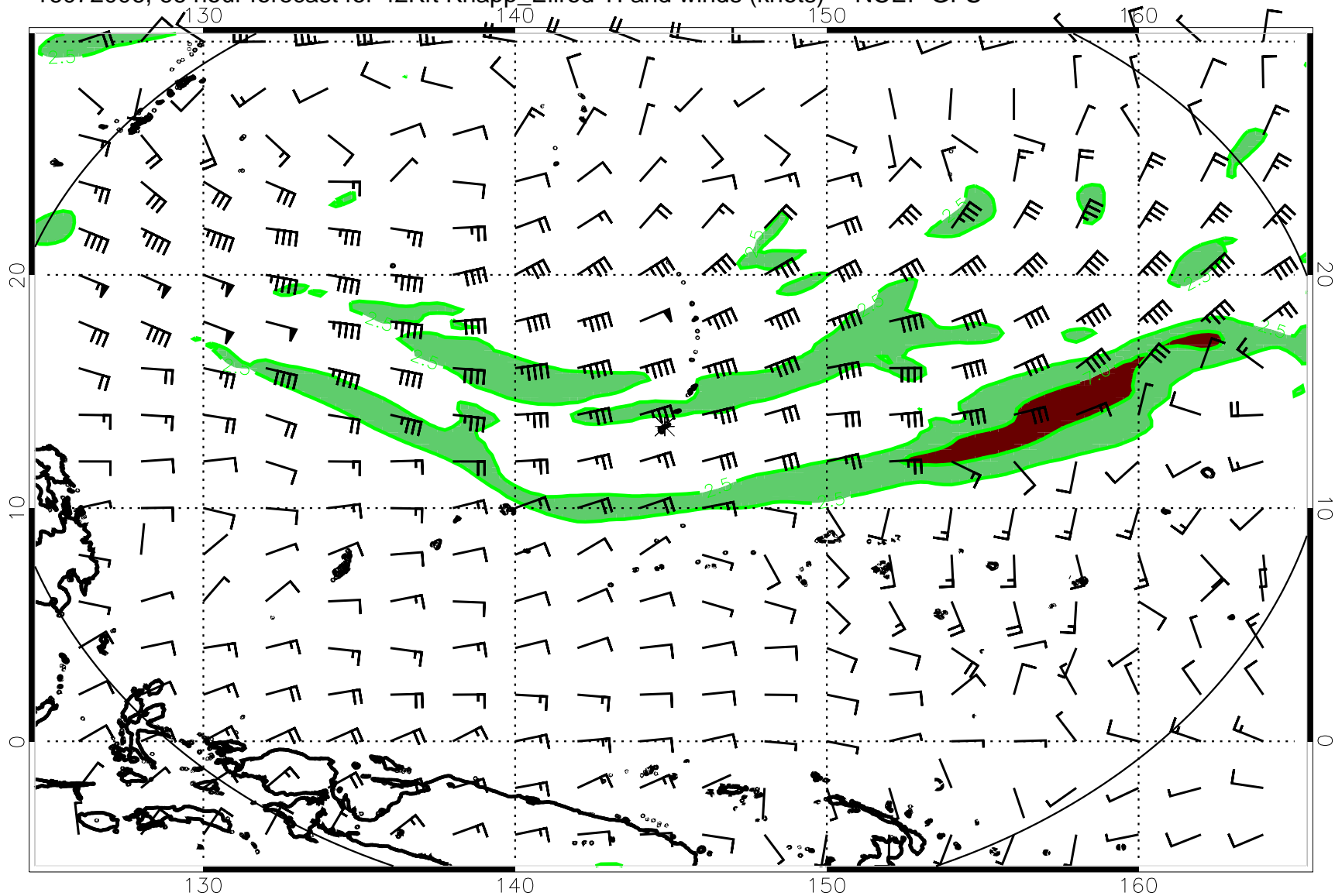
16072006, 66 hour forecast for 42Kft Knapp_Ellrod TI and winds (knots) -- NCEP GFS
