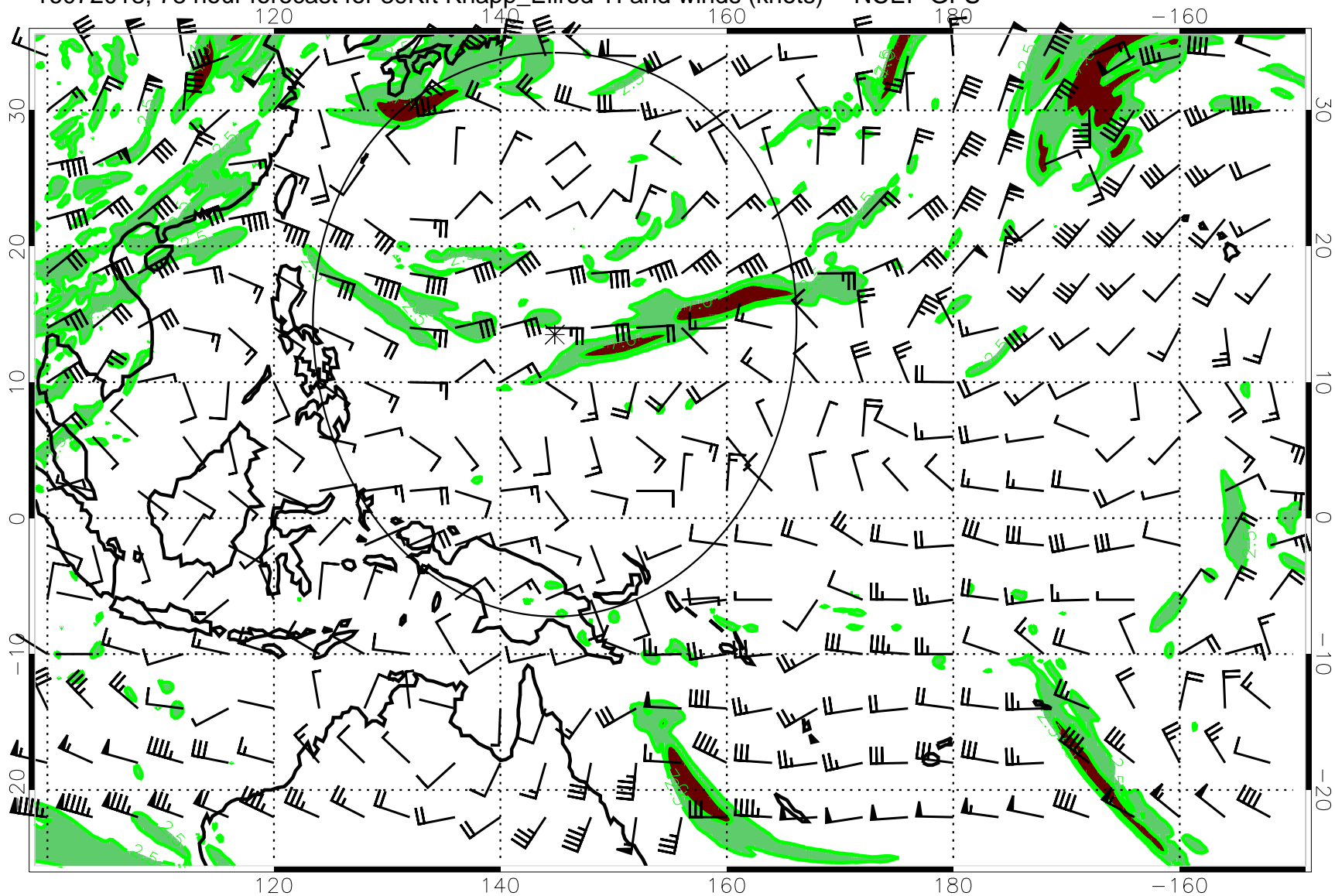
16072018, 78 hour forecast for 39Kft Knapp_Ellrod TI and winds (knots) -- NCEP GFS
