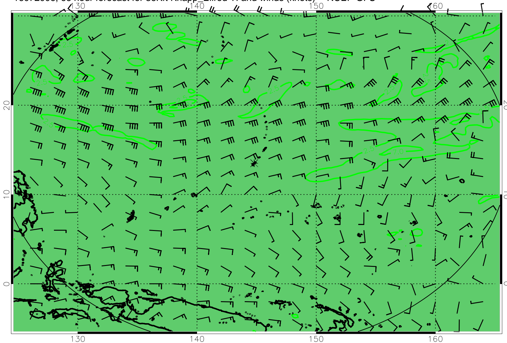
16072006, 66 hour forecast for 36Kft Knapp_Ellrod TI and winds (knots) -- NCEP GFS
