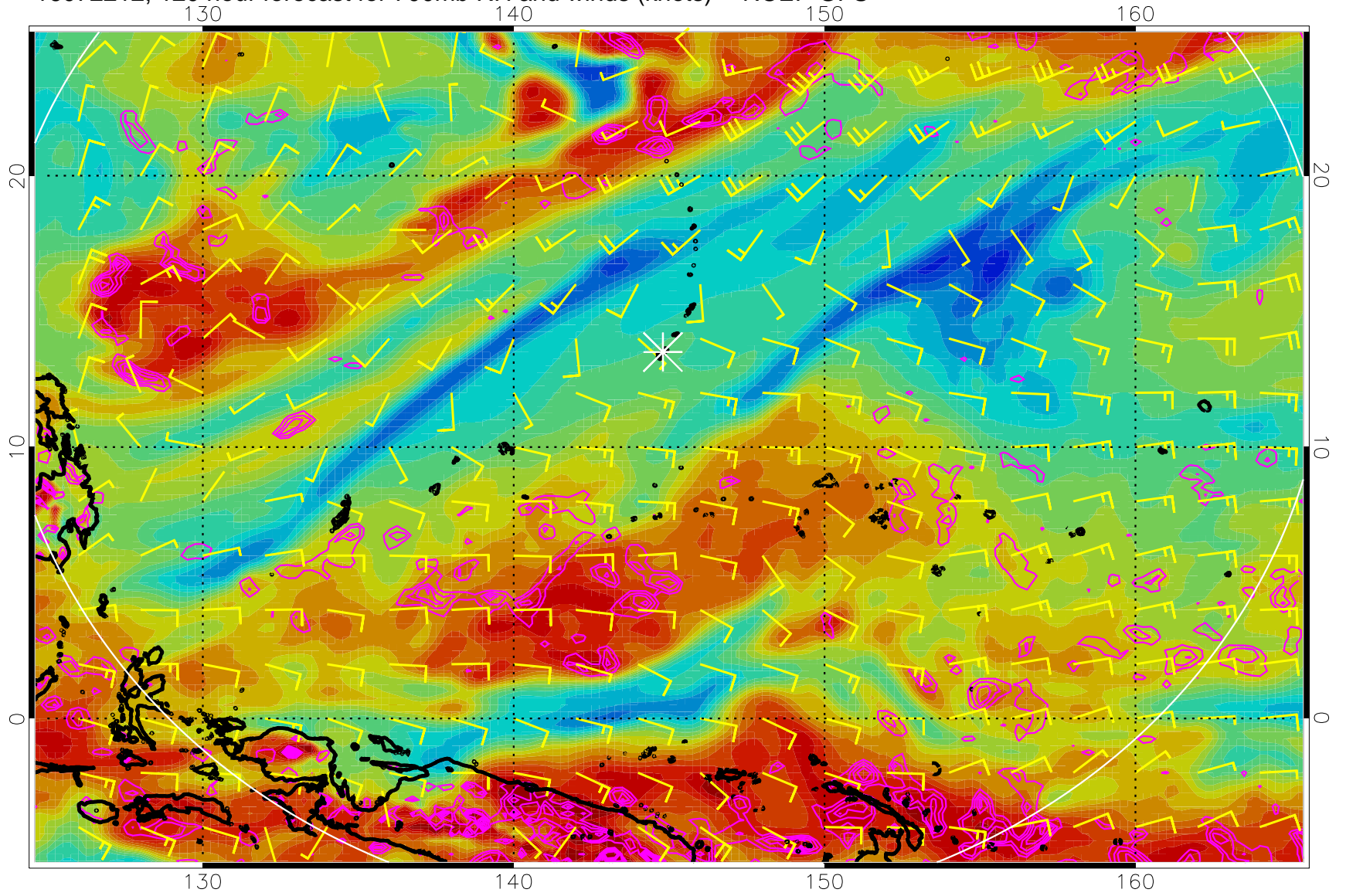
16072212, 120 hour forecast for 700mb RH and winds (knots) -- NCEP GFS
