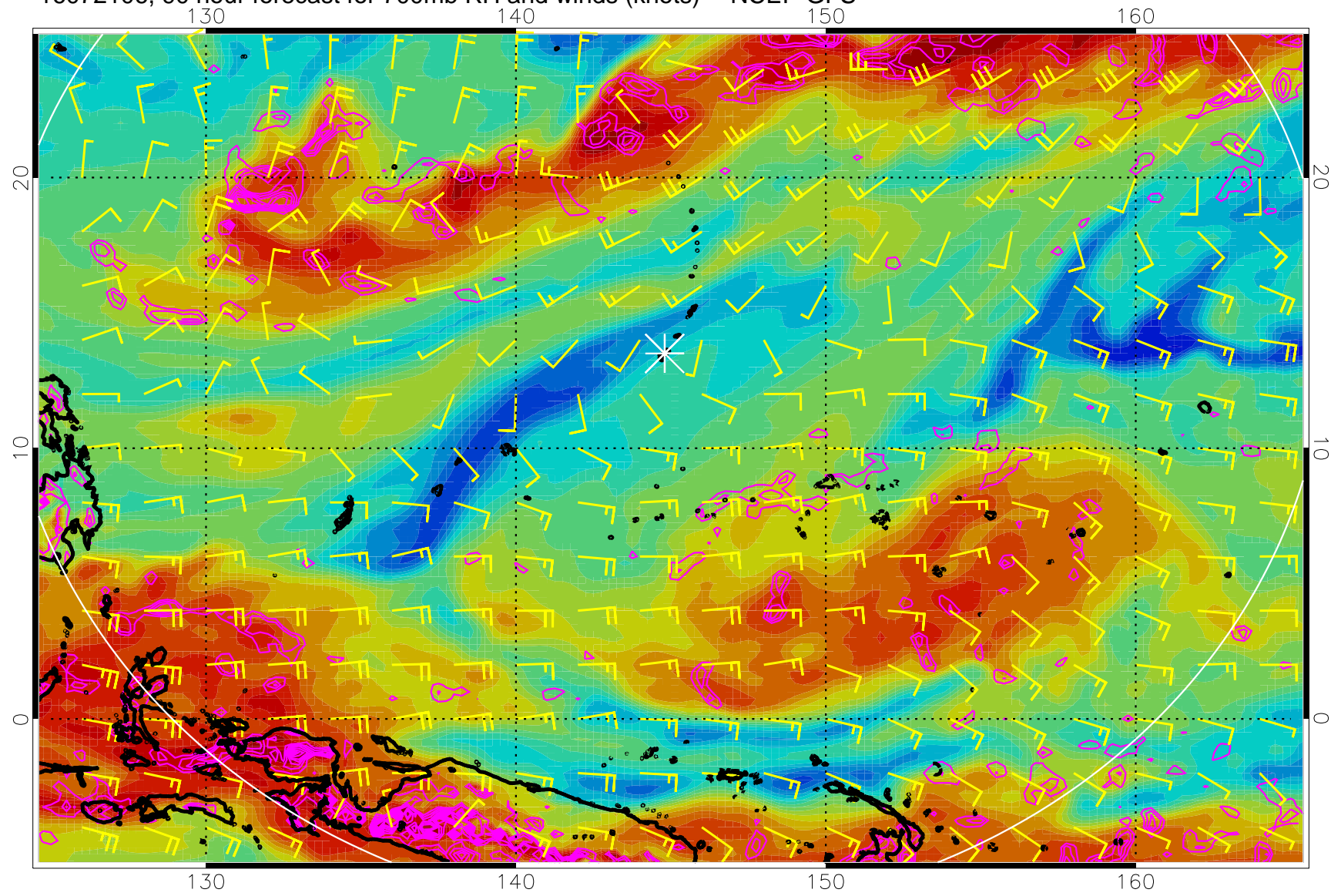
16072106, 90 hour forecast for 700mb RH and winds (knots) -- NCEP GFS
