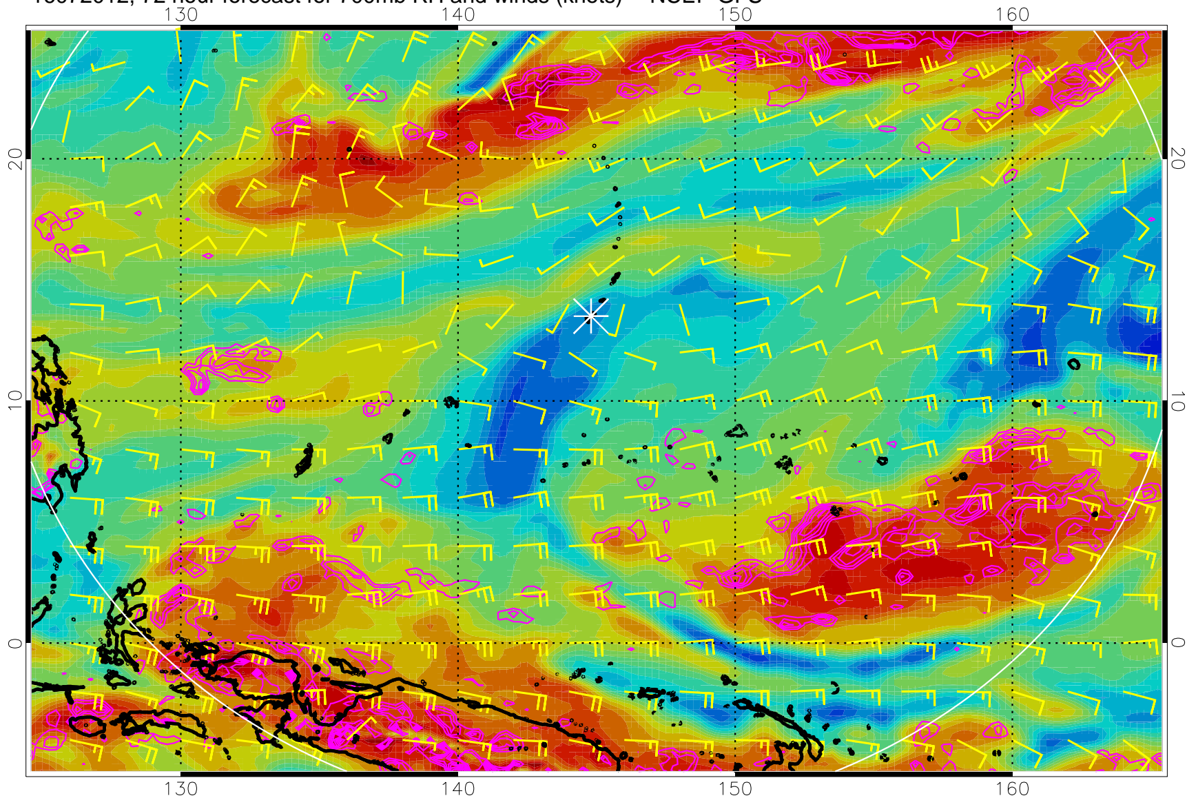
16072012, 72 hour forecast for 700mb RH and winds (knots) -- NCEP GFS
