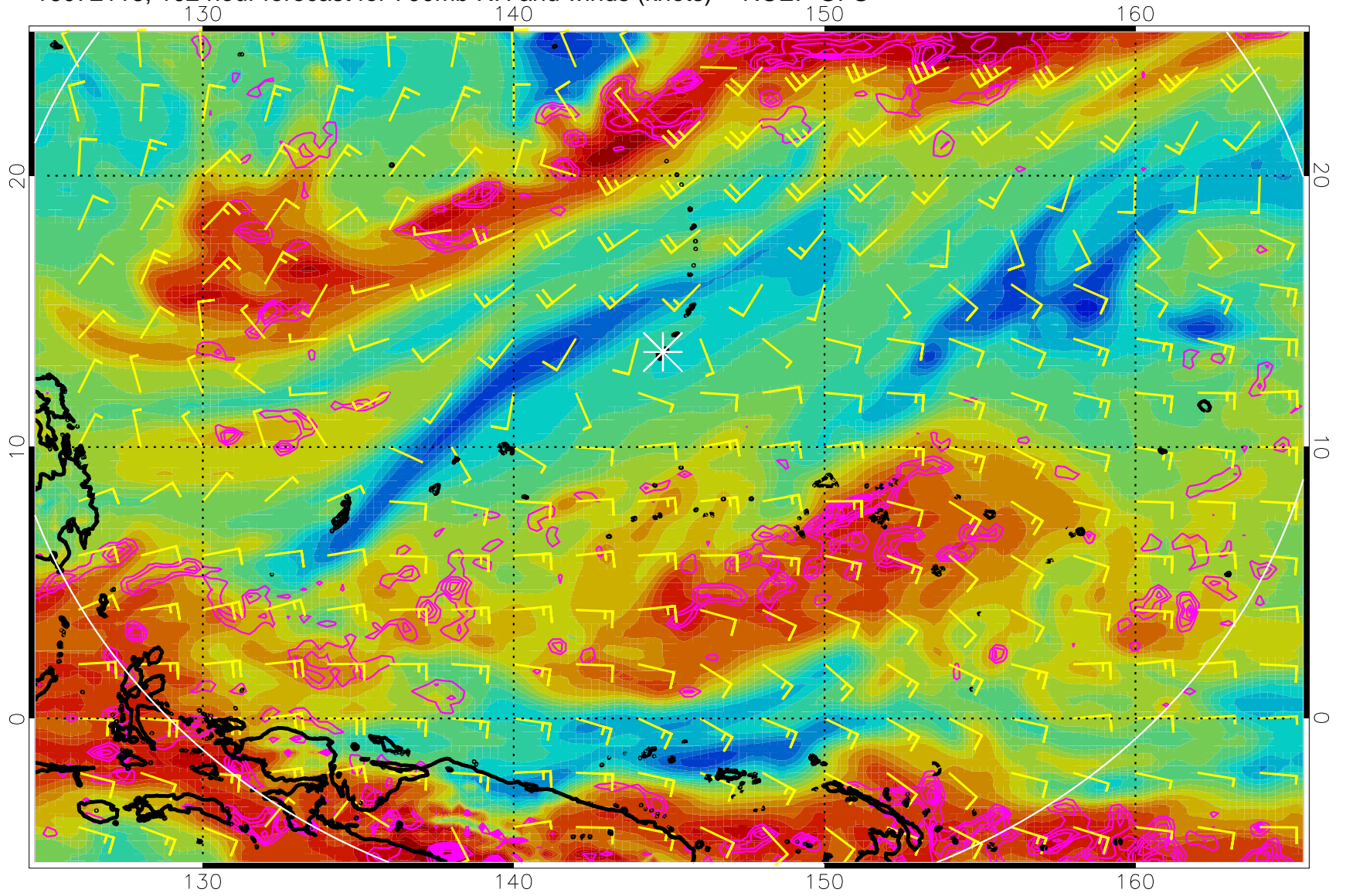
16072118, 102 hour forecast for 700mb RH and winds (knots) -- NCEP GFS
