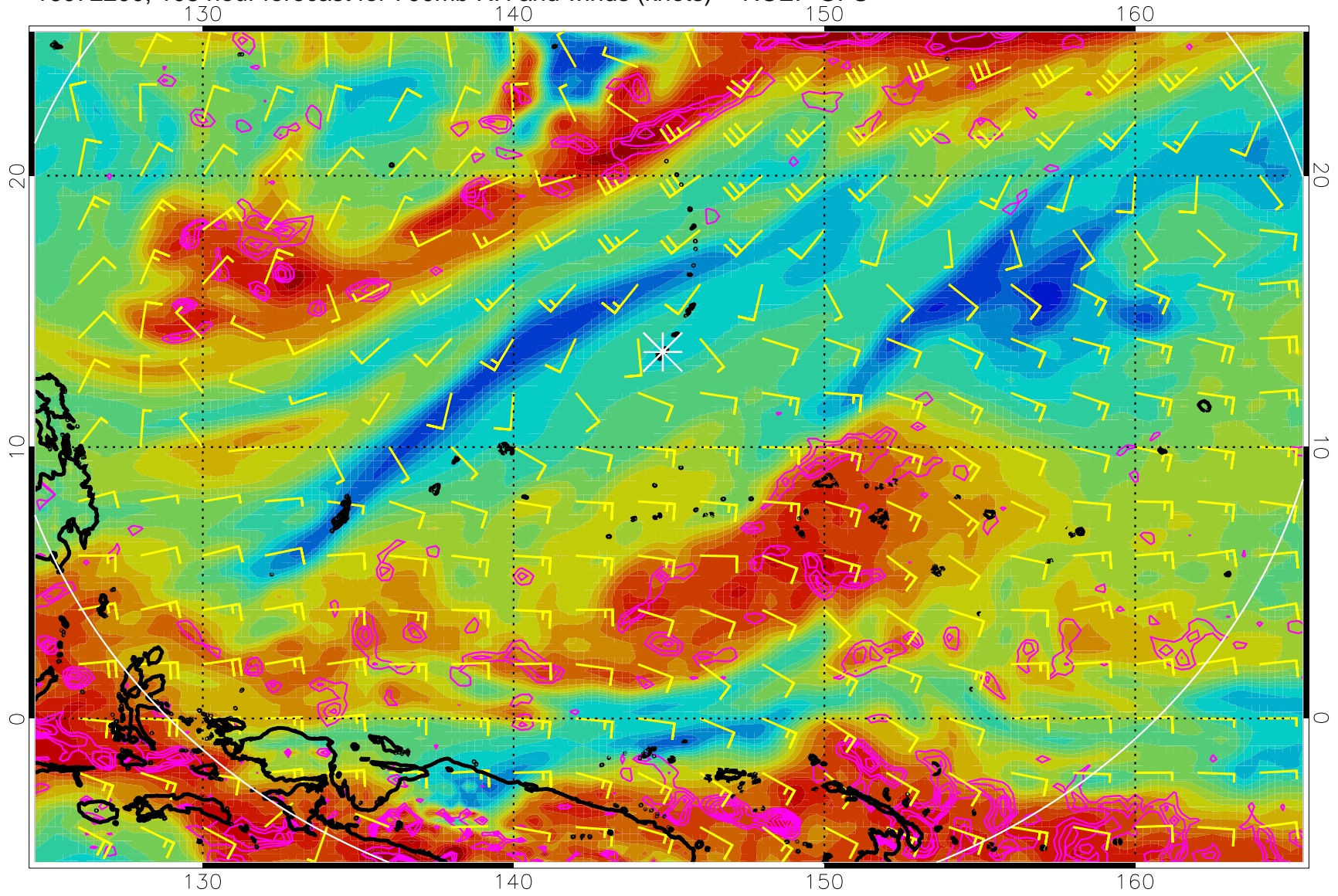
16072200, 108 hour forecast for 700mb RH and winds (knots) -- NCEP GFS
