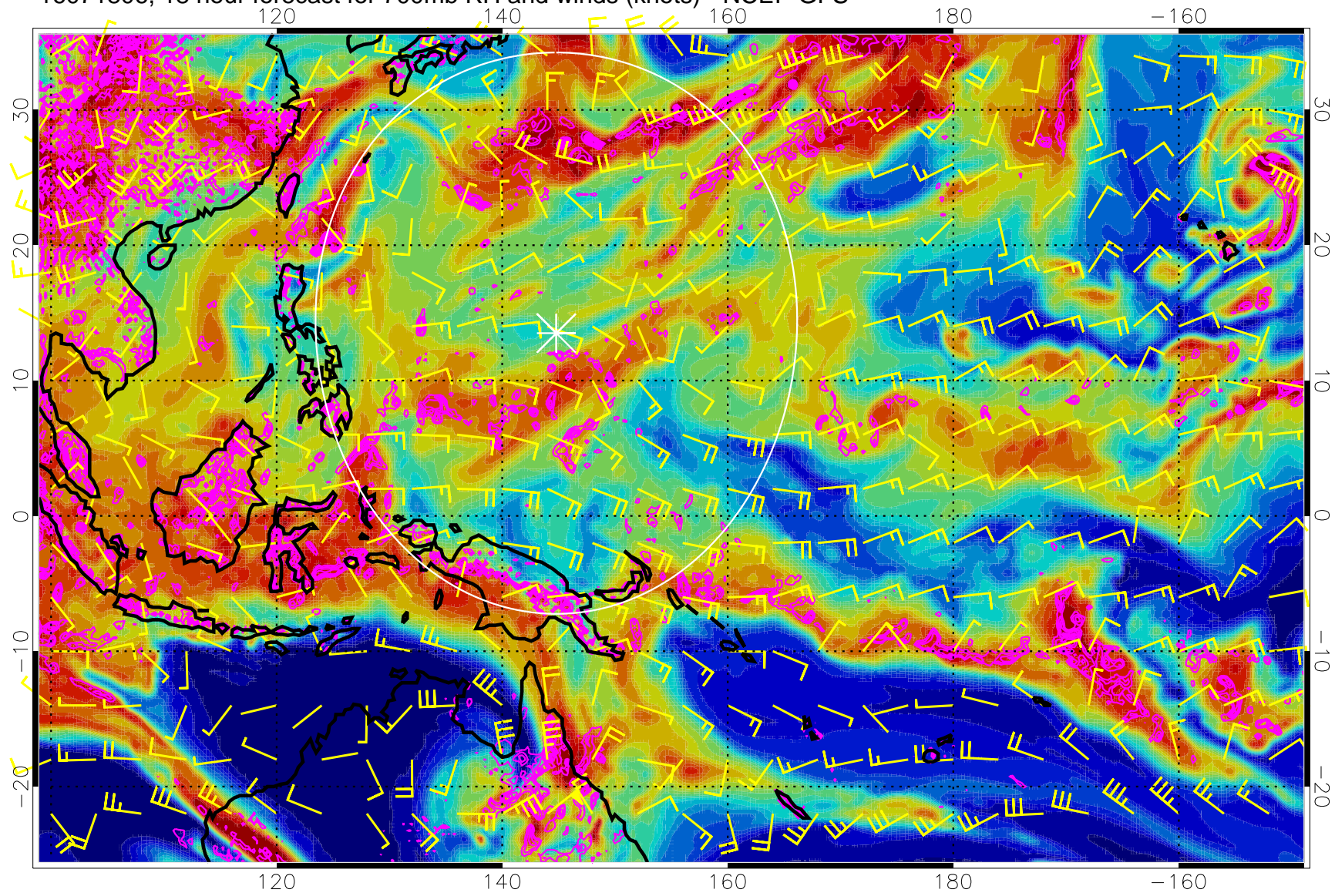
16071806, 18 hour forecast for 700mb RH and winds (knots) - NCEP GFS
