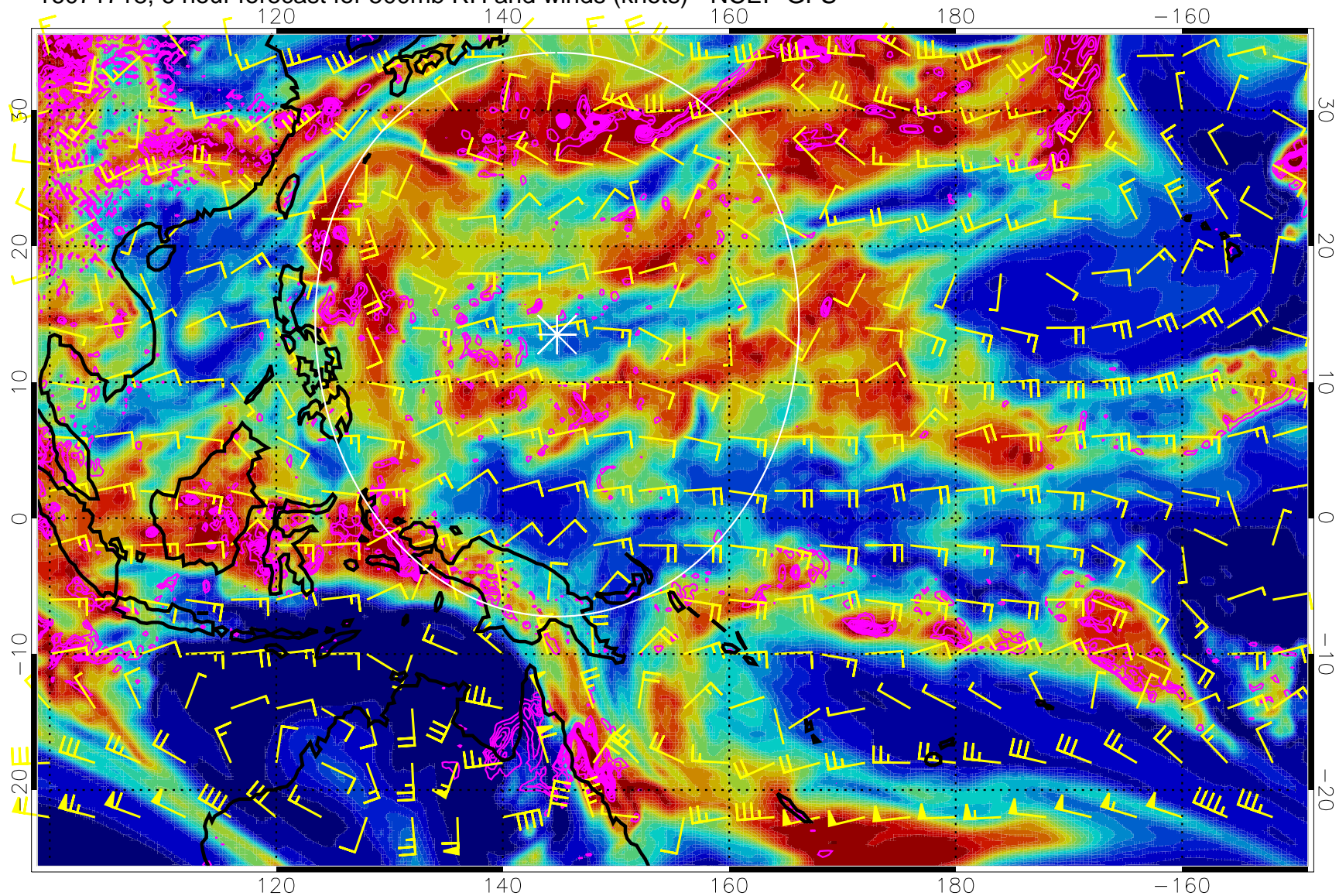
16071718, 6 hour forecast for 500mb RH and winds (knots) - NCEP GFS
