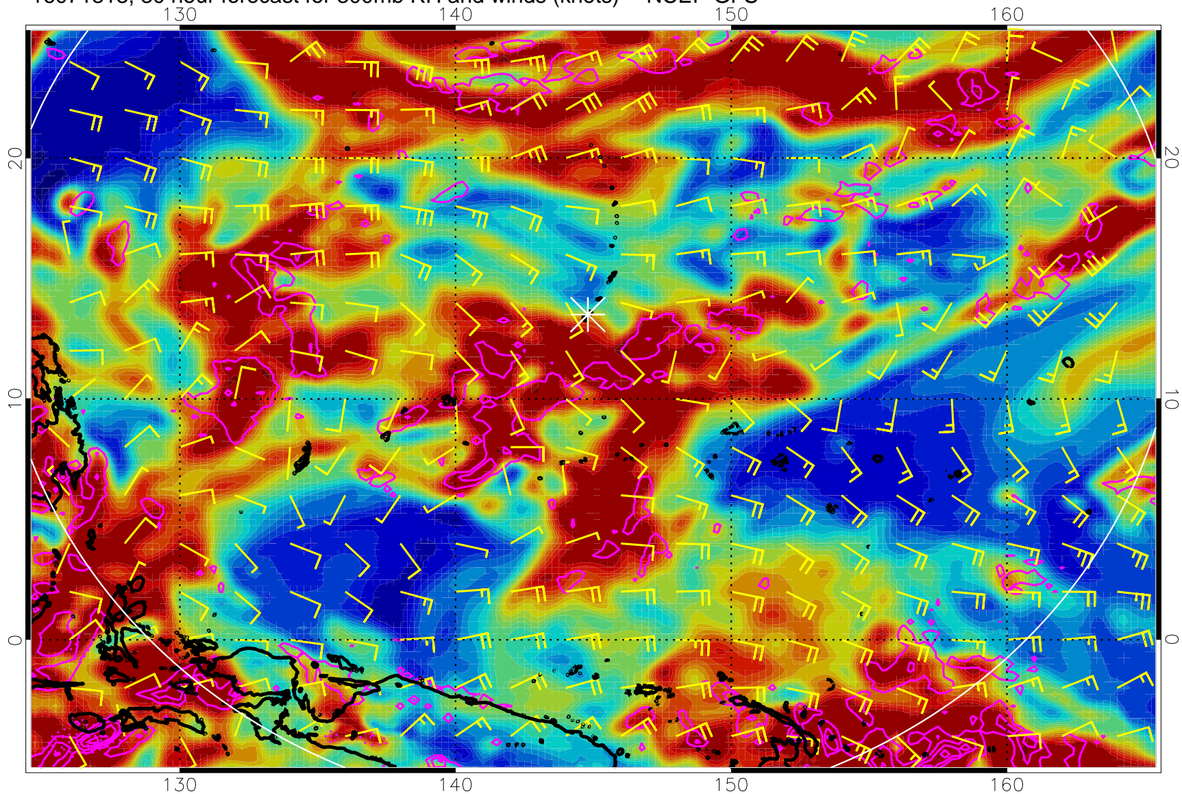
16071818, 30 hour forecast for 300mb RH and winds (knots) -- NCEP GFS
