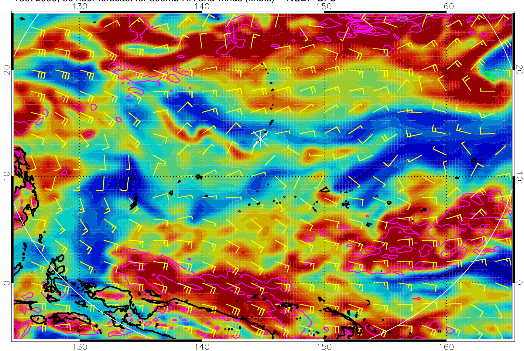
16072006, 66 hour forecast for 300mb RH and winds (knots) -- NCEP GFS
