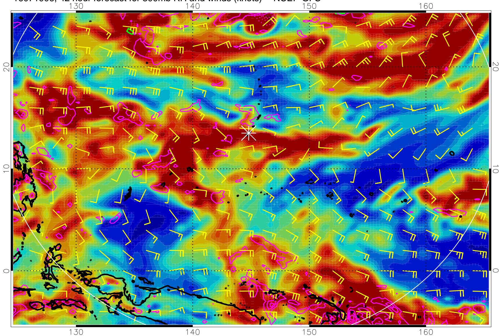
16071906, 42 hour forecast for 300mb RH and winds (knots) -- NCEP GFS
