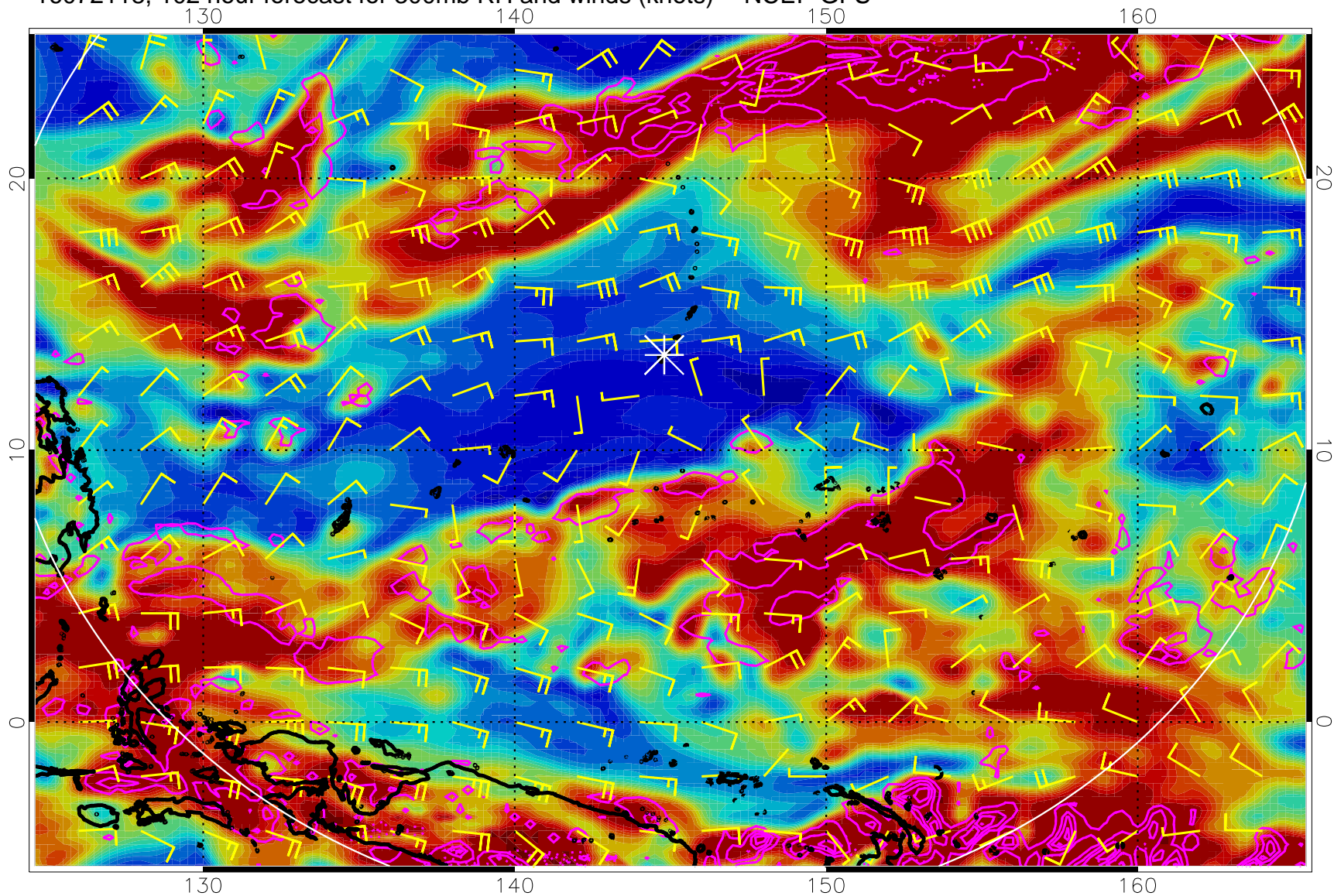
16072118, 102 hour forecast for 300mb RH and winds (knots) -- NCEP GFS
