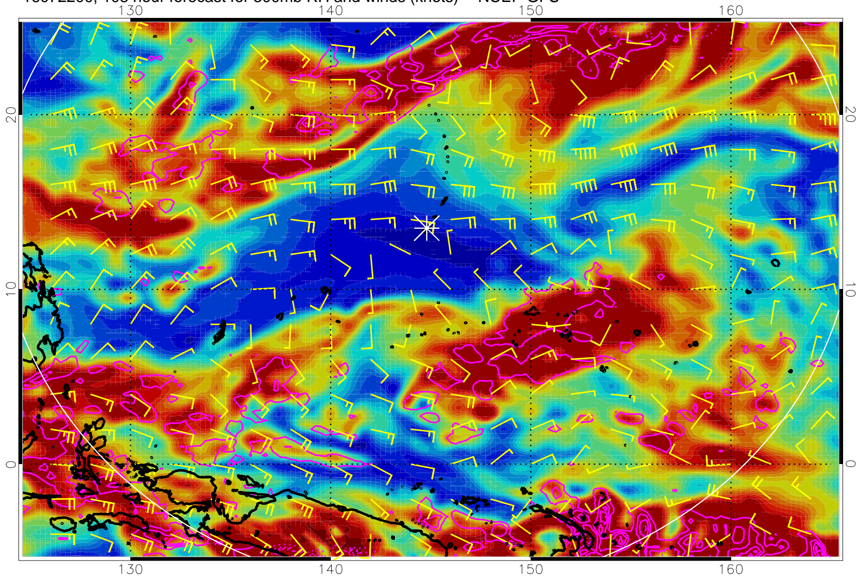
16072200, 108 hour forecast for 300mb RH and winds (knots) -- NCEP GFS
