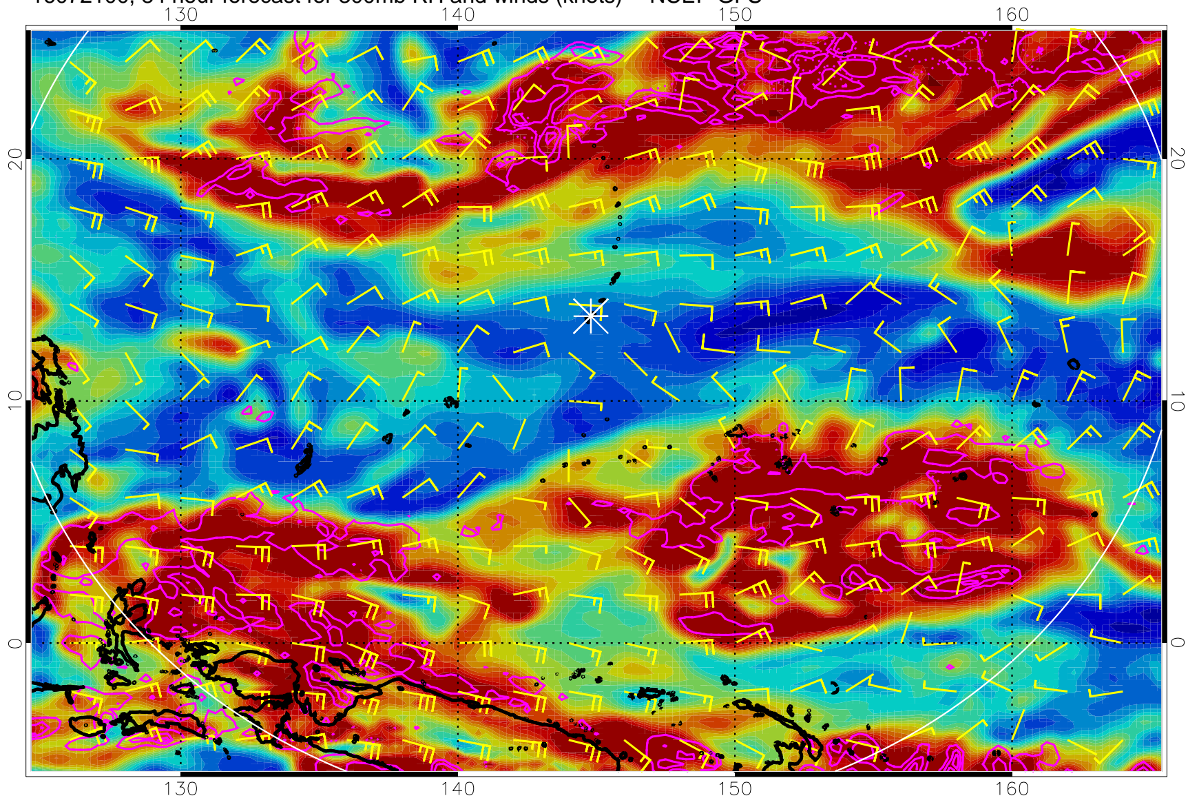
16072100, 84 hour forecast for 300mb RH and winds (knots) -- NCEP GFS
