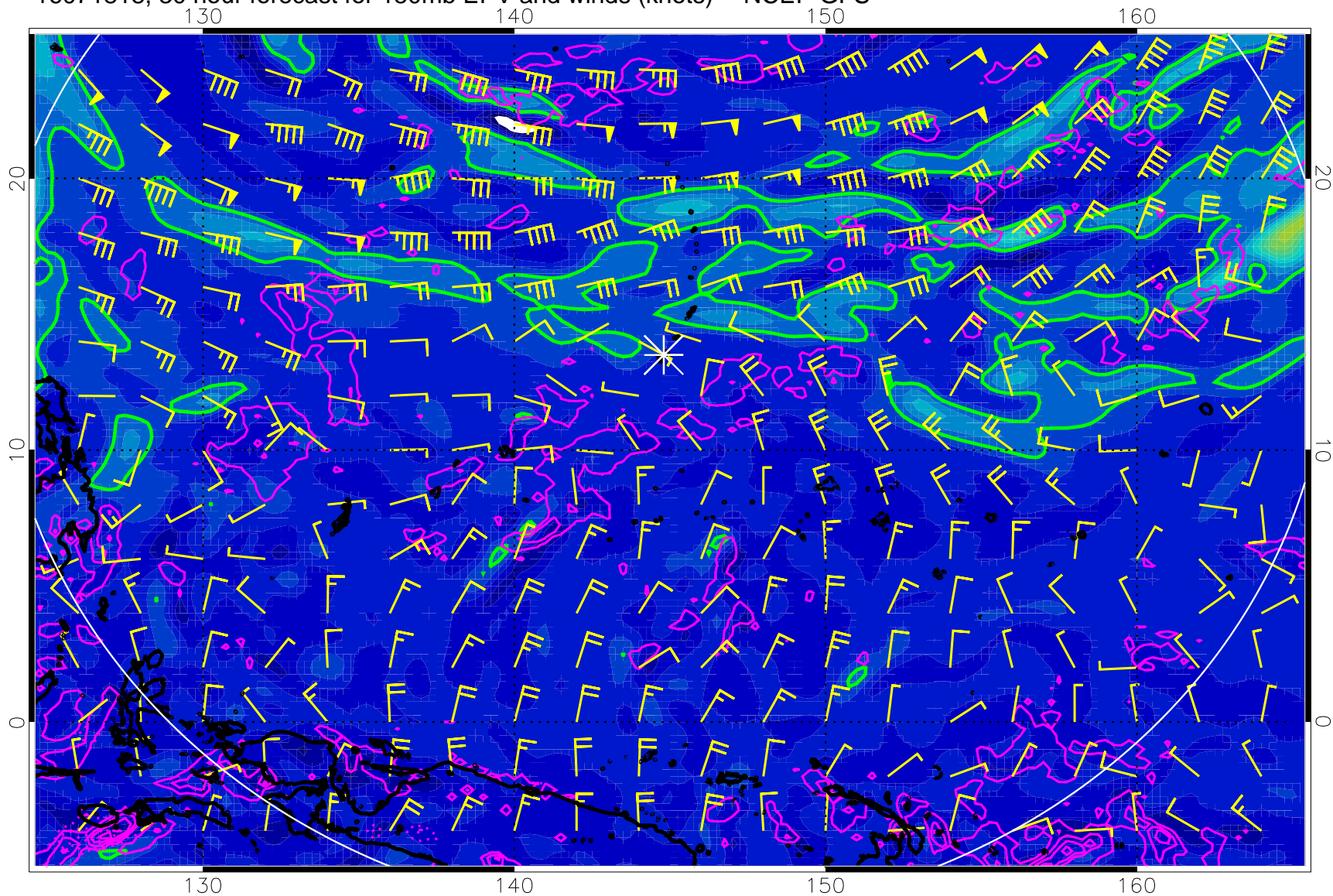
16071818, 30 hour forecast for 150mb EPV and winds (knots) -- NCEP GFS
