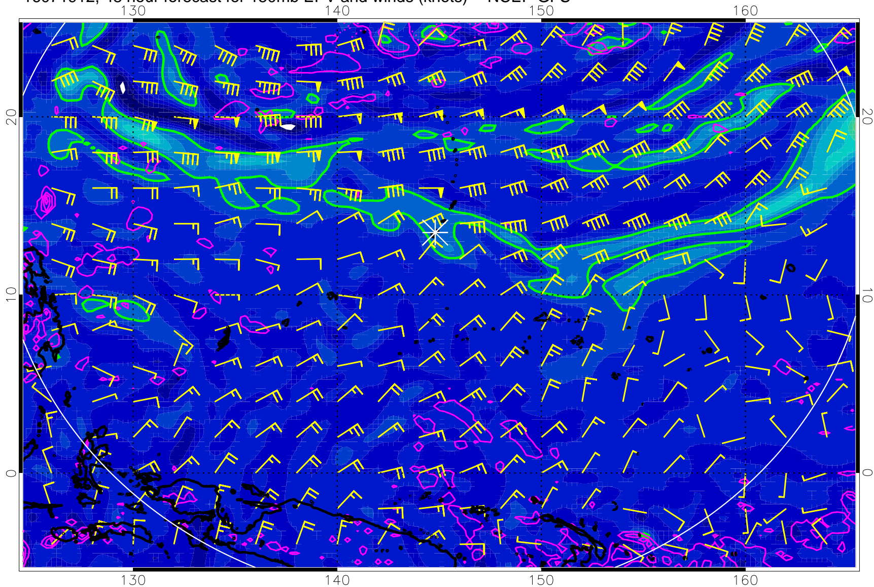
16071912, 48 hour forecast for 150mb EPV and winds (knots) -- NCEP GFS
