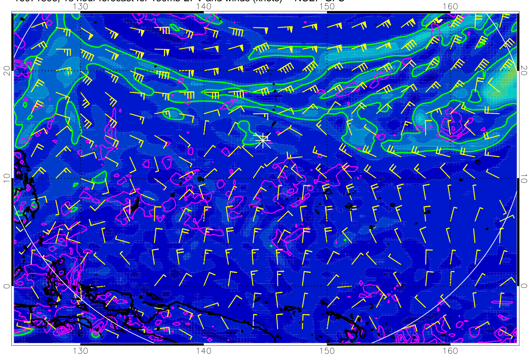
16071806, 18 hour forecast for 150mb EPV and winds (knots) -- NCEP GFS
