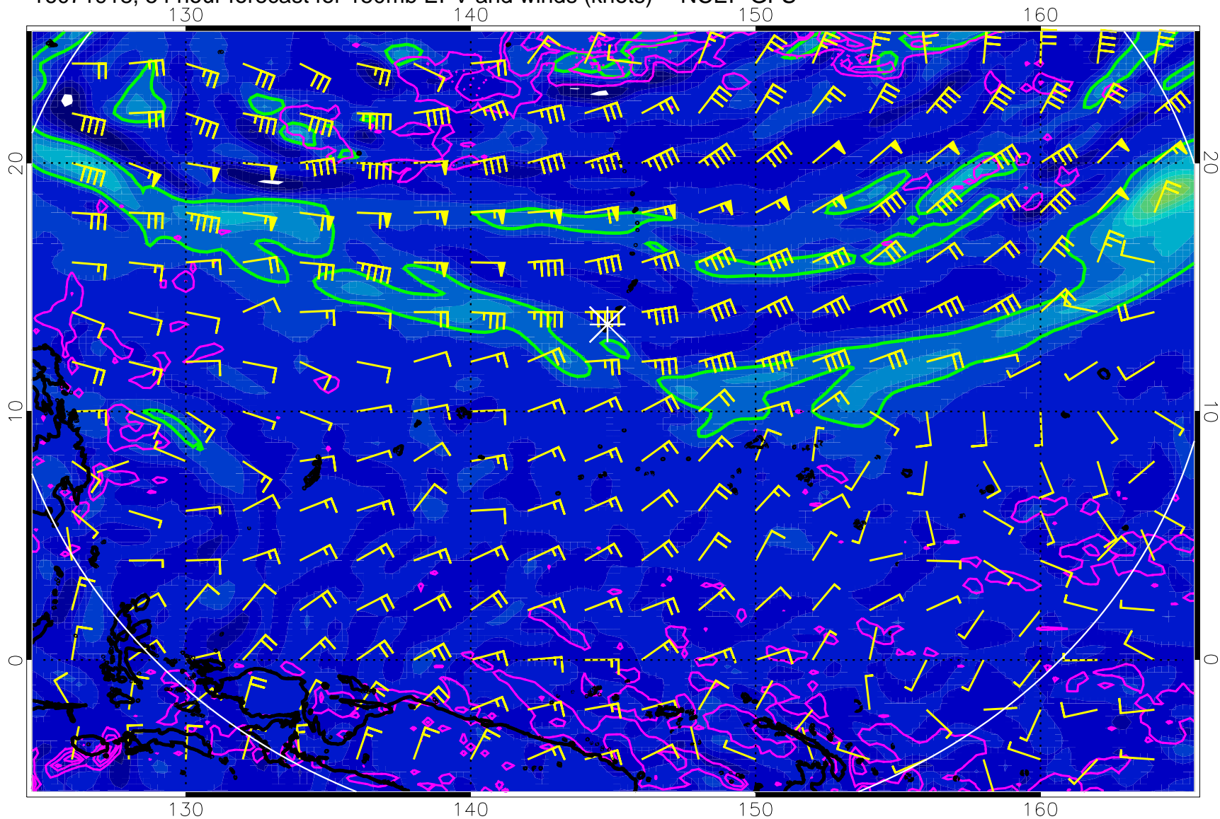
16071918, 54 hour forecast for 150mb EPV and winds (knots) -- NCEP GFS
