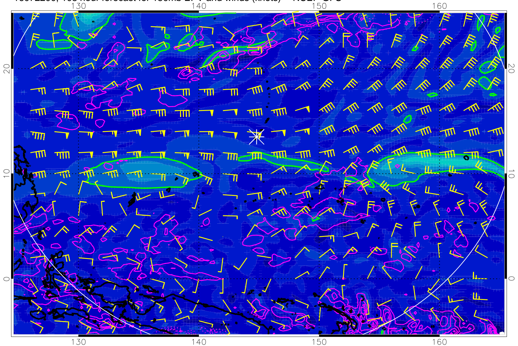
16072200, 108 hour forecast for 150mb EPV and winds (knots) -- NCEP GFS
