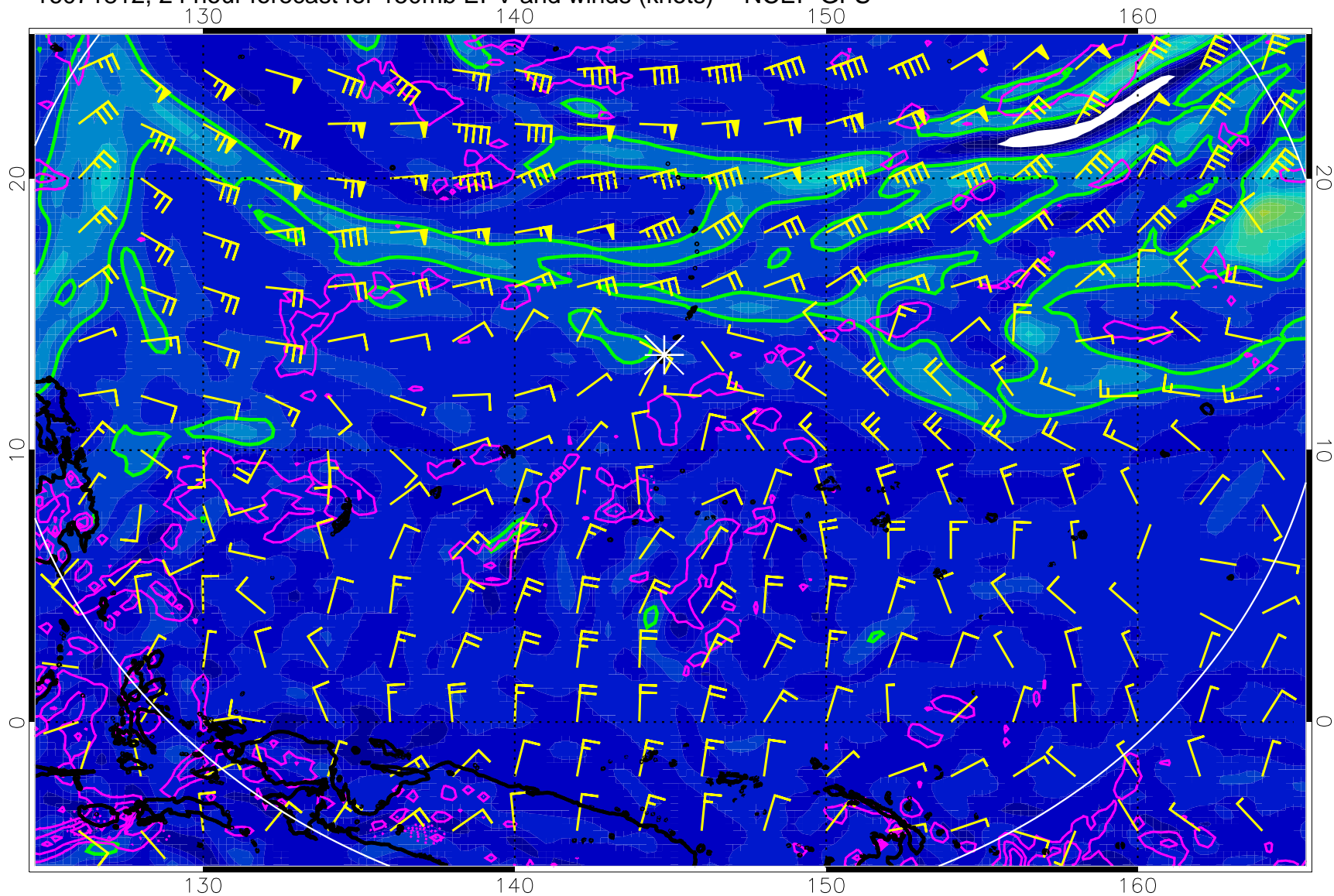
16071812, 24 hour forecast for 150mb EPV and winds (knots) -- NCEP GFS
