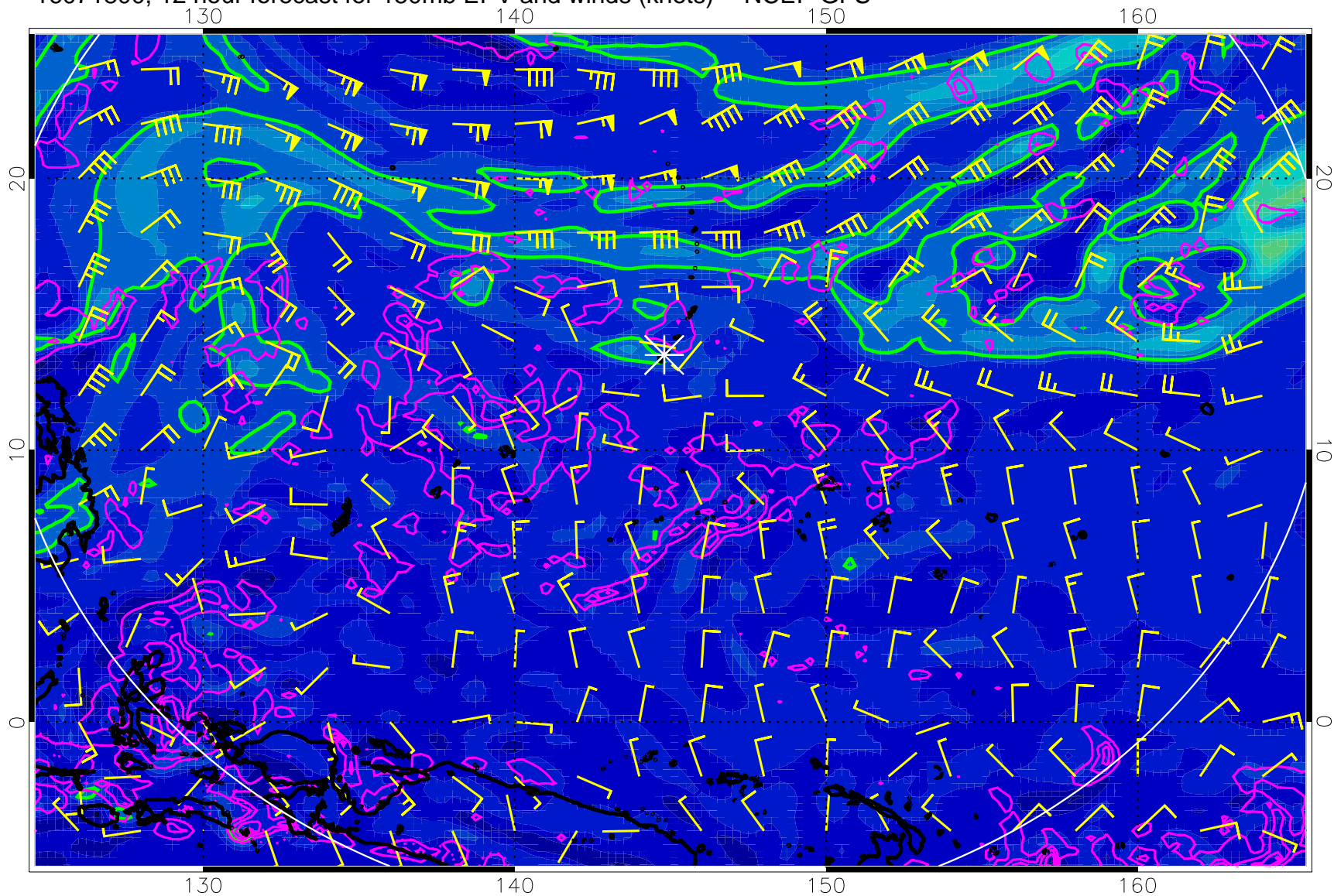
16071800, 12 hour forecast for 150mb EPV and winds (knots) -- NCEP GFS
