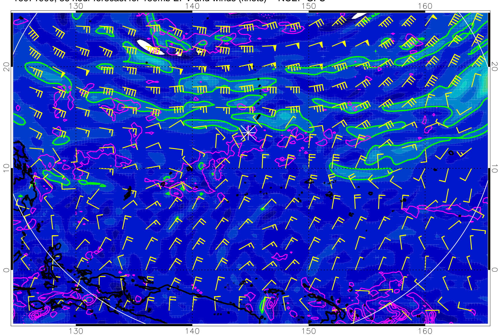
16071900, 36 hour forecast for 150mb EPV and winds (knots) -- NCEP GFS
