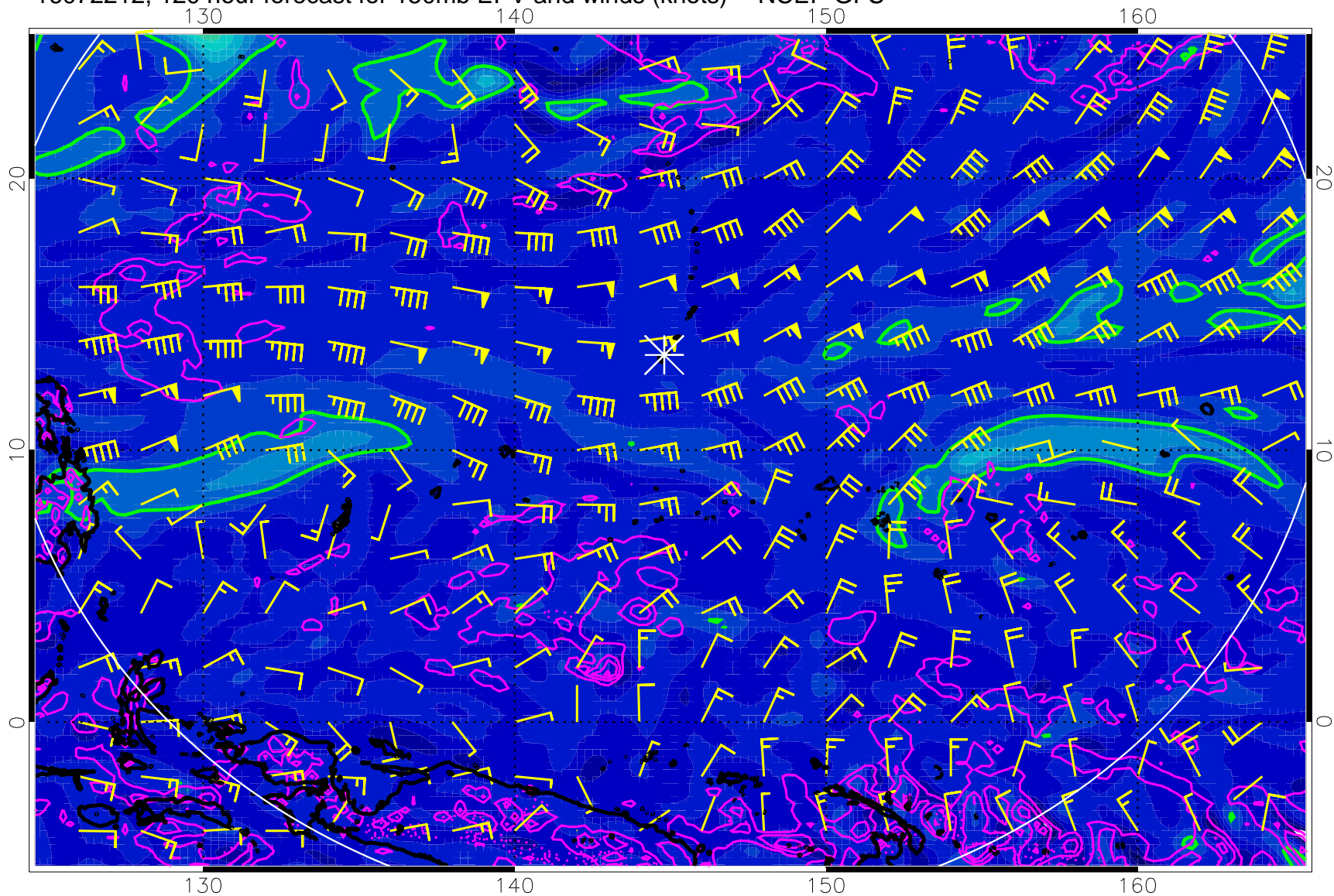
16072212, 120 hour forecast for 150mb EPV and winds (knots) -- NCEP GFS
