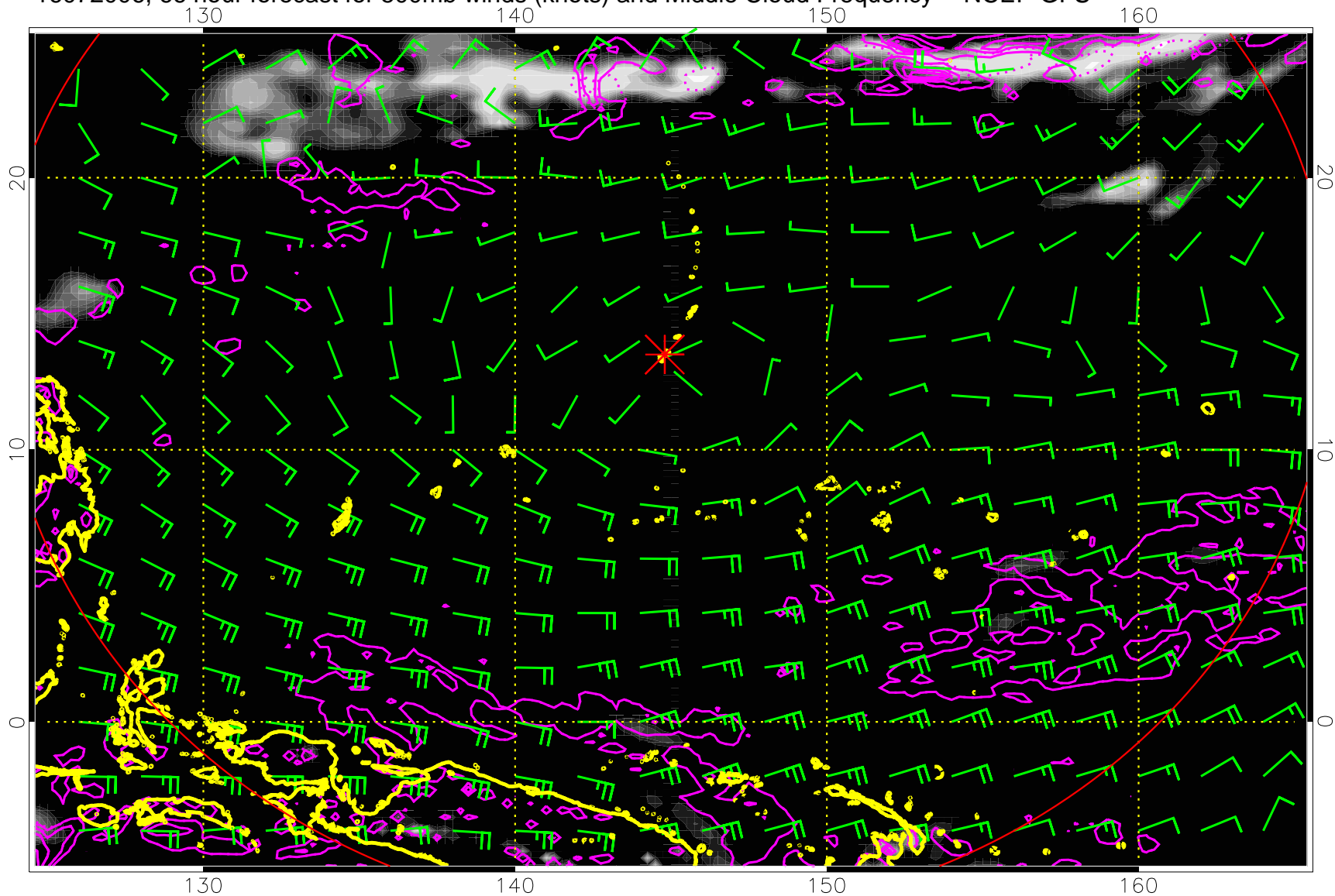
16072006, 66 hour forecast for 500mb winds (knots) and Middle Cloud Frequency -- NCEP GFS
