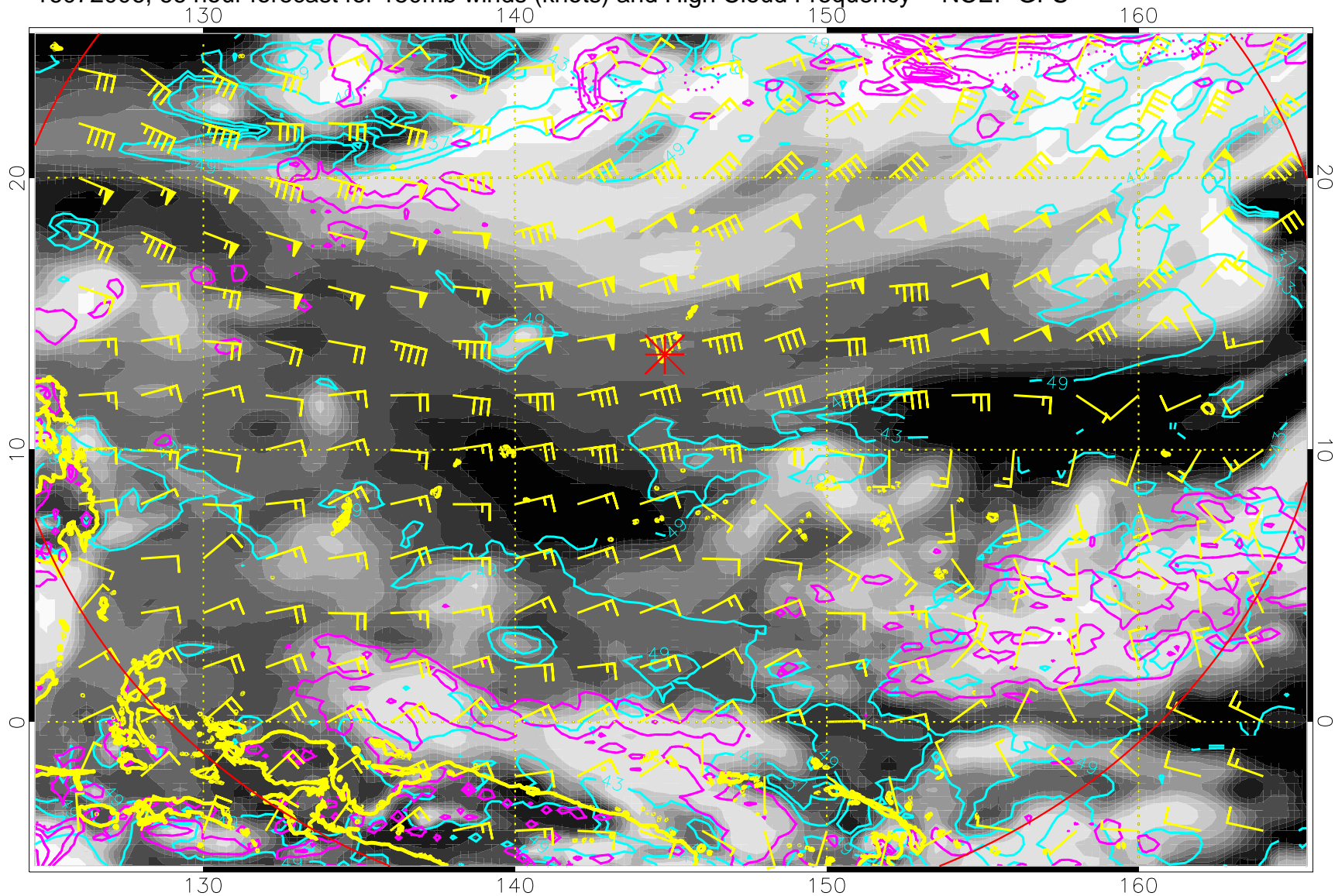
16072006, 66 hour forecast for 150mb winds (knots) and High Cloud Frequency -- NCEP GFS
