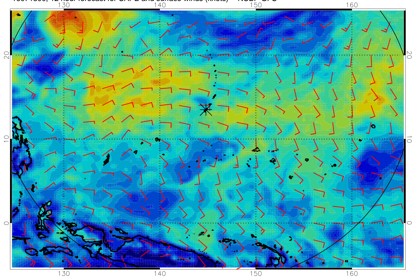
16071800, 12 hour forecast for CAPE and surface winds (knots) -- NCEP GFS
