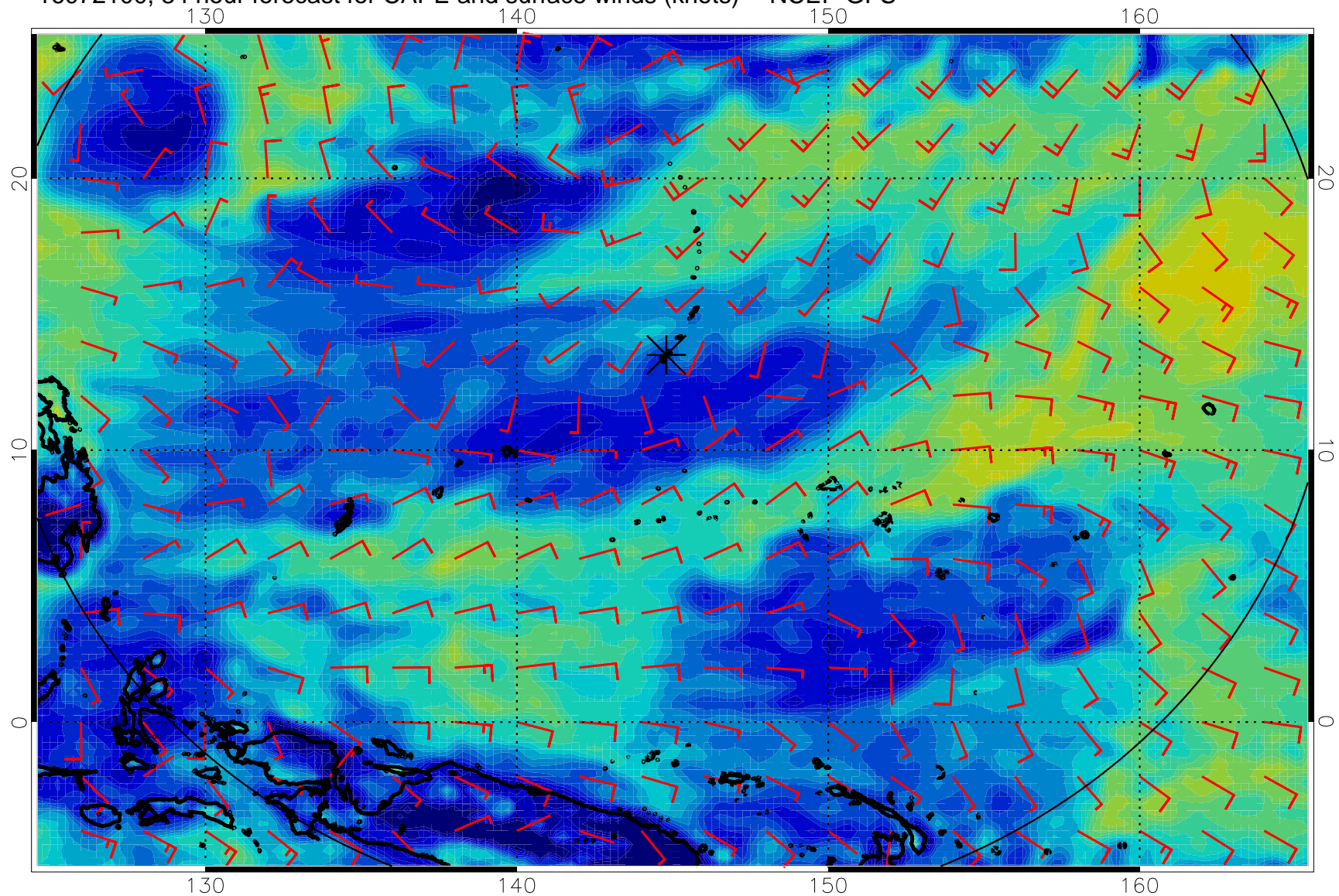
16072100, 84 hour forecast for CAPE and surface winds (knots) -- NCEP GFS
