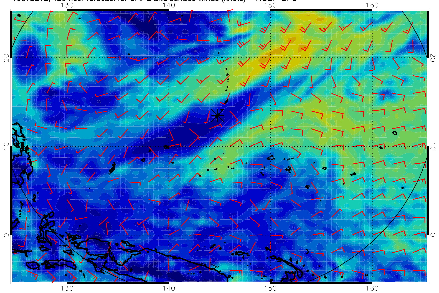
16072212, 120 hour forecast for CAPE and surface winds (knots) -- NCEP GFS
