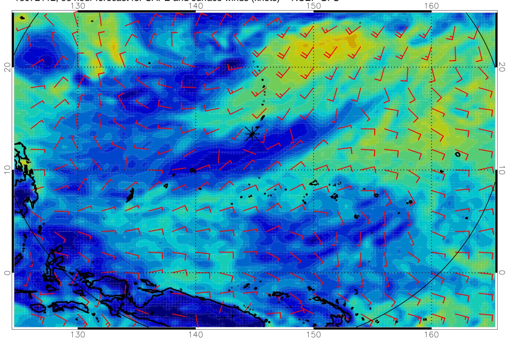
16072112, 96 hour forecast for CAPE and surface winds (knots) -- NCEP GFS
