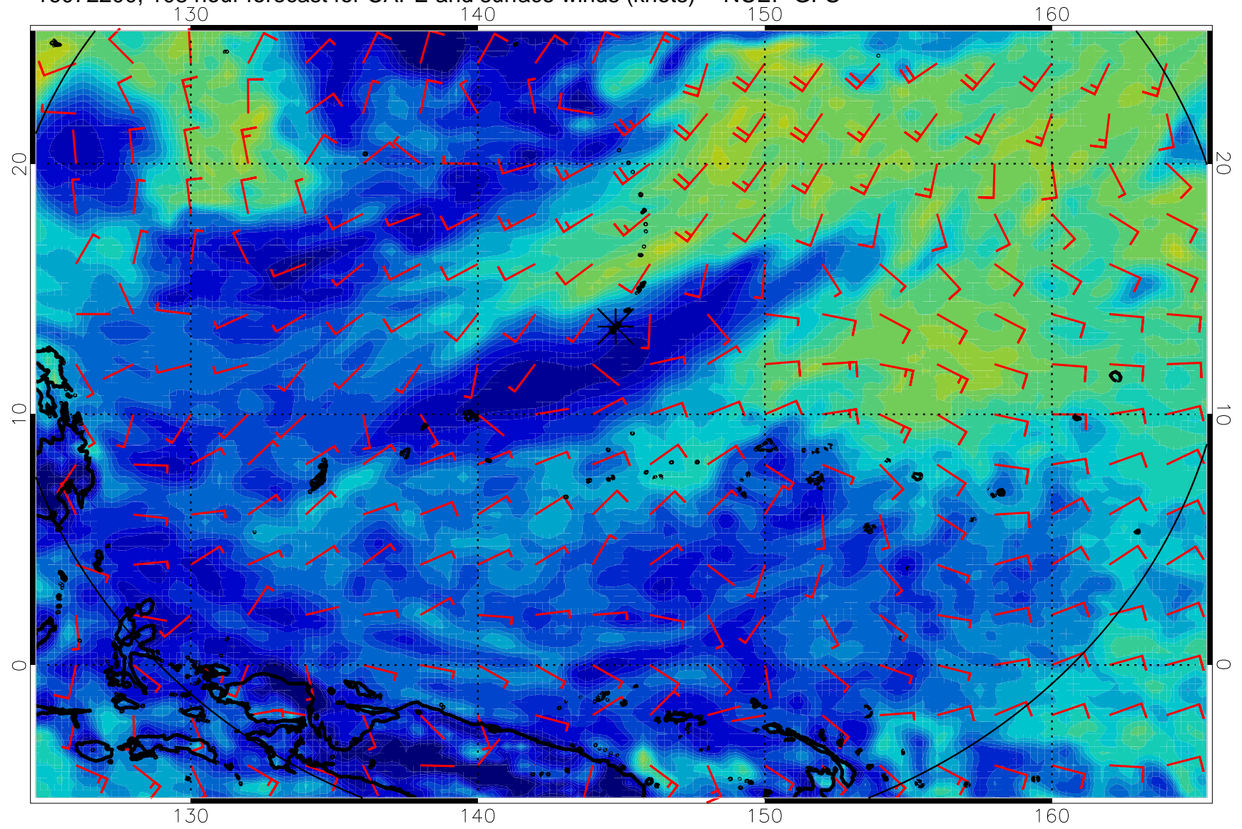
16072200, 108 hour forecast for CAPE and surface winds (knots) -- NCEP GFS
