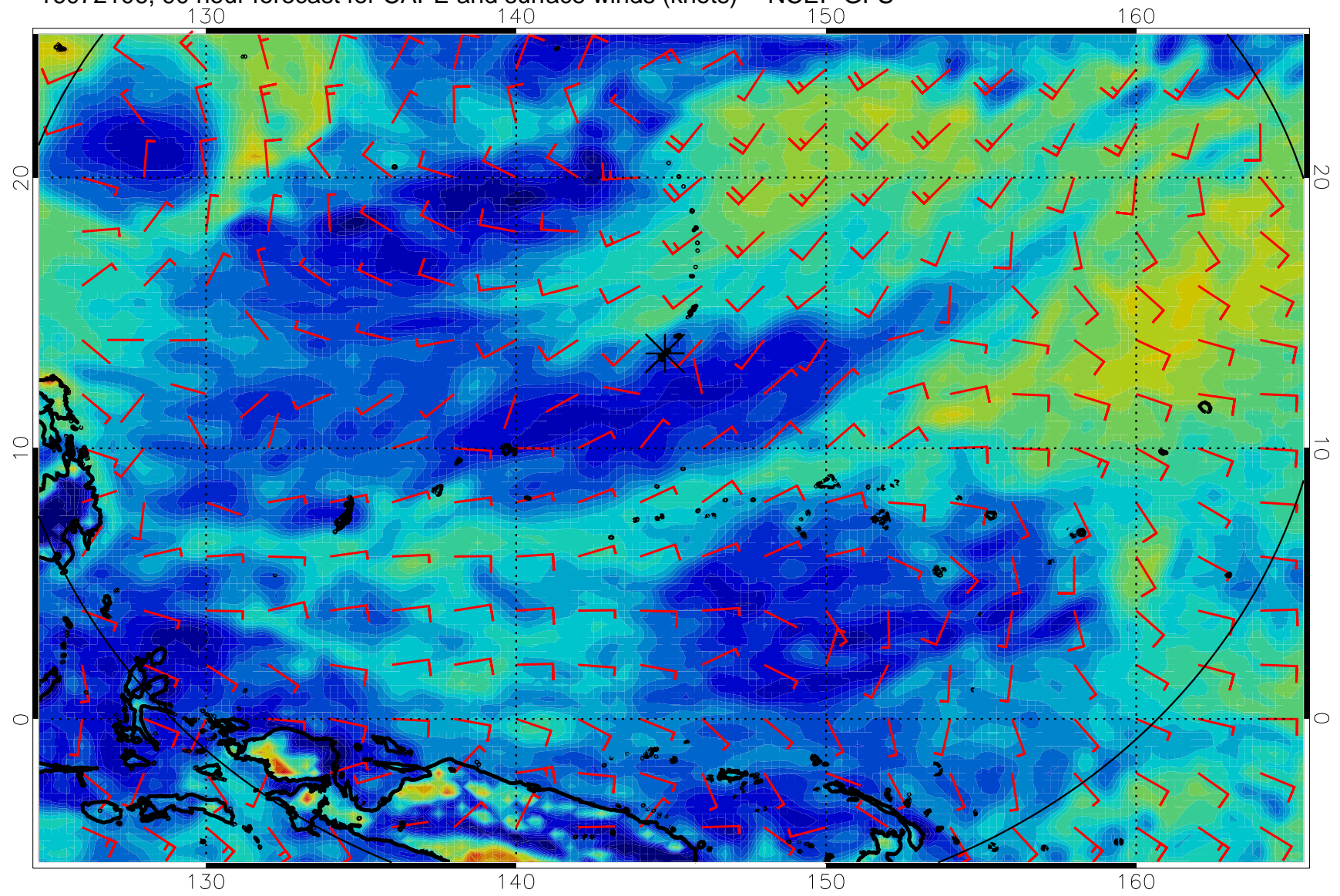
16072106, 90 hour forecast for CAPE and surface winds (knots) -- NCEP GFS
