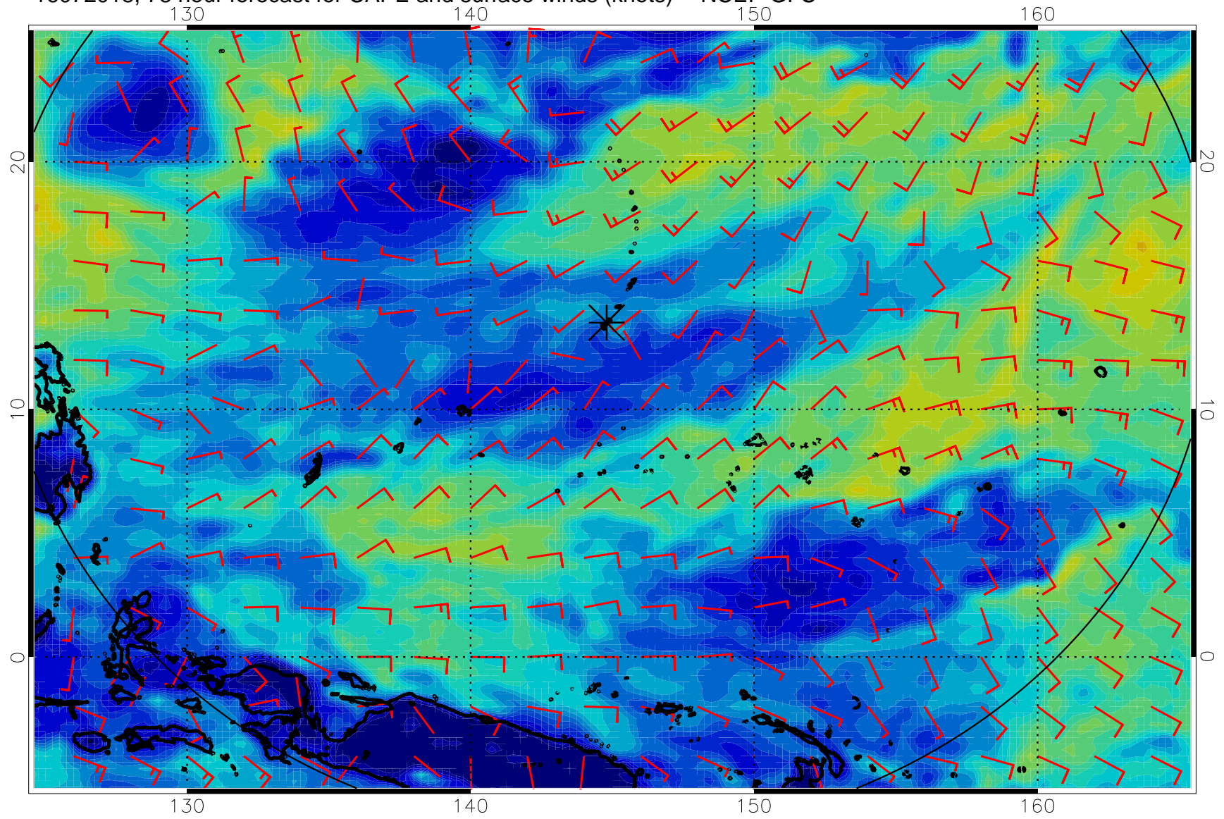
16072018, 78 hour forecast for CAPE and surface winds (knots) -- NCEP GFS
