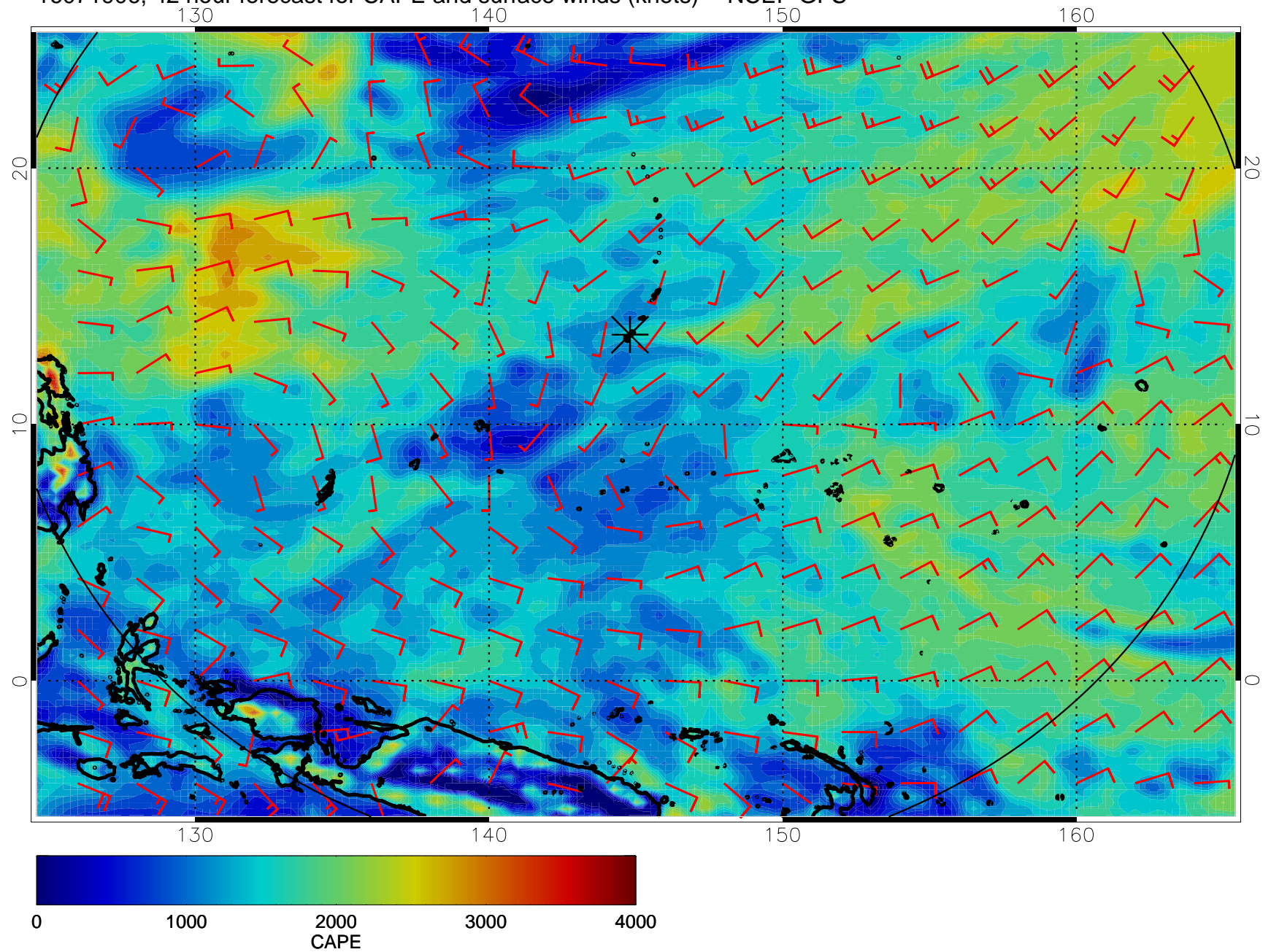
16071906, 42 hour forecast for CAPE and surface winds (knots) -- NCEP GFS
