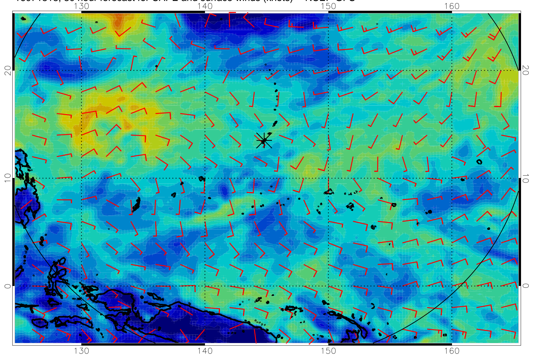
16071818, 30 hour forecast for CAPE and surface winds (knots) -- NCEP GFS
