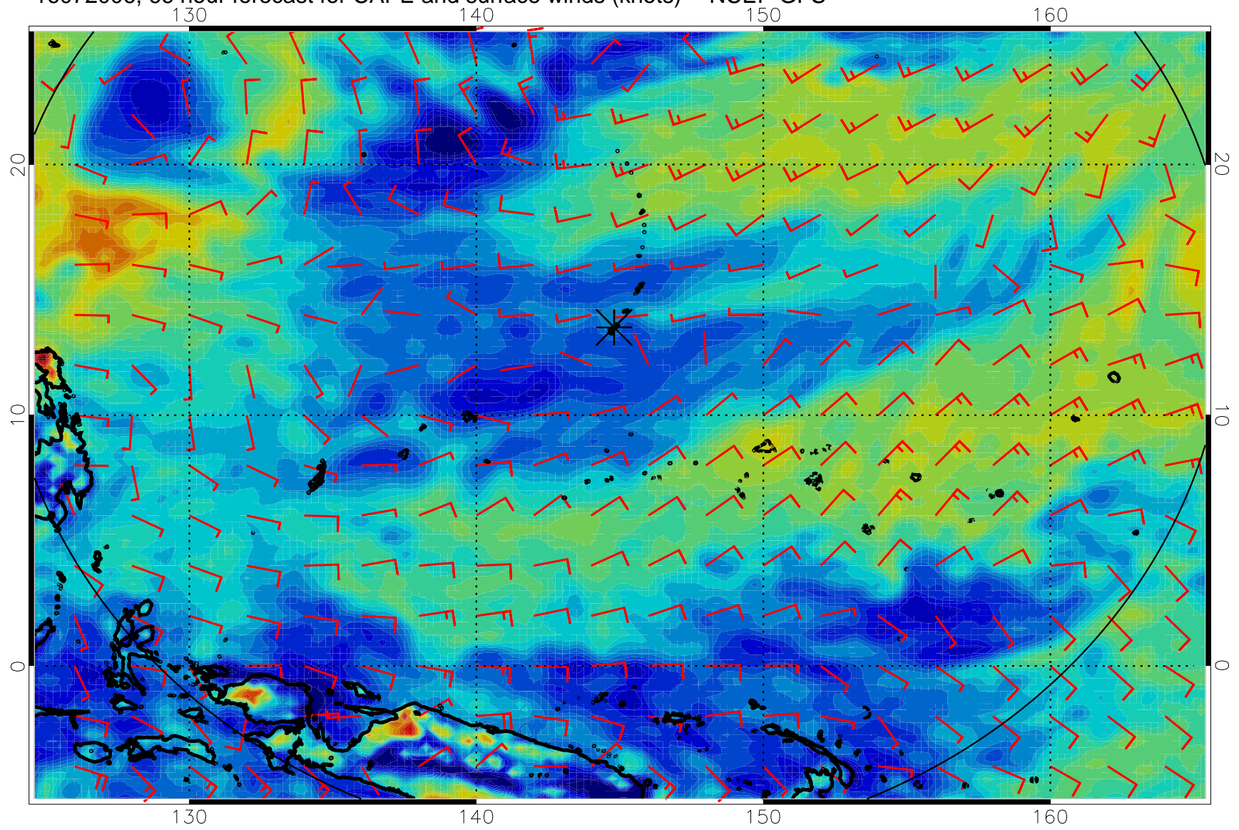
16072006, 66 hour forecast for CAPE and surface winds (knots) -- NCEP GFS
