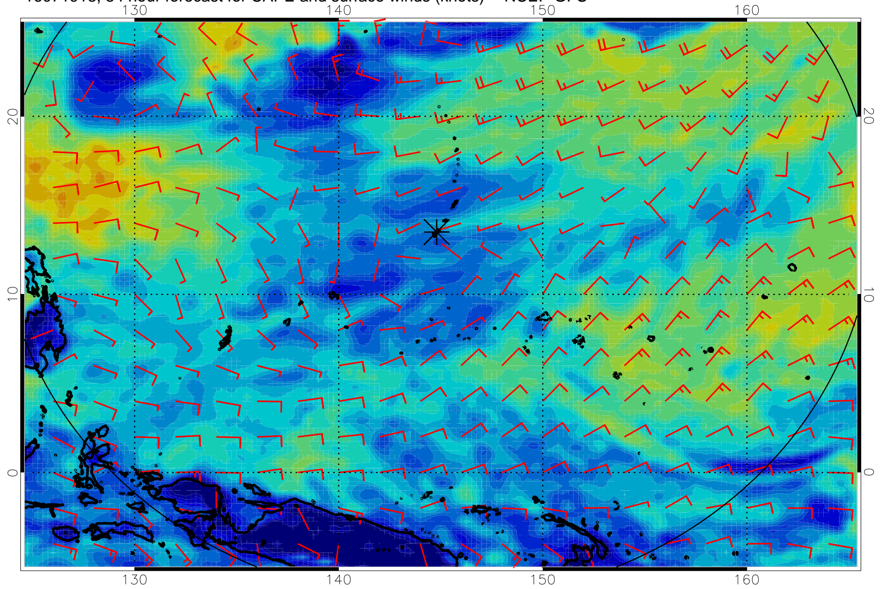
16071918, 54 hour forecast for CAPE and surface winds (knots) -- NCEP GFS
