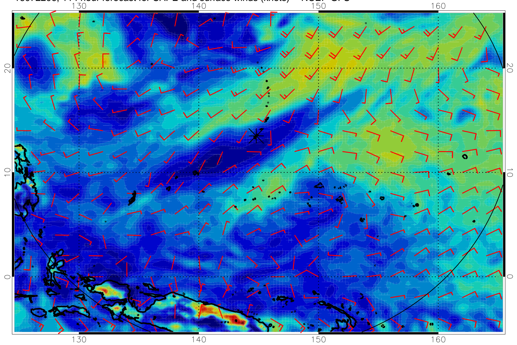
16072206, 114 hour forecast for CAPE and surface winds (knots) -- NCEP GFS
