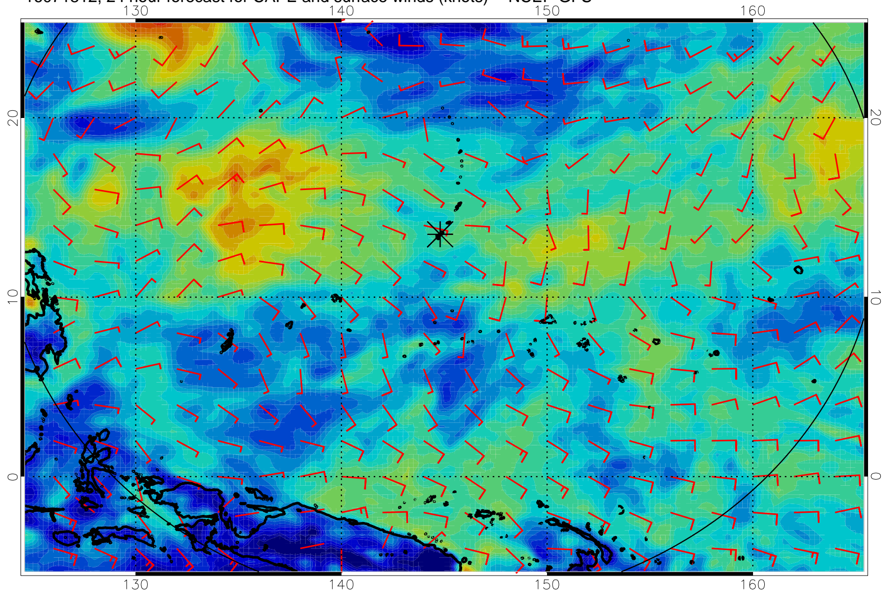
16071812, 24 hour forecast for CAPE and surface winds (knots) -- NCEP GFS
