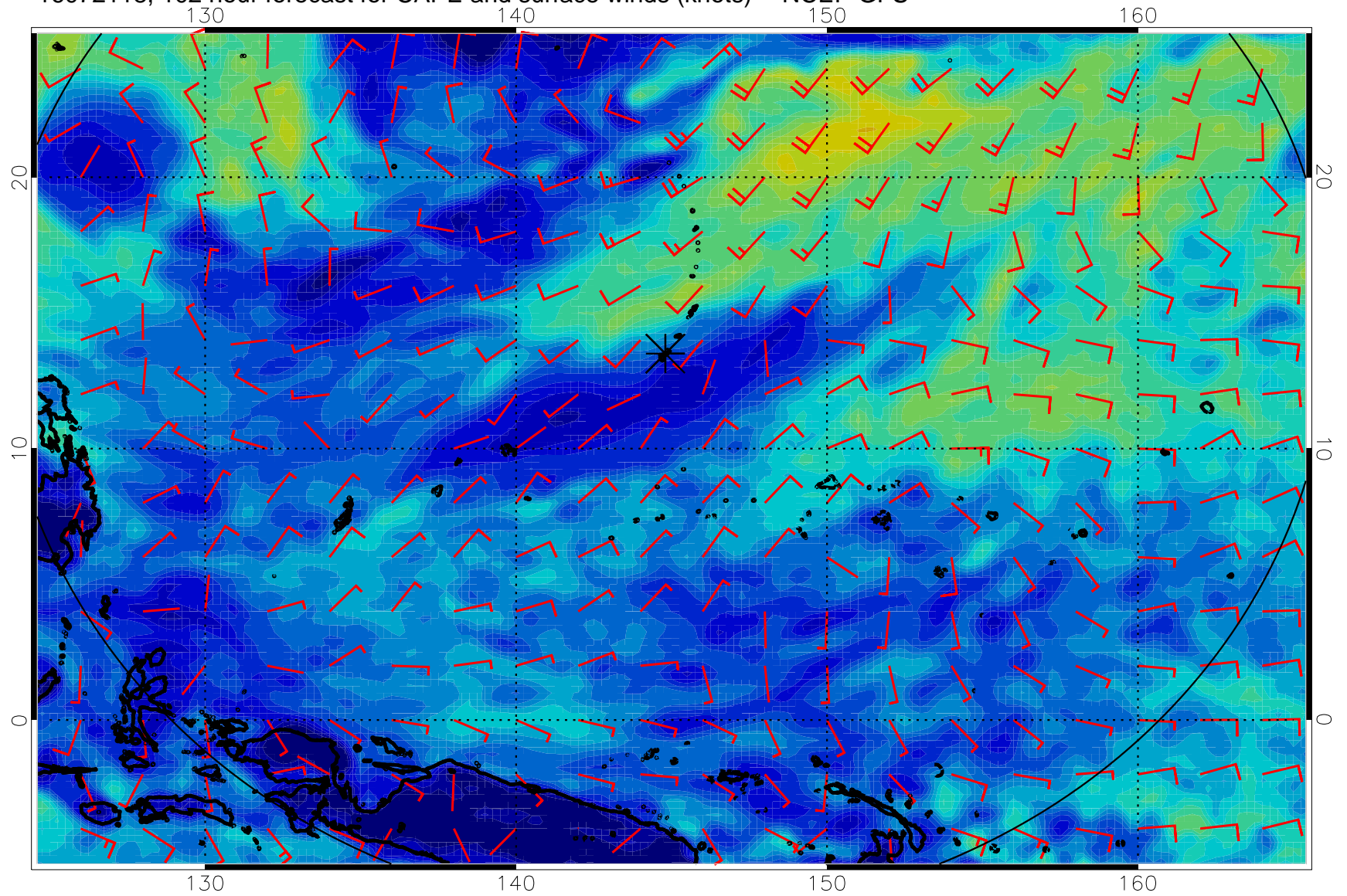
16072118, 102 hour forecast for CAPE and surface winds (knots) -- NCEP GFS
