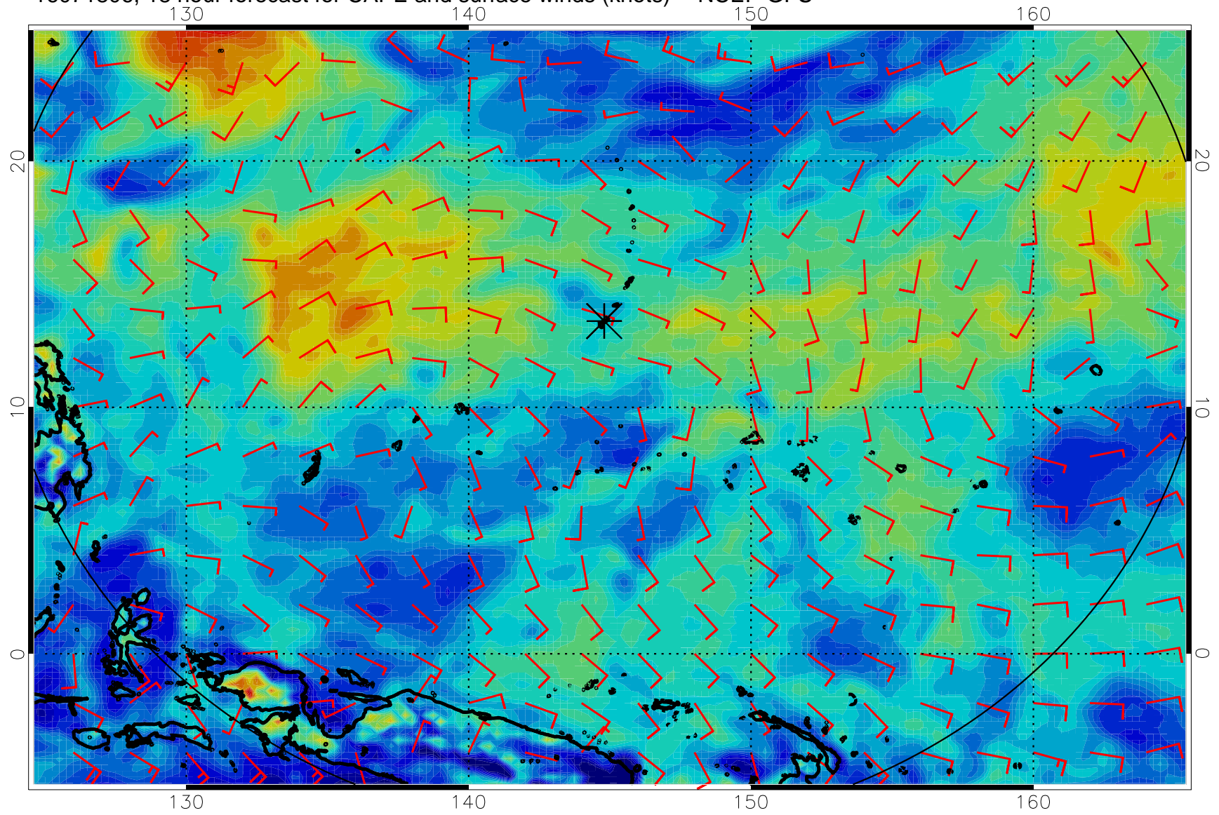
16071806, 18 hour forecast for CAPE and surface winds (knots) -- NCEP GFS
