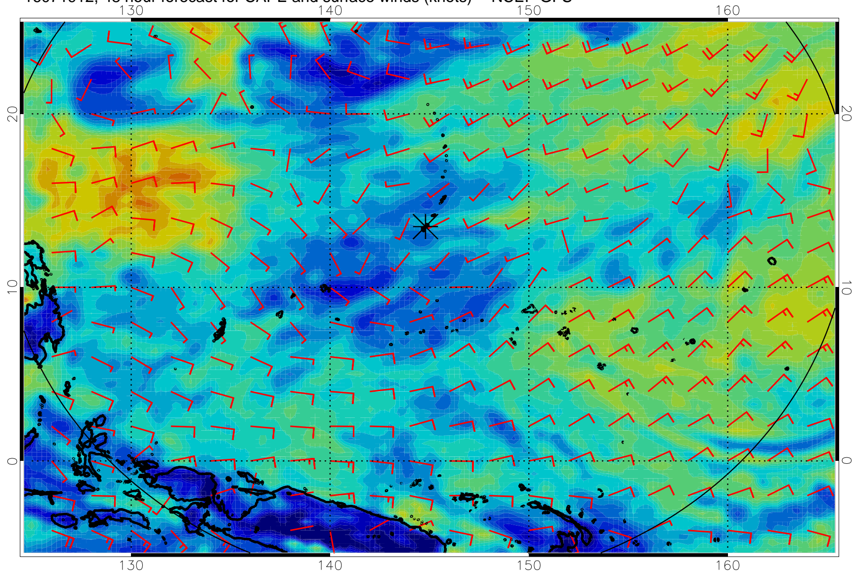
16071912, 48 hour forecast for CAPE and surface winds (knots) -- NCEP GFS
