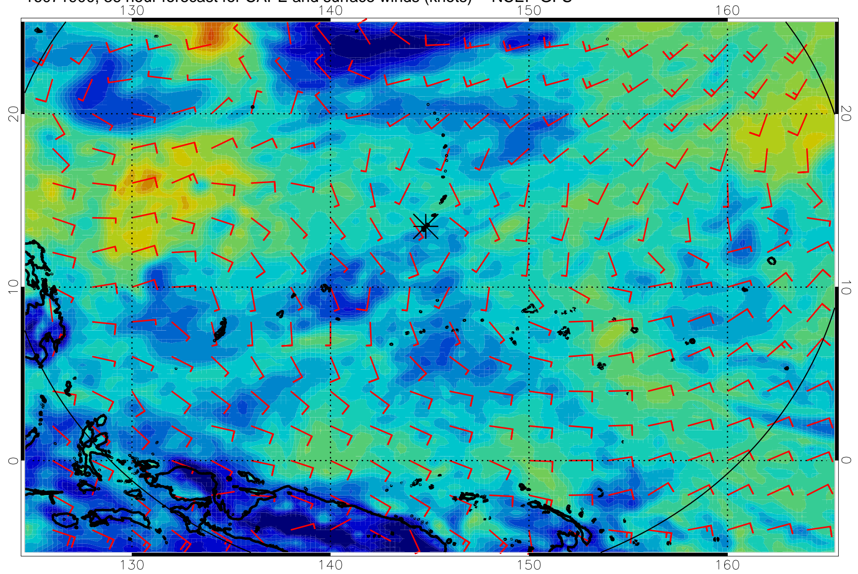
16071900, 36 hour forecast for CAPE and surface winds (knots) -- NCEP GFS
