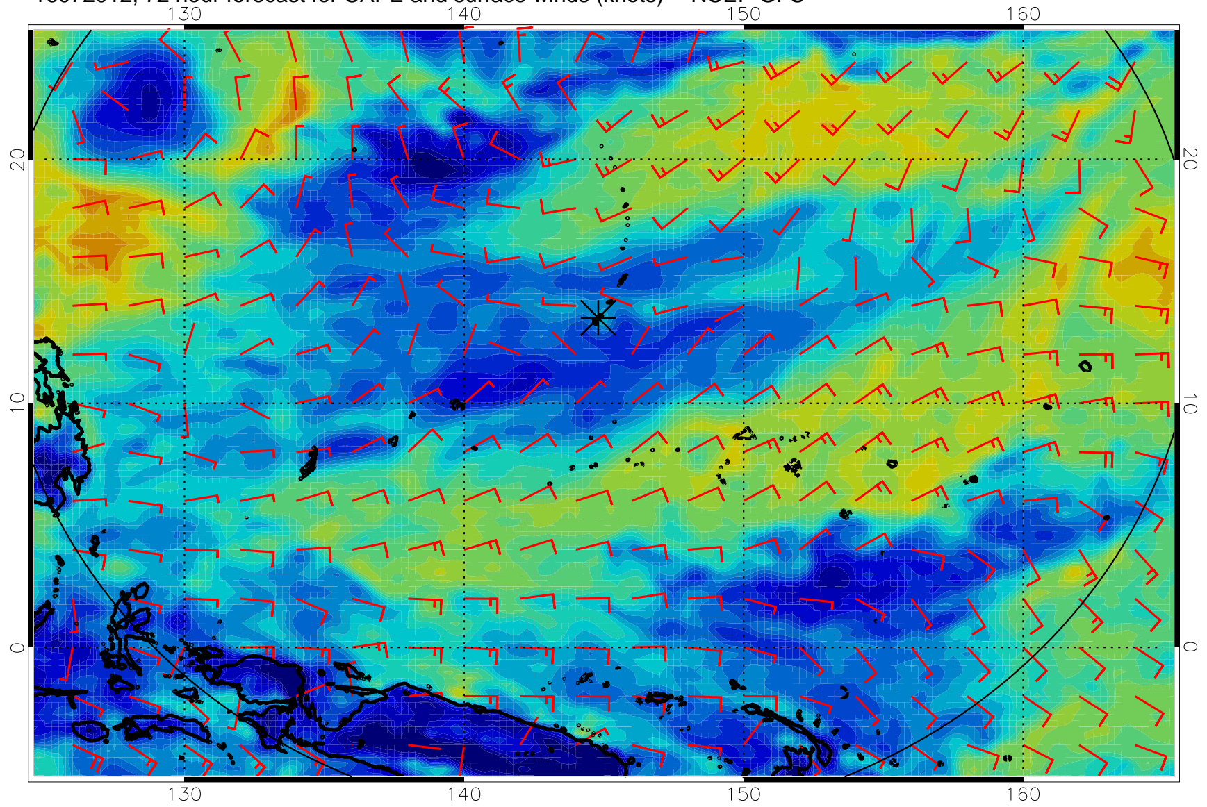
16072012, 72 hour forecast for CAPE and surface winds (knots) -- NCEP GFS
