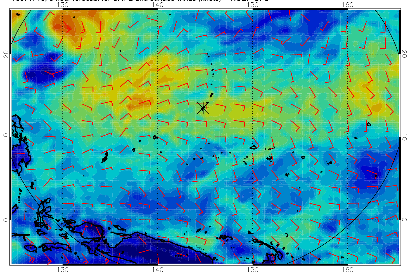
16071718, 6 hour forecast for CAPE and surface winds (knots) -- NCEP GFS
