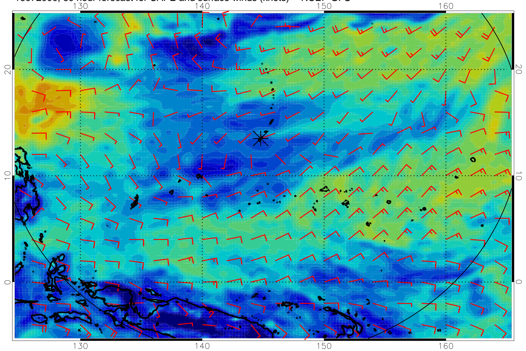
16072000, 60 hour forecast for CAPE and surface winds (knots) -- NCEP GFS
