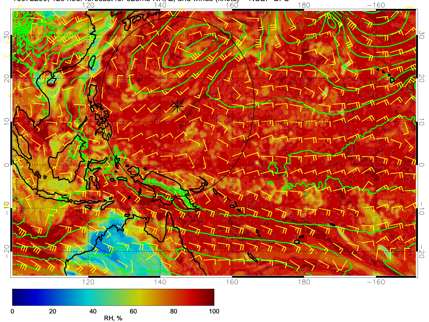
16072200, 120 hour forecast for 925mb RH, Z, and winds (knots) -- NCEP GFS
