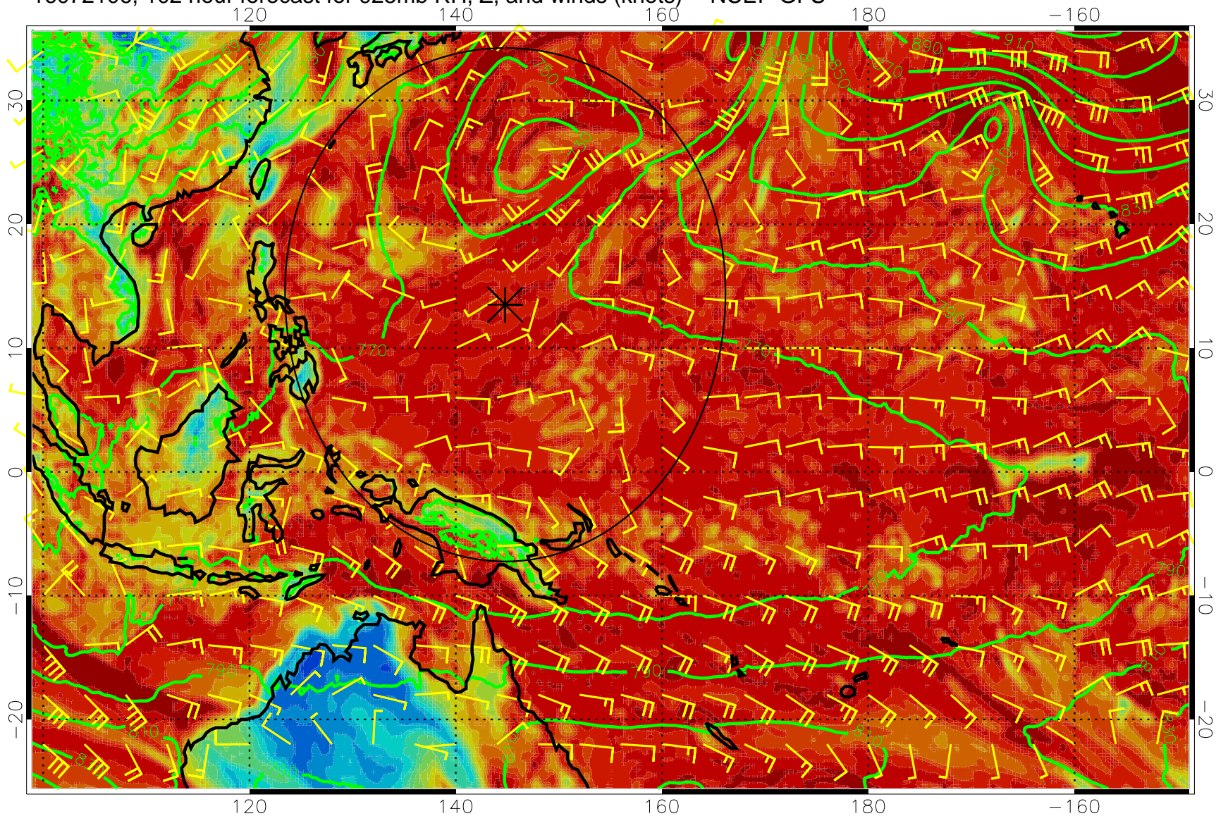
16072106, 102 hour forecast for 925mb RH, Z, and winds (knots) -- NCEP GFS
