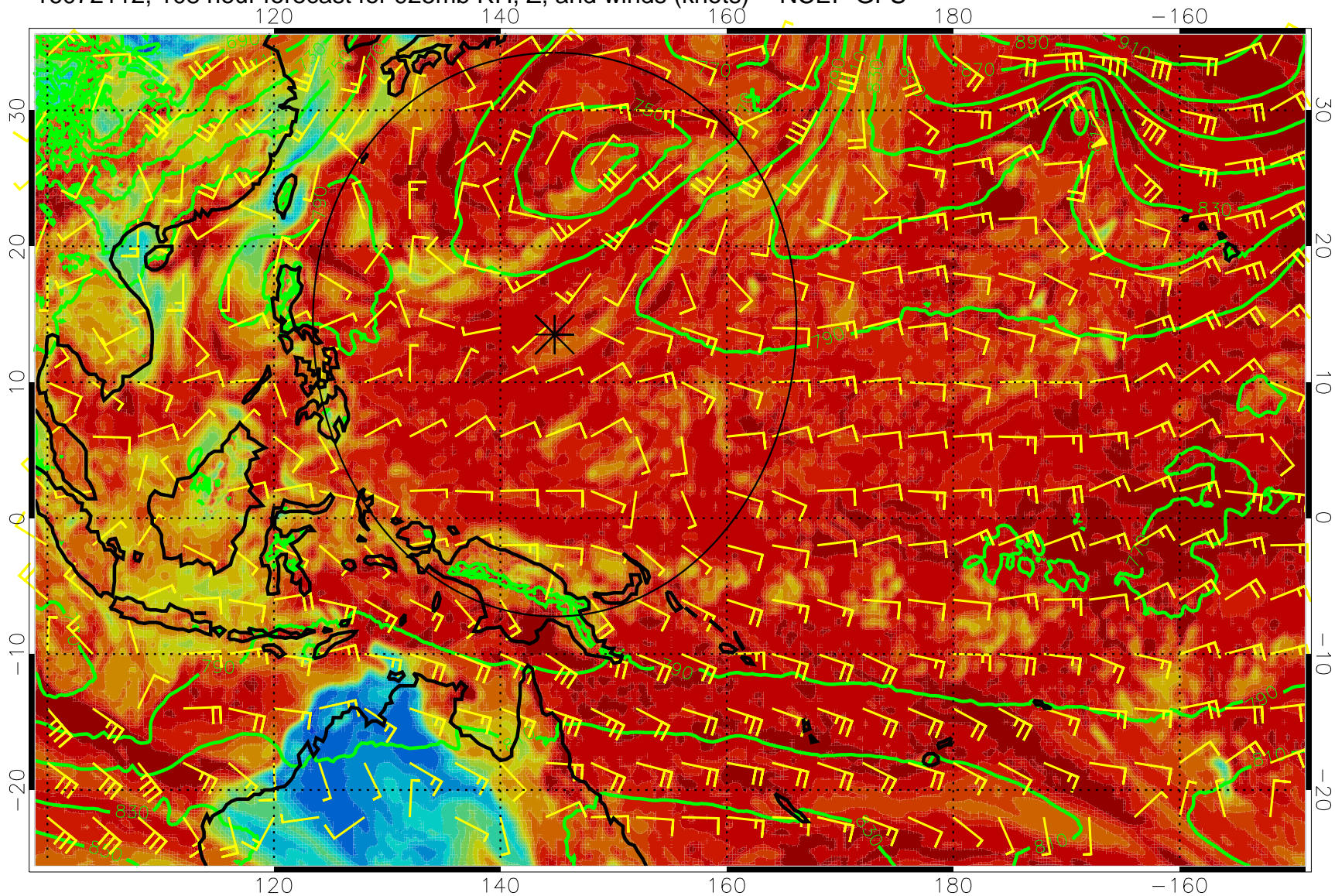
16072112, 108 hour forecast for 925mb RH, Z, and winds (knots) -- NCEP GFS
