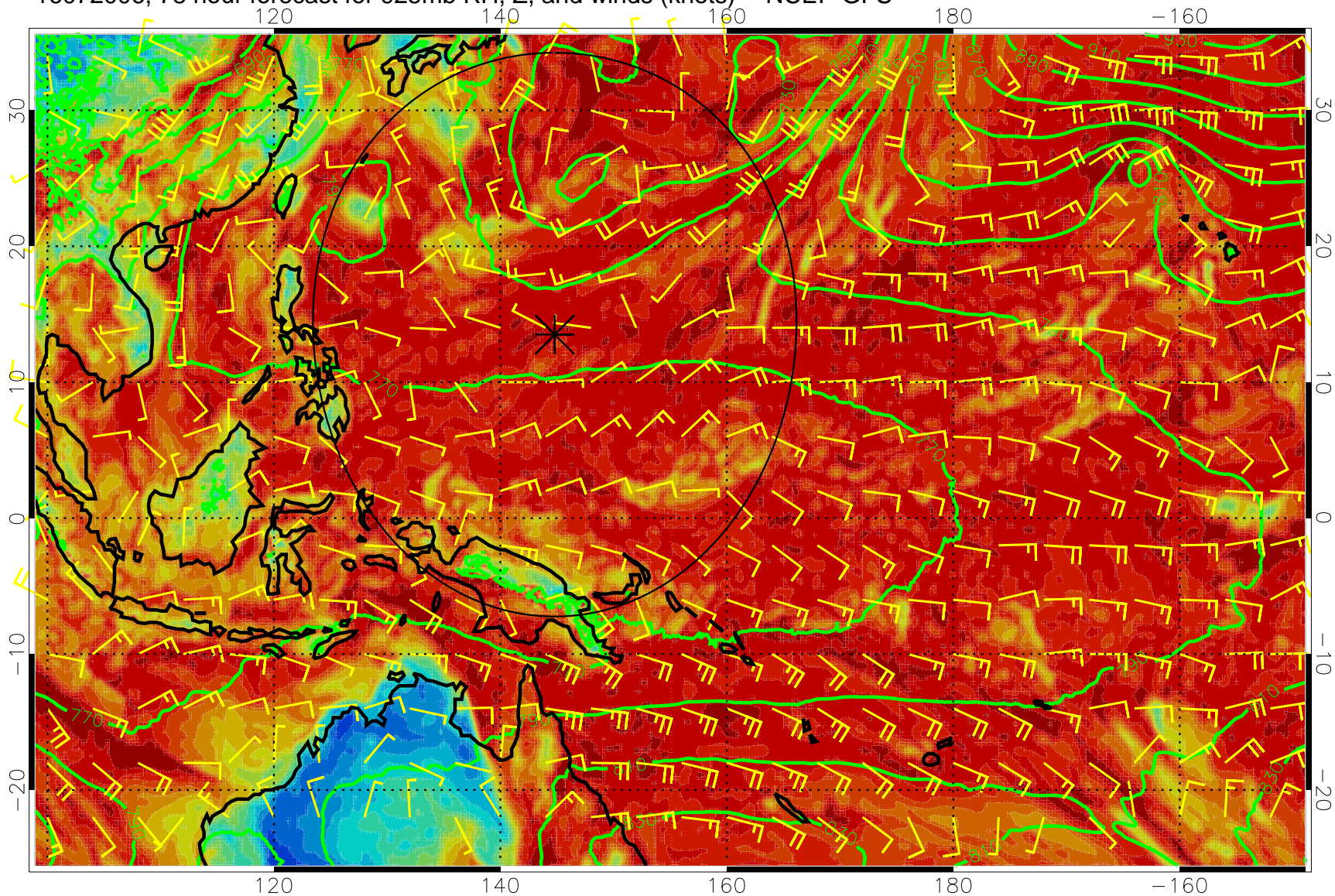
16072006, 78 hour forecast for 925mb RH, Z, and winds (knots) -- NCEP GFS
