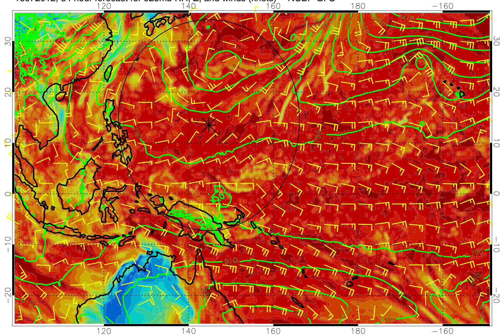
16072012, 84 hour forecast for 925mb RH, Z, and winds (knots) -- NCEP GFS
