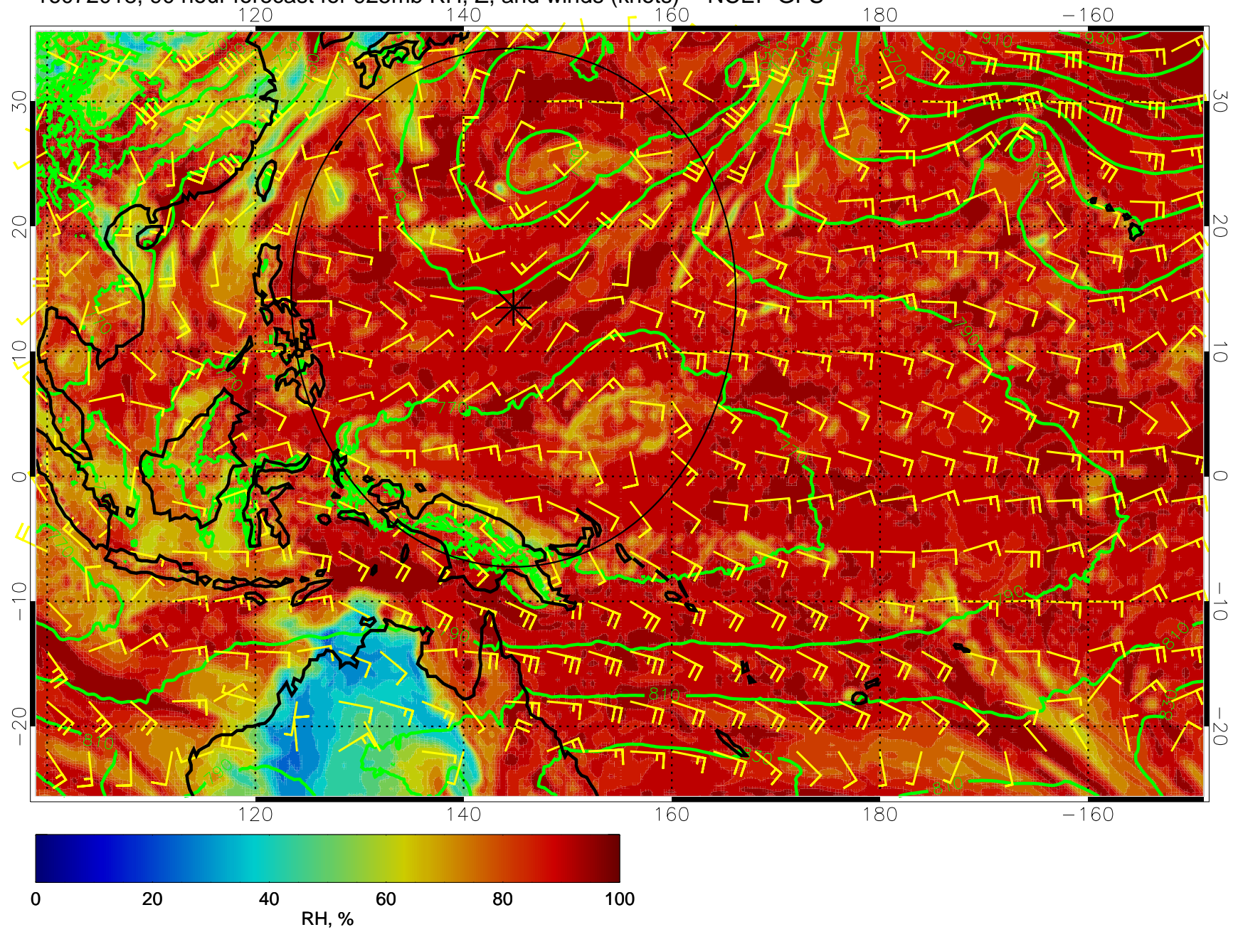
16072018, 90 hour forecast for 925mb RH, Z, and winds (knots) -- NCEP GFS
