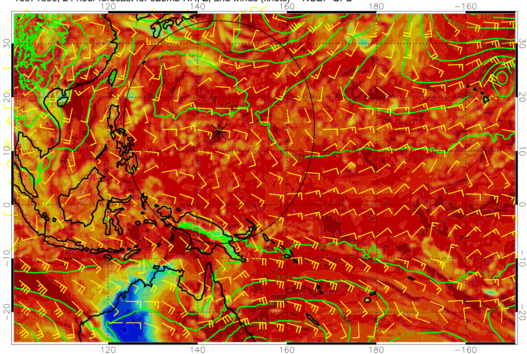
16071800, 24 hour forecast for 925mb RH, Z, and winds (knots) -- NCEP GFS
