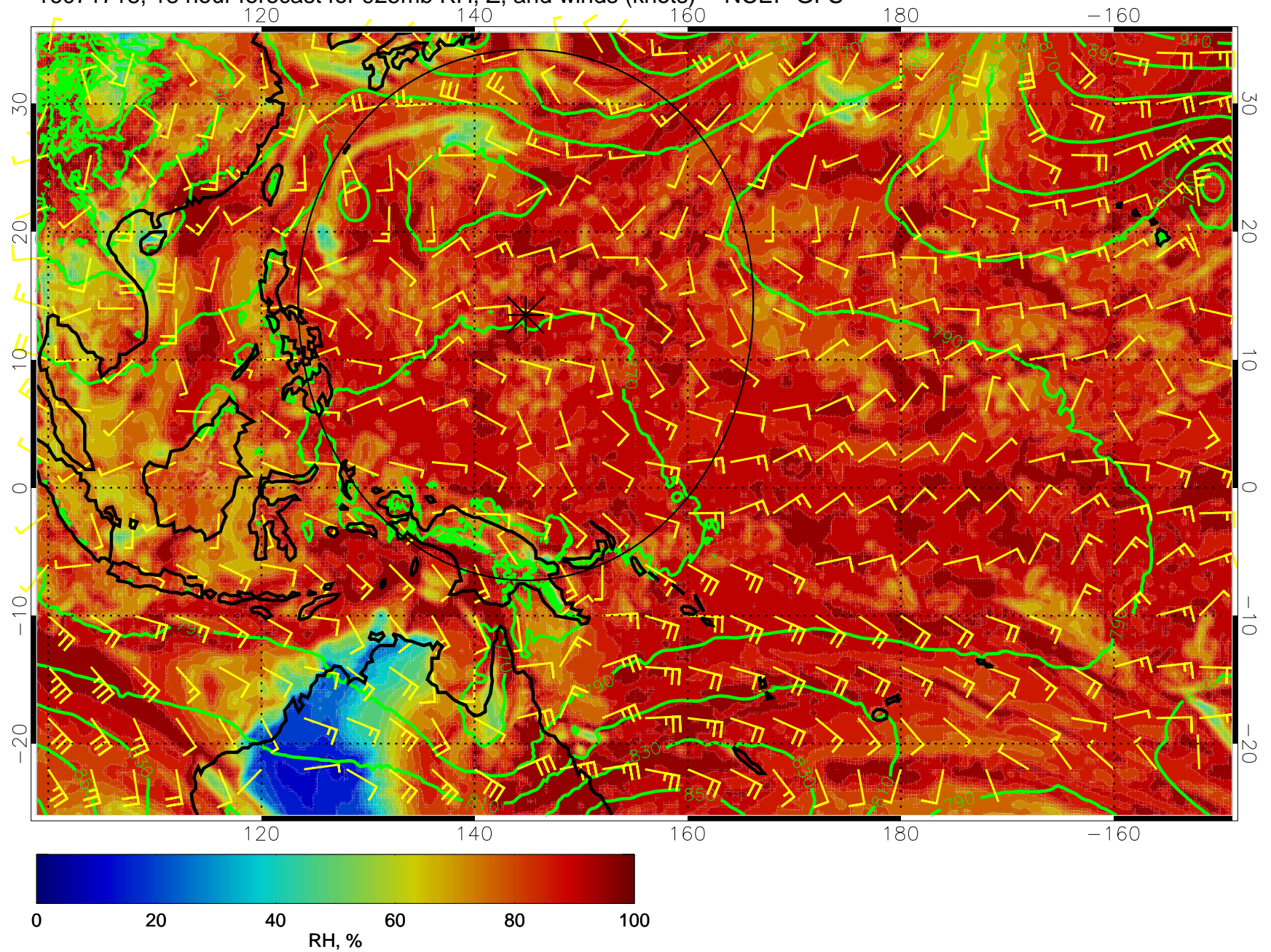
16071718, 18 hour forecast for 925mb RH, Z, and winds (knots) -- NCEP GFS
