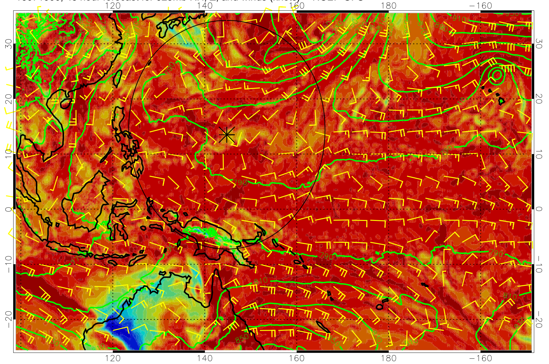
16071900, 48 hour forecast for 925mb RH, Z, and winds (knots) -- NCEP GFS
