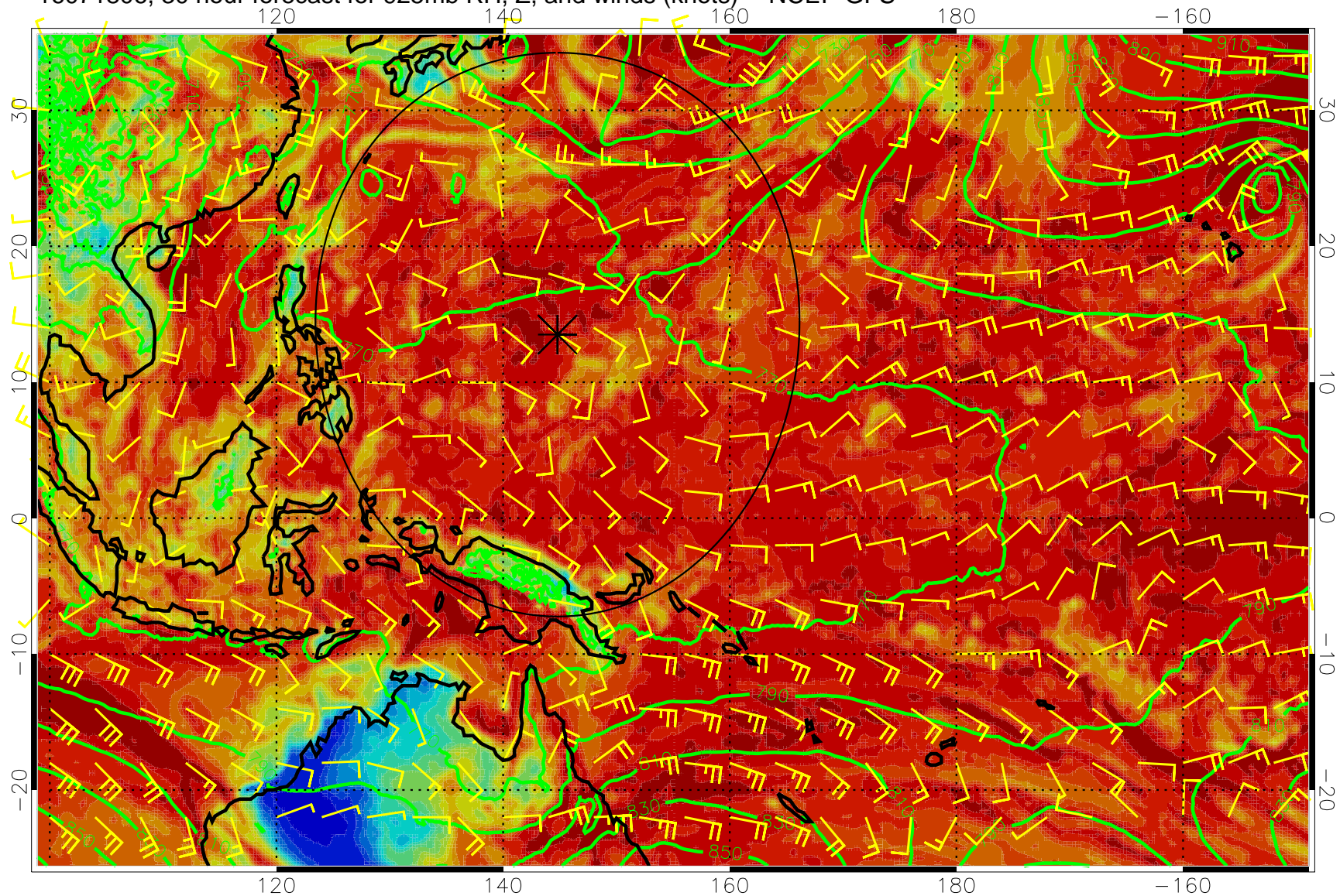
16071806, 30 hour forecast for 925mb RH, Z, and winds (knots) -- NCEP GFS
