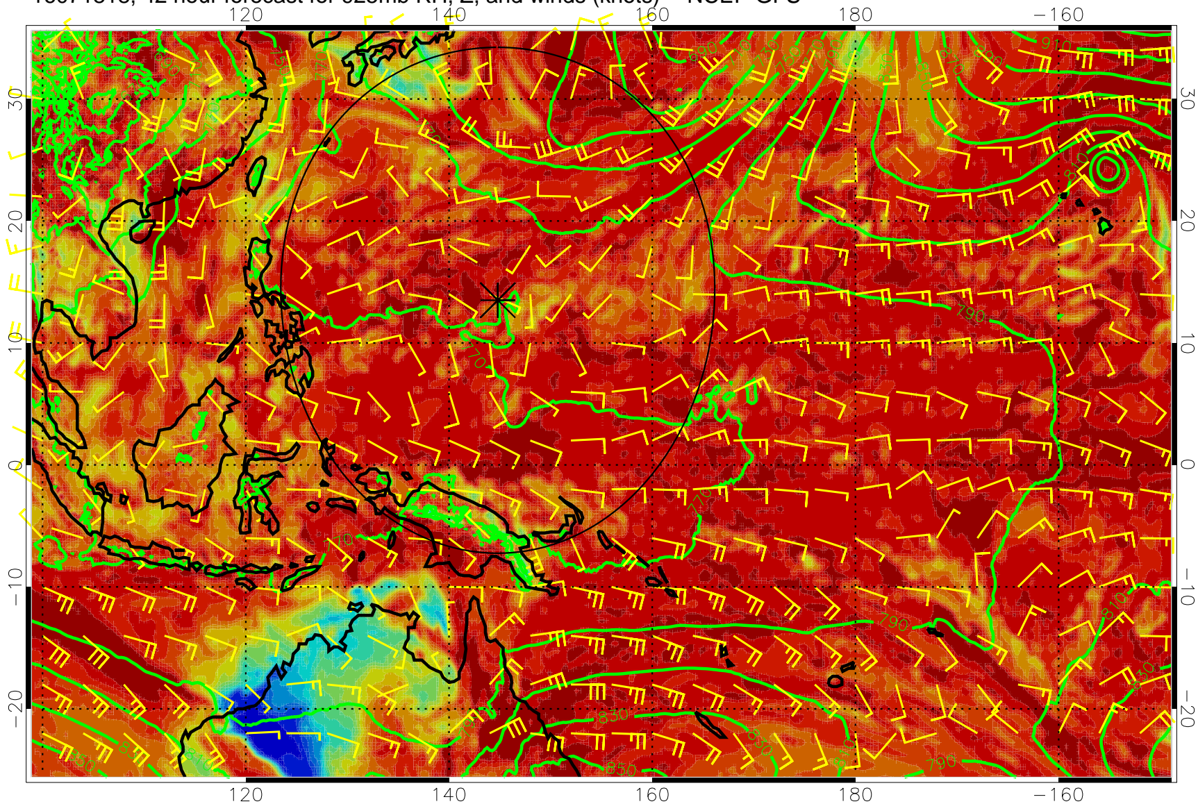
16071818, 42 hour forecast for 925mb RH, Z, and winds (knots) -- NCEP GFS
