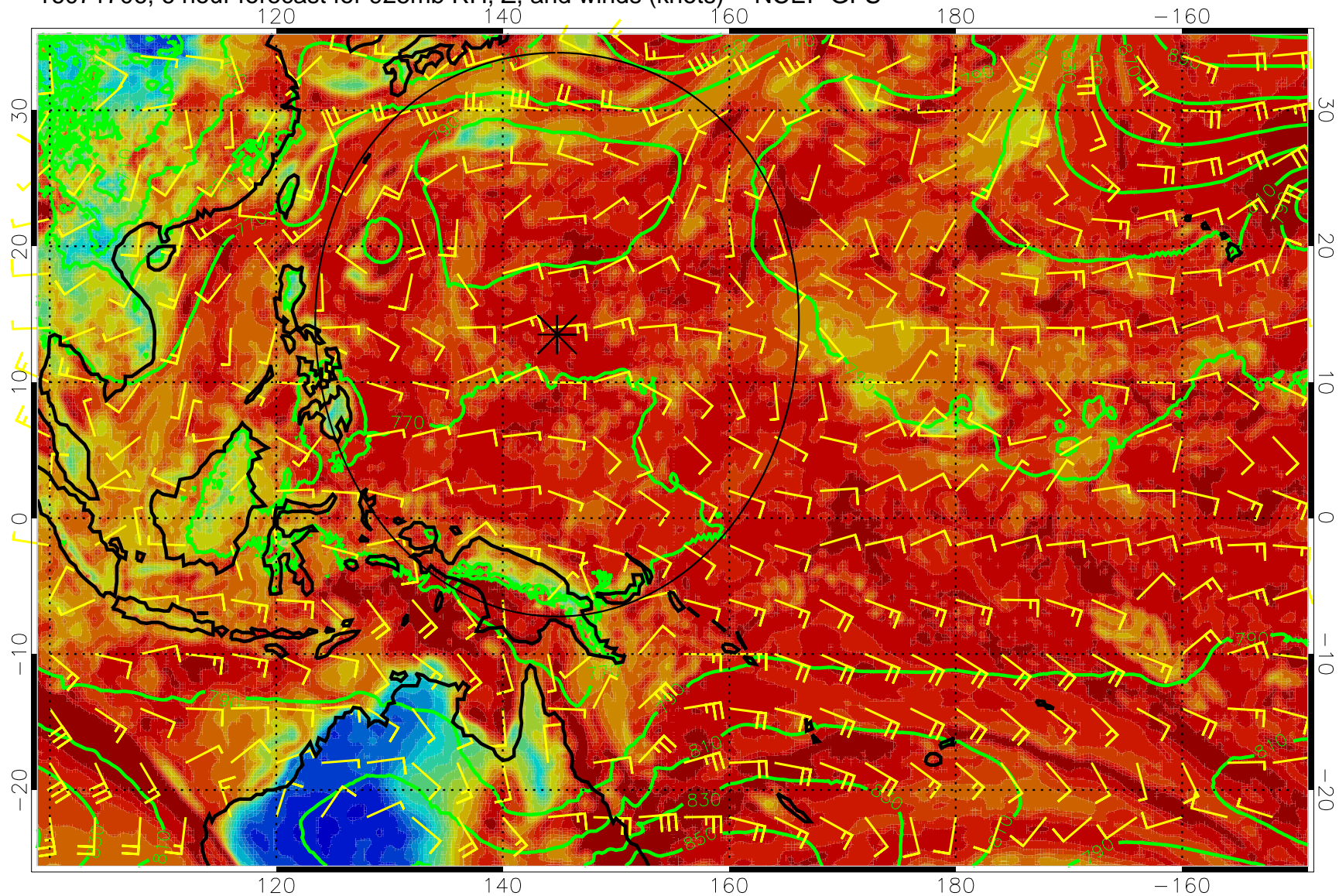
16071706, 6 hour forecast for 925mb RH, Z, and winds (knots) -- NCEP GFS
