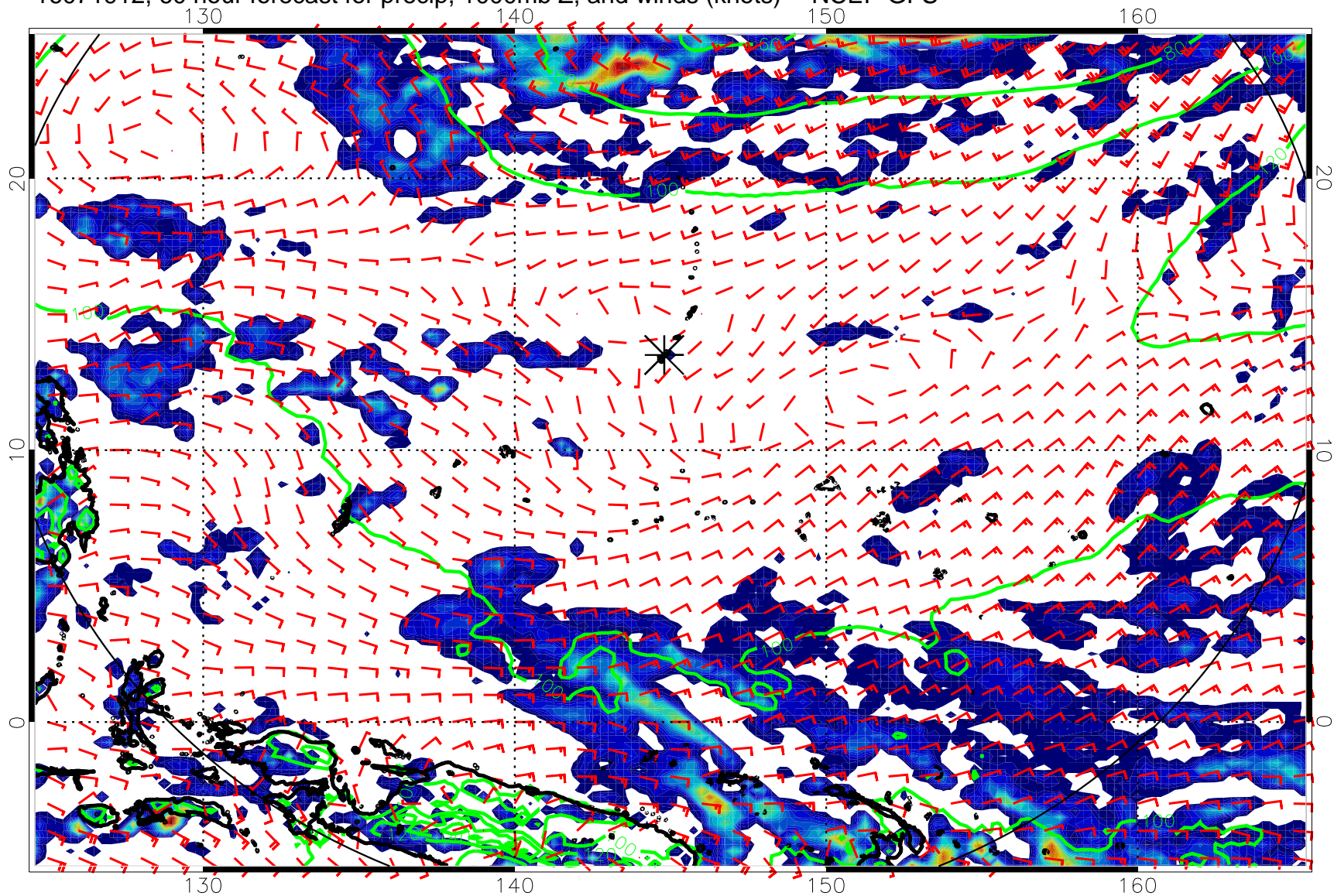
16071912, 60 hour forecast for precip, 1000mb Z, and winds (knots) -- NCEP GFS
