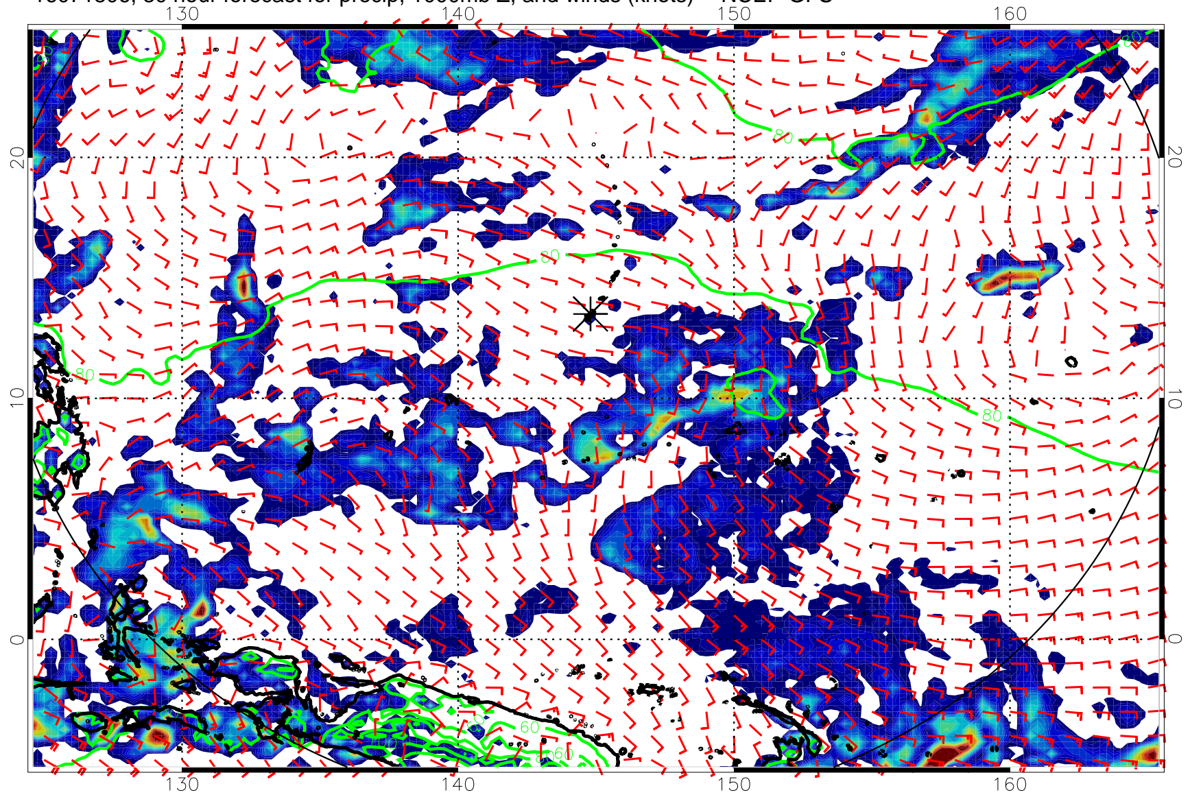
16071806, 30 hour forecast for precip, 1000mb Z, and winds (knots) -- NCEP GFS
