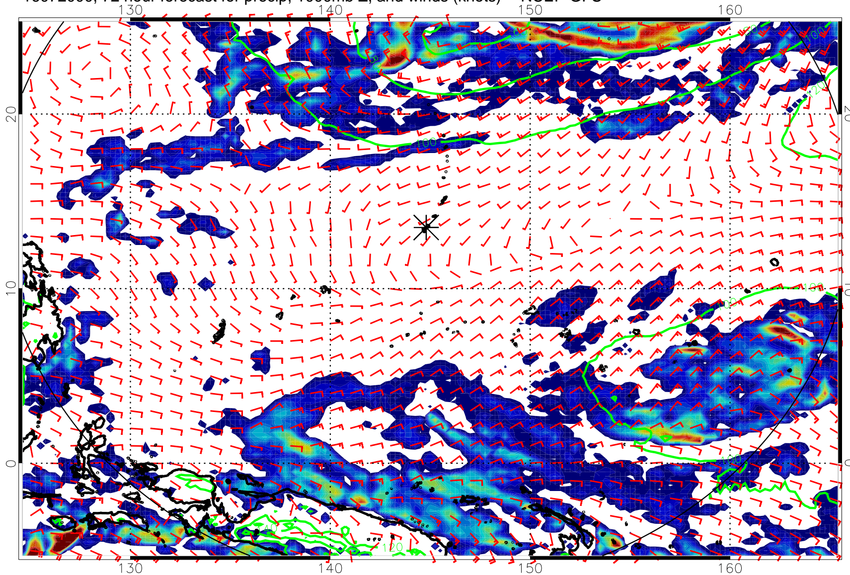
16072000, 72 hour forecast for precip, 1000mb Z, and winds (knots) -- NCEP GFS
