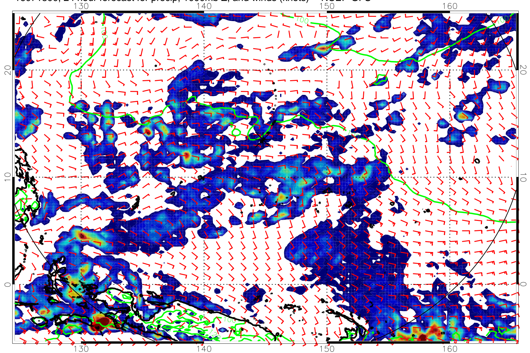
16071800, 24 hour forecast for precip, 1000mb Z, and winds (knots) -- NCEP GFS
