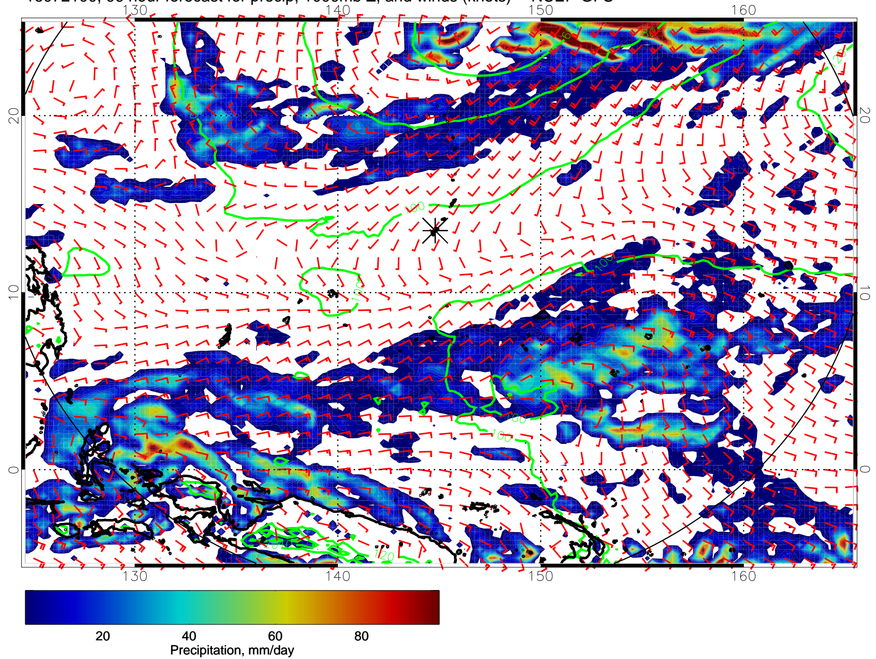
16072100, 96 hour forecast for precip, 1000mb Z, and winds (knots) -- NCEP GFS
