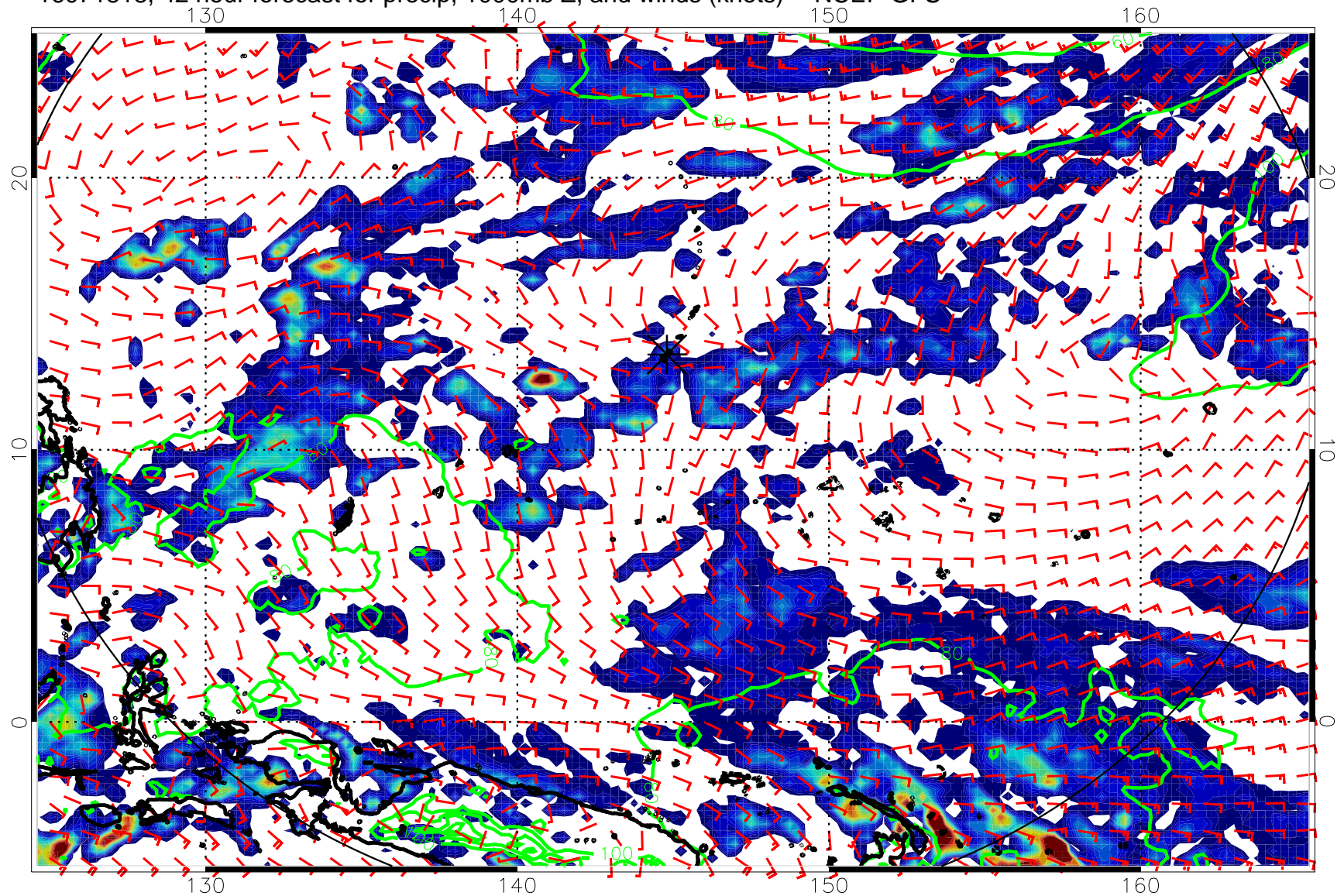
16071818, 42 hour forecast for precip, 1000mb Z, and winds (knots) -- NCEP GFS
