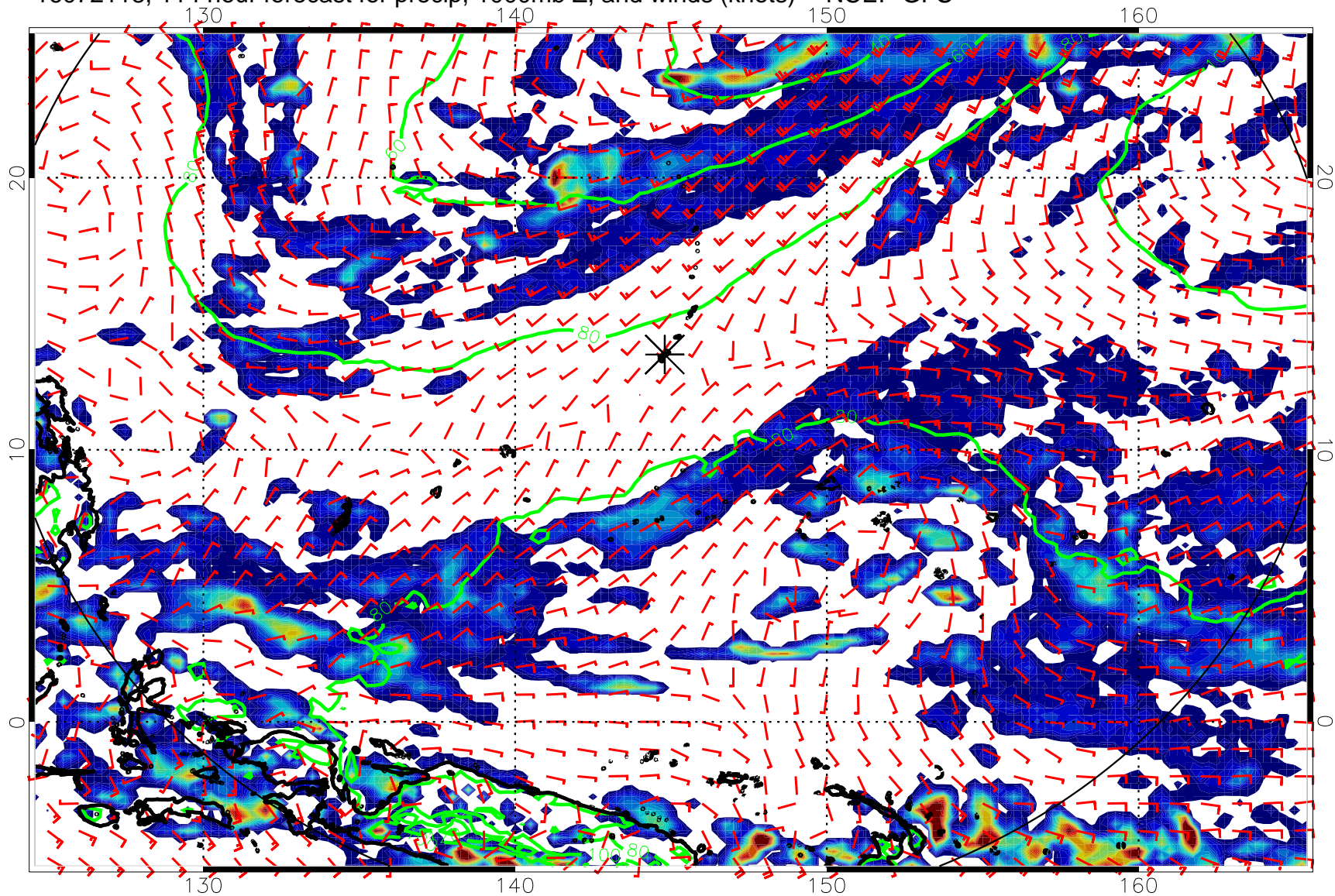
16072118, 114 hour forecast for precip, 1000mb Z, and winds (knots) -- NCEP GFS
