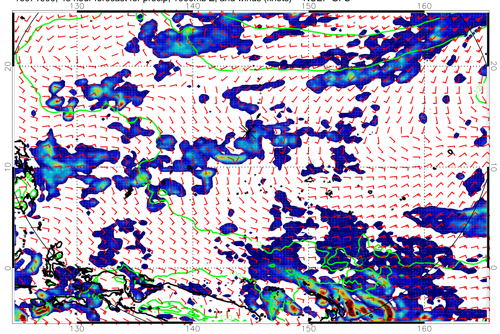
16071900, 48 hour forecast for precip, 1000mb Z, and winds (knots) -- NCEP GFS
