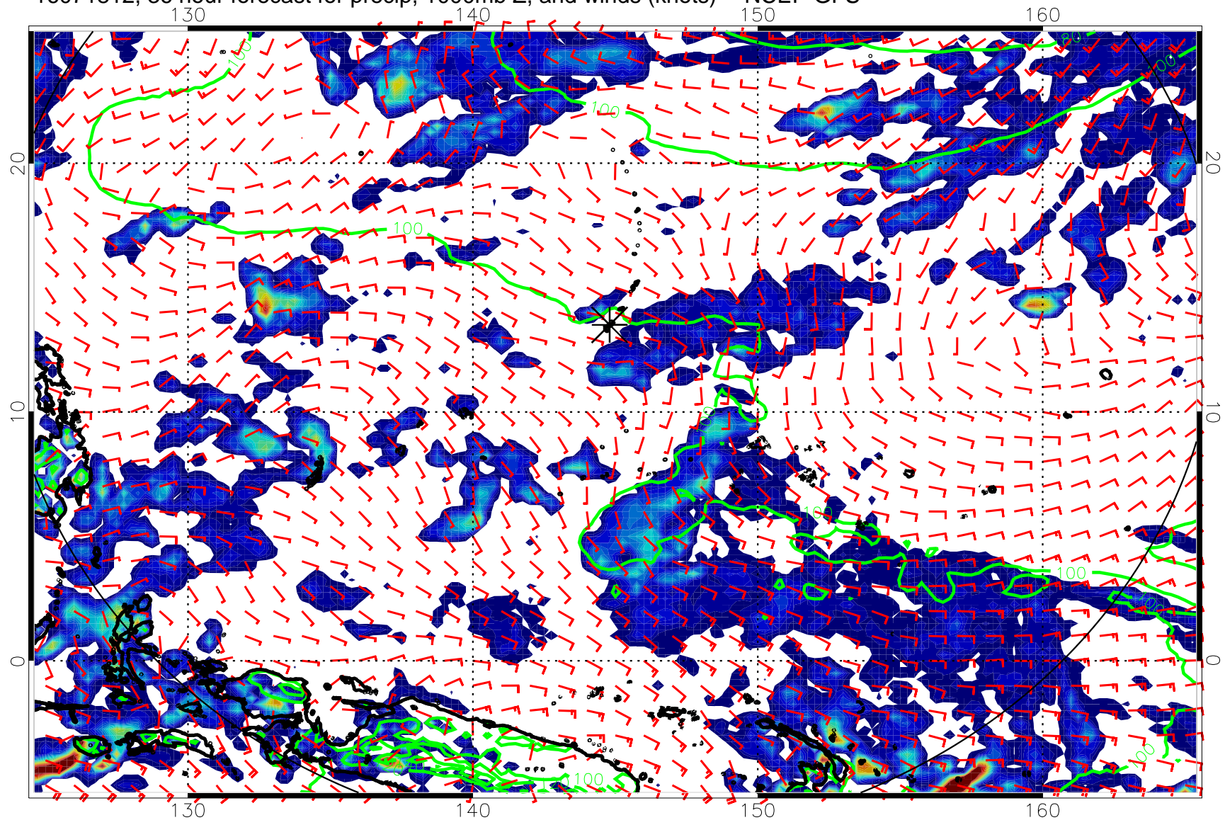
16071812, 36 hour forecast for precip, 1000mb Z, and winds (knots) -- NCEP GFS
