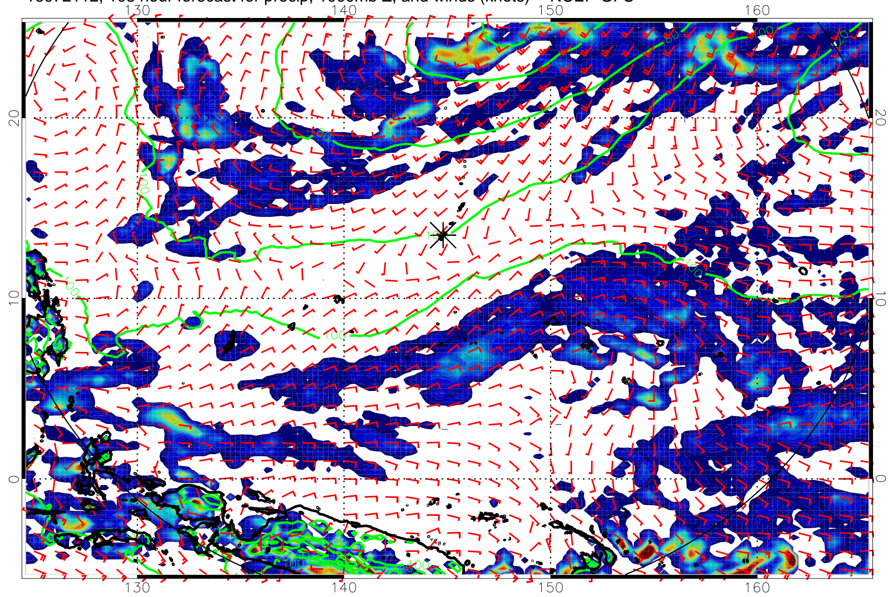
16072112, 108 hour forecast for precip, 1000mb Z, and winds (knots) -- NCEP GFS
