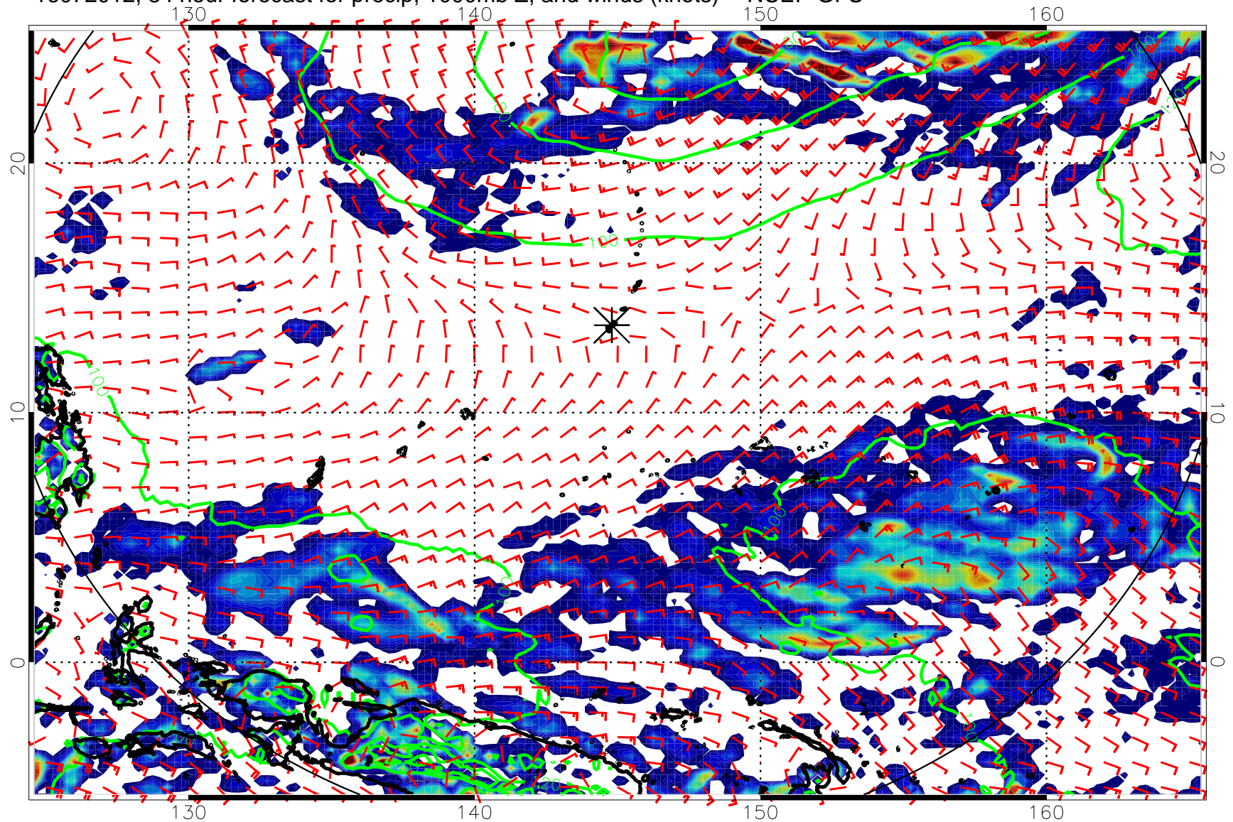
16072012, 84 hour forecast for precip, 1000mb Z, and winds (knots) -- NCEP GFS
