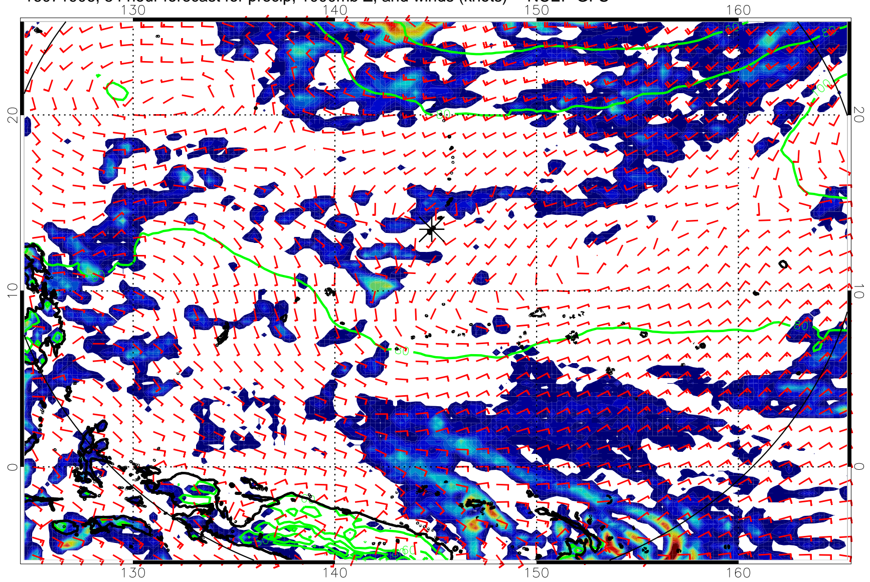
16071906, 54 hour forecast for precip, 1000mb Z, and winds (knots) -- NCEP GFS
