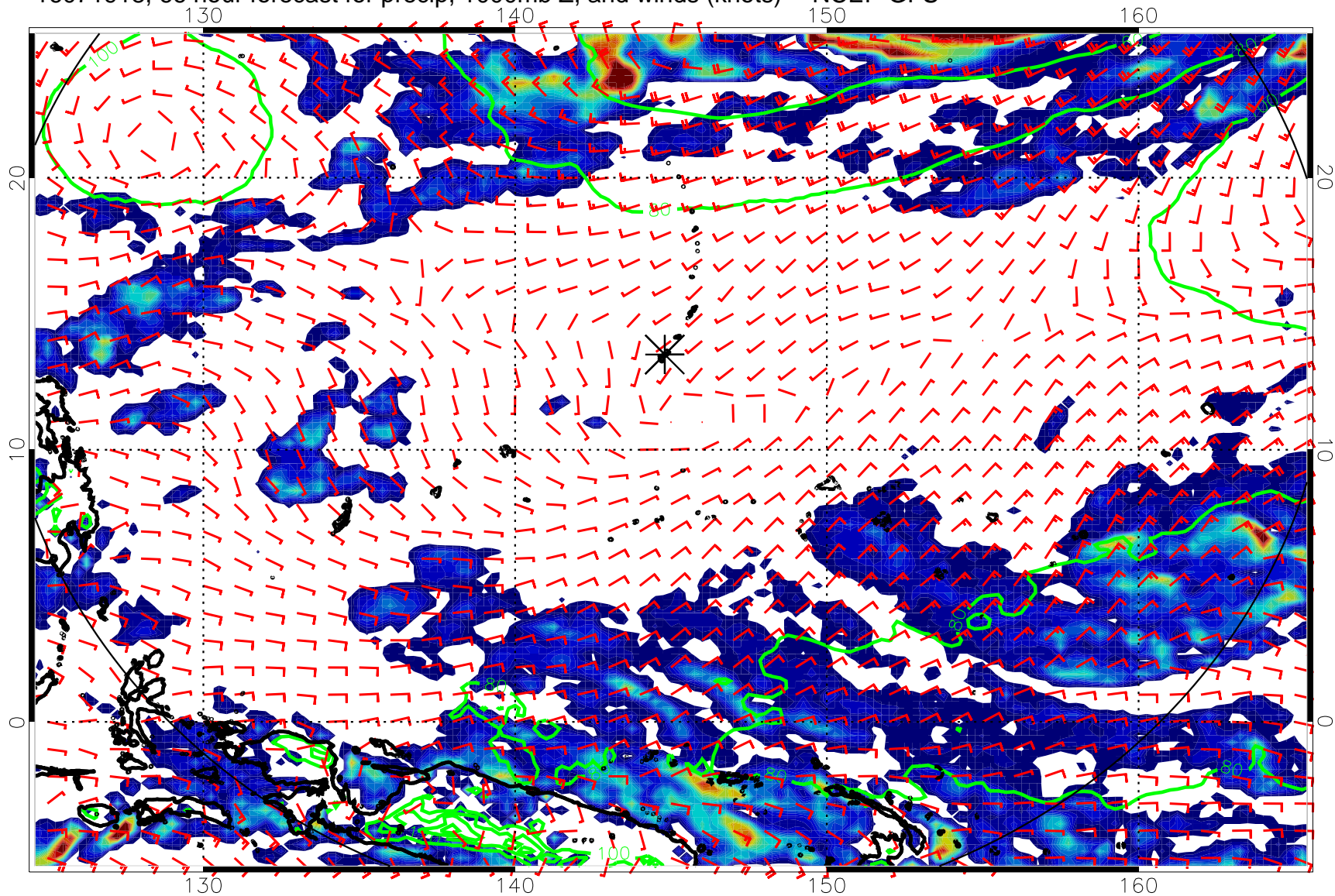
16071918, 66 hour forecast for precip, 1000mb Z, and winds (knots) -- NCEP GFS
