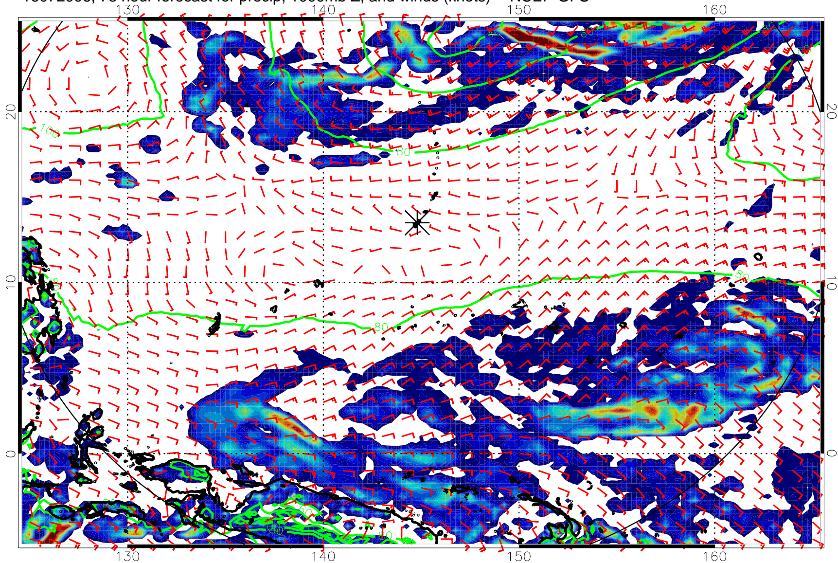
16072006, 78 hour forecast for precip, 1000mb Z, and winds (knots) -- NCEP GFS
