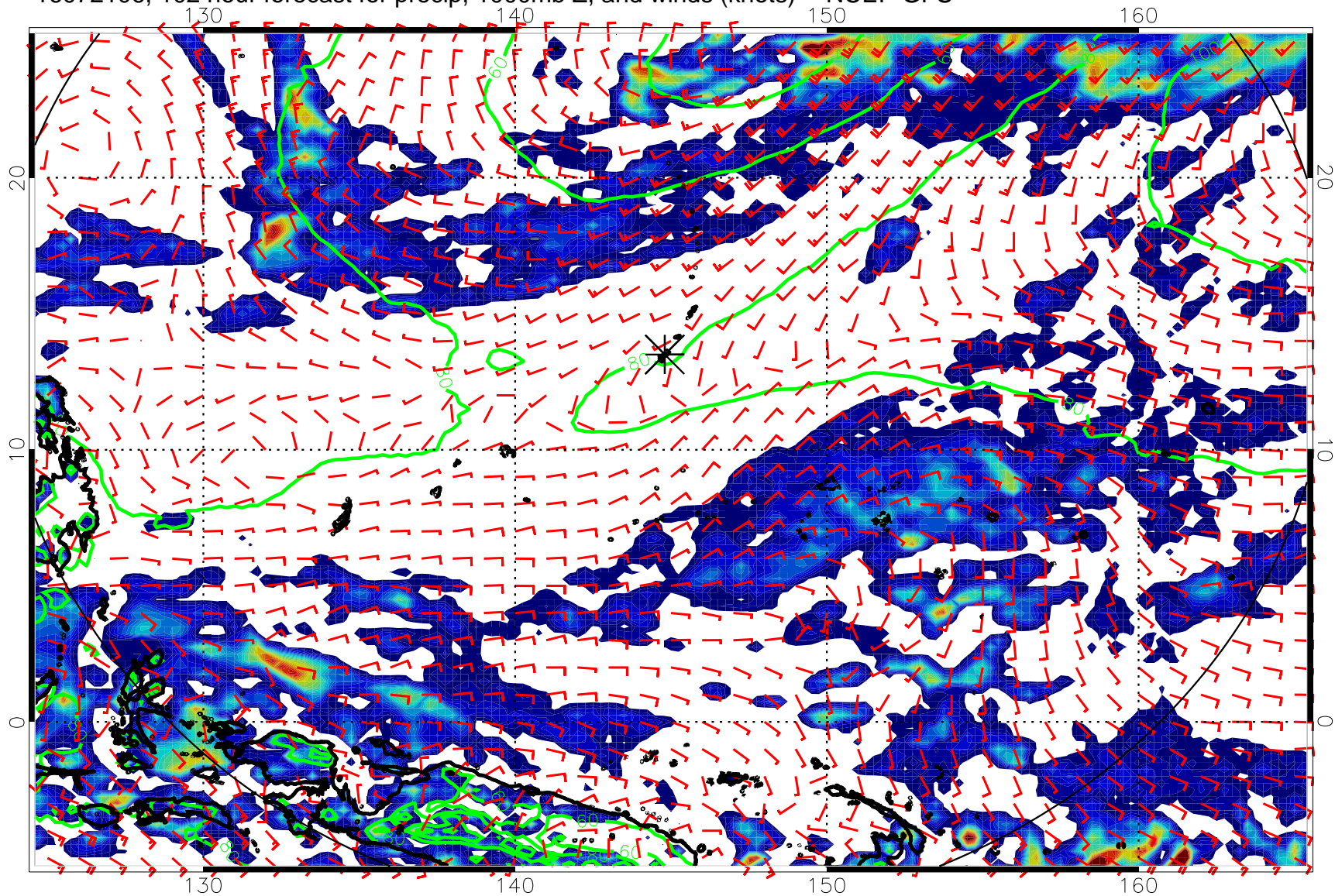
16072106, 102 hour forecast for precip, 1000mb Z, and winds (knots) -- NCEP GFS
