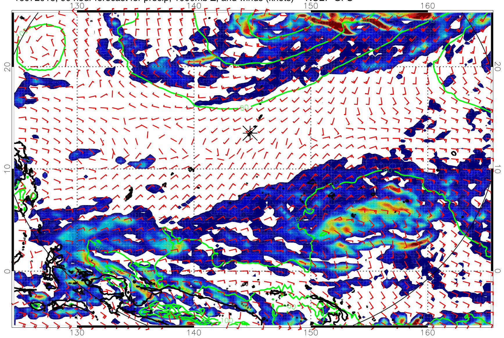
16072018, 90 hour forecast for precip, 1000mb Z, and winds (knots) -- NCEP GFS
