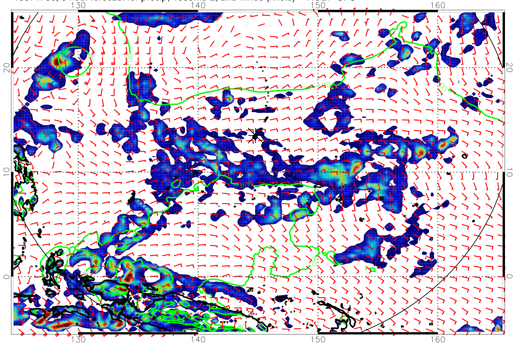
16071706, 6 hour forecast for precip, 1000mb Z, and winds (knots) -- NCEP GFS
