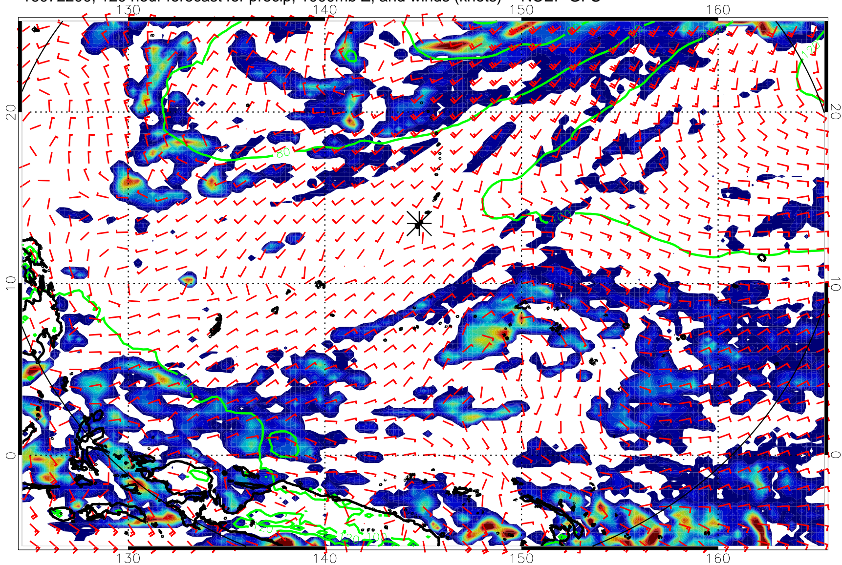
16072200, 120 hour forecast for precip, 1000mb Z, and winds (knots) -- NCEP GFS
