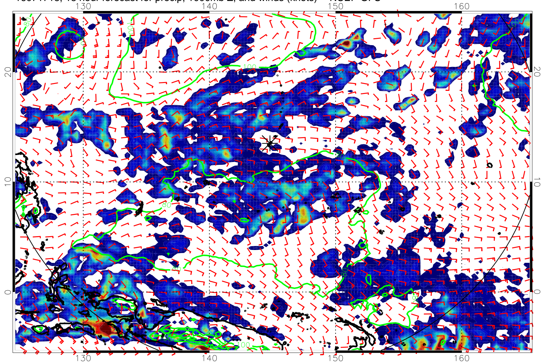
16071718, 18 hour forecast for precip, 1000mb Z, and winds (knots) -- NCEP GFS
