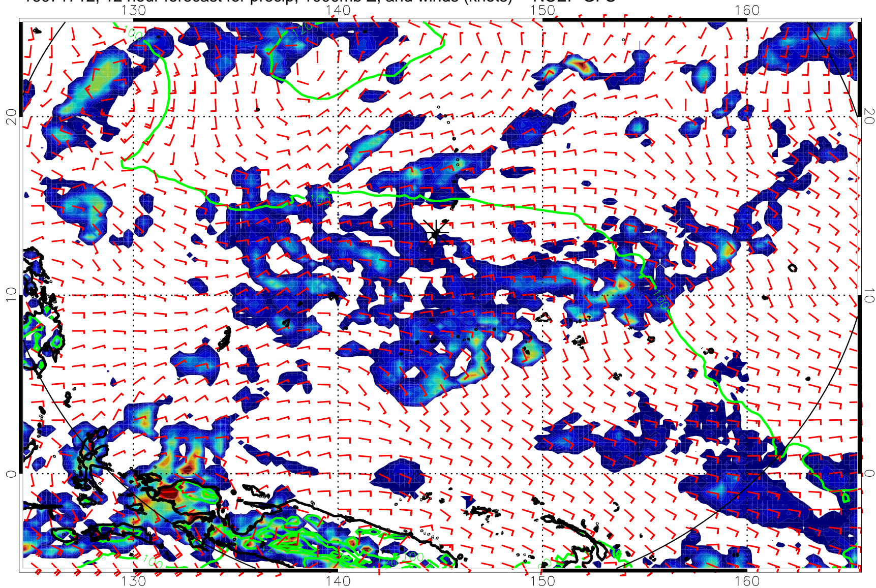
16071712, 12 hour forecast for precip, 1000mb Z, and winds (knots) -- NCEP GFS
