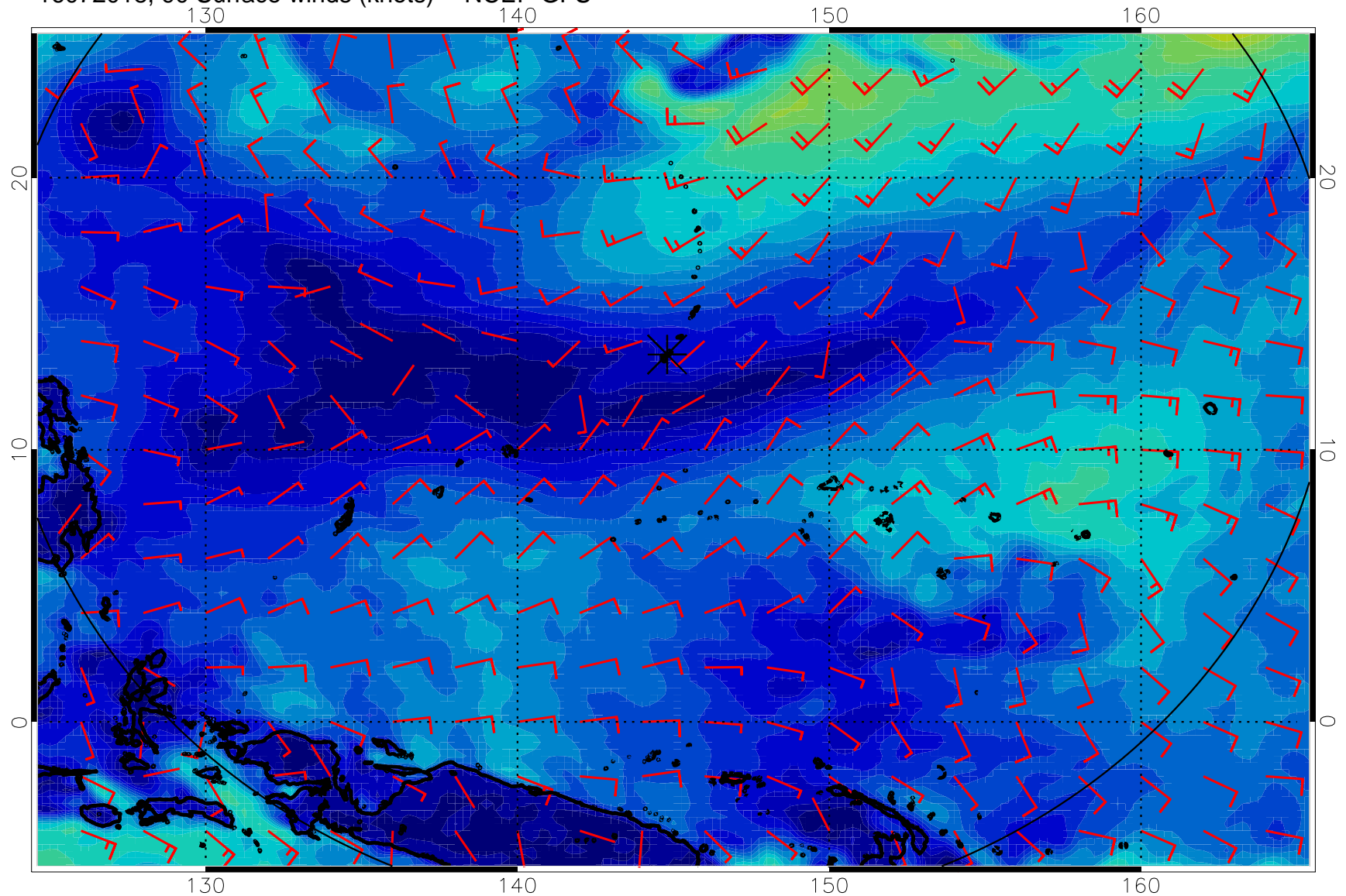
16072018, 90 Surface winds (knots) -- NCEP GFS
