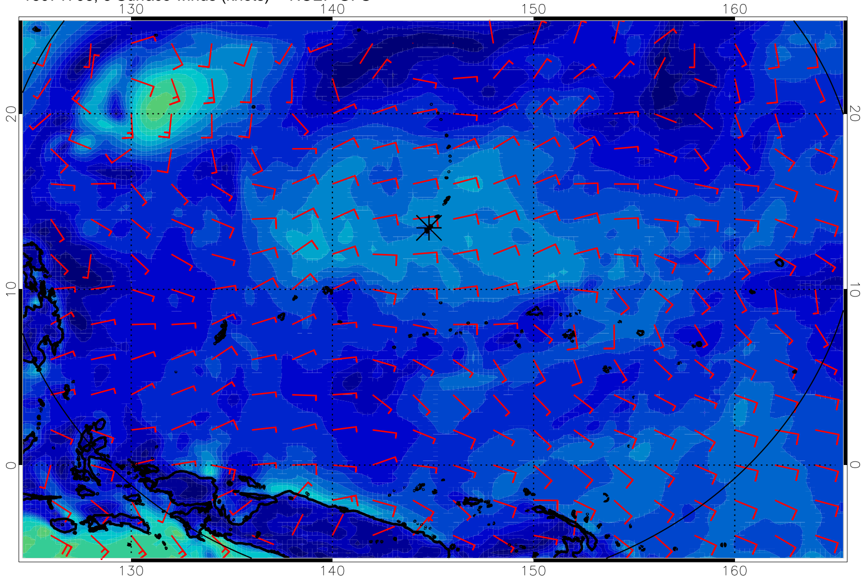
16071706, 6 Surface winds (knots) -- NCEP GFS
