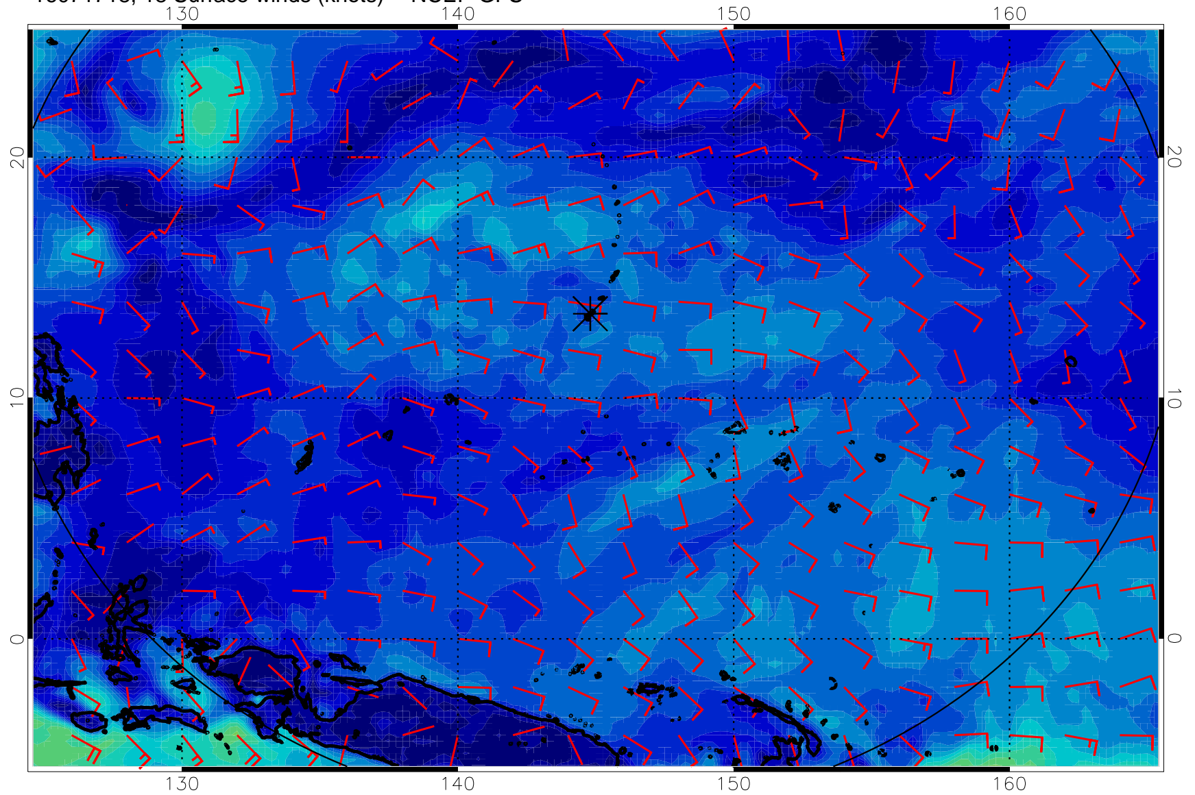
16071718, 18 Surface winds (knots) -- NCEP GFS
