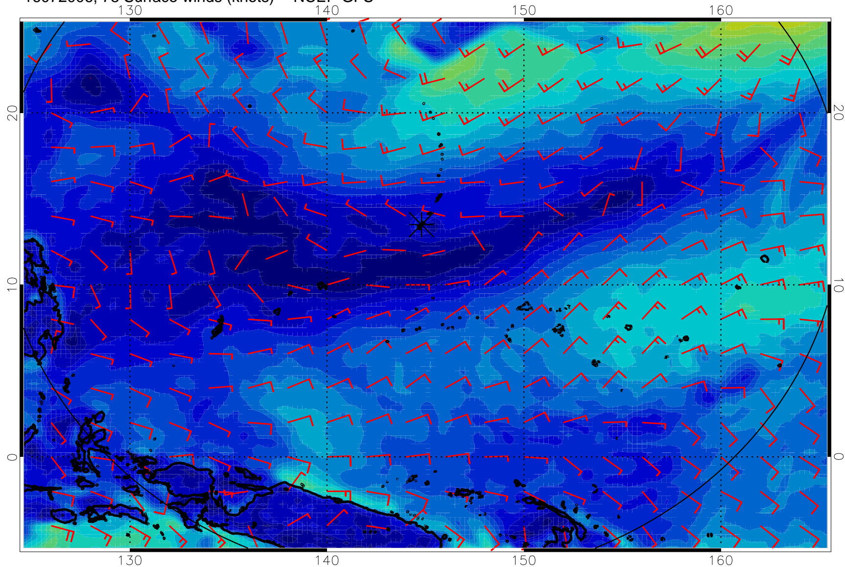
16072006, 78 Surface winds (knots) -- NCEP GFS
