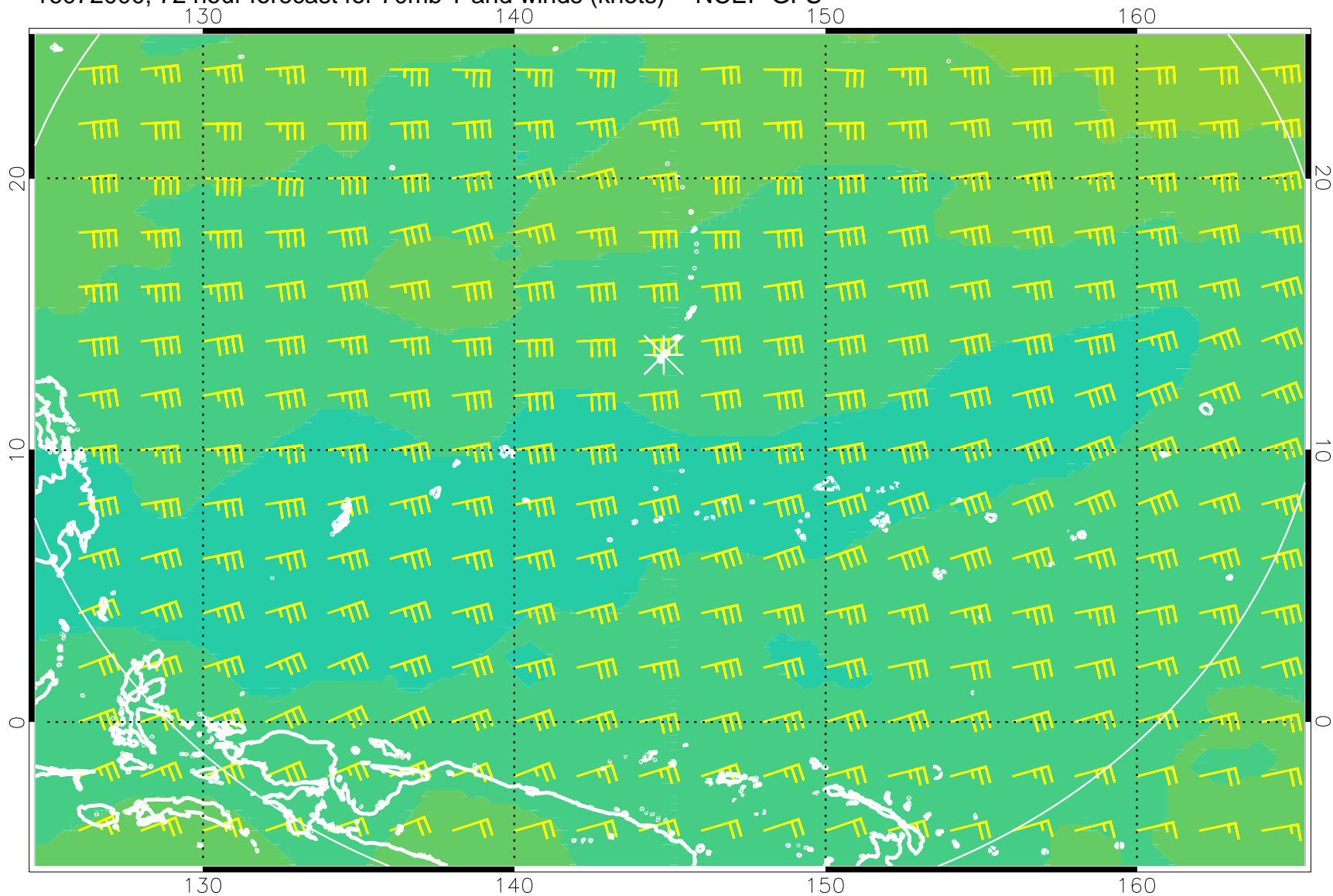
16072000, 72 hour forecast for 70mb T and winds (knots) -- NCEP GFS
