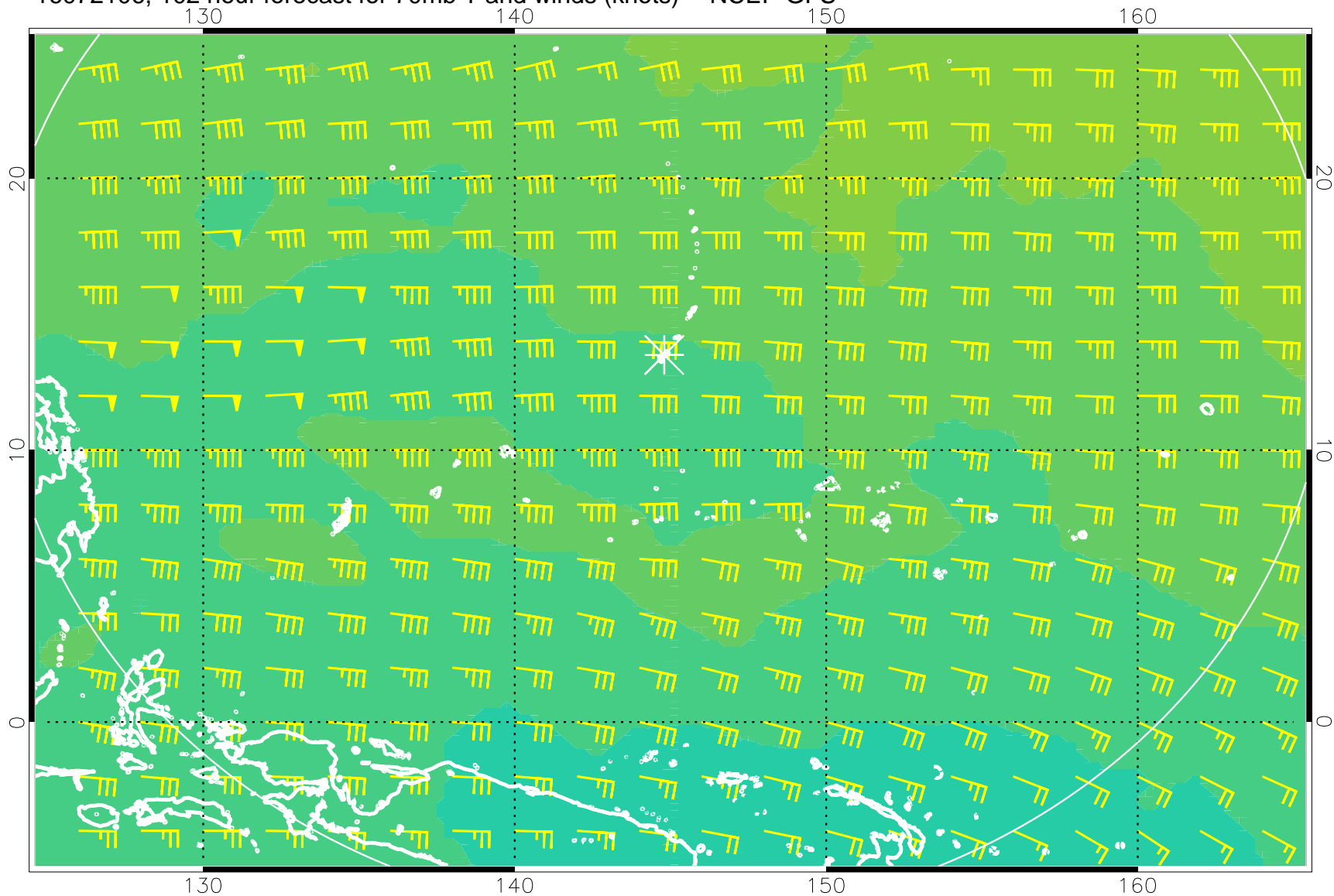
16072106, 102 hour forecast for 70mb T and winds (knots) -- NCEP GFS
