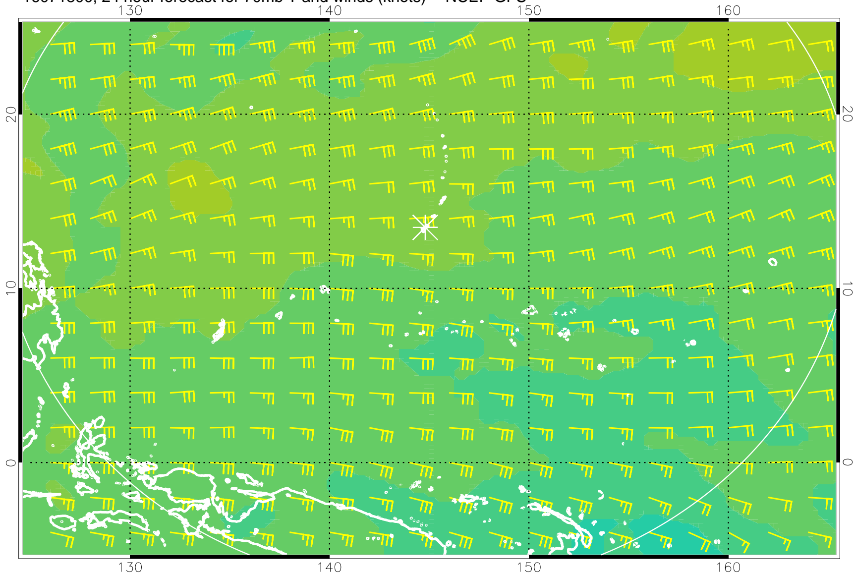
16071800, 24 hour forecast for 70mb T and winds (knots) -- NCEP GFS
