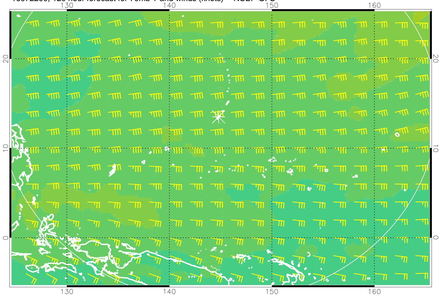
16072200, 120 hour forecast for 70mb T and winds (knots) -- NCEP GFS
