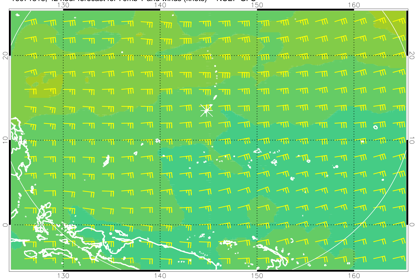
16071818, 42 hour forecast for 70mb T and winds (knots) -- NCEP GFS
