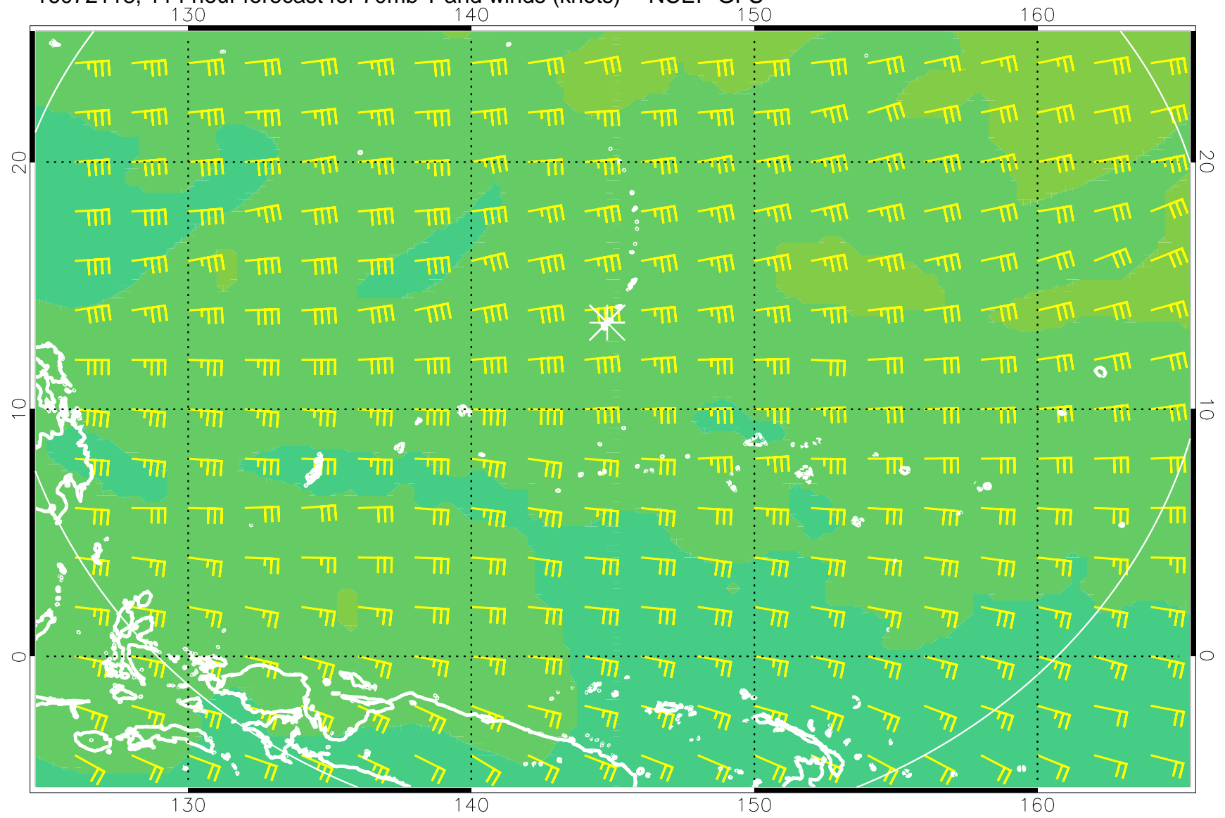
16072118, 114 hour forecast for 70mb T and winds (knots) -- NCEP GFS
