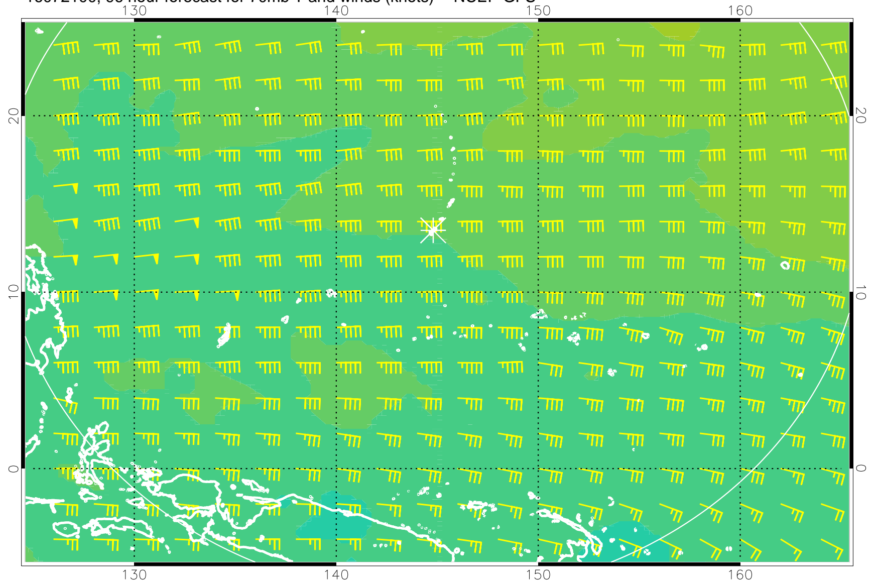
16072100, 96 hour forecast for 70mb T and winds (knots) -- NCEP GFS
