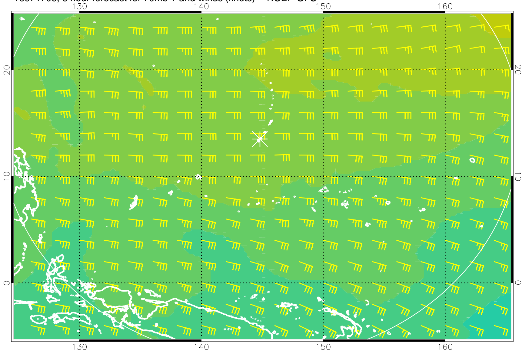
16071706, 6 hour forecast for 70mb T and winds (knots) -- NCEP GFS
