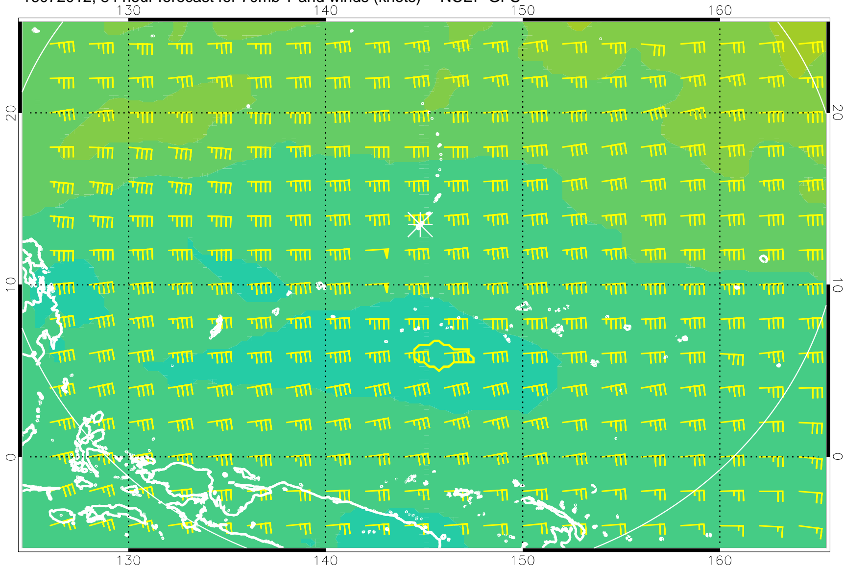
16072012, 84 hour forecast for 70mb T and winds (knots) -- NCEP GFS
