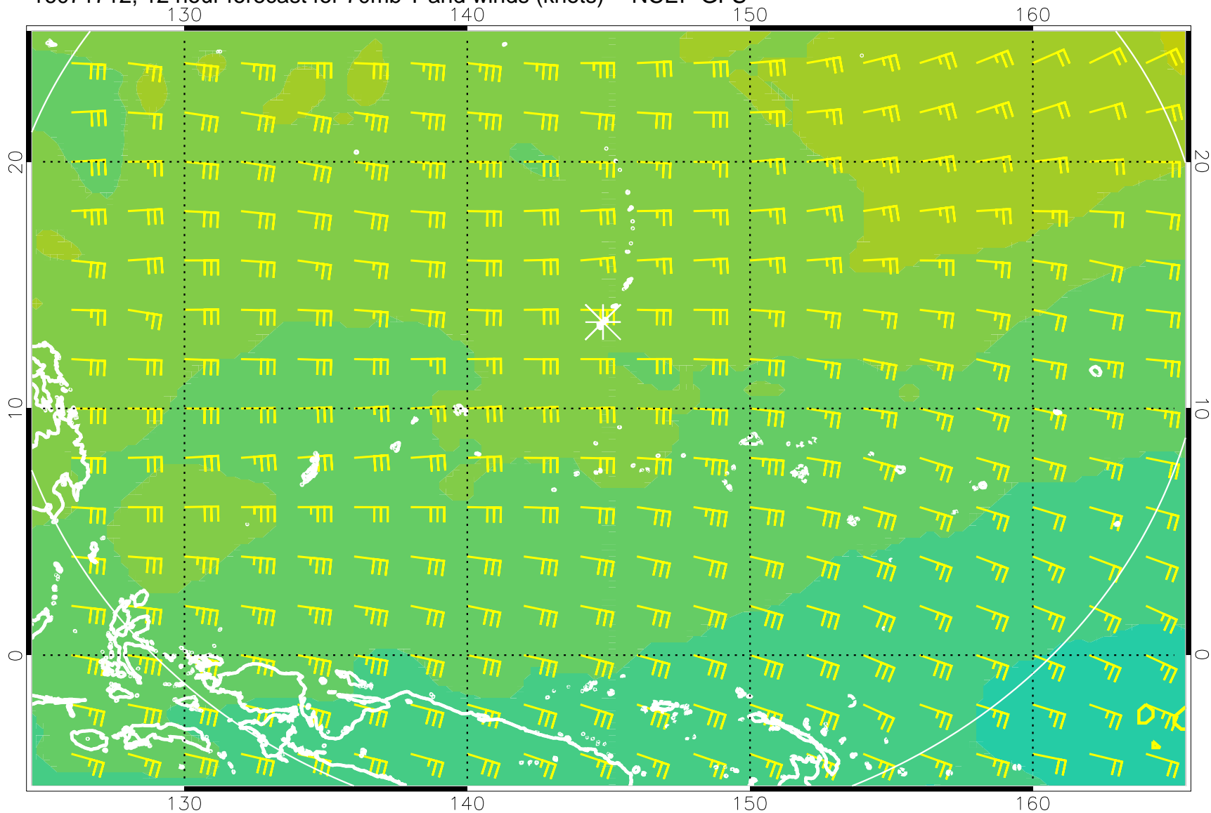
16071712, 12 hour forecast for 70mb T and winds (knots) -- NCEP GFS
