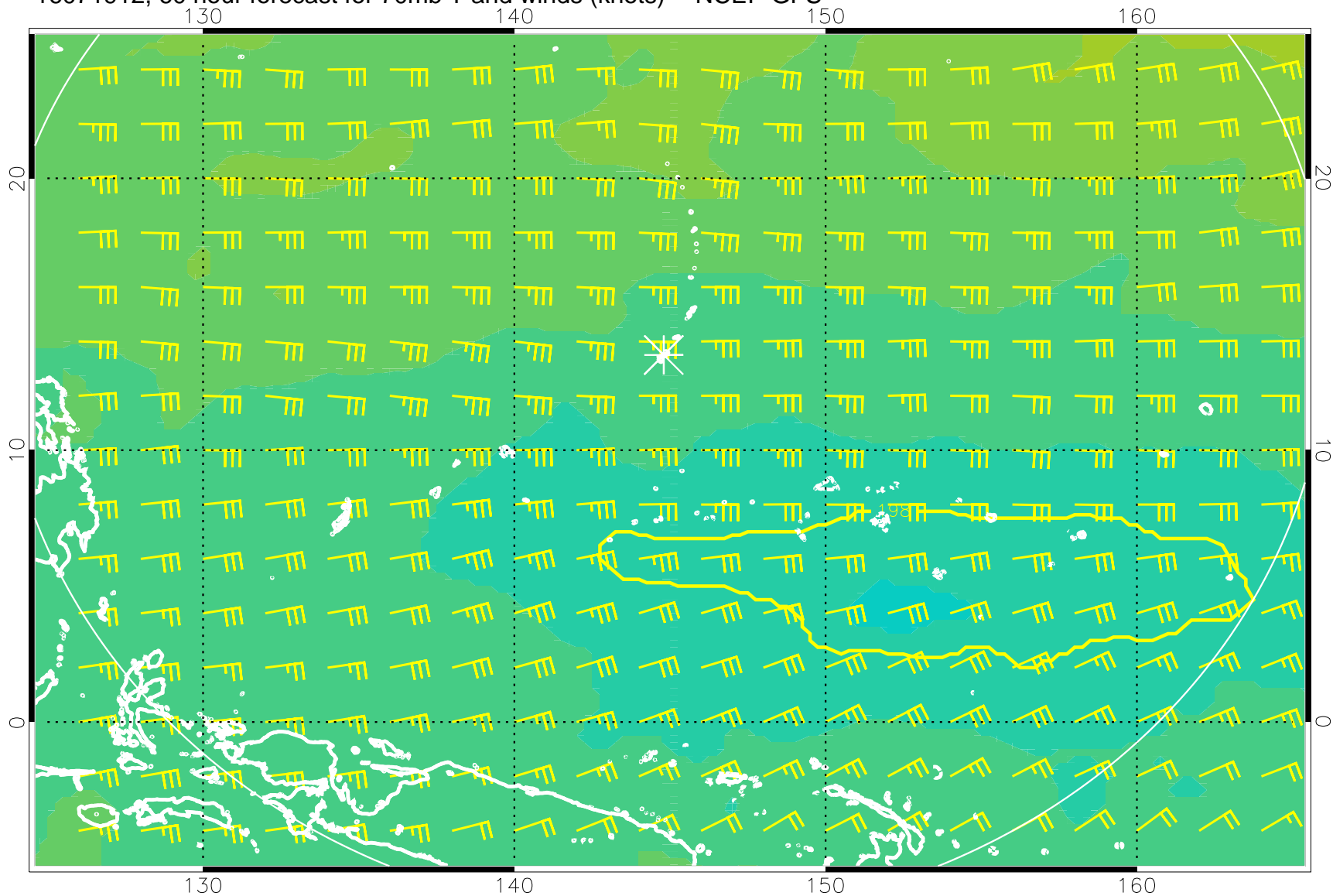
16071912, 60 hour forecast for 70mb T and winds (knots) -- NCEP GFS
