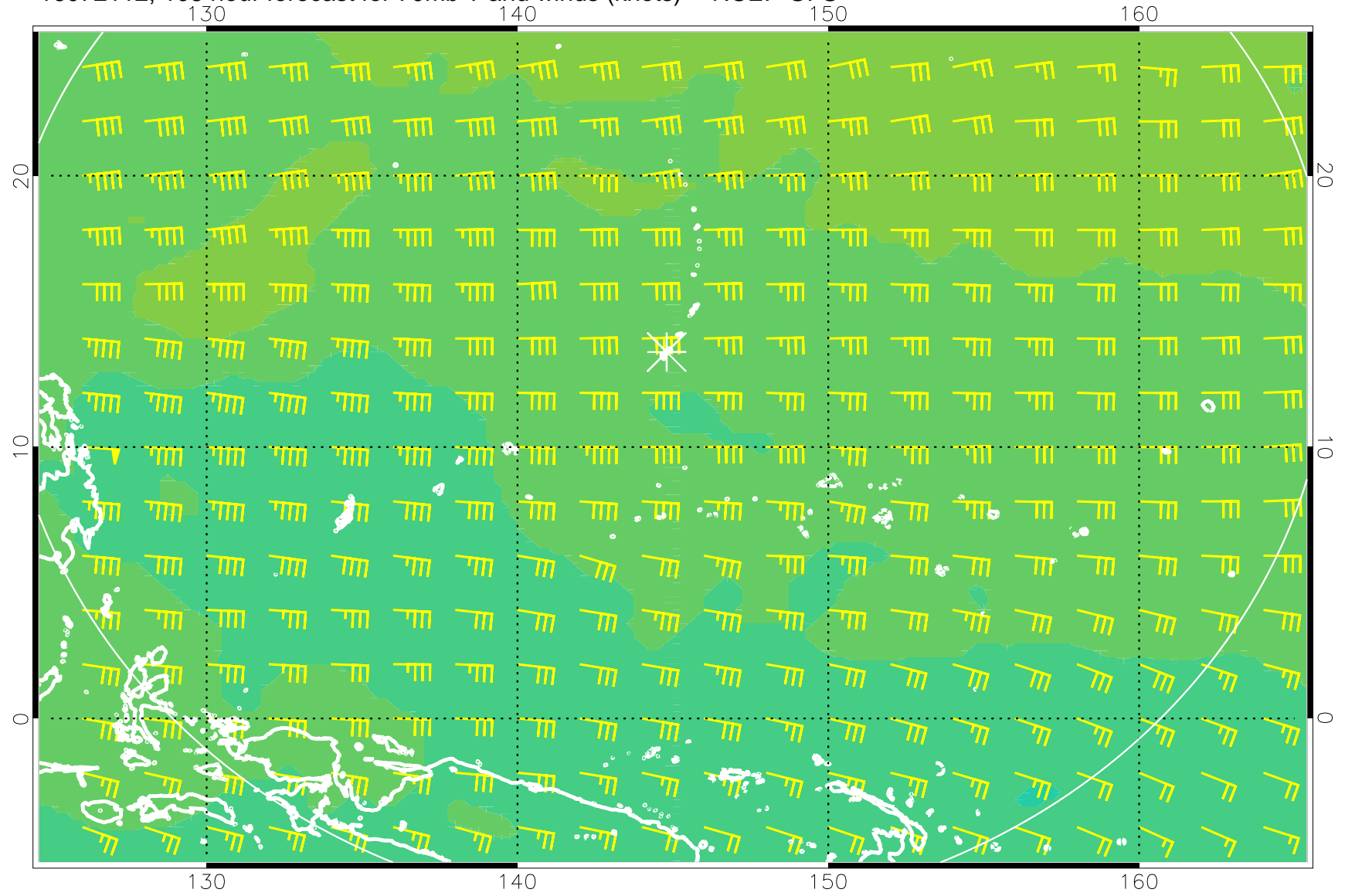
16072112, 108 hour forecast for 70mb T and winds (knots) -- NCEP GFS
