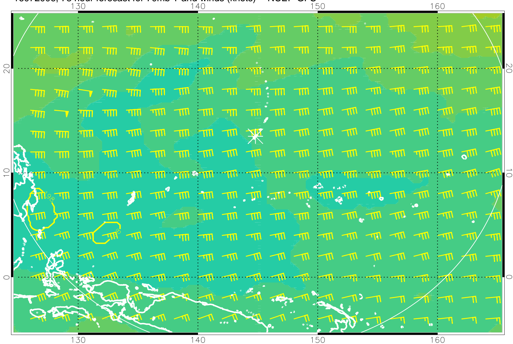
16072006, 78 hour forecast for 70mb T and winds (knots) -- NCEP GFS
