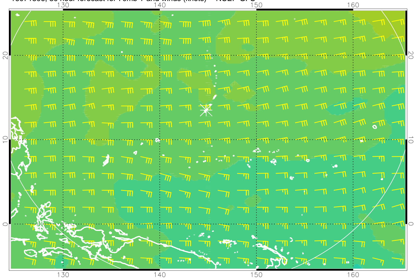
16071806, 30 hour forecast for 70mb T and winds (knots) -- NCEP GFS
