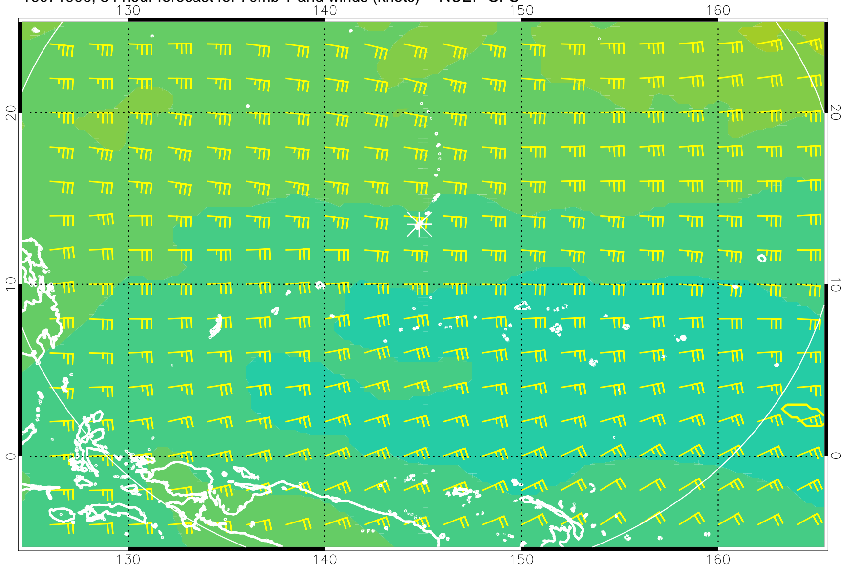
16071906, 54 hour forecast for 70mb T and winds (knots) -- NCEP GFS
