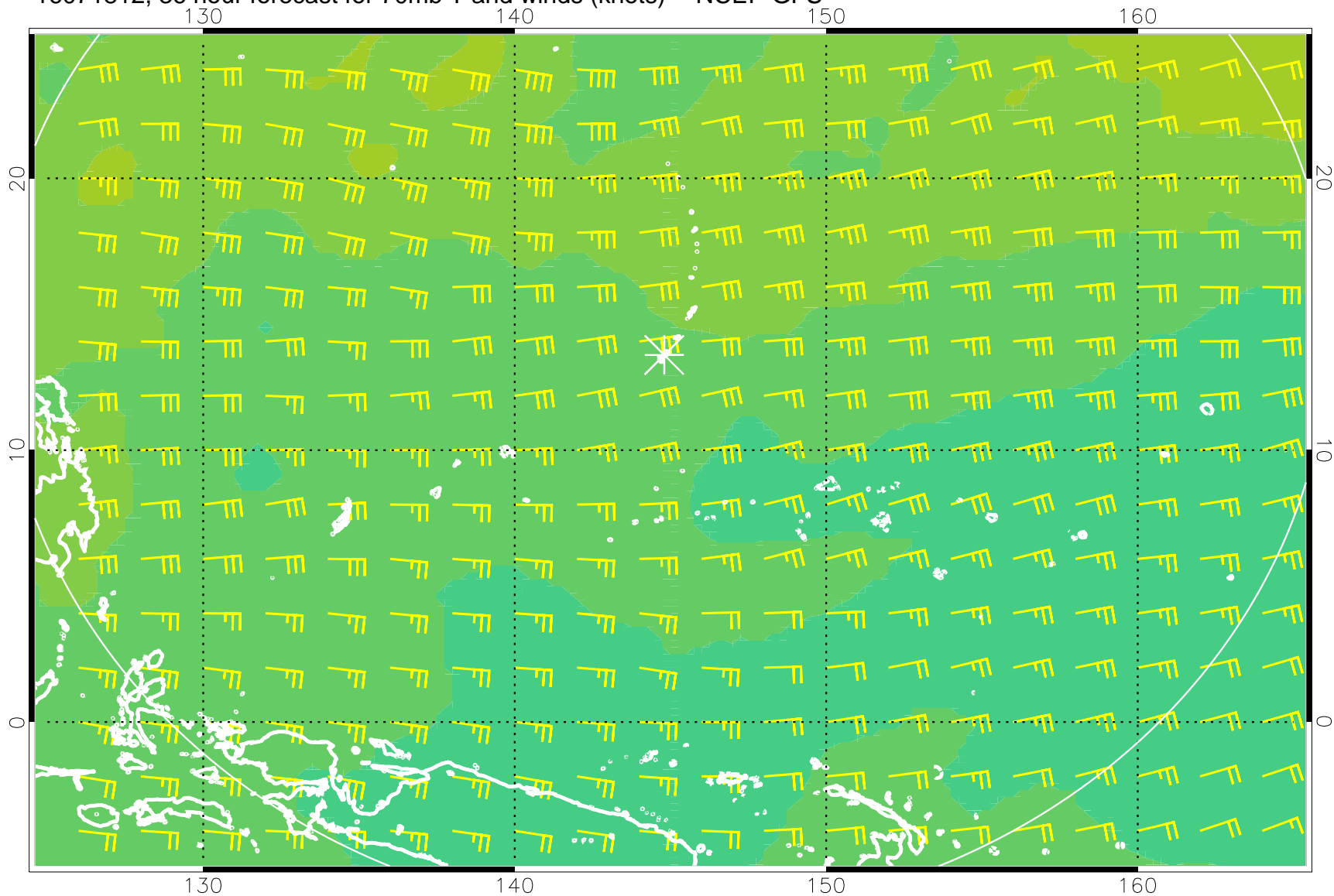
16071812, 36 hour forecast for 70mb T and winds (knots) -- NCEP GFS
