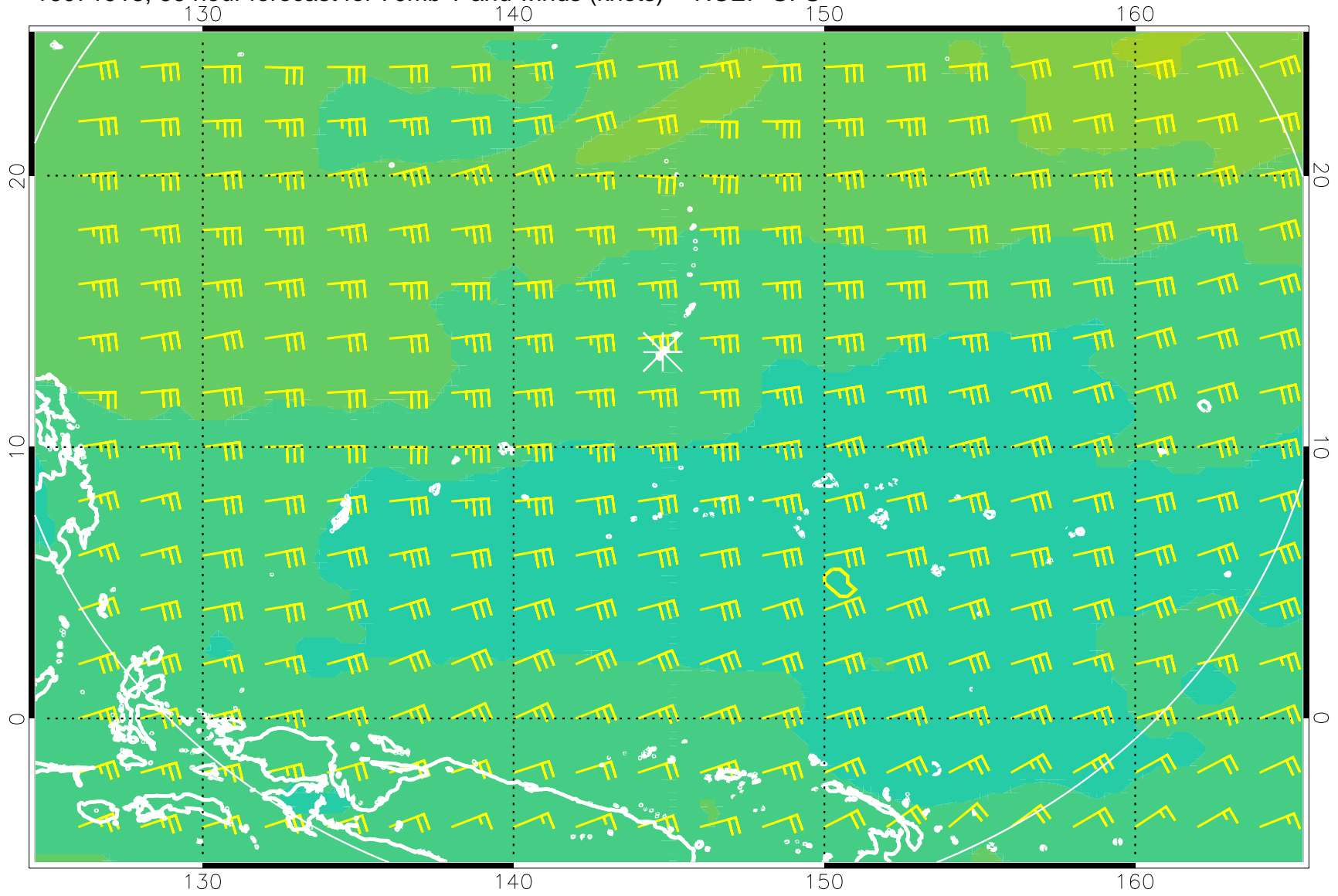
16071918, 66 hour forecast for 70mb T and winds (knots) -- NCEP GFS
