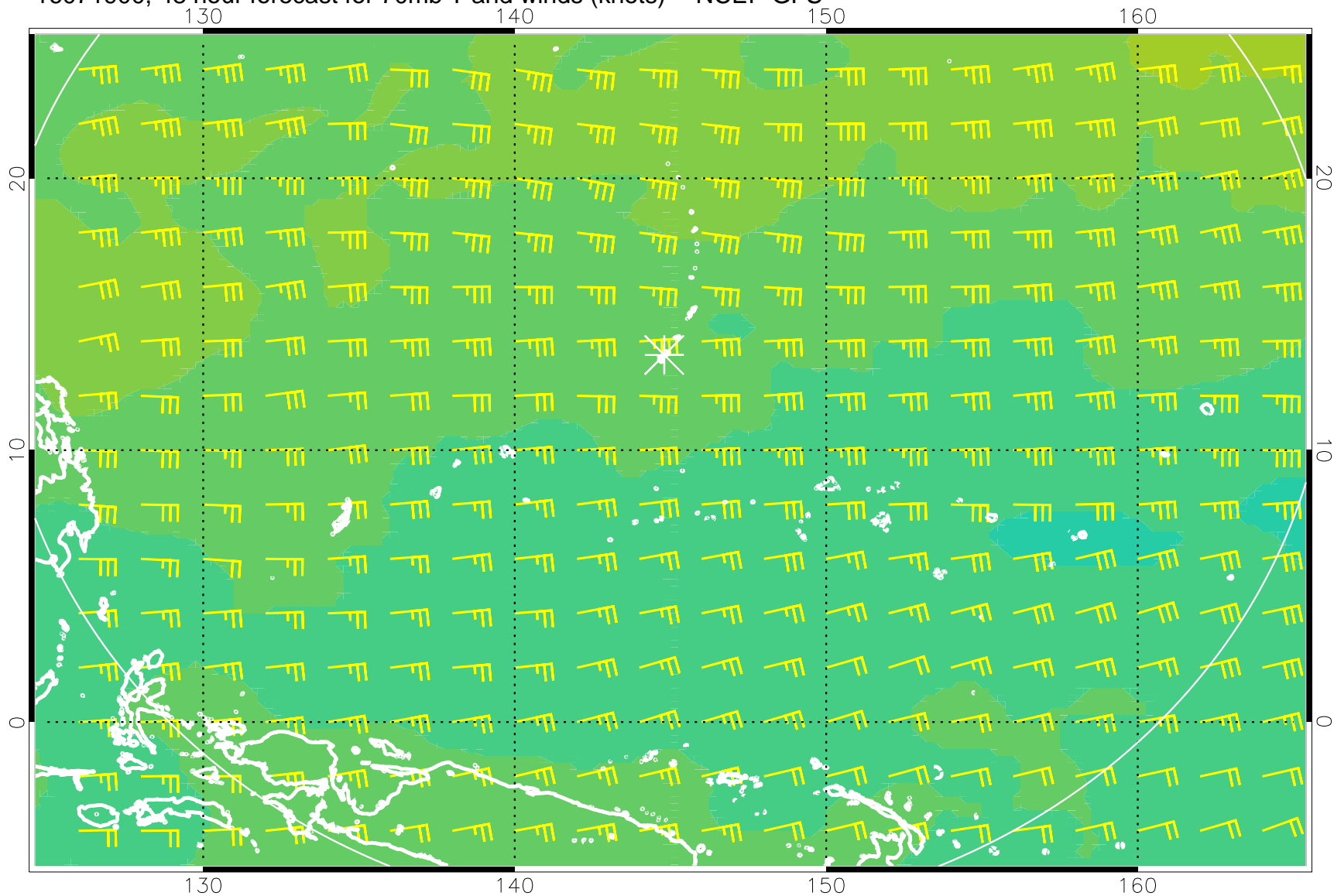
16071900, 48 hour forecast for 70mb T and winds (knots) -- NCEP GFS
