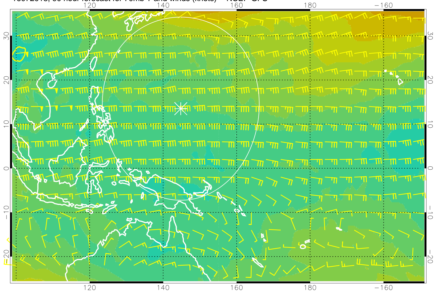
16072018, 90 hour forecast for 70mb T and winds (knots) -- NCEP GFS
