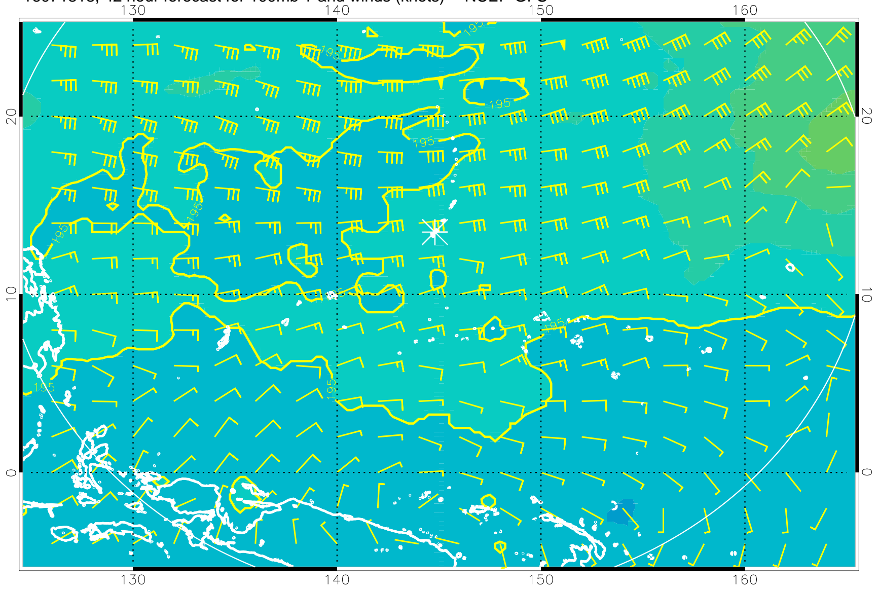
16071818, 42 hour forecast for 100mb T and winds (knots) -- NCEP GFS
