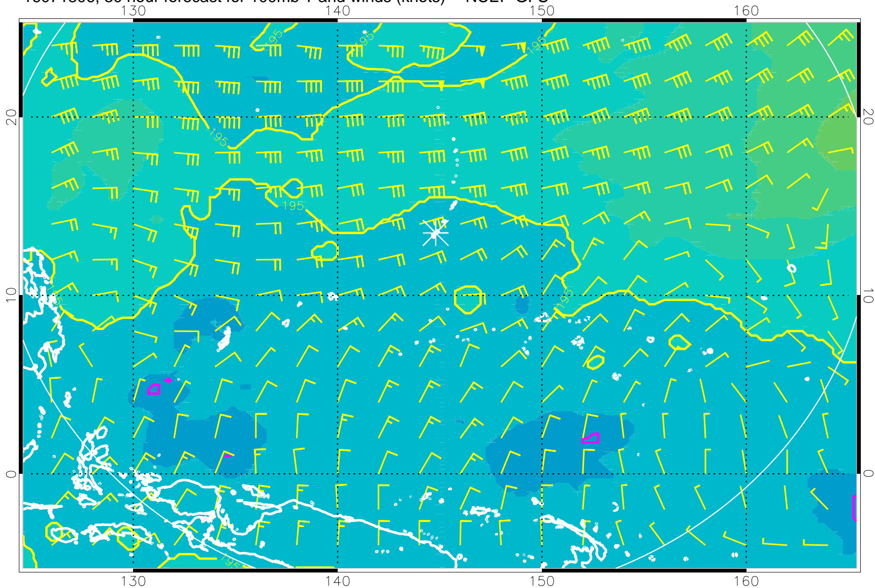
16071806, 30 hour forecast for 100mb T and winds (knots) -- NCEP GFS
