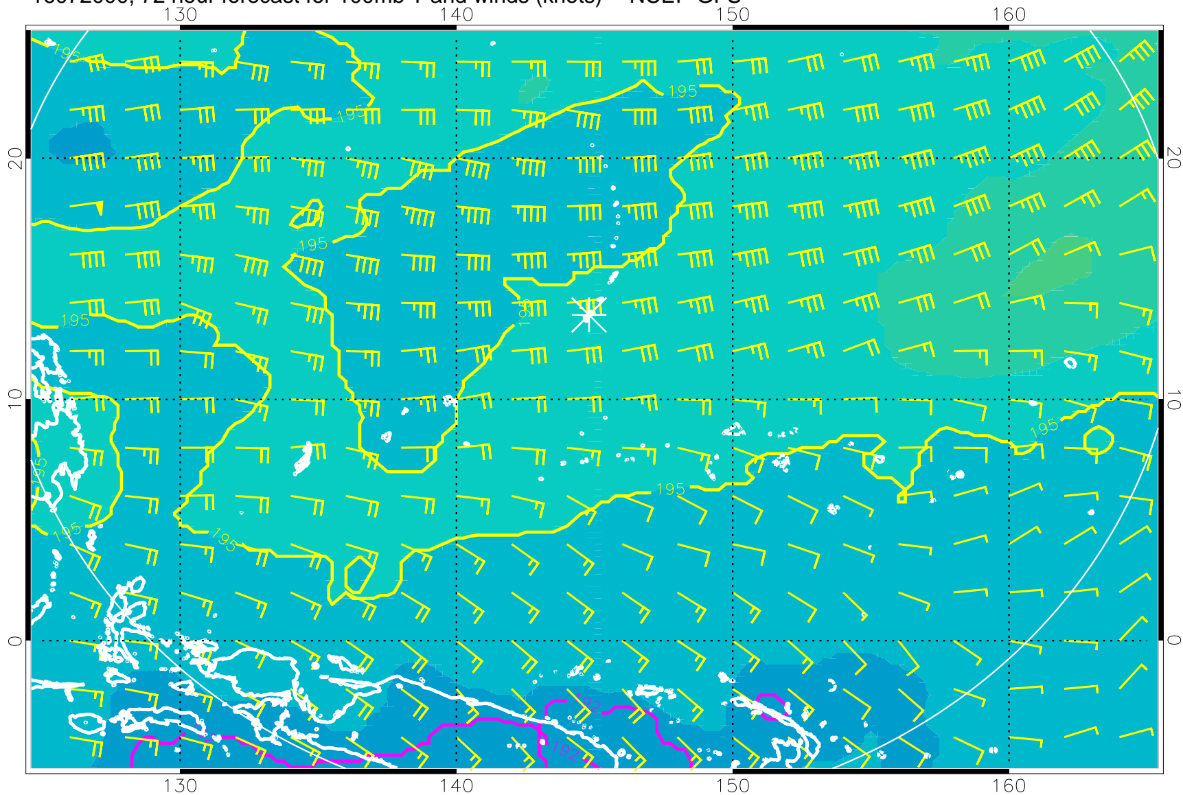
16072000, 72 hour forecast for 100mb T and winds (knots) -- NCEP GFS
