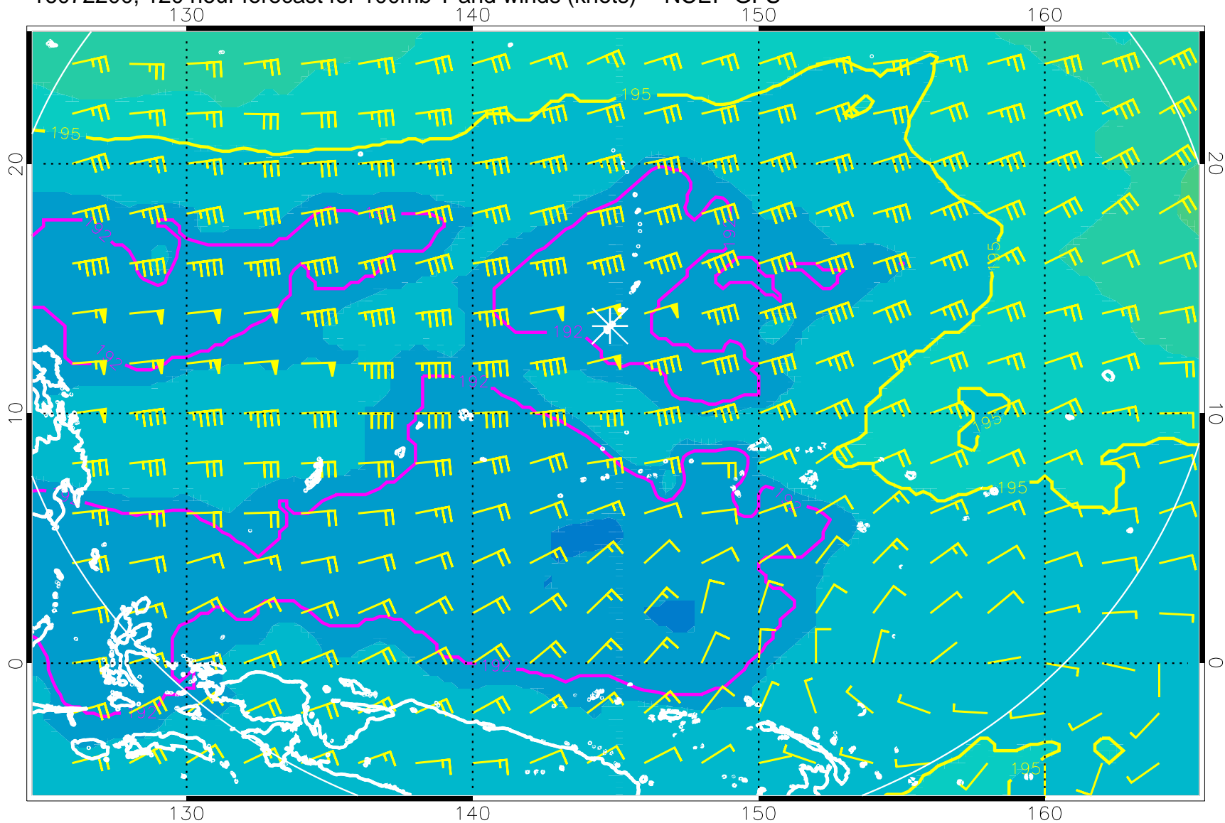
16072200, 120 hour forecast for 100mb T and winds (knots) -- NCEP GFS
