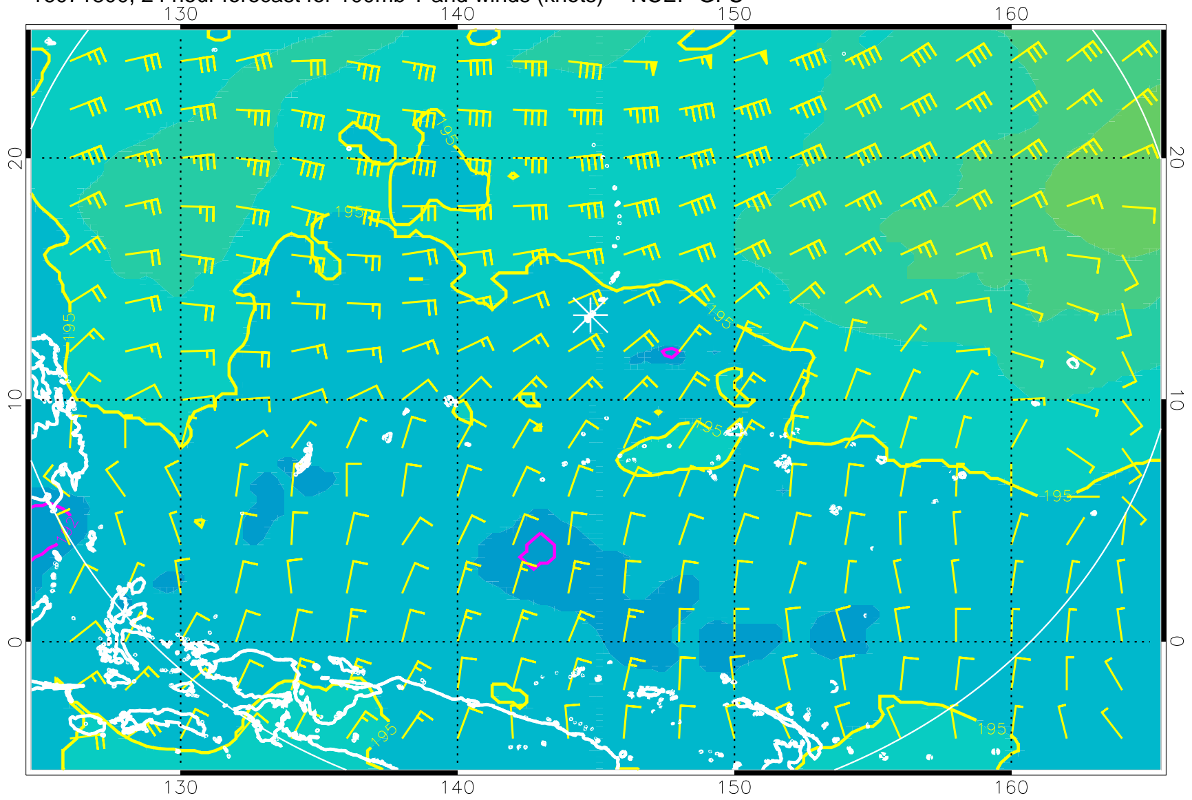
16071800, 24 hour forecast for 100mb T and winds (knots) -- NCEP GFS
