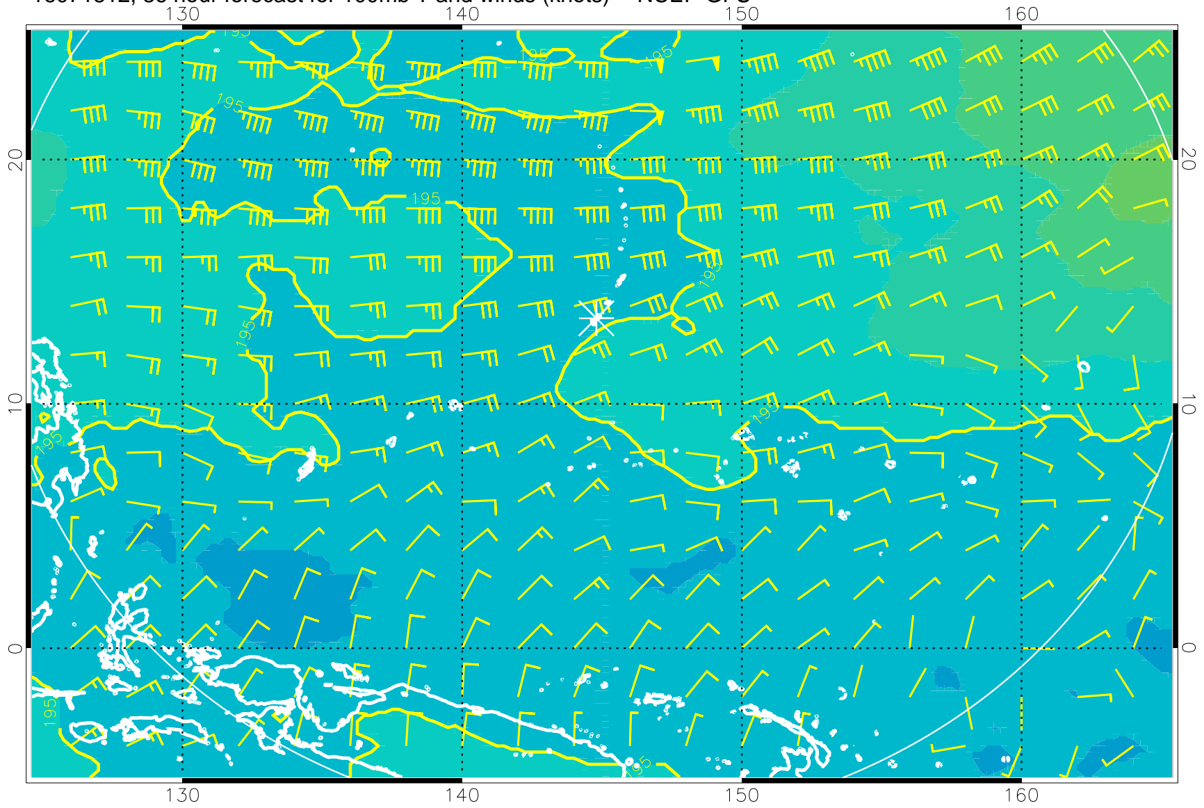
16071812, 36 hour forecast for 100mb T and winds (knots) -- NCEP GFS
