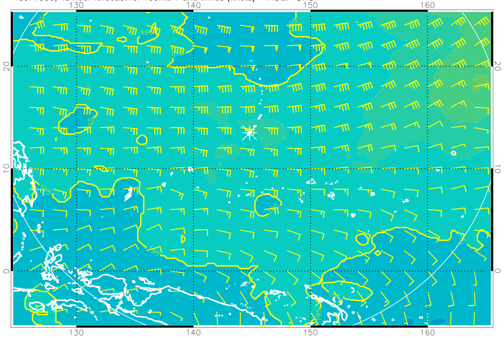
16071900, 48 hour forecast for 100mb T and winds (knots) -- NCEP GFS
