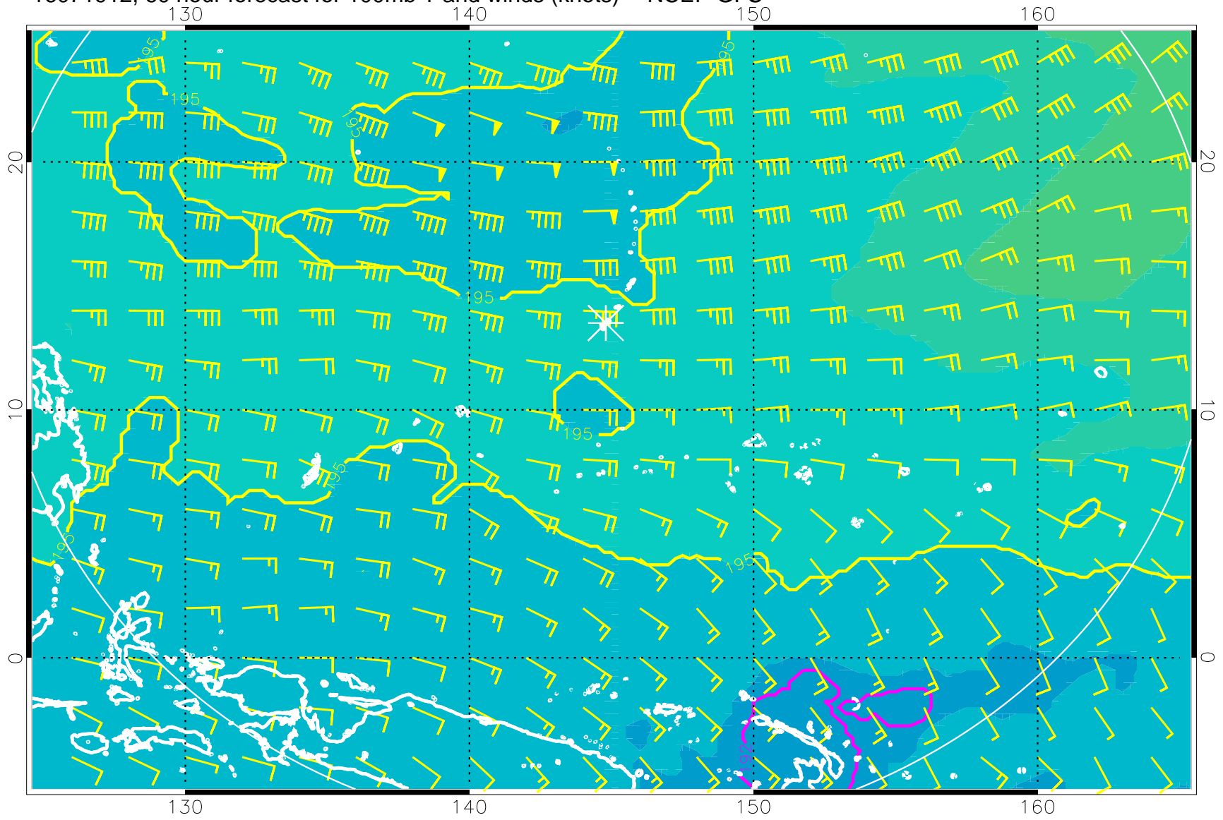
16071912, 60 hour forecast for 100mb T and winds (knots) -- NCEP GFS
