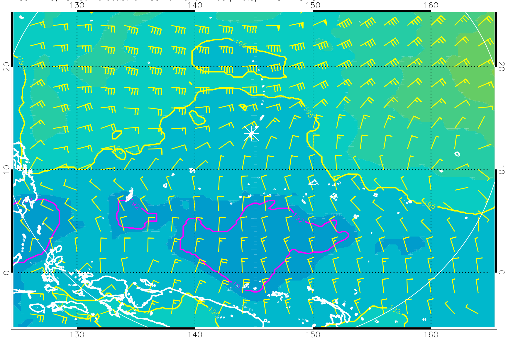
16071718, 18 hour forecast for 100mb T and winds (knots) -- NCEP GFS
