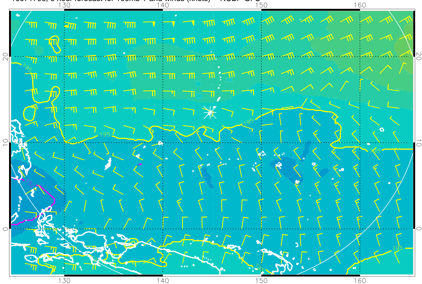
16071706, 6 hour forecast for 100mb T and winds (knots) -- NCEP GFS
