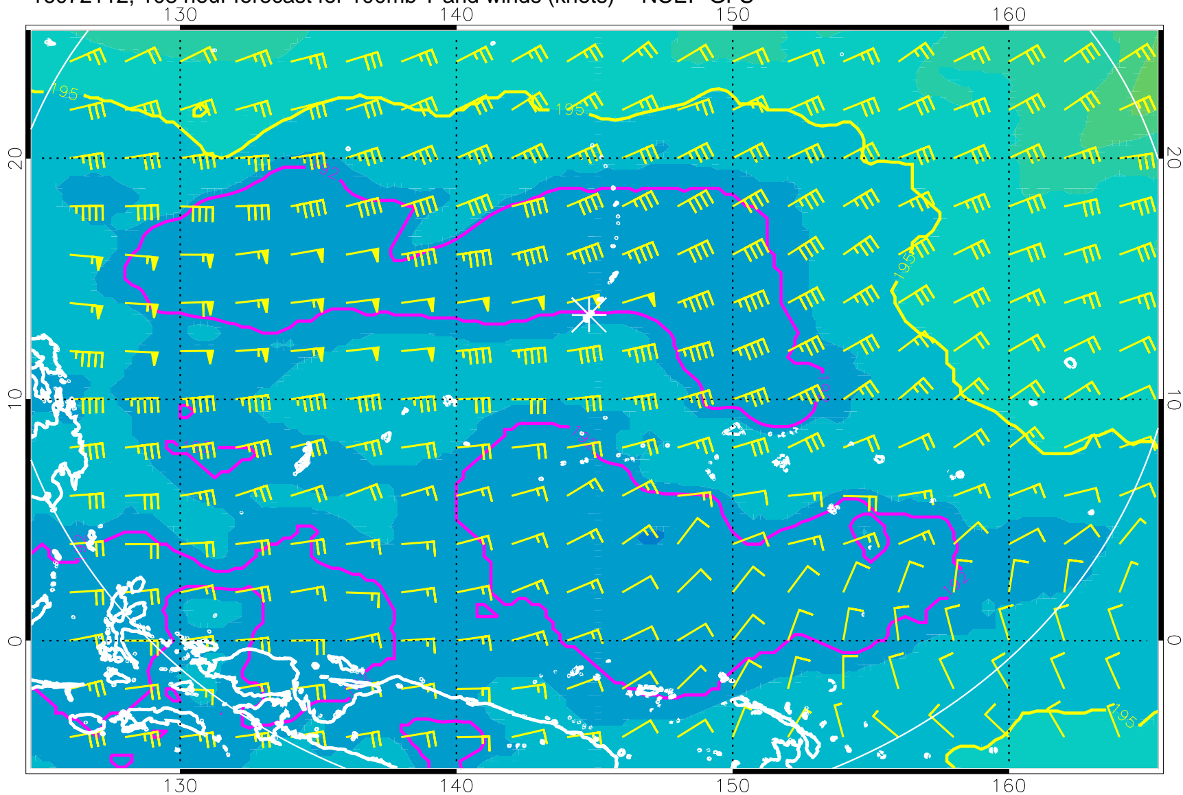
16072112, 108 hour forecast for 100mb T and winds (knots) -- NCEP GFS
