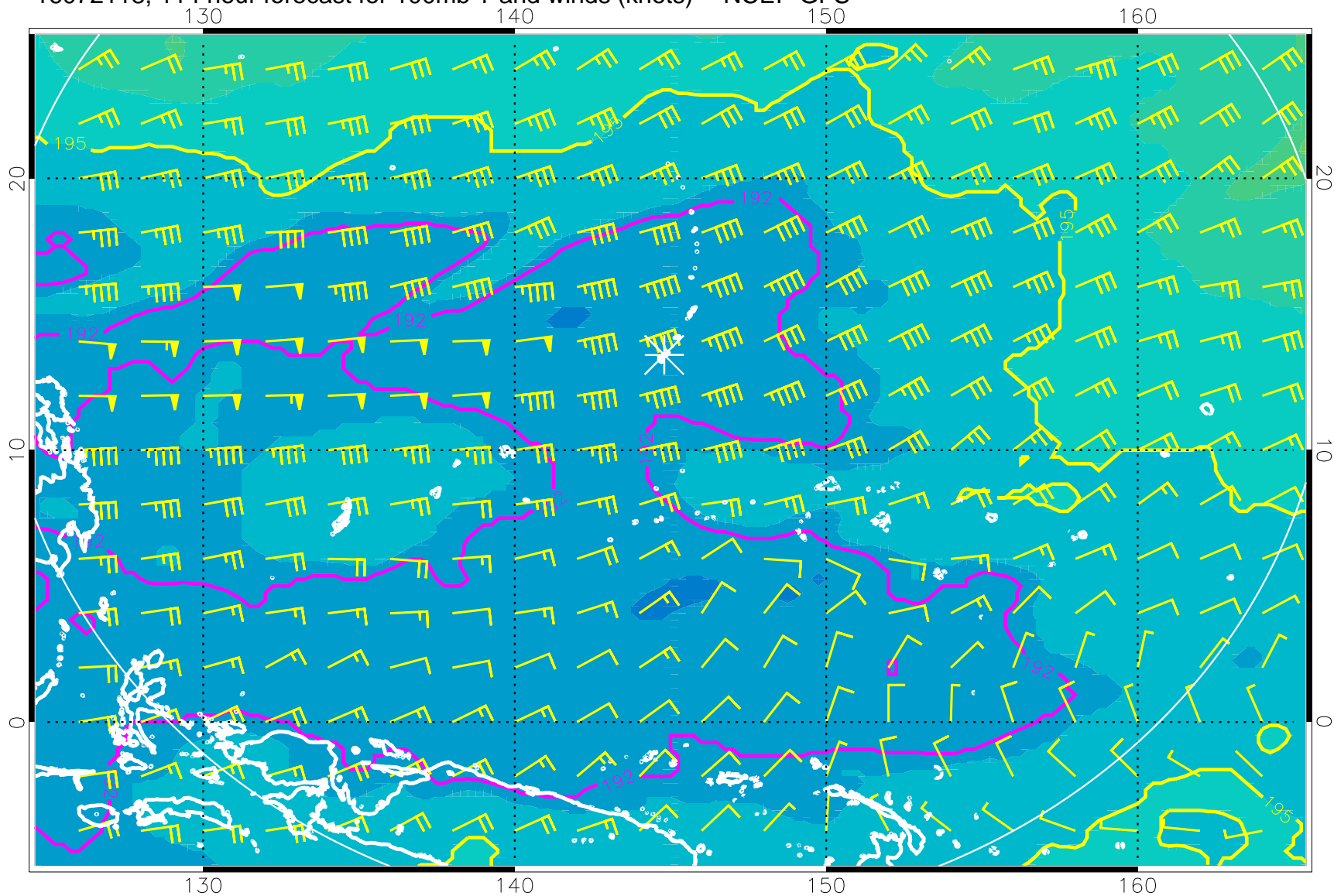
16072118, 114 hour forecast for 100mb T and winds (knots) -- NCEP GFS
