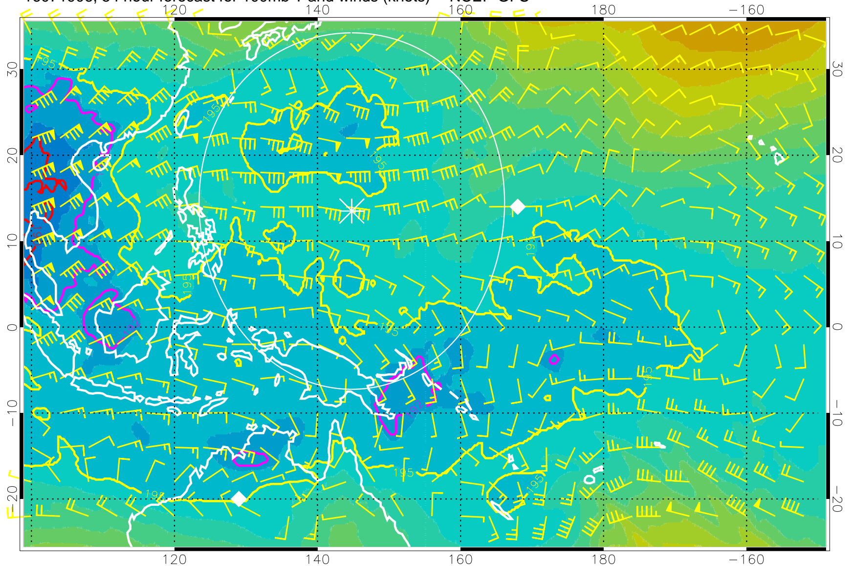
16071906, 54 hour forecast for 100mb T and winds (knots) -- NCEP GFS
