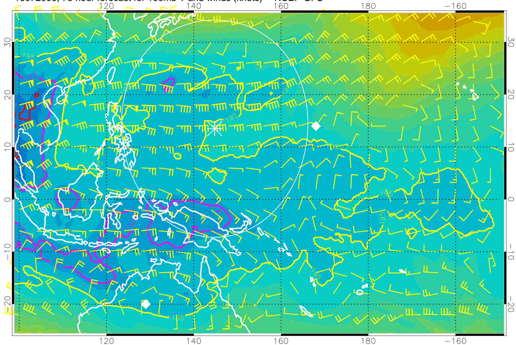
16072006, 78 hour forecast for 100mb T and winds (knots) -- NCEP GFS
