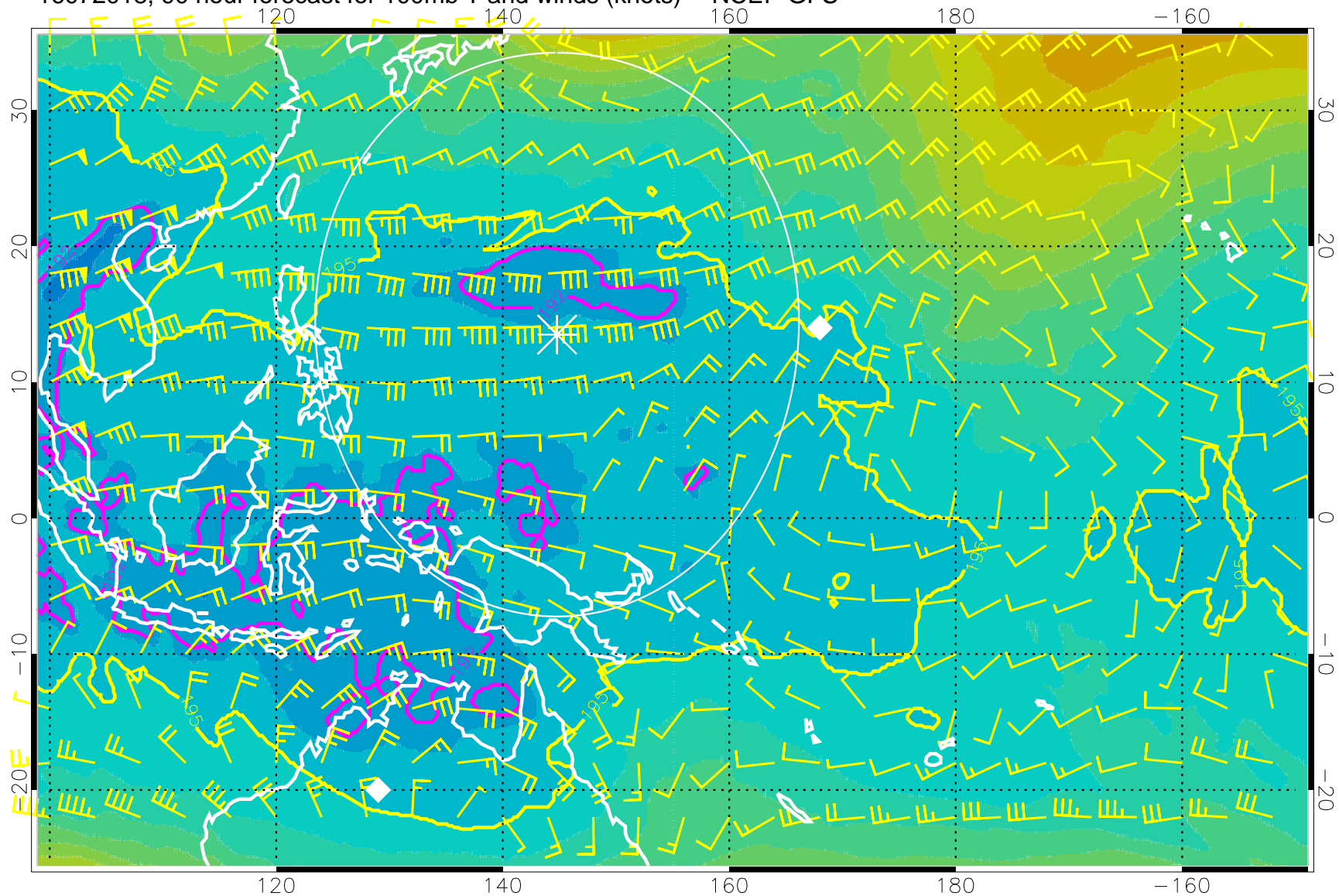
16072018, 90 hour forecast for 100mb T and winds (knots) -- NCEP GFS
