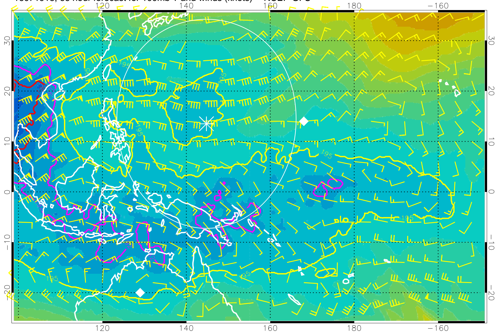
16071918, 66 hour forecast for 100mb T and winds (knots) -- NCEP GFS
