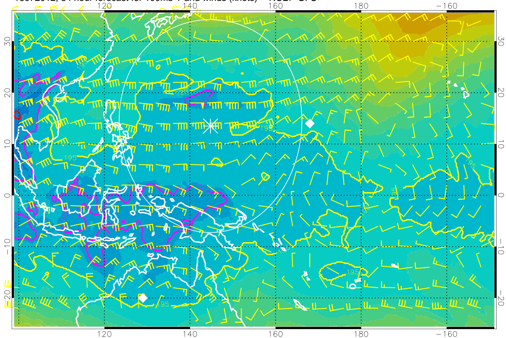
16072012, 84 hour forecast for 100mb T and winds (knots) -- NCEP GFS
