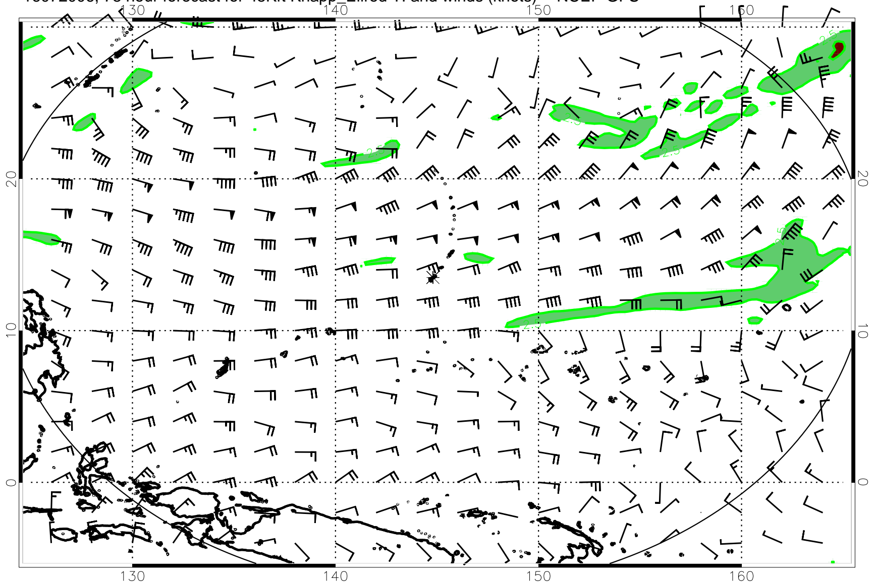
16072006, 78 hour forecast for 45Kft Knapp_Ellrod TI and winds (knots) -- NCEP GFS
