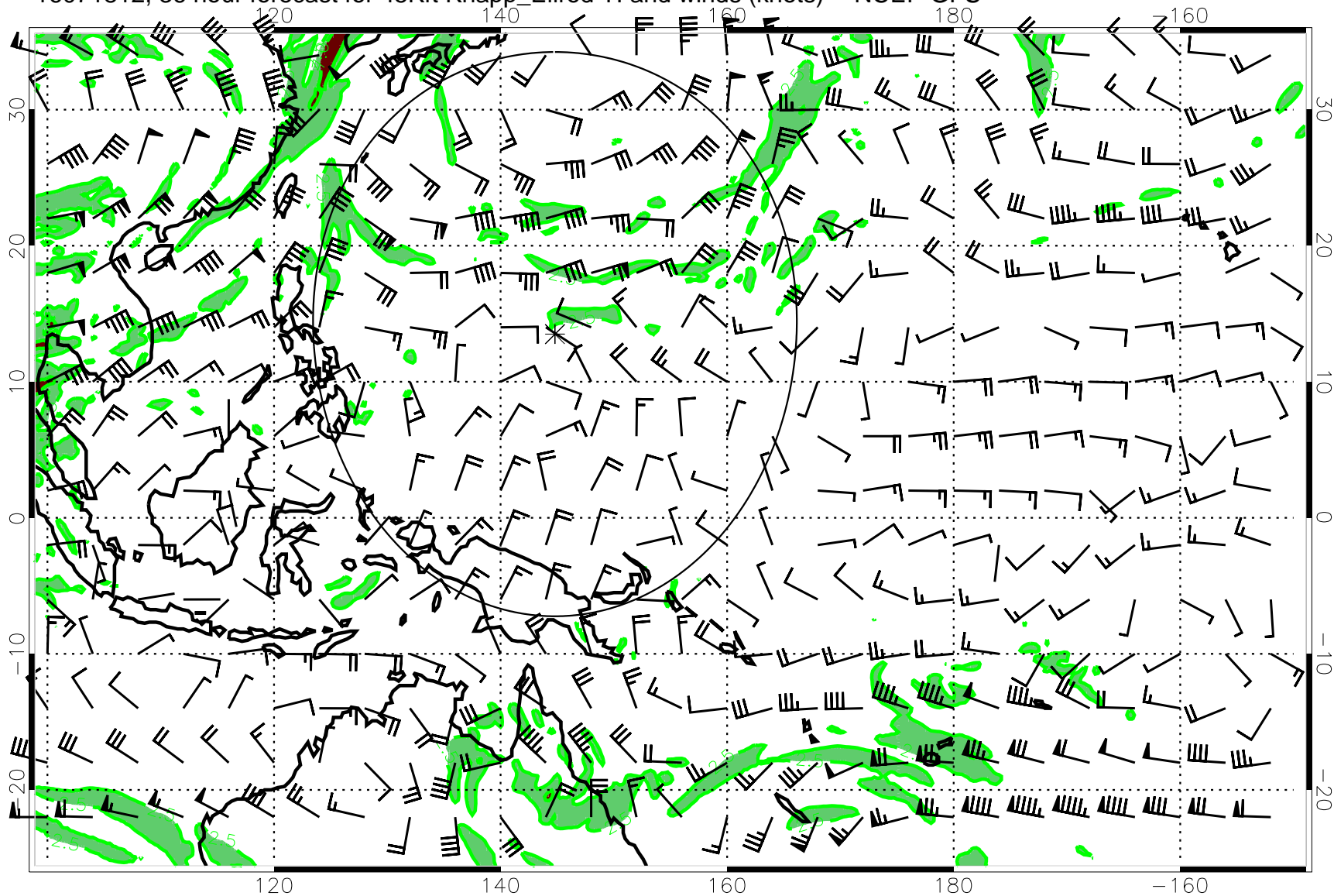
16071812, 36 hour forecast for 45Kft Knapp_Ellrod TI and winds (knots) -- NCEP GFS
