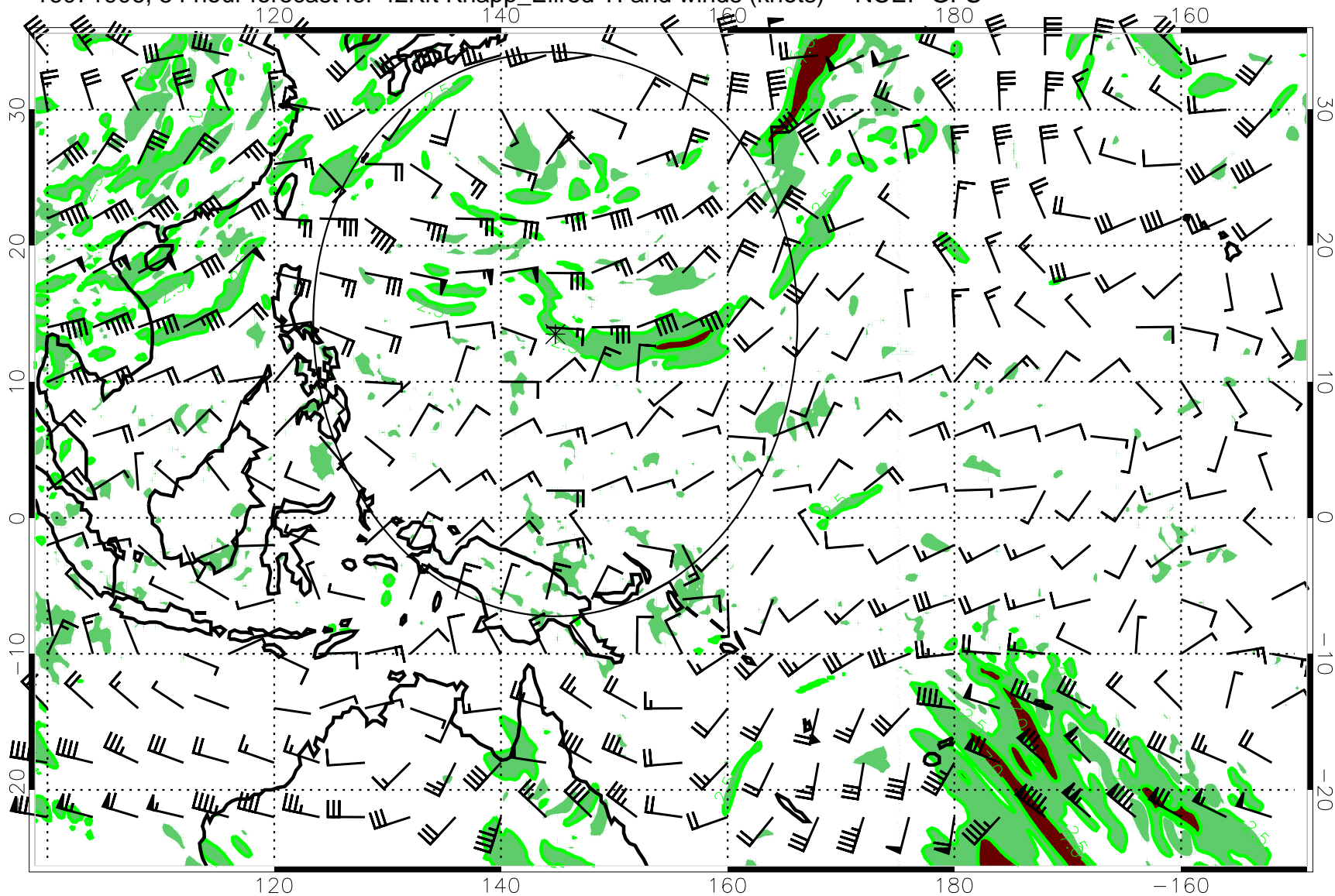
16071906, 54 hour forecast for 42Kft Knapp_Ellrod TI and winds (knots) -- NCEP GFS
