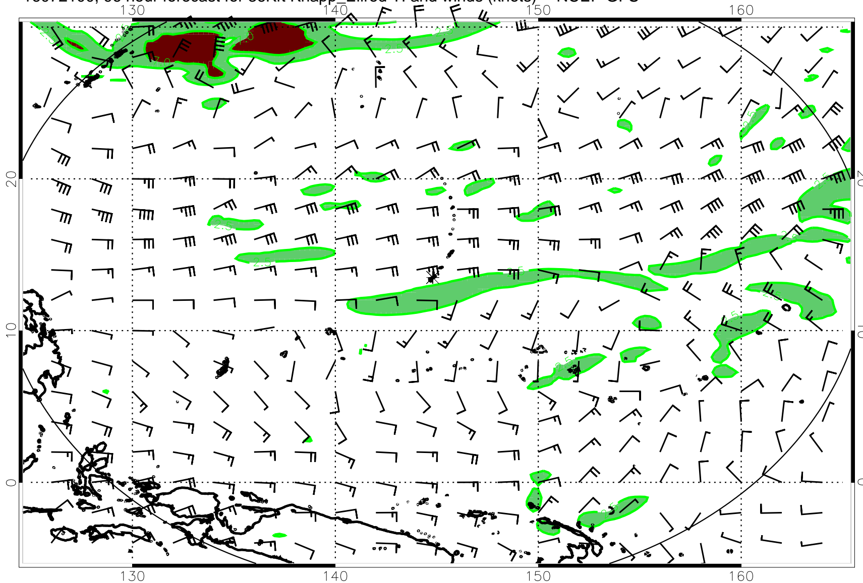
16072100, 96 hour forecast for 36Kft Knapp_Ellrod TI and winds (knots) -- NCEP GFS
