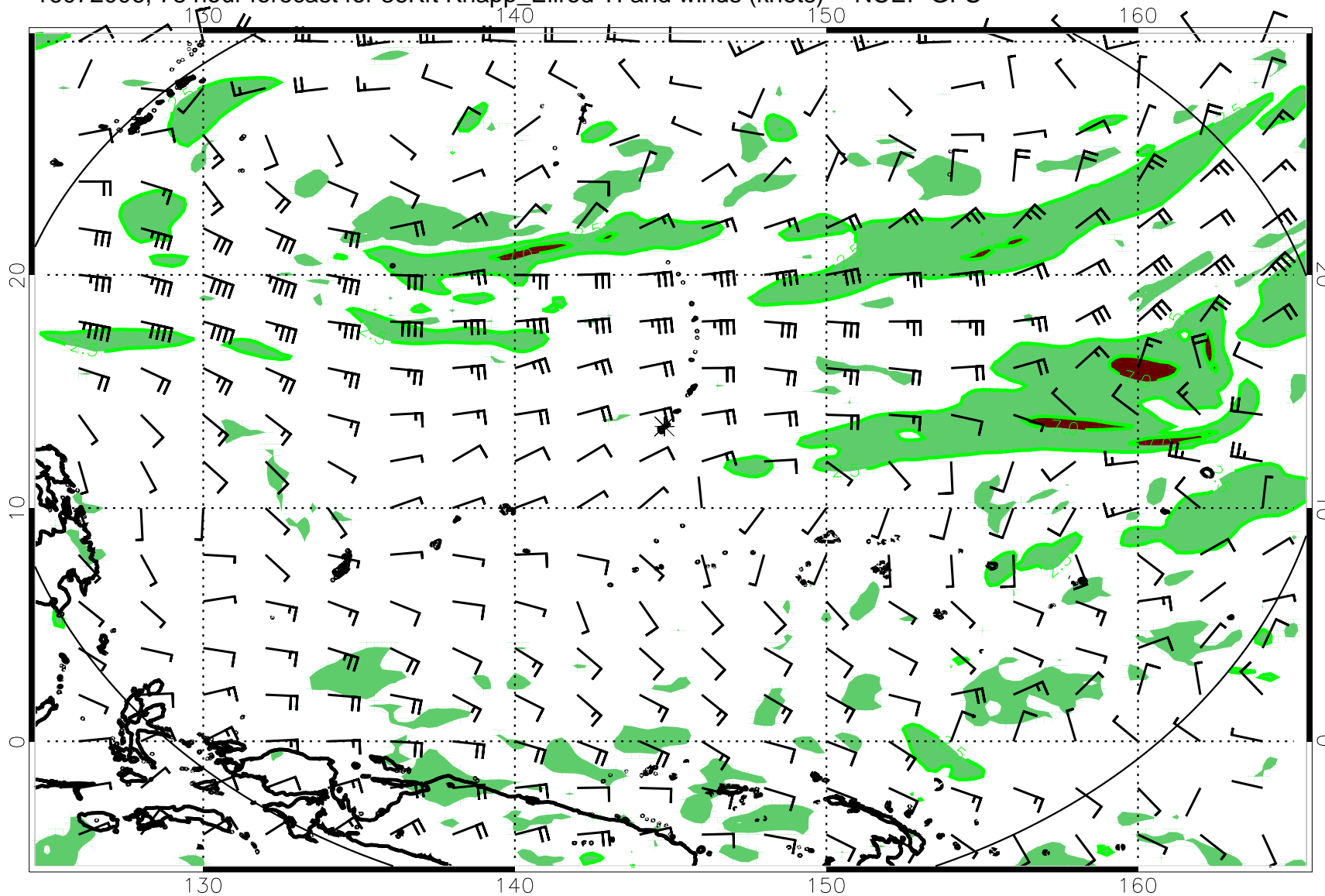
16072006, 78 hour forecast for 36Kft Knapp_Ellrod TI and winds (knots) -- NCEP GFS
