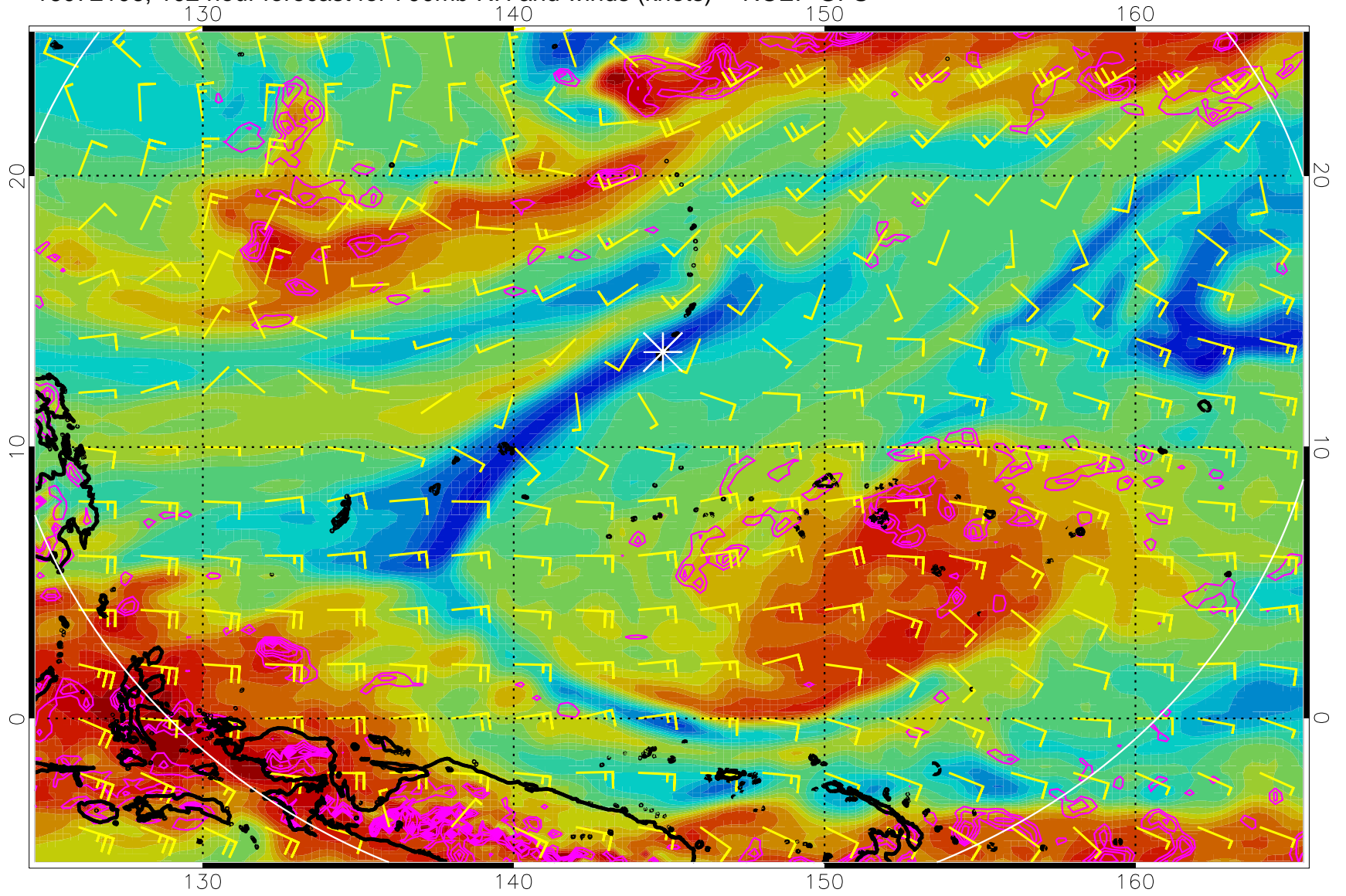
16072106, 102 hour forecast for 700mb RH and winds (knots) -- NCEP GFS
