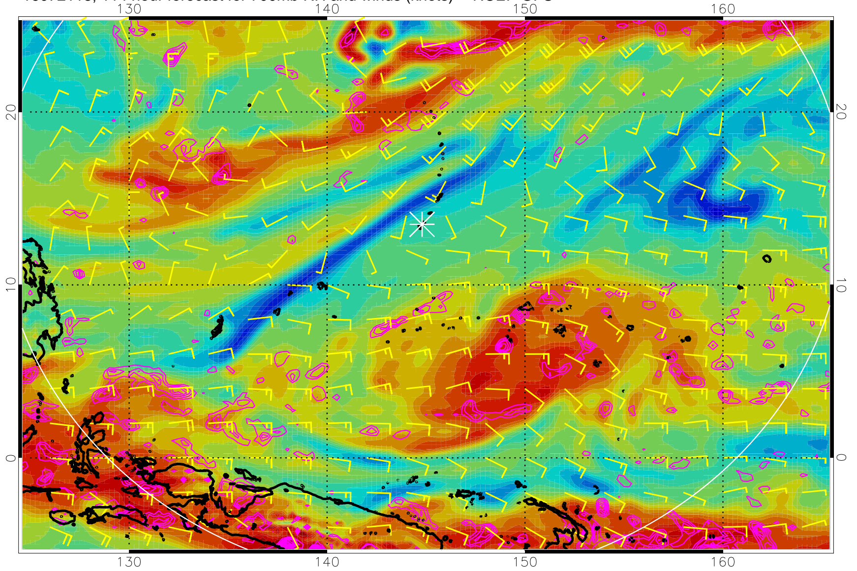
16072118, 114 hour forecast for 700mb RH and winds (knots) -- NCEP GFS
