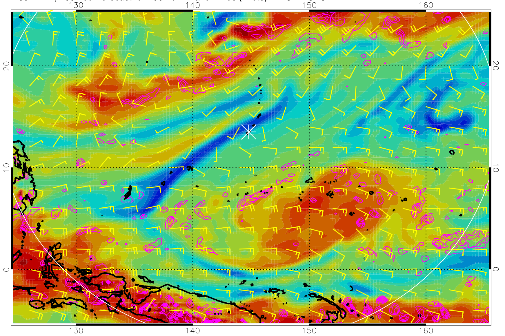
16072112, 108 hour forecast for 700mb RH and winds (knots) -- NCEP GFS
