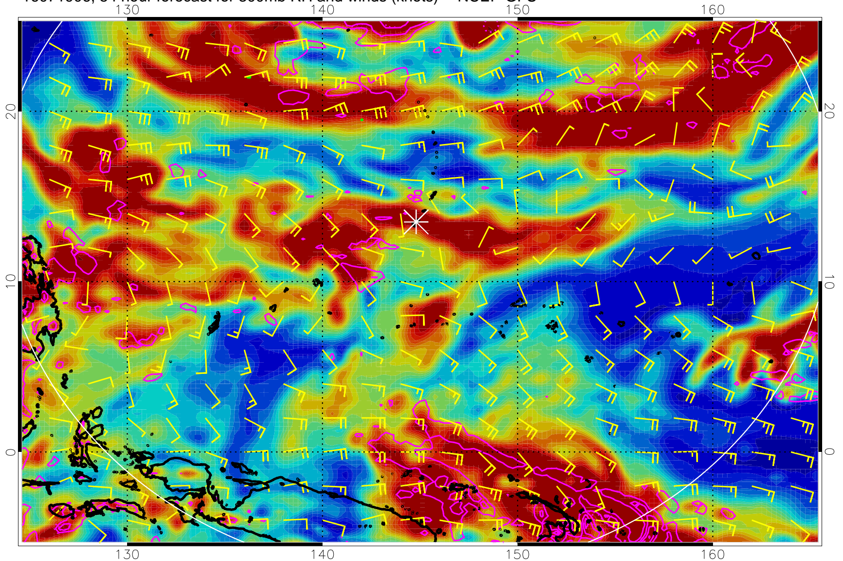
16071906, 54 hour forecast for 300mb RH and winds (knots) -- NCEP GFS
