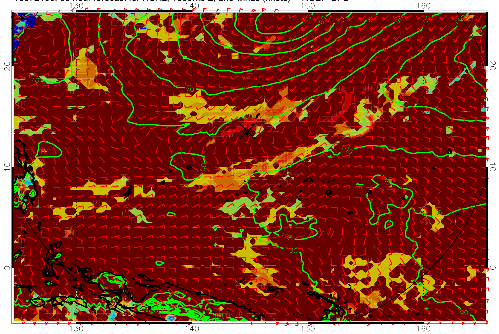
16072100, 96 hour forecast for HCAL, 1000mb Z, and winds (knots) -- NCEP GFS
