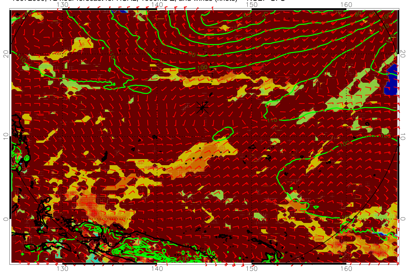
16072000, 72 hour forecast for HCAL, 1000mb Z, and winds (knots) -- NCEP GFS
