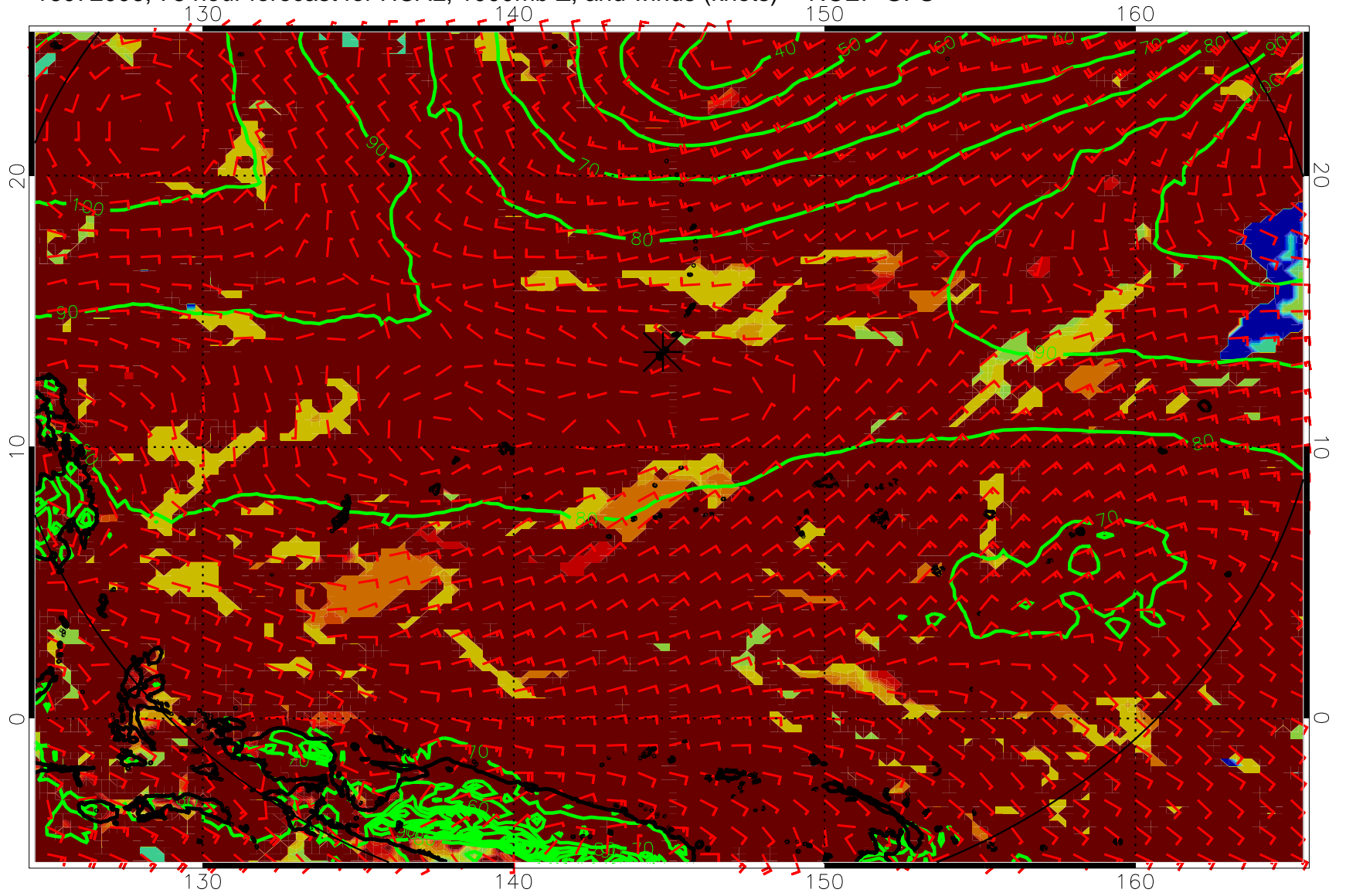
16072006, 78 hour forecast for HCAL, 1000mb Z, and winds (knots) -- NCEP GFS
