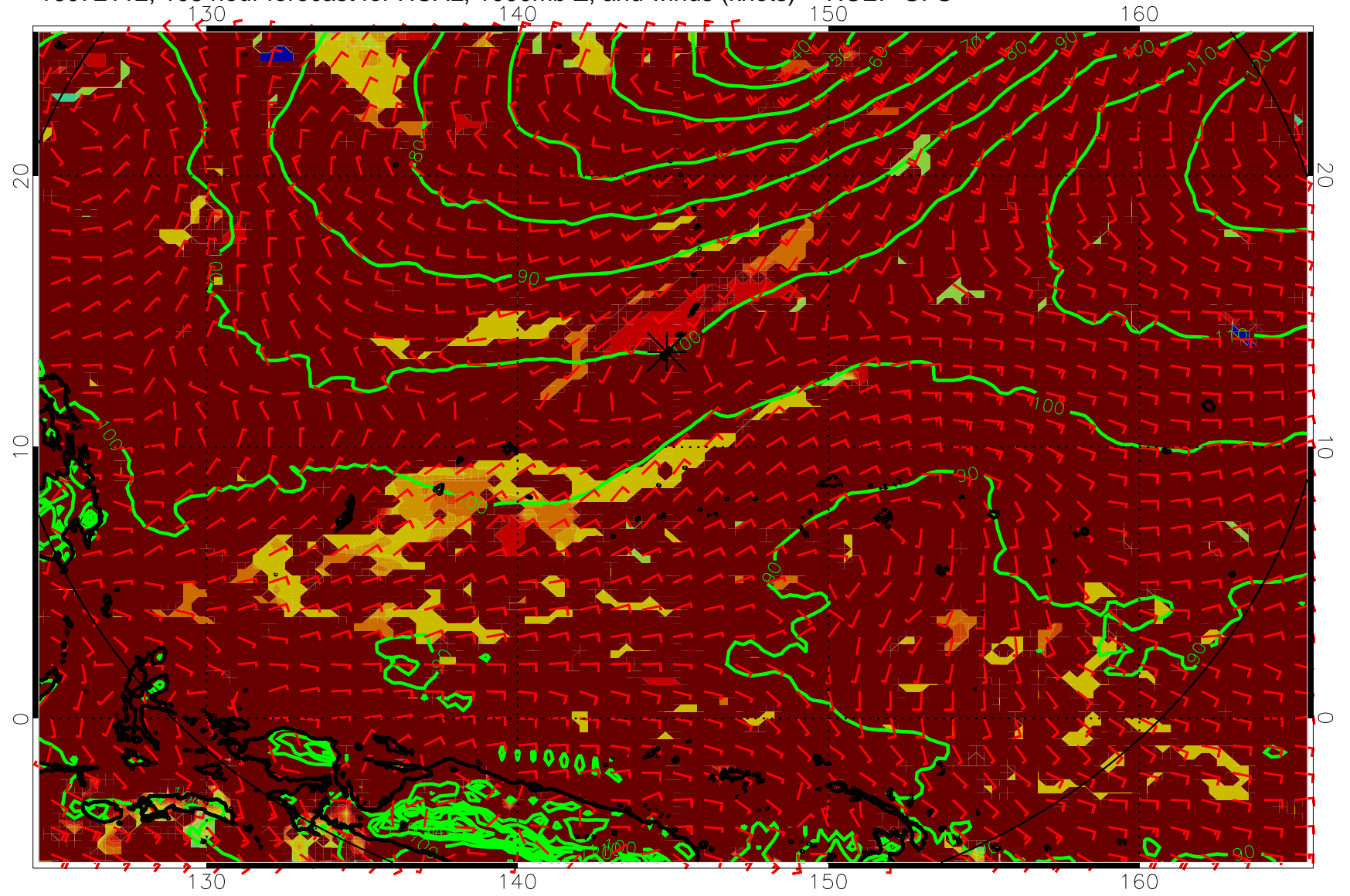
16072112, 108 hour forecast for HCAL, 1000mb Z, and winds (knots) -- NCEP GFS
