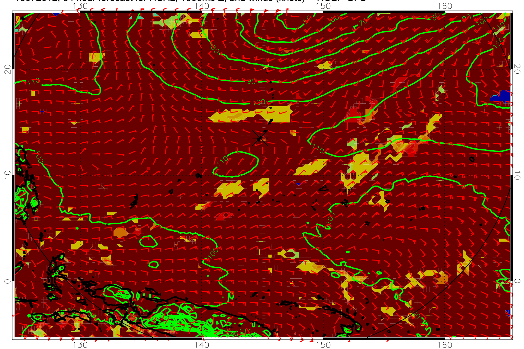
16072012, 84 hour forecast for HCAL, 1000mb Z, and winds (knots) -- NCEP GFS
