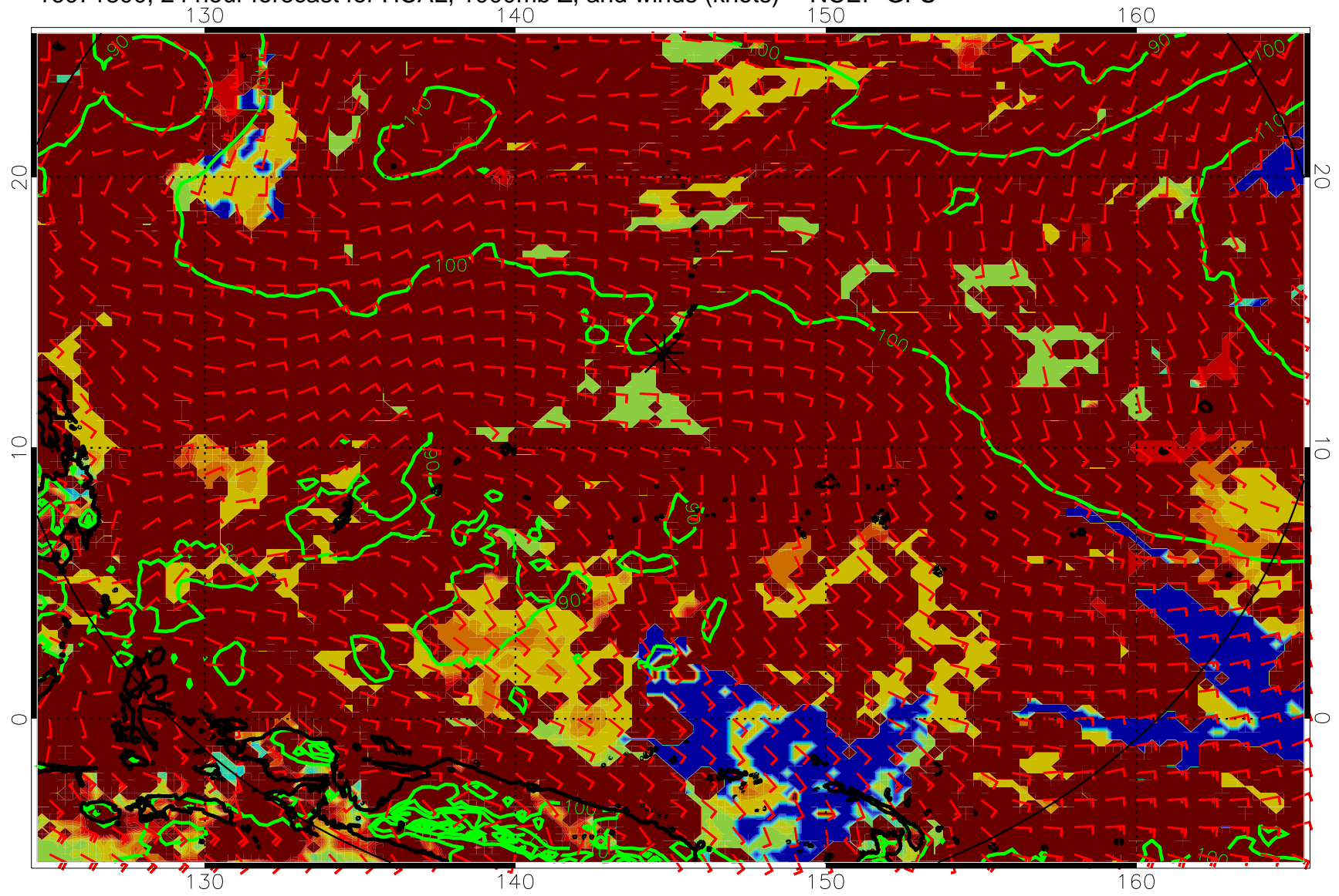
16071800, 24 hour forecast for HCAL, 1000mb Z, and winds (knots) -- NCEP GFS
