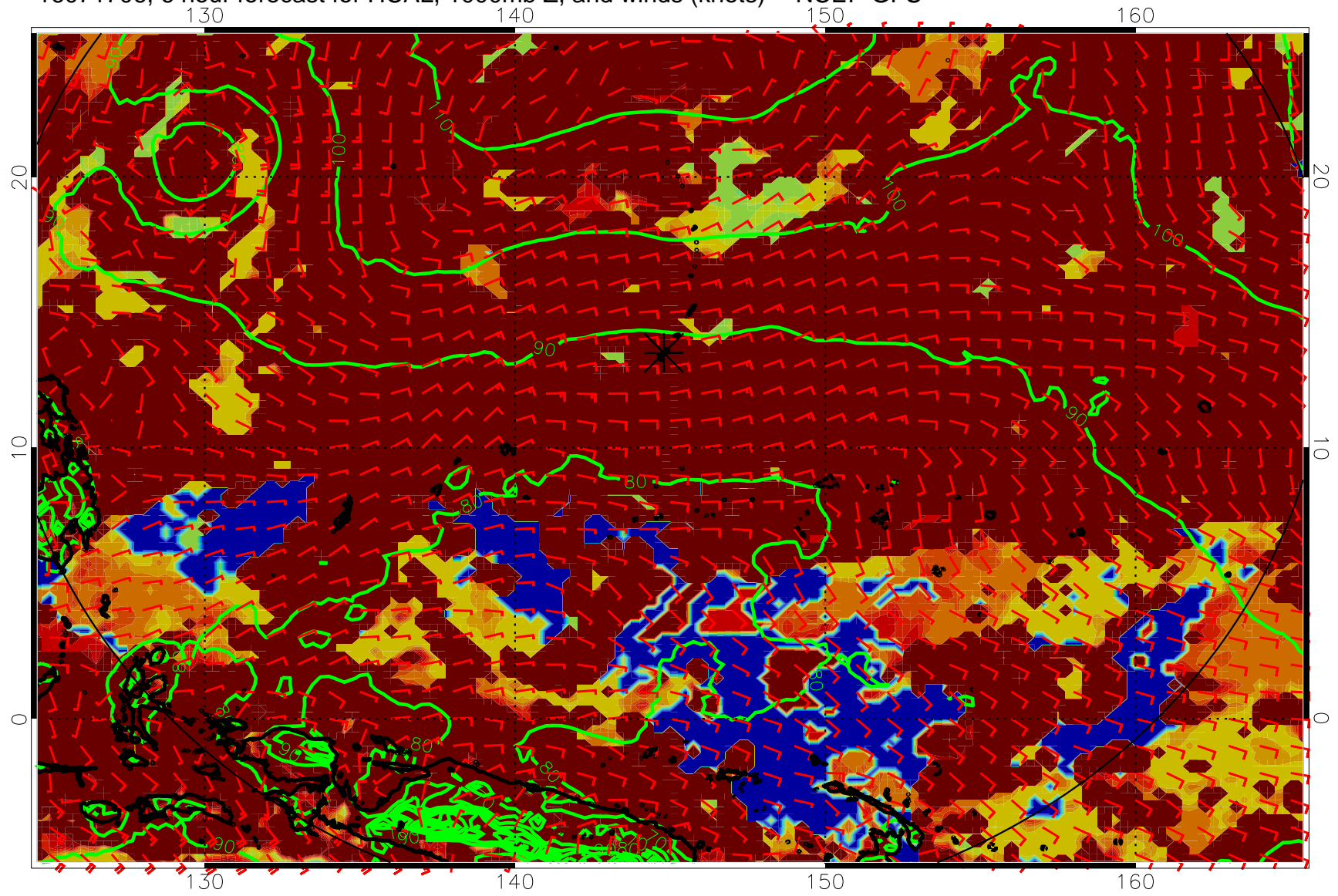
16071706, 6 hour forecast for HCAL, 1000mb Z, and winds (knots) -- NCEP GFS
