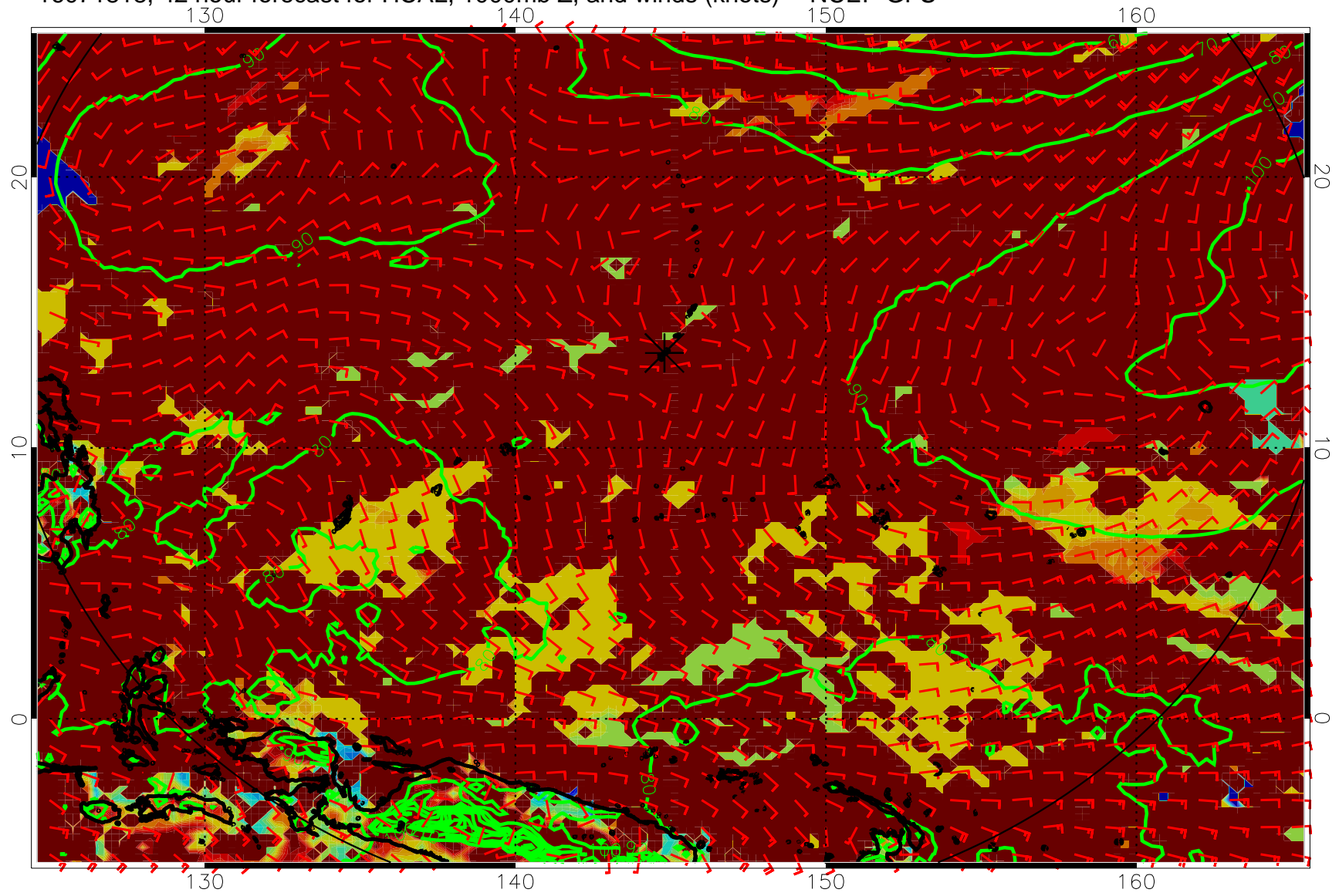
16071818, 42 hour forecast for HCAL, 1000mb Z, and winds (knots) -- NCEP GFS
