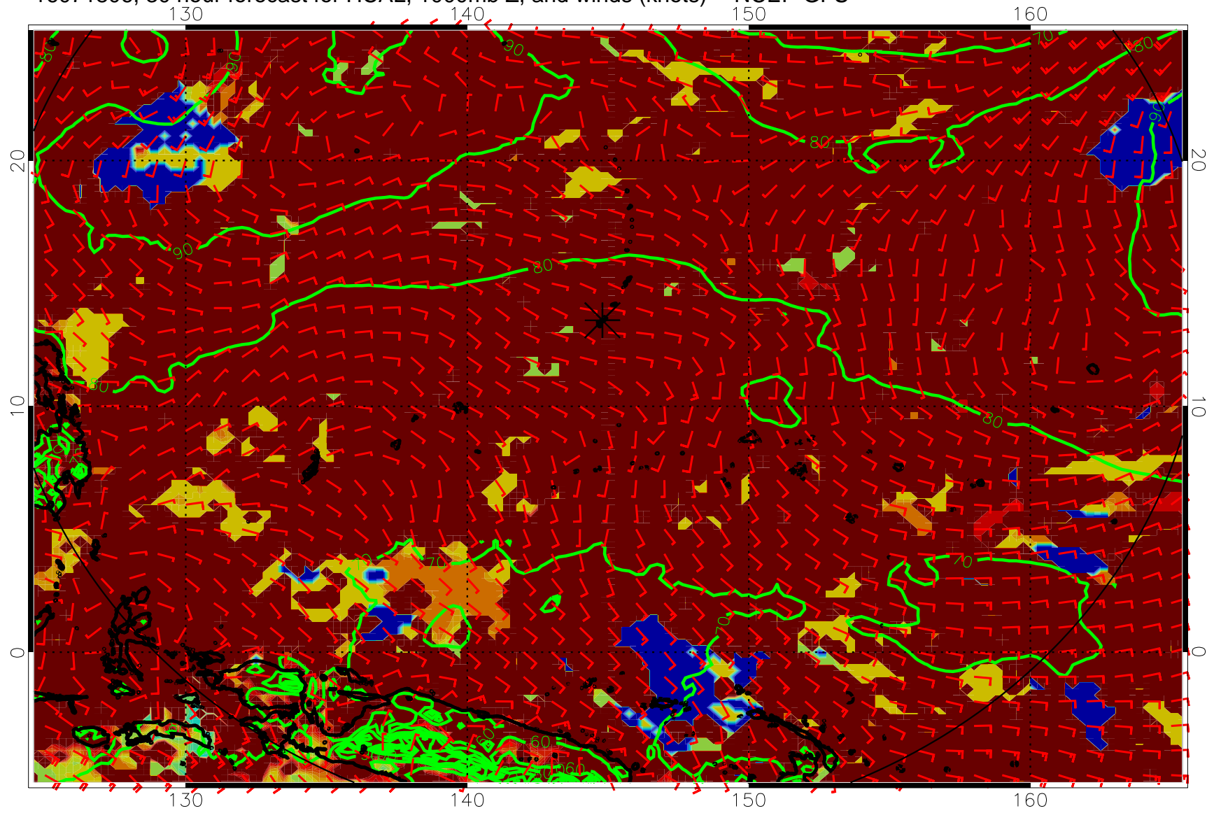
16071806, 30 hour forecast for HCAL, 1000mb Z, and winds (knots) -- NCEP GFS
