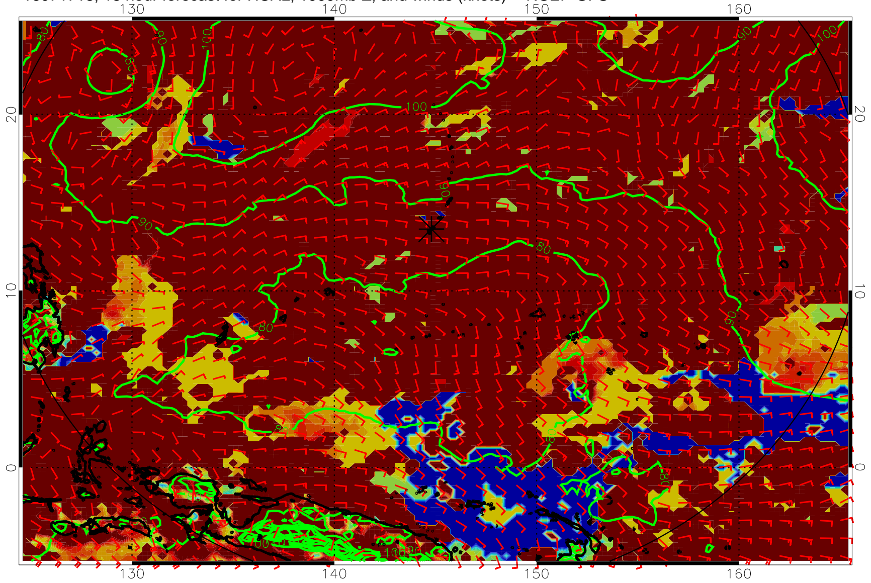
16071718, 18 hour forecast for HCAL, 1000mb Z, and winds (knots) -- NCEP GFS
