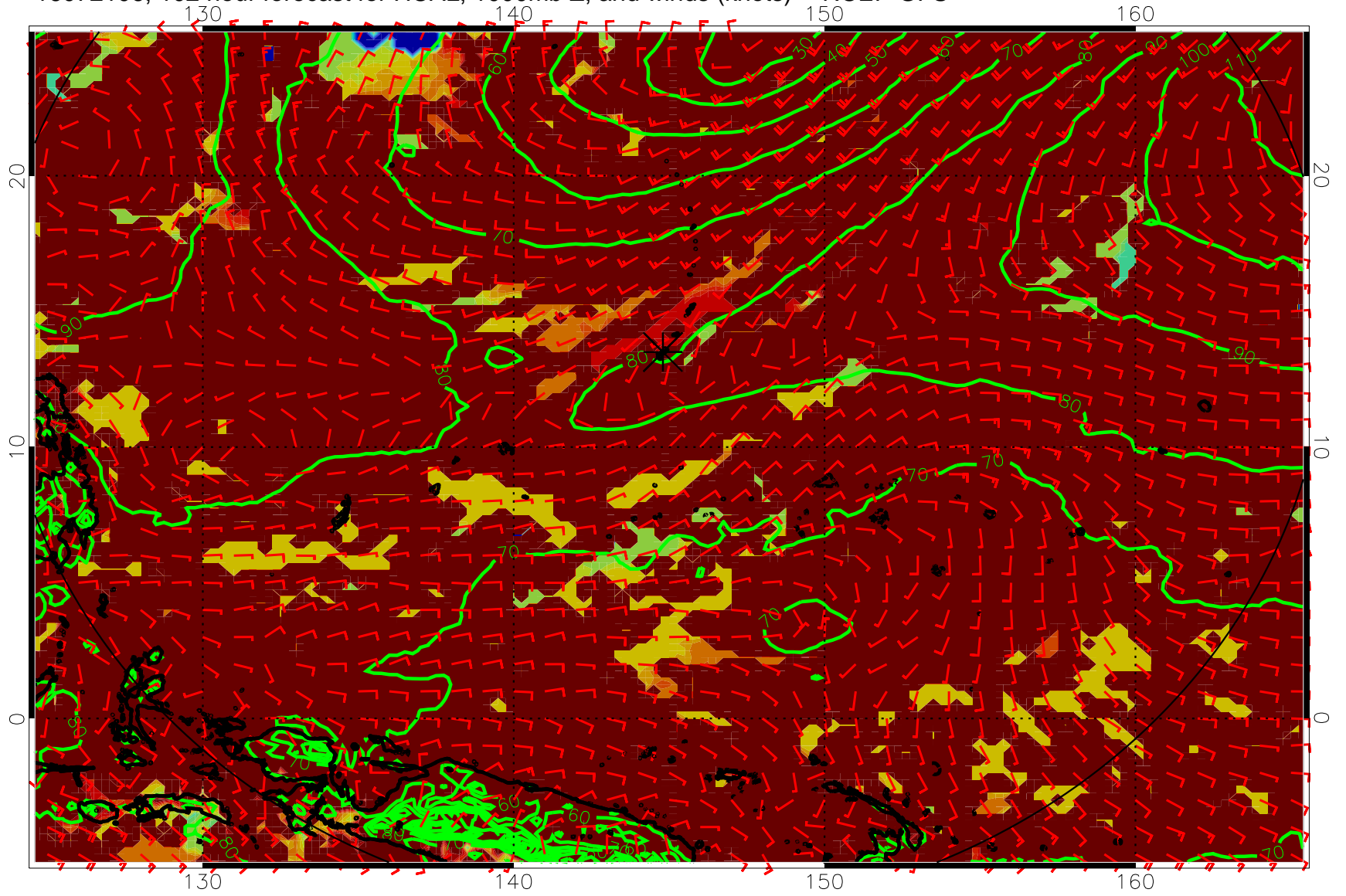
16072106, 102 hour forecast for HCAL, 1000mb Z, and winds (knots) -- NCEP GFS
