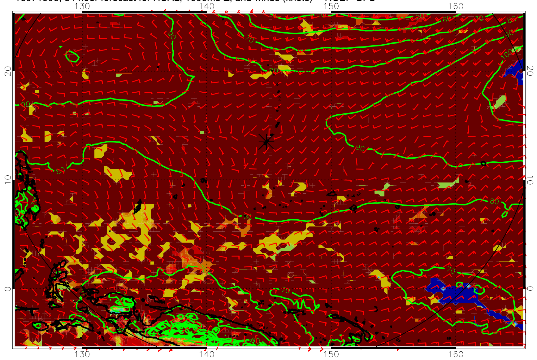
16071906, 54 hour forecast for HCAL, 1000mb Z, and winds (knots) -- NCEP GFS
