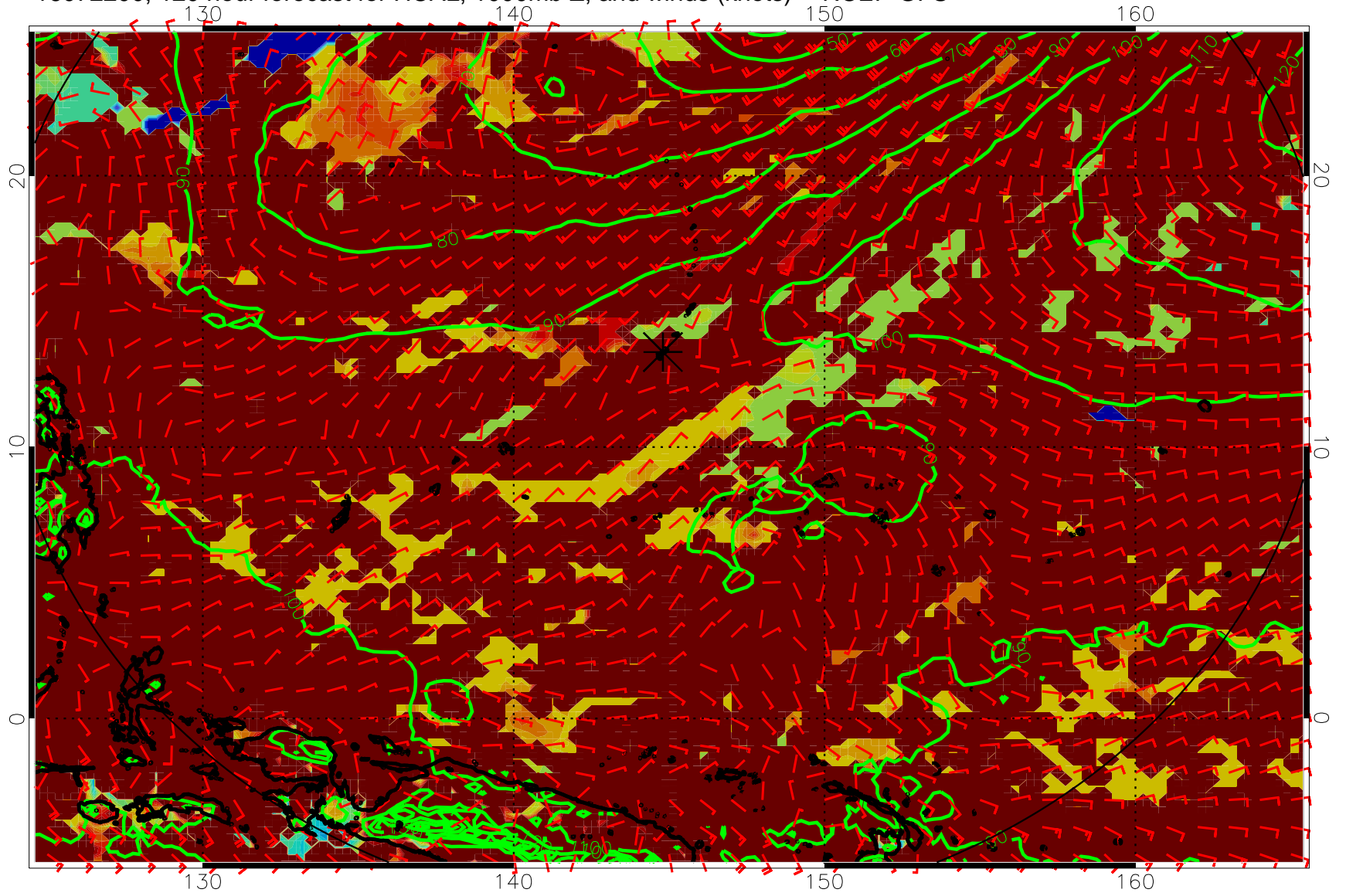
16072200, 120 hour forecast for HCAL, 1000mb Z, and winds (knots) -- NCEP GFS
