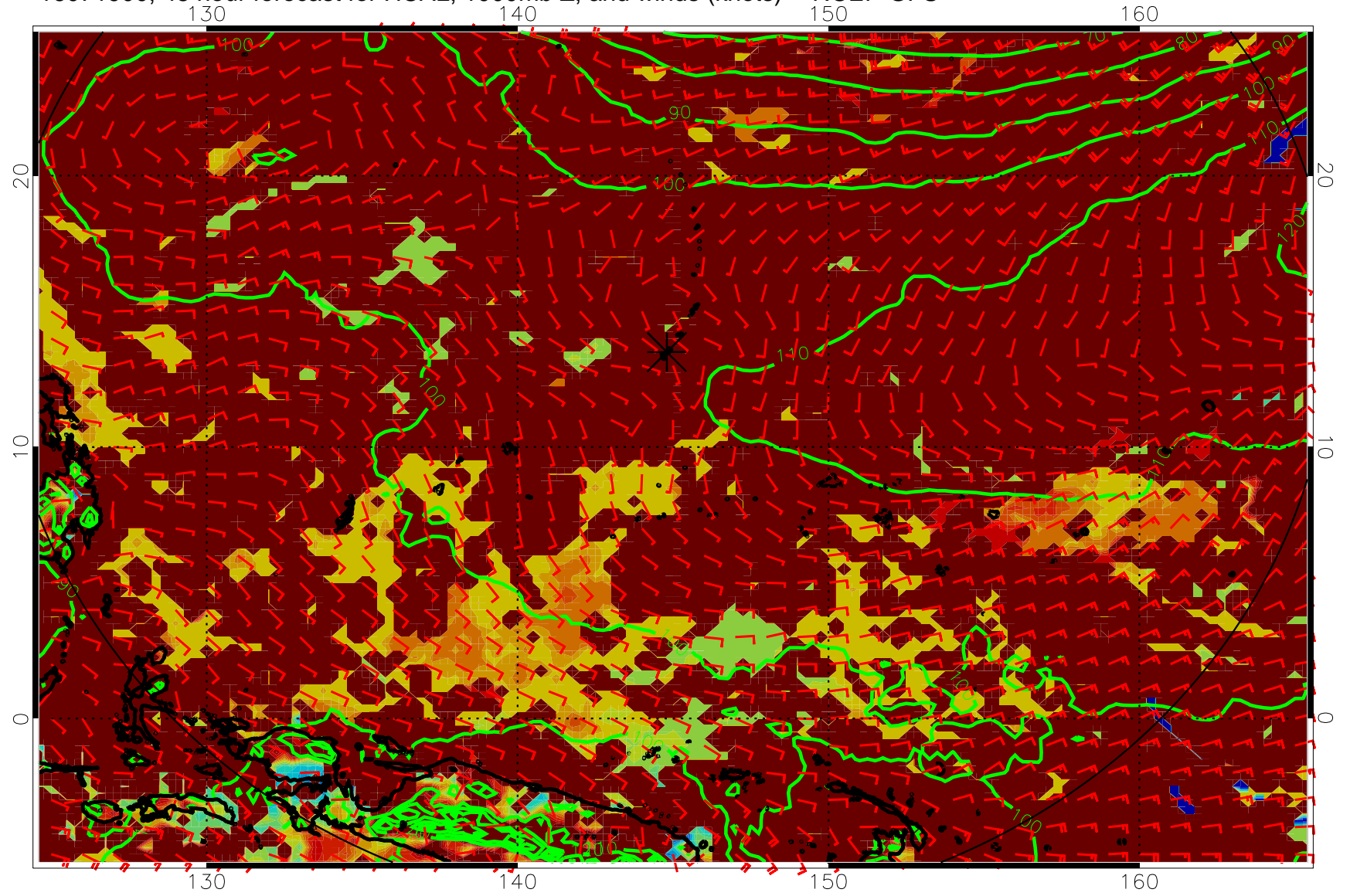
16071900, 48 hour forecast for HCAL, 1000mb Z, and winds (knots) -- NCEP GFS
