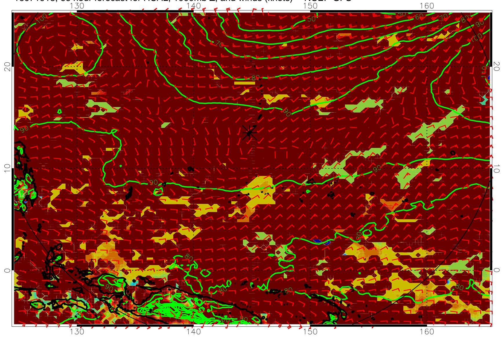
16071918, 66 hour forecast for HCAL, 1000mb Z, and winds (knots) -- NCEP GFS
