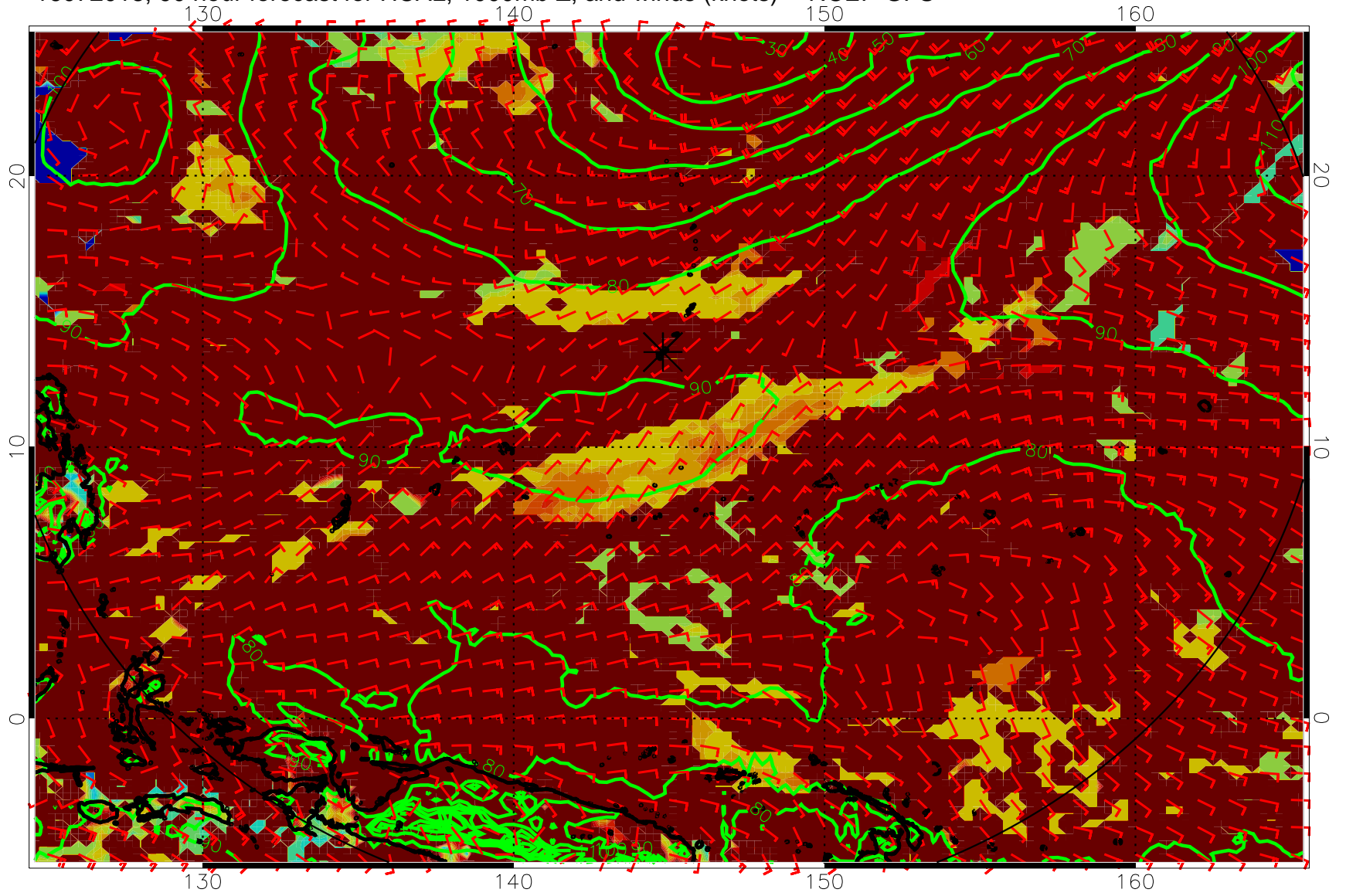
16072018, 90 hour forecast for HCAL, 1000mb Z, and winds (knots) -- NCEP GFS
