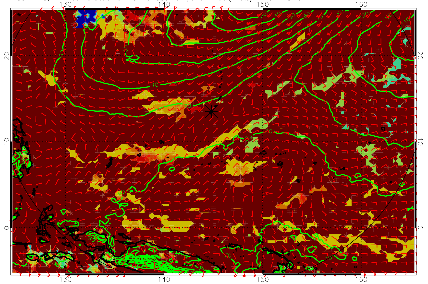
16072118, 114 hour forecast for HCAL, 1000mb Z, and winds (knots) -- NCEP GFS
