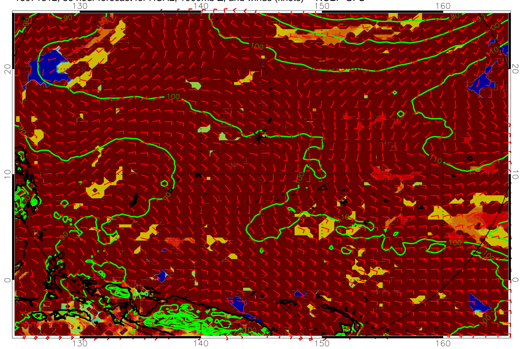
16071812, 36 hour forecast for HCAL, 1000mb Z, and winds (knots) -- NCEP GFS
