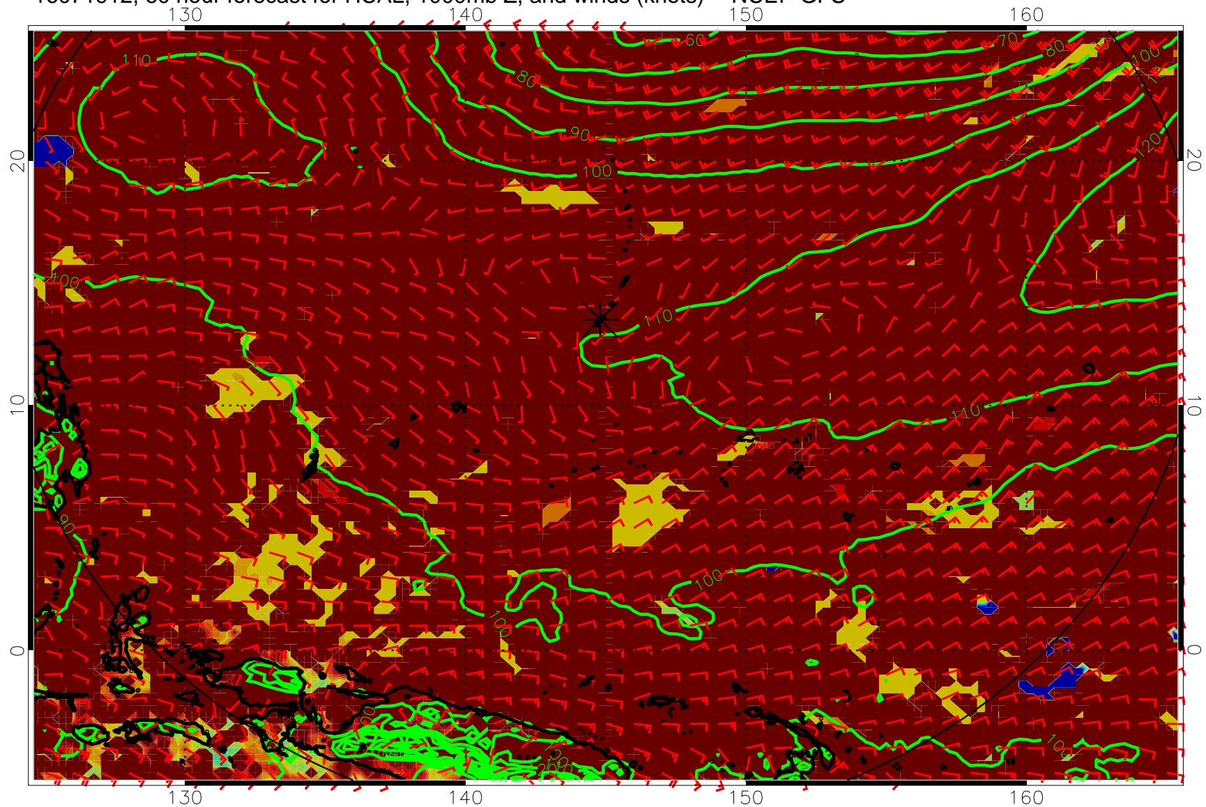
16071912, 60 hour forecast for HCAL, 1000mb Z, and winds (knots) -- NCEP GFS
