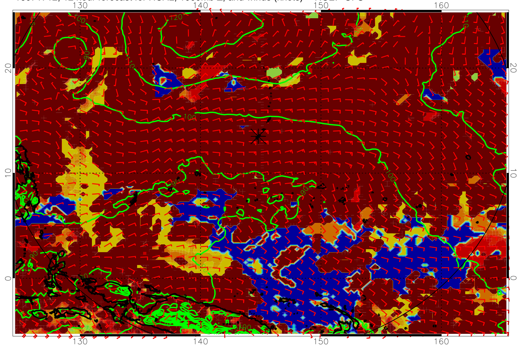
16071712, 12 hour forecast for HCAL, 1000mb Z, and winds (knots) -- NCEP GFS
