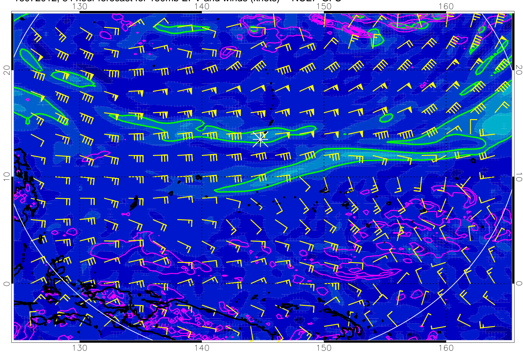
16072012, 84 hour forecast for 150mb EPV and winds (knots) -- NCEP GFS
