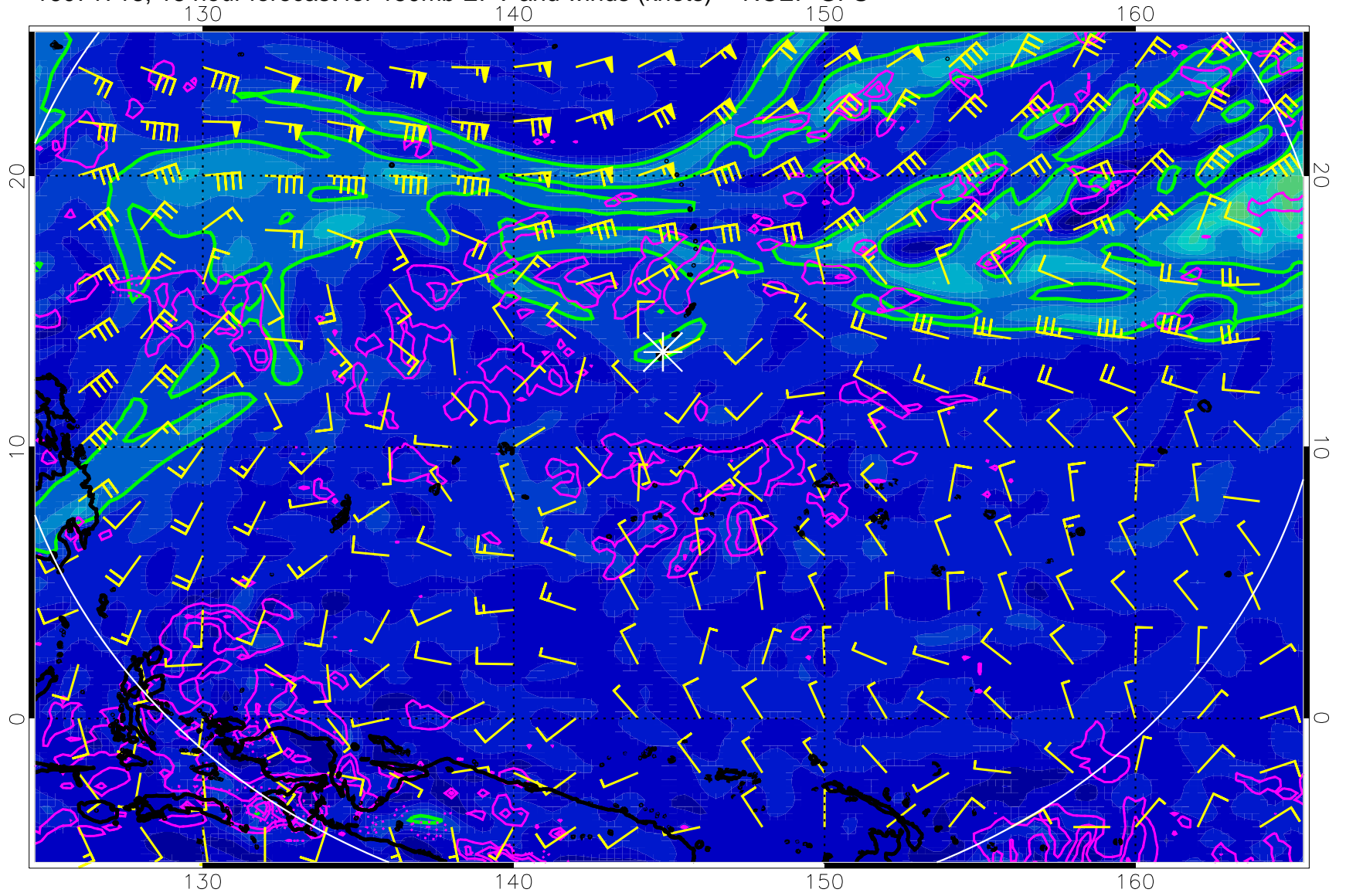
16071718, 18 hour forecast for 150mb EPV and winds (knots) -- NCEP GFS
