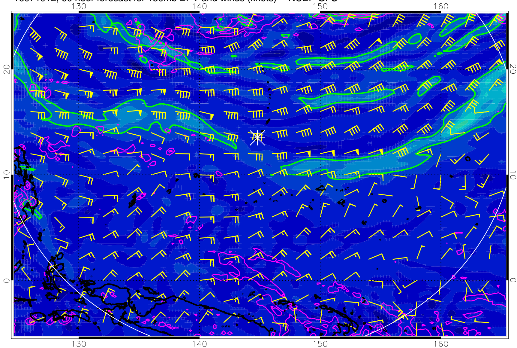
16071912, 60 hour forecast for 150mb EPV and winds (knots) -- NCEP GFS
