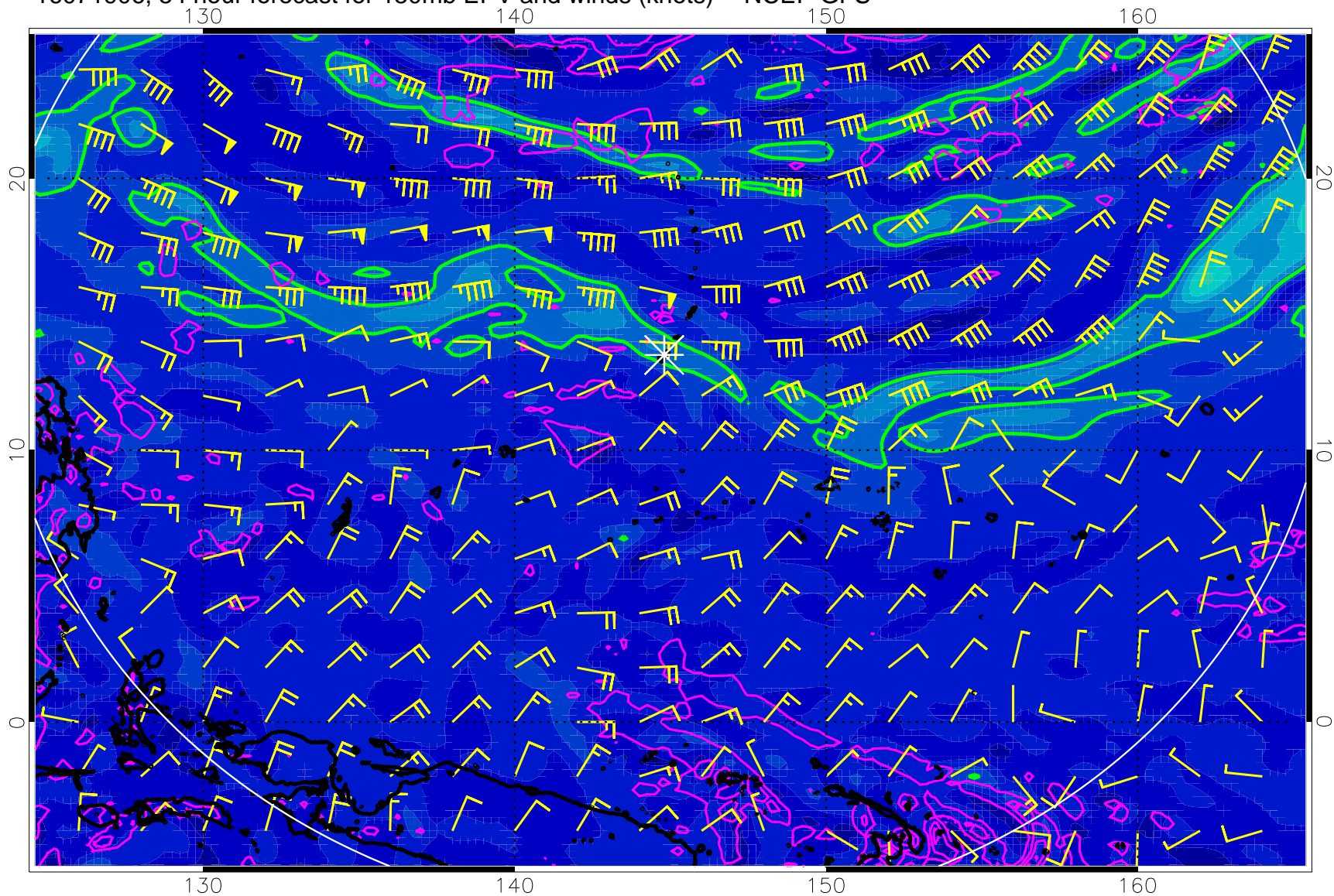
16071906, 54 hour forecast for 150mb EPV and winds (knots) -- NCEP GFS
