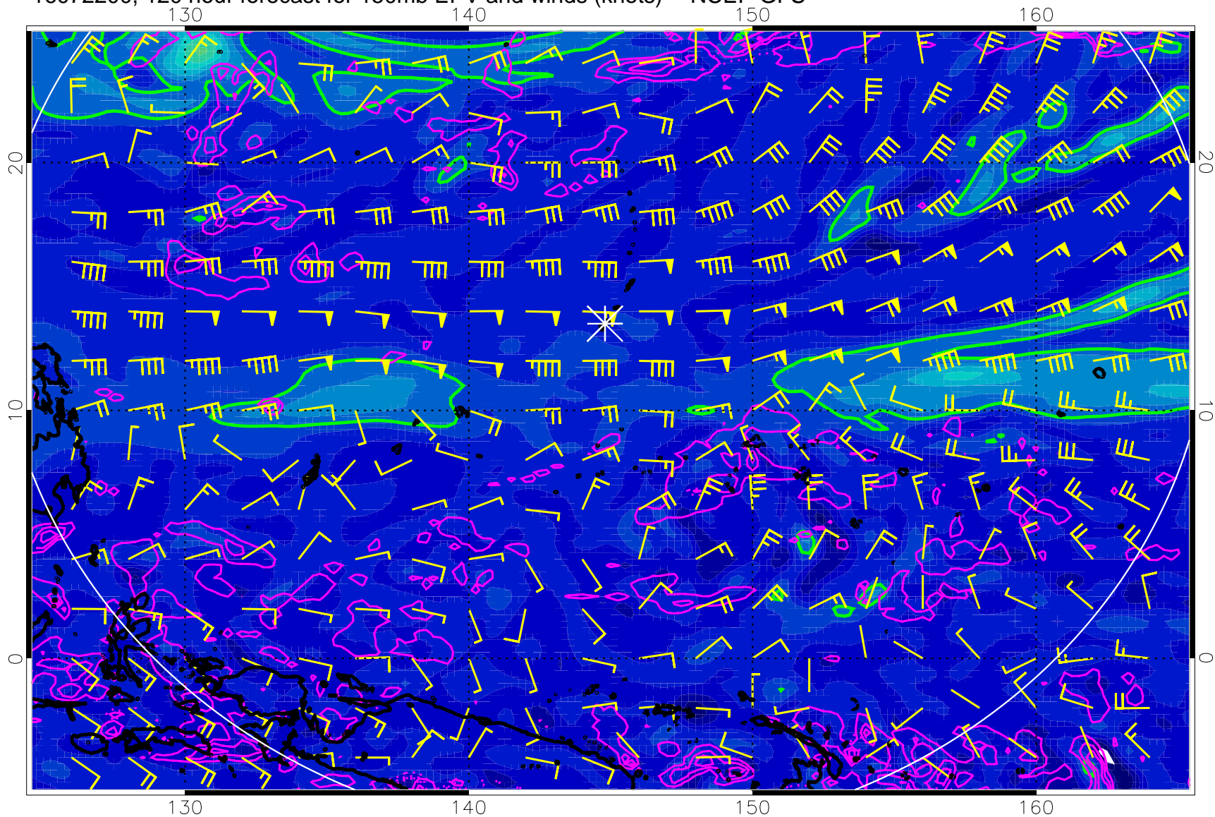
16072200, 120 hour forecast for 150mb EPV and winds (knots) -- NCEP GFS
