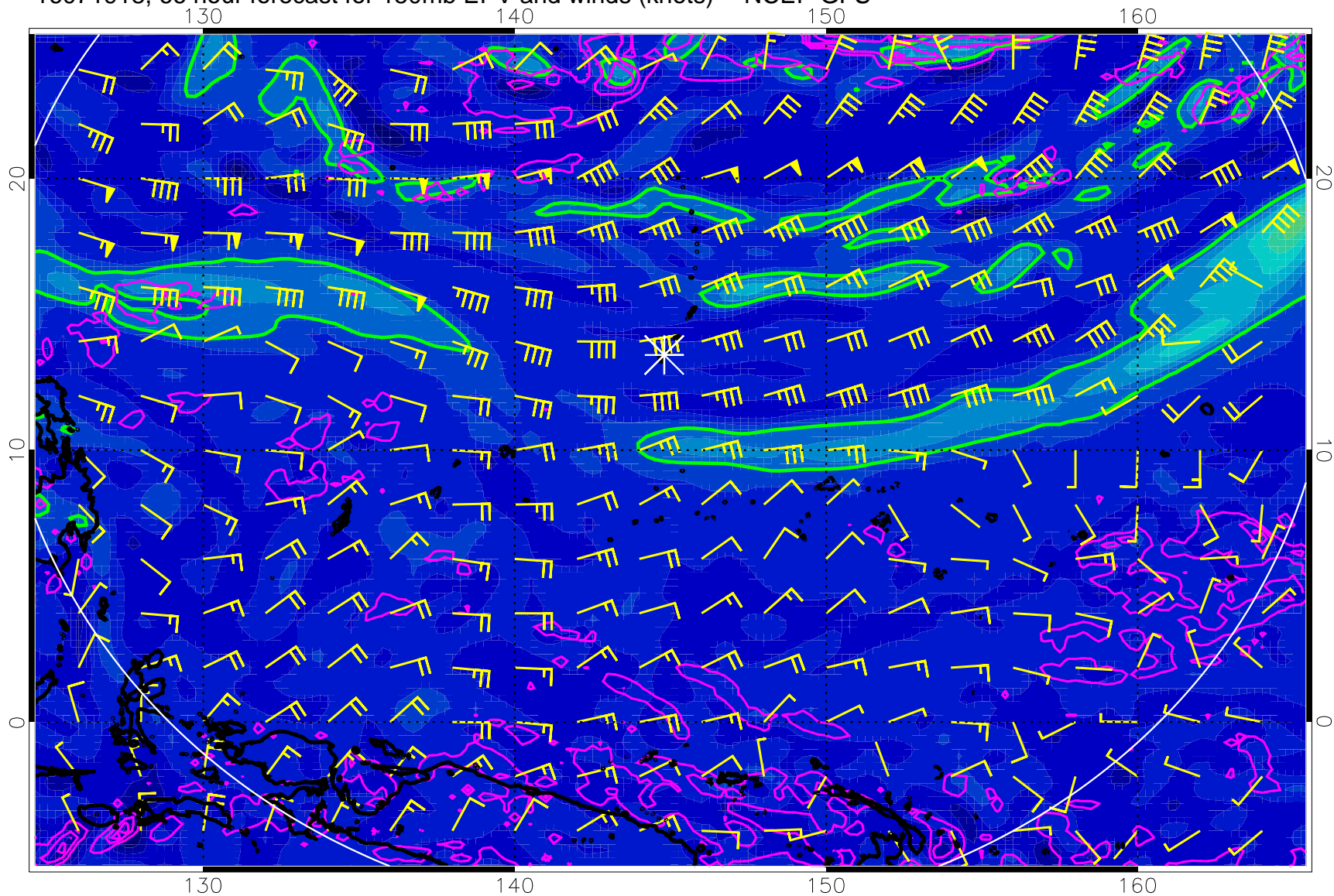
16071918, 66 hour forecast for 150mb EPV and winds (knots) -- NCEP GFS
