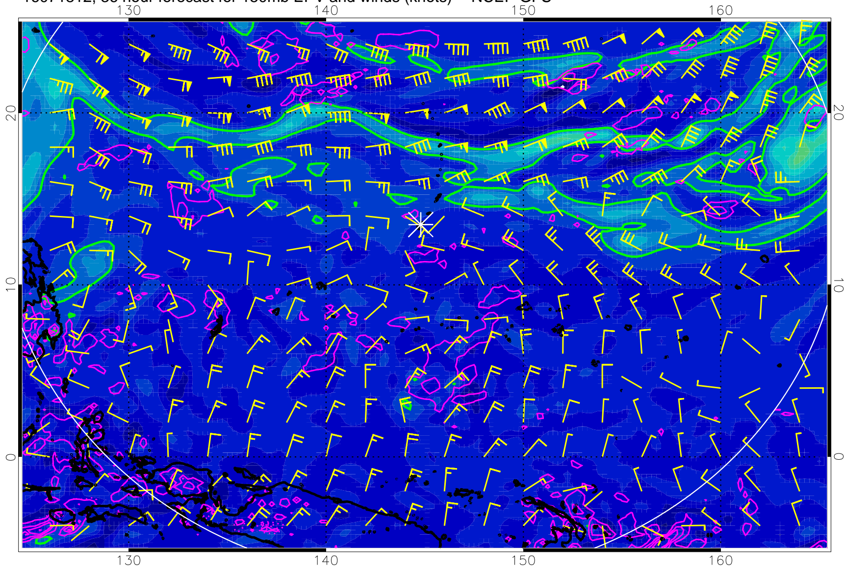
16071812, 36 hour forecast for 150mb EPV and winds (knots) -- NCEP GFS
