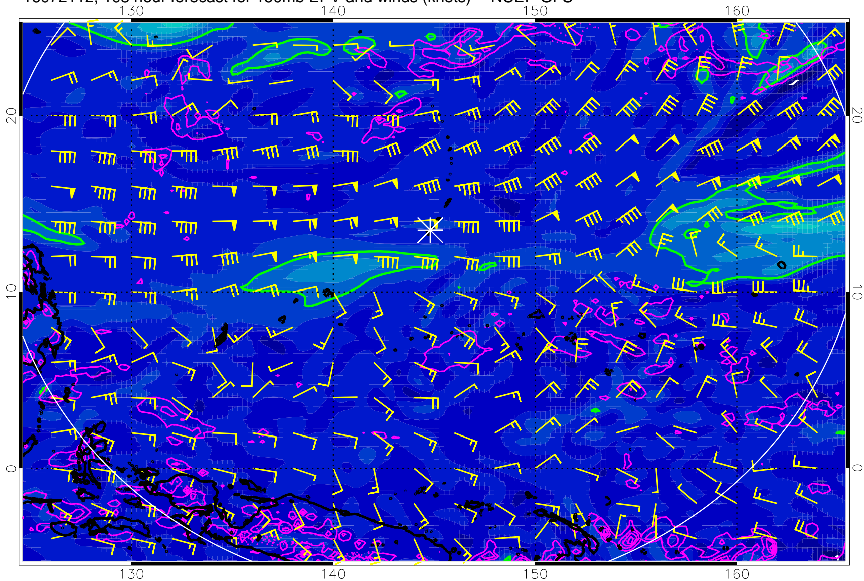
16072112, 108 hour forecast for 150mb EPV and winds (knots) -- NCEP GFS
