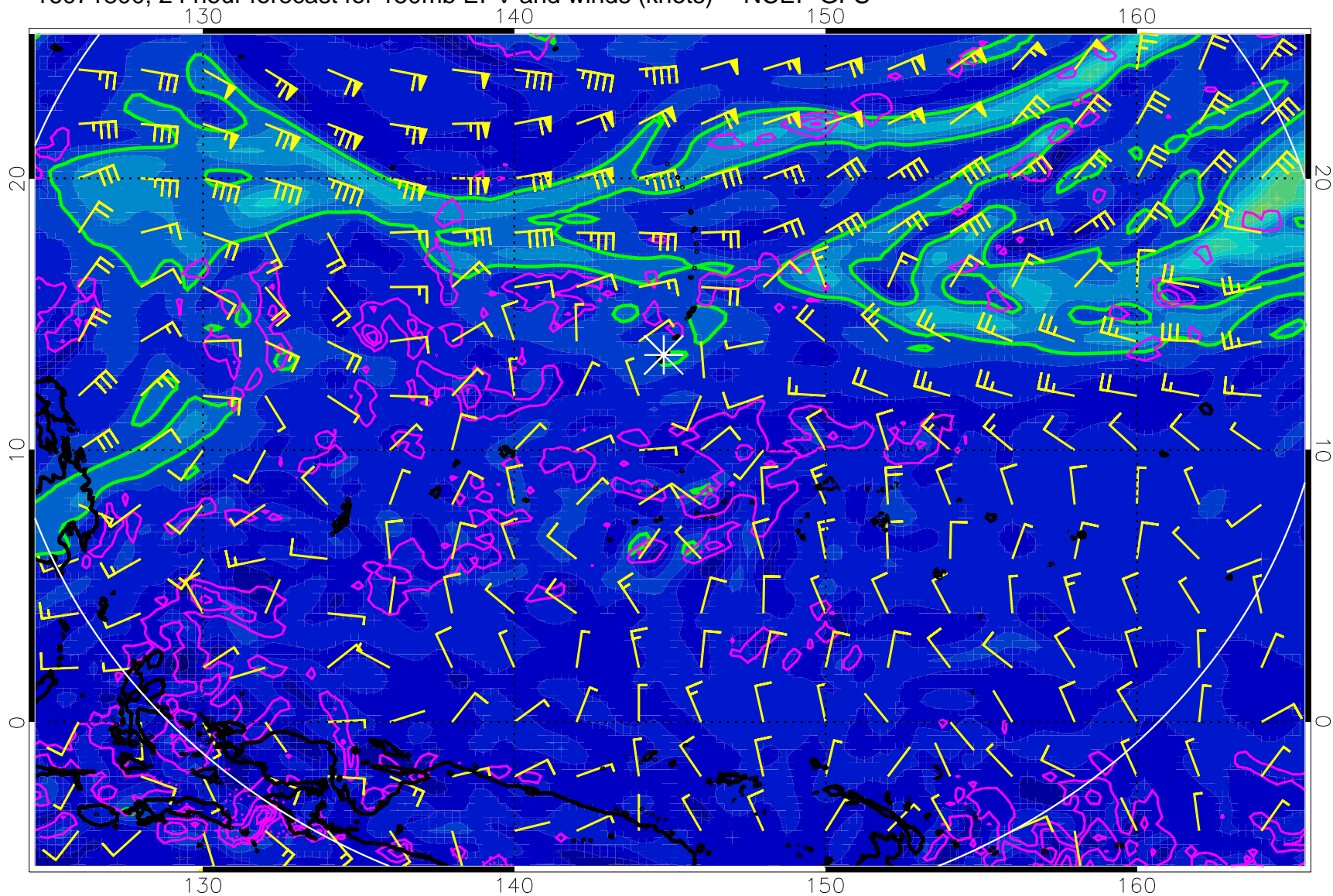
16071800, 24 hour forecast for 150mb EPV and winds (knots) -- NCEP GFS
