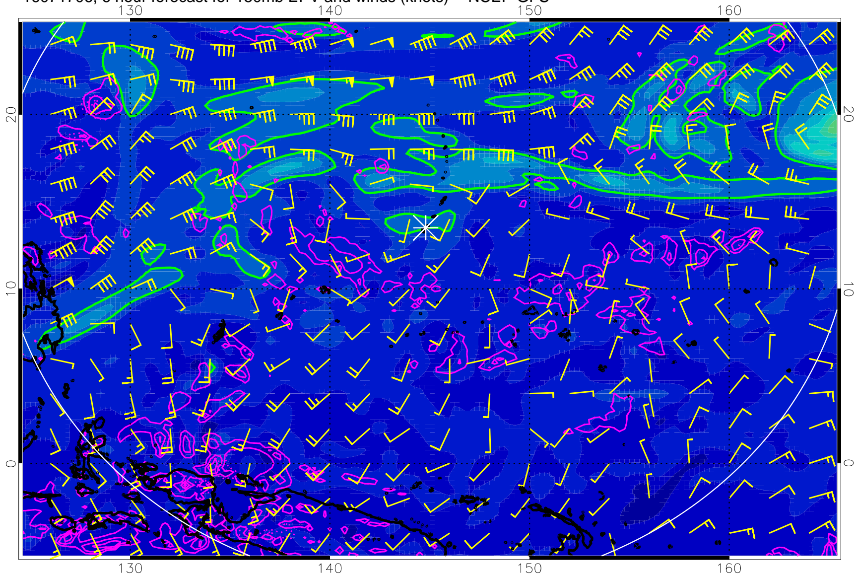
16071706, 6 hour forecast for 150mb EPV and winds (knots) -- NCEP GFS
