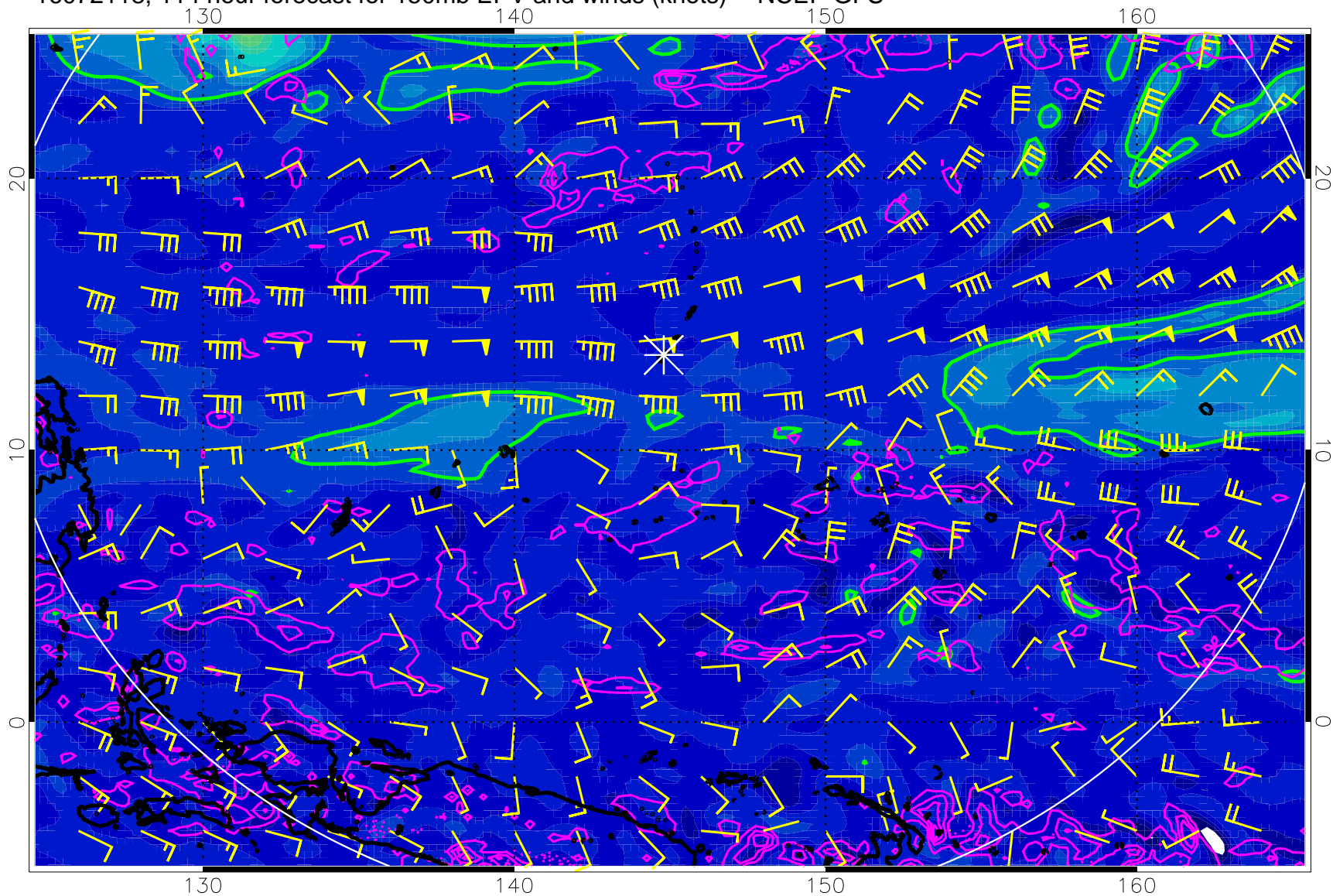
16072118, 114 hour forecast for 150mb EPV and winds (knots) -- NCEP GFS
