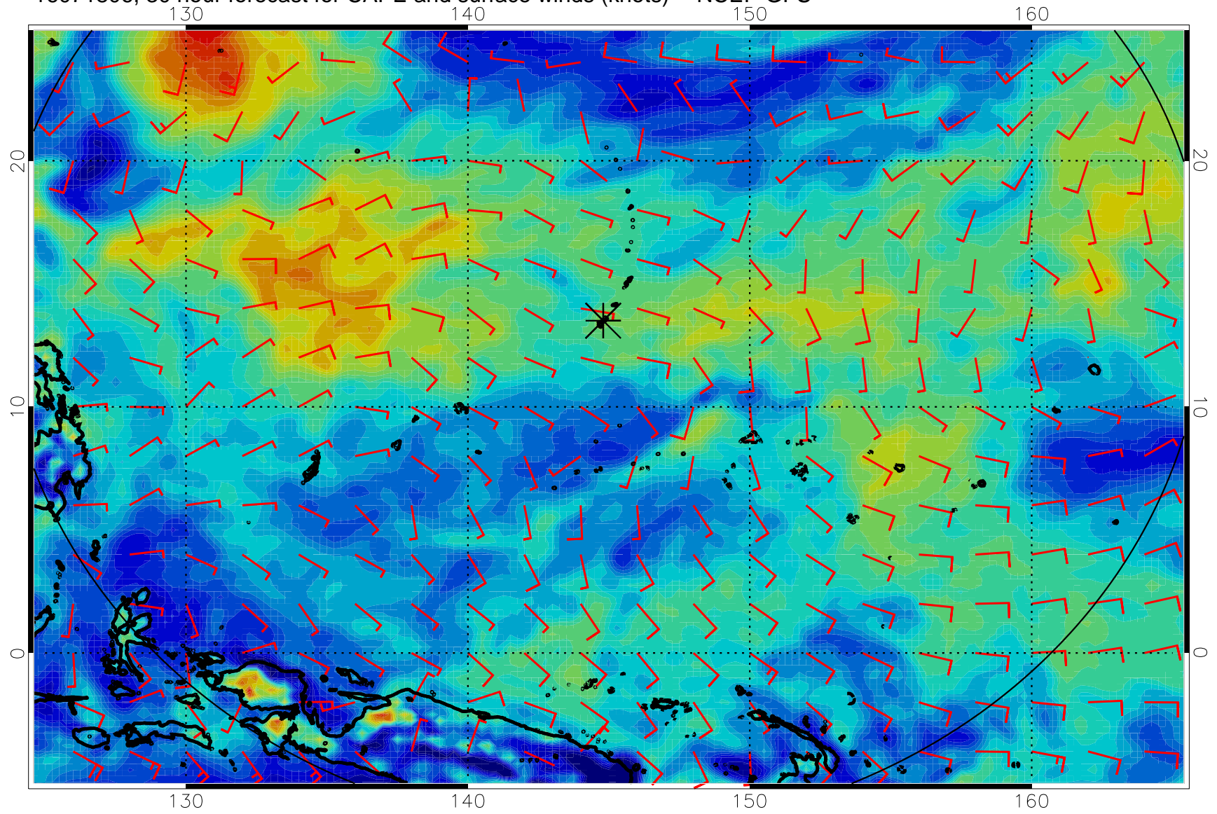
16071806, 30 hour forecast for CAPE and surface winds (knots) -- NCEP GFS
