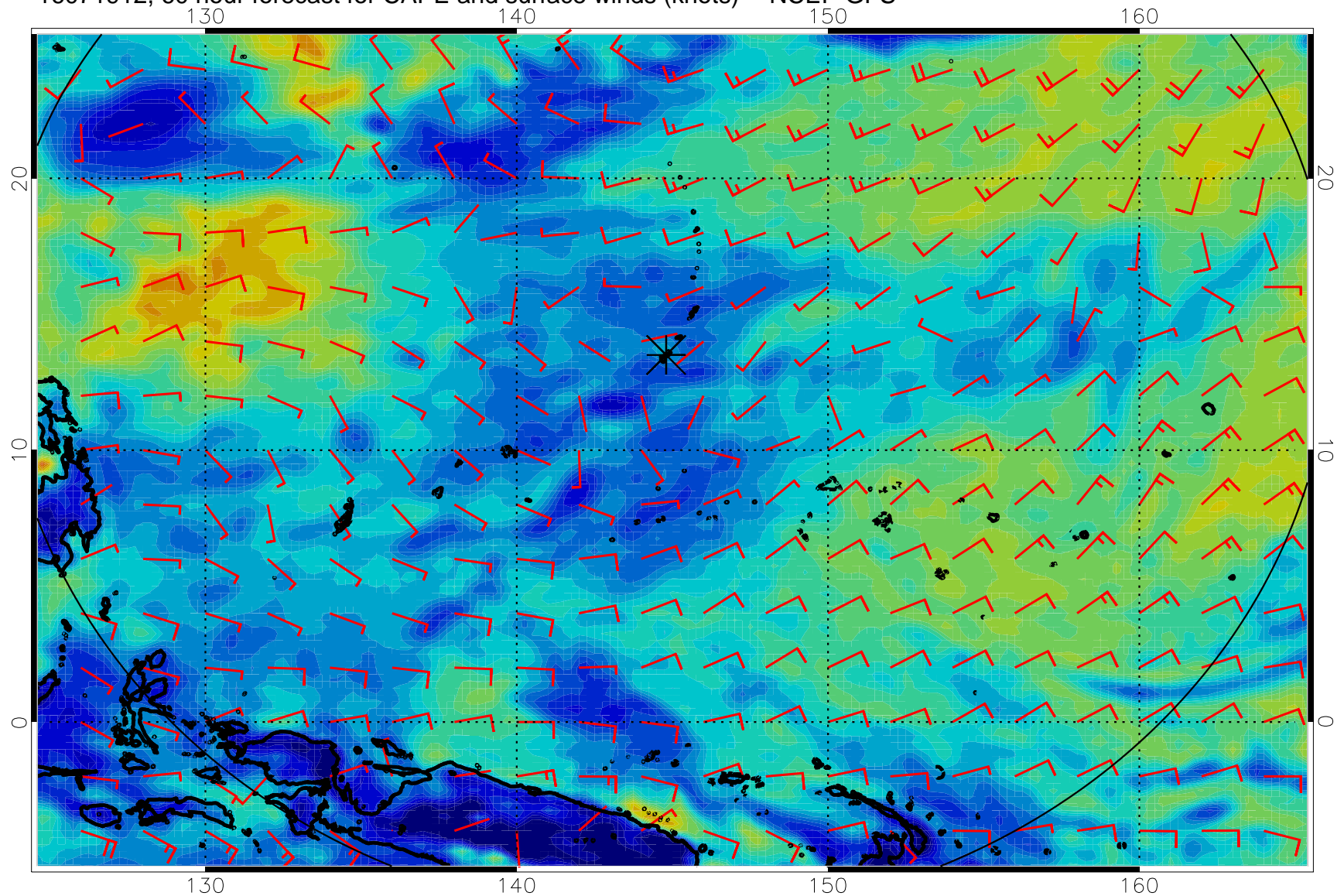
16071912, 60 hour forecast for CAPE and surface winds (knots) -- NCEP GFS
