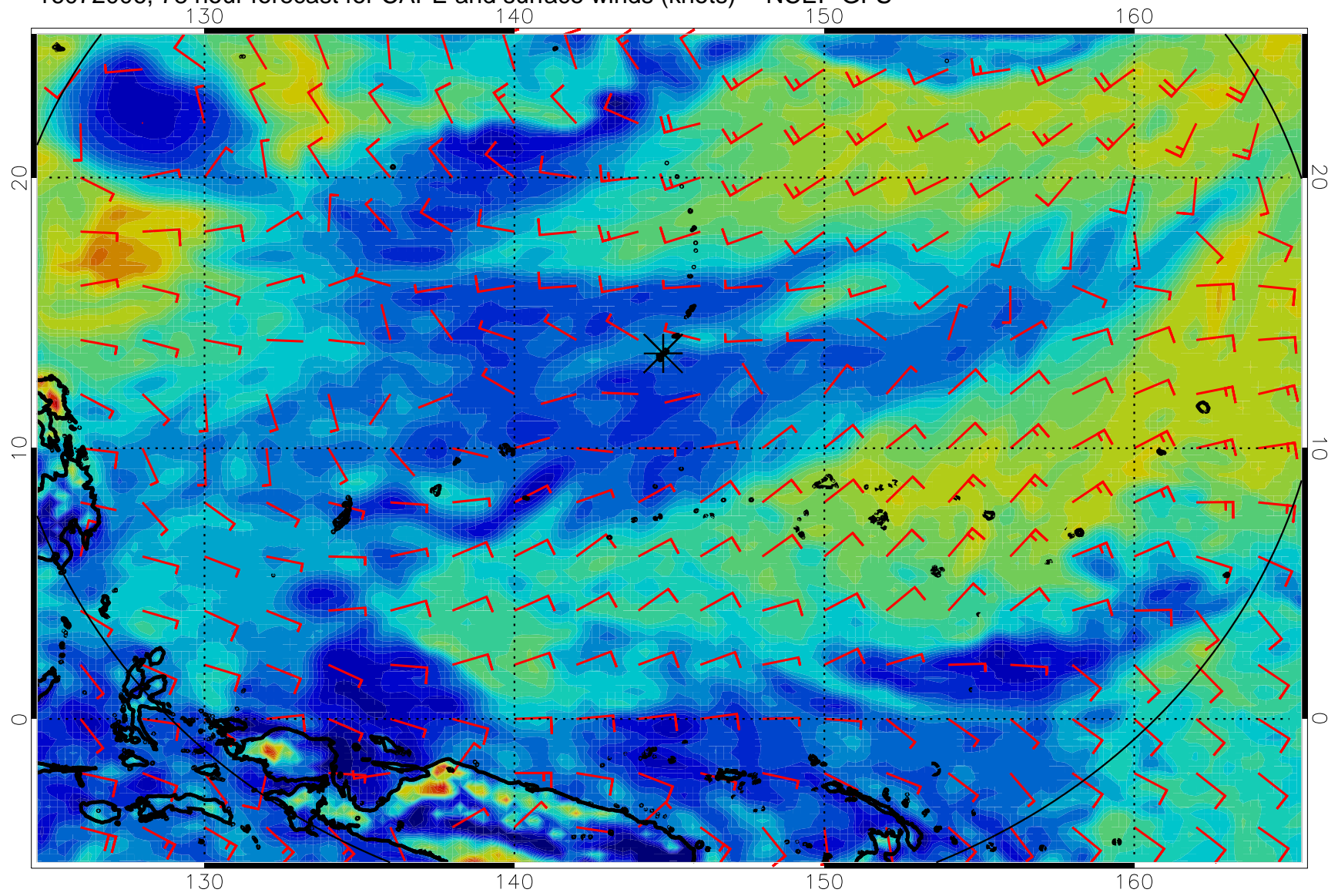
16072006, 78 hour forecast for CAPE and surface winds (knots) -- NCEP GFS
