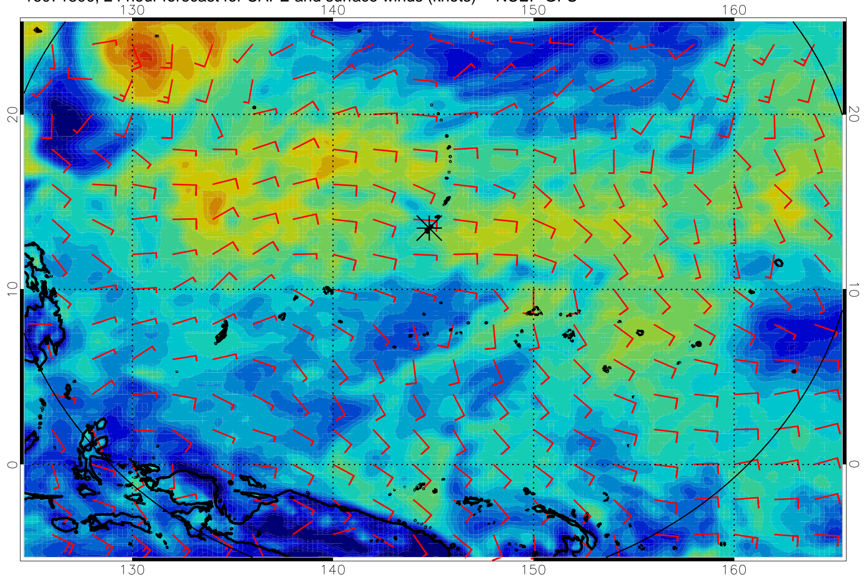
16071800, 24 hour forecast for CAPE and surface winds (knots) -- NCEP GFS
