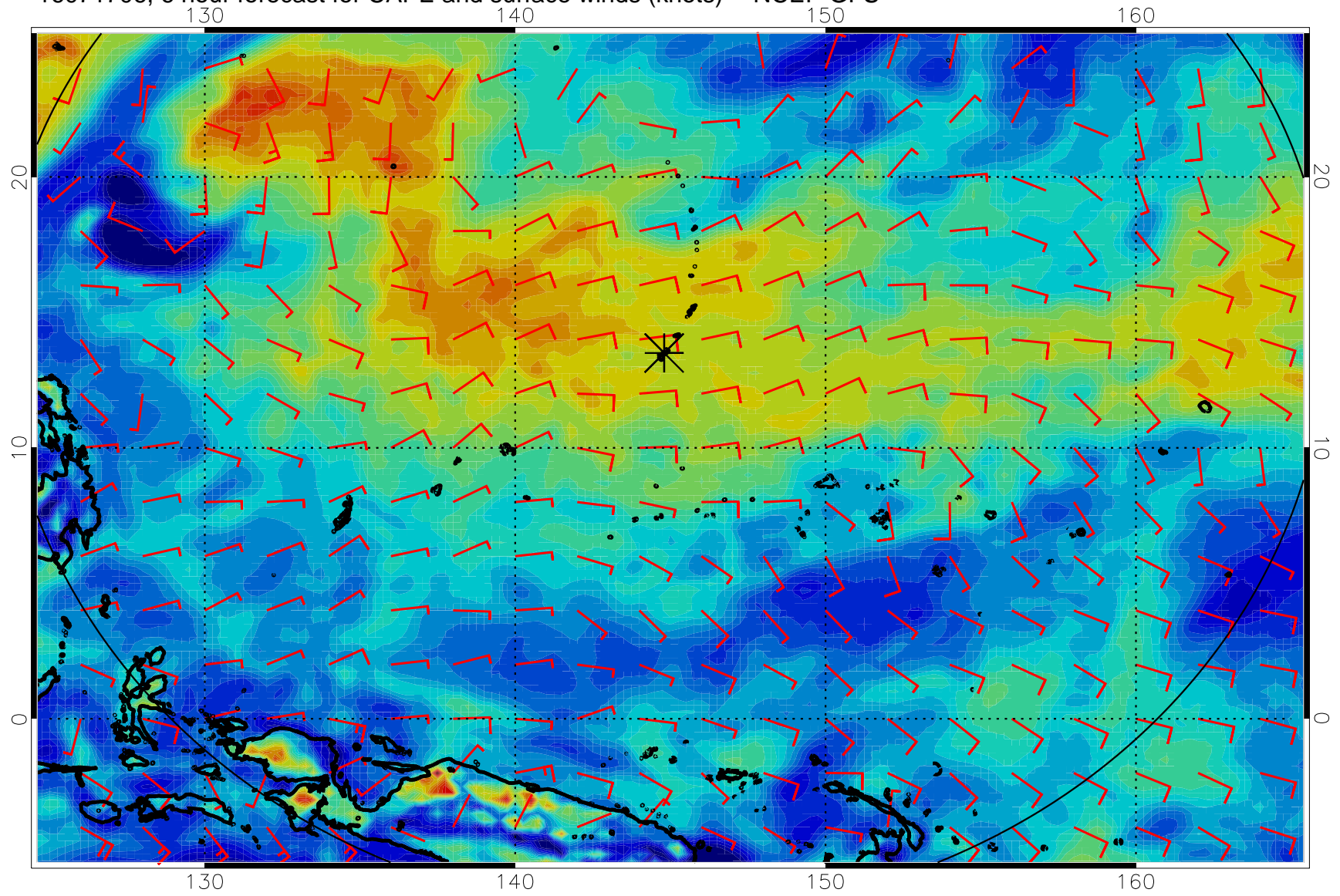
16071706, 6 hour forecast for CAPE and surface winds (knots) -- NCEP GFS
