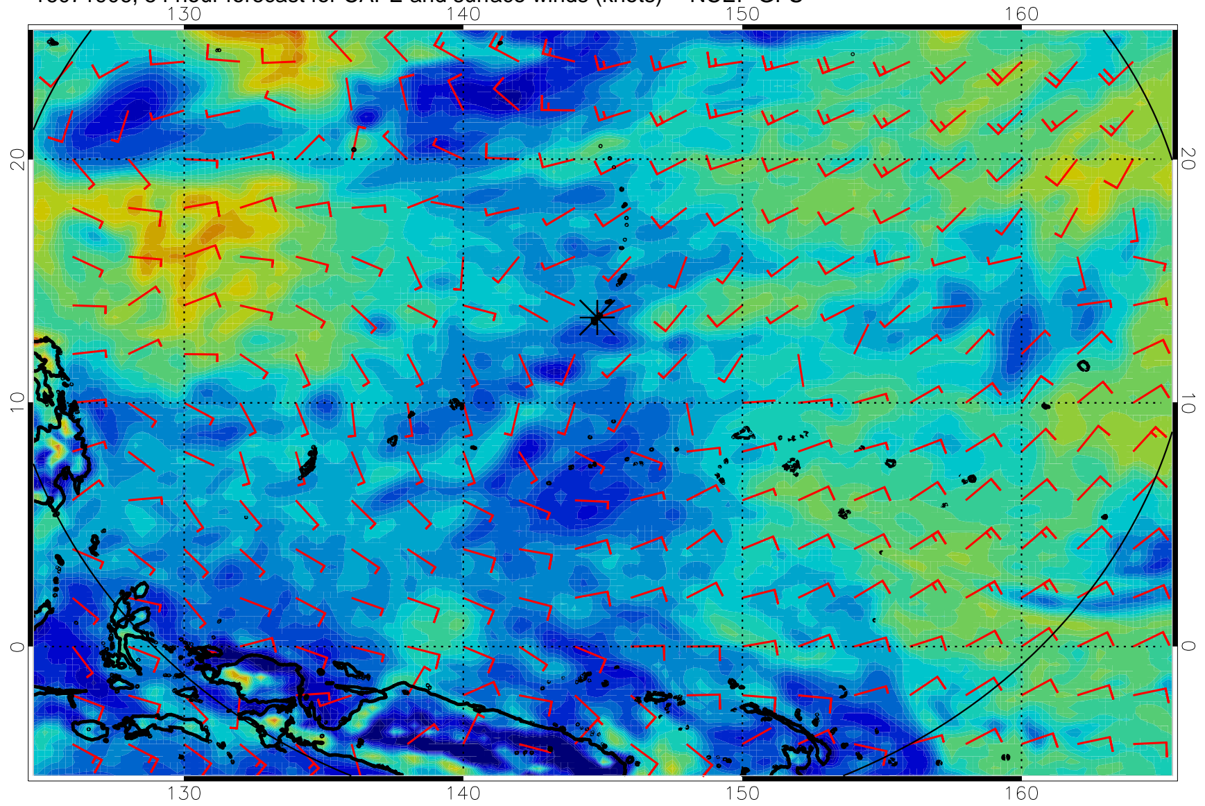
16071906, 54 hour forecast for CAPE and surface winds (knots) -- NCEP GFS
