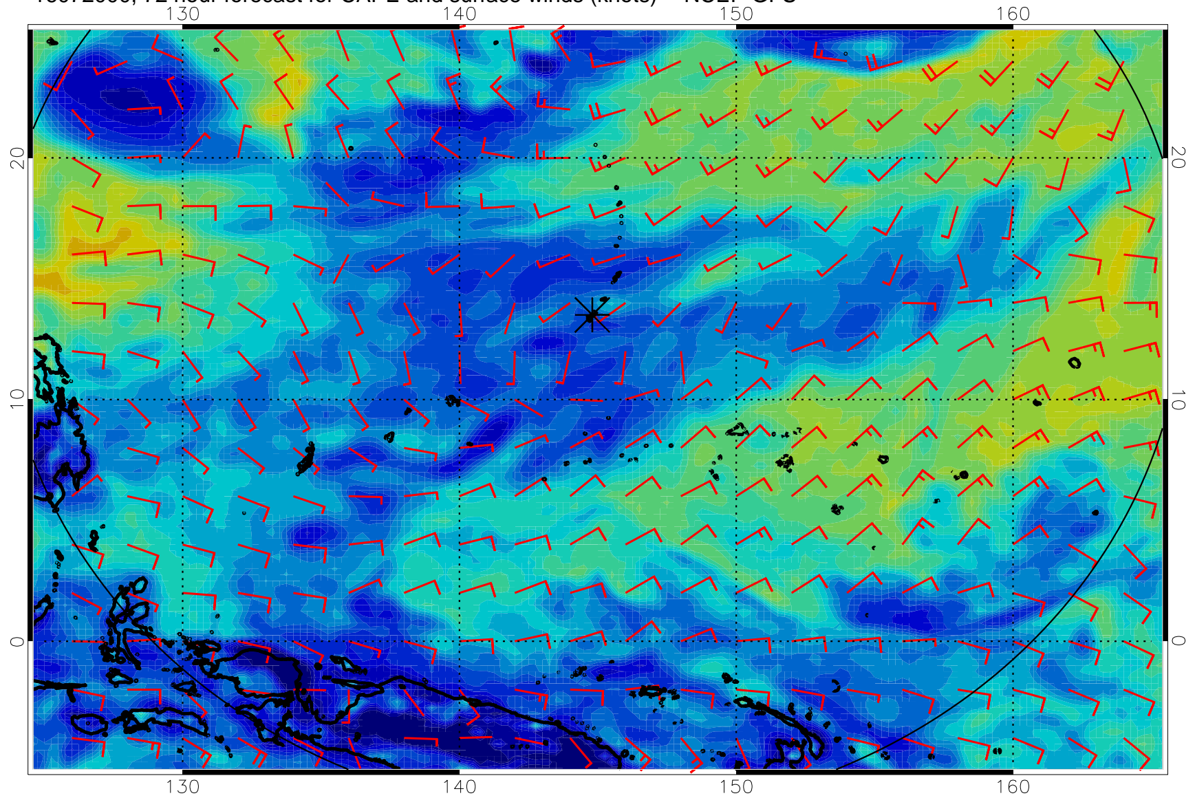
16072000, 72 hour forecast for CAPE and surface winds (knots) -- NCEP GFS
