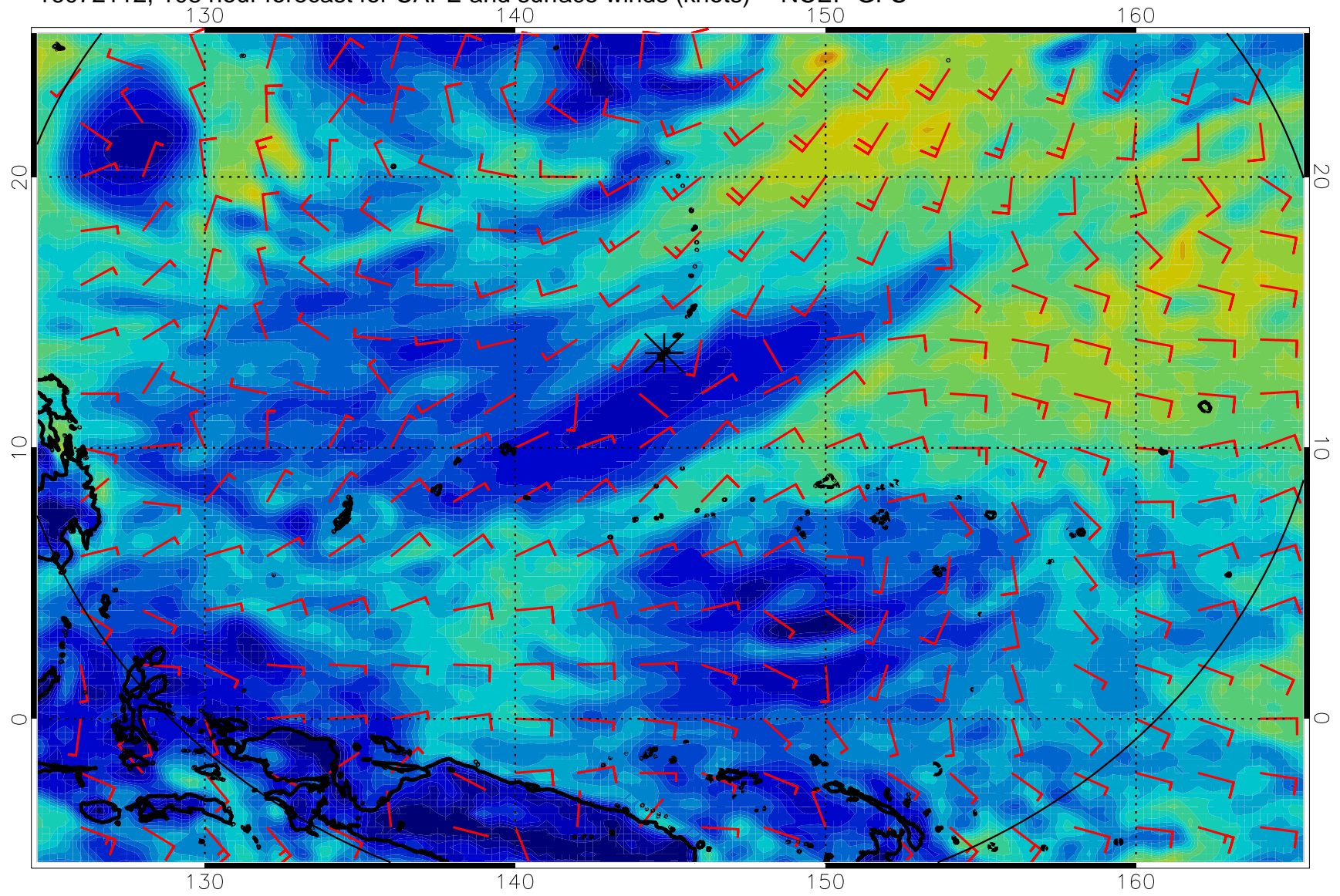
16072112, 108 hour forecast for CAPE and surface winds (knots) -- NCEP GFS
