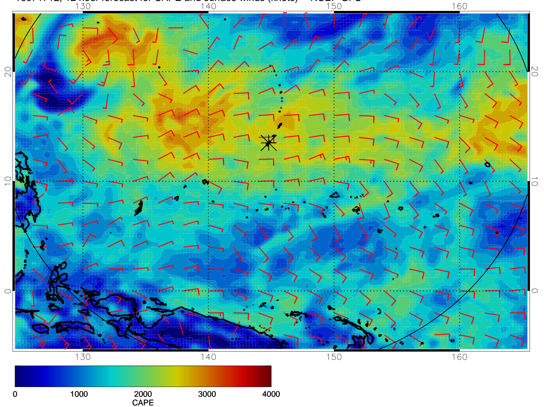
16071712, 12 hour forecast for CAPE and surface winds (knots) -- NCEP GFS
