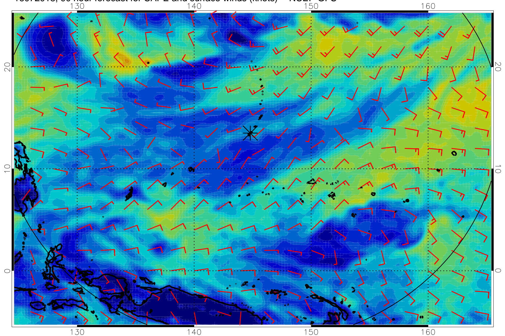
16072018, 90 hour forecast for CAPE and surface winds (knots) -- NCEP GFS
