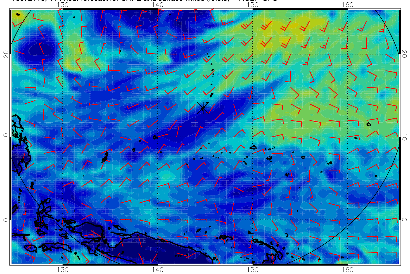
16072118, 114 hour forecast for CAPE and surface winds (knots) -- NCEP GFS
