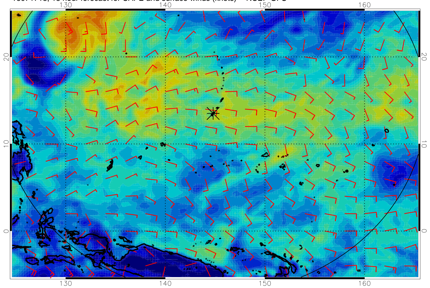
16071718, 18 hour forecast for CAPE and surface winds (knots) -- NCEP GFS
