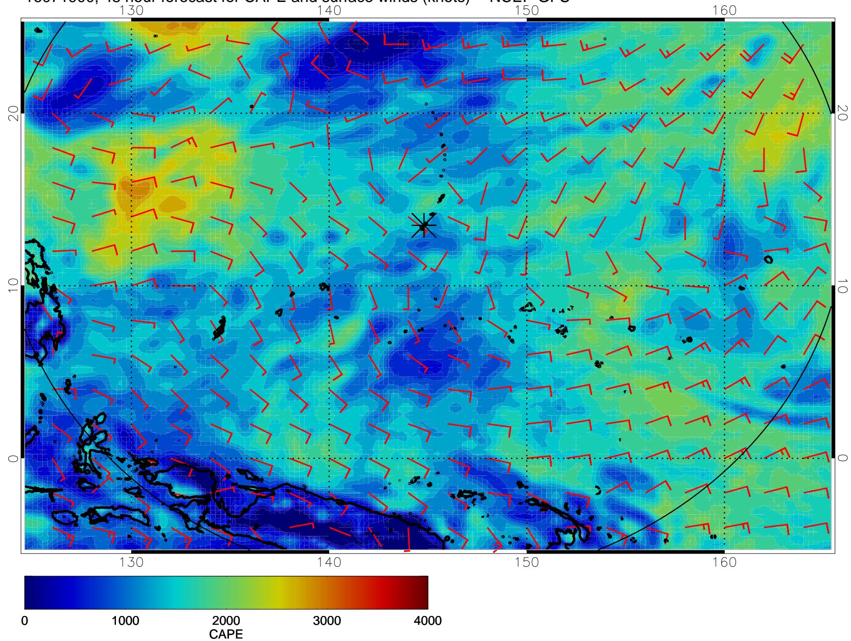
16071900, 48 hour forecast for CAPE and surface winds (knots) -- NCEP GFS
