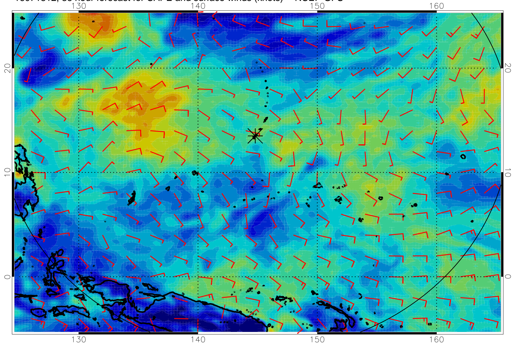
16071812, 36 hour forecast for CAPE and surface winds (knots) -- NCEP GFS
