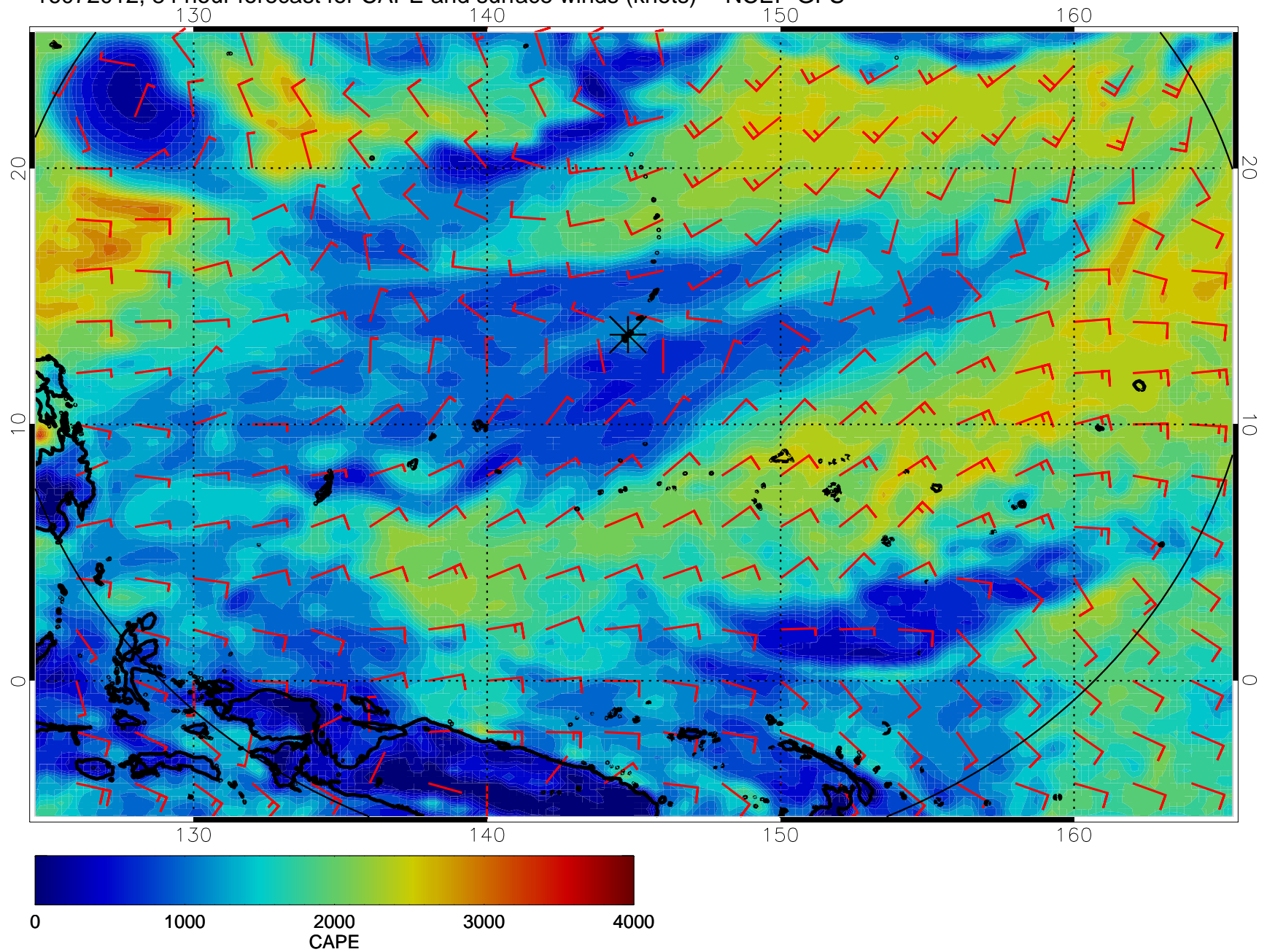
16072012, 84 hour forecast for CAPE and surface winds (knots) -- NCEP GFS
