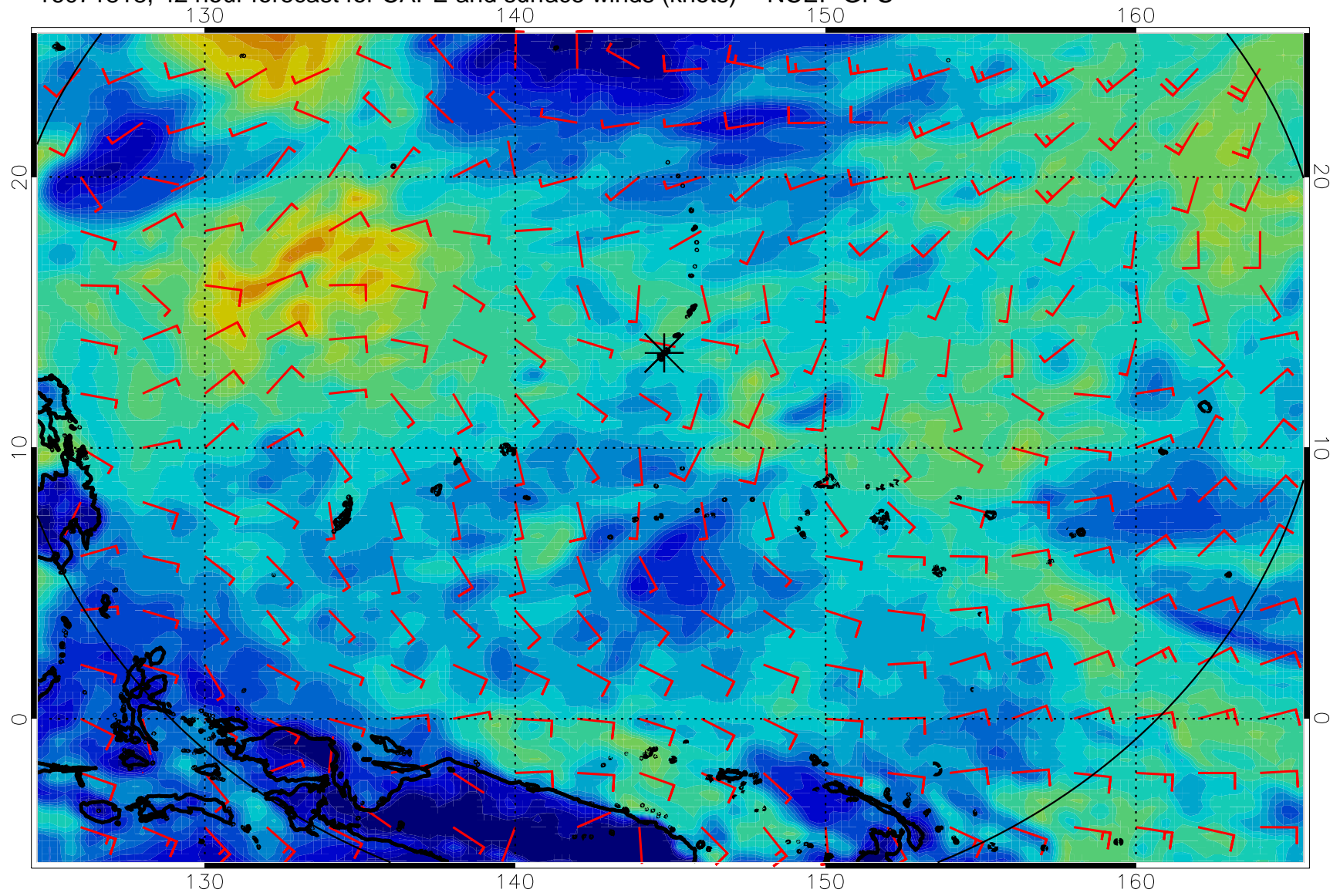
16071818, 42 hour forecast for CAPE and surface winds (knots) -- NCEP GFS
