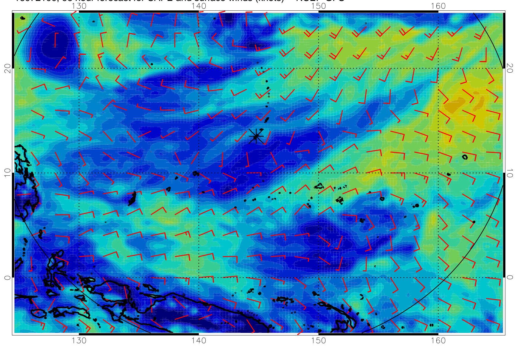
16072100, 96 hour forecast for CAPE and surface winds (knots) -- NCEP GFS
