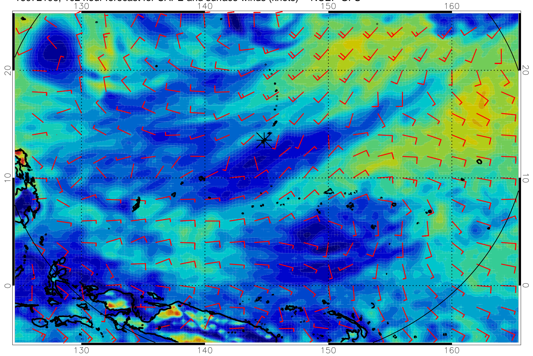
16072106, 102 hour forecast for CAPE and surface winds (knots) -- NCEP GFS
