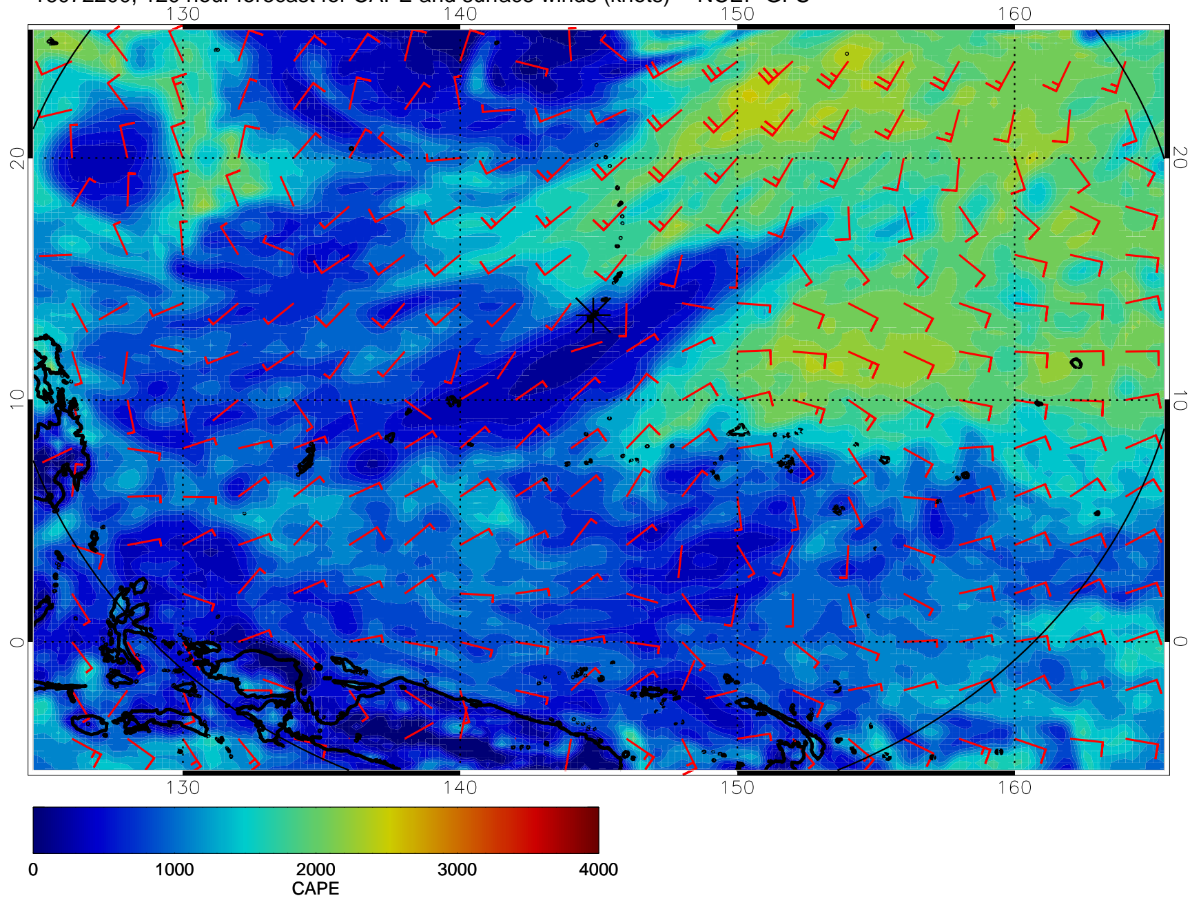
16072200, 120 hour forecast for CAPE and surface winds (knots) -- NCEP GFS
