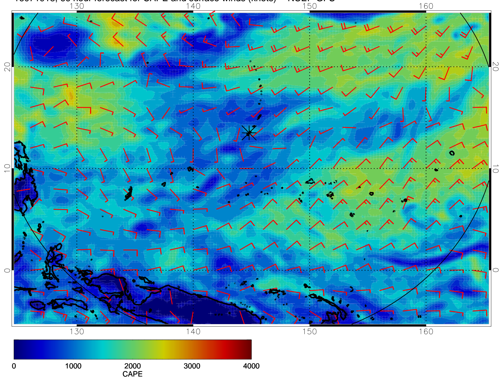
16071918, 66 hour forecast for CAPE and surface winds (knots) -- NCEP GFS
