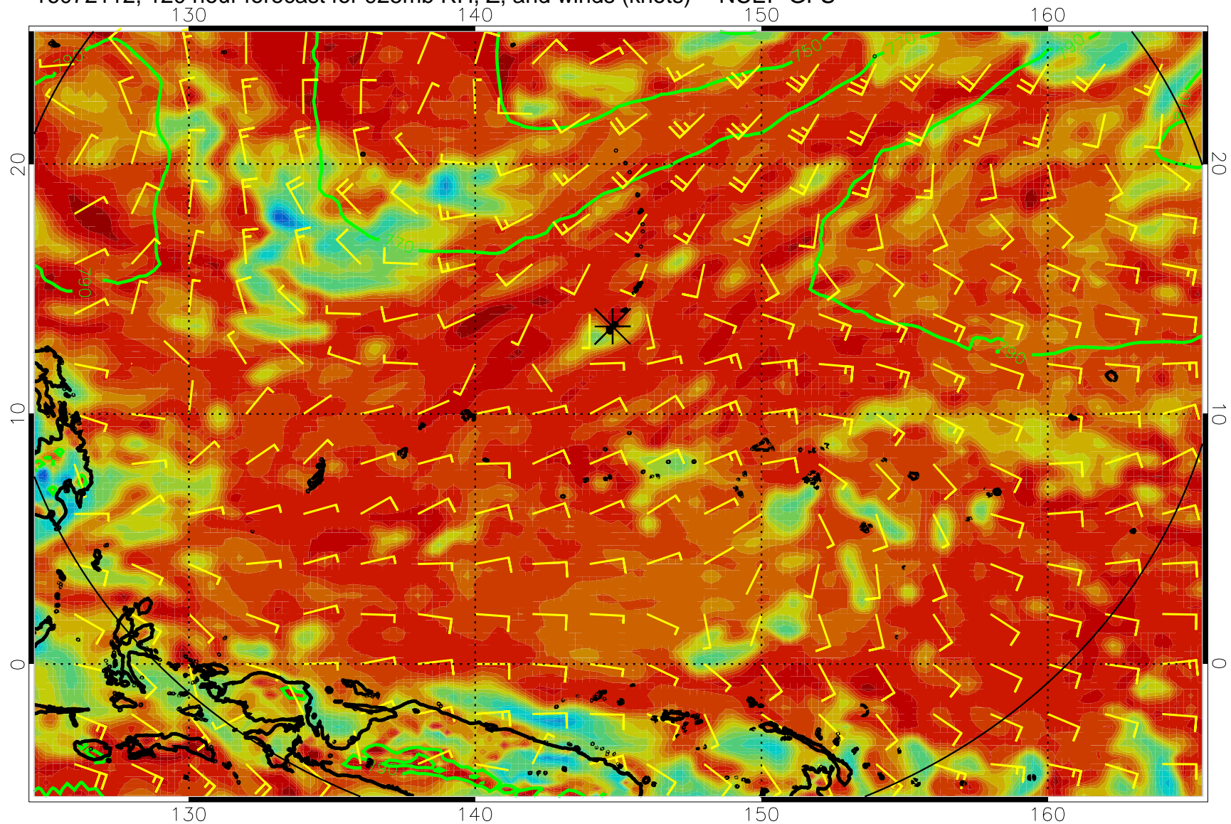
16072112, 120 hour forecast for 925mb RH, Z, and winds (knots) -- NCEP GFS
