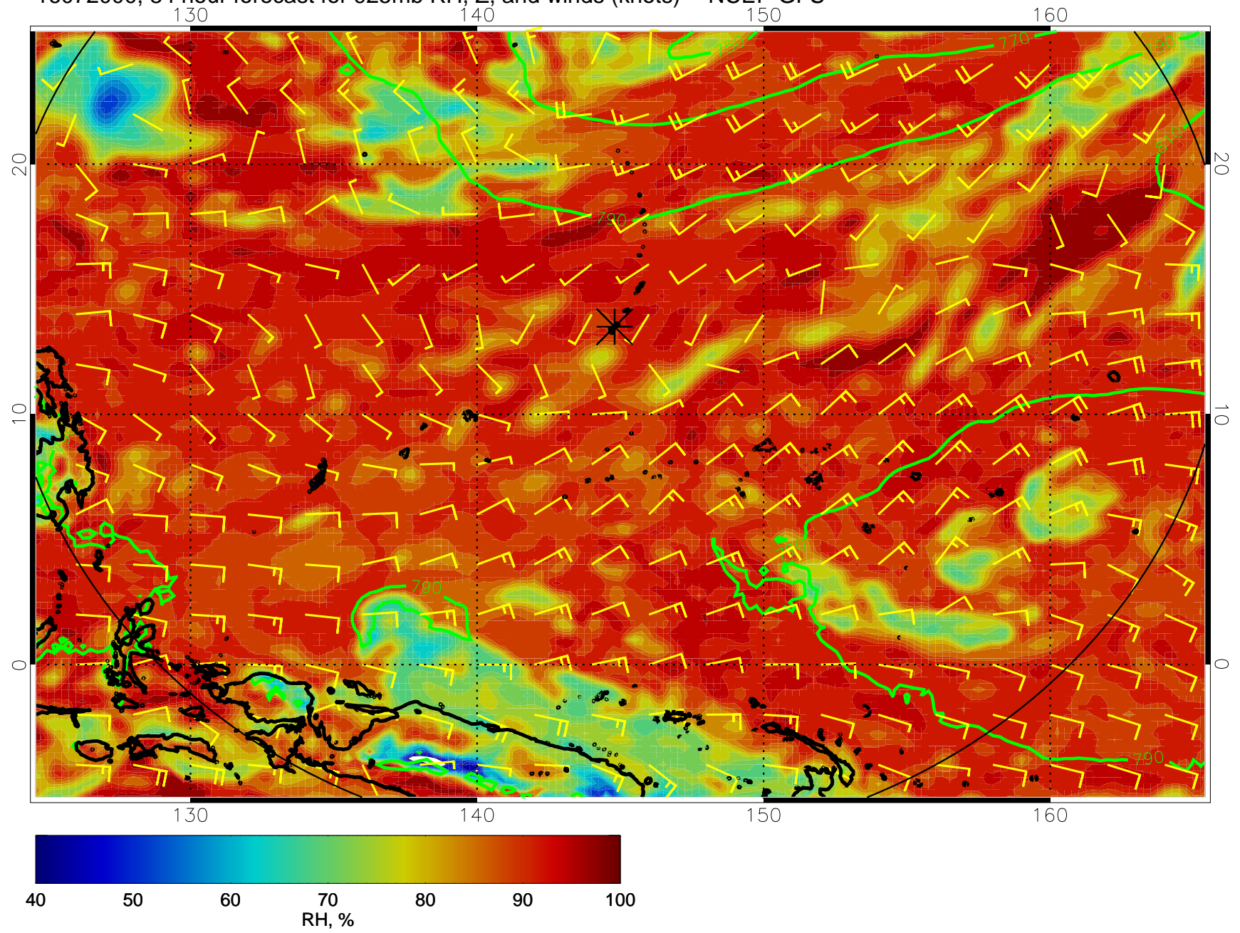
16072000, 84 hour forecast for 925mb RH, Z, and winds (knots) -- NCEP GFS
