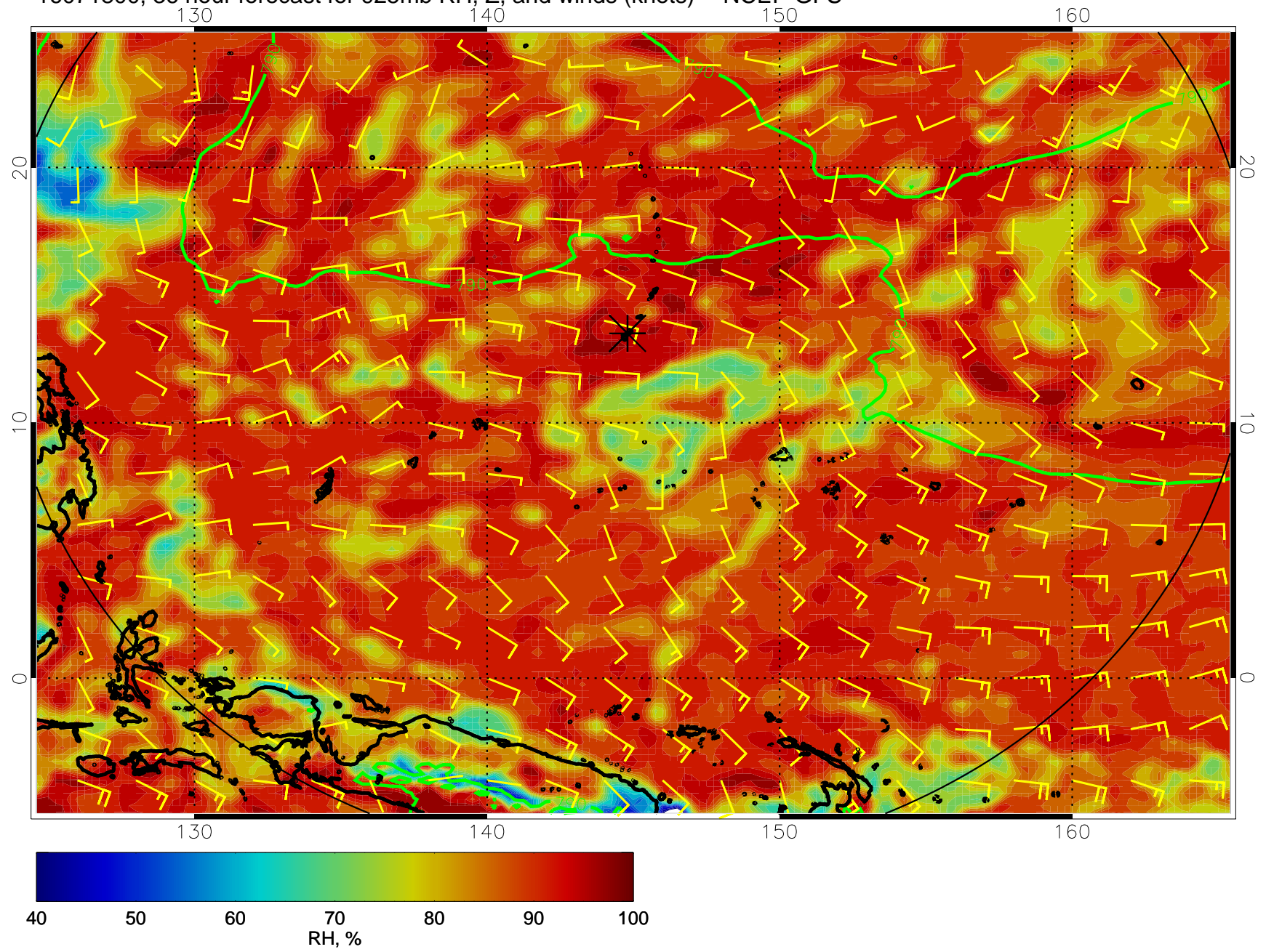
16071800, 36 hour forecast for 925mb RH, Z, and winds (knots) -- NCEP GFS
