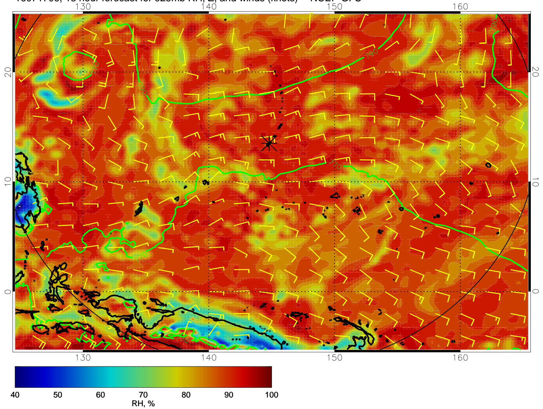
16071706, 18 hour forecast for 925mb RH, Z, and winds (knots) -- NCEP GFS
