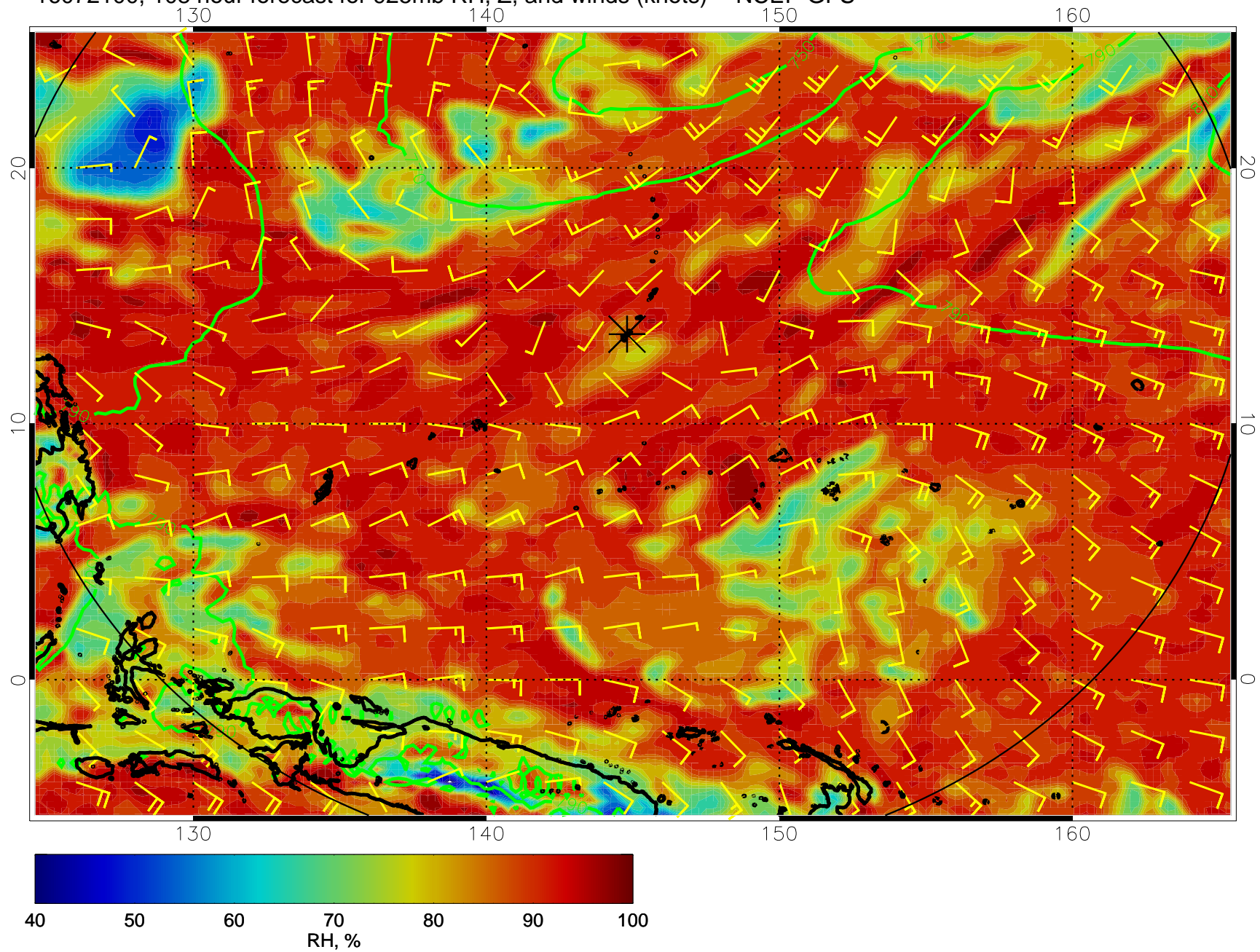
16072100, 108 hour forecast for 925mb RH, Z, and winds (knots) -- NCEP GFS
