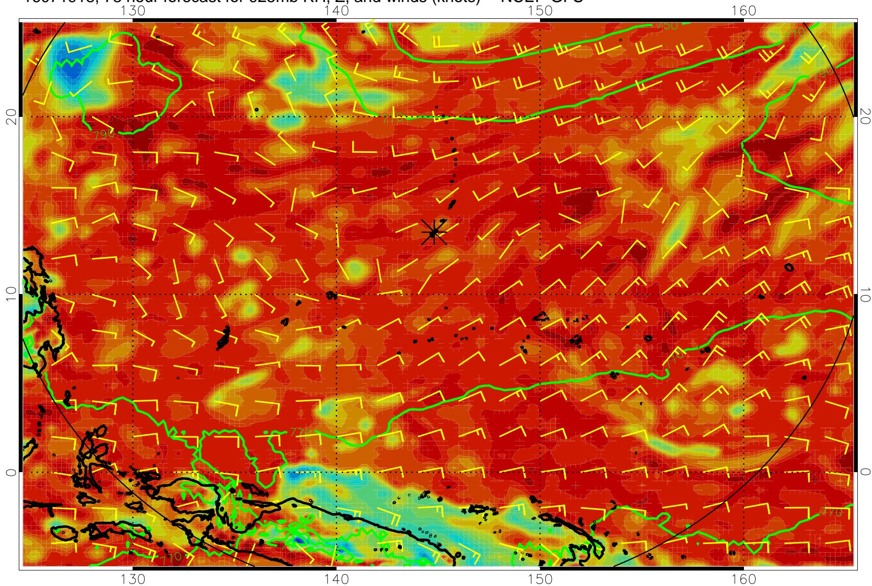
16071918, 78 hour forecast for 925mb RH, Z, and winds (knots) -- NCEP GFS
