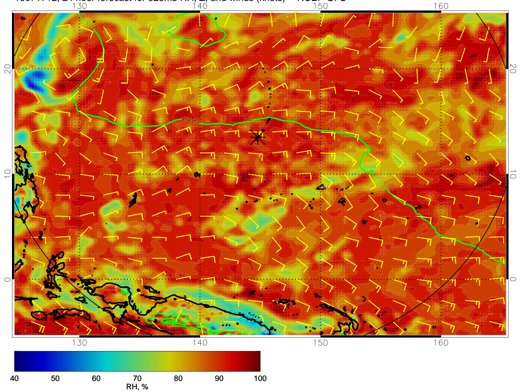
16071712, 24 hour forecast for 925mb RH, Z, and winds (knots) -- NCEP GFS
