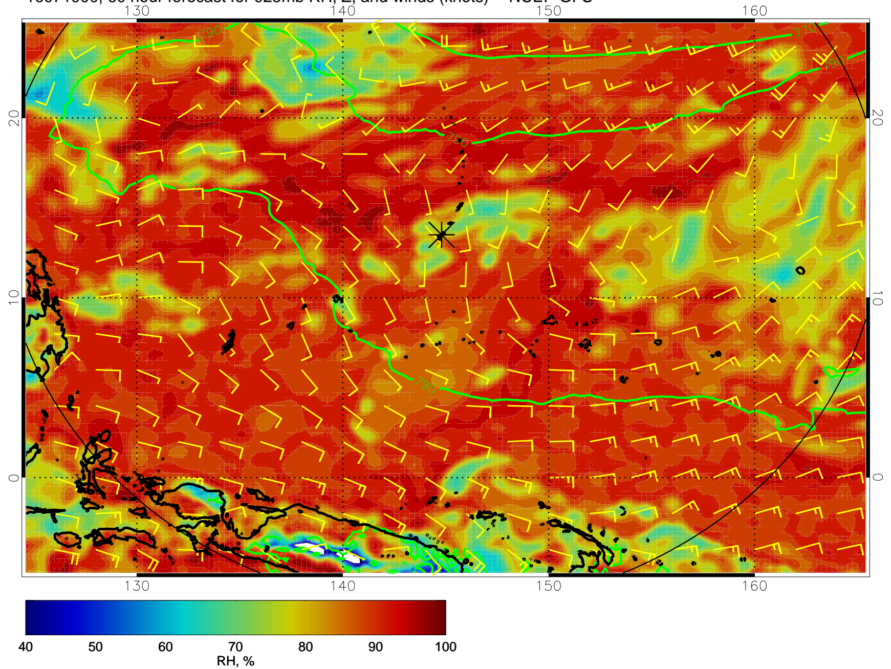
16071900, 60 hour forecast for 925mb RH, Z, and winds (knots) -- NCEP GFS
