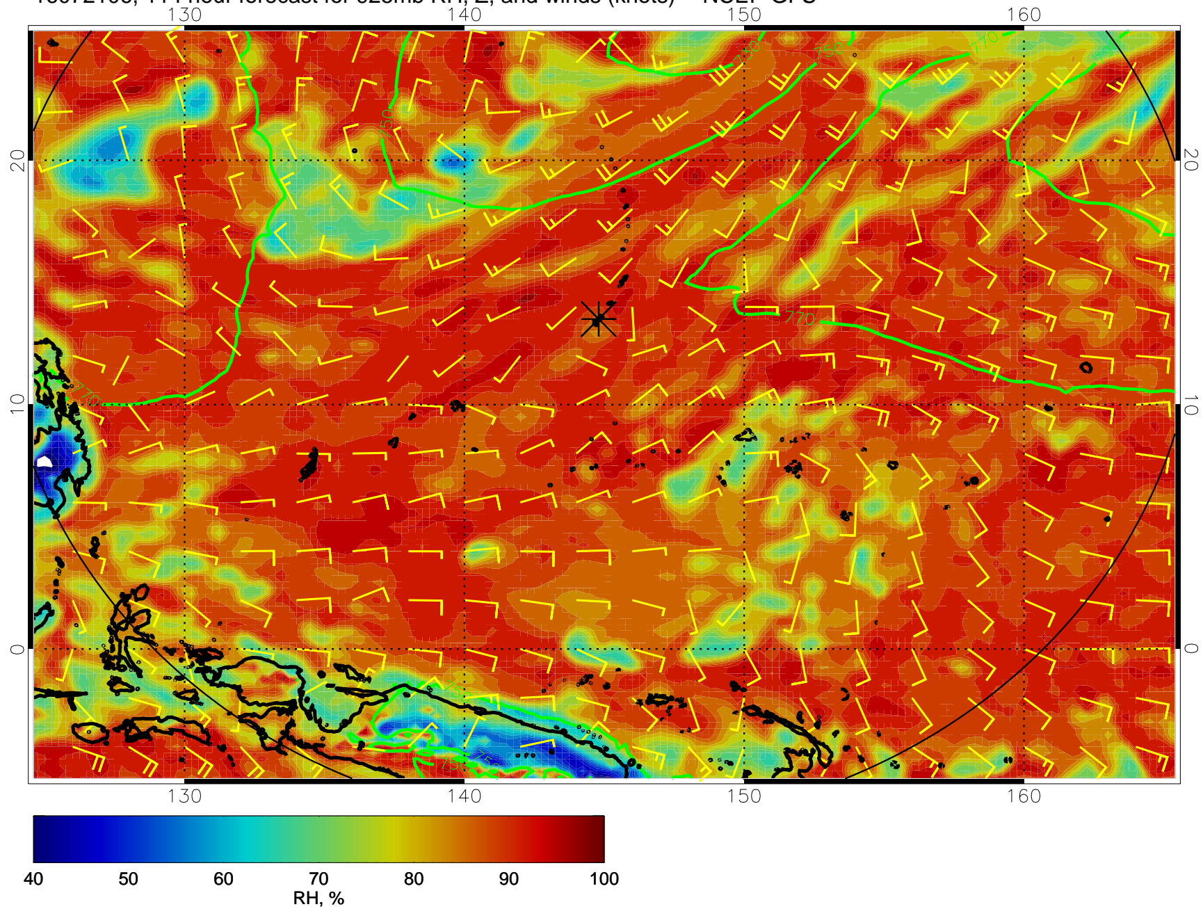
16072106, 114 hour forecast for 925mb RH, Z, and winds (knots) -- NCEP GFS
