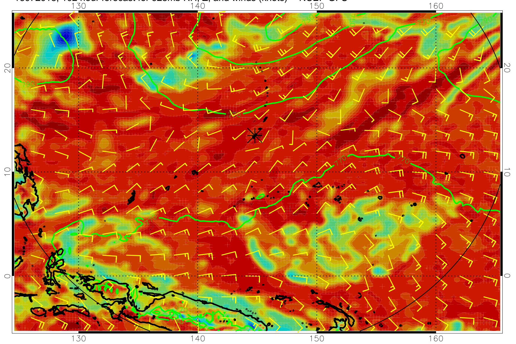
16072018, 102 hour forecast for 925mb RH, Z, and winds (knots) -- NCEP GFS
