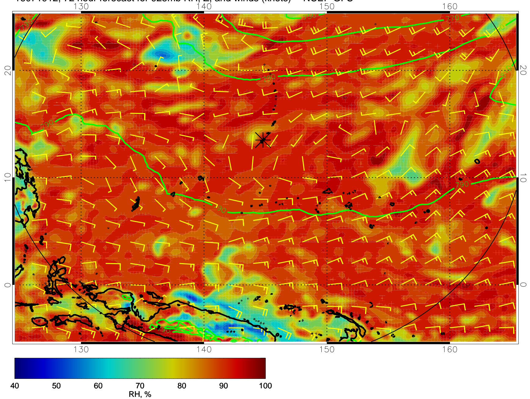
16071912, 72 hour forecast for 925mb RH, Z, and winds (knots) -- NCEP GFS
