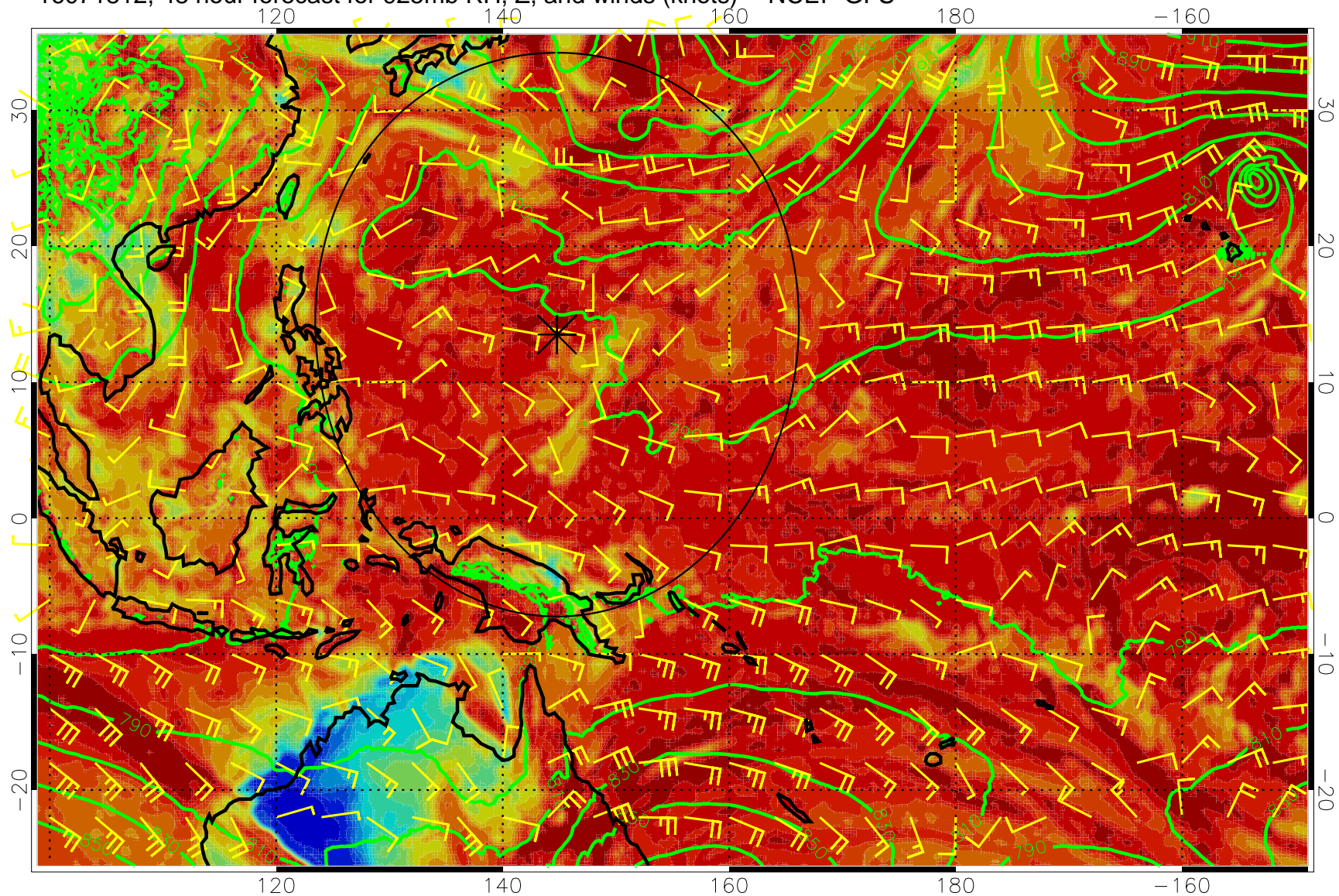
16071812, 48 hour forecast for 925mb RH, Z, and winds (knots) -- NCEP GFS
