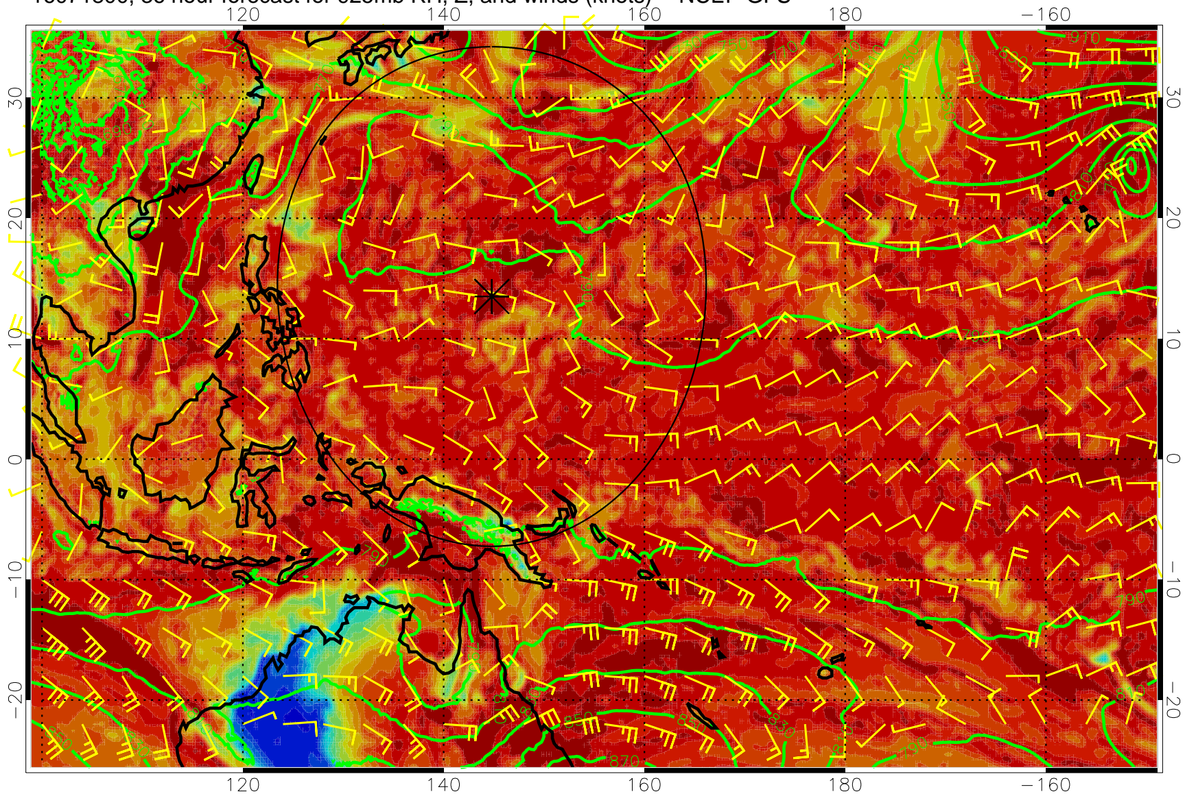
16071800, 36 hour forecast for 925mb RH, Z, and winds (knots) -- NCEP GFS
