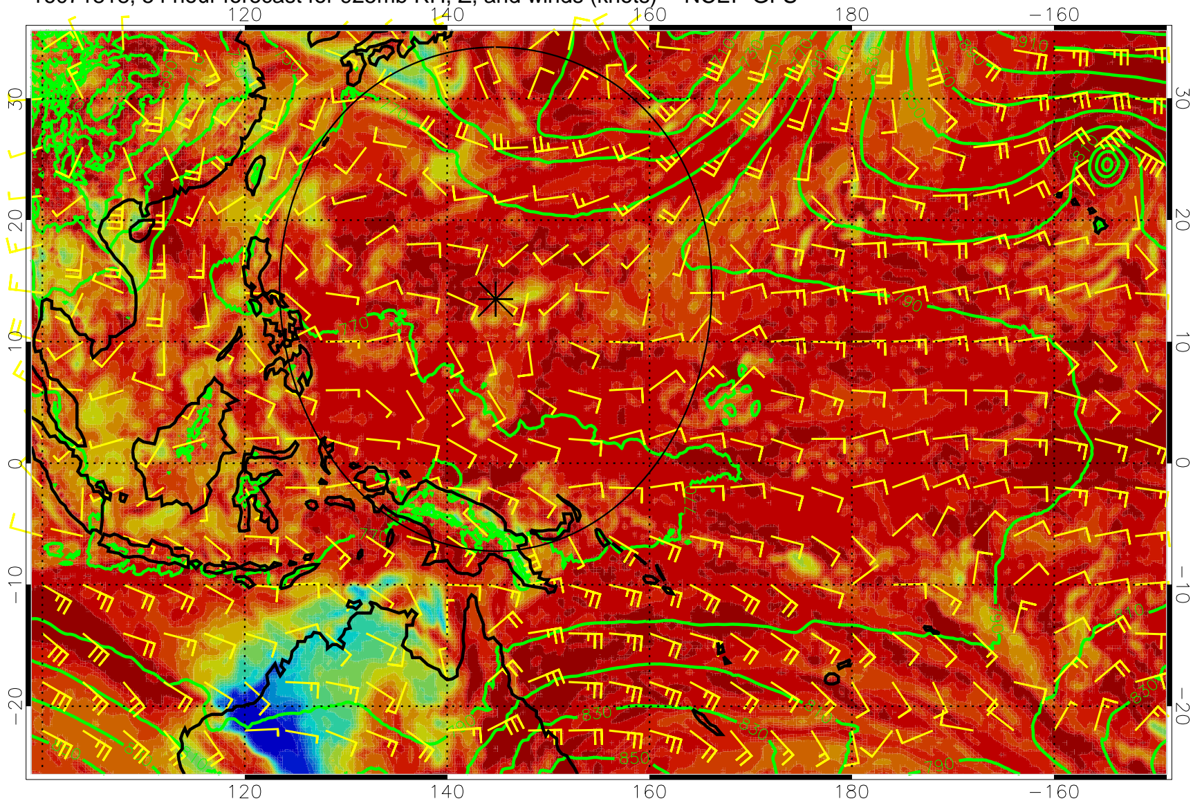
16071818, 54 hour forecast for 925mb RH, Z, and winds (knots) -- NCEP GFS
