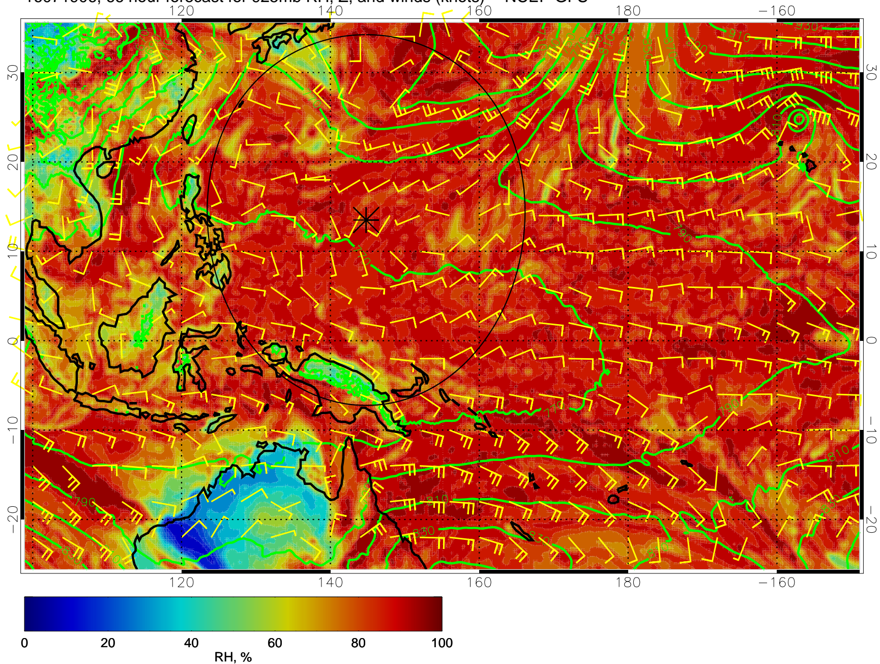
16071906, 66 hour forecast for 925mb RH, Z, and winds (knots) -- NCEP GFS
