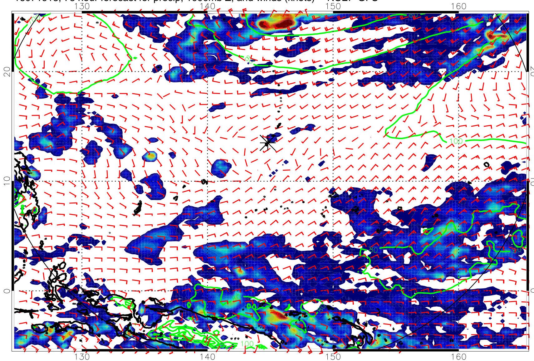
16071918, 78 hour forecast for precip, 1000mb Z, and winds (knots) -- NCEP GFS
