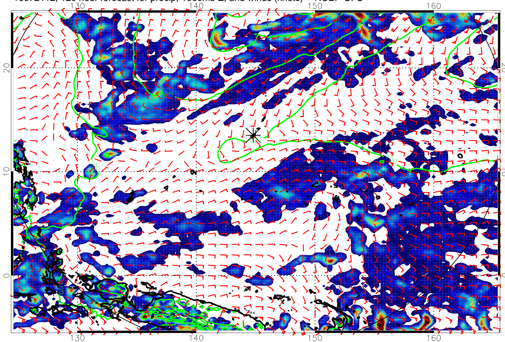
16072112, 120 hour forecast for precip, 1000mb Z, and winds (knots) -- NCEP GFS
