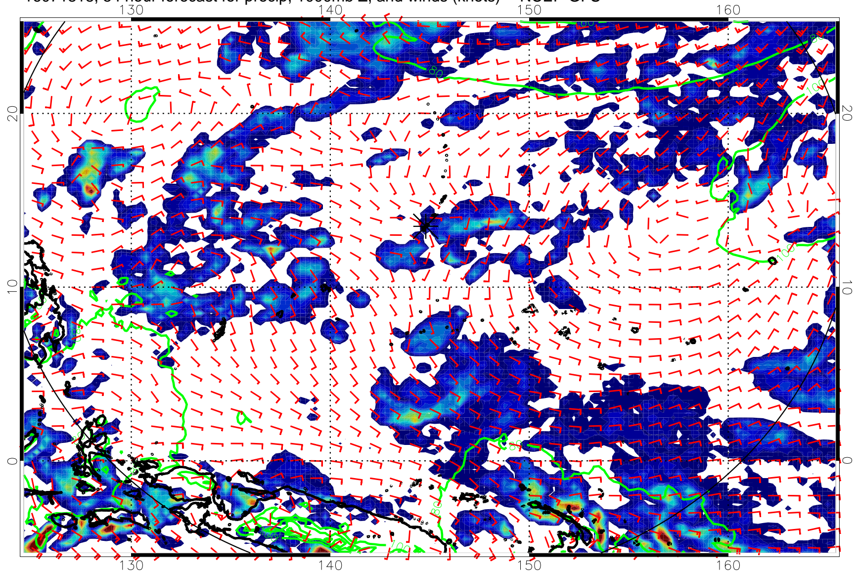
16071818, 54 hour forecast for precip, 1000mb Z, and winds (knots) -- NCEP GFS
