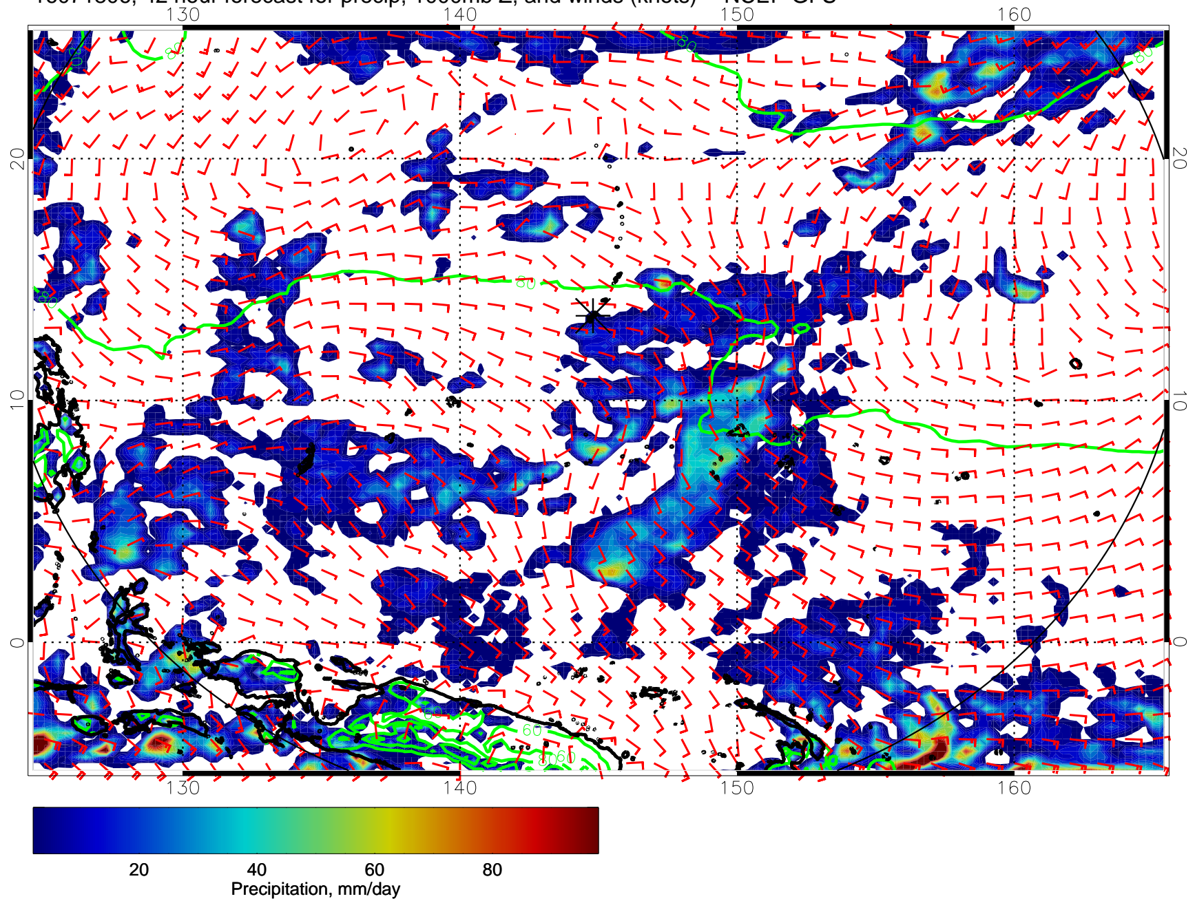
16071806, 42 hour forecast for precip, 1000mb Z, and winds (knots) -- NCEP GFS
