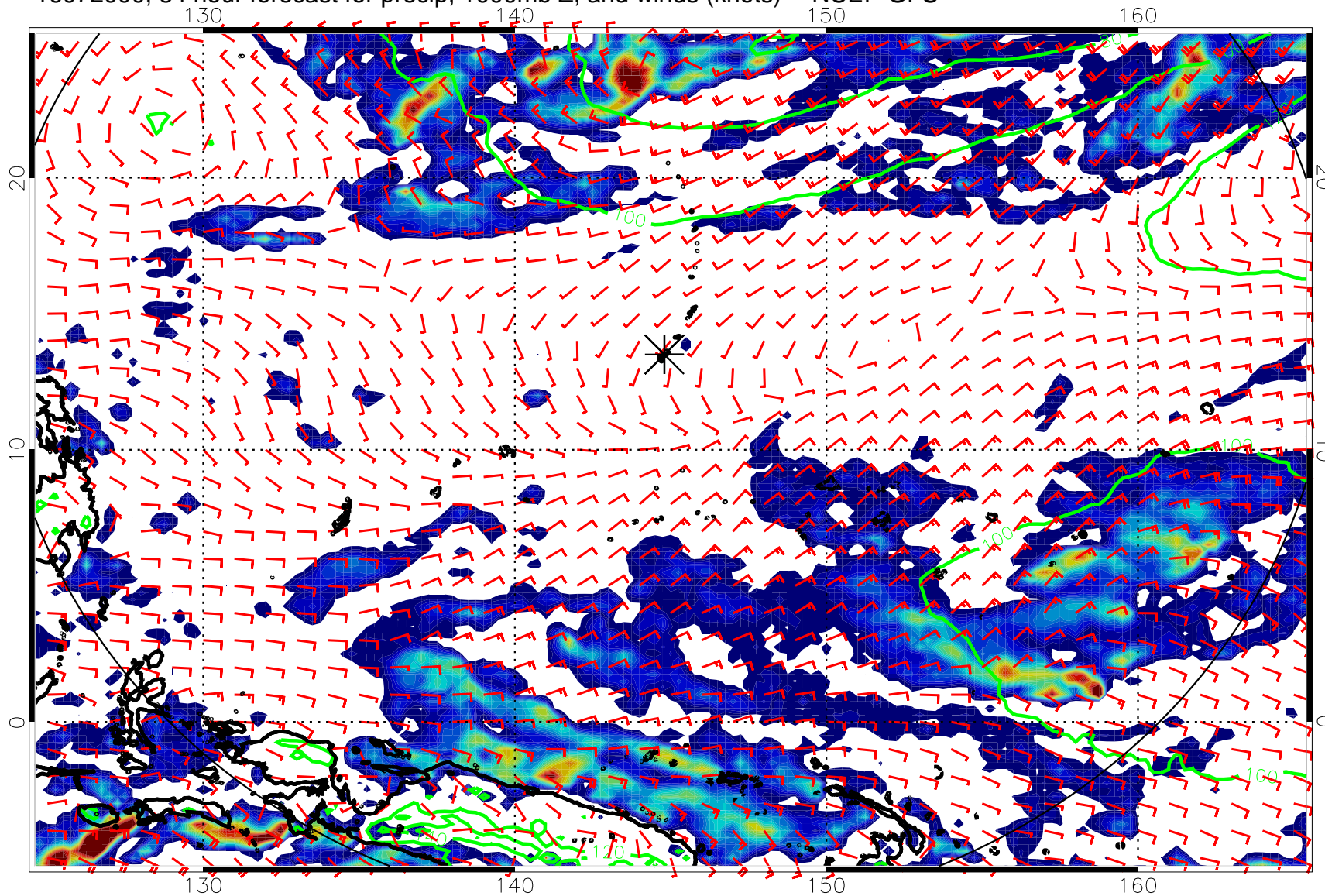
16072000, 84 hour forecast for precip, 1000mb Z, and winds (knots) -- NCEP GFS
