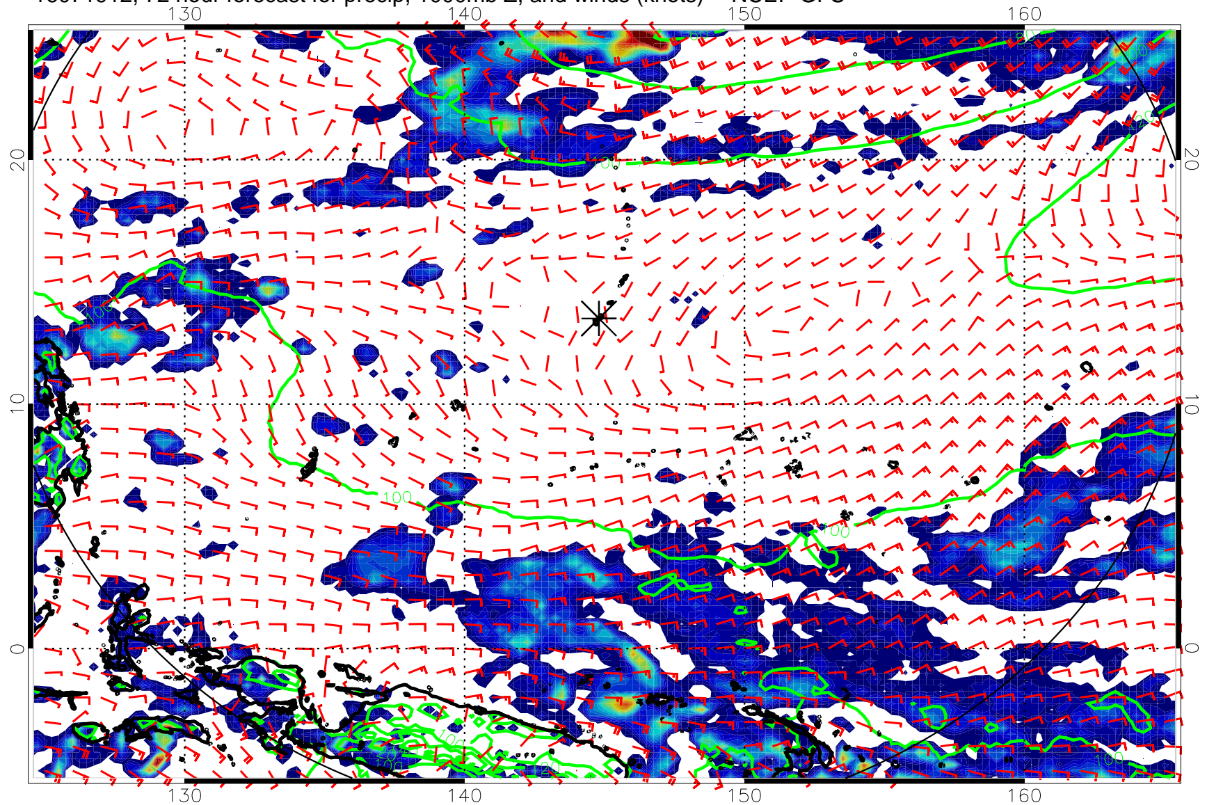
16071912, 72 hour forecast for precip, 1000mb Z, and winds (knots) -- NCEP GFS
