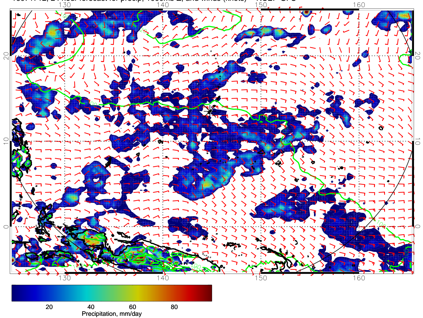
16071712, 24 hour forecast for precip, 1000mb Z, and winds (knots) -- NCEP GFS
