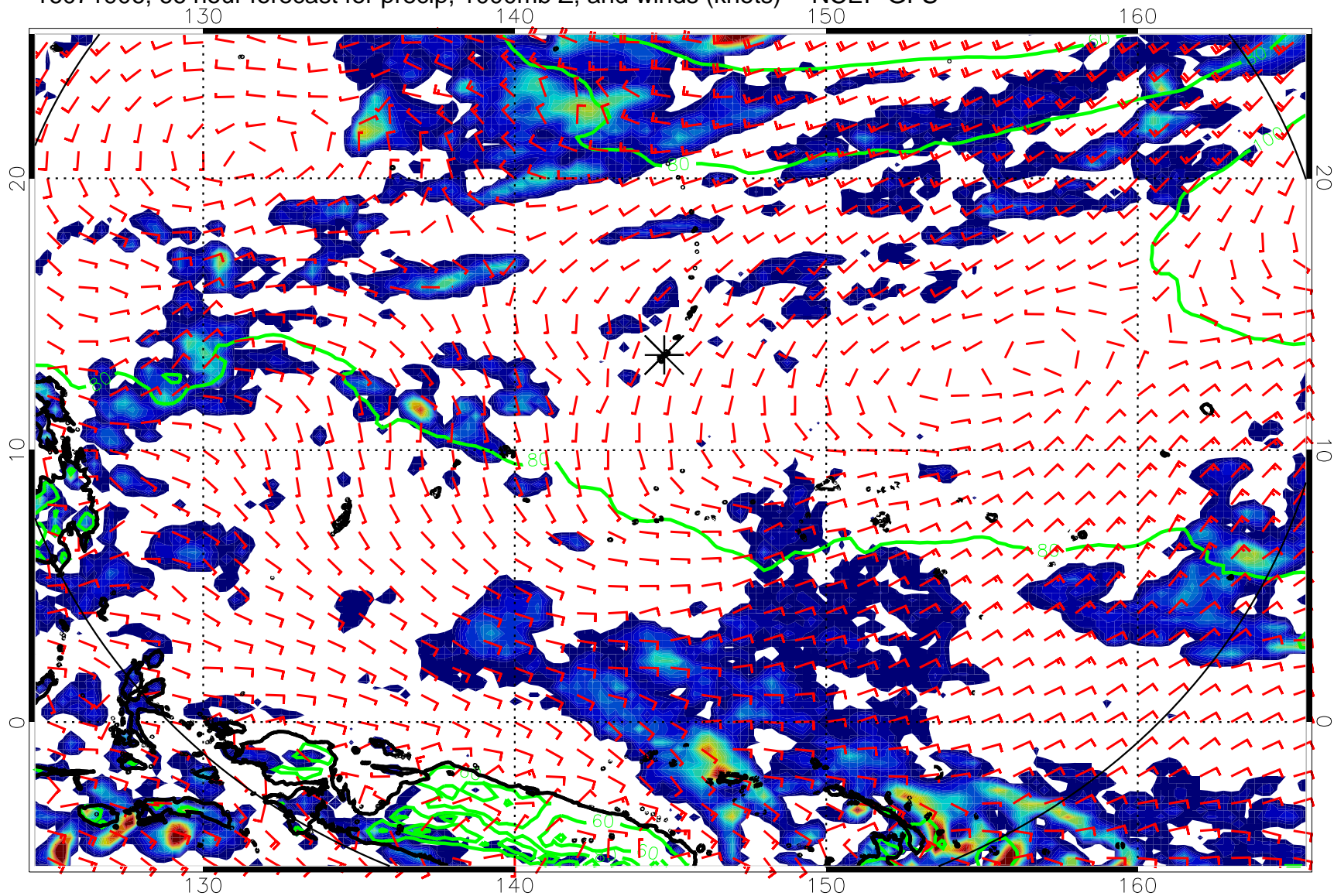
16071906, 66 hour forecast for precip, 1000mb Z, and winds (knots) -- NCEP GFS
