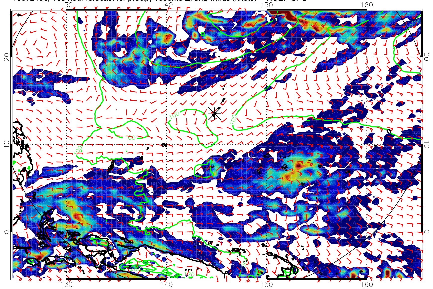
16072100, 108 hour forecast for precip, 1000mb Z, and winds (knots) -- NCEP GFS
