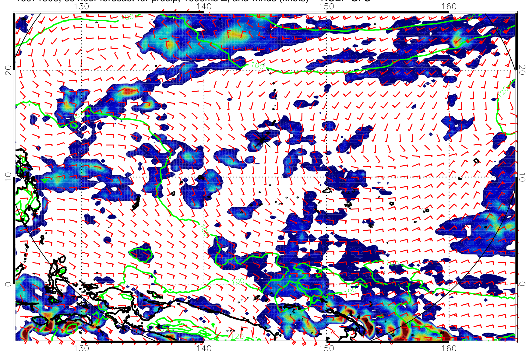
16071900, 60 hour forecast for precip, 1000mb Z, and winds (knots) -- NCEP GFS
