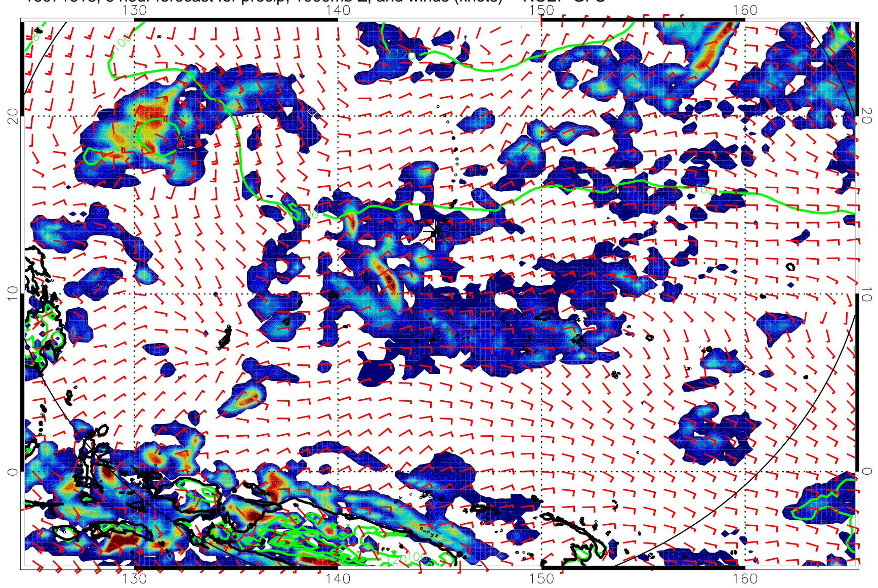
16071618, 6 hour forecast for precip, 1000mb Z, and winds (knots) -- NCEP GFS
