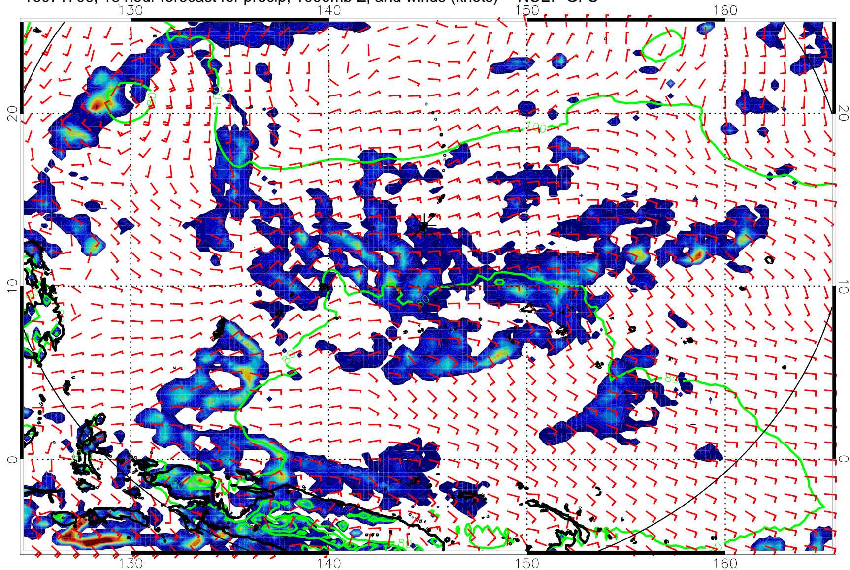
16071706, 18 hour forecast for precip, 1000mb Z, and winds (knots) -- NCEP GFS
