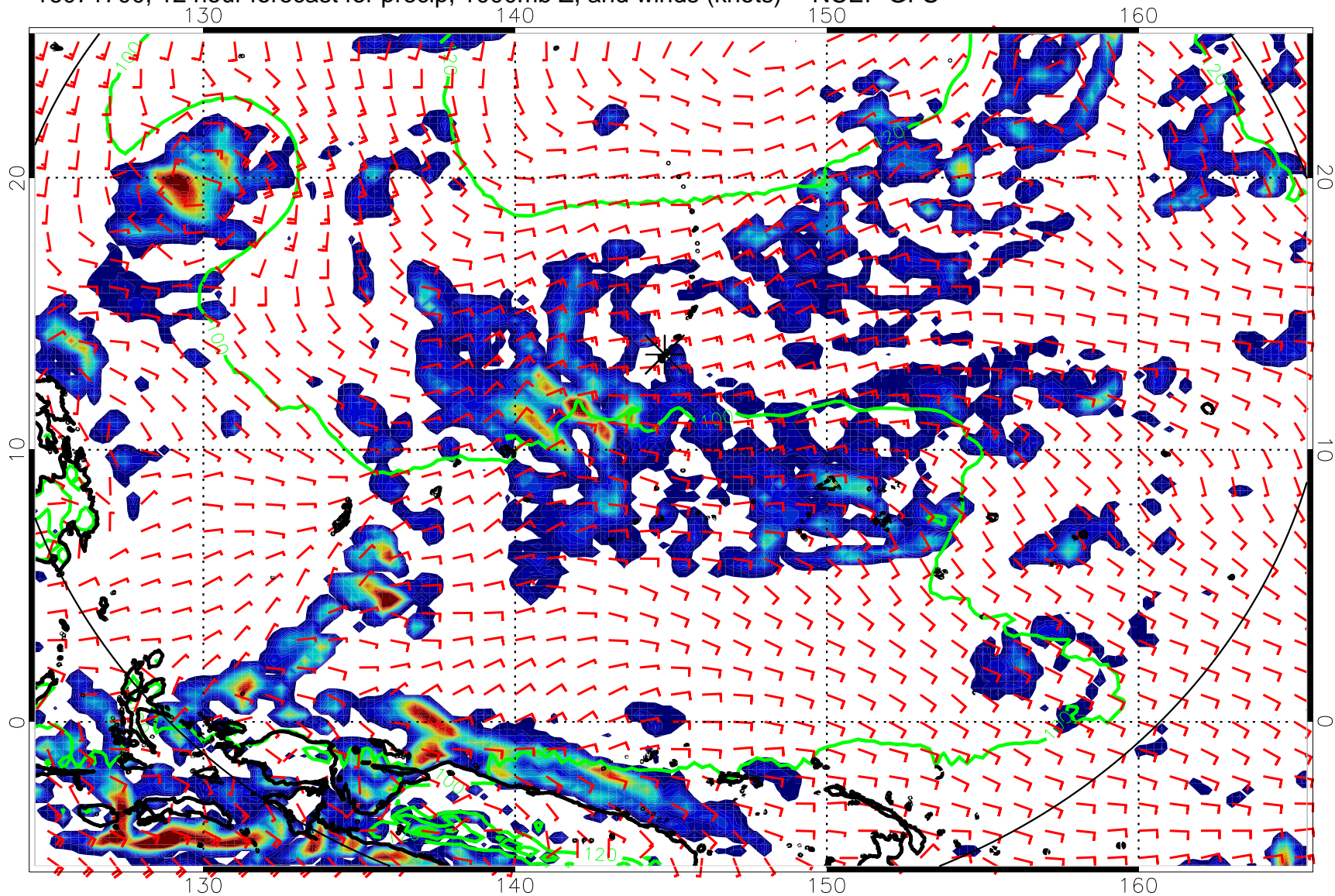
16071700, 12 hour forecast for precip, 1000mb Z, and winds (knots) -- NCEP GFS
