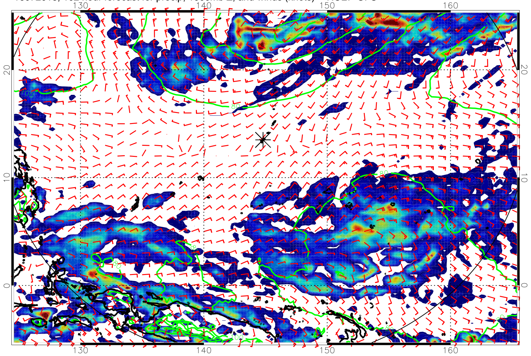
16072018, 102 hour forecast for precip, 1000mb Z, and winds (knots) -- NCEP GFS
