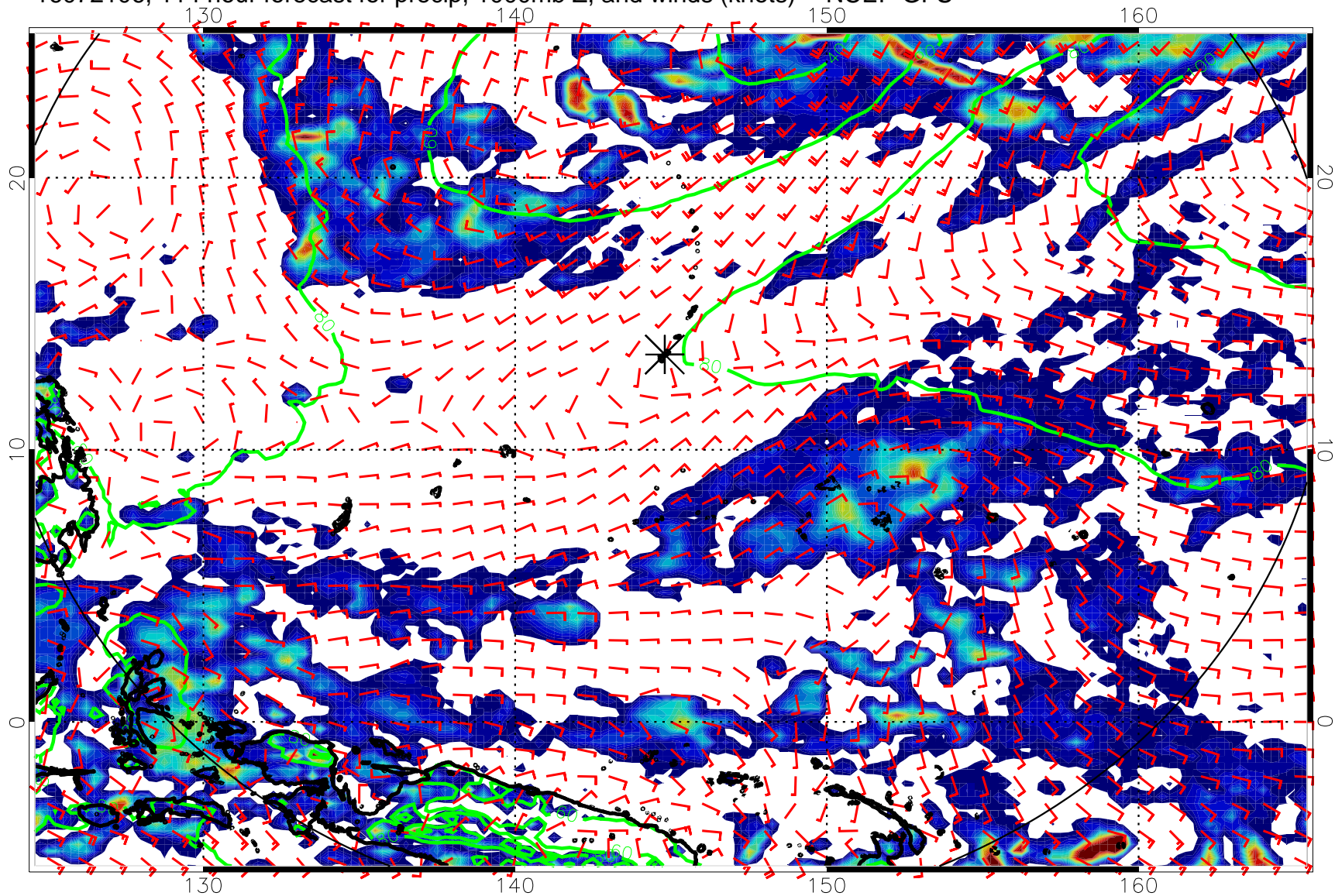
16072106, 114 hour forecast for precip, 1000mb Z, and winds (knots) -- NCEP GFS
