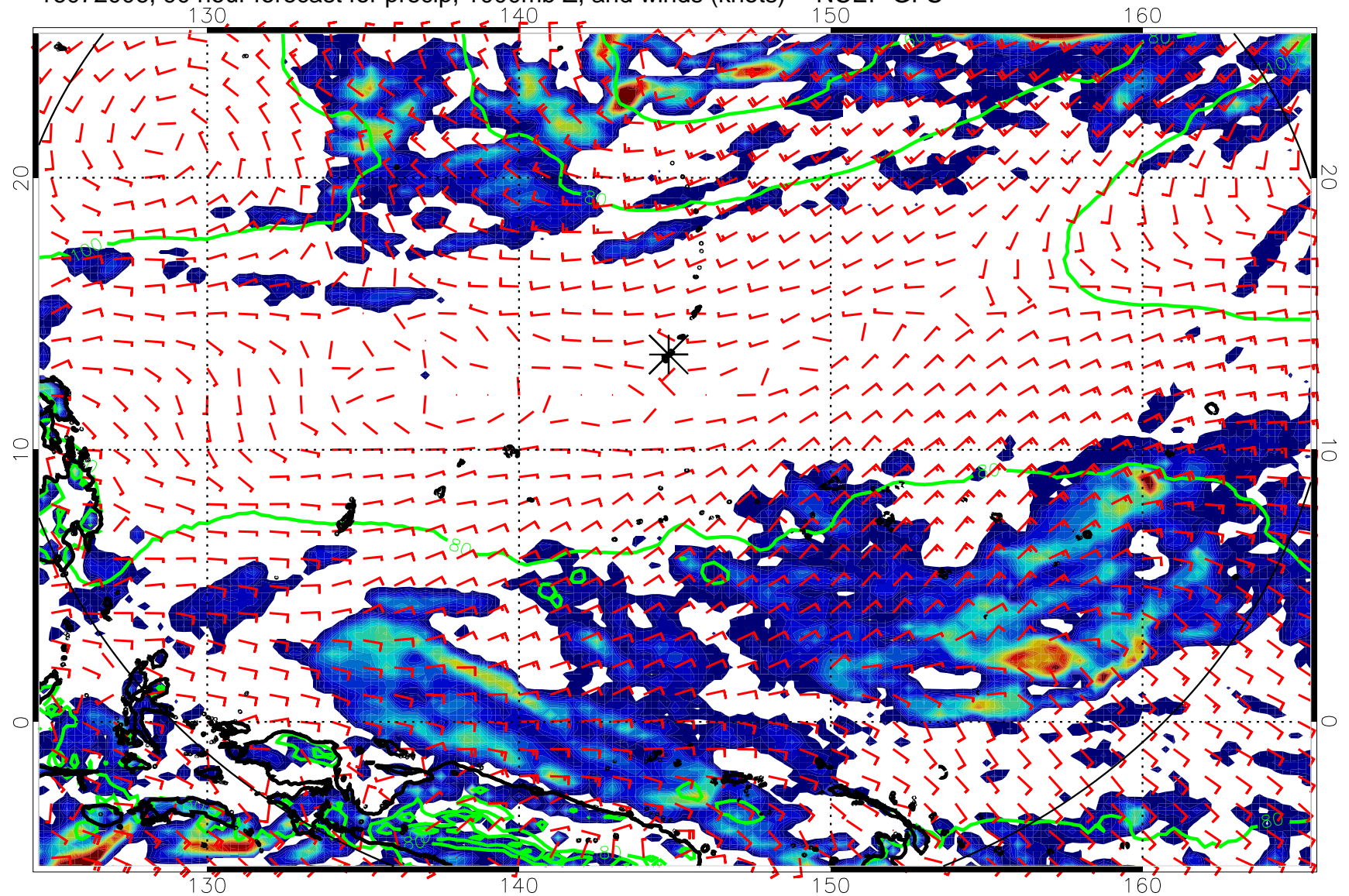
16072006, 90 hour forecast for precip, 1000mb Z, and winds (knots) -- NCEP GFS
