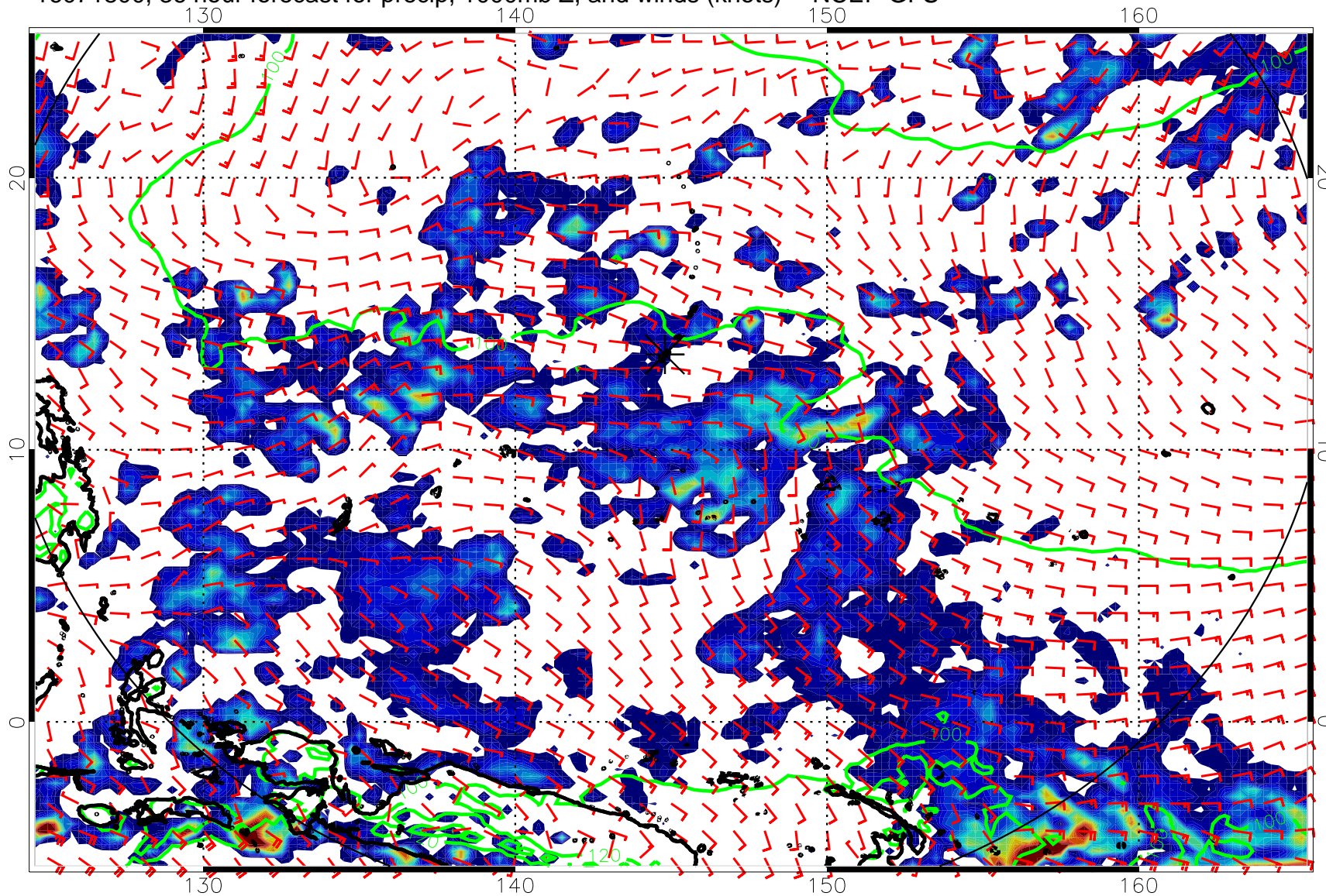
16071800, 36 hour forecast for precip, 1000mb Z, and winds (knots) -- NCEP GFS
