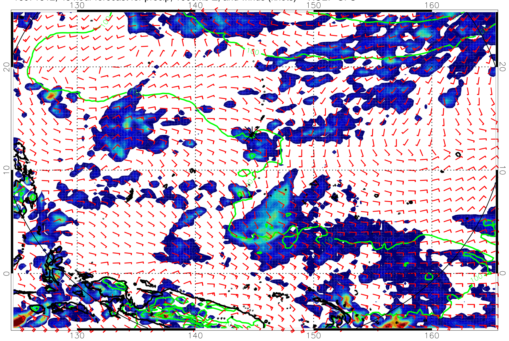
16071812, 48 hour forecast for precip, 1000mb Z, and winds (knots) -- NCEP GFS
