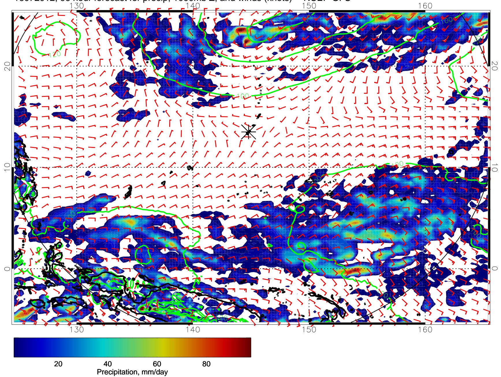
16072012, 96 hour forecast for precip, 1000mb Z, and winds (knots) -- NCEP GFS
