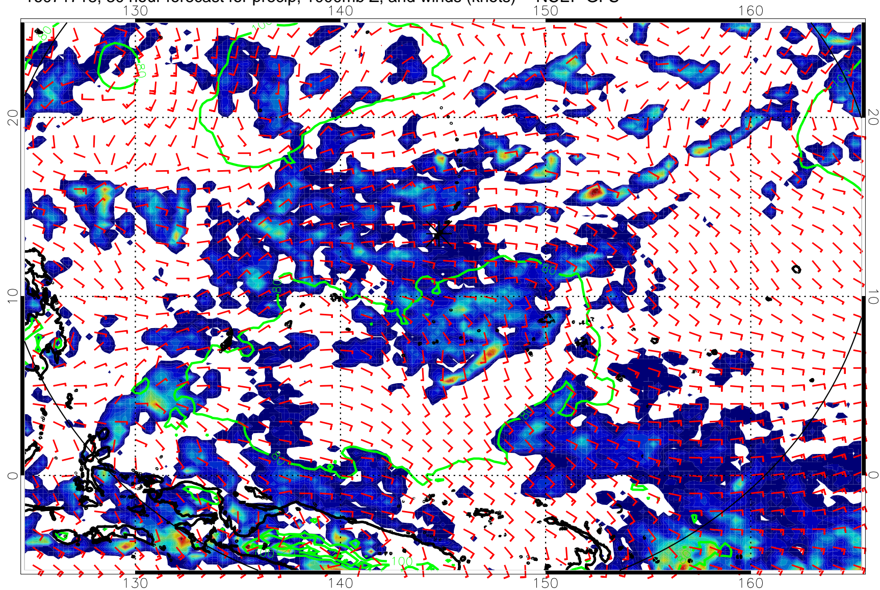
16071718, 30 hour forecast for precip, 1000mb Z, and winds (knots) -- NCEP GFS
