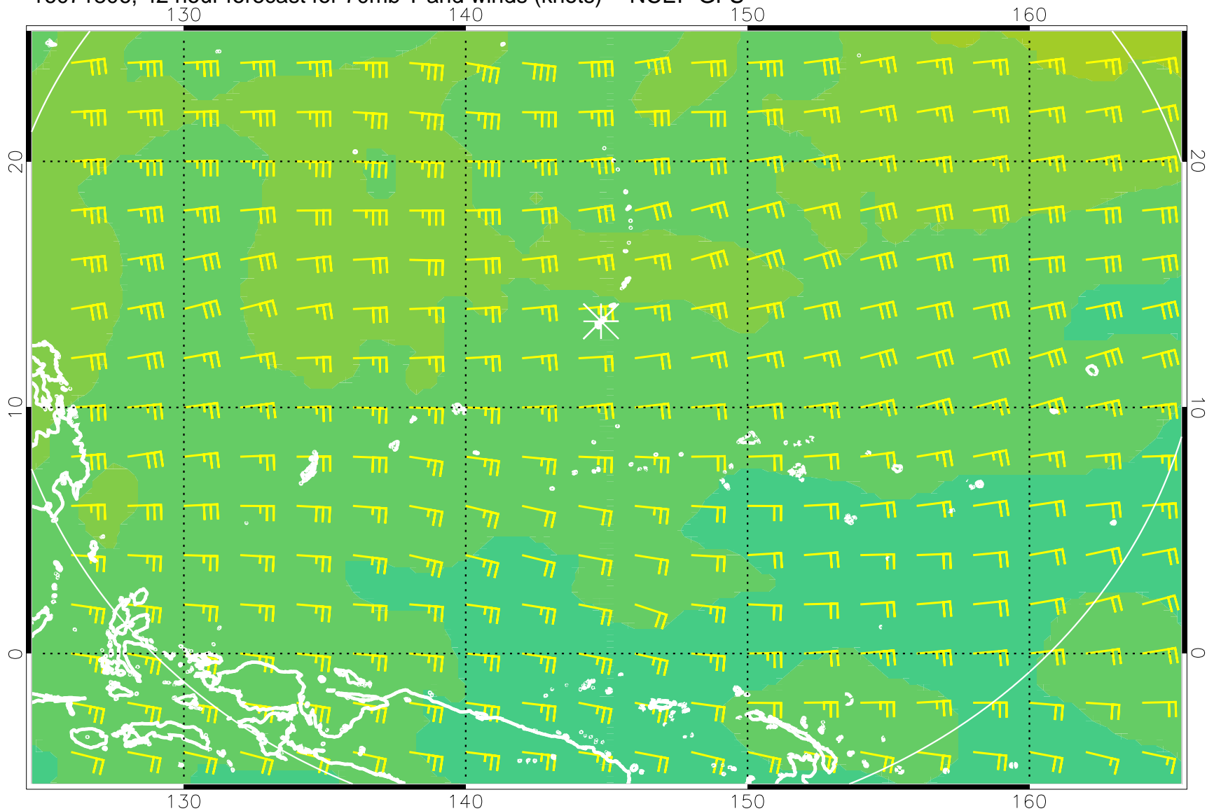
16071806, 42 hour forecast for 70mb T and winds (knots) -- NCEP GFS
