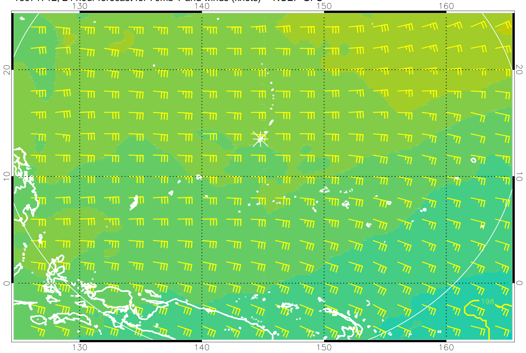
16071712, 24 hour forecast for 70mb T and winds (knots) -- NCEP GFS
