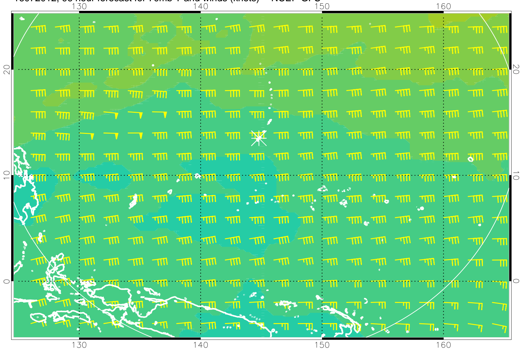
16072012, 96 hour forecast for 70mb T and winds (knots) -- NCEP GFS
