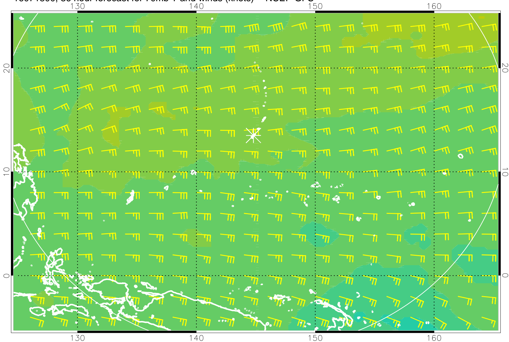
16071800, 36 hour forecast for 70mb T and winds (knots) -- NCEP GFS
