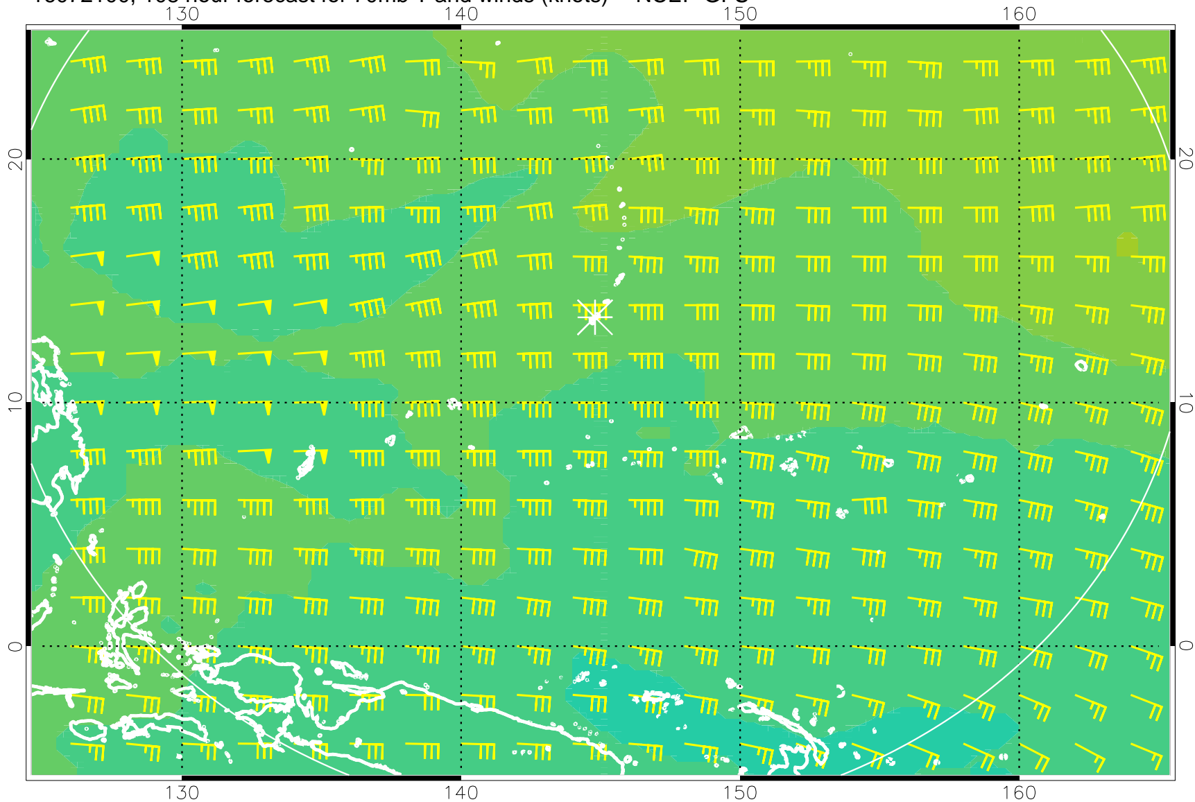
16072100, 108 hour forecast for 70mb T and winds (knots) -- NCEP GFS
