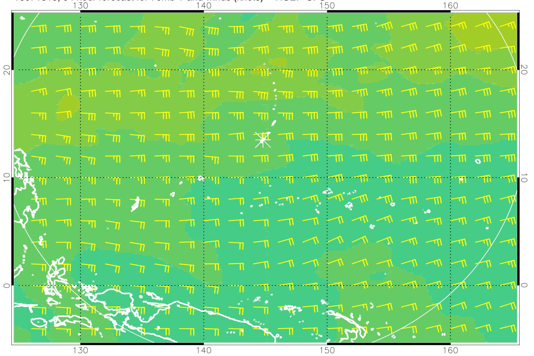
16071818, 54 hour forecast for 70mb T and winds (knots) -- NCEP GFS
