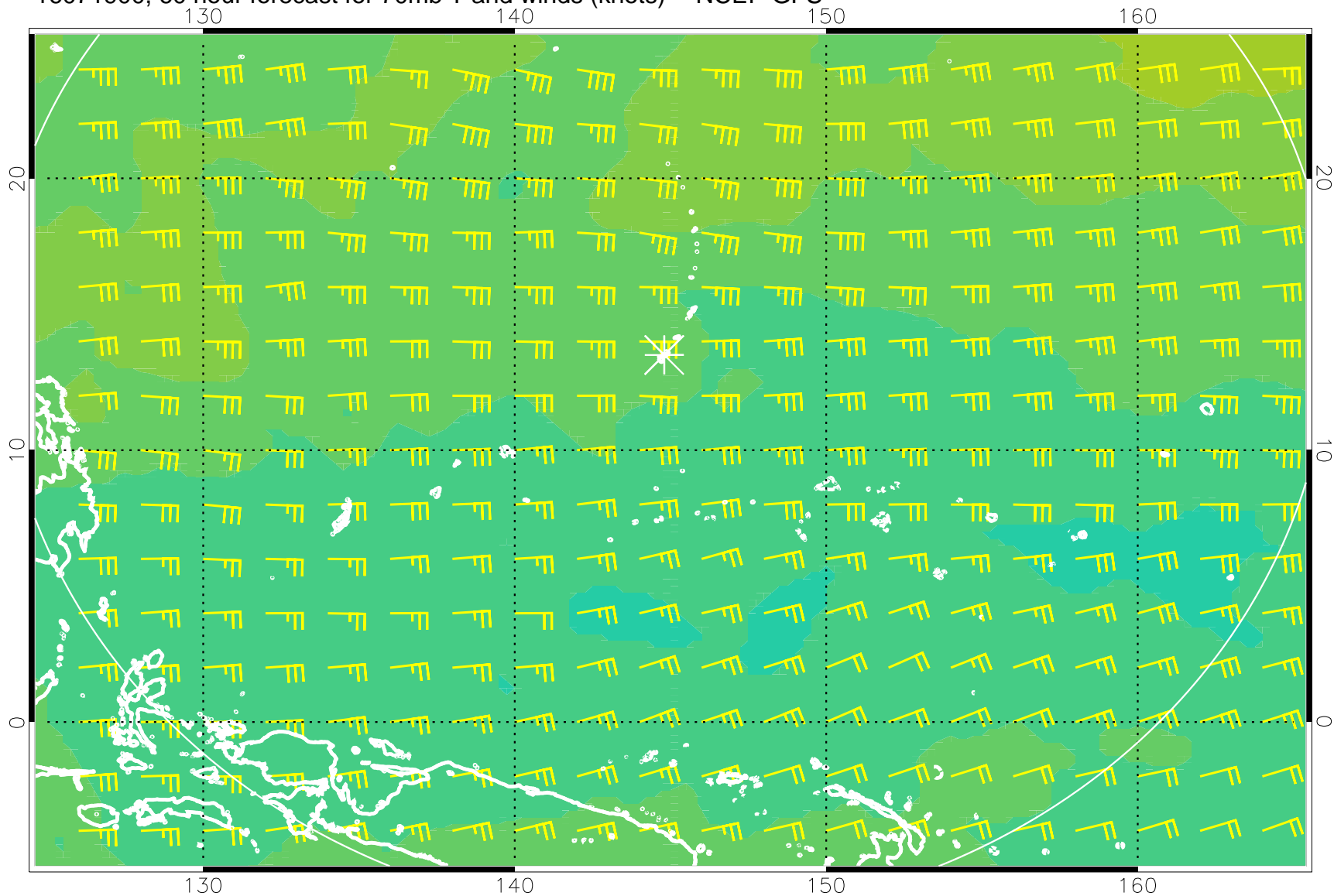
16071900, 60 hour forecast for 70mb T and winds (knots) -- NCEP GFS
