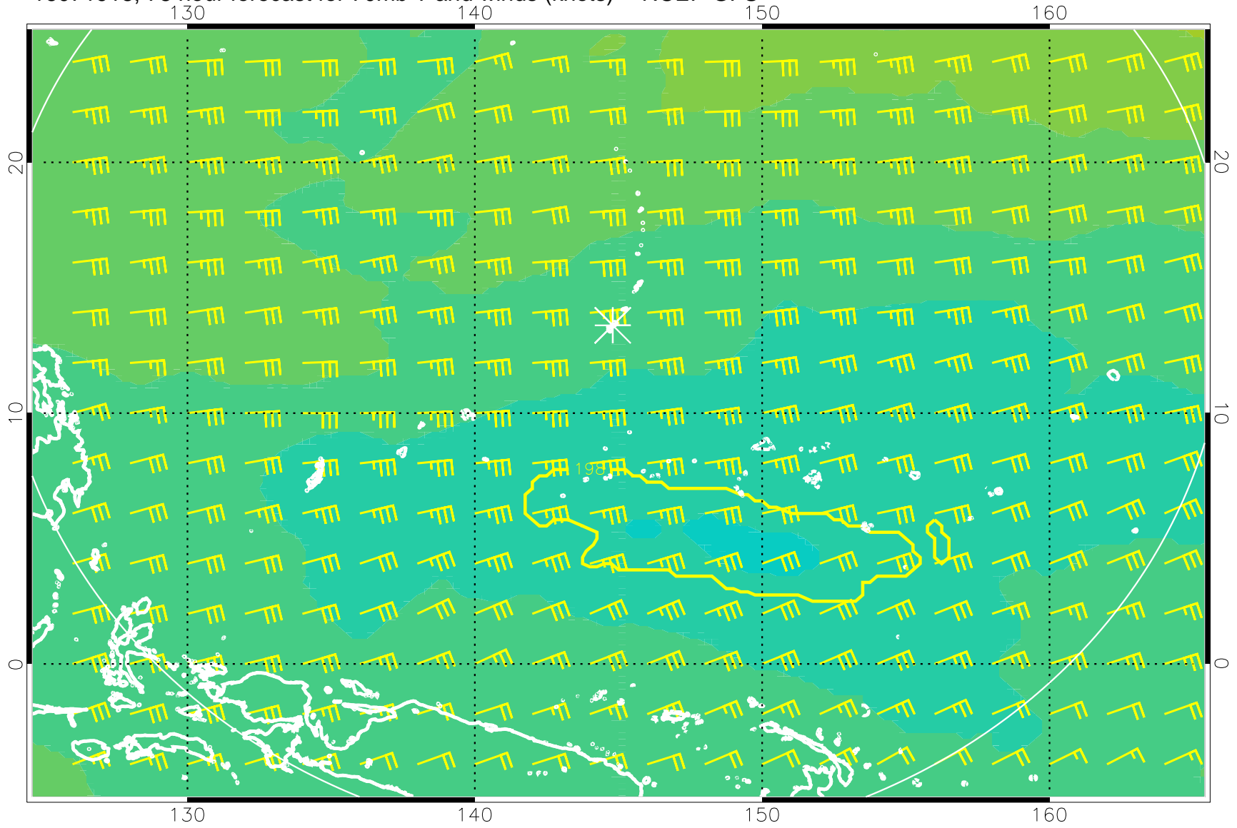
16071918, 78 hour forecast for 70mb T and winds (knots) -- NCEP GFS
