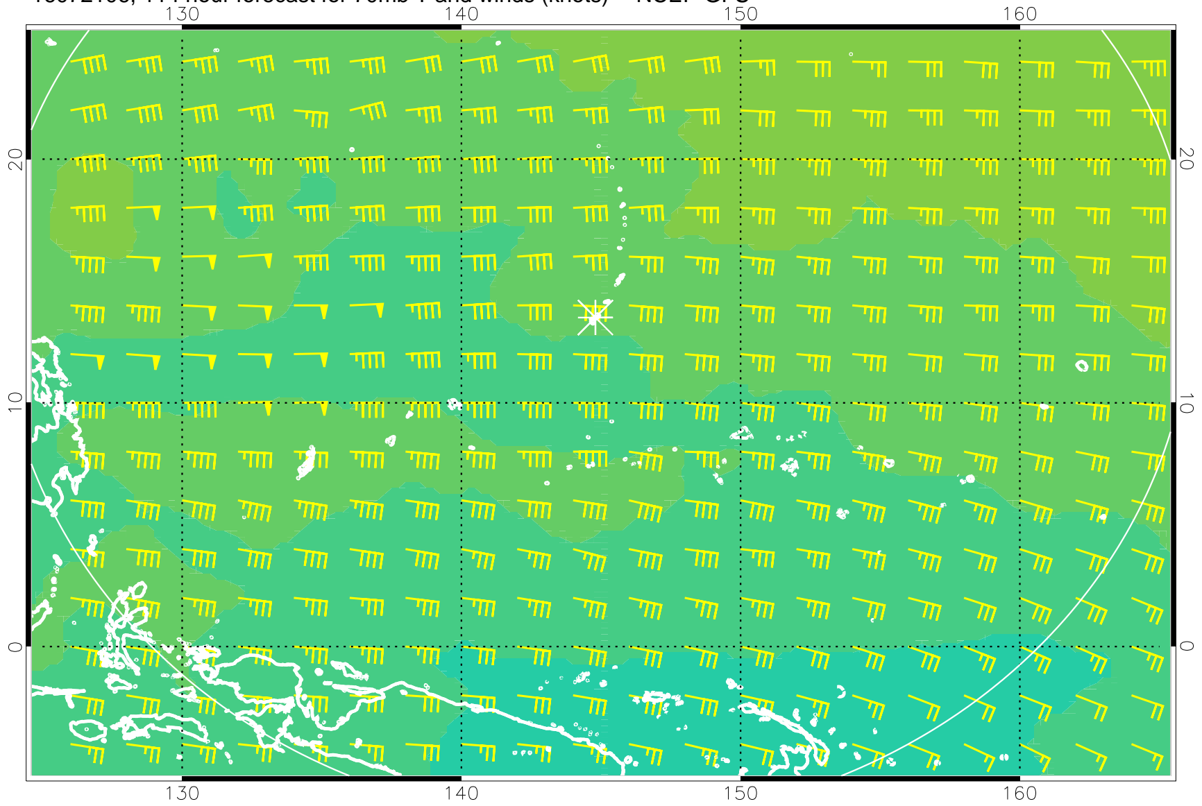
16072106, 114 hour forecast for 70mb T and winds (knots) -- NCEP GFS
