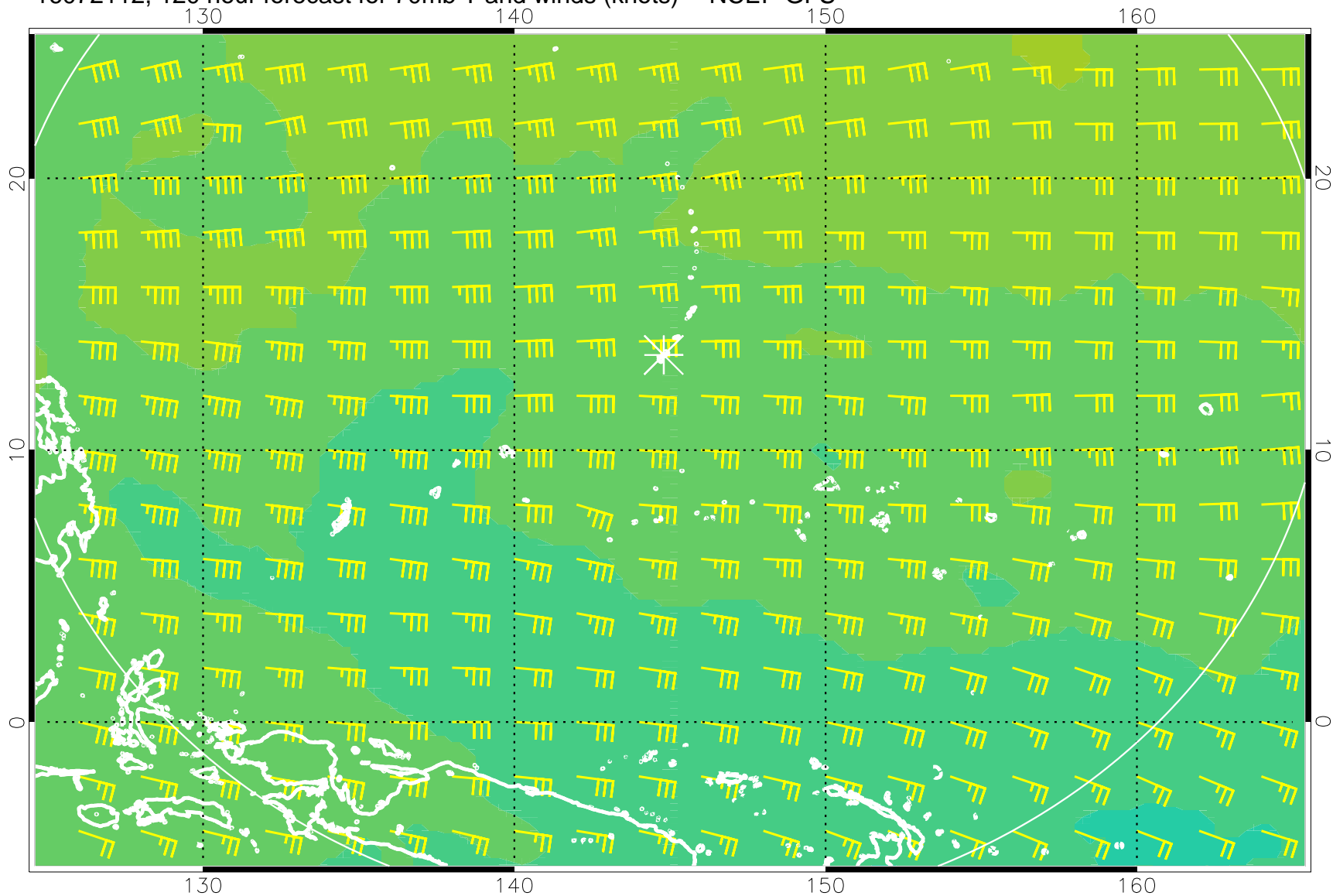
16072112, 120 hour forecast for 70mb T and winds (knots) -- NCEP GFS
