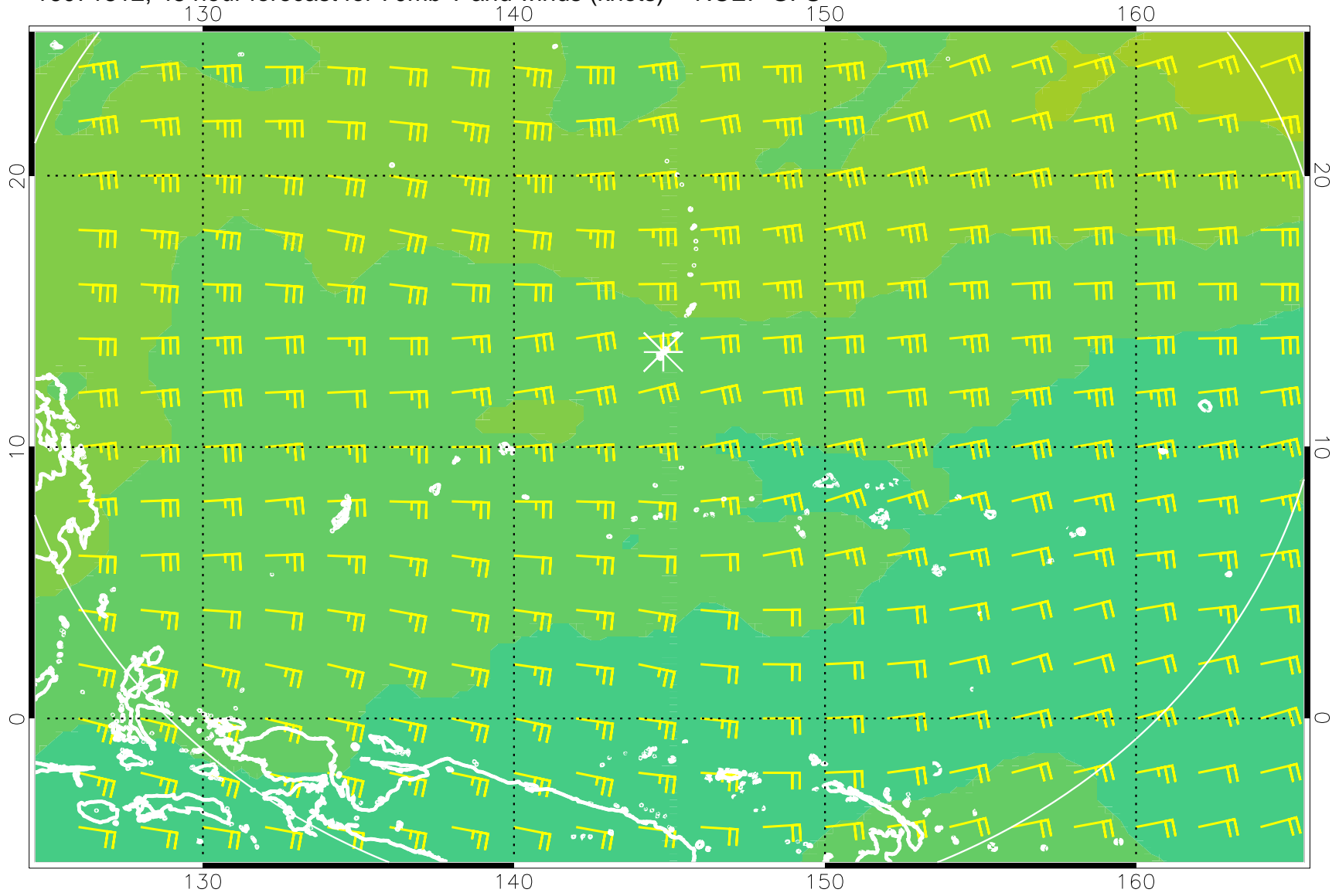
16071812, 48 hour forecast for 70mb T and winds (knots) -- NCEP GFS
