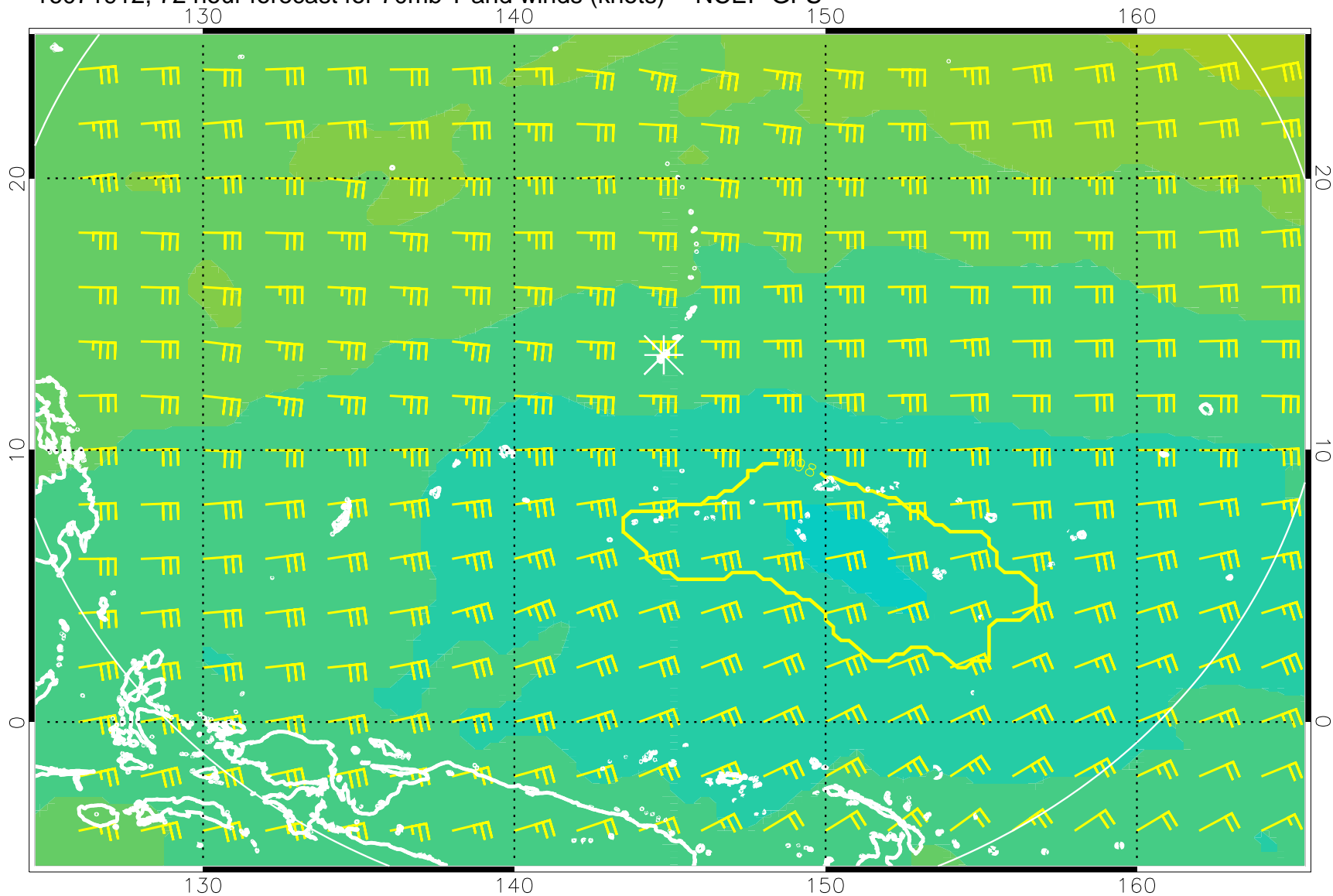
16071912, 72 hour forecast for 70mb T and winds (knots) -- NCEP GFS
