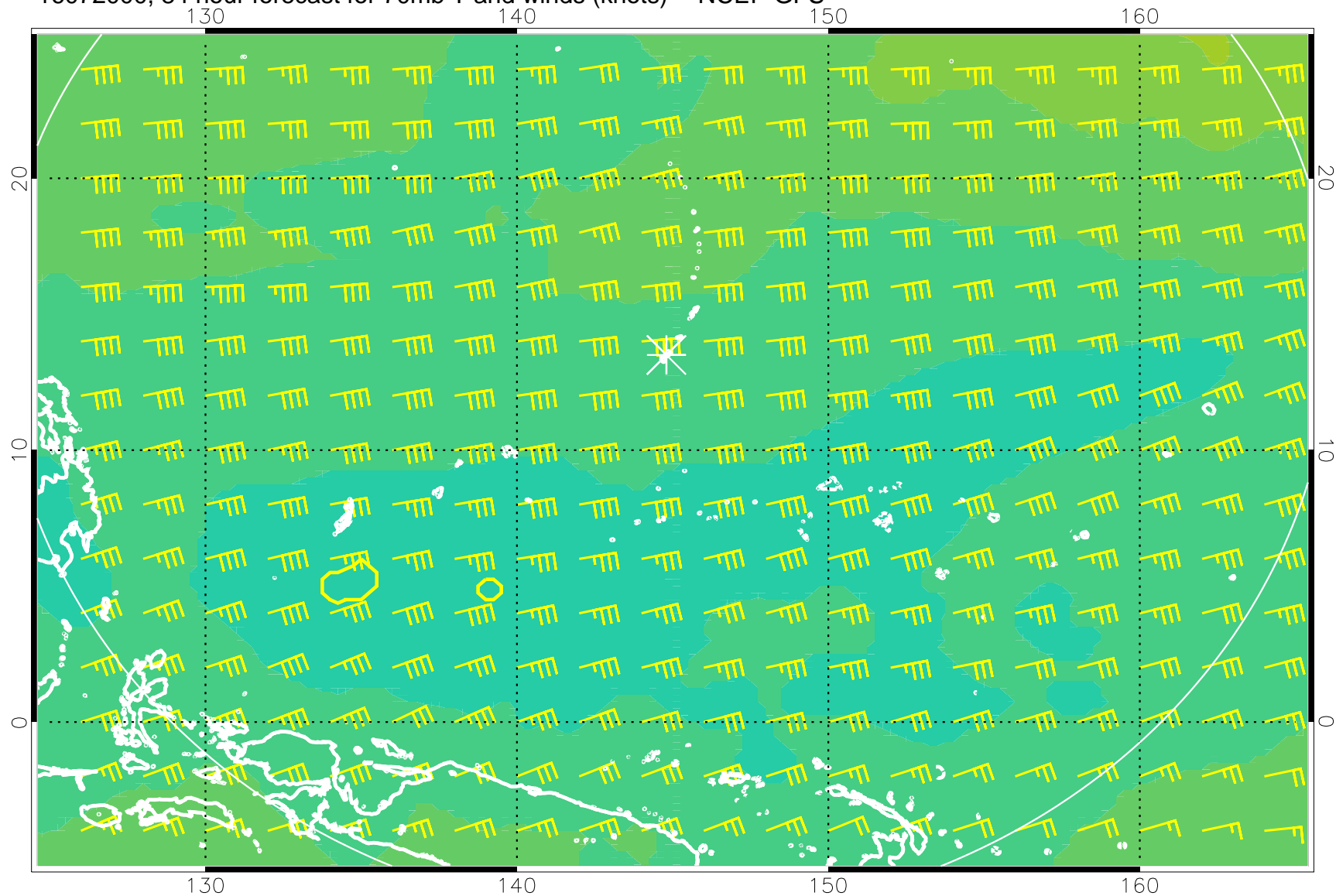
16072000, 84 hour forecast for 70mb T and winds (knots) -- NCEP GFS
