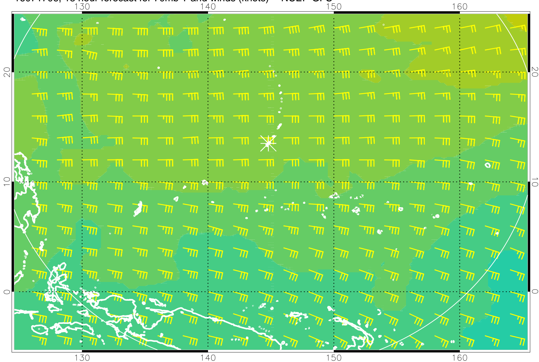
16071706, 18 hour forecast for 70mb T and winds (knots) -- NCEP GFS
