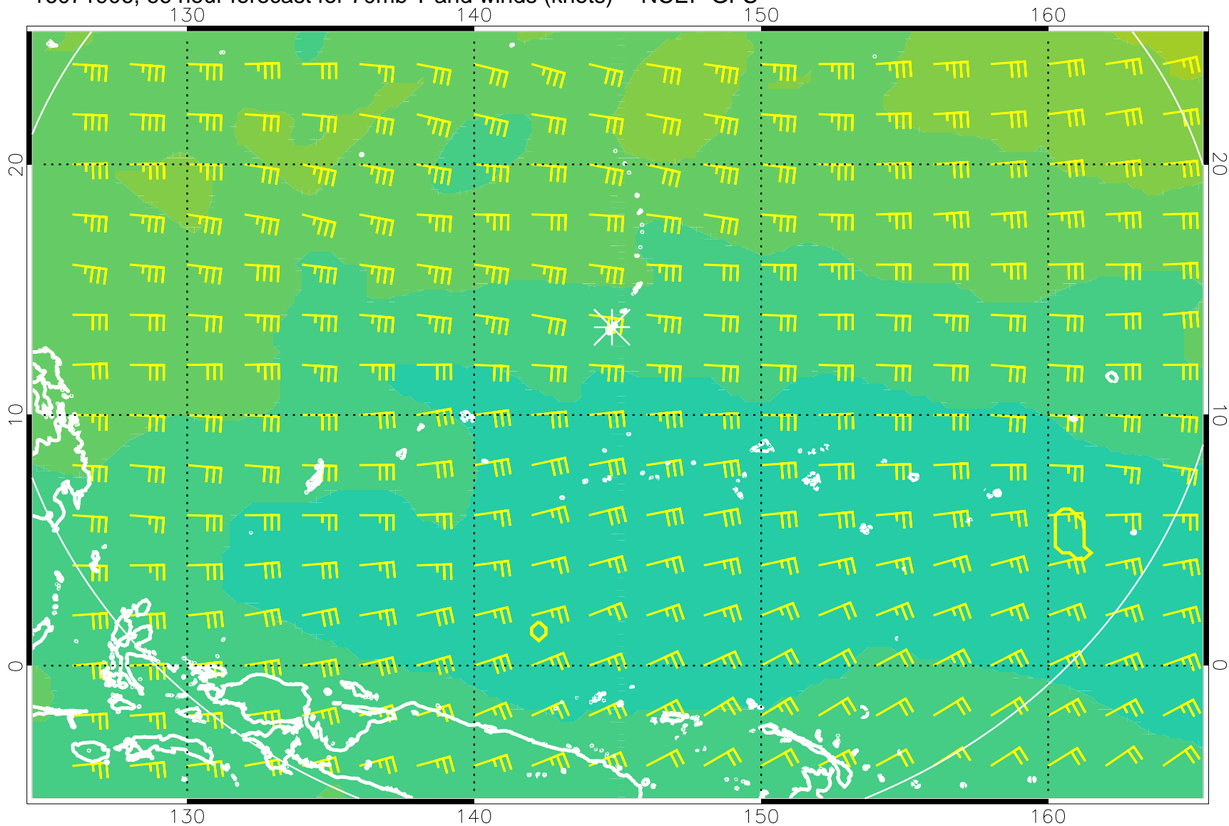
16071906, 66 hour forecast for 70mb T and winds (knots) -- NCEP GFS
