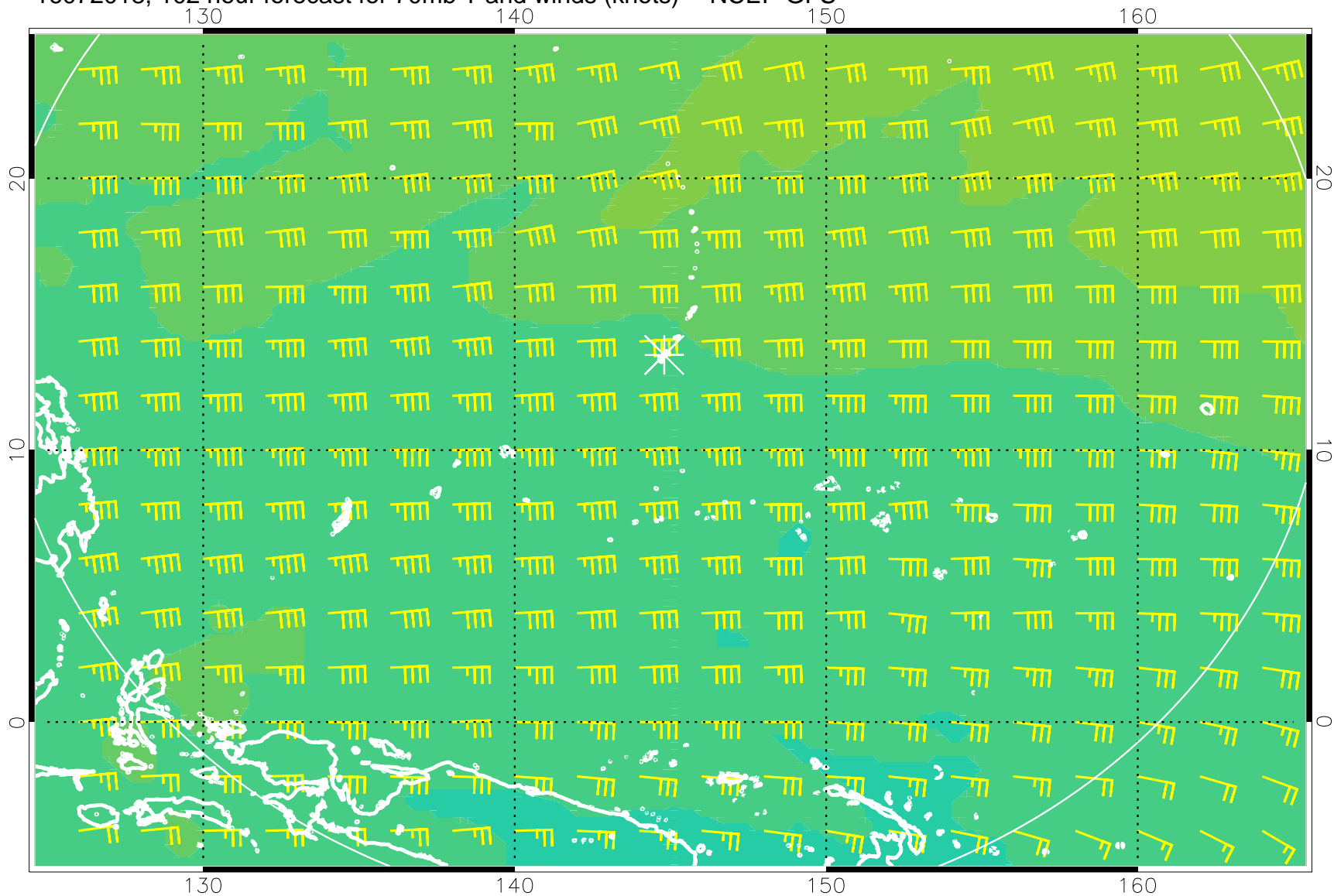
16072018, 102 hour forecast for 70mb T and winds (knots) -- NCEP GFS
