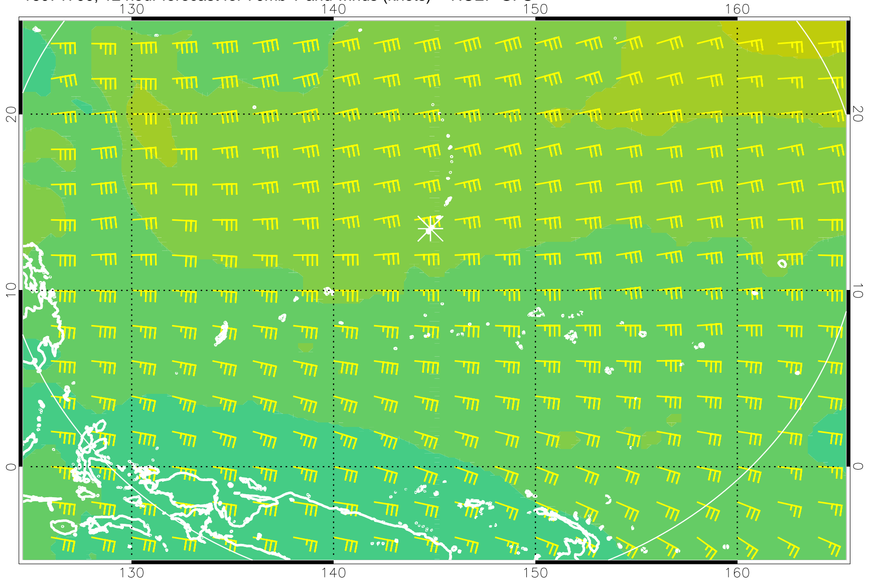
16071700, 12 hour forecast for 70mb T and winds (knots) -- NCEP GFS
