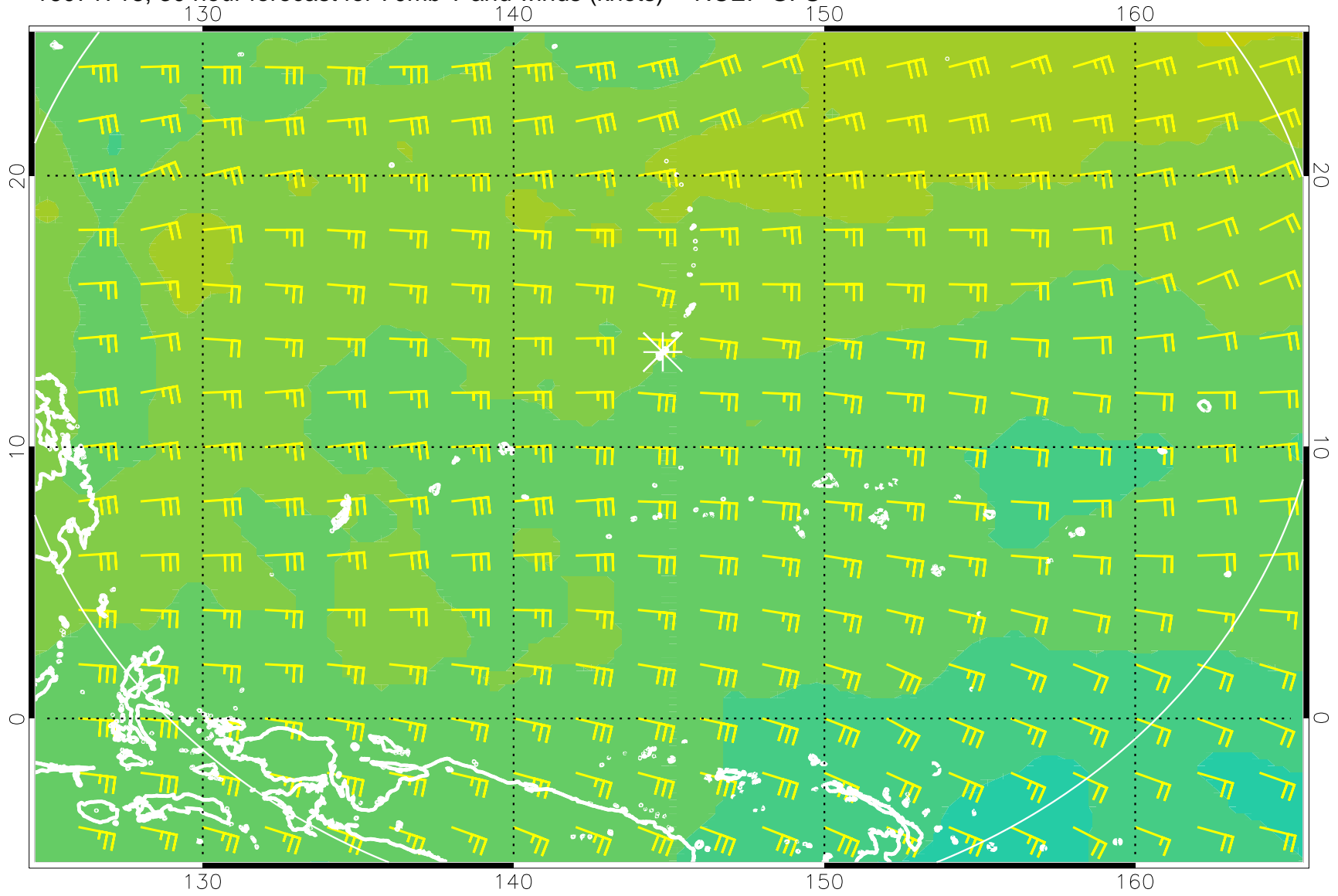
16071718, 30 hour forecast for 70mb T and winds (knots) -- NCEP GFS
