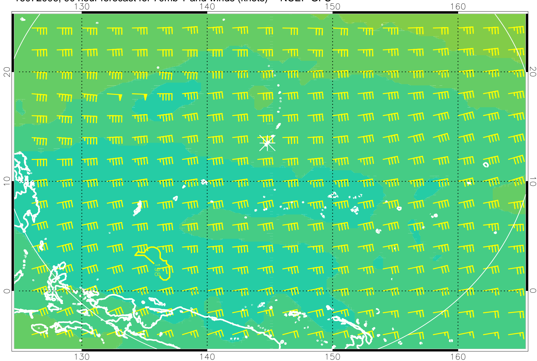
16072006, 90 hour forecast for 70mb T and winds (knots) -- NCEP GFS
