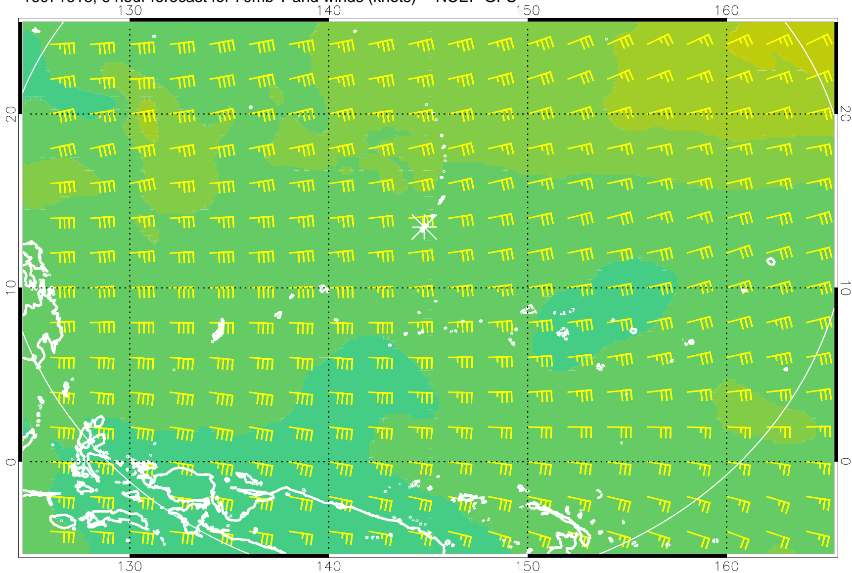
16071618, 6 hour forecast for 70mb T and winds (knots) -- NCEP GFS
