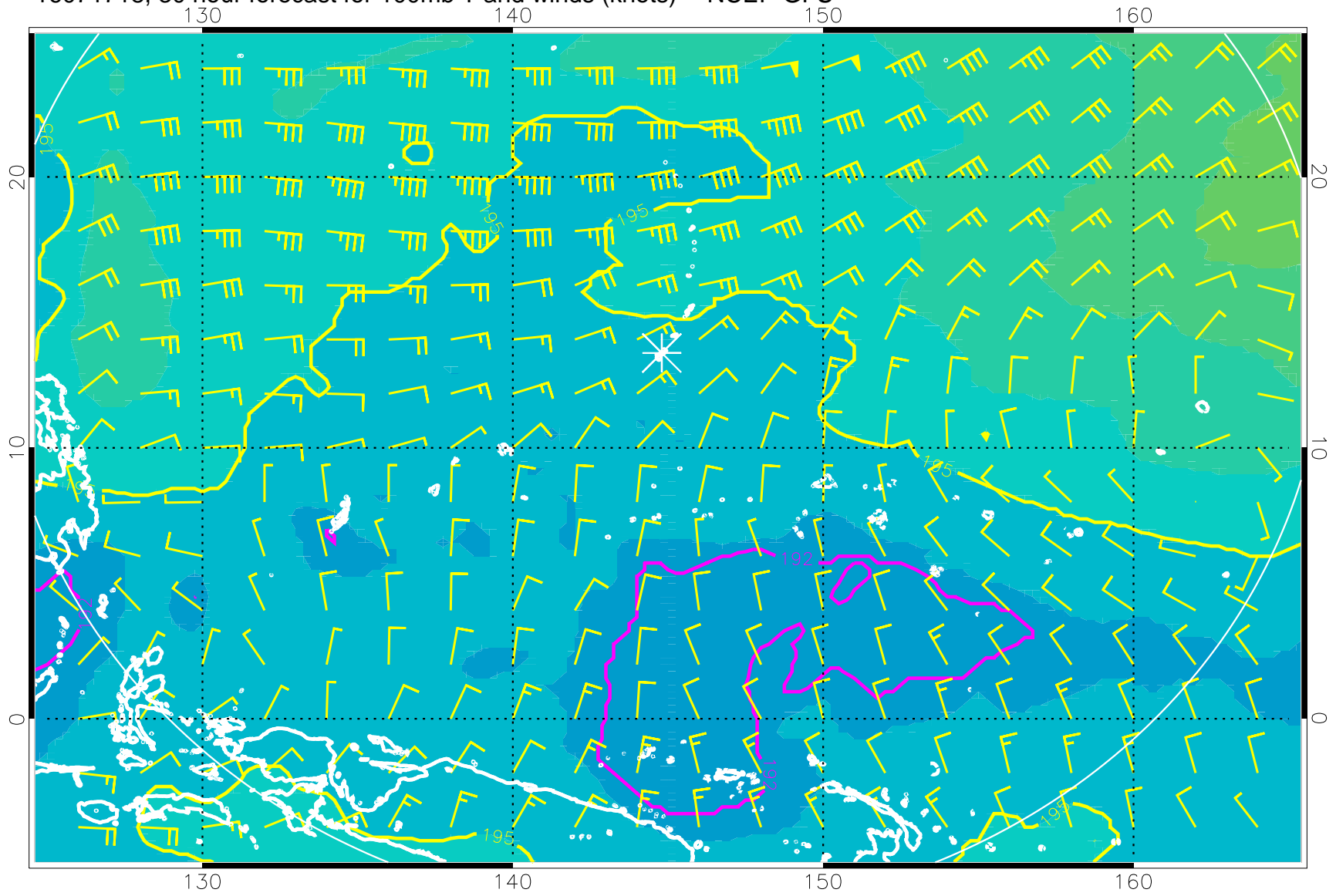
16071718, 30 hour forecast for 100mb T and winds (knots) -- NCEP GFS
