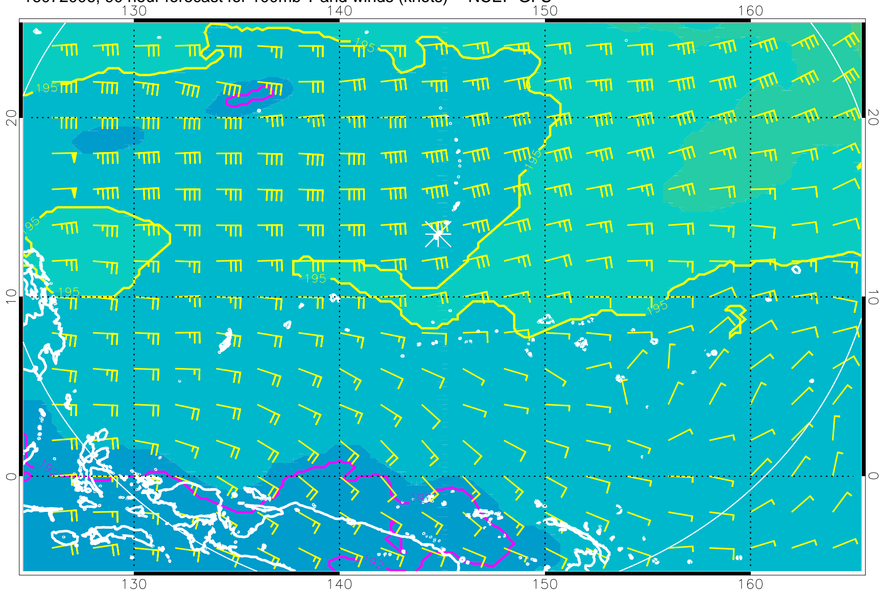
16072006, 90 hour forecast for 100mb T and winds (knots) -- NCEP GFS
