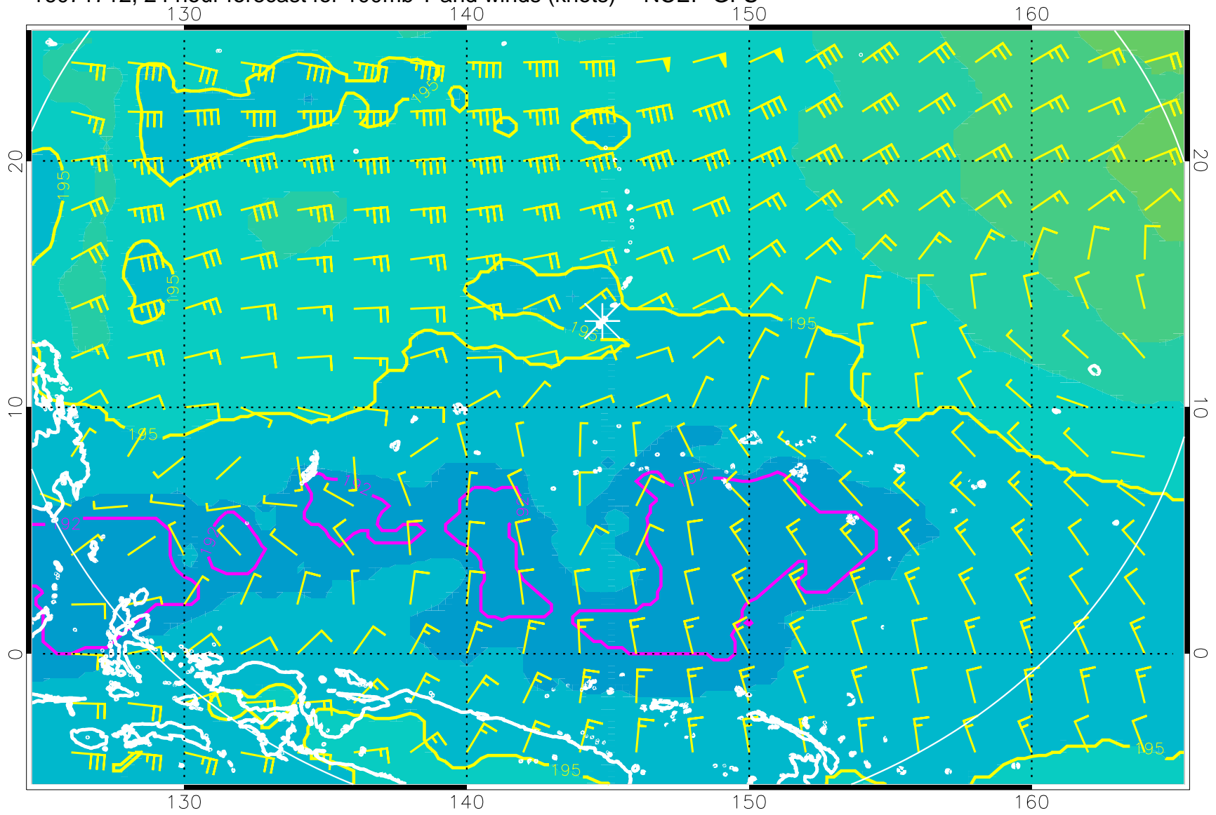
16071712, 24 hour forecast for 100mb T and winds (knots) -- NCEP GFS
