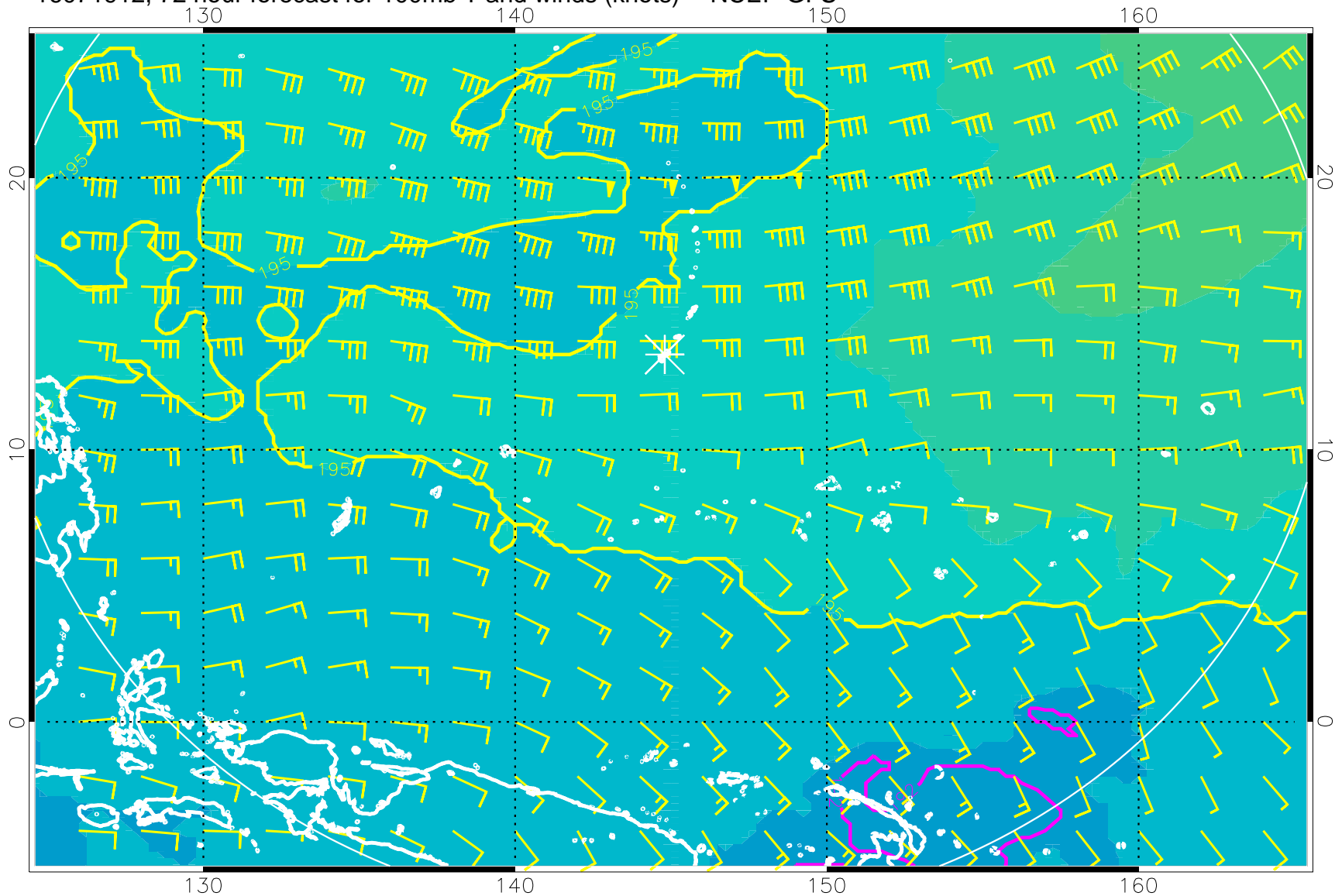
16071912, 72 hour forecast for 100mb T and winds (knots) -- NCEP GFS
