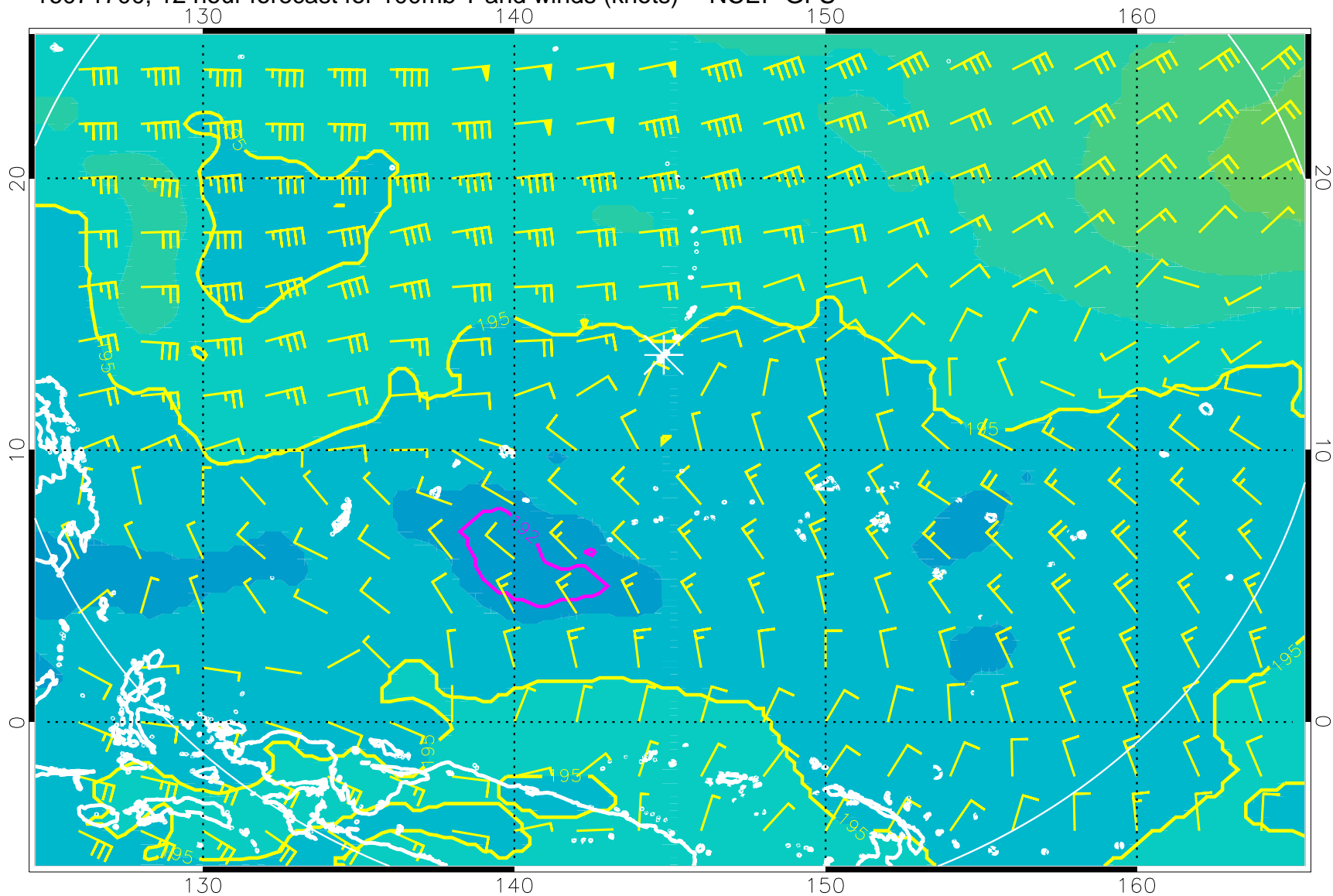
16071700, 12 hour forecast for 100mb T and winds (knots) -- NCEP GFS
