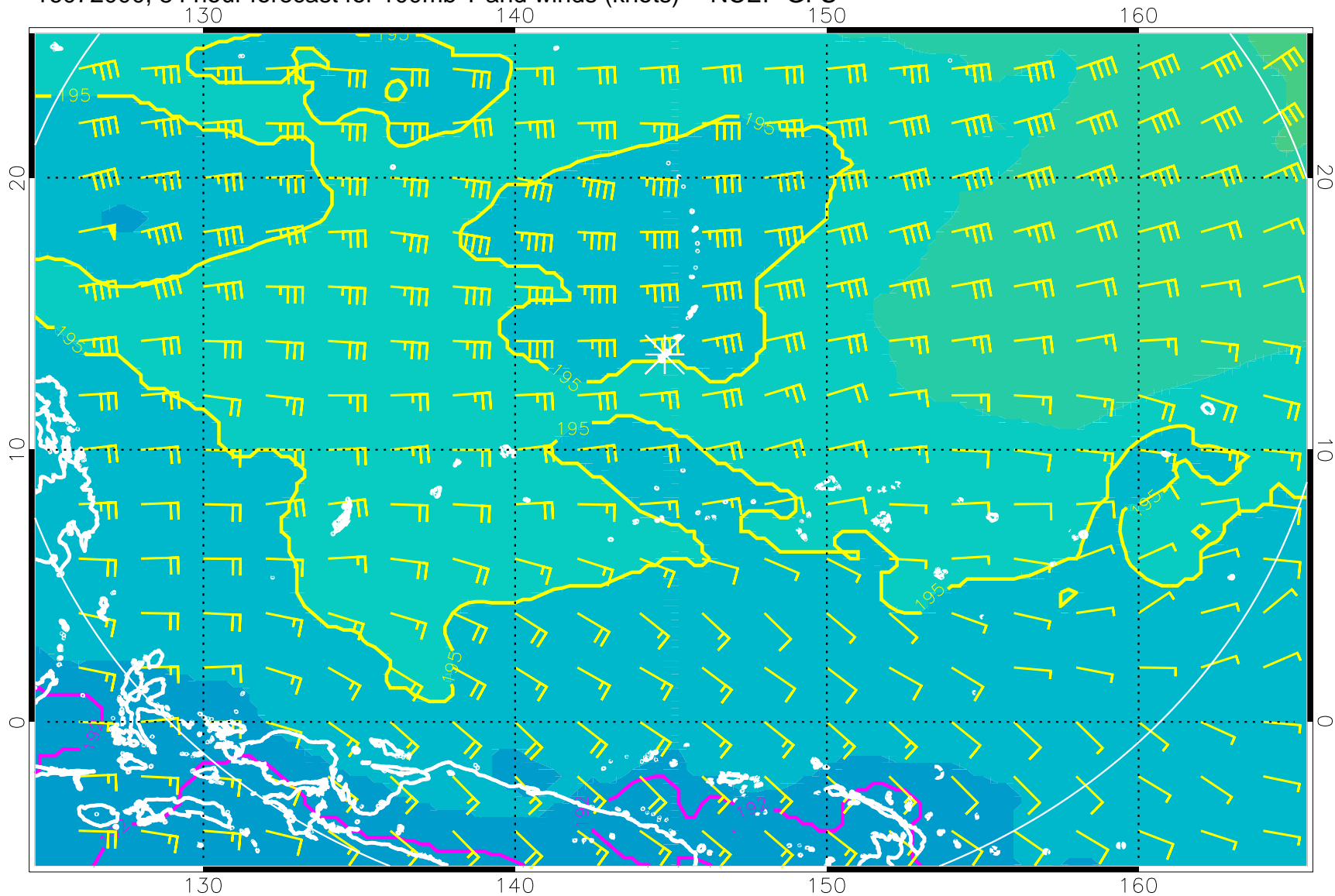
16072000, 84 hour forecast for 100mb T and winds (knots) -- NCEP GFS
