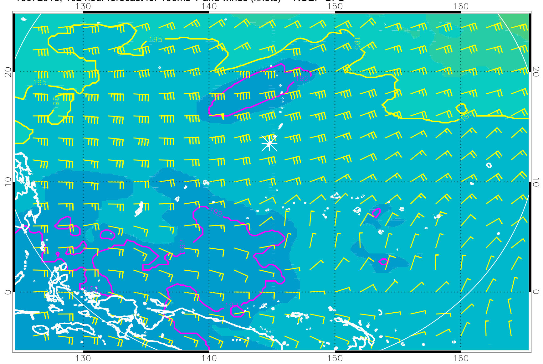
16072018, 102 hour forecast for 100mb T and winds (knots) -- NCEP GFS
