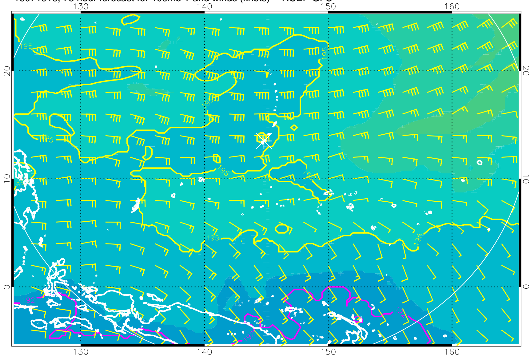
16071918, 78 hour forecast for 100mb T and winds (knots) -- NCEP GFS
