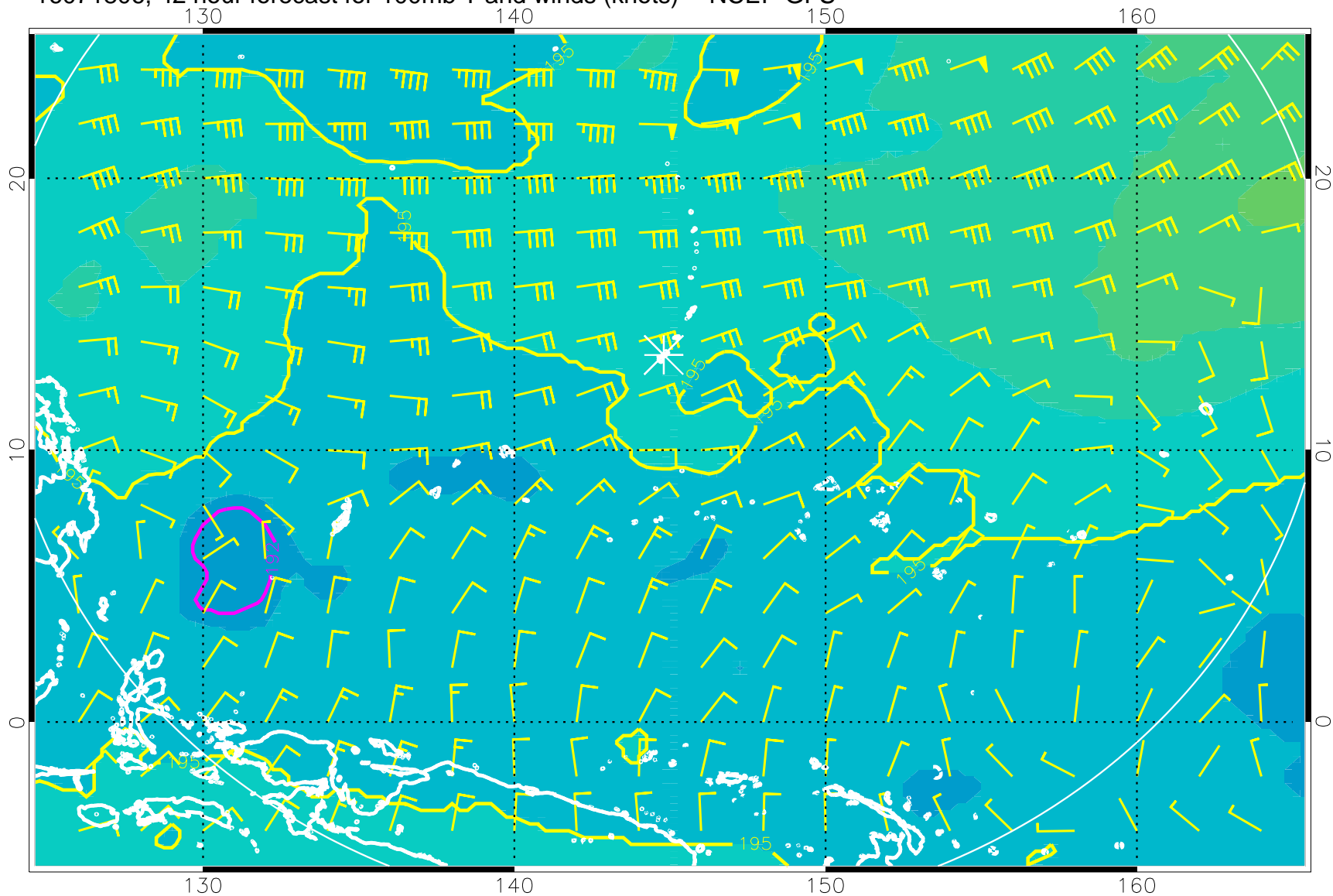
16071806, 42 hour forecast for 100mb T and winds (knots) -- NCEP GFS
