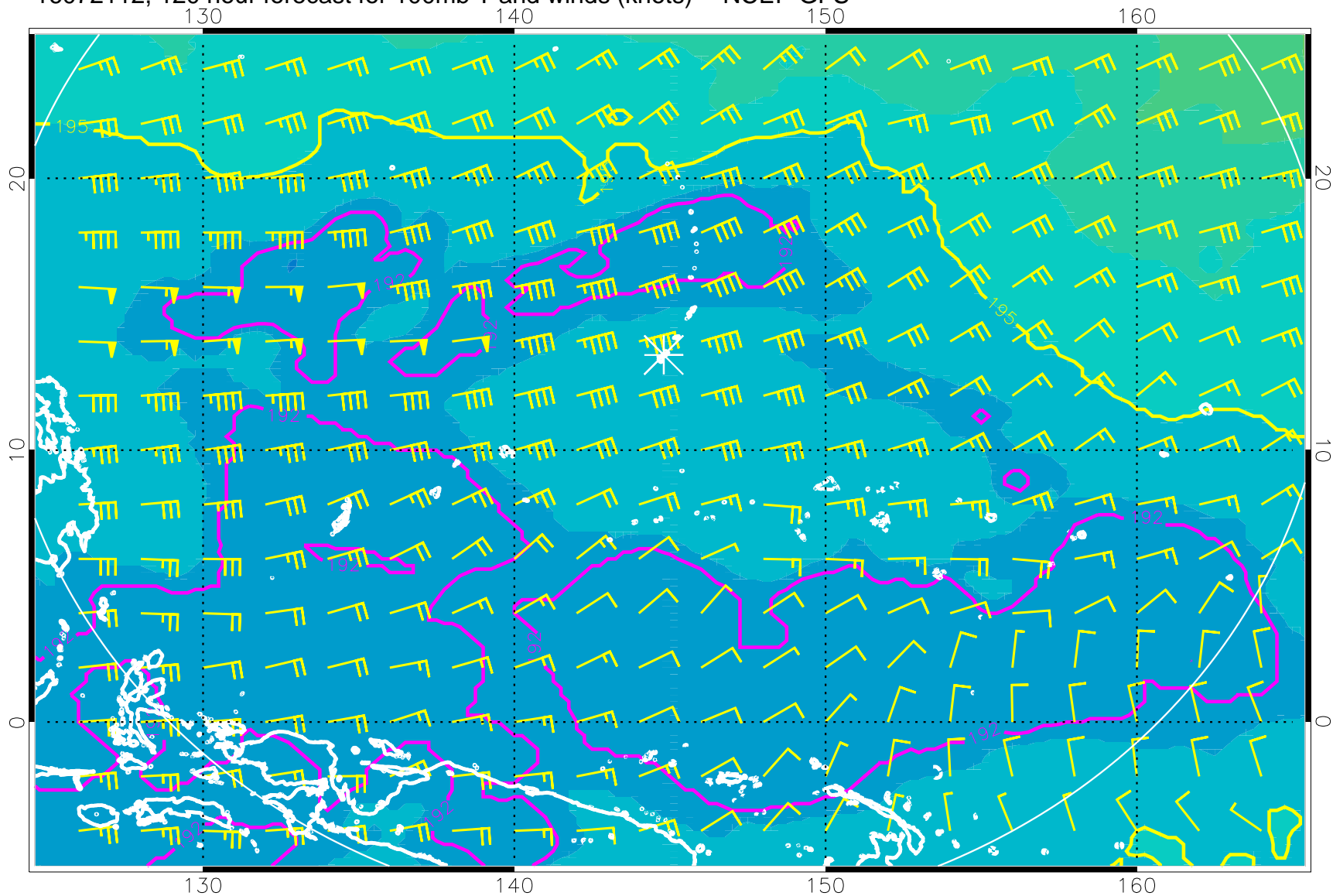
16072112, 120 hour forecast for 100mb T and winds (knots) -- NCEP GFS
