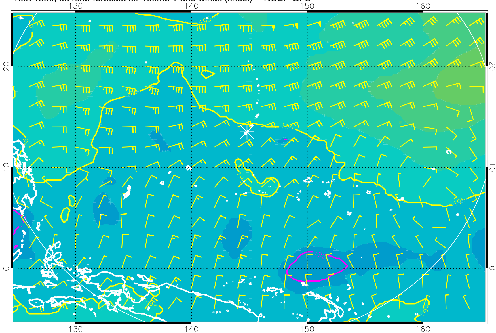
16071800, 36 hour forecast for 100mb T and winds (knots) -- NCEP GFS
