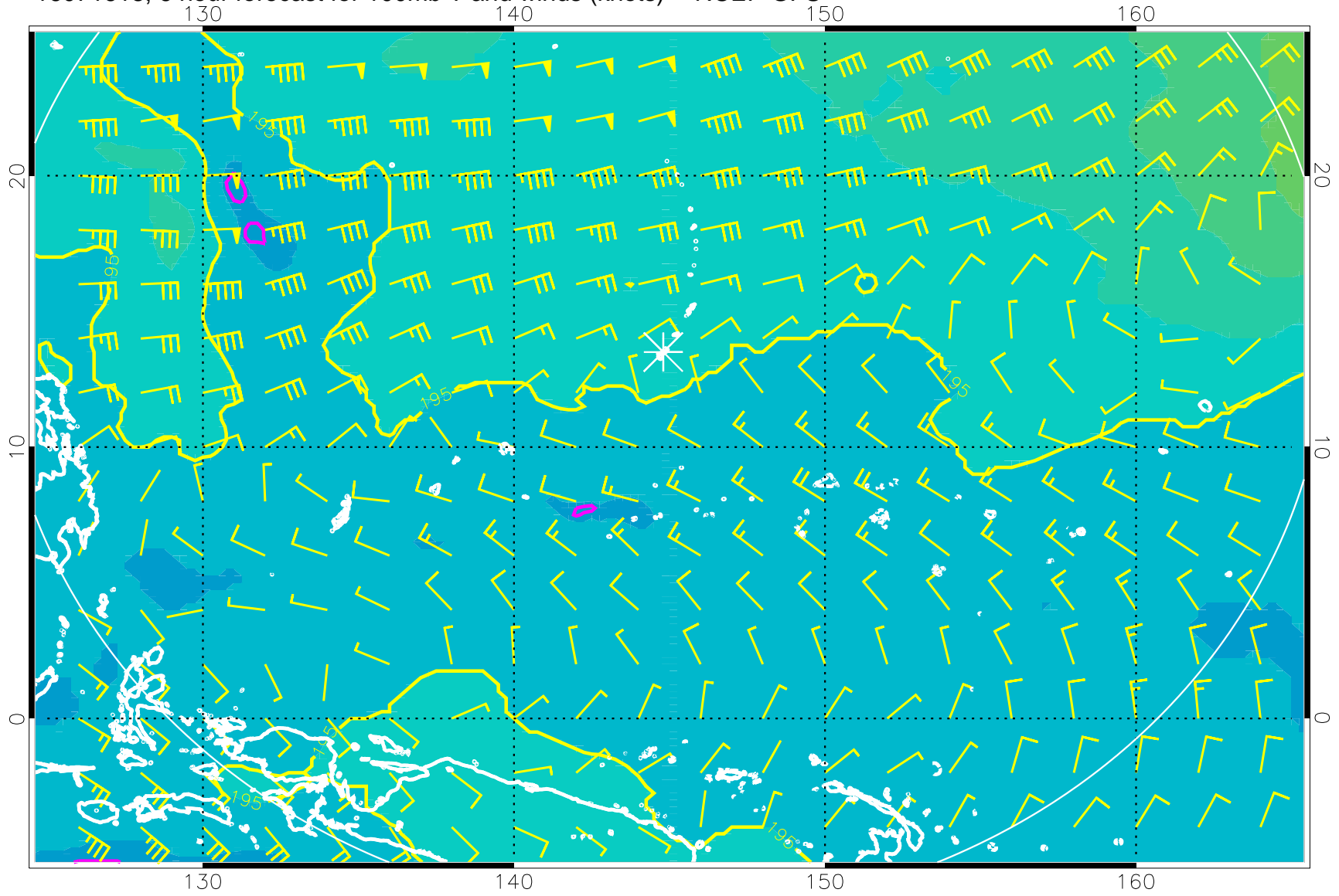
16071618, 6 hour forecast for 100mb T and winds (knots) -- NCEP GFS
