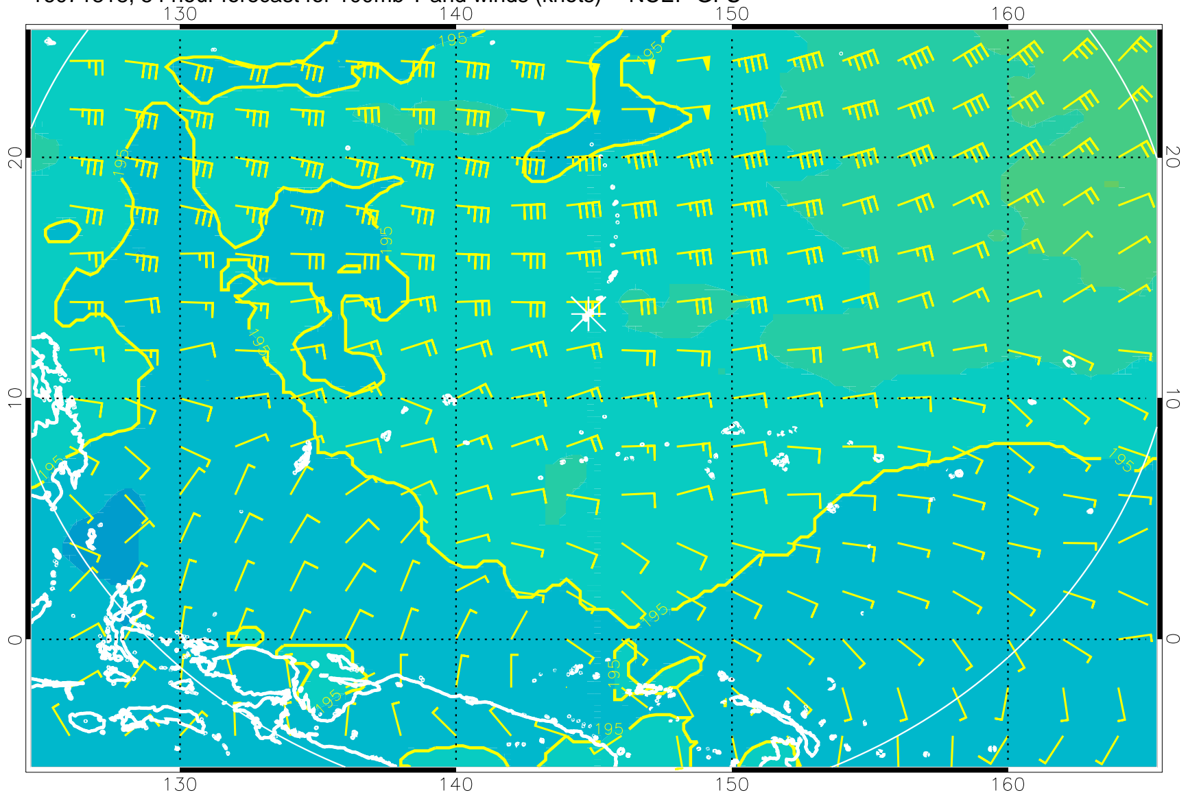
16071818, 54 hour forecast for 100mb T and winds (knots) -- NCEP GFS
