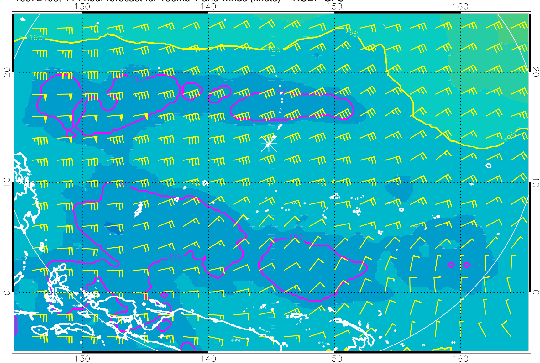
16072106, 114 hour forecast for 100mb T and winds (knots) -- NCEP GFS
