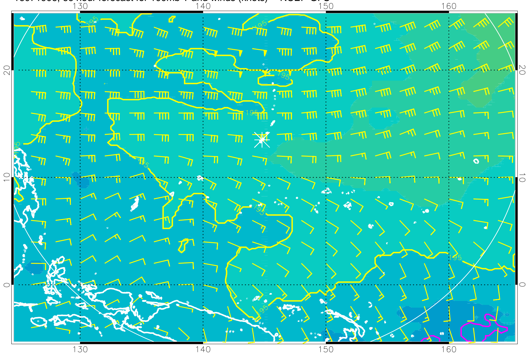
16071906, 66 hour forecast for 100mb T and winds (knots) -- NCEP GFS
