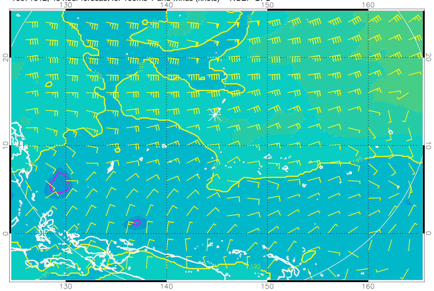
16071812, 48 hour forecast for 100mb T and winds (knots) -- NCEP GFS
