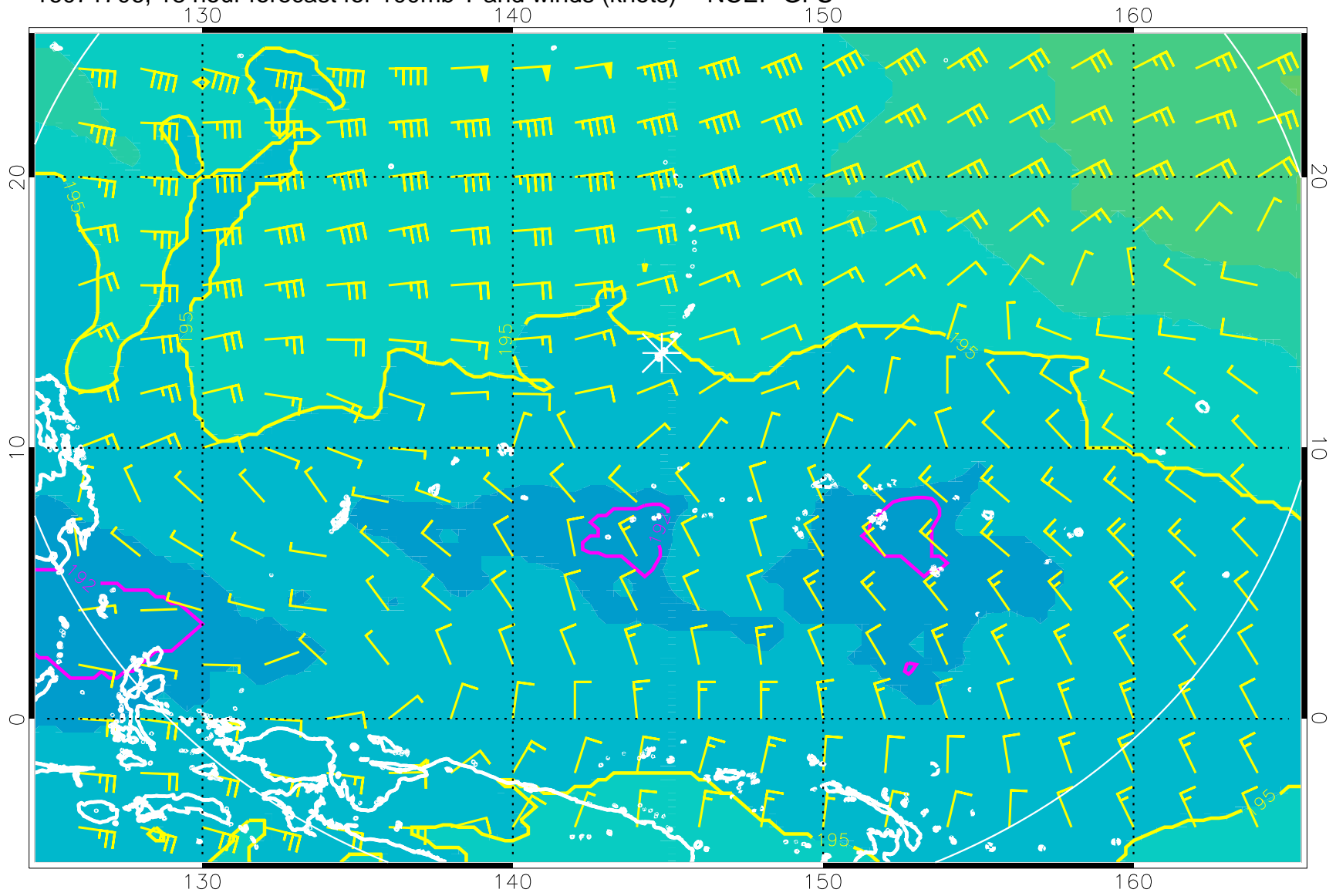
16071706, 18 hour forecast for 100mb T and winds (knots) -- NCEP GFS
