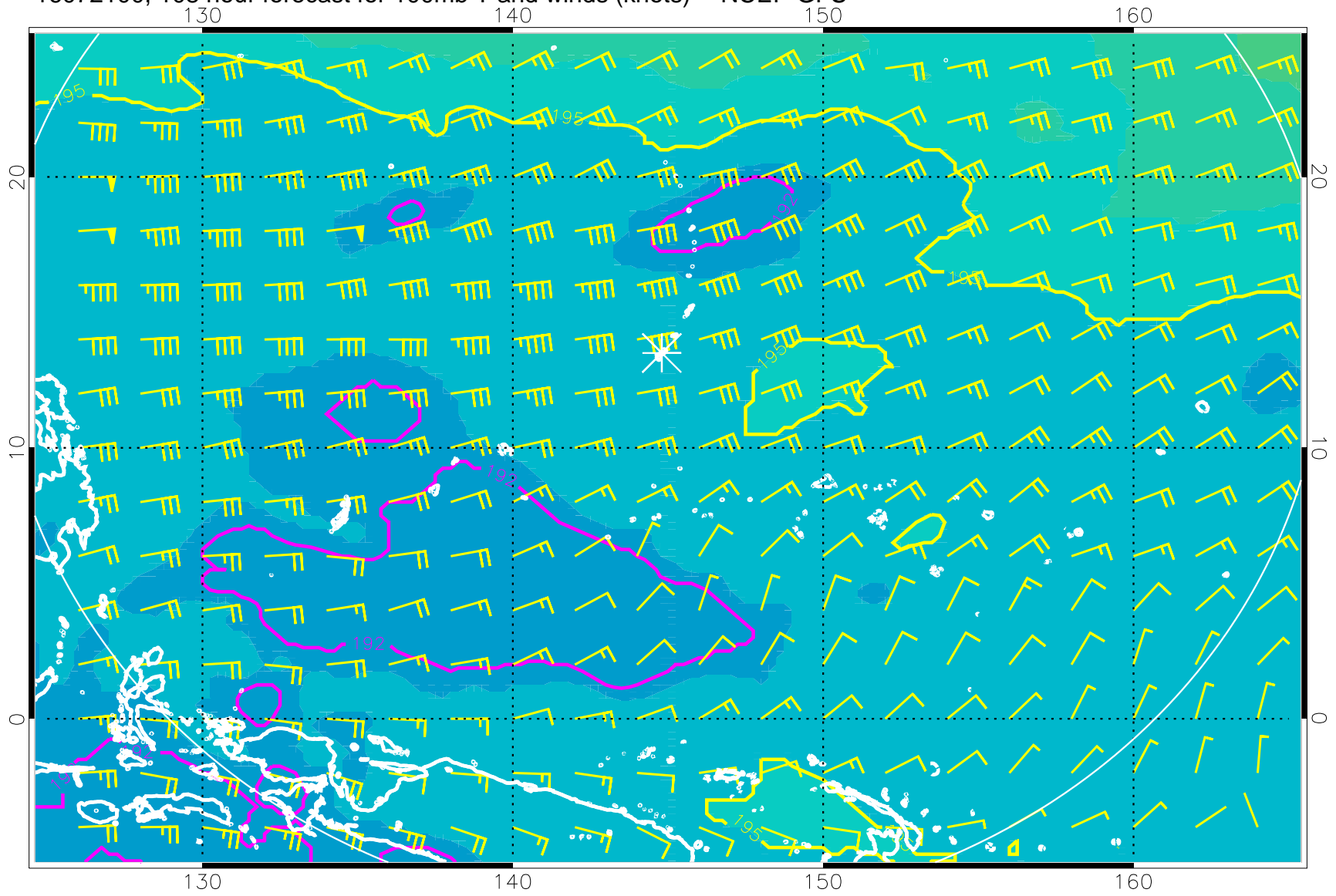
16072100, 108 hour forecast for 100mb T and winds (knots) -- NCEP GFS
