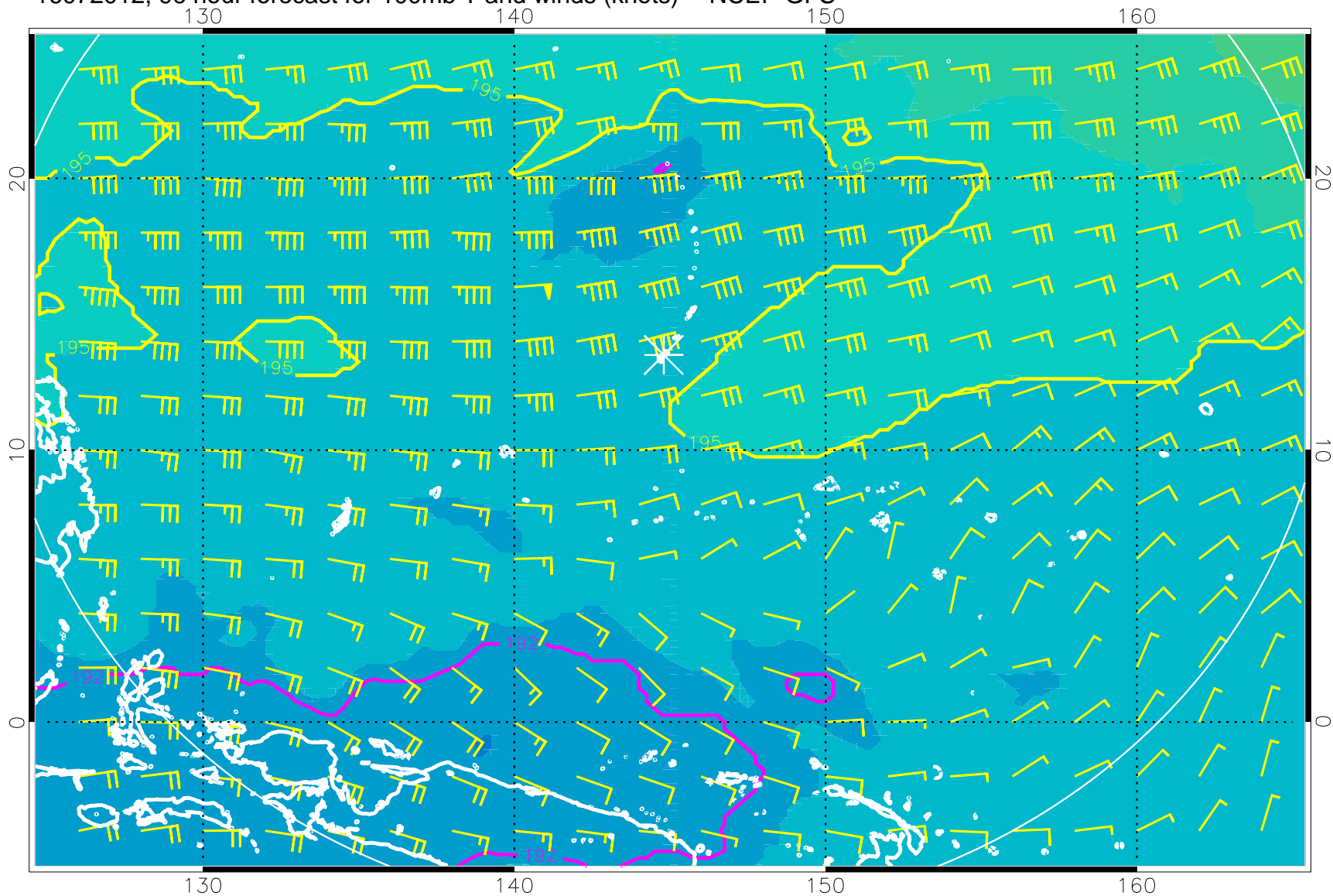
16072012, 96 hour forecast for 100mb T and winds (knots) -- NCEP GFS
