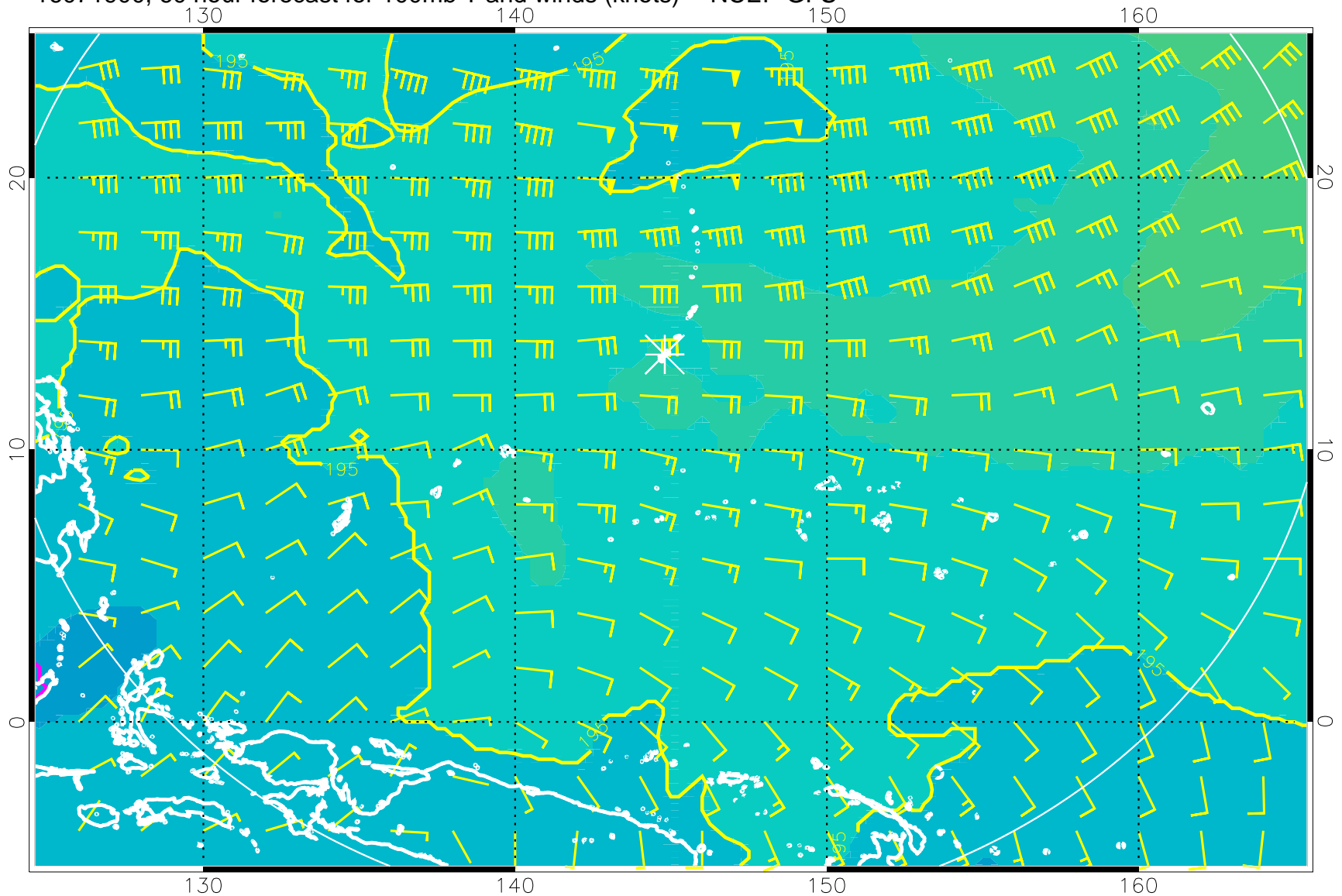
16071900, 60 hour forecast for 100mb T and winds (knots) -- NCEP GFS
