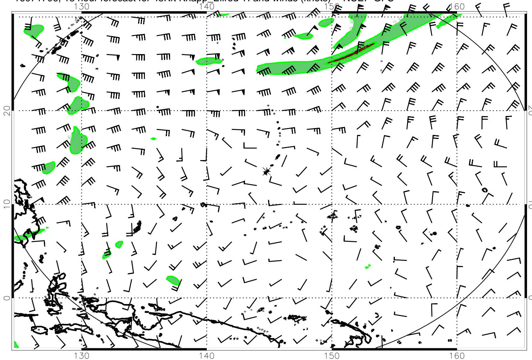
16071706, 18 hour forecast for 45Kft Knapp_Ellrod TI and winds (knots) -- NCEP GFS
