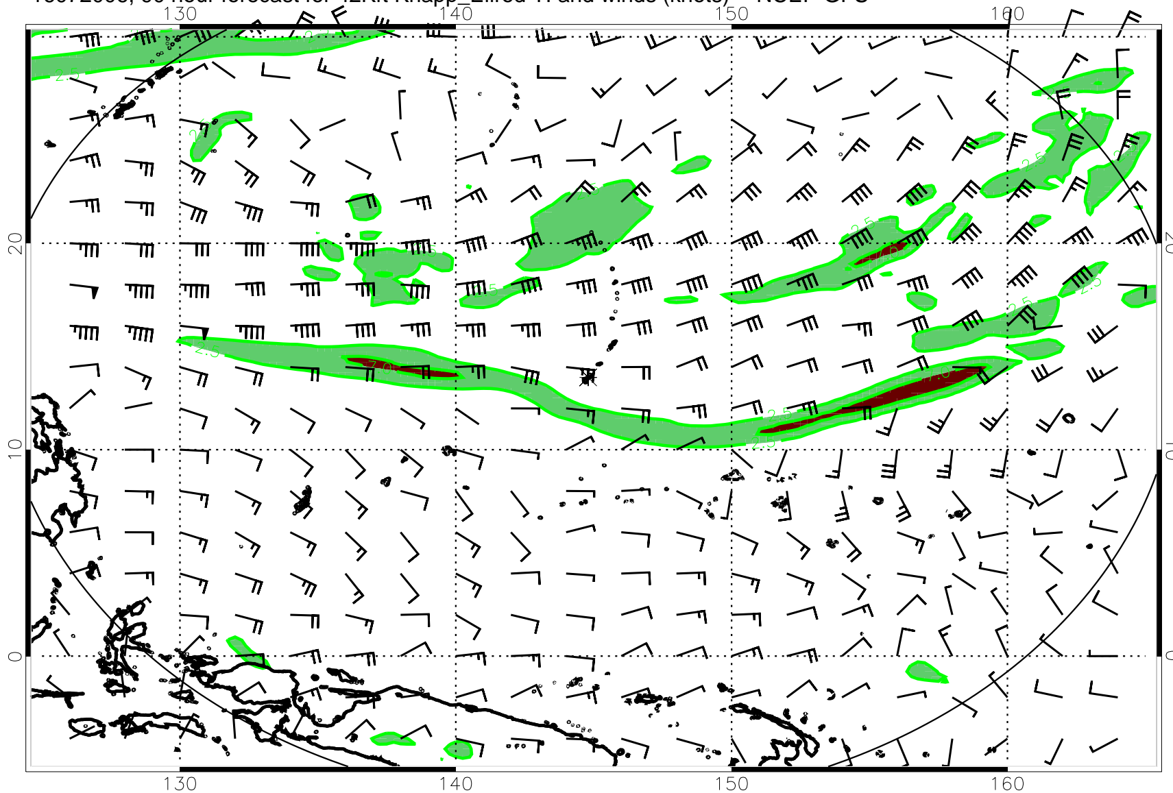
16072006, 90 hour forecast for 42Kft Knapp_Ellrod TI and winds (knots) -- NCEP GFS
