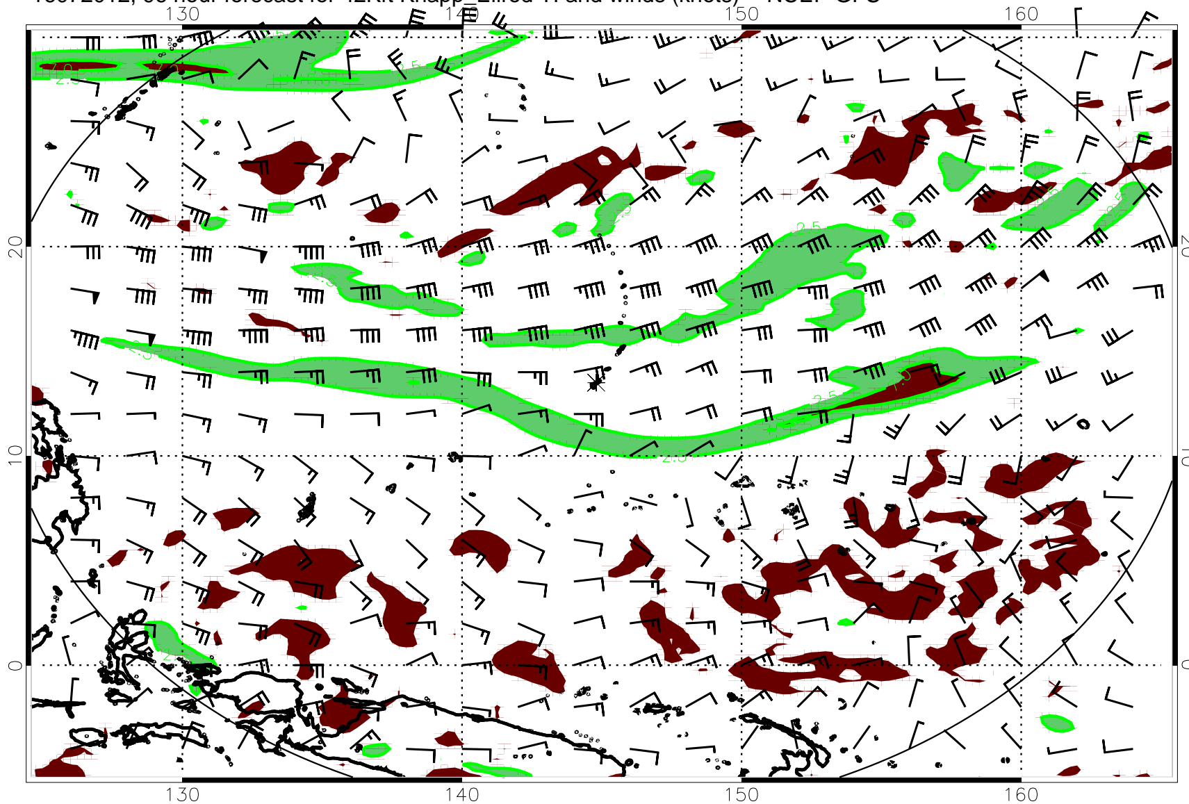
16072012, 96 hour forecast for 42Kft Knapp Ellrod TI and winds (knots) -- NCEP GFS
